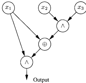
Fig. 12.1 A binary circuit for f(x_1, x_2, x_3) = (x_1 \oplus (x_2 \wedge x_3)) \wedge x_1 .
