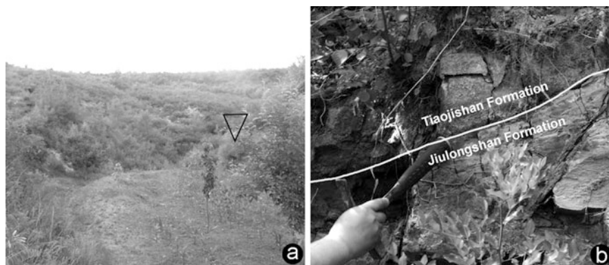
Fig. 4.5 The Jiulongshan Formation. (a) Outcrop of the Jiulongshan Formation (=Haifanggou Formation). (b) Boundary between the Haifanggou Formation and the overlying Tiaojiashan Formation near Sanjiaochengcun in Jinxi, Liaoning, China. Courtesy of Acta Geologica Sinica
