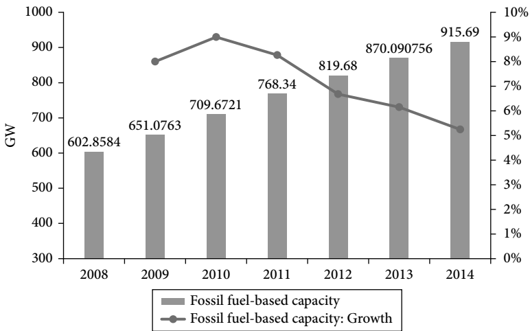
FIGURE 4.4 China: fossil fuel-based power generating capacity and growth 2006–2014
