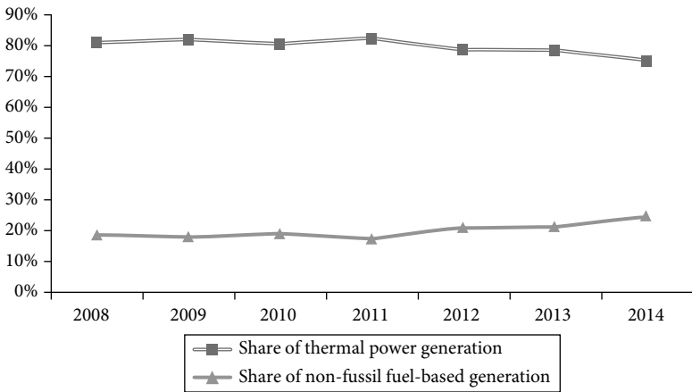
FIGURE 2.8 Shares of electricity generated from fossil fuel sources compared with non-fossil fuel-based electricity generation, 2008–2014
