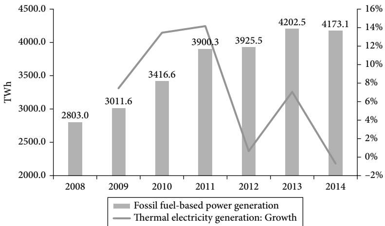
FIGURE 4.2 China: fossil fuel-based power generation and its growth, 2008–2014
