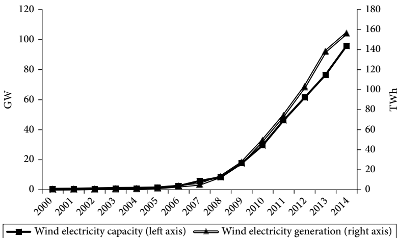
FIGURE 1.2 China's wind power generation, 2000–2014
