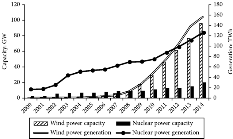
FIGURE 1.3 Electricity generation: wind power vs. nuclear in China
