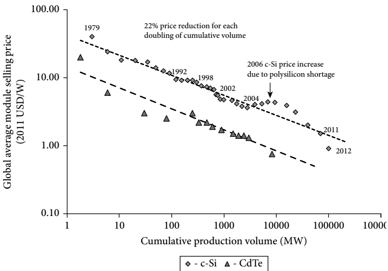
FIGURE 4.10 PV module experience curve, 1976–2013
