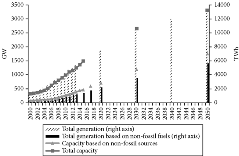
FIGURE 2.9 Projections for electric generation and capacity up to 2050, made by the National Centre of Electric Power Planning and Research 2013
