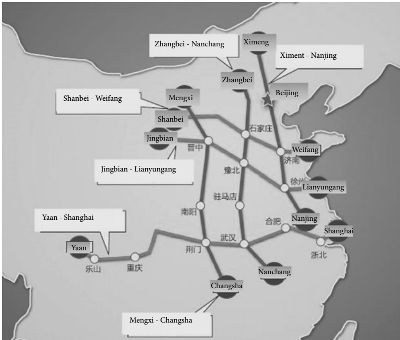
FIGURE 4.7 China's UHV plan for the strong and smart grid
