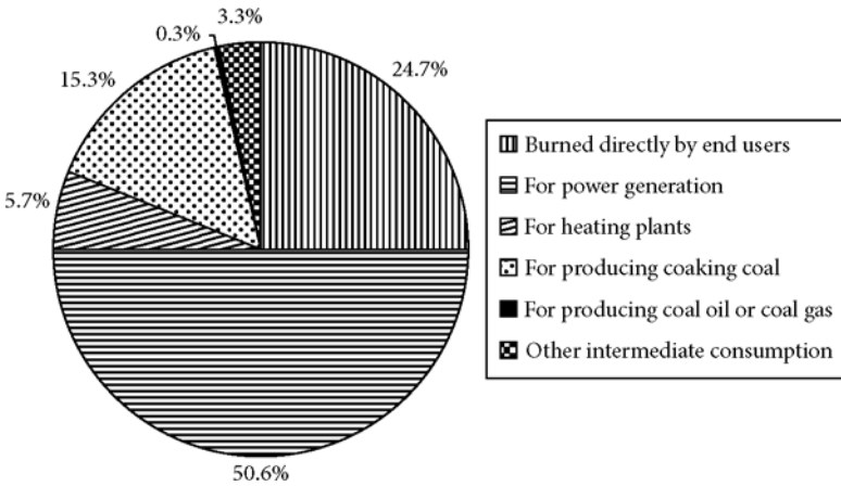
FIGURE 3.4 Coal consumption in China, 2012: where the coal was burnt Source: Authors. Based on data available from the National Statistics Bureau, China.
