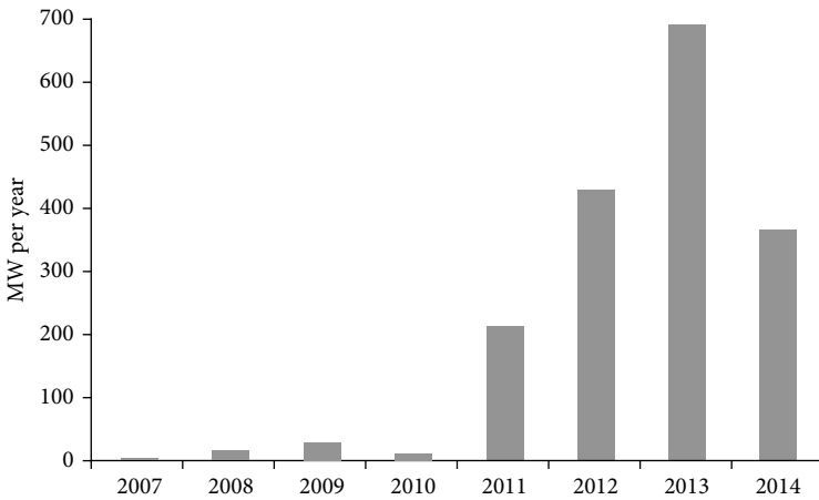
FIGURE 3.8 Exports of Chinese wind turbines: 2007–2014
