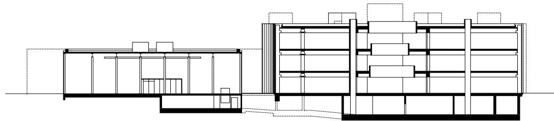
Cross section
