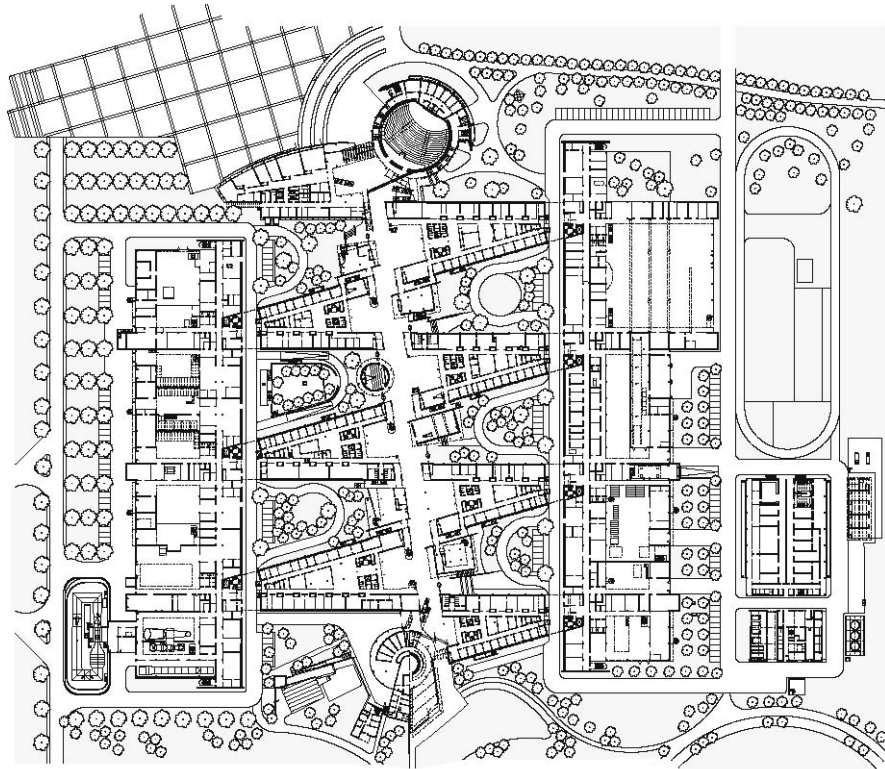
Ground floor plan with landscaping
