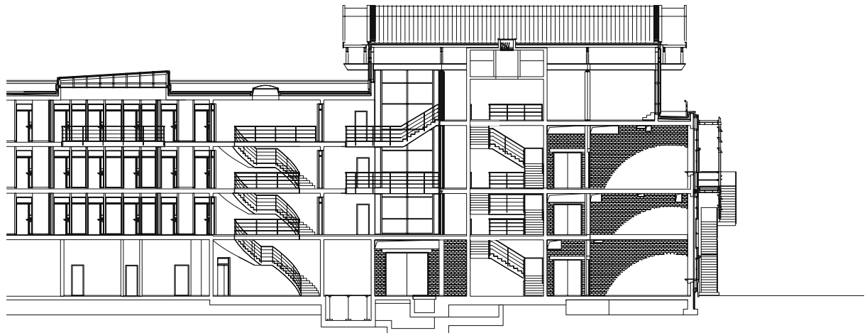
Cross section
