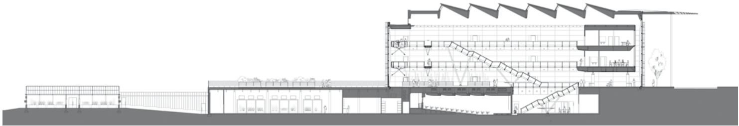
Longitudinal section with greenhouses and plant growth chambers
