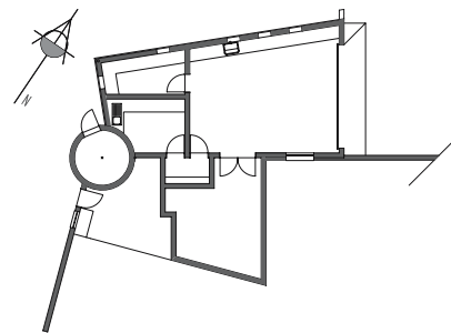
Ground floor plan of entrance tower
