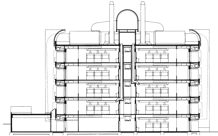
Cross section
