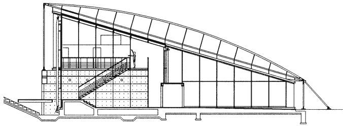
Cross section
