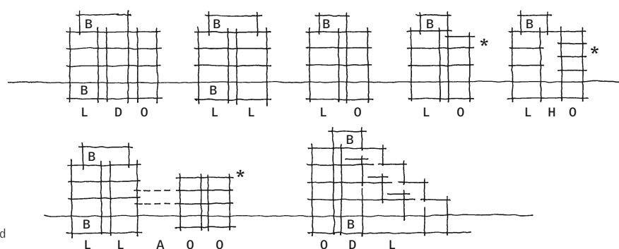
Building structures L - Laboratory O - Office D - Dark zone B - Building service complex A - Atrium or open space * - Office space floor height not adapted to laboratory space floor height
