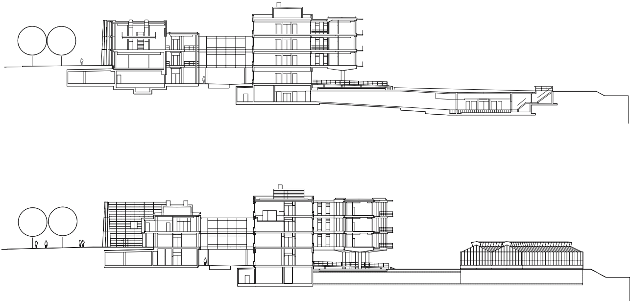
Cross sections
