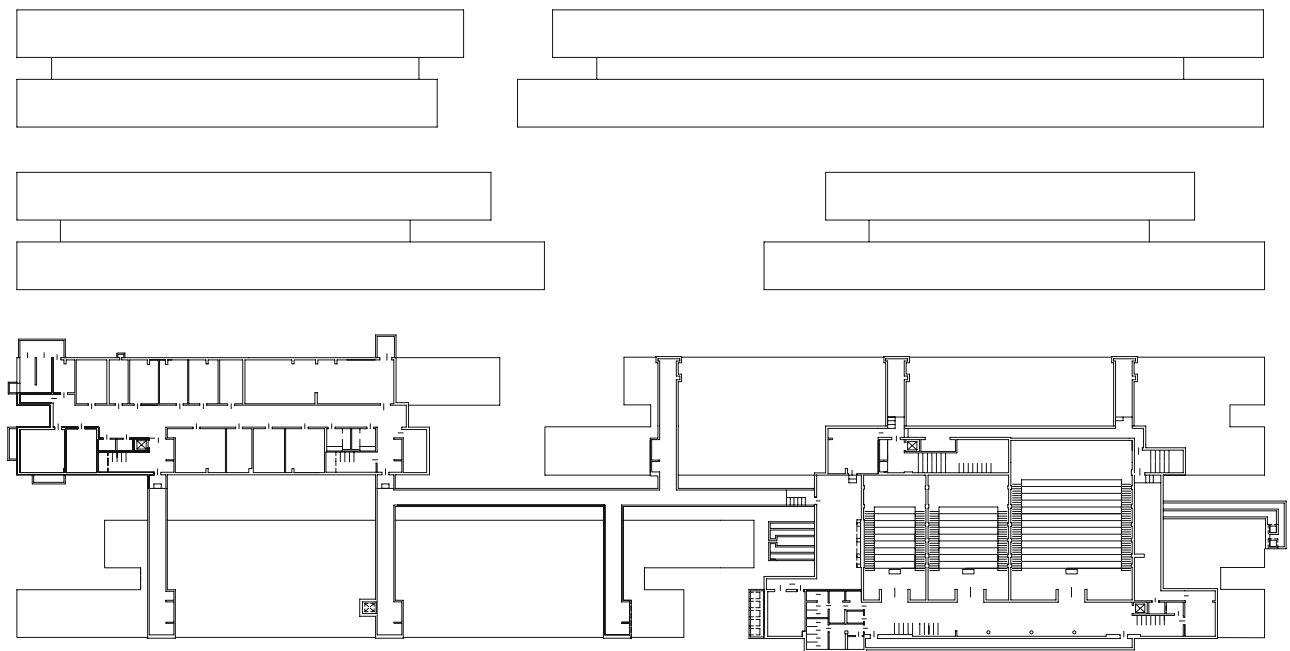
Basement floor plan with auditoriums
