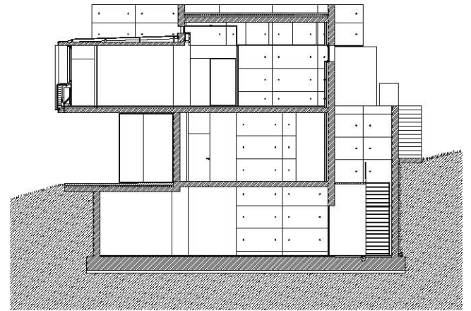
Cross section
