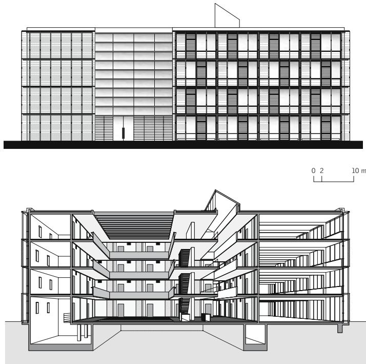
Sectional perspective
