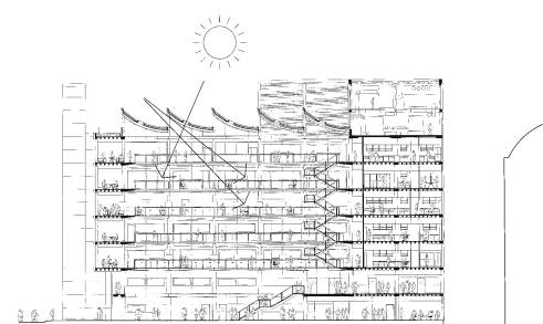
North-south longitudinal section
