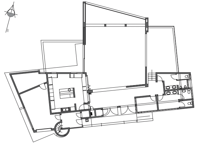
Ground floor plan of multi-purpose building
