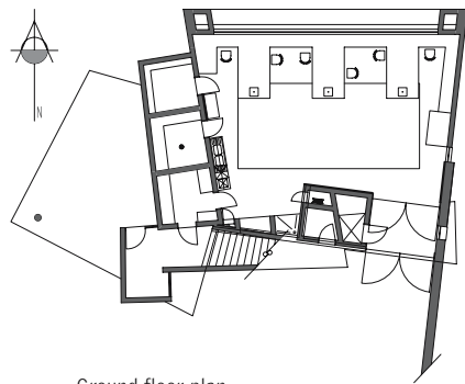
Ground floor plan of laboratory building
