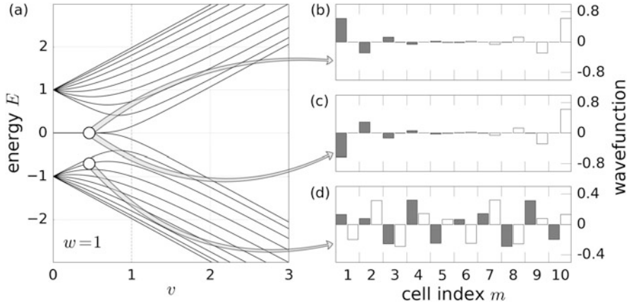
Fig. 1.4 Energy spectrum and wave functions of a finite-sized SSH model. The number of unit cells is N = 10 . (a) Energy spectrum of the system for intercell hopping amplitude w = 1 as a function the intracell hopping amplitude v . v < 1 ( v > 1 ) corresponds to the topological (trivial) phases. (b) and (c) shows the wave functions of the hybridized edge states, while (d) shows a generic bulk wave function
