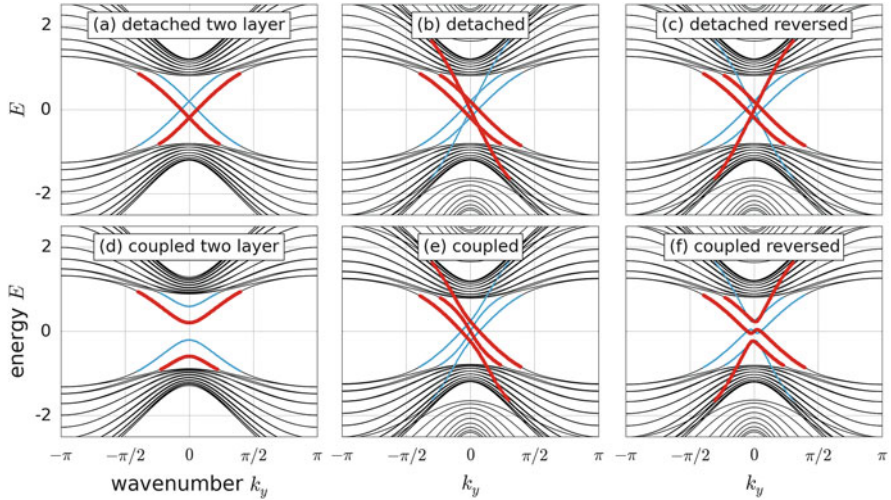
Fig. 6.8 Dispersion relations of strips of multilayered QWZ model, N = 10 unit cells wide. In all cases the bulk Hamiltonian of the first layer \hat{H}_{L1} is the QWZ Hamiltonian with u = -1.2 . To elucidate the interplay of the edge states we consider a finite potential acting on the edge \mu_{L1}^{(1)/(N)} = 0.2/-0.2 . In the left column ((a) and (d)), we have two layers, with bulk \hat{H}_{L2} = -\hat{H}_{L1} and edge onsite potential \mu_{L2}^{(1)/(N)} = \mu_{L1}^{(1)/(N)} . In the middle ((b), (e)) and right ((c), (f)) columns, we have three layers. The third layer is characterized in the bulk by \hat{H}_{L3} = \hat{H}_{L1} and on the edge by \mu_{L3}^{(1)/(N)} = -\mu_{L1}^{(1)/(N)} . In (b) and (e) \hat{H}_{L2} = 2\hat{H}_{L1} , while in (d) and (e) \hat{H}_{L2} = -2\hat{H}_{L1} . For all four cases \mu_{L2}^{(1)/(N)} = 0 . Coupling in (d), (e) and (f) is uniform with magnitude C = 0.4
