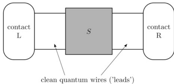
Fig. 10.2 Simple model of a phase-coherent conductor in the presence of scatterers. The ideal contacts L and R are connected via ideal leads to the disordered region represented by the scattering matrix S
