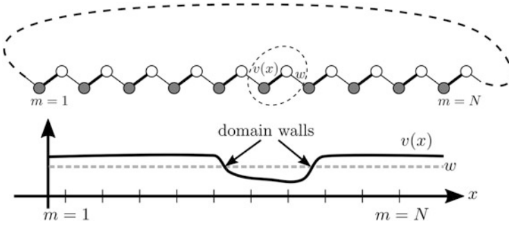
Fig. 7.2 Inhomogeneous intracell hopping and domain walls in the SSH model. The dashed ellipse denotes the unit cell. The dashed line connecting the edges of the chain denotes the periodic boundary condition
