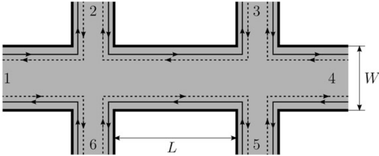
Fig. 10.6 HgTe quantum well patterned in the Hall-bar geometry (gray area). Numbered terminals lead to metallic contacts. Solid and dashed lines depict counterpropagating edge states
