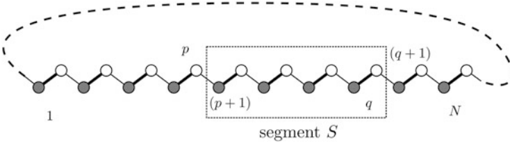
Fig. 5.1 A segment enclosed by two cross sections in the one-dimensional SSH model. The segment S is defined as the part of the chain between the p th and (q + 1) th unit cells. The current operators corresponding to the two cross sections can be established by considering the temporal change of the number of particles in the segment. The dashed line represents the periodic boundary condition
