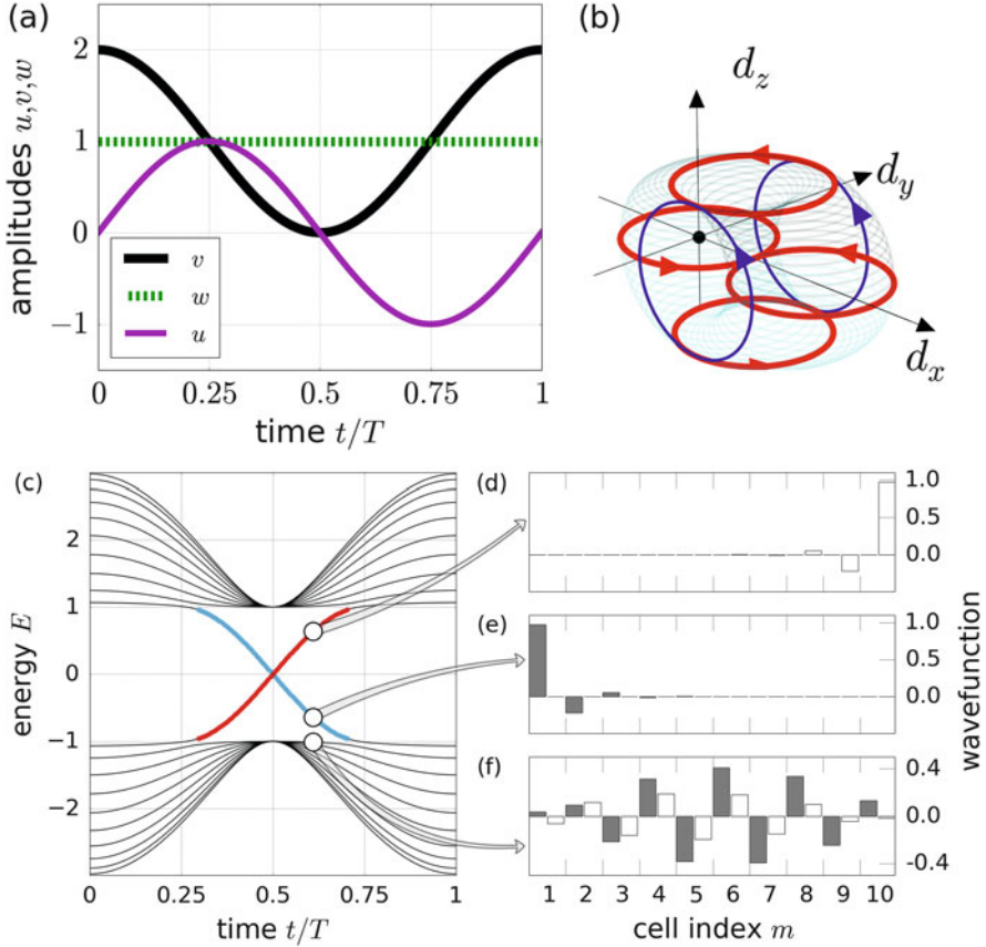
Fig. 4.3 The smooth pump sequence of the Rice-Mele model for \bar{v} = 1 . The hopping amplitudes and the sublattice potential (a) are varied smoothly as a function of time. The vector \mathbf{d}(k, t) corresponding to the bulk momentum-space Hamiltonian (b) traces out a torus in the 3-dimensional space. Instantaneous spectrum of the Hamiltonian \hat{H}(t) on an open chain of N = 10 sites (c) reveals that during a cycle, one state crosses over to the upper band on the right edge, and one to the lower band on the left edge (dark red/light blue highlights energies of edge states, whose wavefunctions have than 60 % weight on the rightmost/leftmost 2 unit cells). The wavefunctions of the edge states (d,e) are exponentially localized to one edge and have support overwhelmingly on one sublattice each. In contrast a typical bulk state (f) has a delocalized wavefunction with support on both sublattices
