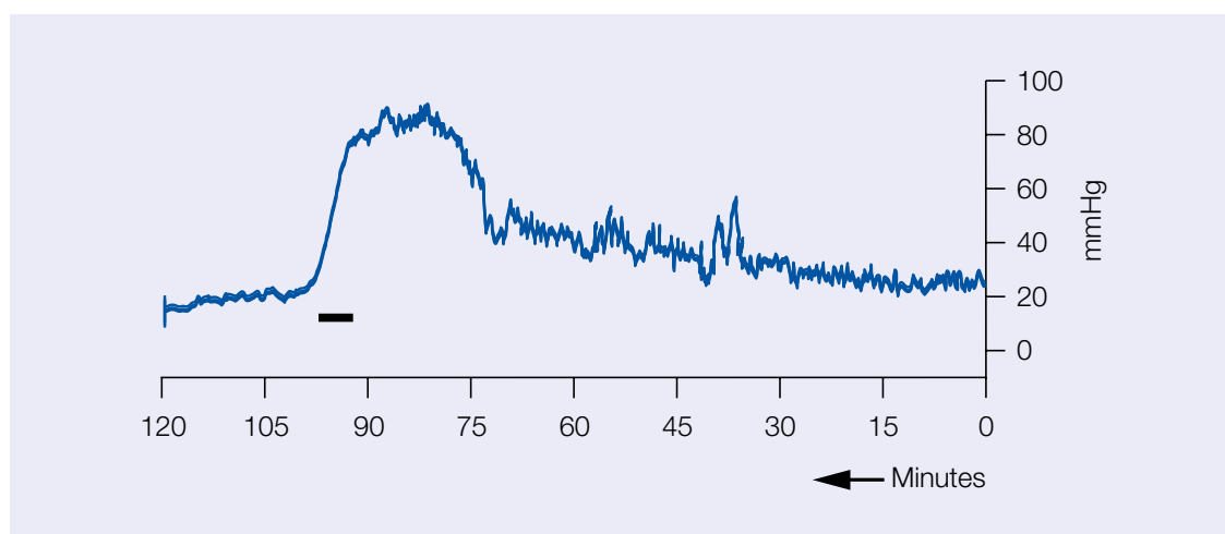
Fig. 4-2. Continuous modification of intracranial pressure at the bedside in a patient with severe traumatic brain injury from the seminal work of Lundberg et al . The curve, recorded 24 hours after accident, shows the basic level of intracranial pressure to be slightly above normal (high by contemporary standards). This is followed by a sudden spontaneous rise to an extremely high level (about 90 mmHg) and after about 20 minutes a rapid fall in pressure. The increase in pressure was accompanied by tonic extension of the limbs and cardiovascular disturbances; these symptoms disappeared at once when the ventricular fluid pressure decreased. The horizontal bar indicates intravenous administration of urea. The small rhythmic oscillations of the pressure curve (1-per-min waves) were related to the Cheyne-Stokes breathing of the patient
