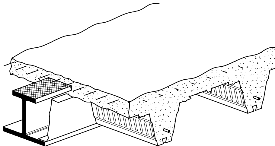
Figure 4.4 Slimdek construction
