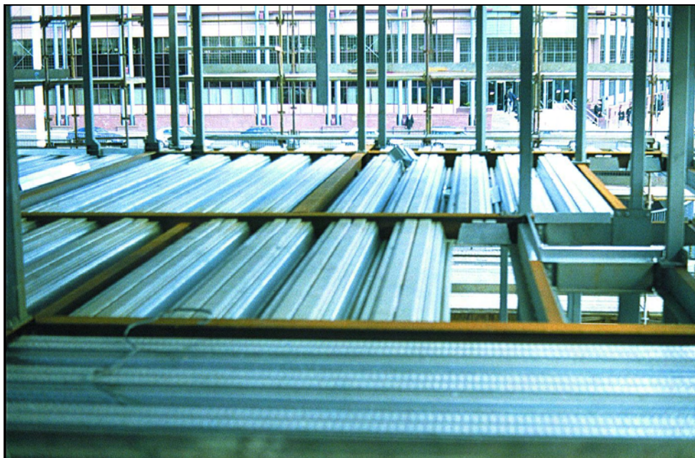
Figure 4.5 Slimdek and SHS columns used in a residential building
