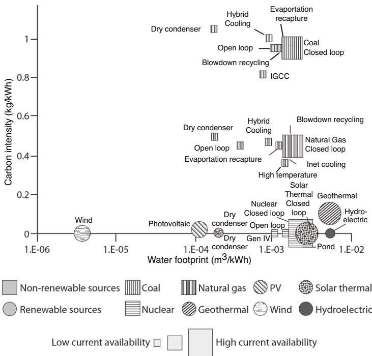
Figure 20 Effects of emerging technologies on carbon and water intensity of electricity sources (World Bank, 2011)
