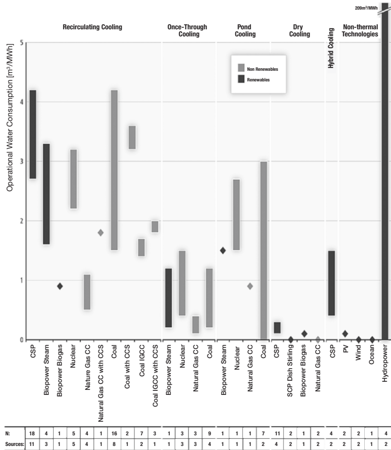
Figure 12 Ranges of rates of operational water consumption by thermal and non-thermal electricity-generating technologies based on a review of available literature (m³/MWh). Bars represent absolute ranges from available literature, diamonds single estimates; n represents the number of estimates reported in the sources. Note that upper values for hydropower result from few studies measuring gross evaporation values, and may not be representative
