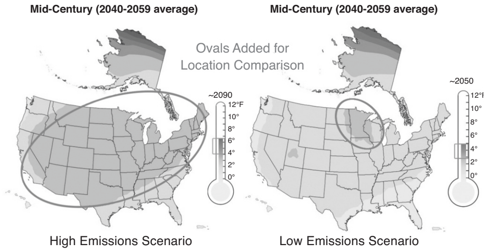
Figure 3 USGCRP: Potential temperature increases
