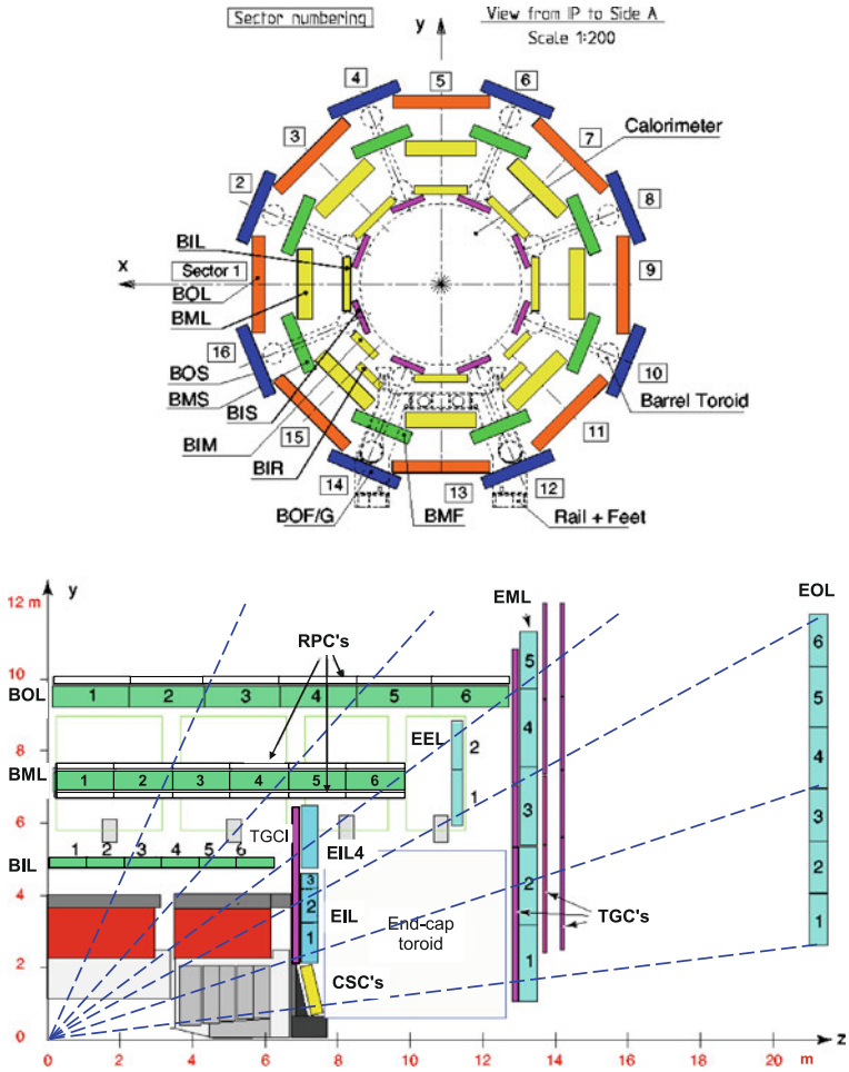
Fig. 3.10 A schematic diagram showing a cross section through the ATLAS muon system in both the transverse plane ( top ) and the r - z bending plane ( bottom ), showing the arrangement of the different tracking and triggering chambers. Images from Ref. [2]
