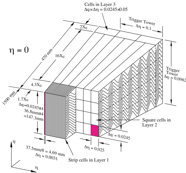
Fig. 3.7 A schematic diagram showing a slice through a barrel module of the ATLAS LAr EM calorimeter. Image from Ref. [2]
