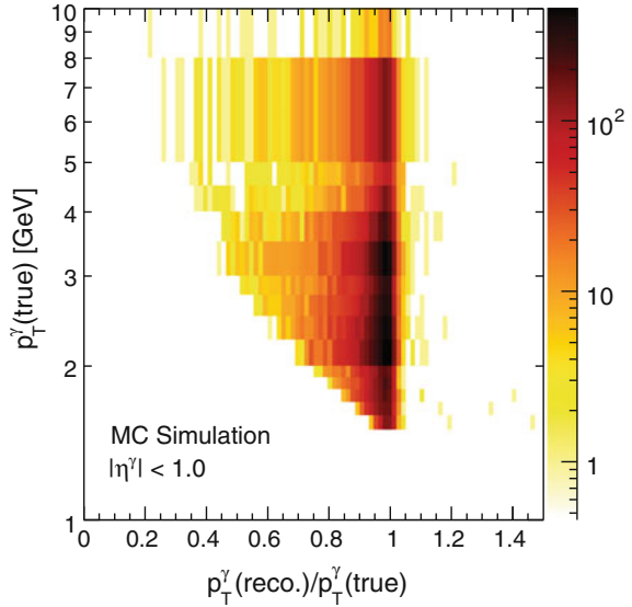
Fig. 6.12 The effective experimental resolution in p_T^\gamma (parametrised as the ratio of reconstructed p_T^\gamma to true p_T^\gamma ) as a function of the true value of p_T^\gamma . The fiducial cut p_T^\gamma > 1.5 GeV is applied to the reconstructed value of p_T^\gamma
