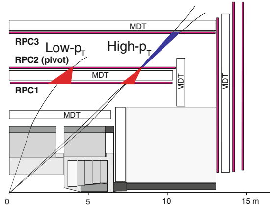
Fig. 4.10 A schematic diagram of the ATLAS muon trigger detectors. The diagram shows two examples of low p_T trigger roads (red) between the first and second stations and a high p_T extension road (blue) between the second and third stations. Image from Ref. [5]
