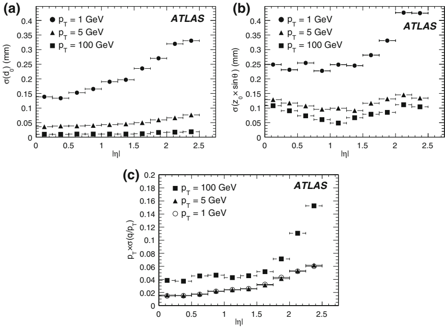
Fig. 4.2 The resolutions of the track parameters a d_0 , b z_0 \cdot \sin(\theta) and c q/p_T (bottom) as functions of |\eta| , determined from MC simulation, for muon tracks with various transverse momenta. Figures taken from Ref. [2]
