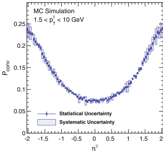
Fig. 6.10 The conversion probability, derived from MC simulation, for photons with p_T^\gamma > 1.5 GeV as a function of \eta^\gamma . The method used to estimate of the systematic uncertainty is discussed in Sect. 6.8
