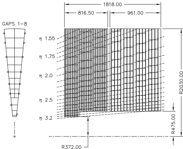
Fig. 3.8 A schematic diagram showing the segmentation in r \times \phi (left) and r \times z (right) of the Hadronic Endcap (HEC) calorimeter. Image from Ref. [2]
