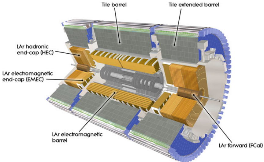
Fig. 3.6 A schematic diagram of the ATLAS calorimeter systems [2]. Image © CERN
