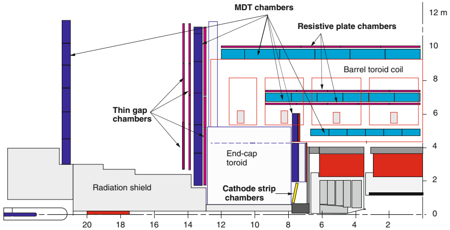
Fig. 4.4 A schematic diagram of the ATLAS muon system showing the three stations of tracking and trigger detectors. Image from Ref. [2]
