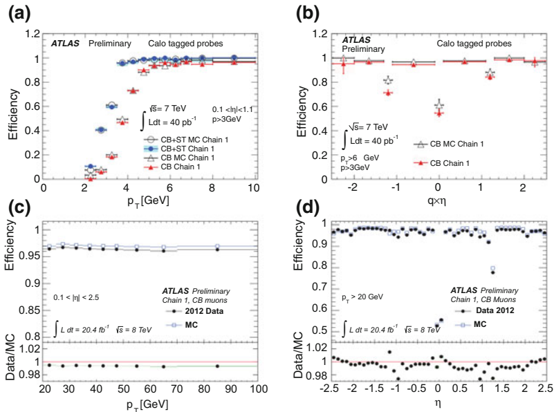
Fig. 4.5 The reconstruction efficiency for muons reconstructed with the combined (CB) approach and Staco algorithm (denoted chain 1). The efficiency is measured in data with J/\psi \rightarrow \mu^+\mu^- events (a and b) and Z \rightarrow \mu^+\mu^- events (c and d) and is compared to that derived in MC simulation. Figures taken from Refs. [6, 7]
