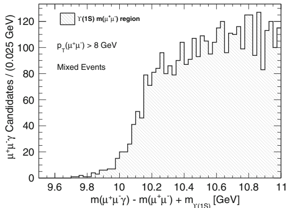
Fig. 5.4 The mass difference m(\mu^+\mu^-\gamma) - m(\mu^+\mu^-) + m_{\Upsilon(1S)} distribution for a sample of mixed data events. This sample is built by associating data events which satisfy the \Upsilon(1S) selection with photon information from the previous event
