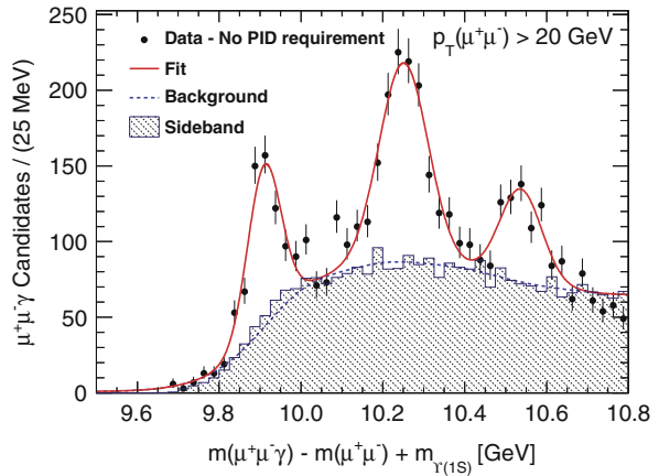
Fig. 5.9 Fit to m(\mu^+\mu^-\gamma) - m(\mu^+\mu^-) + m_{\Upsilon(1S)} distribution for \chi_b(nP) \rightarrow \Upsilon(1S)\gamma candidates with no “loose” photon identification requirement imposed. The fit procedure is identical to the nominal fit but an alternative background PDF is used, derived by performing the Gaussian kernel estimation procedure on the “low mass” sideband distribution [17]
