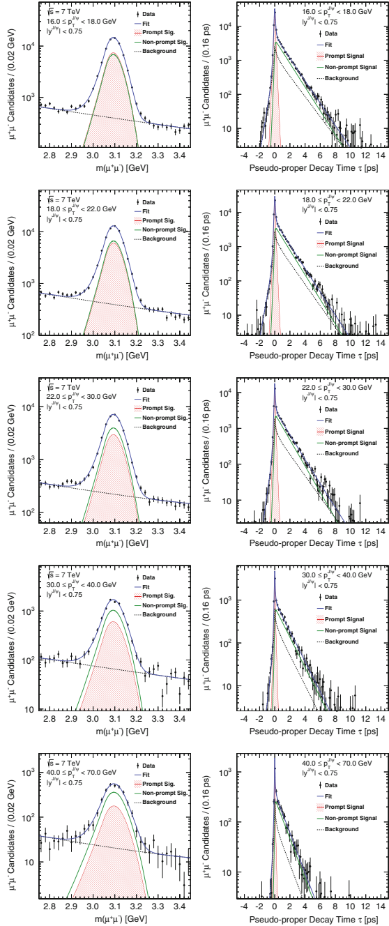
Fig. 6.37 Simultaneous fits to the di-muon invariant mass, m(\mu^+\mu^-) , and pseudo-proper decay time, \tau , distributions of J/\psi \rightarrow \mu^+\mu^- candidates in five bins of p_T^{J/\psi} within 16 < p_T^{J/\psi} < 70 GeV
