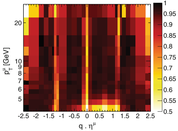
Fig. 6.9 The muon identification efficiency as a function of reconstructed muon transverse momentum p_T^\mu and charge-signed pseudorapidity q \cdot \eta^\mu . The efficiency map is determined using the tag-and-probe method from a sample of J/\psi \rightarrow \mu^+ \mu^- decays in data [19]
