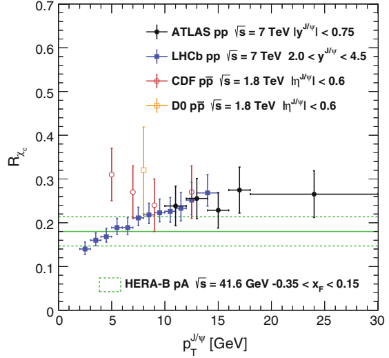
Fig. 6.33 A comparison of R_{\chi_c} measurements from hadron collider and fixed target experiments. The results presented here are denoted ATLAS and are compared to the measurements of LHCb [22], CDF [10], D0 [11] and HERA-B [43]. x_F denotes the Feynman longitudinal momentum fraction
