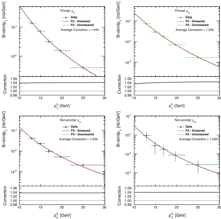
Fig. 6.22 Measured p_T^{\chi_c} distributions for prompt and non-prompt \chi_{c1} and \chi_{c2} , fitted with an analytical function convolved with a resolution function ( solid grey line ). The de-convolved function is shown as the red dashed line . The bin migration corrections are shown in the panels below the fitted p_T^{\chi_c} distributions
