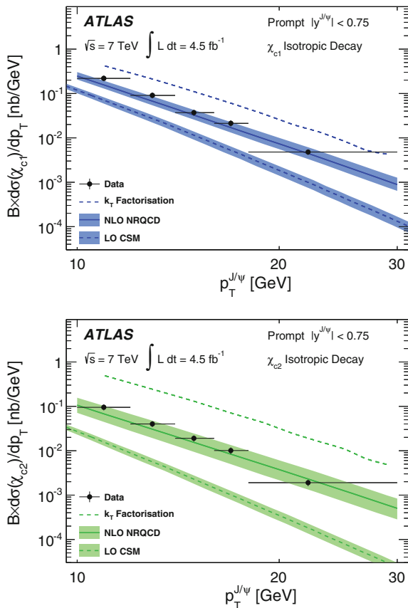
Fig. 6.26 Differential cross sections for prompt \chi_{c1} (top) and \chi_{c2} (bottom) measured as a function of p_T^{J/\psi} . The measurements are compared to the predictions of NLO NRQCD [34, 35], the CSM [37] and the k_T factorisation approach [38, 39]. The positions of the data points within each bin reflect the average p_T^{J/\psi} of the \chi_c candidates within the bin. The error bars represent the total uncertainty on the measurement (statistical and systematic), assuming isotropic decay angular distributions (in some cases, the error bar is smaller than the data point)
