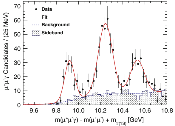
Fig. 5.8 An alternative fit to the m(\mu^+\mu^-\gamma) - m(\mu^+\mu^-) + m_{\Upsilon(1S)} distribution for \chi_b(nP) \rightarrow \Upsilon(1S)\gamma candidates. The alternative background PDF is derived by performing the Gaussian kernel estimation procedure on the “low mass” sideband distribution [17], as discussed in Sect. 5.6
