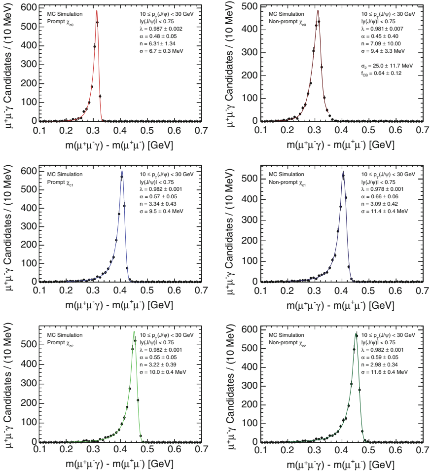
Fig. 6.17 \Delta m distributions for simulated prompt and non-prompt \chi_{cJ} events, each fitted with a Crystal Ball function
