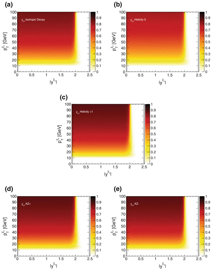
Fig. 6.4 Acceptance maps binned in p_T^{\chi_c} and |y^{\chi_c}| for \chi_{c1} \rightarrow J/\psi\gamma \rightarrow \mu^+\mu^-\gamma decays, calculated for each of the polarisation scenarios considered. a Isotropic, b Helicity 0, c Helicity \pm 1 , d AZ+, e AZ–
