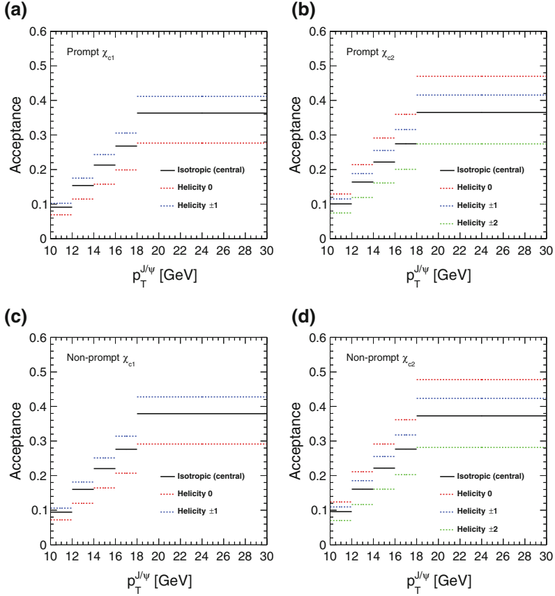
Fig. 6.6 Acceptance corrections binned in p_T^{J/\psi} for \chi_{c1} (a, c) and \chi_{c2} (b, d), for isotropic decay angular distributions ( central value ) and for the helicity 0, \pm 1 , \pm 2 scenarios. The scenarios which include azimuthal anisotropy ( AZ_{\pm} ) are not shown, as for \chi_{c1} they closely follow the helicity \pm 1 scenarios while for \chi_{c2} they closely follow the isotropic central values
