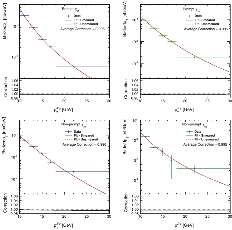
Fig. 6.23 Measured p_T^{J/\psi} distributions for prompt and non-prompt \chi_{c1} and \chi_{c2} , fitted with an analytical function convolved with a resolution function ( solid grey line ). The de-convolved function is shown as the red dashed line . The bin migration corrections are shown in the panels below the fitted p_T^{J/\psi} distributions
