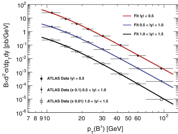
Fig. 6.42 Fitted B^\pm production differential cross sections, in three B^\pm rapidity intervals. Data points from Ref. [47] and B = \mathcal{B}(B^\pm \rightarrow J/\psi K^\pm) . \mathcal{B}(J/\psi \rightarrow \mu^+ \mu^-)
