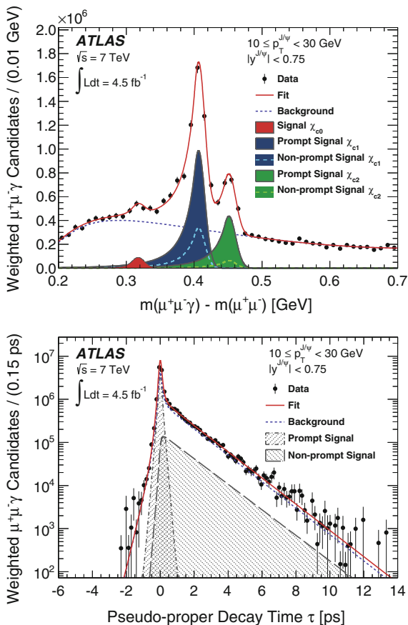
Fig. 6.18 The \Delta m and \tau projections of a simultaneous unbinned maximum likelihood fit performed to the inclusive sample of reconstructed \chi_{cJ} decays ( 10 \leq p_T^{J/\psi} < 30 GeV), weighted with the prompt \chi_{c1} acceptance correction
