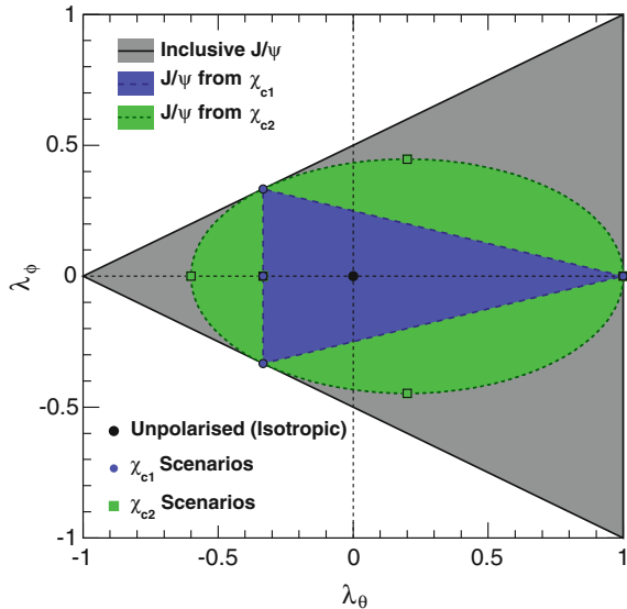
Fig. 6.3 The allowed values of the \lambda_\theta and \lambda_\phi coefficients for inclusive J/\psi production (grey) and for J/\psi produced in radiative \chi_{c1} (blue) and \chi_{c2} (green) decays. Information is taken from Ref. [21]
