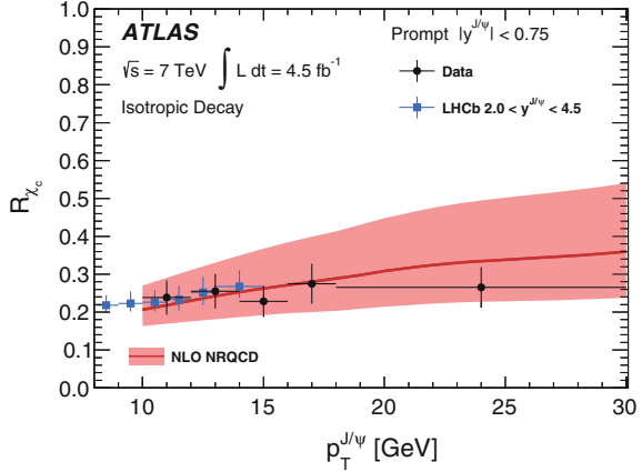
Fig. 6.29 The fraction of prompt J/\psi produced in feed-down from radiative \chi_{cJ} decays, measured as a function of p_T^{J/\psi} . The measurements are compared to the predictions of NLO NRQCD [34, 35] and the measurement of LHCb [22]. The error bars represent the total uncertainty on the measurement (statistical and systematic), assuming isotropic decay angular distributions
