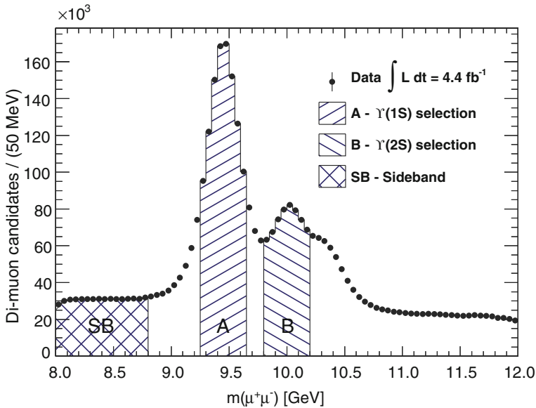
Fig. 5.1 The invariant mass m(\mu^+\mu^-) distribution of \Upsilon(mS) \rightarrow \mu^+\mu^- candidates satisfying the criteria described in Sect. 5.2.2. Regions A and B show the invariant mass selection criteria for \Upsilon(1S) \rightarrow \mu^+\mu^- and \Upsilon(2S) \rightarrow \mu^+\mu^- candidates respectively. The region denoted SB shows the “low mass” sideband
