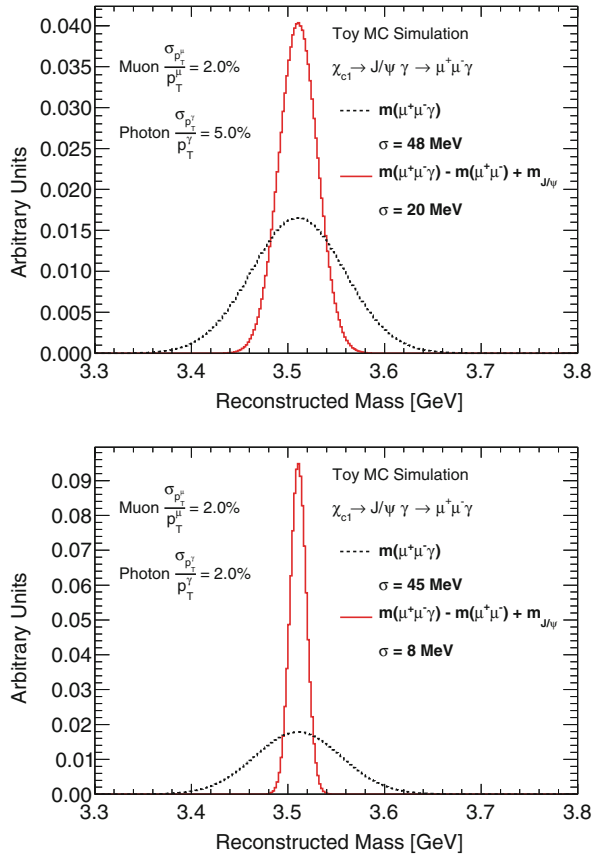
Fig. 4.12 A demonstration of the resolution improvement gained with mass difference technique in simulated \chi_{c1} \rightarrow J/\psi \gamma \rightarrow \mu^+ \mu^- \gamma events. The simulation result in the upper figure is processed with a photon transverse momentum resolution of 5% (a figure comparable to that achievable with the ATLAS calorimeter) while the lower figure is processed with a photon transverse momentum resolution of 2% (a figure comparable to that achievable through the reconstruction of photon conversions in the ATLAS ID)
