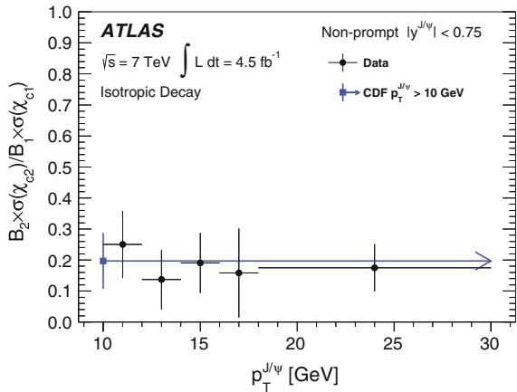
Fig. 6.31 The cross section of non-prompt \chi_{c2} relative to non-prompt \chi_{c1} , measured as a function of p_T^{J/\psi} . The measurements are compared to that of CDF in p\bar{p} collisions at \sqrt{s} = 1.96 TeV [12]. The error bars represent the total uncertainty on the measurement (statistical and systematic), assuming isotropic decay angular distributions
