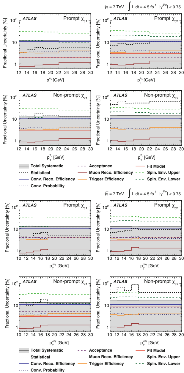
Fig. 6.24 The individual contributions to the systematic uncertainty on the cross-section measurements binned in p_T^{\chi_c} ( top ) and p_T^{J/\psi} ( bottom ). The common contributions of integrated luminosity (1.8%) and track reconstruction (1%) are not shown. The lines denoted Spin. Env. represent the upper and lower bounds of the polarisation envelope (not included in the total systematic uncertainty)
