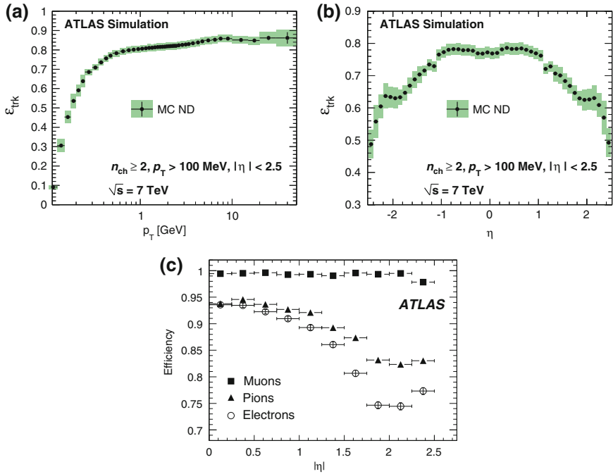
Fig. 4.3 The track reconstruction efficiency for charged particles as a function of p_T (a) and \eta (b) for charged particles produced in non-diffractive (ND) minimum bias events in MC simulation [4]. The track reconstruction efficiency as a function of |\eta| for three charged particle species (c) with transverse momentum p_T = 5 GeV, derived from simulation [2]
