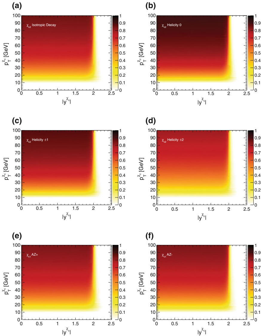
Fig. 6.5 Acceptance maps binned in p_T^{\chi_c} and |y^{\chi_c}| for \chi_{c2} \rightarrow J/\psi\gamma \rightarrow \mu^+\mu^-\gamma decays, calculated for each of the polarisation scenarios considered. a Isotropic, b Helicity 0, c Helicity \pm 1 , d Helicity \pm 2 , e AZ+, f AZ–
