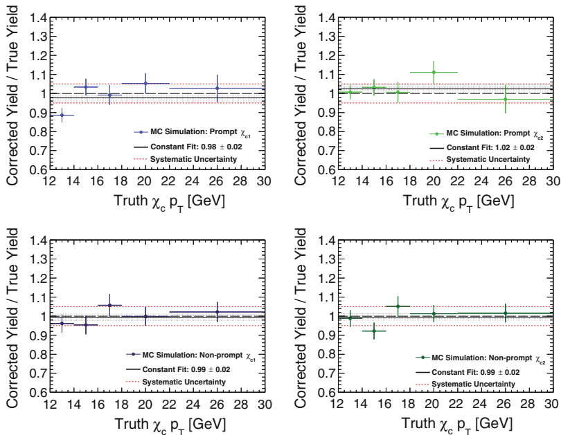
Fig. 6.15 The efficiency corrected number of reconstructed simulated \chi_{cJ} \rightarrow J/\psi \gamma decays divided by the true number of \chi_{cJ} \rightarrow J/\psi \gamma decays, measured in bins of p_T^{\chi_c} . The systematic uncertainty on the method ( \pm 5\% ) derived from toy simulations is also shown as the dashed red line
