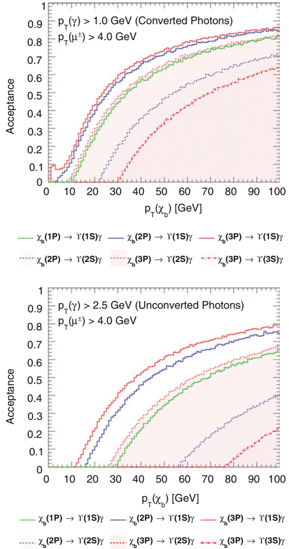
Fig. 5.12 The kinematic acceptance of \chi_b(nP) \rightarrow \Upsilon(mS)\gamma decays reconstructed with converted ( upper ) and unconverted ( lower ) photons. The kinematic acceptance for \chi_b(nP) \rightarrow \Upsilon(mS)\gamma decays reconstructed with converted photons is significantly greater than for unconverted photons, for a given \chi_b transverse momentum
