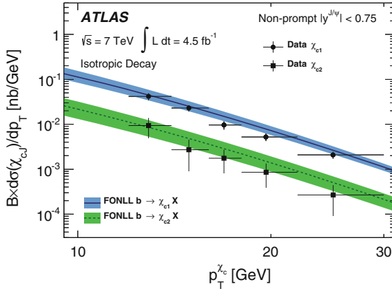
Fig. 6.27 Differential cross sections for non-prompt \chi_{c1} (blue) and \chi_{c2} (green) measured as a function of p_T^{\chi_c} . The measurements are compared to the predictions of a theoretical prediction based on the FONLL model of b hadron production [40]. The positions of the data points within each bin reflect the average p_T^{\chi_c} of the \chi_c candidates within the bin. The error bars represent the total uncertainty on the measurement (statistical and systematic), assuming isotropic decay angular distributions
