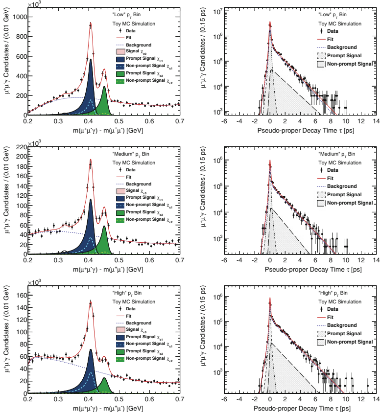
Fig. B.1 Simultaneous fits to m(\mu^+\mu^-\gamma) - m(\mu^+\mu^-) and \tau distributions generated using the toy MC method. Pseudo-data are generated in three characteristic p_T bins; “Low” p_T (top), “Medium” p_T (middle) and “High” p_T (bottom)
