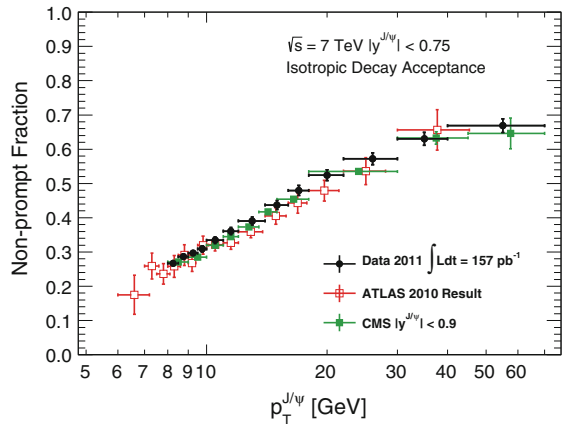
Fig. 6.40 The fraction of J/\psi produced in the decay of b -hadrons, f_{\text{non-prompt}} , measured as a function of p_T^{J/\psi} , in pp collisions at \sqrt{s} = 7 TeV. The black points show the measurements of this analysis, while the red points show the reference measurements from [17]. The measurements of CMS, within the region |y^{J/\psi}| < 0.9 , are also shown by the green data points [23]
