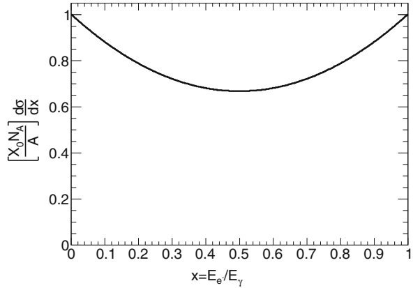
Fig. 4.7 The differential cross section for photon conversion, normalised by a material dependent pre-factor, as a function of the energy sharing parameter x . Information from [8]
