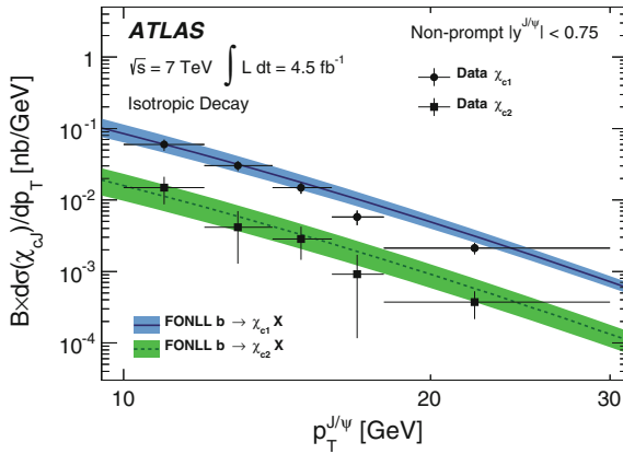
Fig. 6.28 Differential cross sections for non-prompt \chi_{c1} (blue) and \chi_{c2} (green) measured as a function of p_T^{J/\psi} . The measurements are compared to the predictions of a theoretical prediction based on the FONLL model of b hadron production [40]. The positions of the data points within each bin reflect the average p_T^{J/\psi} of the \chi_c candidates within the bin. The error bars represent the total uncertainty on the measurement (statistical and systematic), assuming isotropic decay angular distributions
