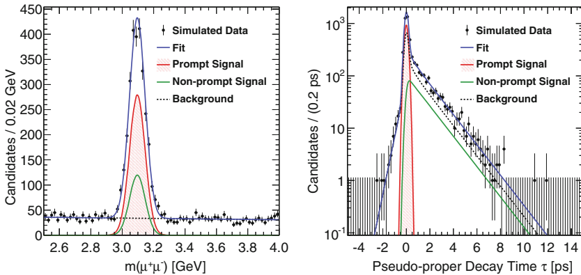
Fig. 4.13 A demonstration of a simultaneous fit to the invariant mass and pseudo-proper decay time distributions of reconstructed charmonium states ( J/\psi \rightarrow \mu^+\mu^- in this example). The prompt (red and shaded) and non-prompt (green) yields of the charmonium state can be simultaneously determined by exploiting the discriminating power of the pseudo-proper decay time distribution
