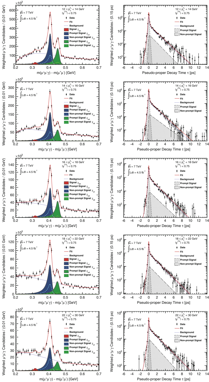
Fig. 6.20 The \Delta m and \tau projections of a simultaneous unbinned maximum likelihood fit performed to reconstructed \chi_{cJ} decays in bins of p_T^{c} . The data are weighted with the prompt \chi_{c1} acceptance correction
