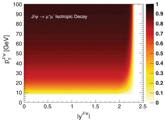
Fig. 6.34 Acceptance map for J/\psi \rightarrow \mu^+\mu^- decays binned in p_T^{J/\psi} and |y^{J/\psi}| , to correct for the fiducial cuts p_T^\mu > 4 GeV and |\eta^\mu| < 2.3
