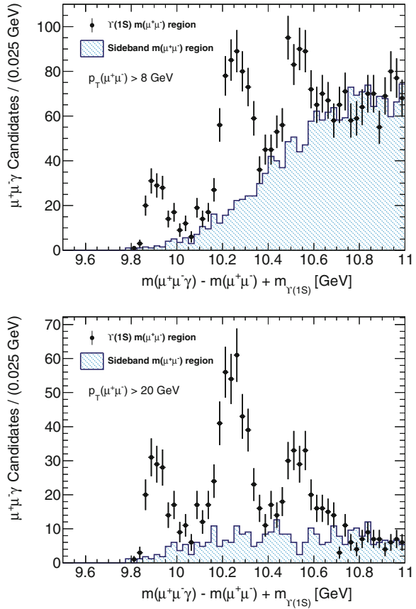
Fig. 5.2 The m(\mu^+\mu^-\gamma) - m(\mu^+\mu^-) + m_{\Upsilon(1S)} distributions for \chi_{bJ}(nP) \rightarrow \Upsilon(1S)\gamma candidates reconstructed with unconverted photons. The same distributions for \mu^+\mu^-\gamma candidates with a di-muon invariant mass within the “low mass” sideband region is overlaid and normalised to the same number of events as the \chi_b candidate distribution in the region above 10.7 GeV. The \mu^+\mu^-\gamma candidates in the lower plot are required to have a di-muon transverse momentum p_T^{\mu^+\mu^-} > 20 GeV
