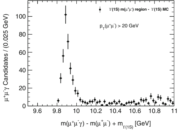
Fig. 5.6 The mass difference m(\mu^+\mu^-\gamma) - m(\mu^+\mu^-) + m_{\Upsilon(1S)} distribution for a sample of simulated \chi_b(1P) \rightarrow \Upsilon(1S)\gamma events. The peak in the distribution corresponds to \chi_b(1P) \rightarrow \Upsilon(1S)\gamma . Neglecting this mass peak, no further mass peaks similar to those observed in data are present
