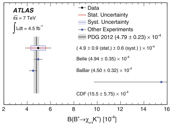
Fig. 6.44 The measured value of \mathcal{B}(B^\pm \rightarrow \chi_{c1} K^\pm) compared to the world average and the measurements of Belle, BaBar and CDF [4, 45, 46, 50]
