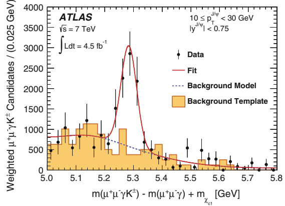
Fig. 6.43 The results of weighted unbinned maximum likelihood fits to the \tilde{m}_{\chi_{c1}} (top) and \tilde{m}_{J/\psi} (bottom) distributions of reconstructed B^\pm \rightarrow \chi_{c1} K^\pm and B^\pm \rightarrow J/\psi K^\pm decays, respectively
