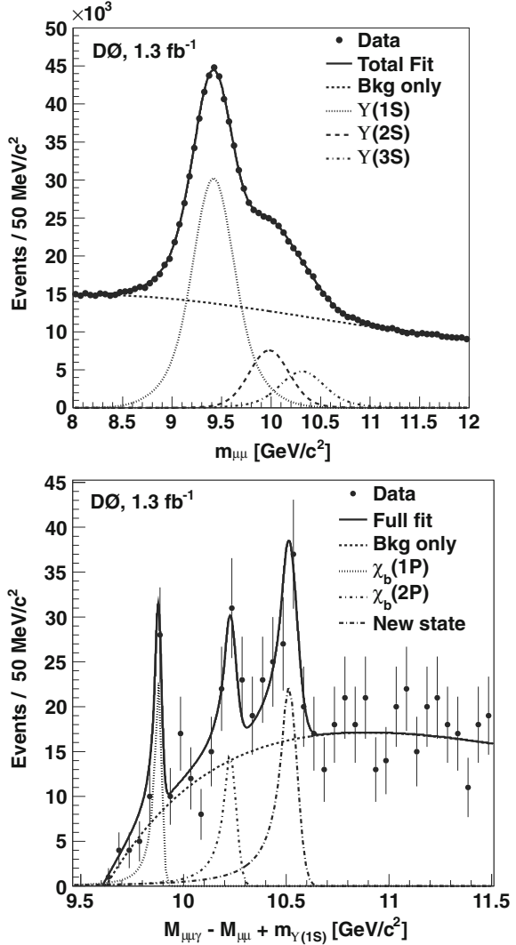
Fig. 5.13 The di-muon invariant mass distribution of \Upsilon(nS) \rightarrow \mu^+\mu^- candidates reconstructed by the D0 experiment [22] ( upper ). The mass difference distribution M_{\mu^+\mu^-\gamma} - M_{\mu^+\mu^-} + M_{\Upsilon(1S)} of \chi_b \rightarrow \Upsilon(1S)\gamma candidates reconstructed by D0 [22] ( lower ). Mass peaks corresponding to the \chi_b(1P) and \chi_b(2P) states, along with the new higher mass state, compatible with the \chi_b(3P) candidate observed by ATLAS, are visible
