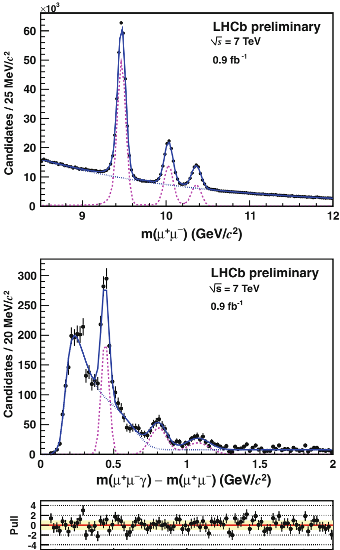
Fig. 5.14 The di-muon invariant mass distribution of \Upsilon(nS) \rightarrow \mu^+\mu^- candidates reconstructed by the LHCb experiment [23] ( upper ). The mass difference distribution m(\mu^+\mu^-\gamma) - m(\mu^+\mu^-) of \chi_b \rightarrow \Upsilon(1S)\gamma candidates reconstructed by LHCb [23] ( lower ). Mass peaks corresponding to the \chi_b(1P) and \chi_b(2P) states, along with the \chi_b(3P) candidate, compatible with that observed by ATLAS, are visible
