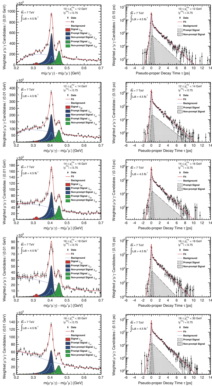
Fig. 6.19 The \Delta m and \tau projections of a simultaneous unbinned maximum likelihood fit performed to reconstructed \chi_{cJ} decays in bins of p_T^{J/\psi} . The data are weighted with the prompt \chi_{c1} acceptance correction
