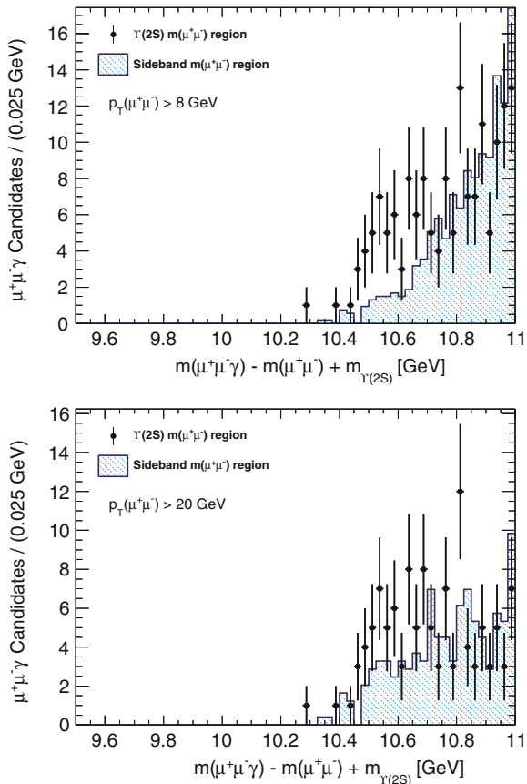
Fig. 5.3 The m(\mu^+\mu^-\gamma) - m(\mu^+\mu^-) + m_{\Upsilon(2S)} distributions for \chi_b(nP) \rightarrow \Upsilon(2S)\gamma candidates reconstructed with unconverted photons. The same distributions for \mu^+\mu^-\gamma candidates with a di-muon invariant mass within the “low mass” sideband region is overlaid and normalised to the same number of events as the \chi_b candidate distribution in the region above 10.7 GeV. The \mu^+\mu^-\gamma candidates in the lower plot are required to have a di-muon transverse momentum p_T^{\mu^+\mu^-} > 20 GeV
