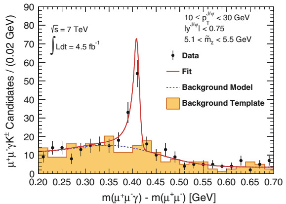
Fig. 6.41 The m(\mu^+ \mu^- \gamma) - m(\mu^+ \mu^-) distribution of selected B^\pm \rightarrow \chi_{c1} K^\pm candidates within 5.1 < \tilde{m}_{\chi_{c1}} < 5.5 GeV, the region around the B^\pm peak ( \tilde{m}_{\chi_{c1}} = m(\mu^+ \mu^- \gamma K^\pm) - m(\mu^+ \mu^- \gamma) + m_{\chi_{c1}} )
