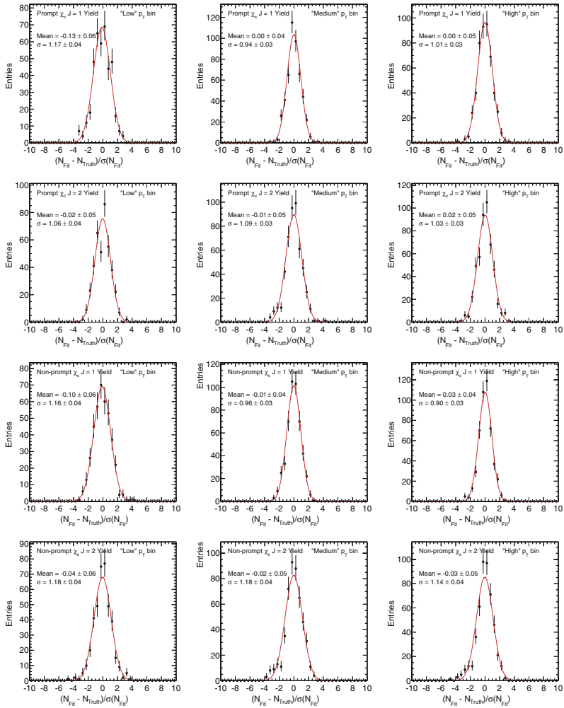
Fig. B.2 Pull distributions for prompt and non-prompt \chi_{c1} and \chi_{c2} yields in three characteristic p_T bins
