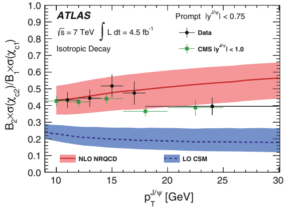
Fig. 6.30 The cross section of prompt \chi_{c2} relative to prompt \chi_{c1} , measured as a function of p_T^{J/\psi} . The measurements are compared to the predictions of NLO NRQCD [34, 35] and the CSM [37] and the measurement of CMS [16]. The error bars represent the total uncertainty on the measurement (statistical and systematic), assuming isotropic decay angular distributions
