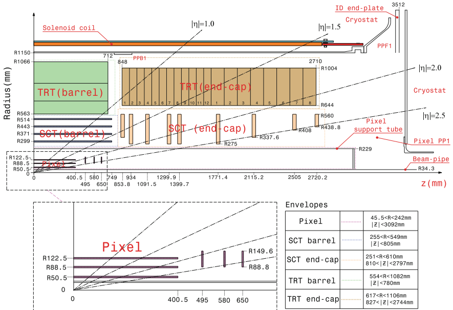
Fig. 3.5 A schematic diagram showing an r-z view of the active layers of the ATLAS inner detector in addition to the major services and support structures [2]. Image from Ref. [2]
