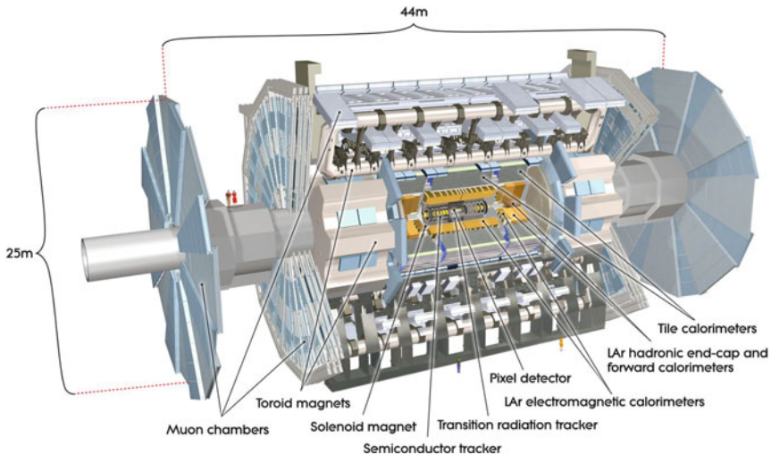
Fig. 3.3 A schematic diagram showing a slice through the ATLAS Detector [2]. Image © CERN
