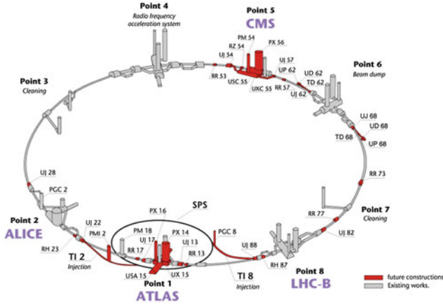
Fig. 3.1 A schematic diagram of the LHC ring showing the locations of the four experiments [1]. Image © CERN
