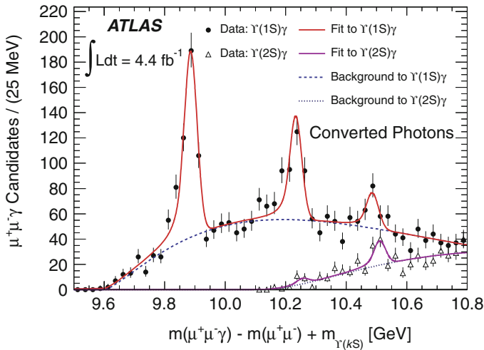
Fig. 5.11 The result of a simultaneous unbinned maximum likelihood fit to the m(\mu^+\mu^-\gamma) - m(\mu^+\mu^-) + m_{\Upsilon(1S)} and m(\mu^+\mu^-\gamma) - m(\mu^+\mu^-) + m_{\Upsilon(2S)} distributions for \chi_b(nP) \rightarrow \Upsilon(kS)\gamma candidates reconstructed with converted photons
