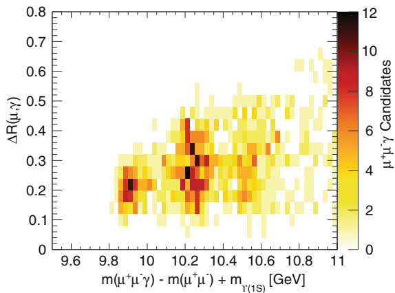
Fig. 5.5 The spatial separation \Delta R(\mu, \gamma) , versus the mass difference m(\mu^+\mu^-\gamma) - m(\mu^+\mu^-) + m_{\Upsilon(1S)} distribution for selected \chi_b(nP) \rightarrow \Upsilon(1S)\gamma candidates. The distribution shows that the \mu^+\mu^-\gamma candidates within the \chi_b(nP) signal peaks in the m(\mu^+\mu^-\gamma) - m(\mu^+\mu^-) + m_{\Upsilon(1S)} distribution are distributed with no strong dependence on \Delta R(\mu, \gamma)
