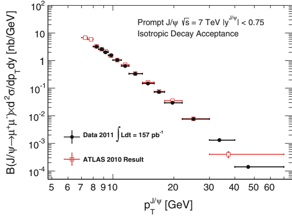
Fig. 6.39 The differential cross section for prompt ( top ) and non-prompt ( bottom ) J/\psi production in pp collisions at \sqrt{s} = 7 TeV. The black points show the measurements of this analysis, while the red points show the reference measurements from [17]
