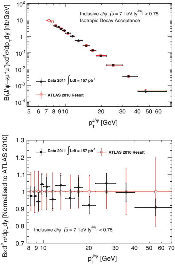
Fig. 6.38 The differential cross section for inclusive J/\psi production in pp collisions at \sqrt{s} = 7 TeV. The black points show the measurements of this analysis, while the red points show the reference measurements from [17]. The lower figure shows the ratio of the measurements with respect to the published ATLAS results, B = (J/\psi \rightarrow \mu^+\mu^-)
