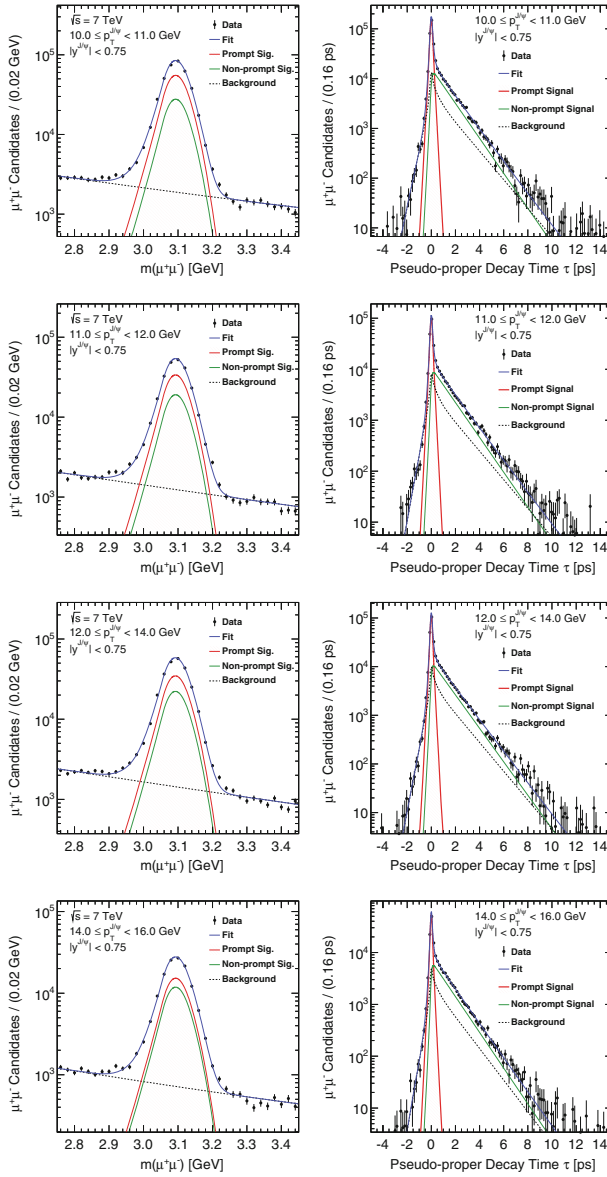
Fig. 6.36 Simultaneous fits to the di-muon invariant mass, m(\mu^+\mu^-) , and pseudo-proper decay time, \tau , distributions of J/\psi \rightarrow \mu^+\mu^- candidates in four bins of p_T^{J/\psi} within 10 < p_T^{J/\psi} < 16 GeV
