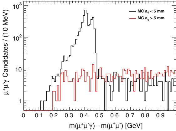
Fig. 6.2 The mass difference distribution m(\mu^+\mu^-\gamma) - m(\mu^+\mu^-) for \chi_{c1} and \chi_{c2} candidates reconstructed from the MC simulation samples described in Sect. 6.3. The black histogram shows reconstructed \chi_{cJ} \rightarrow J/\psi \gamma candidates which satisfy the requirement a_0 < 5 mm while the red histogram shows candidates which fail this requirement. No evidence for \chi_{cJ} peaks is observed in the sample which fail the requirement
