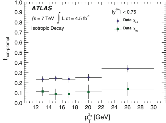
Fig. 6.32 The fraction of \chi_{c1} and \chi_{c2} produced in the decays of b -hadrons measured as a function of p_T^{\chi_c} . The error bars represent the total uncertainty on the measurement (statistical and systematic), assuming isotropic decay angular distributions
