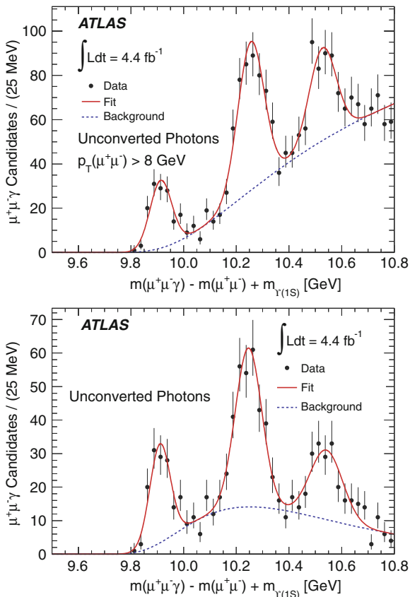
Fig. 5.7 The results of unbinned maximum likelihood fits to the m(\mu^+\mu^-\gamma) - m(\mu^+\mu^-) + m_{\Upsilon(1S)} distribution for \chi_b(nP) \rightarrow \Upsilon(1S)\gamma candidates reconstructed with unconverted photons. The requirement p_T^{\mu^+\mu^-} > 8 GeV is imposed in the upper figure while p_T^{\mu^+\mu^-} > 20 GeV is imposed in the lower figure. The fit result shown in the lower figure is used to measure experimental mass barycentres of the \chi_b signals
