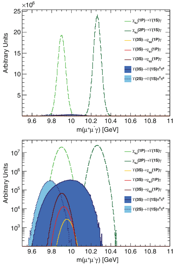
Fig. 5.10 Simulation of the shape of contributions to the mass difference distribution from partially reconstructed bottomonium decays resulting in a \Upsilon(1S)\gamma final state. The simulation uses the \Upsilon(mS) differential cross sections measured by ATLAS as an input [19]. The simulation approximates the inclusive \chi_{b,J}(1P) and \chi_{b,J}(2P) cross sections (i.e. the sum of all three spin states) to the measured \Upsilon(1S) and \Upsilon(2S) cross sections respectively, scaled by 0.75 (this approximation and scaling is motivated by the prompt \chi_{c,J} cross section relative to the prompt J/\psi cross section, measured in Chap. 6). The simulation applies all fiducial cuts on final state particles and smears m(\mu^+\mu^-\gamma) by \pm 40 MeV to mimic the experimental mass resolution (modelling of reconstruction efficiencies is neglected). All channels are normalised with the appropriate world average branching fractions [5]. The decay chains considered all produce smooth and broad contributions to the distribution and together result in contributions (relative to the \chi_b(1P) peak) to the mass difference distribution of less than 5 %
