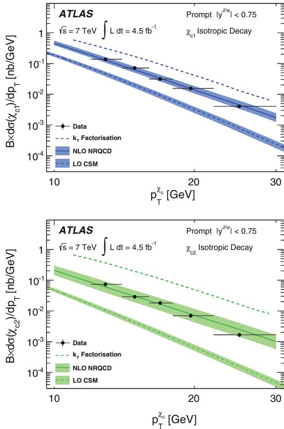
Fig. 6.25 Differential cross sections for prompt \chi_{c1} ( top ) and \chi_{c2} ( bottom ) measured as a function of p_T^{\chi_c} . The measurements are compared to the predictions of NLO NRQCD [34, 35], the CSM [37] and the k_T factorisation approach [38, 39]. The positions of the data points within each bin reflect the average p_T^{\chi_c} of the \chi_c candidates within the bin. The error bars represent the total uncertainty on the measurement (statistical and systematic), assuming isotropic decay angular distributions (in some cases, the error bar is smaller than the data point)
