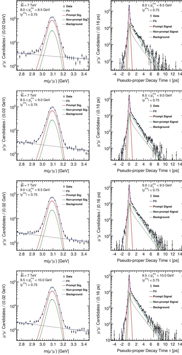
Fig. 6.35 Simultaneous fits to the di-muon invariant mass, m(\mu^+\mu^-) , and pseudo-proper decay time, \tau , distributions of J/\psi \rightarrow \mu^+\mu^- candidates in four bins of p_T^{J/\psi} within 8 < p_T^{J/\psi} < 10 GeV
