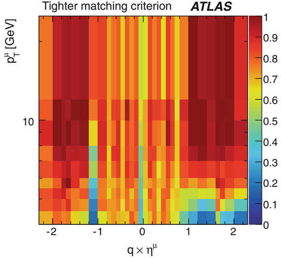
Fig. 6.7 The single muon RoI efficiency component of the EF_2mu4 trigger efficiency, \epsilon_{\text{RoI}} . Figures from Ref. [19]. The “tighter matching criterion” simply refers to the \Delta R < 0.01 matching requirement between the muon reconstructed in the trigger and offline reconstructed muon
