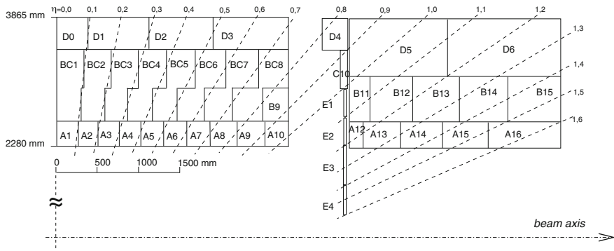
Fig. 3.9 A schematic diagram showing the segmentation in r \times z (and \eta in dashed lines) of the Tile Calorimeter. Image from Ref. [2]
