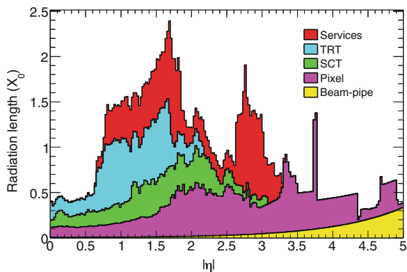
Fig. 4.8 The material budget of the ATLAS inner detector (up to the solenoid) measured in radiation lengths as a function of |\eta| , broken down into the individual detector components. Figure taken from Ref. [2]
