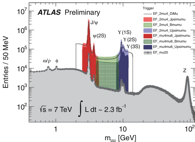
Fig. 4.11 A comparison of the data samples collected by various ATLAS muon triggers. The dedicated low p_T di-muon triggers (coloured histograms) significantly improve the acceptance for J/\psi \rightarrow \mu^+ \mu^- and \Upsilon(nS) \rightarrow \mu^+ \mu^- events in comparison to a single high p_T muon trigger (grey histogram). The shaded histograms represent the number of events collected by triggers with different muon p_T and di-muon invariant mass cuts. Figure from Ref. [11]
