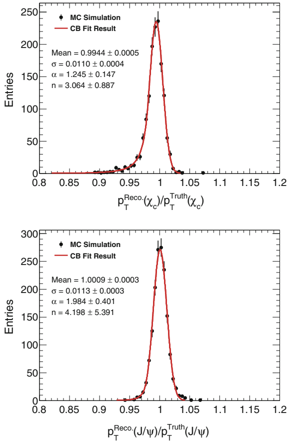
Fig. 6.21 The experimental resolution in p_T^{\chi_c} (top) and p_T^{J/\psi} (bottom) for the fiducial region 10 < p_T^{J/\psi} < 30 GeV and |y^{J/\psi}| < 0.75 , derived from MC simulation. Both distributions are fitted with a CB function
