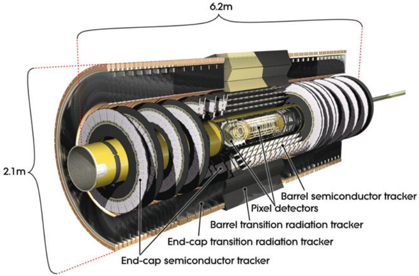
Fig. 3.4 A schematic diagram the showing the individual components of the ATLAS Inner Detector (ID) [2]. Image © CERN
