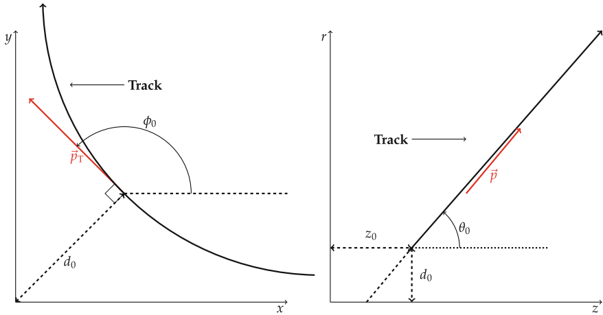
Fig. 4.1 Diagram showing the definition of the perigee track parameters in the ATLAS coordinate system in the transverse plane ( left ) and r - z plane ( right )
