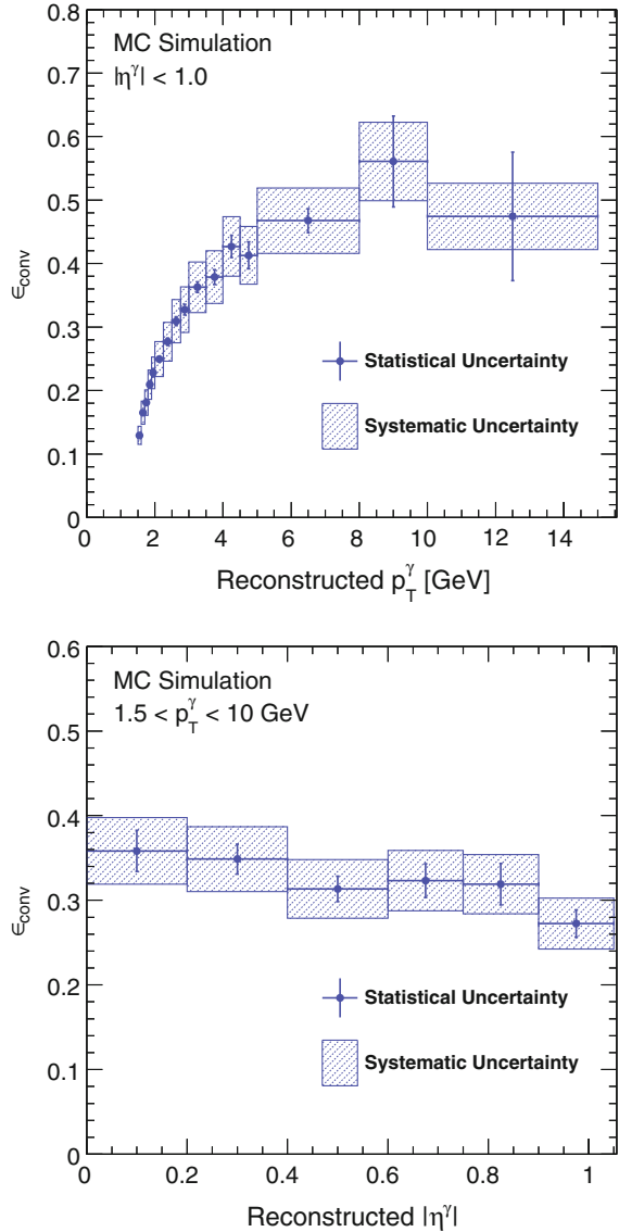
Fig. 6.14 The conversion reconstruction efficiency calculated as a function of measured p_T^\gamma , for |\eta^\gamma| < 1.0 (top) and as a function of measured |\eta^\gamma| , for 1.5 < p_T^\gamma < 10 GeV (bottom). The estimate of the systematic uncertainty shown in both figures is discussed in Sect. 6.8
