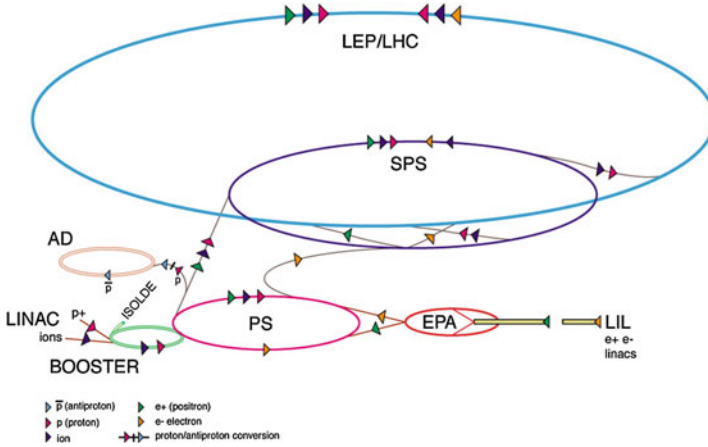
Fig. 3.2 The CERN accelerator complex. The particle accelerators involved in the LHC injection chain (LINAC→BOOSTER→PS→SPS→LHC) are shown [1]. Image © CERN
