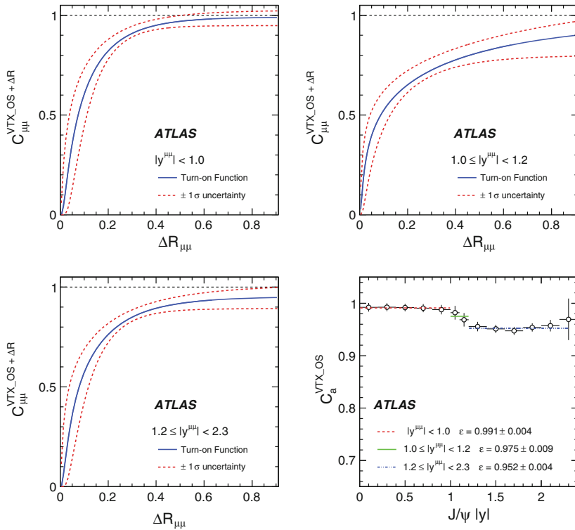
Fig. 6.8 The di-muon correction to the EF_{2\mu 4_{J\psi\text{simu}\mu}} trigger efficiency, c_{\mu^+\mu^-} . The upper plots and the lower left plots show the di-muon correction term c_{\mu^+\mu^-} of \epsilon_{\text{trig}} , for different |y^{J/\psi}| regions, as a function of \Delta R measured between the two muons within the di-muon pair. The lower right plot shows the plateau values (at asymptotically large \Delta R ) of c_{\mu^+\mu^-} as a function of the absolute rapidity of the di-muon system. Figures taken from Ref. [19]. The \pm 1\sigma systematic bands are used to estimate the systematic uncertainty on the measured \chi_{cJ} cross sections due to the parameterisation of the c_{\mu^+\mu^-} correction (this is discussed in detail in Sect. 6.8). The y axis of the upper and lower left plots is identical to c_{\mu^+\mu^-} while the y axis of the lower right plot represents the value that c_{\mu^+\mu^-} approaches asymptotically at large \Delta R
