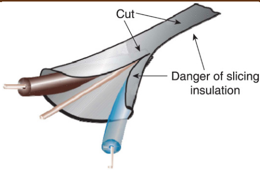
FIGURE 2.39 Terminating flat cable.
