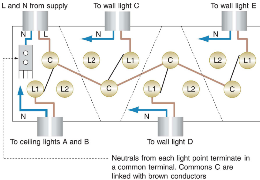
FIGURE 2.19 Wiring for feeding the switch.
