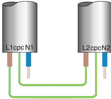
FIGURE 7.8 L and cpc cross connection.
