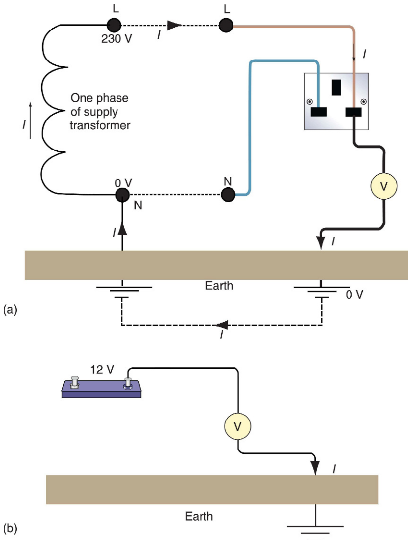
FIGURE 3.2 (a) Earth path, (b) No earth path.
