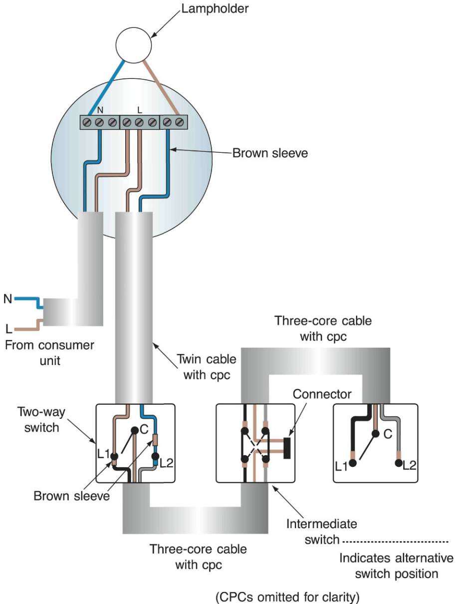
FIGURE 2.15 Two way and intermediate switching.
