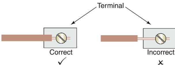
FIGURE 2.44 Termination technique.
