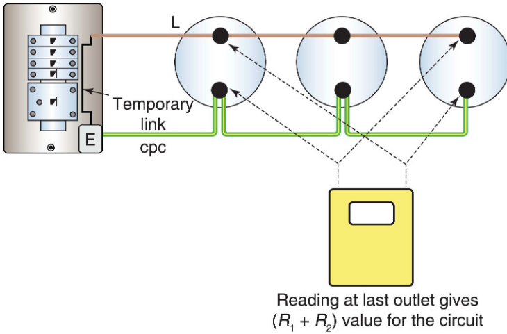
FIGURE 7.3 CPC continuity.
