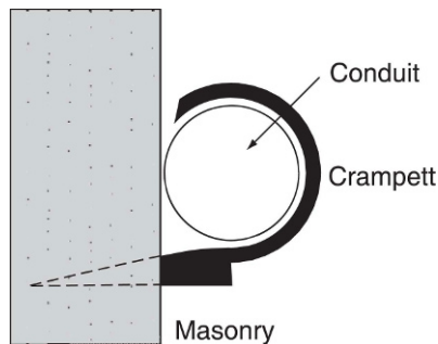
FIGURE 2.37 Crampett fixing.
