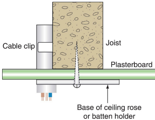
FIGURE 2.34 Fixing to joist.
