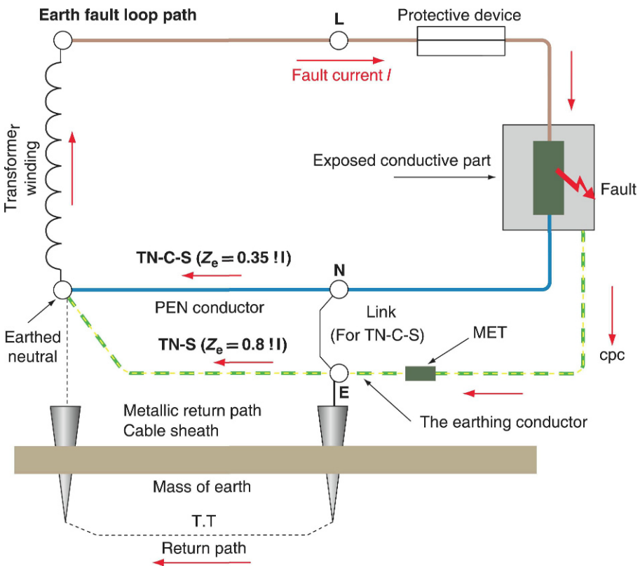
FIGURE 3.4 Earth fault loop path.
