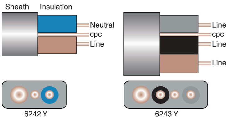
FIGURE 2.23 Flat profile cable.
