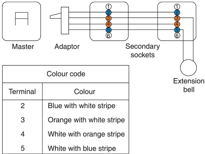
FIGURE 8.4 Telephone socket wiring.
