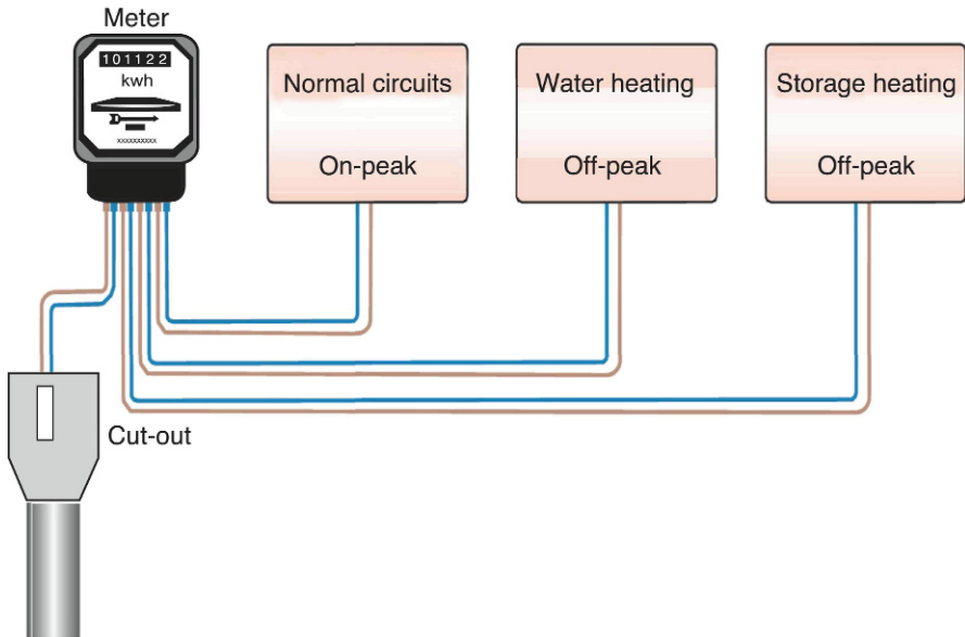
FIGURE 2.4 Off-peak system.
