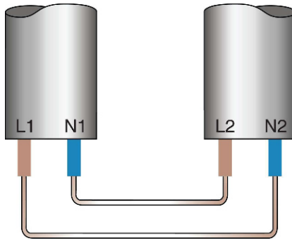
FIGURE 7.7 L and N cross connection.
