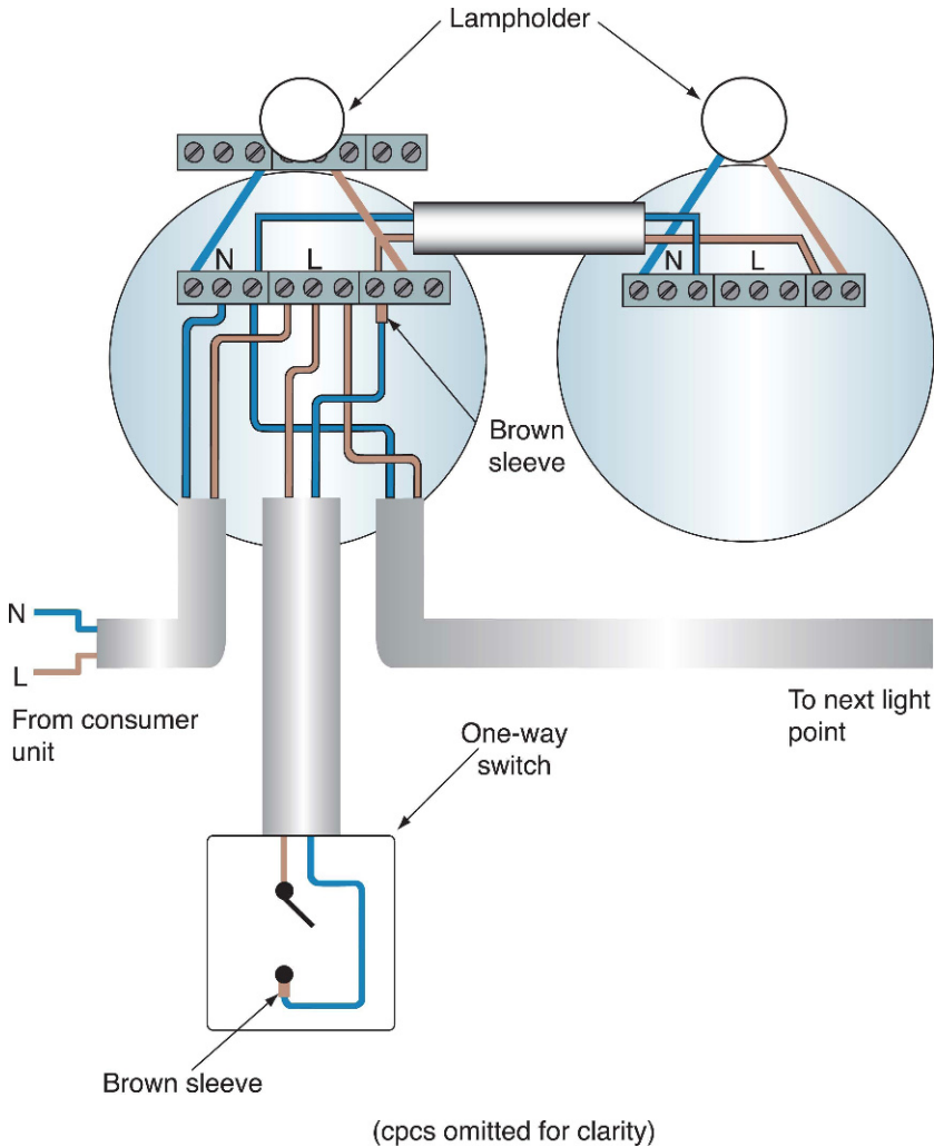
FIGURE 2.12 One way switch controlling two points.
