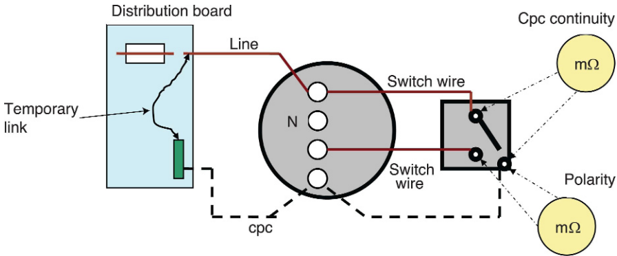
FIGURE 7.10 Lighting polarity.
