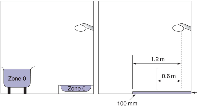
FIGURE 4.1 Zone 0.
