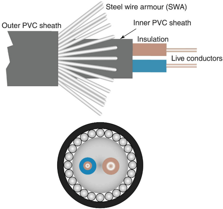
FIGURE 2.24 Steel wire armoured cable (SWA).
