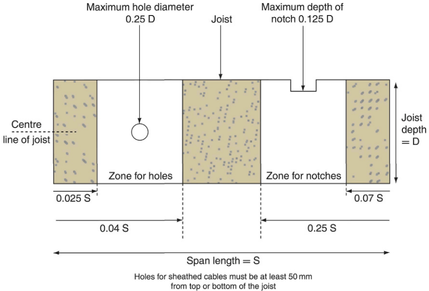
FIGURE 2.33 Holes and notches in joists.
