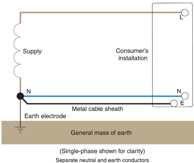
FIGURE 1.6 TN-S system.
