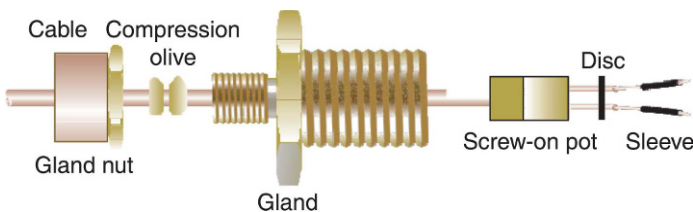
FIGURE 2.42 Mineral cable termination.
