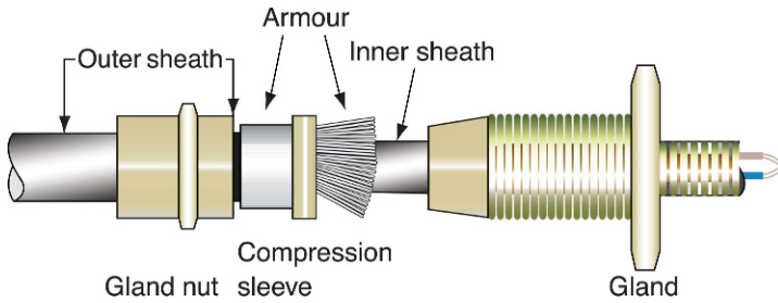
FIGURE 2.43 SWA termination.
