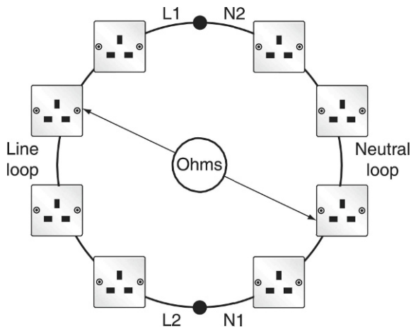
FIGURE 7.6 Circle formed by cross connection.
