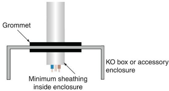
FIGURE 2.41 Entry to KO box.
