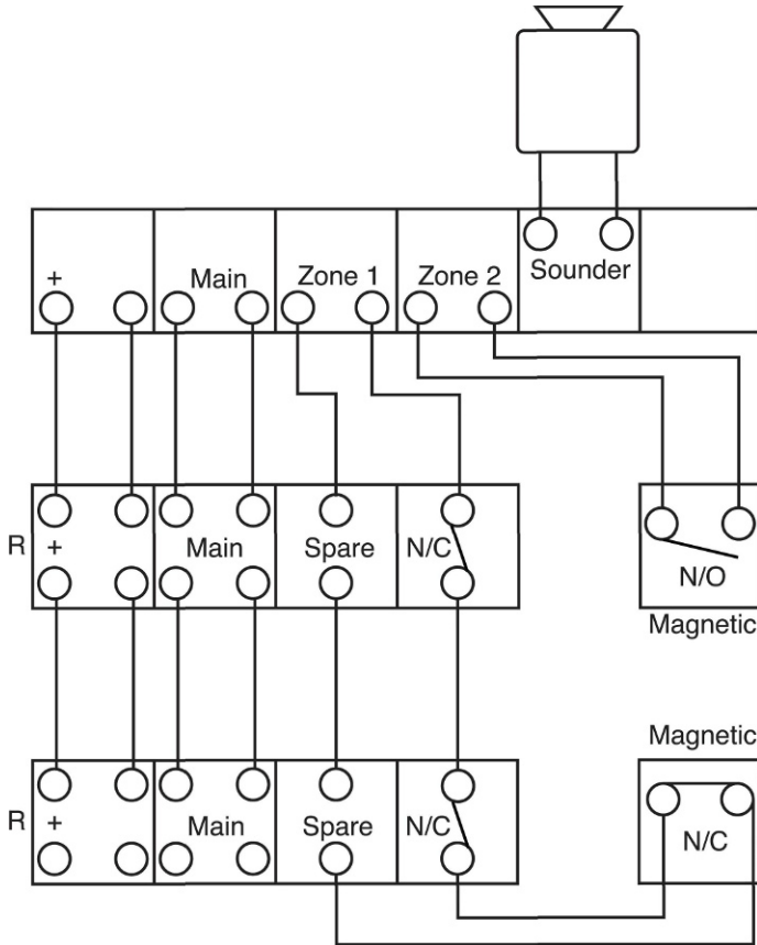
FIGURE 8.2 Sensor connections.
