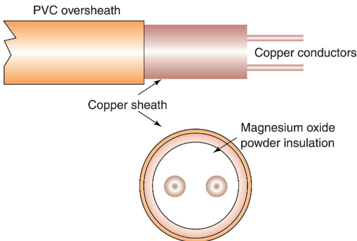
FIGURE 2.25 Mineral insulated cable.
