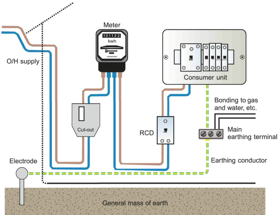
FIGURE 2.1 TT system.
