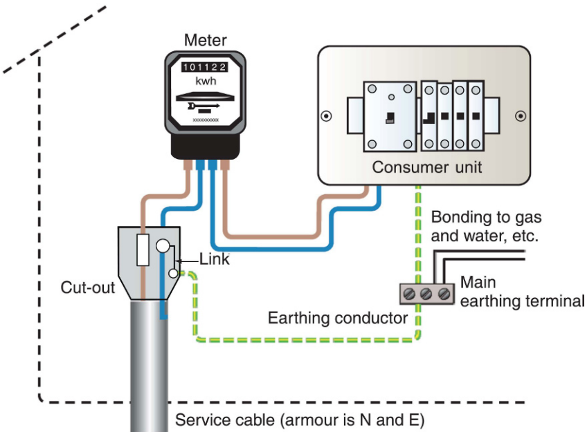
FIGURE 2.3 TN-C-S system.
