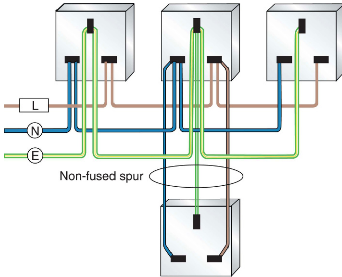
FIGURE 2.20 Non-fused spur.
