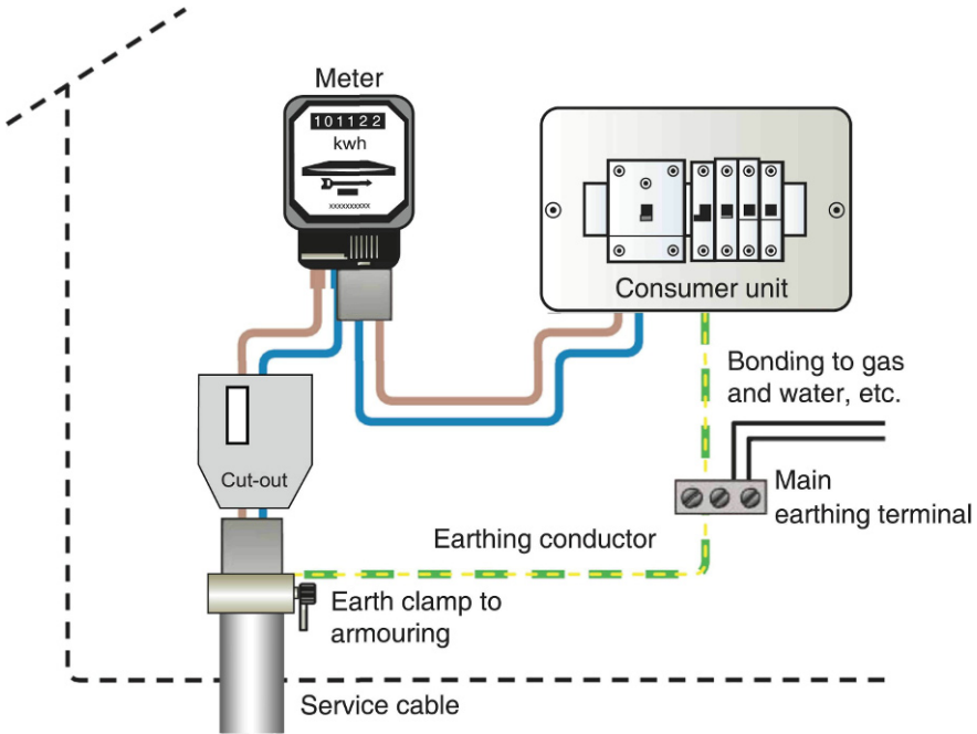
FIGURE 2.2 TN-S system.
