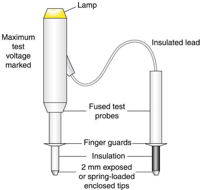
FIGURE 7.1 Approved test lamp.
