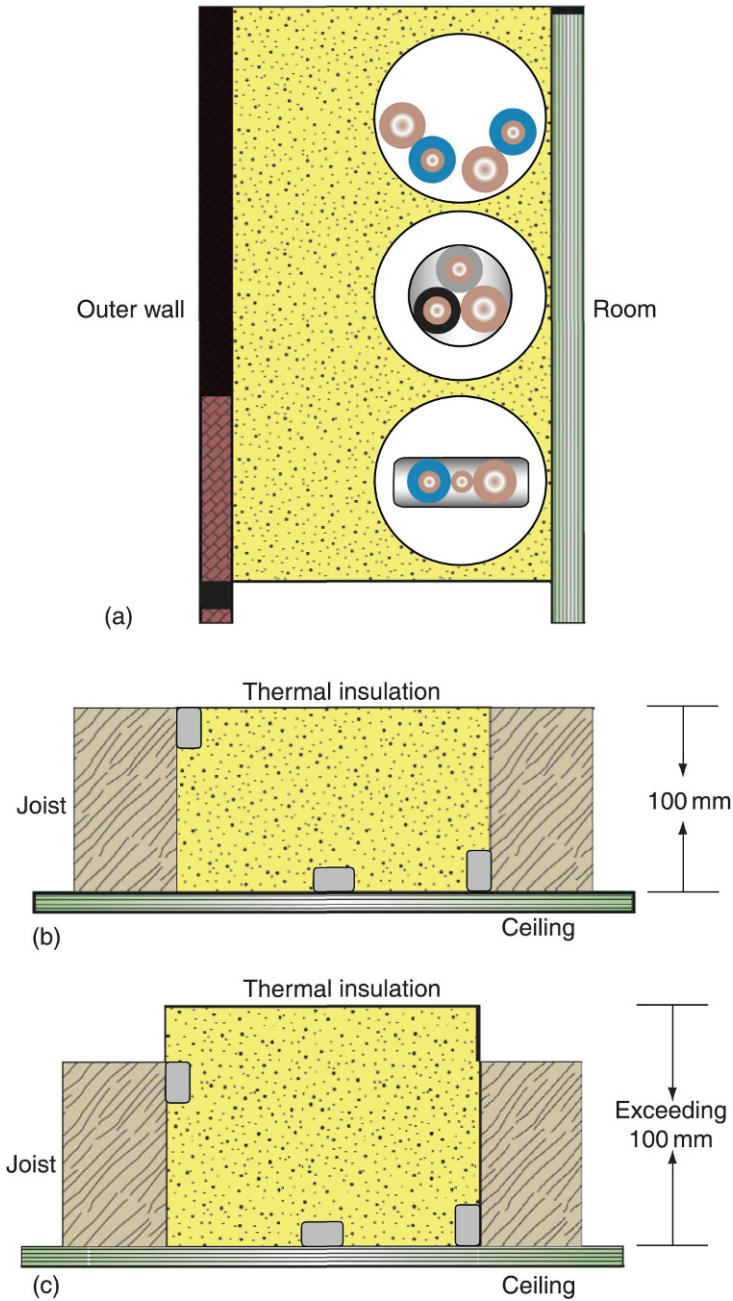
FIGURE 2.31 (a) Method A, (b) Method 100, (c) Method 101. (Continued)
