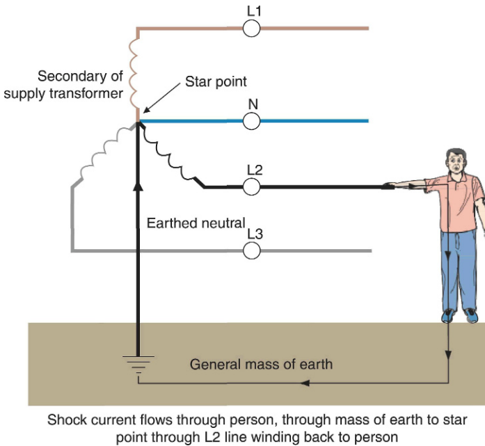
FIGURE 1.4 Shock Path.
