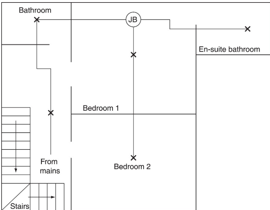
FIGURE 2.11 Lighting circuit with junction box.
