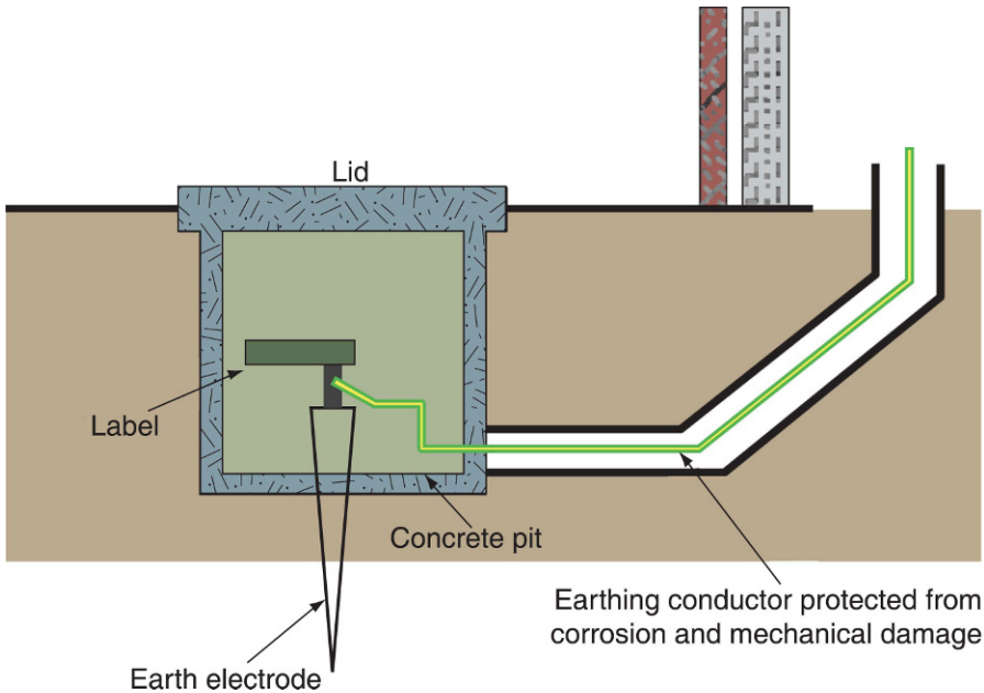
FIGURE 2.7 Earth electrode installation.
