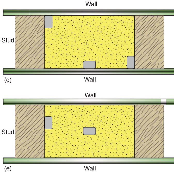
FIGURE 2.31 (Continued) (d) Method 102, (e) Method 103.
