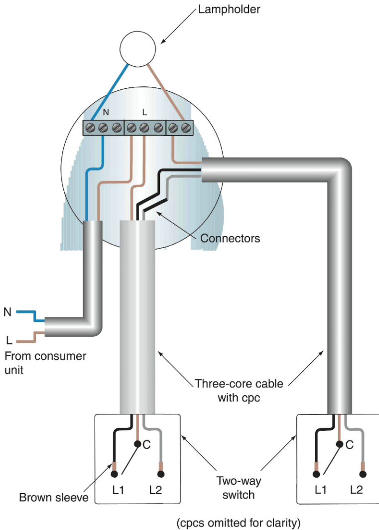
FIGURE 2.13 Two way switching via the ceiling rose.
