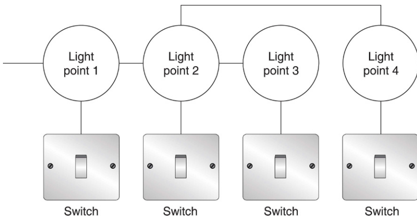
FIGURE 2.9 Lighting circuit with no junction box.
