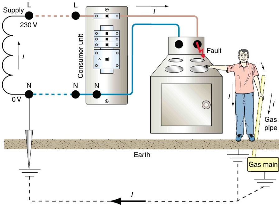
FIGURE 3.3 Shock path.
