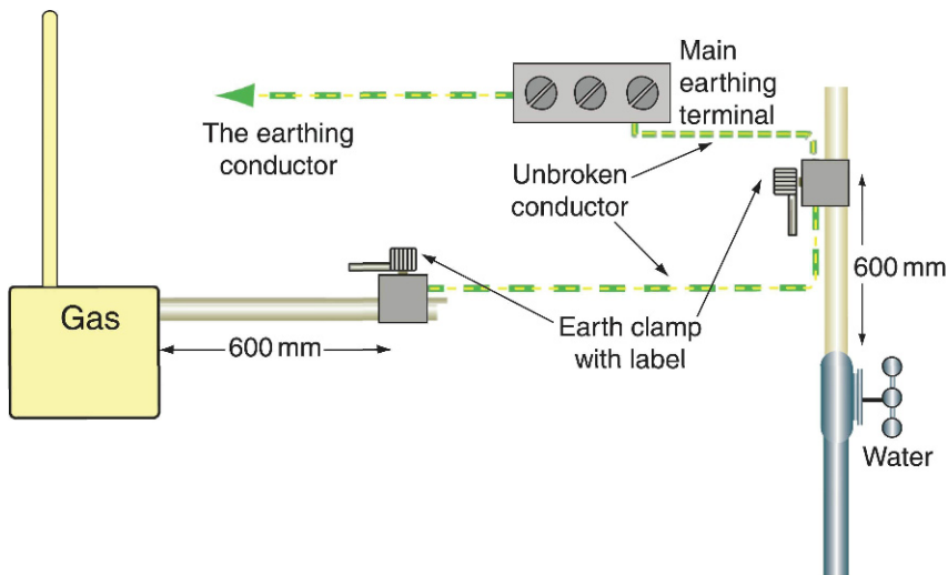
FIGURE 2.6 Bonding conductors.
