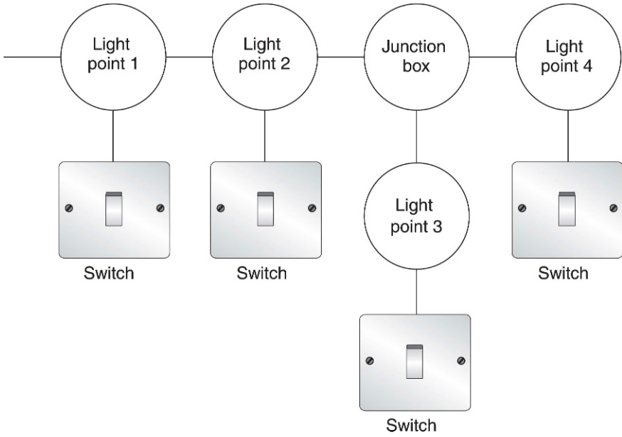
FIGURE 2.10 Lighting circuit with junction box.
