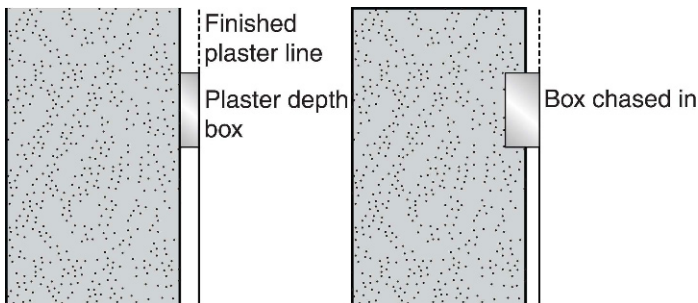
FIGURE 2.32 Fixing knock-out boxes.
