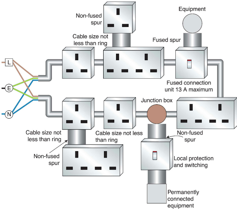
FIGURE 2.22 Ring final circuit.
