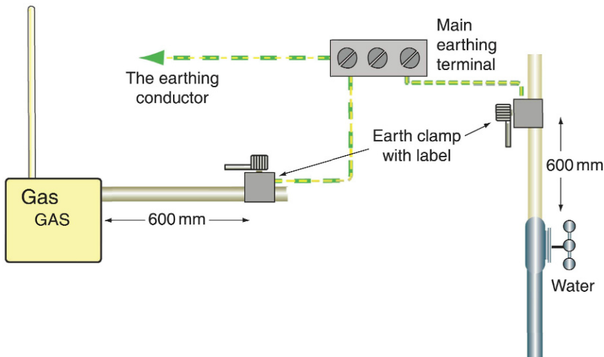
FIGURE 2.5 Bonding conductors.
