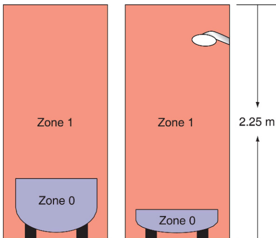
FIGURE 4.2 Zone 1.
