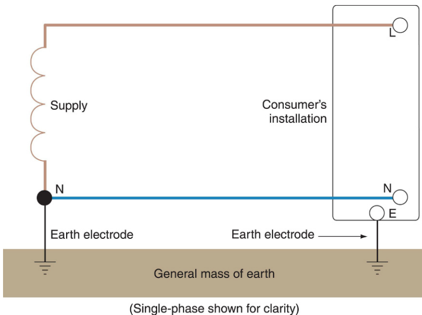
FIGURE 1.5 TT system.
