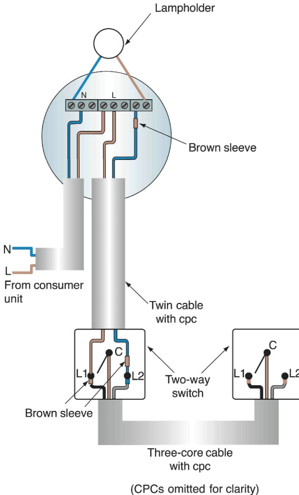
FIGURE 2.14 Two way switching via the switches.
