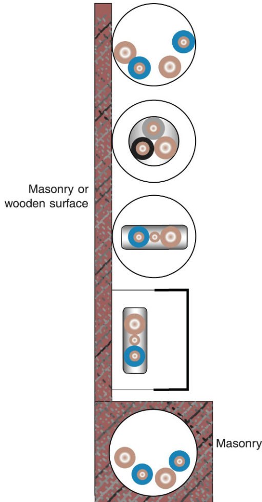
FIGURE 2.30 Method B.
