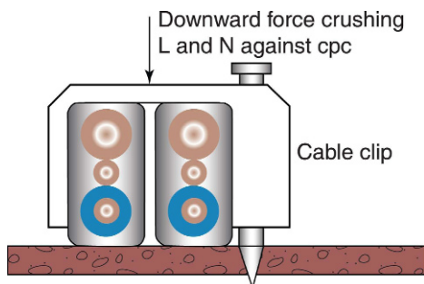
FIGURE 2.28 Incorrect cable clipping.
