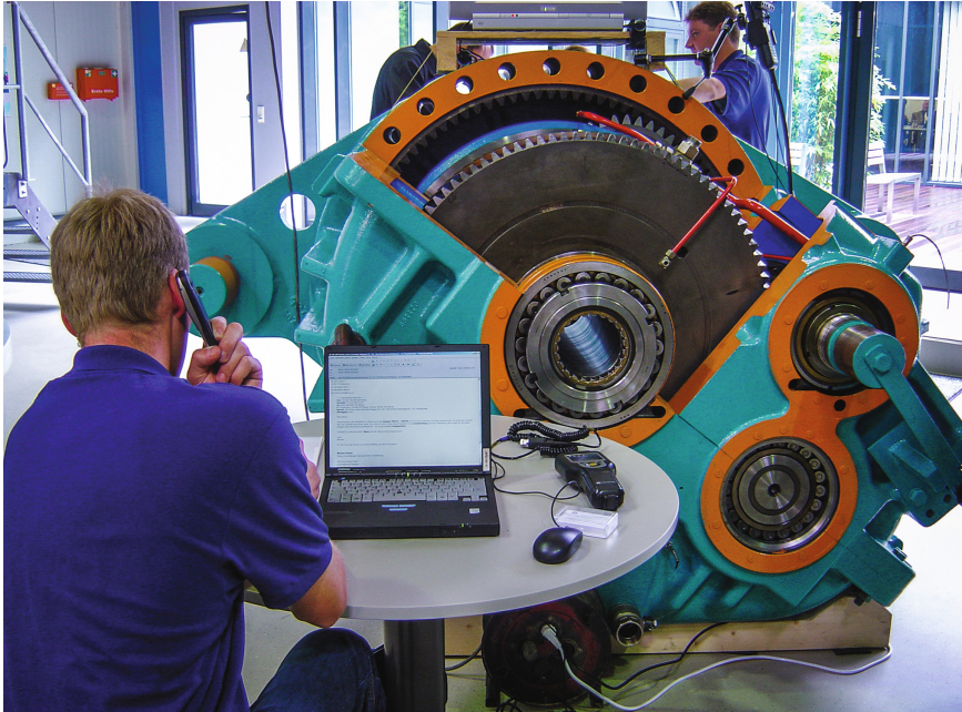
Fig. 5.2 Analysis of a gear box
