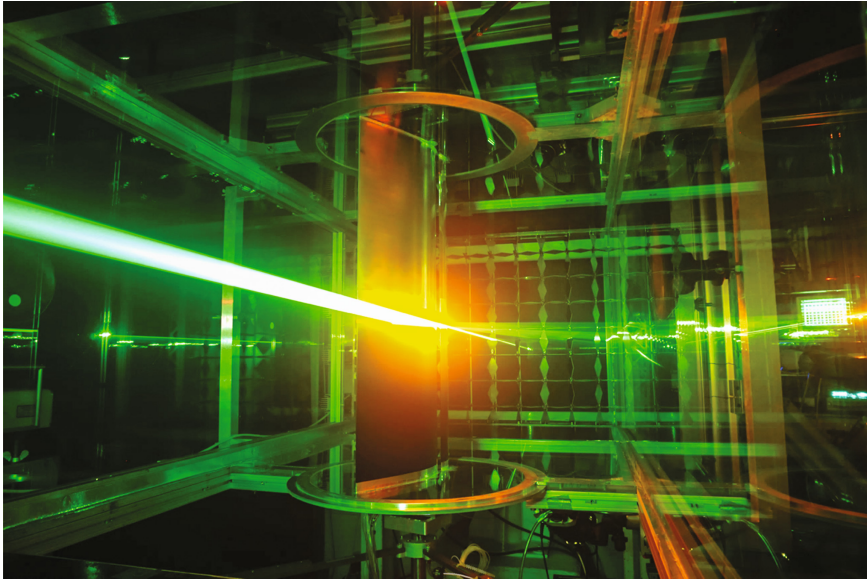
Fig. 3.1 Advanced aerodynamic measurements of a rotor blade profile. PIV measurements in the wind tunnel with a turbulence generating grid
