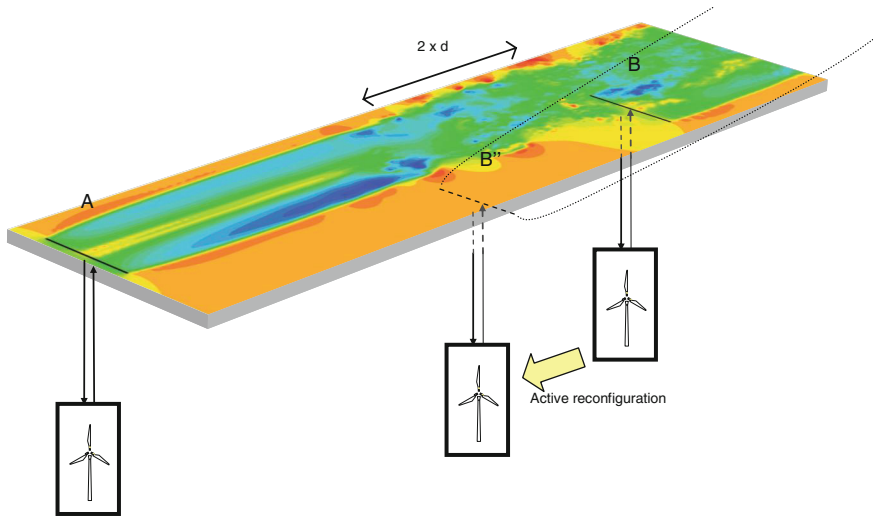
Fig. 4.2 Controlled relocation of floating wind turbine B to avoid the wake of the upstream wind turbine A.
