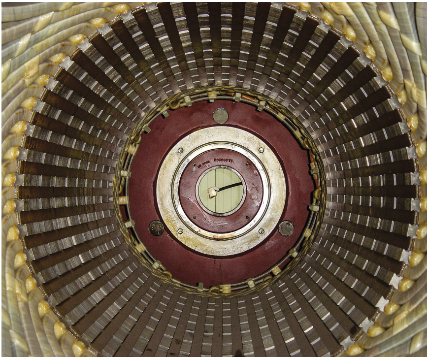
Fig. 5.1 Stator of an electrical generator, designed specifically for wind turbines
