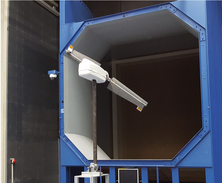
Fig. 4.1 A model rotor in an open jet wind tunnel to test trailing edge flaps for load control
