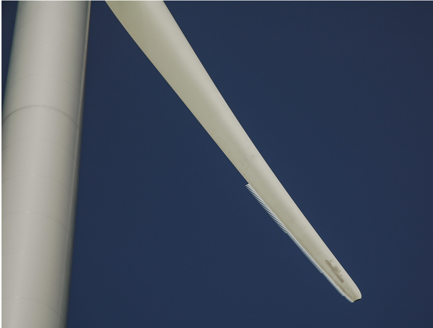
Fig. 3.2 Serrated trailing edge to reduce high frequency noise emission by wind turbine rotors
