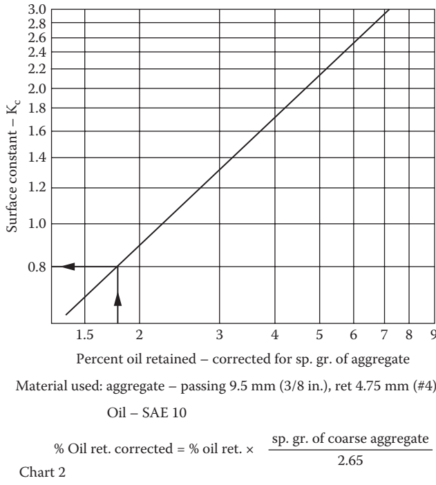
FIGURE 14.6 Charts for Hveem mix design method. (Courtesy of California Department of Transportation, Sacramento, CA.)
