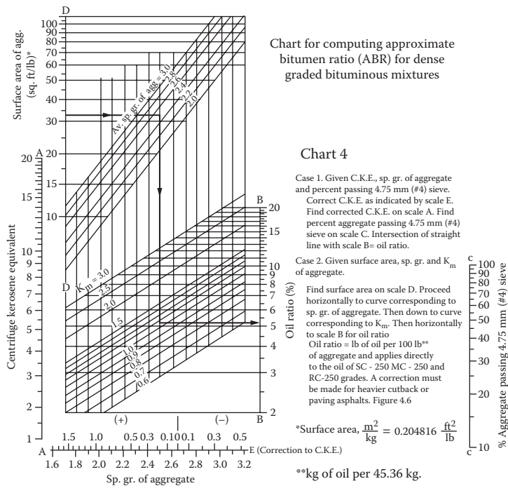
FIGURE 14.6 (continued) Charts for Hveem mix design method. (Courtesy of California Department of Transportation, Sacramento, CA.)
