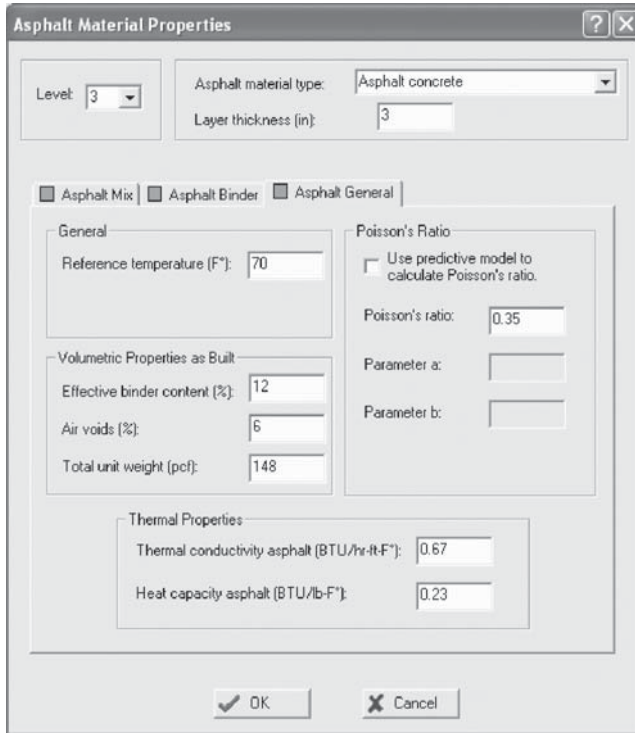
FIGURE 14.40 Asphalt material properties—volumetric properties.
