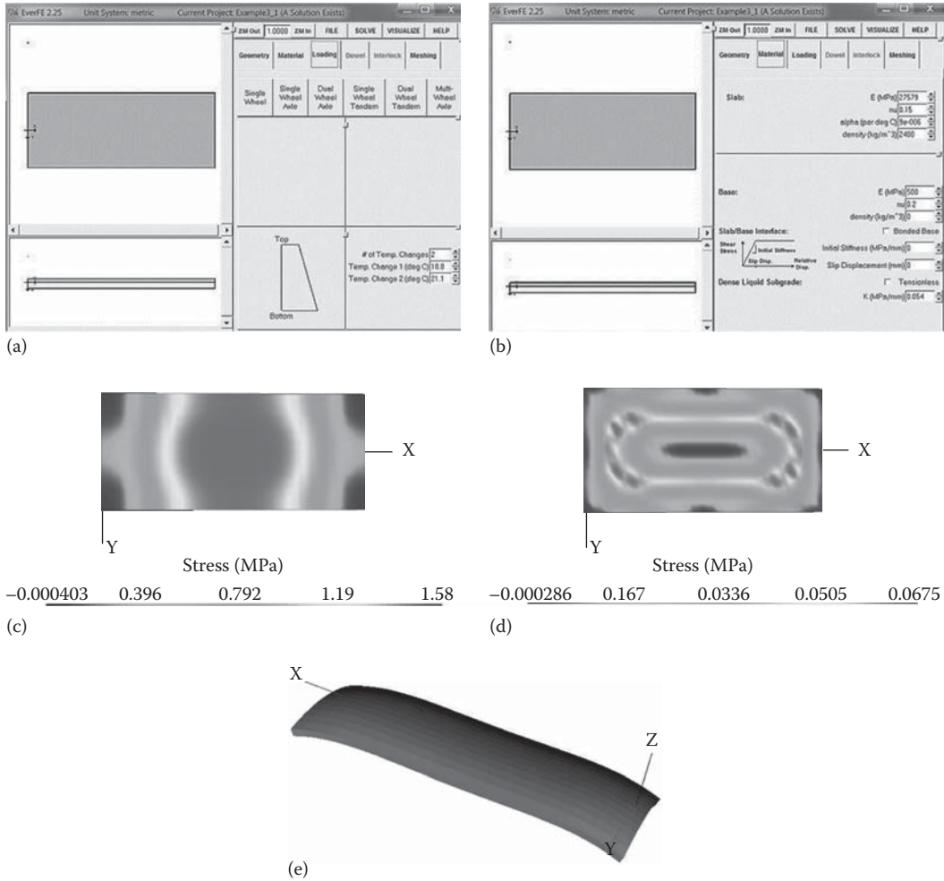
FIGURE 3.12 (a) EverFE input page for temperature gradient, (b) EverFE input page for materials properties, (c) EverFE output results for stress at the top of the slab, (d) EverFE output results for stress at the middle of the slab, and (e) EverFE output results for slab deflection due to temperature curling.
