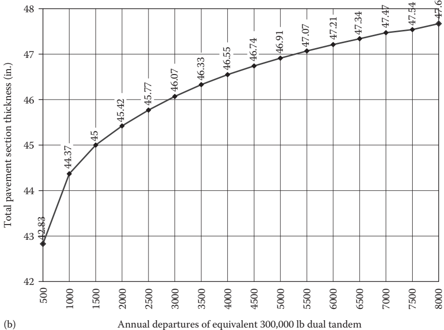
FIGURE 19.4 Change in thickness with (a) CBR and (b) departures. Note that the CBR of the different layers can be determined by evaluation tests, such as those using nondestructive testing (NDT). Also, rounding off thicknesses of equivalent layers (derived using layer equivalencies) is not recommended.
