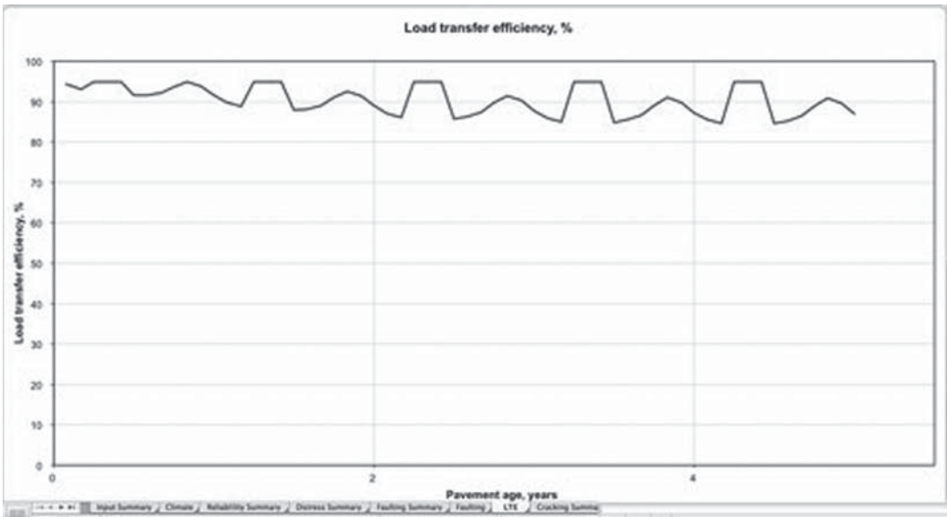
FIGURE 15.20 MEPSG example output for LTE.
