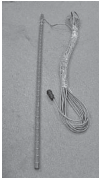
FIGURE 22.3 Frost depth measurement instrument. (Courtesy of Lauren Swett.)
