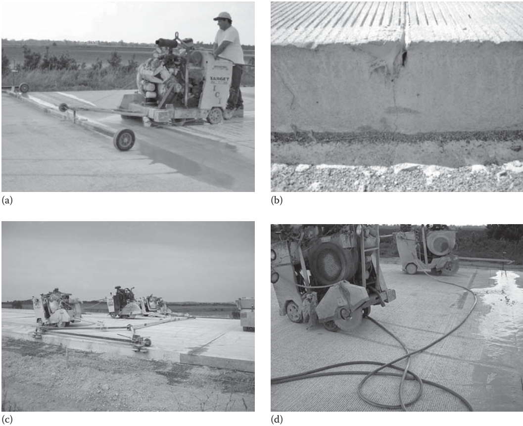
FIGURE 17.16 (a–d) Joint sawing operations in PCC pavements. (Courtesy of Wouter Gulden, ACPA-SE Chapter, Duluth, GA.)
