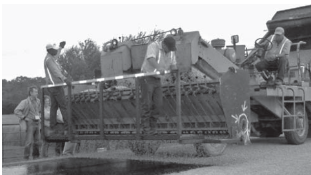
FIGURE 18.6 Chip seal. (Courtesy of Maureen Kestler, USDA Forest Services, Washington, DC.)
