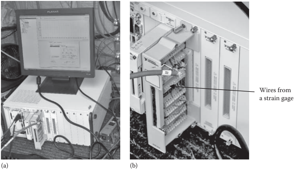
FIGURE 22.8 Data acquisition systems. (a) Data acquisition system with module in computer. (b) Close-up view of the module showing connection from a strain gage.
