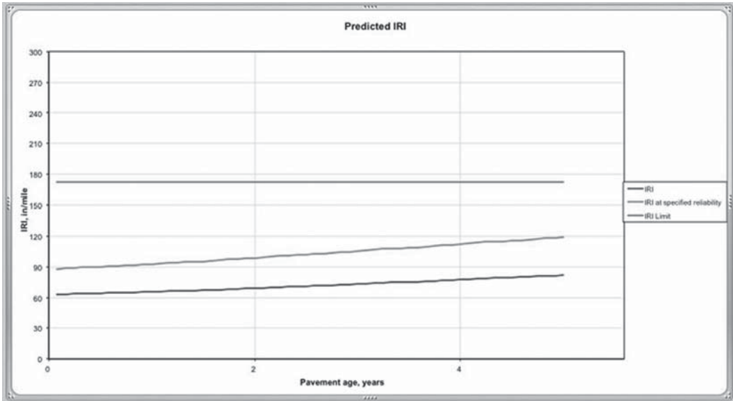
FIGURE 15.19 MEPSG example output for predicted IRI.
