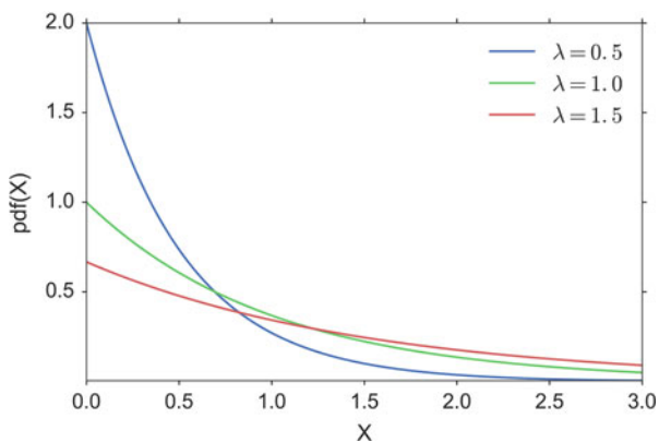
Fig. 6.20 Exponential distribution
