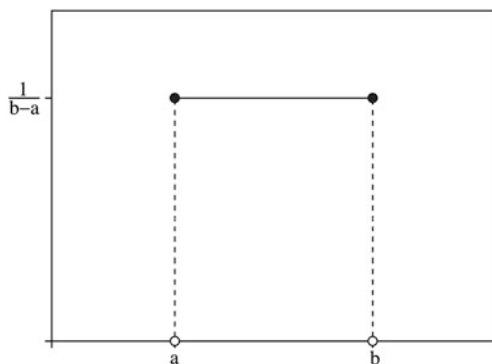
Fig. 6.21 Uniform distribution
