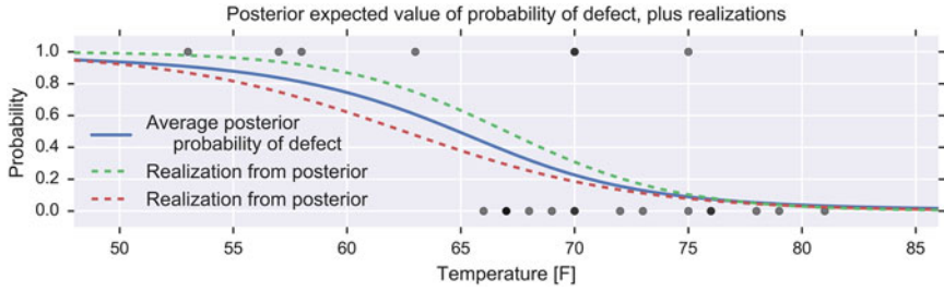
Fig. 14.2 Probability for an O-ring failure, as a function of temperature
