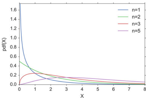
Fig. 6.15 Chi-square distribution
