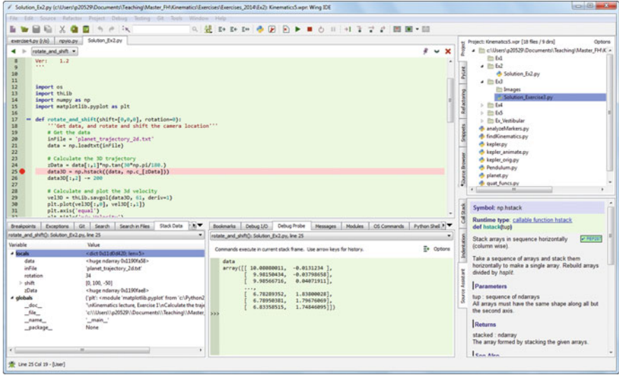
Fig. 2.7 Wing is my favorite development environment, with probably the best existing debugger for Python. Tip: If Python does not run right away, you may have to go to Project -> Project Properties and set the Custom Python Executable and/or Python Path
