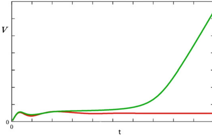
Fig. 5.1 The velocity v(t) for E < E_c (red) and E_c > E_c (green)
