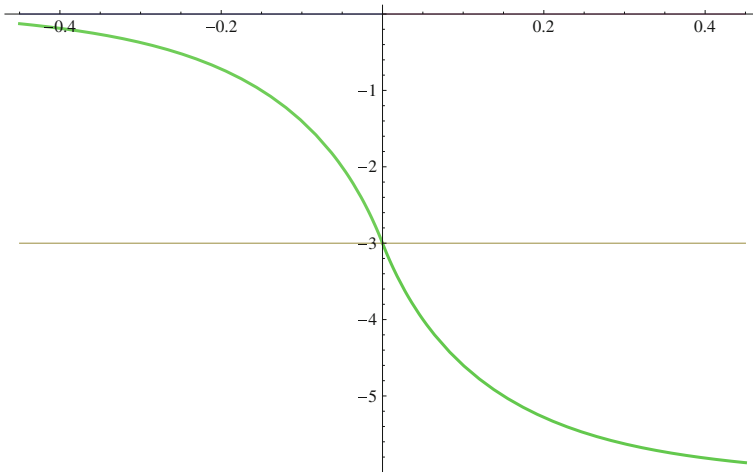
Fig. 2.25 \beta e V(x) in the non-degenerate case (with c = 3 )
