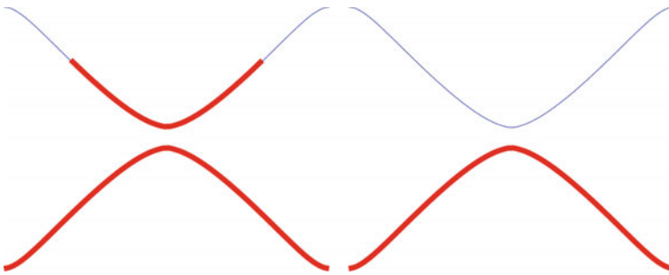
Fig. 2.16 Band filling in metals and insulators
