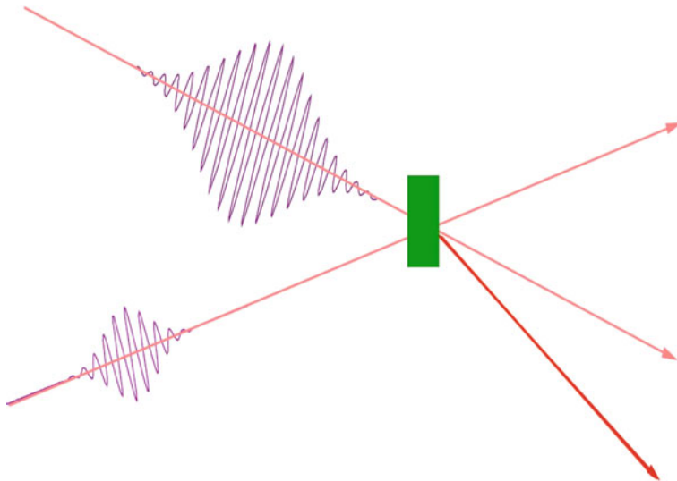
Fig. 6.3 Four-wave-mixing experiment
