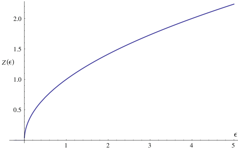
Fig. 2.1 Free one-electron state density z(\varepsilon)
