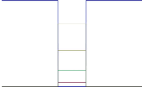
Fig. 2.7 Energy levels in the well for C^2 = 38
