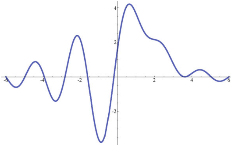
Fig. 2.15 Stationary state of the Wannier ladder
