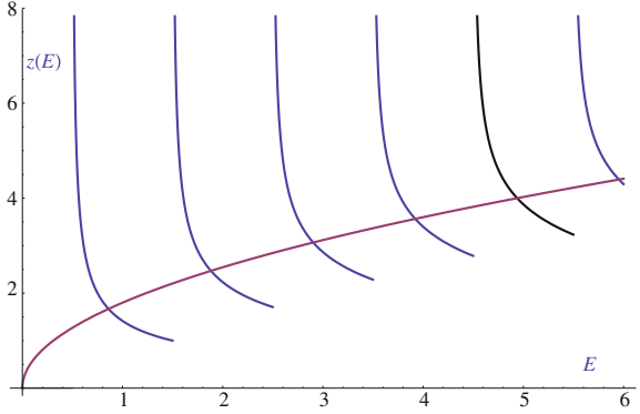
Fig. 2.5 State density z(E) in magnetic field
