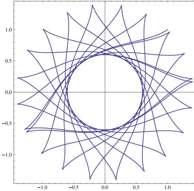
Fig. 8.2 Classical relative motion of opposite charged particles in 2D in the presence of a transverse magnetic field
