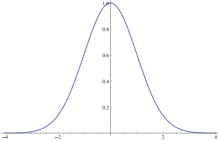
Fig. 2.4 The ground-state Landau function \Phi_{0,0}(x)
