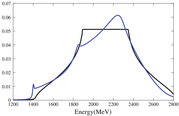
Fig. 3.1 Exciton state density in the whole band calculated within the Wannier model. (black—without Coulomb interaction, blue—with Coulomb interaction)
