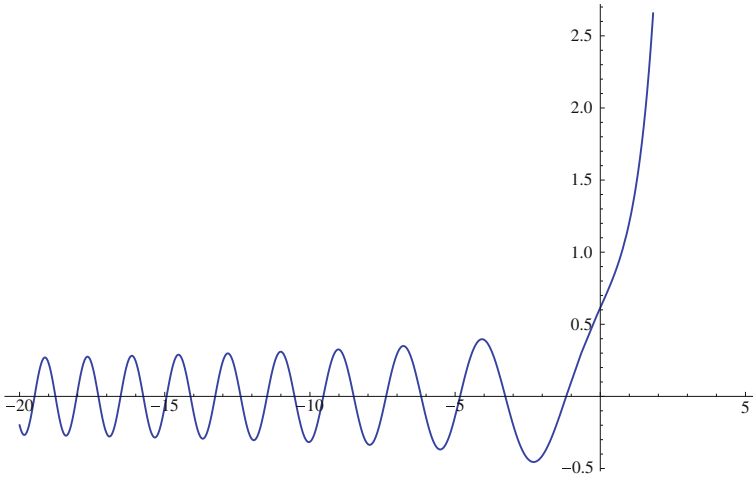
Fig. 2.3 Airy function
