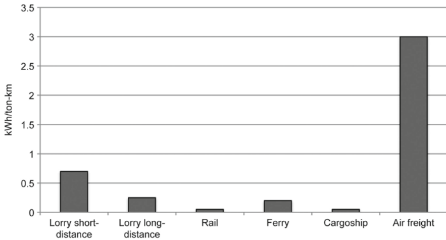
Fig. 17.1 Specific energy use for goods transport in 2000 (Source: Åkerman and Höjer 2006)
