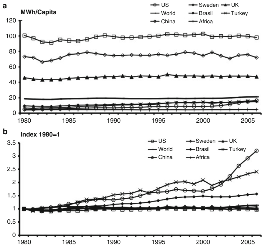
Fig. 3.1 (a) Total primary energy consumption per capita between 1980 and 2006 in MWh. (b) Total primary energy consumption per capita between 1980 and 2006. Index 1980=1. Source: International Energy Annual 2006, Department of Energy, US
