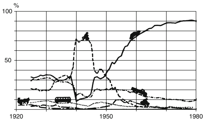
Fig. 8.3 Market share of different vehicles 1925–1980 counted at the end of October, as a percent (Source: Dufwa 1986, p. 78)
