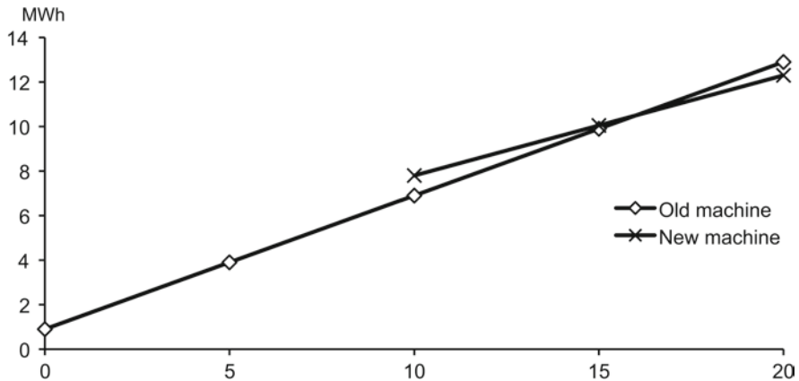
Fig. 16.2 Comparison of the cumulative energy consumption for use of a washing machine over a 20-year life cycle, with the replacement of the machine after 10-years of use (Source: Heiskanen E Conditions for Product Life Extension, Heiskanen 1996, p. 12 (Figure redrawn to MWh))
