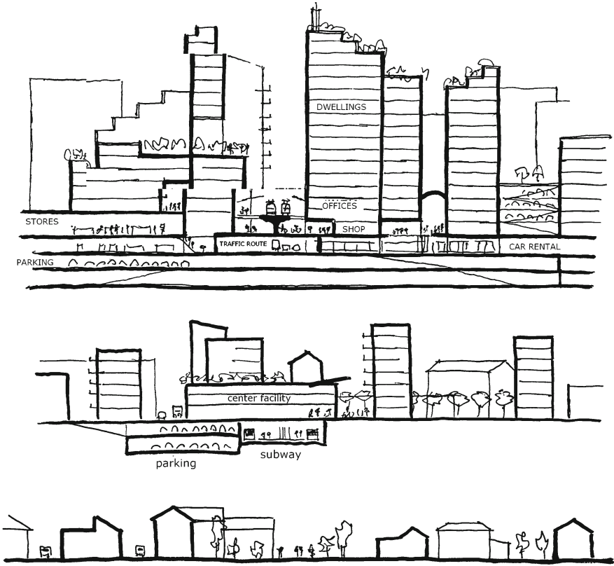
Fig. 21.4 Section through the housing in alternatives Urban Cores, Suburban Centers and Low-rise Settlements
