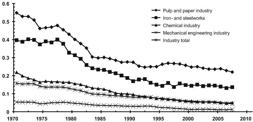
Fig. 16.1 Industry specific electricity and oil use 1970–2007, kWh/SEK production value, 2,000 prices (Source: Energy in Sweden – Facts and Figures, 2008, table to Fig. 19)
