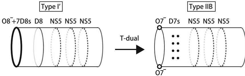
Fig. 3.4 T-dual of the Type I' brane configuration realizing S^1 compactified higher rank E-string theory. The \text{O8}^- plane wrapping S^1 becomes two \text{O7}^- planes and the eight D8s become eight D7 branes, while the NS5 branes in type I' remain to be NS5. From: [23]
