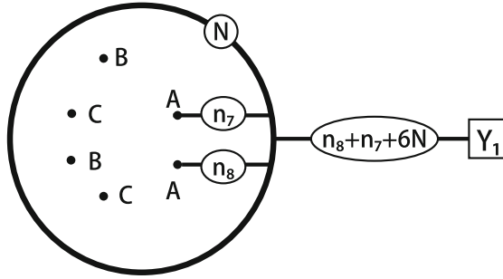
Fig. 3.8 The Type IIB web for the 6d theory \mathcal{T}^{(M9, su)}\{u_i\} on S^1 with Kaluza–Klein modes. We have N circles of 5-branes. Outside the circles, we have a leg of 6N + n_7 + n_8 5-branes terminated at 7-branes as specified by the partition Y_1 . Inside the circle, we have six 7-branes A^2BCBC . n_7 and n_8 5-branes are attached to the two A 7-branes respectively. From: [23]
