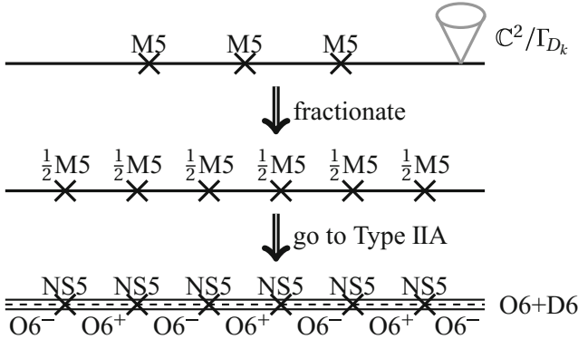
Fig. 2.8 M-theory and Type IIA brane construction of conformal matter \mathcal{T}_N^{(D_k, D_k)} . Since the D6 brane charges of O6^\pm is different by eight, the number of D6 branes stacked with O6^\pm should be adjusted so that the total D6 charge is the same between left and right side of each NS5 brane. Thus, the tensor branch theory is read to be an \mathfrak{so}(2k) - \mathfrak{usp}(2k - 8) alternating quiver
