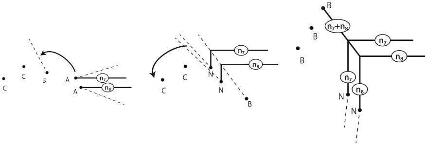
Fig. 3.9 The 7-brane rearrangement inside the circle of 5-branes. Extra n_7 and n_8 5-branes attached to two A create the junction of 5-branes due to the Hanany–Witten effect. First, we move two A across the cut of B . A becomes N and we obtain the middle configuration. Second, we move two C s through the branch cuts of N s. After that process, C^2 becomes B^2 since they cross the cuts from two N . Finally, by moving one B along its cut, we obtain the configuration in right. From: [23]
