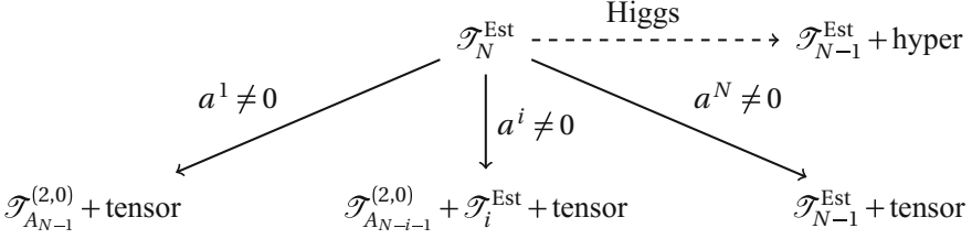
Fig. 2.5 RG flows from \mathcal{T}_N^{\text{Est}} . a_i denotes the tensor vev of i th tensor mode counting from the left of Fig. 2.4d. On 1 dimensional subset of the tensor branch, the theory flows to sum of an \mathcal{N} = (2, 0) theory, an E-string theory and a Nambu–Goldstone tensor mode. On the Higgs branch, the theory flows to the E-string theory with less rank plus NG hyper modes
