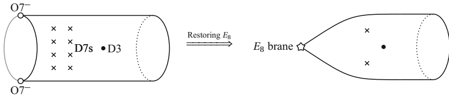
Fig. 3.1 Depiction of the brane realization of the Coulomb branch \mathcal{H} of rank 1 E-string theory. The left shows perturbative configuration where E_8 flavor is broken. The geometry depicted is a cylinder divided by the orientifold \mathbb{Z}_2 , and the gray curve between O7 s are identified with the other curve between them. Colliding O7 s and 6 D7 , they non-perturbatively become an E_8 brane, and the Coulomb branch looks like the right picture. The position of the D3 corresponds to the Coulomb branch coordinate u , the E_8 -brane represents the superconformal point where the E_8 theory of Minahan and Nemeschansky is realized, and the remaining 2 D7 -branes represents two free-hyper point in \mathcal{H} . Far away from the singular points, the Coulomb branch is a cylinder described by (3.6)
