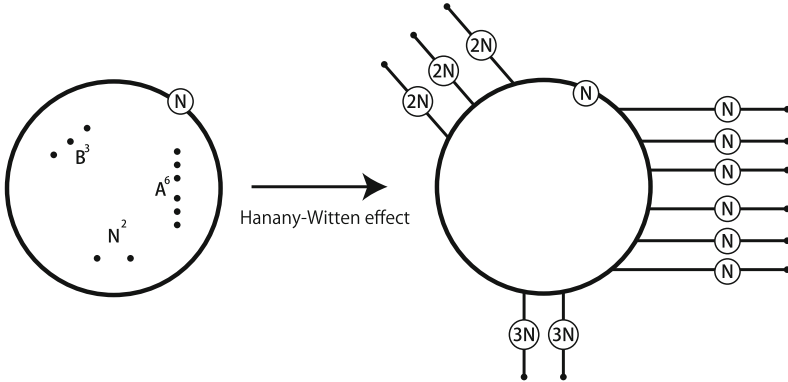
Fig. 3.6 Pulling out eleven 7-branes \mathbf{A}^6\mathbf{B}^3\mathbf{N}^2 from the inside of the N circles of 5-brane creates the 5-brane junction with three legs due to Hanany–Witten effect. Each leg consists of 6N 5-branes. These 5-branes are grouped as shown in the right hand side of the figure and each group is terminated at a 7-brane. From: [23]
