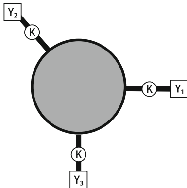
Fig. 3.2 The 5-brane web configuration introduced in [25]. It has three legs made up of K 5-branes of type (1, 0) , (0, 1) and (1, -1) respectively. The 5-branes in each leg terminate on 7-branes of the same type. The ending pattern of each leg at the 7-branes determines the Young diagram Y_i . Since the internal 5-brane web configuration is determined (up to flop transitions) by the boundary data K and Y_i ( i = 1, 2, 3 ), we do not write it explicitly. The 5d SCFT from this web is the 5d uplift \widehat{\mathcal{T}}_K\{Y_1, Y_2, Y_3\} of the class S theory \mathcal{T}_K\{Y_1, Y_2, Y_3\} . From: [23]
