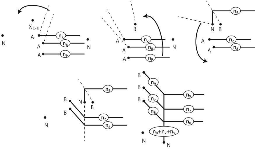
Fig. 3.12 The 7-brane rearrangement inside the circle of 5-branes. Extra 5-branes attached to the three A branes create the junction of 5-branes due to the Hanany–Witten effect. From: [23]
