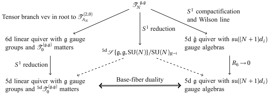
Fig. 3.13 Relation between \mathcal{T}_N^{(g,g)} and 6d and 5d gauge theories. After taking R_6 \rightarrow 0 limit and decoupling the 5d G = \text{SU}(N) vector, Wilson line and tensor vev becomes different mass deformations (denoted by dashed lines) of the 5d SCFT 5d \mathcal{T}_N^{(g,g)} , and this relation is nothing but the base-fiber duality when \mathfrak{g} = A
