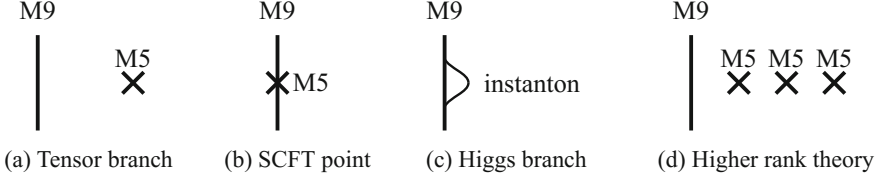
Fig. 2.4 The E-string theory is the worldvolume theory on an M5-brane probing an M9-brane. Higgs branch is identified with instanton moduli. The higher rank generalization refers to multiplet M5-branes probing M9
