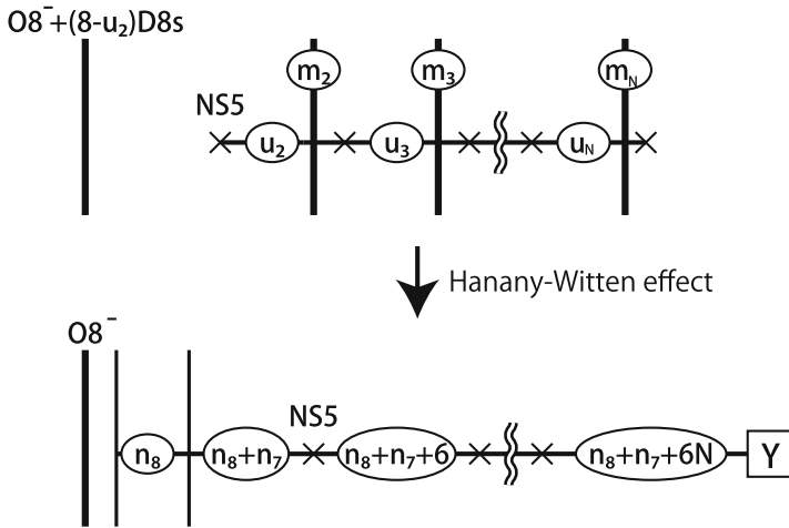
Fig. 3.7 Upper: The same as Fig. 2.12. Lower: Type I' configuration after the pre-processing Hanany–Witten transitions. There are two D8 branes near the O8^- plane, each has n_7 and n_8 D6 branes ending on it, and u_N + 6 D8 branes on the right side of the N th NS5 brane. The K = n_8 + n_7 + 6N D6 branes end on the stack of u_N + 6 D8 branes, and the pattern of the ending is specified by the Young diagram Y_1 (3.61) [35]. From: [23]
