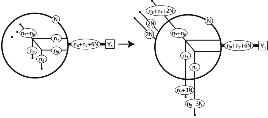
Fig. 3.10 Pulling the eleven 7-branes from the inside of the circles of 5-branes, we again obtain the junction of 5-branes with three external legs. From: [23]
