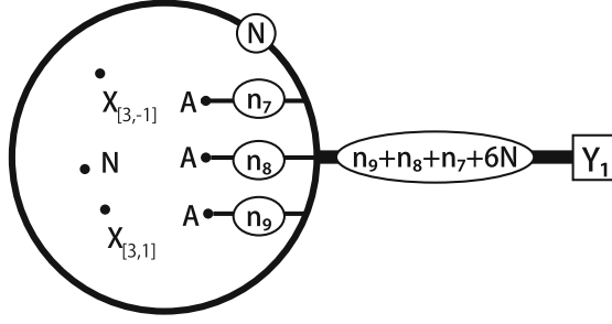
Fig. 3.11 The Type IIB web for the 6d theory \mathcal{F}_*^{(M9,su)}\{u_i\} on S^1 with Kaluza–Klein modes. We have N circles of 5-brane. Outside the circles, we have a leg of 6N + n_7 + n_8 + n_9 5-branes terminated at 7-branes. Inside the circles, we have six 7-branes A^3 X_{[3,-1]} N X_{[3,1]} . n_7 , n_8 and n_9 5-branes are attached to three A 7-branes respectively. From: [23]
