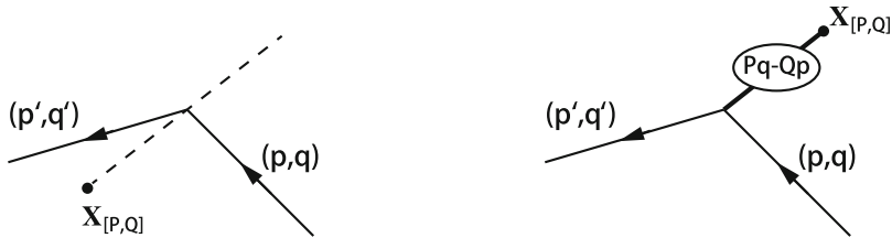
Fig. 3.3 The Hanany–Witten effect between a 7-brane and a 5-brane. From: [23]
