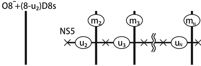
Fig. 2.12 Type I' brane construction of \mathcal{T}_N^{(M9, \mathfrak{su})}\{u_i\} [41, 42]. The \times mark represents an NS 5 brane, the horizontal line represents the stack of D6 branes, and the vertical lines represent D8 branes or the stack of O8 - plane and D8 branes. The symbols in the circles are the numbers of the branes there. The m_i D8 branes intersecting with u_i D6 segments supports \mathfrak{su}(m_i) flavor symmetry. The gauge anomaly cancellation requires m_i = 2u_i - u_{i-1} - u_{i+1} . From: [48]
