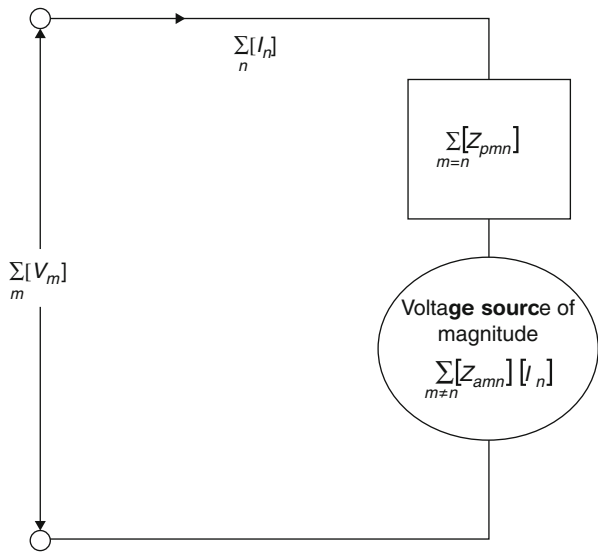
Fig. 18.3 Equivalent circuit of CMS activity based model of a polyphase system
