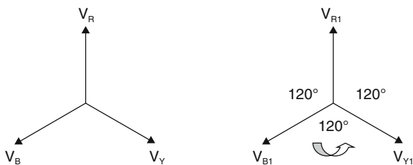
Fig. 8.8 Phasor diagram of phase voltages and positive sequence voltages
