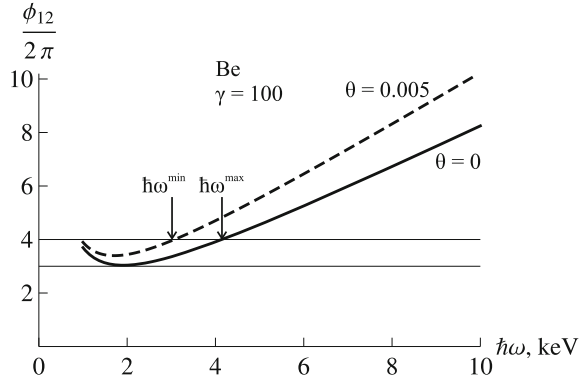
Fig. 5.14 The phase diagram for the outgoing angles of RTR photons \theta = 0 (the lower curve) and \theta = 5 mrad for E = 50 MeV; Be— \ell_1 = 10 \mu\text{m} , \ell_2 = 10 \mu\text{m}
