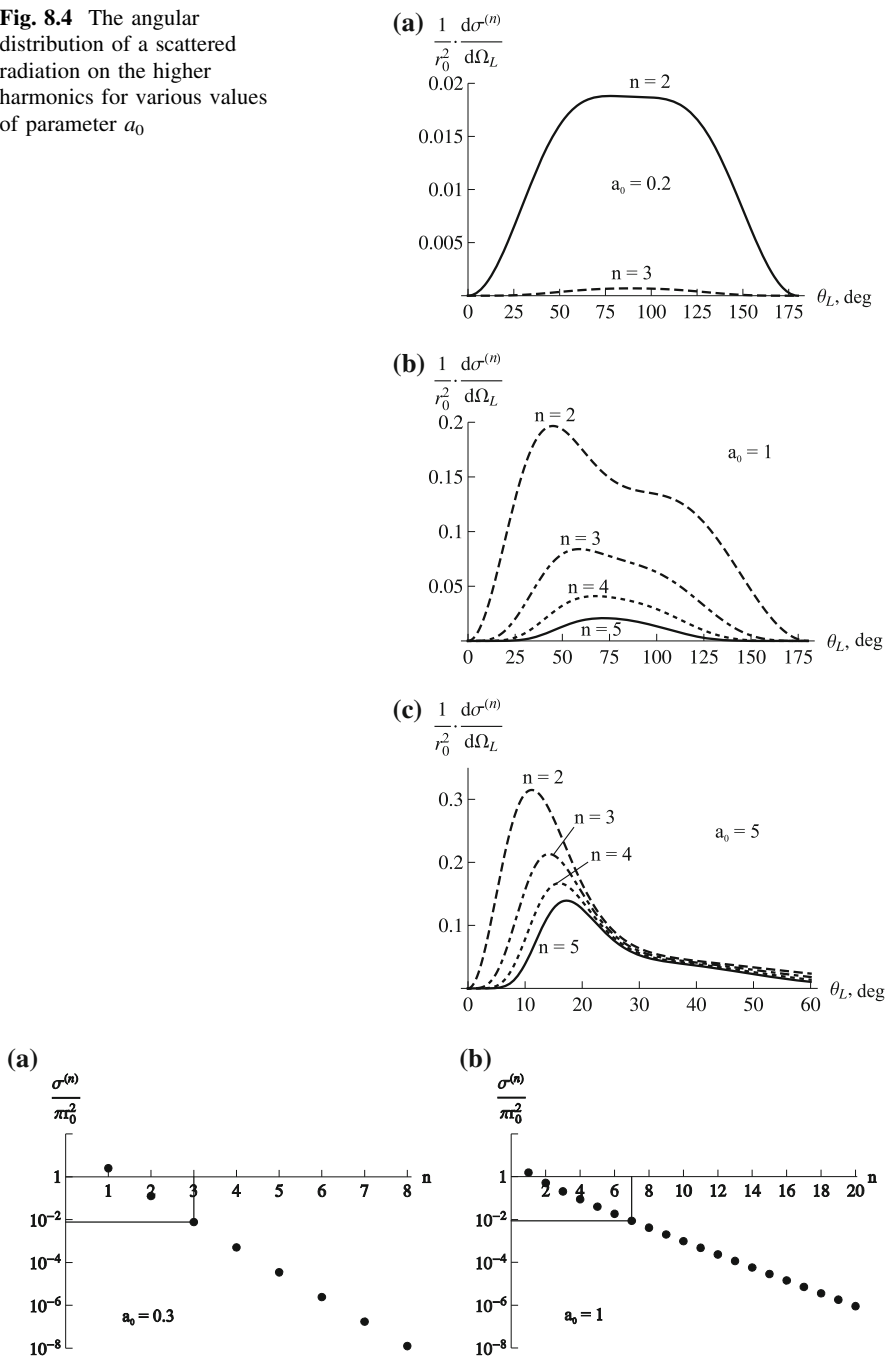
Fig. 8.5 Dependence of the “partial” cross-sections of intense wave scattering by a rest electron for the parameter a_0 = 0.3 (a) and a_0 = 1 (b)
