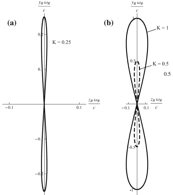
Fig. 3.2 An electron trajectory in R -system in yz -plane for various values of parameter K
