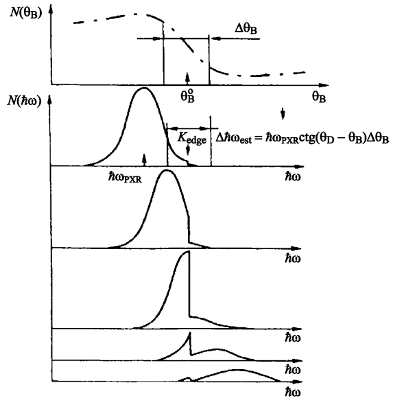
Fig. 6.12 History of a shape of the spectral PXR line in case of changing the orientation angle \theta_B
