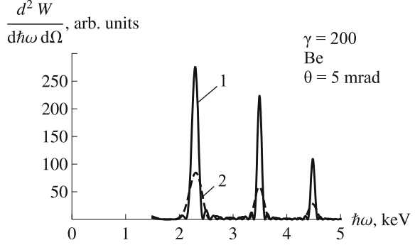
Fig. 5.10 Spectrum of RTR generated by an electron beam with energy E = 100 MeV in a stack from N = 10 beryllium foils (the curve 1), separated by vacuum gaps ( \ell_1 = 10 \mu , \ell_2 = 50 \mu ), and in the stack with N = 5 foils (the curve 2). The angle of observation \theta = 5 mrad
