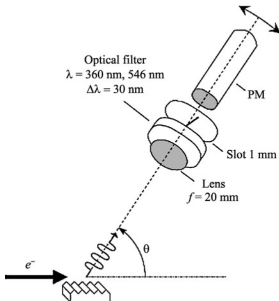
Fig. 7.25 The scheme of the experiment [19] for study of the Smith–Purcell optical radiation from a beam of electrons with energy 855 MeV
