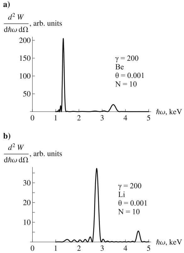
Fig. 5.13 The RTR spectra for layered targets from different materials
