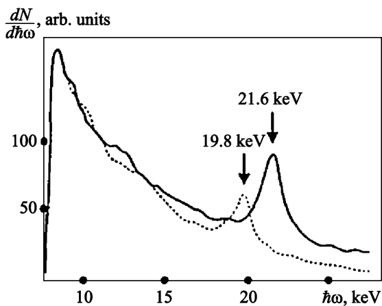
Fig. 6.10 The spectra measured at 2\theta_B = 312 mrad (the curve) and 2\theta_B = 324 mrad (the points)
