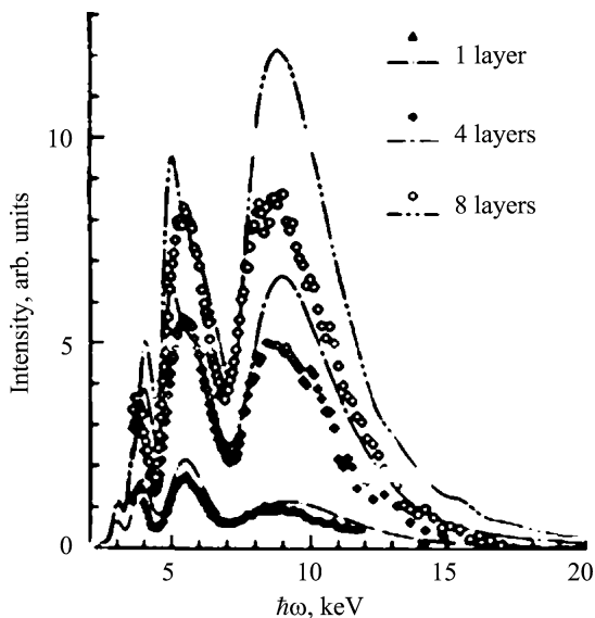
Fig. 5.23 Comparison of measured and calculated RTR spectra of electrons with energy 1 GeV in a target from mylar of 1, 4, 8 layers, with thickness \ell_1 = 50 \mu\text{m} and period d = \ell_1 + \ell_2 = 250 \mu\text{m}
