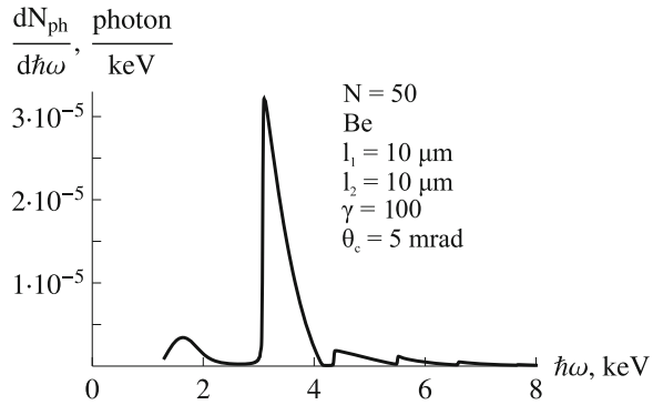
Fig. 5.15 The RTR photon spectrum in a layered Be target
