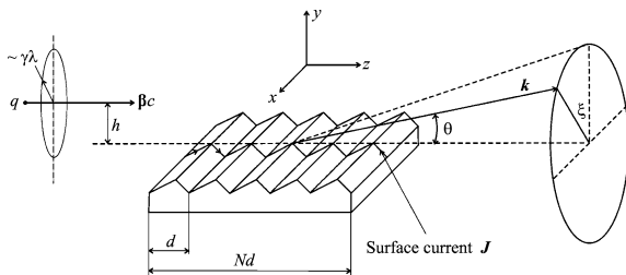
Fig. 7.1 Periodically changing current \mathbf{J} induced by a flying charge above the deformed conducting surface
