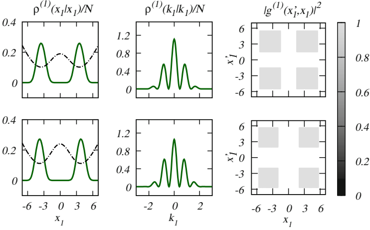
Fig. 5.4 Density distribution, momentum distribution and first-order coherence obtained by using the GP equation for high barriers. The first two columns show the GP one-particle density \rho^{(1)}(x_l|x_l)/N (left) and the GP one-particle momentum distribution \rho^{(1)}(k_l|k_l)/N (middle) at barrier heights A = 19 and A = 24 (solid lines). In the first column the trapping potential is also shown (dashed-dotted line). The GP equation models the density well, but fails at the computation of the momentum distribution, compare with Fig. 5.3. The third column shows the absolute value squared of the normalized first-order correlation function |g^{(1)}(x'_l, x_l)|^2 computed with the GP equation at the same barrier heights. The normalized first-order correlation function is incorrectly described by the solution of the GP equation. The quantities shown are dimensionless
