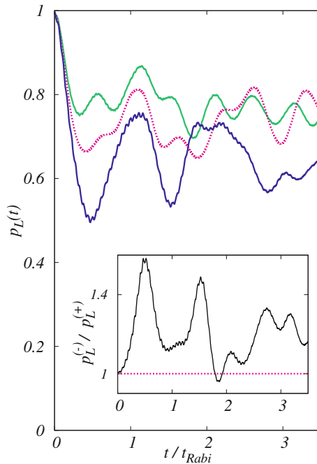
Fig. 7.1 Bose–Hubbard versus full-Hamiltonian, numerically-exact dynamics of attractive and repulsive Josephson junctions. Shown is the “survival probability” as a function of time, p_L(t) , computed with the full many-body Hamiltonian for attractive (solid green line) and repulsive (solid blue line) interaction. MCTDHB with M = 8 orbitals was used for the full many-body results. The Bose–Hubbard result (dashed magenta line) is for both attractive and repulsive interactions. The parameters used are N = 20 , |U/J| = 0.226 , |\lambda_0| = 0.0129 , and t_{Rabi} = 140.66 . The inset shows the ratio p_L^{(-)}/p_L^{(+)} of attractive to repulsive “survival probabilities” as a function of time. The black–solid line is the full-Hamiltonian results which exhibit a complex dynamics, whereas the dashed–magenta line is the Bose–Hubbard result, showing no dynamics at all. All quantities are dimensionless
