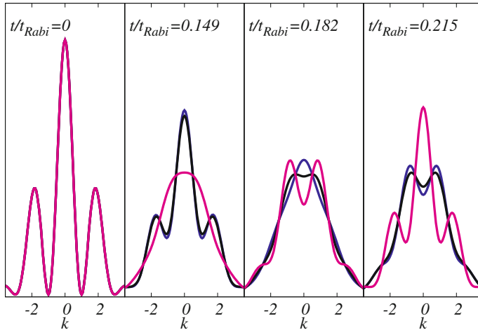
Fig. 8.3 Quench dynamics in a double well as in Fig. 8.2. Shown is the one-particle momentum distribution of the exact solution ( blue line ), the Bose–Hubbard model using time-dependent ( black line ) and time-independent ( magenta line ) Wannier functions at different times. The initial state is fully coherent and for some time the three results have similar momentum distributions (not shown). Differences between the results occur at later times whenever their respective natural orbital occupations differ, compare Fig. 8.2. The Bose–Hubbard result using time-dependent Wannier functions is always much closer to the exact one than the one using time-independent Wannier functions
