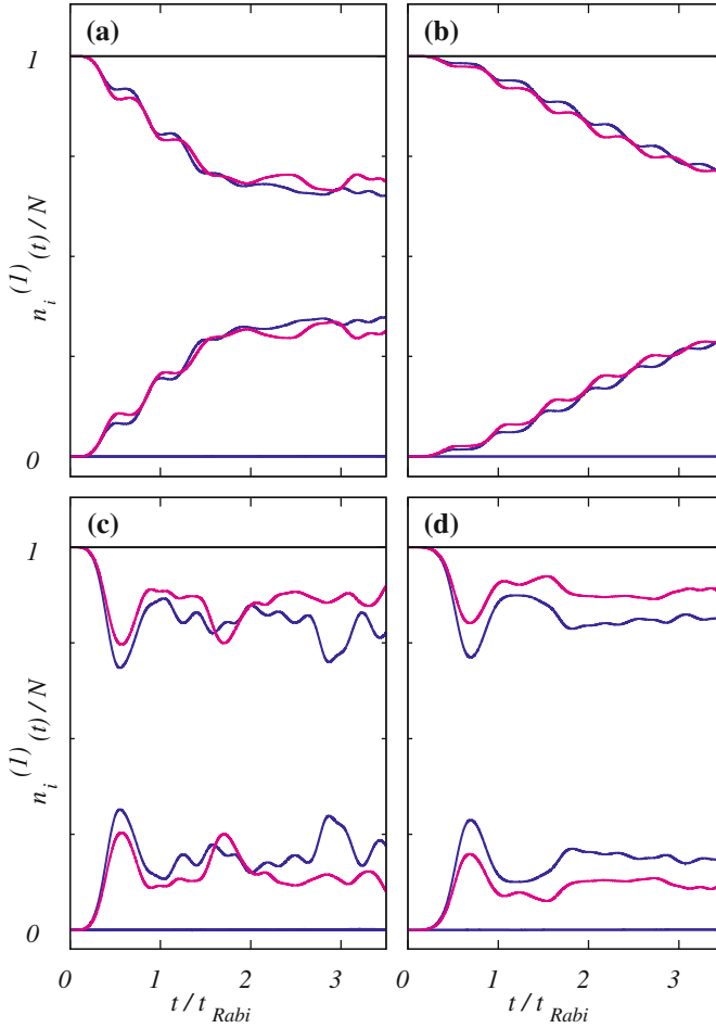
Fig. 6.3 Natural orbital occupations n_i^{(1)}(t) for the same parameter values as in Fig. 6.2. Shown is the full many-body result (solid blue lines) together with the respective Gross–Pitaevskii (solid black lines) and Bose–Hubbard (solid magenta lines) results. The full many-body result is seen to fragment quickly in all cases shown. While the Bose–Hubbard results follow qualitatively the full many-body results for \lambda = 0.152 in (a) and (b), this is not the case for slightly stronger interaction at \lambda = 0.245 shown in (c) and (d). In all cases shown only two natural orbitals of the full many-body result are macroscopically occupied. The Gross–Pitaevskii result has only one natural orbital and is therefore restricted to a fully condensed system at all times. All quantities shown are dimensionless.
