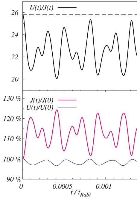
Fig. 8.4 Time-dependence of the hopping J(t) and the on-site interaction matrix element U(t) of the Bose-Hubbard model with time-dependent Wannier functions for the quench in Fig. 8.2. Top : the ratio U(t)/J(t) oscillates rapidly with a large amplitude between about 26 and 20. Note the time scale. The ratio is always considerably smaller than its initial value ( dashed line ). Bottom : The ratios J(t)/J(0) and U(t)/U(0) oscillate in time. J(t) is always larger, U(t) always smaller than its initial value. The oscillations are due to a rapid expansion and contraction of the density following the quench. J(t) varies over almost 25%, U(t) over about 4% of its initial value. The respective BH results with time-independent Wannier functions are constant in time and are not shown
