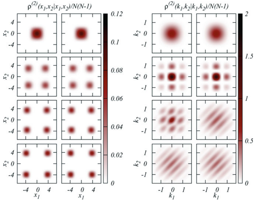
Fig. 5.5 Two-particle density and two-particle momentum distribution at different barrier heights. The first two columns (from left to right) show the two-particle density \rho^{(2)}(x_1, x_2|x_1, x_2)/N(N-1) of the many-body (left) and BMF (right) wave function for the barrier heights A = 0, 13, 19, 24 , from top to bottom. At low barrier heights ( A = 0, 13 ) the system is condensed, and the two-particle density factorizes into a product of the one-particle densities. At higher barriers ( A = 19, 24 ), the system fragments and the two-particle density does not factorize into a product of the one-particle densities. The fragmentation transition is not visible in the two-particle density. The results of the many-body and BMF wave function cannot be distinguished at any barrier height. The third and fourth column show the two-particle momentum distribution \rho^{(2)}(k_1, k_2|k_1, k_2)/N(N-1) of the many-body (left) and BMF (right) solution at the same barrier heights as above. The transition from a condensed state to a fragmented state is clearly visible. At A = 19 the BMF solution does not reproduce the many-body results. The system is in a true many-body state, inaccessible to mean-field methods. At even higher barriers A \geq 24 the system fully fragments, and a mean-field description is applicable again. The quantities shown are dimensionless
