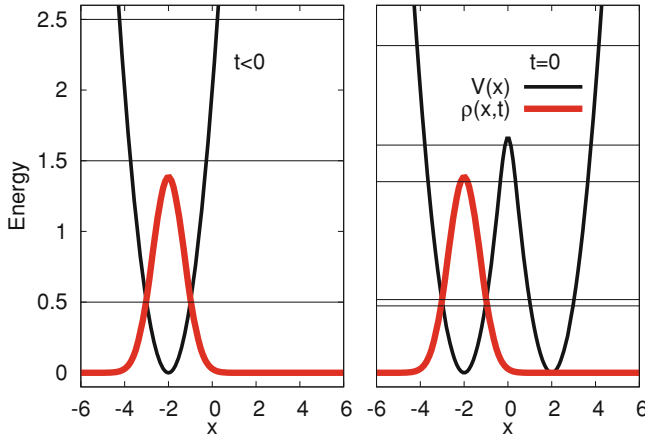
Fig. 6.1 Preparation procedure. Shown is the density (red line) of the many-body ground state in one trap (left) and the subsequent switch to a different potential in which the system evolves in time (right). The trapping potential (thick black line) changes from harmonic (left) to a symmetric double well (right). The parameter values shown for the system shown here are M = 8 , N = 20 , \lambda = \lambda_0(N - 1) = 0.152 . Also shown are the single-particle energy levels (thin black lines) in the respective trapping potentials. The lowest four single-particle energy levels e_1 = 0.473 , e_2 = 0.518 , e_3 = 1.352 and e_4 = 1.611 of the double-well potential V(x) (right) are lower than the barrier height V(0) = 1.667
