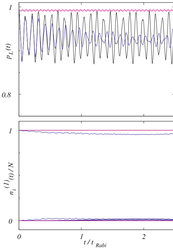
Fig. 6.4 Full quantum dynamics of a 1D bosonic Josephson junction at \Lambda = 18.1 . Top as in Fig. 6.2 the full many-body result (blue line) for the probability of finding a boson in the left well, p_L(t) , is shown. The full many-body solution is self-trapped on the time scale shown with \bar{p}_L(2t_{\text{Rabi}}) = 0.93 . Note the scale. Bottom as in Fig. 6.3 the natural orbital occupations are shown (lines). For comparison, the respective Gross–Pitaevskii (solid black lines) and Bose–Hubbard (solid magenta lines) results are shown as well. The parameter values are N = 20 , \lambda = 1.96 , M = 8 . Since the full many-body solution shows little fragmentation the Gross–Pitaevskii result is close to the full many-body one. The Bose–Hubbard result differs qualitatively. All quantities shown are dimensionless.
