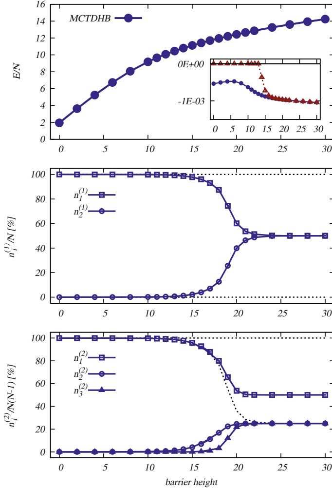
Fig. 5.1 Energy per particle, natural orbital and natural geminal occupations of the ground state of N = 1,000 bosons at \lambda_0 = 0.01 in a harmonic trap with a central barrier. Shown is the dependence on the barrier height. Top: energy per particle E/N of the many-body solution. Inset: energy difference per particle between the best mean-field and the GP solution, (E_{BMF} - E_{GP})/N (triangles), and between the many-body and GP solution, (E_{MCTDHB} - E_{GP})/N (circles). Middle: the eigenvalues n_1^{(1)} and n_2^{(1)} of the first-order RDM \rho^{(1)}(x_1|x'_1) . The ground state fragments with increasing barrier height. Bottom: the eigenvalues n_1^{(2)} , n_2^{(2)} and n_3^{(2)} of the second-order RDM \rho^{(2)}(x_1, x_2|x'_1, x'_2) . The dashed lines in the middle and bottom panel indicate upper and lower bounds on the largest eigenvalue of the first- and second-order RDMs. See text for details. The quantities shown are dimensionless
