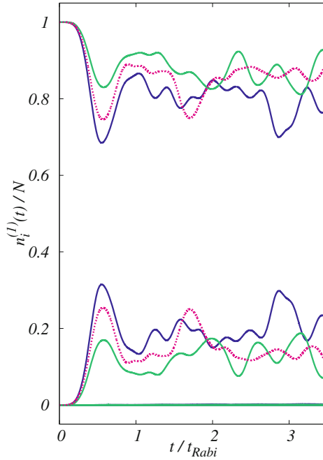
Fig. 7.2 Bose–Hubbard versus full-Hamiltonian, numerically-exact dynamics of attractive and repulsive Josephson junctions. Shown are the occupation numbers of the first order RDM as a function of time, n_i^{(1)}(t) , computed with the full many-body Hamiltonian for attractive (solid green line) and repulsive (solid blue line) interaction. The Bose–Hubbard result (dashed magenta line) is for both attractive and repulsive interactions. The two-site Bose–Hubbard dynamics has two occupation numbers only. The full-Hamiltonian dynamics has many occupation numbers. It is seen that the occupation numbers n_{i>2}^{(1)}(t) are essentially zero. The parameters used are the same as in Fig. 7.1. All quantities are dimensionless
