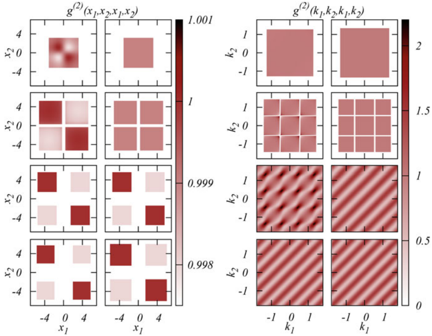
Fig. 5.6 Second-order coherence at different barrier heights. The first two columns (from left to right) show the diagonal of the normalized second-order correlation function in real space g^{(2)}(x_1, x_2, x_1, x_2) of the many-body (left) and BMF (right) solution at barrier heights A = 0, 13, 19, 24 , from top to bottom. g^{(2)}(x_1, x_2, x_1, x_2) is very close to one at all barrier heights. Note the scale! The system seems to be second-order coherent and the results of the many-body and BMF solution agree well with each other. The third and fourth column depict the diagonal of the normalized second-order correlation function in momentum space g^{(2)}(k_1, k_2, k_1, k_2) of the many-body (left) and BMF (right) solution at the same barrier heights. The fragmentation transition is clearly visible between A = 13 and A = 24 . At A = 19 there are strong many-body correlations between the momenta (local maxima in black color) and g^{(2)}(k_1, k_2, k_1, k_2) exhibits a complicated pattern, see text for more details. A mean-field description fails here. In the limit of high barriers, A \geq 24 , the correlations of the many-body state become again describable by those of the BMF solution. The quantities shown are dimensionless
