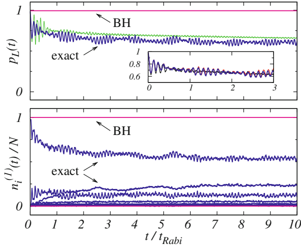
Fig. 6.5 Emergence of equilibration of the density at interaction strength \lambda = 4.9 . Top same as Fig. 6.2, but for N = 10 (solid blue line) and N = 100 (solid green line). The respective Bose–Hubbard (solid magenta lines) results are on top of each other. In contrast to the Bose–Hubbard dynamics which is completely self-trapped, the full many-body dynamics is not. p_L(t) tends towards its long-time average p_L = 0.5 . For N = 100 particles M = 4 orbitals were used. The inset shows the convergence of the full many-body solution for N = 10 bosons: M = 4 (solid black line), M = 10 (solid blue line), M = 12 (solid red line). The M = 4 result follows the trend of the converged M = 12 result. Bottom corresponding natural orbital occupations for N = 10 bosons. The system becomes fragmented and roughly four natural orbitals are macroscopically occupied. All quantities are dimensionless.
