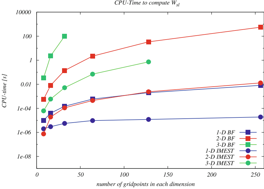
Fig. A.1 Performance of the IMEST-algorithm and the brute force algorithm. Shown is the average CPU-time needed for the evaluation of \mathbf{W}_{sl} as a function of the number of grid points in each direction n_{j,j} = 1, \dots, D (see text for details) and different dimensions D = 1, 2, 3 . The times are obtained by averaging over fifty evaluations of \mathbf{W}_{sl} . The CPU-times of the IMEST-algorithm (lines with circles) are always below the CPU-times of the brute force algorithm (lines with squares). Even in 1D the IMEST-algorithm is orders of magnitude faster than the brute force algorithm. The larger the dimension the greater is the difference between the CPU-times of the two algorithms. The CPU-time needed by the IMEST algorithm in 2D is about the same as that of the brute force algorithm in 1D up to about n_j = 256
