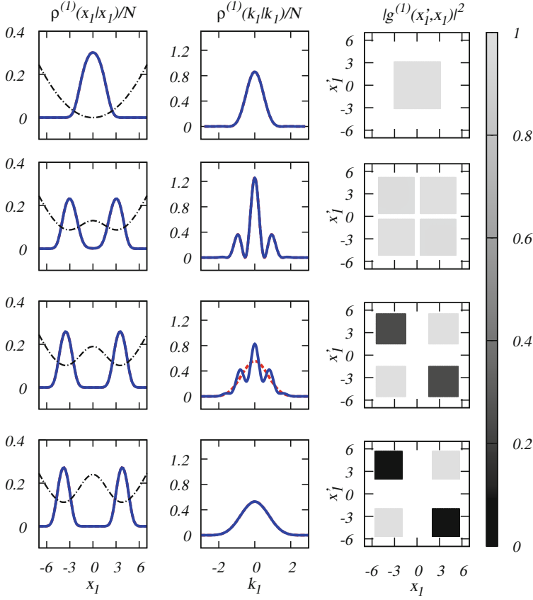
Fig. 5.3 Density distribution, momentum distribution and first-order coherence. The first two columns show the one-particle density \rho^{(1)}(x_1|x_1)/N and the one-particle momentum distribution \rho^{(1)}(k_1|k_1)/N of the many-body solution ( solid lines ) and of the BMF solution ( dashed line ), respectively. The trapping potential is shown as a dashed-dotted line. From top to bottom the height of the central barrier is A = 0, 13, 19, 24 . The BMF result agrees well with the many-body result for a large range of barrier heights. Only at A = 19 , in the many-body regime, deviations are visible in the momentum distribution. See text for details. The third column shows the absolute value squared of the normalized first-order correlation function |g^{(1)}(x'_1, x_1)|^2 at the same barrier heights. An initially coherent condensate splits into two separate condensates which are no longer mutually coherent. Only the coherence within each of the wells is preserved. The quantities shown are dimensionless
