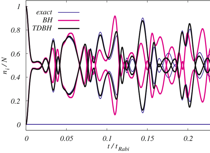
Fig. 8.2 Quantum quench dynamics in a double well. Shown are the natural orbital occupations following a quench from \lambda = 0 ( U/J = 0 ) to \lambda = 0.6 ( U/J = 25.8 ) as a function of time. The results of the BH model using time-independent (magenta lines), and time-dependent (black lines) Wannier functions are depicted together with those of the numerically exact solution of the many-body Schrödinger equation (blue lines). If time-independent Wannier functions are used the BH results deviate from the exact ones after short times. If time-dependent Wannier functions are used the BH results follow the exact ones closely. Starting from a fully condensed state the dynamics is complex and shows oscillations between partially and fully fragmented states
