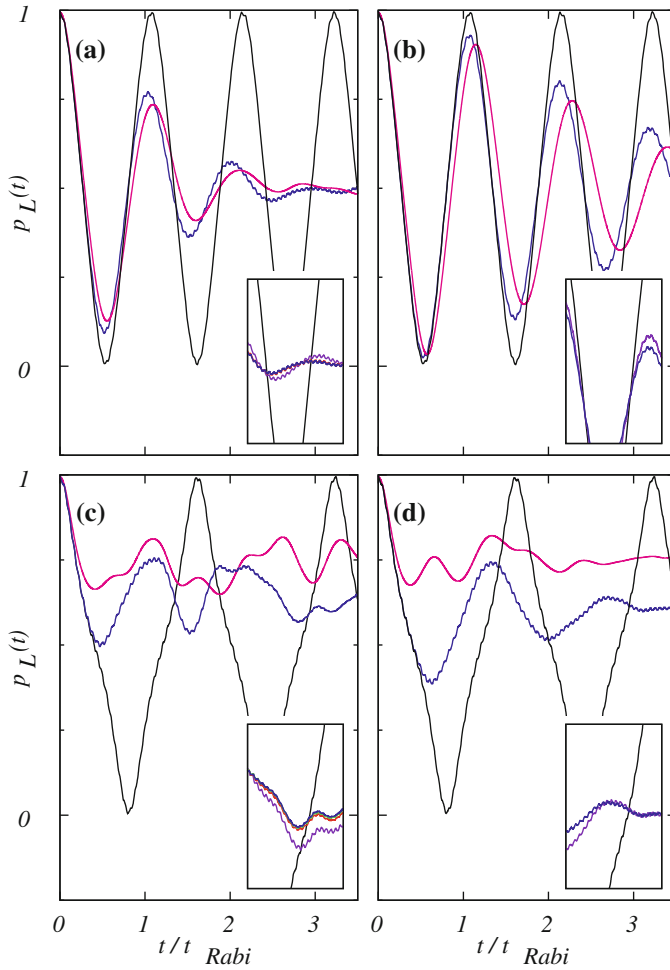
Fig. 6.2 Full quantum dynamics of a 1D bosonic Josephson junction below ( \Lambda < \Lambda_c ) and above ( \Lambda > \Lambda_c ) the transition to self-trapping as defined by the two-mode Gross-Pitaevskii theory. Shown is the full many-body result (solid blue lines) for the probability of finding a boson in the left well, p_L(t) . For comparison, the respective Gross-Pitaevskii (solid black lines) and Bose-Hubbard (solid magenta lines) results are shown as well. The parameter values are: a N = 20 , \lambda = 0.152 and b N = 100 , \lambda = 0.152 ( \Lambda < \Lambda_c ), c N = 20 , \lambda = 0.245 and d N = 100 , \lambda = 0.245 ( \Lambda > \Lambda_c ). The Gross-Pitaevskii and Bose-Hubbard results are found to deviate from the full many-body results already after short times. The insets show the convergence of the full many-body results. a,c: M = 2 (solid purple line), M = 4 (solid red line), M = 6 (solid green line), M = 8 (solid blue line). The M = 2 results are seen to deviate slightly from the converged results for M \geq 4 . b,d: The results for M = 2 (solid purple line) and M = 4 (solid blue line) are shown. All quantities shown are dimensionless.
