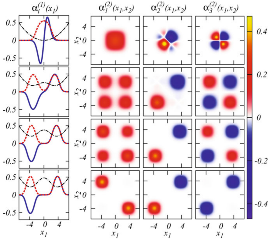
Fig. 5.2 Natural orbitals and geminals at different barrier heights. First column: the natural orbitals \alpha_1^{(1)}(x_1) (dashed red line) and \alpha_2^{(1)}(x_1) (solid blue line) of the many-body solution at different barrier heights A = 0, 13, 19, 24 , from top to bottom. The trapping potential is shown as a dashed-dotted black line in the first column. The state of the system changes from condensed to fragmented between A = 13 and A = 24 . Second to fourth columns: natural geminals \alpha_1^{(2)}(x_1, x_2) , \alpha_2^{(2)}(x_1, x_2) and \alpha_3^{(2)}(x_1, x_2) from left to right at the same barrier heights as above. While the natural orbitals remain qualitatively unchanged during the fragmentation transition, the natural geminals take on their final shapes only when the system becomes fully fragmented. At low barrier heights only one natural geminal is occupied. At high barriers three natural geminals are occupied, see Fig. 5.1. The total energy is minimized by the occupation of a natural geminal that contributes practically nothing to the interaction energy. See text for more details. The quantities shown are dimensionless
