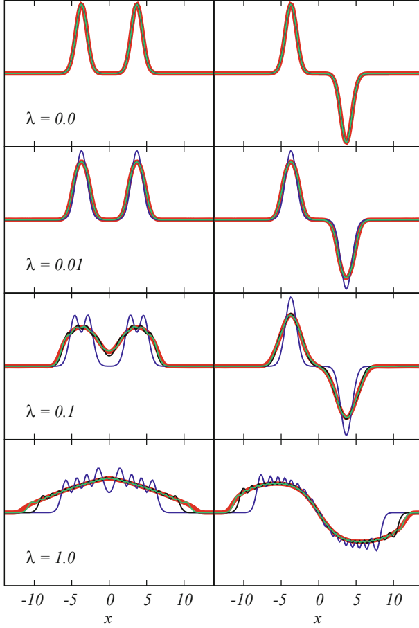
Fig. F.1 Expansion of natural orbitals in Wannier functions. Shown is the first ( left panels ) and the second ( right panels ) natural orbital of the ground state of N = 1000 bosons in a trap at different interaction strengths \lambda = 0, 0.01, 0.1, 1.0 (from top to bottom). MCTDHB (thick red lines) with M = 2 orbitals was used to obtain the natural orbitals. Also shown are the approximations \psi_k to the natural orbitals for different accuracies: \epsilon = 0.1 (blue), 0.01 (black), 0.001 (green). See text for details. Even at a medium accuracy of \epsilon = 0.01 a large numbers of bands \kappa is needed to represent the natural orbitals at any nonzero interaction strength: from top to bottom \kappa = 1, 3, 7, 28 . The corresponding many-body basis set sizes are astronomically large, see Table F.1
