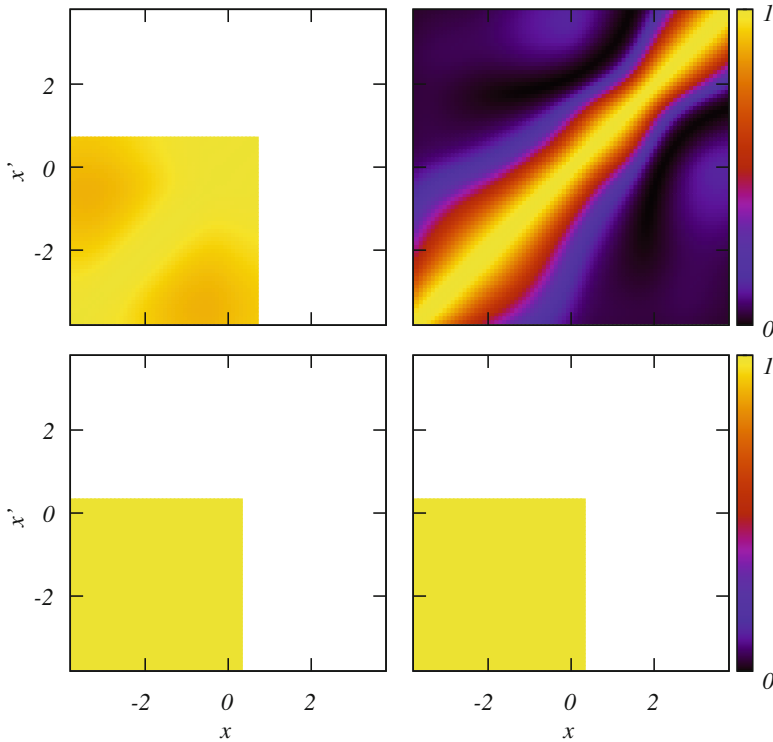
Fig. 6.6 Dynamics of the first order correlation function for \lambda = 4.9 at which the equilibration phenomenon of Fig. 6.5 occurs. Shown is |g^{(1)}(x', x; t)|^2 of N = 10 bosons at different times. Top left full many-body result at t = 0 . The initial state exhibits coherence over the entire extent of the system. Top right full many-body result at t = 10t_{Rabi} . The coherence is lost. The system is incoherent even on short length scales. Bottom left Bose-Hubbard result at t = 0 . Bottom right Bose-Hubbard result at t = 10t_{Rabi} . In contrast to the full many-body result, the Bose-Hubbard wave function remains completely coherent.
