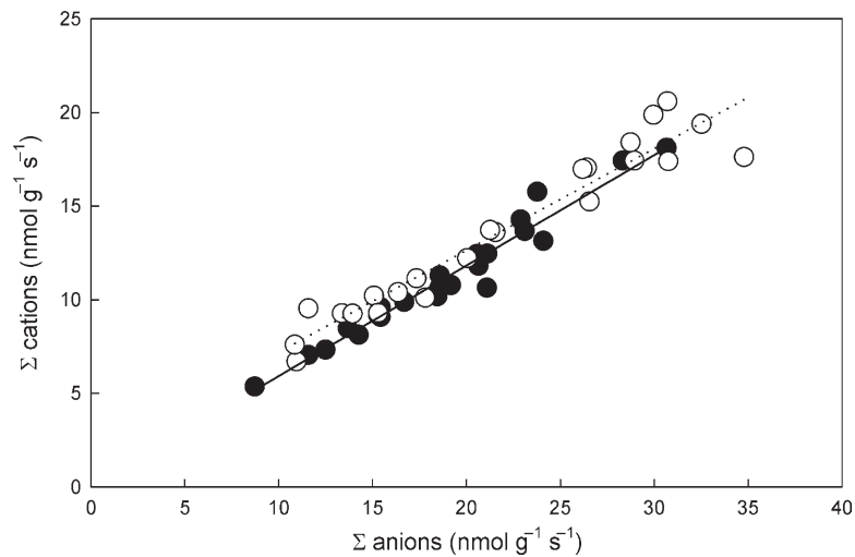
Fig. 3. Sum of anion plotted against the sum of cation flux per shoot mass for ammonium-fed plants ( closed symbols ) and nitrate-fed plants ( open symbols ). Anions are nitrate, chloride, sulfate and phosphate, and the major organic acids malate, succinate and citrate. Cations are ammonium, potassium, sodium, magnesium and calcium. A linear regression performed on the ammonium data is significant (solid line; F=493.7 , p<0.0001 ) and has a slope of 1.62 and r^2=0.96 . A linear regression performed on the nitrate data is significant (dotted line; F=284.5 , p<0.0001 ) and has a slope of 1.71 and r^2=0.93 . An analysis performed on the regression lines showed that the slopes are not significantly different ( F=2.96 , p=0.1 ).
