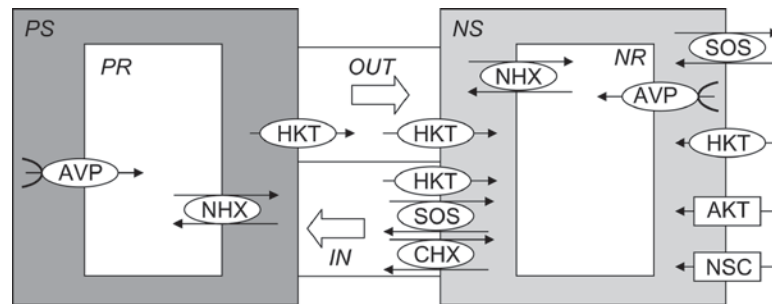
Fig. 4. Tentative assignment of plant transporter families to the telescope model. For simplicity only the cellular components of the model presented in Fig. 12.3 are shown. PS, PR, NS and NR stand for prioritised space, prioritised reservoir, non-prioritised space and non-prioritised reservoir, IN and OUT for inlet and outlet (see Fig. 3). Both K + -selective (e.g., AKT1) and non-selective channels (NSC) provide pathways for Na + uptake into cells but there is some evidence that their relative abundance differs between prioritised and non-prioritised tissues (e.g., leaf epidermis and mesophyll). Members of the HKT gene family have been implicated in Na + uptake into root epidermal cells but their main importance lies in the retrieval of Na + from the xylem (IN), although a function in loading and un-loading of the phloem (OUT) has also been proposed. Active export of Na + from cells is mediated by SOS1, which, together with a member of the CHX family, also provides a means for regulating long-distance Na + flux in the xylem. Compartmentalization of Na + into the vacuolar reservoirs by NHX1 homologues occurs in both prioritised and non-prioritised tissues, and is supported by the action of proton pumps such as the H + -PPase, AVP1. For details and references see main text.
