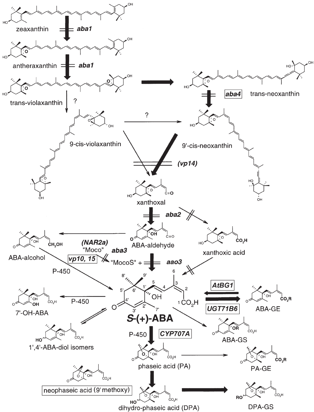
Fig. 4. Metabolic pathways of ABA after zeaxanthin, with positions of steps blocked in mutants indicated. Recently discovered genes are boxed (Modified from Finkelstein and Rock 2002).
