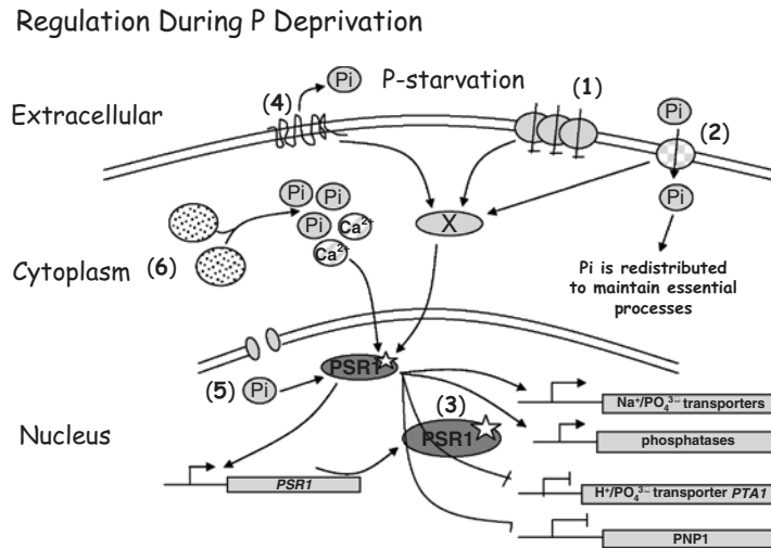
Fig. 6. Model depicting P-deprivation responses. When P becomes limiting in the growth medium, the \text{PO}_4^{3-} (Pi in figure)-uptake activity of the low affinity transporter (1) declines, but transport through the high-affinity system (2) is maintained. The declining \text{PO}_4^{3-} levels in the cell and/or transport of \text{PO}_4^{3-} exclusively through the high affinity system may provide a signal, designated X in this figure, that is transmitted to PSR1 in the nucleus and that enables PSR1 to activate transcription; the signal that alters PSR1 activity can even be just below the normal intracellular levels of \text{PO}_4^{3-} . Alteration of PSR1 during P deprivation is indicated with a star. PSR1 mRNA and protein abundance increases within 2 h of the transfer of cells to P-deficient medium (3), and this increased expression precedes activation of the \text{Na}^+/\text{PO}_4^{3-} transporter and the inducible phosphatase genes, and repression of PTA1 and PNP. Temporal difference in the expression of genes following the imposition of \text{PO}_4^{3-} deprivation may reflect the affinity of the individual promoters for PSR1. An alternative model is that the signal to activate PSR1 is transmitted when Pi dissociates from an external sensor (4); PSR1 might also respond to changes in the nuclear Pi concentration (5) as acclimation proceeds, cytoplasmic poly(P) is degraded, which buffers the cytoplasmic \text{PO}_4^{3-} concentration until the poly(P) stores are depleted (6); other mechanisms involving microRNA control and sumoylation may occur in vascular plants.
