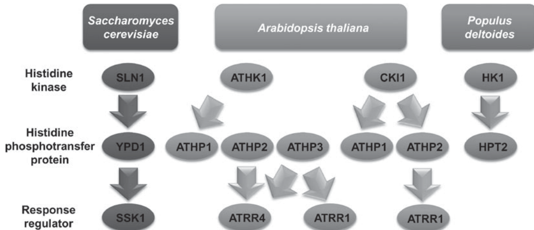
Fig. 4. Schematic representation of interacting partners of two component system. Histidine kinase interacts with histidine phosphotransfer protein, which further interacts with response regulator. In Saccharomyces cereviceae (Posas et al. 1996), histidine kinase (SLN1) interacts with histidine phosphotransfer protein (YPD1) and YPD1 interacts with response regulator (SSK1). In Arabidopsis thaliana , ATHK1 selectively interacts with ATHP1, not with ATHP2 and ATHP3, whereas ATHP2 and ATHP3 interact redundantly with ATRR4 (Urao et al. 2000). ATHP3 also interacts with ATRR1. In tree plant Populus deltoides , HK1 interacts with HPT2 (Chefdor et al. 2006).
