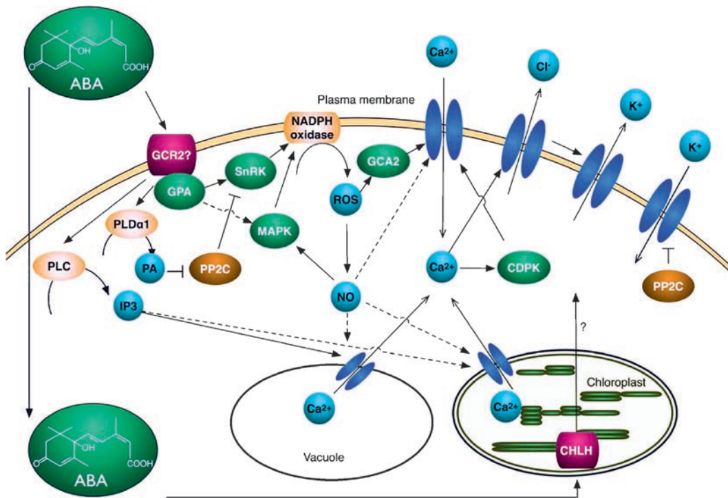
Fig. 3. Schematic illustration of Abscisic Acid (ABA) signaling in stomatal closure. Arrows indicate positive or negative interactions between the factors. Dashed arrows indicate possible regulation. See Chapter 3, p 40.
