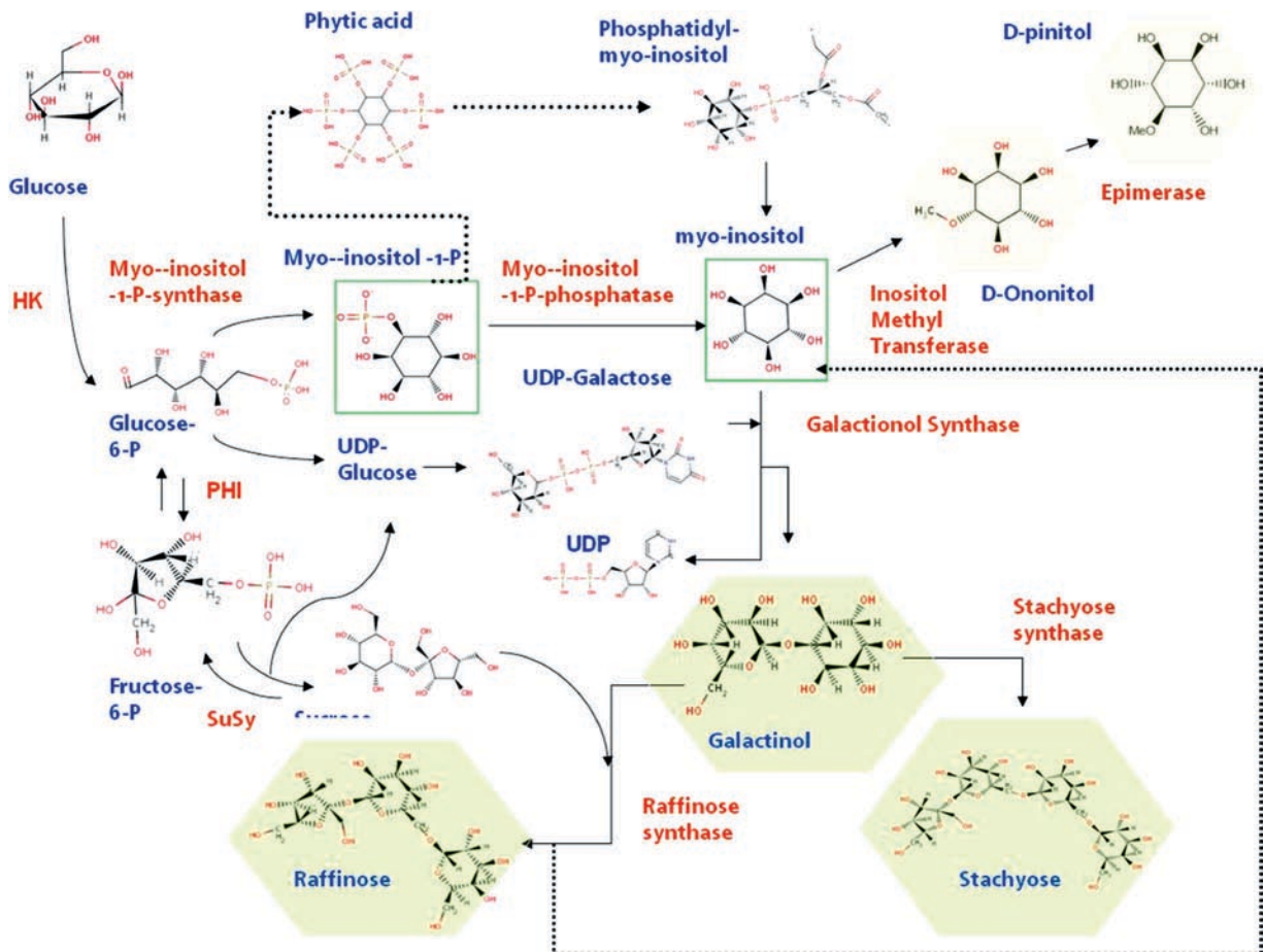
Fig. 4. Inositol utilization in synthesis of various osmolytes.
