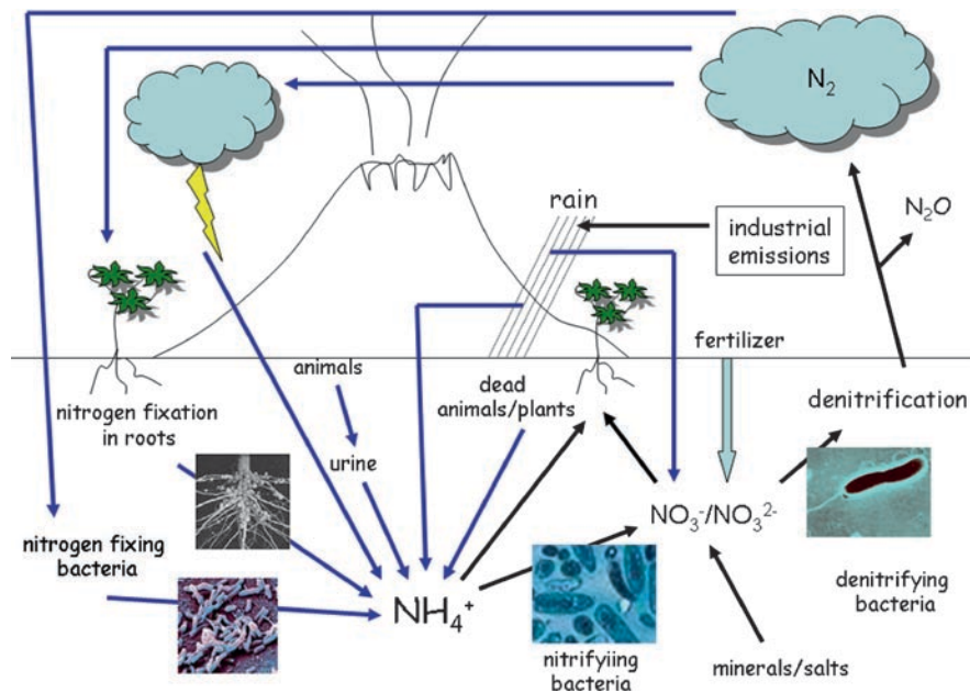
Fig. 14. Nitrogen cycle. Generally, \text{NO}_3^{2-} is the major form of nitrogen in the environment; although \text{NH}_4^+ and \text{NO}_2^- can be present at significant levels as well (high \text{NH}_4^+ levels are often toxic to organisms). As indicated, \text{NH}_4^+ can be generated from \text{N}_2 through the action of animal metabolism, lightning, volcanic activity and \text{N}_2 fixation. The fixation of \text{N}_2 can be performed by either free-living bacteria or bacteria associated with the nodules of leguminous plants. \text{NH}_4^+ can be oxidized through the action of nitrifying bacteria, which use ammonia monooxygenase to oxidize ammonia to hydroxylamine ( \text{NH}_2\text{OH} ) and then nitrite oxidoreductase to oxidize \text{NO}_2^- to \text{NO}_3^- . Oxides of nitrogen can be converted to \text{N}_2 by denitrification, an anaerobic process performed by specific bacteria (Modified from http://telstar.ote.cmu.edu/enviro/m3/s4/graphics/embedded/nitronodules.gif ; http://www.markergene.com/WebNewsletter7.4_files/image007.gif ; http://www.anoxkaldnes.com/Bilder/jpg/RD7.jpg ; http://staffwww.fullcoll.edu/tmorris/elements_of_ecology/images/bacteria_denitrifying.jpg ). See Chapter 15, p 310.
