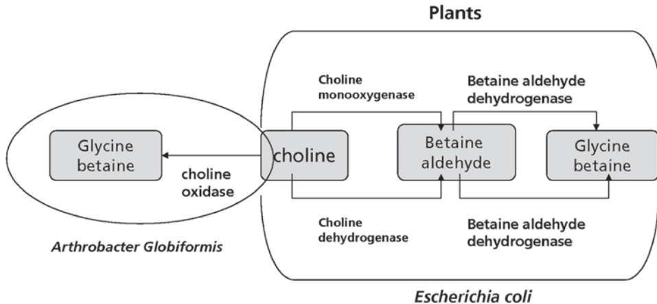
Fig. 2. Different pathways for synthesis of glycine betaine.
