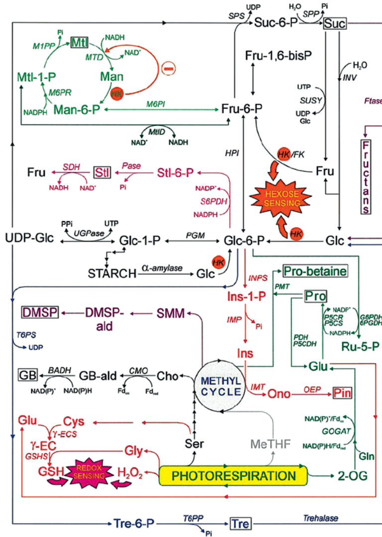
Fig. 1. Various osmolytes and their pathway of synthesis (Adapted from Hare et al. 1997).
