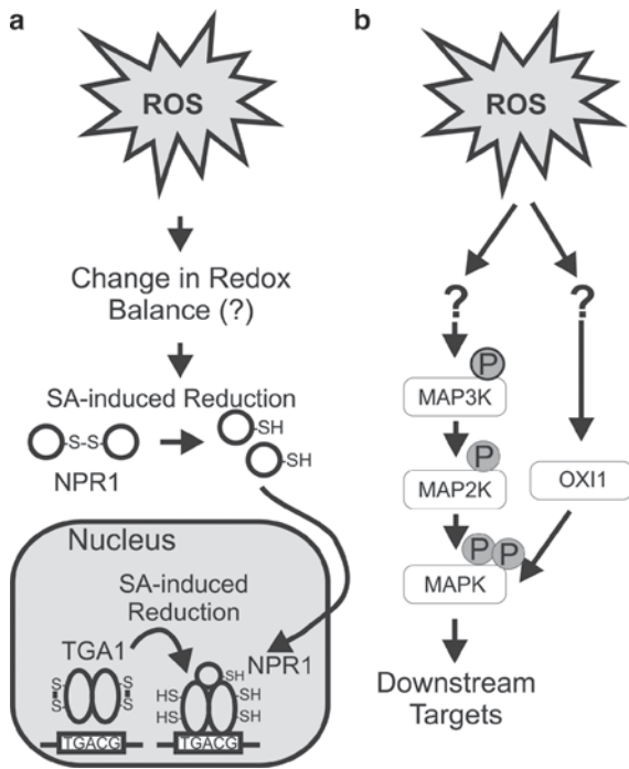
Fig. 2. Examples of reactive oxygen species (ROS) signalling. (a) PR1/TGA1 signalling. ROS-induced SA production causes the reduction of NPR1 and TGA1 to allow complex formation and DNA binding of the proteins. The encircled P indicates phosphorylation events; (b) MAPK signaling pathway. Phosphorylation cascade leads to transcriptional change and subsequently to stress response.
