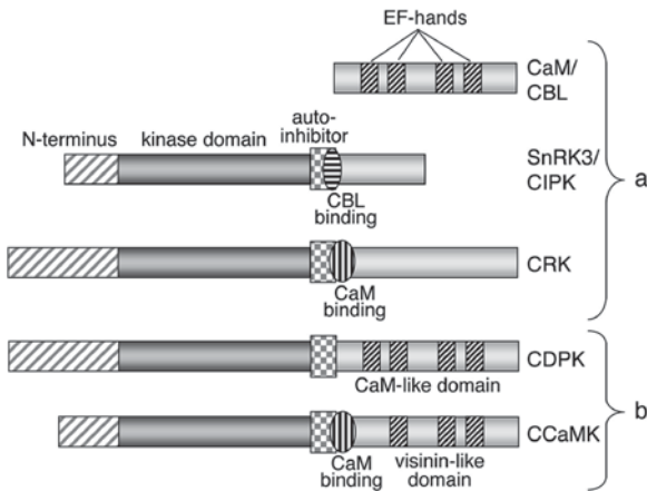
Fig. 2. Domain structure of plant calcium sensors. (a) Sensor relays and protein kinase partners. CaM and CBL are sensor relays that bind calcium through EF-hand motifs. CaM subsequently regulates many different target proteins including protein kinases (CRKs), whereas CBLs mainly activate CIPKs by interacting with the FISL/NAF domain (CBL binding) to release auto-inhibition; (b) Sensor protein kinases: In contrast to CRKs and CIPKs, the kinases CDPK and CCaMK can directly bind calcium through their EF-hand motifs. As a result, CDPKs function independently of other \text{Ca}^{2+} sensors whereas CCaMK activity can be further modulated by CaM (Adapted from Harper et al. 2004).
