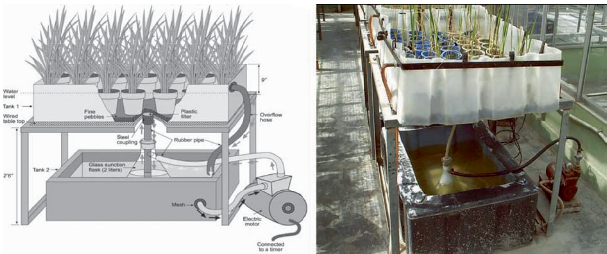
Fig. 6. Line diagram and actual system for adult-plant screening (Adapted from Singh and Mishra 2004).
