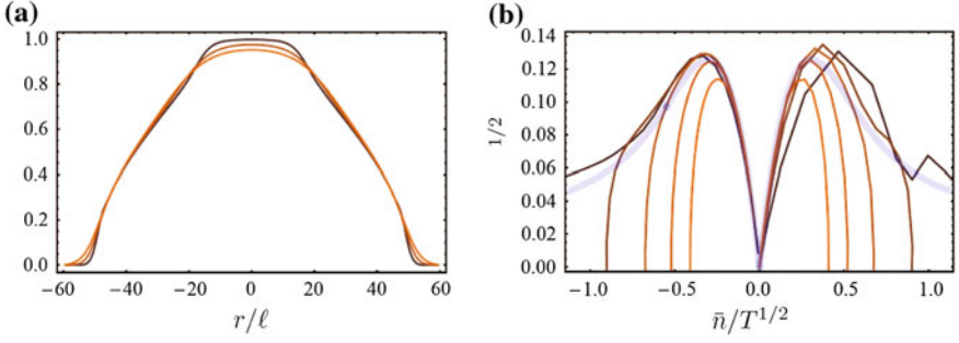
Fig. 13.2 Extracting universal behavior and dynamical critical exponents from density profiles of the trapped one-dimensional Bose-Hubbard model. a Exact density profiles of the one dimensional harmonically trapped hard core Bose-Hubbard model for N = 70 particles at temperatures \bar{T} \equiv T/t = 0.1, 0.24, 0.38 , with larger temperatures corresponding to lower central density. Here, r is the radial displacement in the trap and d is the lattice spacing. These density profiles are non-universal: for example, they depend on temperature. b Our construction for obtaining universal scaling curves applied to this system, plotting \bar{\kappa} \bar{T}^{d/z} versus \bar{n}/\bar{T}^{1/2} (defining \bar{\kappa} \equiv \kappa - \kappa_0 , \bar{n} \equiv n - n_0 , and \bar{T} = T/t ) for this d = 1 , z = 2 transition and temperatures \bar{T} = 0.1, 0.17, 0.24, 0.31, 0.38 . The compressibility is approximated by \kappa = \partial n / \partial \mu \approx (\partial n / \partial r) / (m \omega^2 r) , where \omega is the trap frequency, and \partial n / \partial r is obtained by numerically differentiating the density. Lower temperatures display a larger region of collapse. We observe good collapse up to T \sim 0.25t , and that the analysis accurately reproduces the homogeneous infinite system's scaling curve ( shaded gray line ) within \lesssim 10\% for T \gtrsim 0.05t for the transition near n = 1 ( \bar{n} < 0 ) and for T \gtrsim 0.15t for the transition near n = 0 ( \bar{n} > 0 ). This collapse occurs even for drastically different density profiles obtained by adjusting the trap depth in place of temperature (not shown). With moderately larger particle numbers ( N \sim 200 , not shown), the simulated data at low temperatures even more accurately reproduces the infinite homogeneous system's universal scaling function (the extracted curve lies within the shaded gray region )
