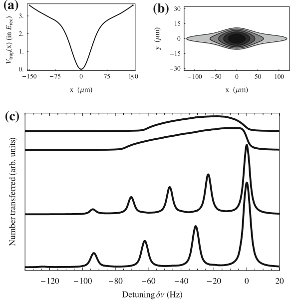
Fig. 4.5 a A slice of the anharmonic potential V_{\text{trap}}(\mathbf{r}) similar to the one found in experiments. b Contour lines of constant density in the x - y plane for n = 1, 2, \dots, 5 in the anharmonic trap at V_0 = 35E_{\text{rec}} . c Corresponding spectra (using the “spherical trap model” discussed in text) for V_0 = 5, 10, 25, 35E_{\text{rec}} with N = 1.4 \times 10^7 particles
