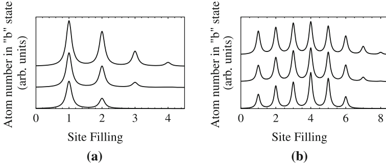
Fig. 6.3 Finite temperature RF spectra in the deep Mott limit for a harmonically trapped system. The temperatures are T = 0.01, 0.7, 1.5 in units of U_a from bottom to top. Vertical offsets are for clarity only. The chemical potential is \mu = 1.4, 5.7 (corresponding to n = 2, 6 zero-temperature site fillings at the trap center) in (a) and (b) respectively
