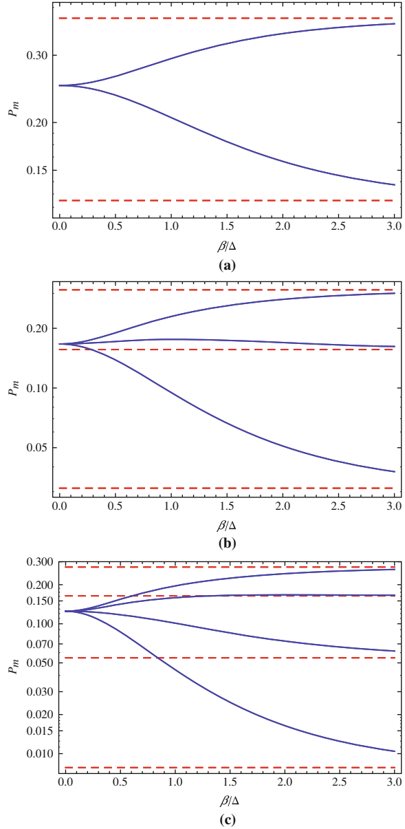
Fig. 11.1 Thermal expectation values \overline{\langle s|P_m|s \rangle} versus inverse temperature \beta\Delta . At high temperature, all states are equally likely, while at low temperature they tend to a binomial distribution, indicated by the dashed red lines. Top to bottom: N = 3, 5, 7 . It should be clear from the graphs which curves correspond to which m
