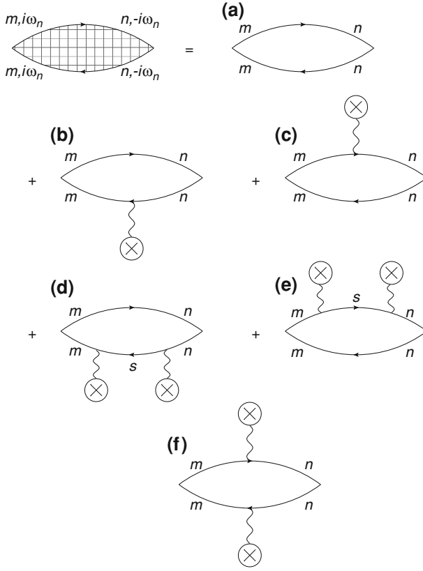
Fig. 11.3 Representative diagrams for the two-site slave boson perturbation theory at low order in “ t/U ”
