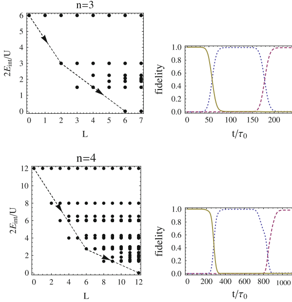
Fig. 9.3 (Color online) Transferring atoms using multiple pulses. Left : paths from initial to Laughlin states for n = 3, 4 . Right : Solid line is the fidelity with the initial state, dotted with the intermediate (L, E) = (2\hbar, 3(U/2)) state, and the dashed line with the Laughlin state. All pulses are Gaussians. Despite using multiple pulses, this technique is faster than using a higher order m = 2 pulse. The frequencies (\Omega_p) , shape ( m ), and pulse times ( \tau ) for the N = 3 sequence were \hbar(\omega - \Omega_p)/(U/2) = 3.00, 3.035 , m = 2, 4 , and \tau/\tau_0 = 16.95, 19.2 . For both, V_p = 0.05(U/2) . For N = 4 , using two pulses with m = 2 and V_p = 0.2(U/2) , we achieve > 98\% fidelity after a total two-pulse sequences with \hbar(\omega - \Omega_p)/(U/2) = 3.130, 1.0376 and \tau/\tau_0 = 82.5, 87.0
