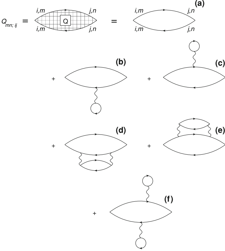
Fig. 11.2 Representative diagrams for the slave boson perturbation theory at low order in “ t/U ”
