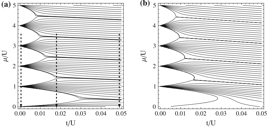
Fig. 4.2 a Gutzwiller Mean Field phase diagram with constant density contours. The vertical dashed lines show the spatial dependance of the chemical potential for a trapped gas in the LDA: from left-to-right these correspond to the deep Mott limit, the “corrugated superfluid” situation appropriate to Fig. 4.4b, and the dilute superfluid. b Phase diagram with contours of constant \langle n \rangle g_2 = \langle n(n-1) \rangle / \langle n \rangle . Contours are spaced by 0.1, with additional lines at m \pm 0.01 , for integer m , to emphasize the Mott regions
