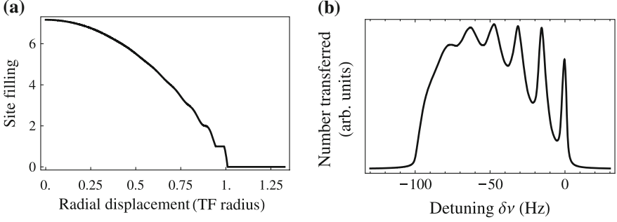
Fig. 4.4 a The density as a function of distance from the trap center for a harmonic trap in units of the Thomas–Fermi radius \ell_{\text{TF}} , defined as \ell_{\text{TF}} \equiv \sqrt{(\mu_0 - \epsilon_0)/(m\omega^2/2)} . The density profile corresponds to the LDA contour at t/U_a = 0.018 of Fig. 4.2a. The corrugation of the density is observable, but not dramatic; it would be particularly difficult to image in experiments looking at columnar integrated densities. b The hyperfine spectra arising from the density plotted in (a)
