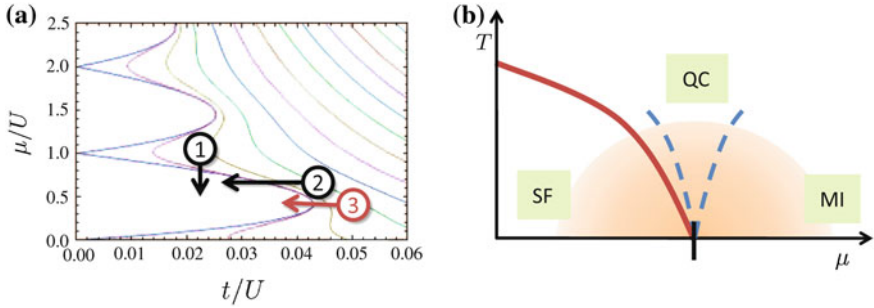
Fig. 13.1 Quantum critical crossovers in the Bose-Hubbard model. a Mott insulator to superfluid phase boundaries for (left to right) temperatures T/U = 0.00, 0.06, 0.12, \dots, 0.96 , calculated via finite temperature Gutzwiller theory (see Chap. 14) in d = 2 . The parameters t , \mu , and U are the tunneling rate, chemical potential, and on-site interaction energy of the Bose-Hubbard model. Paths (1,2) are governed by the dilute Bose gas universality class, and path (3) (passing through the tip) is governed by the O(2) universality class. See Chap. 14 for more details. b Slice through the quantum phase transition at fixed t/U . Slices with fixed \mu/U are similar. The abbreviations “SF”, “MI”, and “QC” denote the superfluid, Mott insulator-like normal fluid, and quantum critical regime, with the Mott insulator being strictly defined only at T = 0 . The shaded region indicates where the physics is governed by the quantum critical point. The dashed lines represent smooth crossovers between the qualitatively distinct “QC” and “low temperature” regions. Deep in the former, T is the only relevant energy scale
