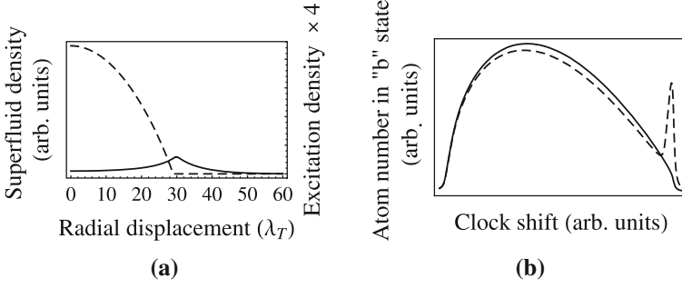
Fig. 6.1 a Condensate and excitation densities of a finite temperature superfluid at a temperature of 30 in units of the coupling constant U_x , the radial displacement is in units of the thermal de Broglie wavelength \lambda_T , and the trapping potential is \alpha r^2 with \alpha = 10^{-2} U_x / \lambda_T^2 . The excitation density is rescaled to make it more visible. b Corresponding RF spectra at temperatures T = 1, 30 for the solid and dashed curves respectively. b The peak at low densities comes from the normal fluid tail
