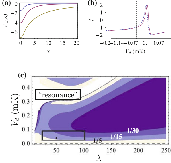
Fig. 16.1 a Rescaled mediated potential as a function of interparticle separation divided by \lambda , as given by Eq. 16.9, with \xi = 1, 4, 15 from top to bottom. b Scattering amplitudes f as a function of mediated potential depth factor V_d \equiv (2\delta^2)/(\pi^3\lambda_0^2MC_3^2) = V_0(\lambda/\lambda_0)^2 with \lambda_0 \equiv 50 \text{ \AA} , for the triplet (dashed) and singlet (solid) scattering channels. Vertical lines indicate V_d for the typical parameters given in the text (dashed line) and for V_d = 0 (solid). The divergences near V_d = 0 have been rounded off for display. c Contour plot of the factor by which V_{\text{med}} reduces the frequency shift as a function of \lambda and V_d . Typical values of parameters are shown by the black dot, while factor of two variations comprise the interior of the black rectangle. The contour plot is hidden in the white “resonance” region (far away from the relevant regime), where the scattering amplitude diverges
