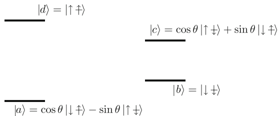
Fig. 17.1 Hyperfine level diagram for hydrogen atom in a B = 4.6 T magnetic field, where the mixing angle is \theta = 3 \times 10^{-3} . Vertical axis schematically denotes energy, while horizontal axis has no physical meaning. Arrows denote electron ( no-slash arrow ) and nuclear ( slashed arrow ) spin projections
