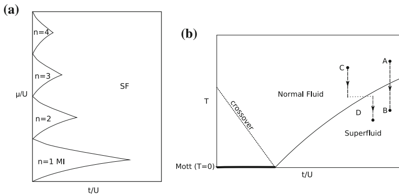
Fig. 18.3 A schematic review of the Bose-Hubbard model: The phase diagrams for the Hubbard or coupled Josephson junction model. Here t is the tunneling rate, \mu is the chemical potential, U is a measure of the interaction strength between particles on the same site, and T is the temperature. The “ n = x ” states are the x -particle per lattice site Mott insulating states. (a) Zero-temperature phase diagram, consisting of Mott insulating lobes with integer fillings and a superfluid phase; presumably the supersolid phase is far from the Mott lobes. (b) The finite temperature phase diagram, with a normal fluid and a superfluid phase. While A \rightarrow B would be a cooling path for a system directly described by the Hubbard model, our theory associate a more indirect path in t/U with the experimental cooling, as illustrated by the path C \rightarrow D
