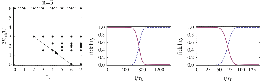
Fig. 9.2 (Color online) Using a rotating m -fold symmetric perturbation to drive n = 3 particle clusters from L = 2 to the \nu = 1/2 Laughlin state. Left : path on the energy level diagram. Center : second-order process coming from a deformation with m = 2 . Right : direct transition produced with m = 4 . Solid (dashed) lines are fidelities with the initial (Laughlin) state. In both cases the peak deformation is V_p = 0.05(U/2) . Both use a Gaussian pulse. The frequencies and pulse times \tau we used for m = 2, 4 were \omega - \Omega_p = (3.00/2)(U/2), 3.035(U/2) and \tau/\tau_0 = 218, 21 . Note how much more rapid the direct process is
