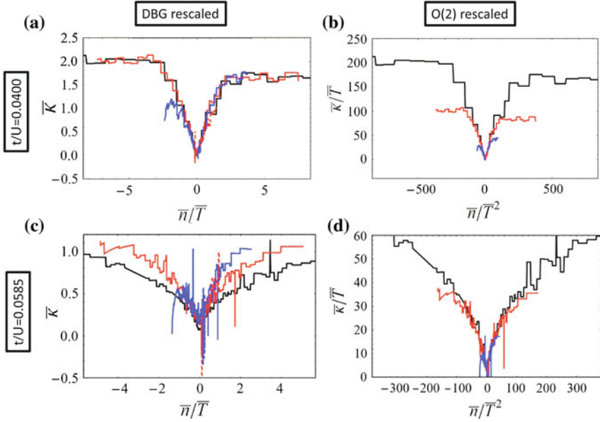
Fig. 13.3 Extracting universal behavior and dynamical critical exponents from density profiles of the trapped two-dimensional Bose-Hubbard model. Each panel shows an application of our analysis procedure to simulated density profiles (as described in text) for temperature T/t = 1/4, 1/2, 1, 2 , and 4 using the data in a density range |n - 1| < 0.15 . The symbols \bar{n} , \bar{k} , and \bar{T} are defined in Fig. 13.2. Lower temperature curves are identified by noting that they span a wider \bar{n} range. On the left (a and c), we plot \bar{k} versus \bar{n}\bar{T}^{-1} , while on the right (b and d) we plot \bar{k}\bar{T}^{-1} versus \bar{n}\bar{T}^{-2} ; these will show collapse if the dynamical critical exponent is respectively z = 2, 1 . Top (a and b) shows data with t/U = 0.0400 , which should be described by the dilute Bose gas universality class ( z = 2 ). Bottom (c and d) shows data with t/U = 0.0585 , which should be better described by the O(2) rotor model universality class ( z = 1 ): the tip of the n = 1 Mott lobe in the homogeneous system is at t/U = 0.0593 . As expected, we see collapse in a and d. The scatter in data points corresponds to stochastic noise in our Monte-Carlo simulations amplified by the differentiation. This noise is of comparable size to what would be seen in an experiment
