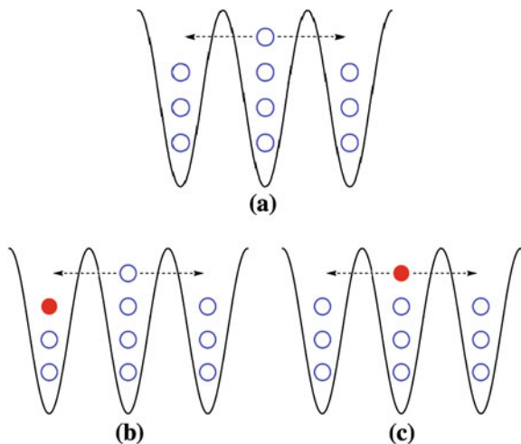
Fig. 5.1 (Color online) Illustration of two types of RF-active excitations of the lattice superfluid near the Mott transition. Open (blue) circles are atoms in the |a\rangle state, filled (red) circles are atoms in the |b\rangle state, and the arrows indicate a delocalized particle while other particles are localized. a Illustrates the initial superfluid state, consisting of a dilute gas of atoms moving in a Mott background. Final states in b and c , show the excitation of a core or delocalized atom
