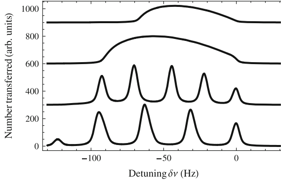
Fig. 4.1 Theoretical spectra showing the number of ^{87}\text{Rb} atoms transferred from hyperfine state |a\rangle = |F=1, m_F=-1\rangle to state |b\rangle = |F=2, m_F=1\rangle when excited by light detuned from resonance by the frequency \delta\nu . The N = 9 \times 10^4 atoms are confined by a harmonic potential with \bar{\omega} = (\omega_x \omega_y \omega_z)^{1/3} = 2\pi \times 100 Hz and a three-dimensional periodic potential with lattice depth V_0 = 5, 10, 25, 35E_{\text{rec}} (from top to bottom )
