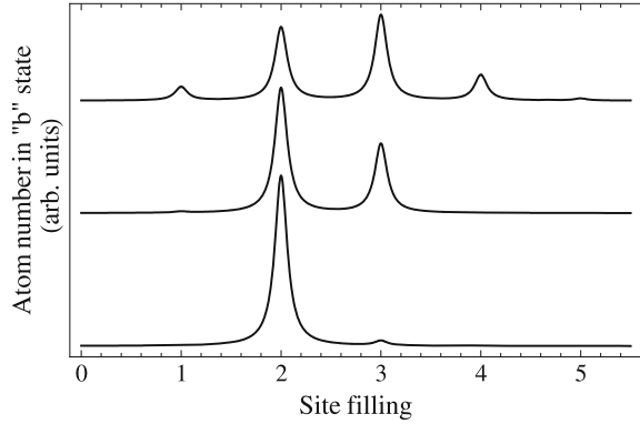
Fig. 6.2 Finite temperature RF spectrum in the deep Mott limit for a homogeneous system , at temperatures T = 0.05, 0.2, 0.8 in units of U_a , from bottom to top . The appearance of multiple peaks signals the occupation of states with different site fillings. The chemical potential is \mu = 1.8 (corresponding to a n = 2 site filling at zero temperature)
