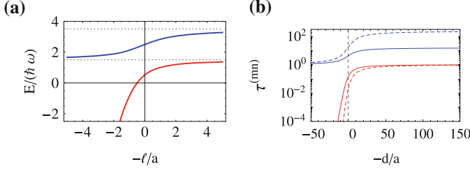
Fig. 10.2 ( Color online ) Left: On-site two-particle energy as a function of scattering length a rescaled by the on-site harmonic oscillator energy \hbar\omega = 2\sqrt{V_0 E_R} , for the two lowest energy branches. The corresponding characteristic length is \ell = \sqrt{\hbar/m\omega} . Right: Log plot of rescaled hopping matrix elements \tau^{(mn)} \equiv t^{(mn)}/(t\sqrt{(m+1)n}) . Solid and dashed curves are t^{(11)}/(\sqrt{2}t) and t^{(12)}/(2t) , respectively. We have chosen the lattice depth V_0 = 15E_R ; this affects only the horizontal scale. In the ordinary Bose-Hubbard model, t^{(mn)}/(\sqrt{(m+1)n}t) = 1 for all m, n , as confirmed by this figure's a = 0^- lowest (red) branch and a = 0^+ second (blue) branch limits. The resonance at -d/a = 0 separates the molecular side (left), from the atomic side (right). Note that t^{(10)}/t (not shown) is universally equal to unity regardless of interaction strength, since interatomic correlations are absent when there is a single particle per site
