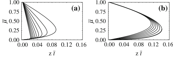
Fig. 10.4 Single lobe of the Mott insulator/superfluid boundary. Complete characterization of the mean-field lobe shape in the z\bar{t} - \bar{\mu} plane for all possible t^\pm 's (see Eq. 10.7 for definitions). a Fix t^- = 0.5 , vary t^+ from 1 (outer curve) to 21 (inner curve) in steps of 2. b Fix t^+ = 1.5 , vary t^- from 0 (outer curve) to 1 (inner curve) in steps of 0.15
