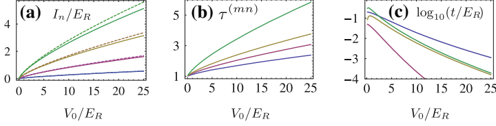
Fig. 10.1 (Color online) a On-site energy with non-interacting energies subtracted off, I_n = E_n - (3\hbar\omega/2 - \mu)n , and energies scaled by E_R = \hbar^2\pi^2/(2md^2) , using typical ^{87}\text{Rb} parameters: lattice spacing d = 532 nm, scattering length a = 5.32 nm. Dashed : neglecting on-site correlations, solid : including correlations. Bottom to top curve : n = 2, 3, 4, 5 . b Representative hopping matrix elements with on-site correlations, relative to those neglecting on-site correlations, \tau^{(mn)} \equiv t^{(mn)}/(t\sqrt{(m+1)n}) , as a function of lattice depth V_0 on a scale. Bottom to top line : t^{(03)}, t^{(31)}, t^{(05)}, t^{(35)} . c For comparison, t^{(01)}/E_R calculated from the exact Wannier states ( upper curve ) along with our Gaussian approximation to it with and without non-orthogonality corrections (second and third highest, respectively); also shown is the next-nearest neighbor hopping matrix element ( bottom curve ). The effective Hamiltonian parameters are calculated perturbatively in a/d for a Gaussian ansatz
