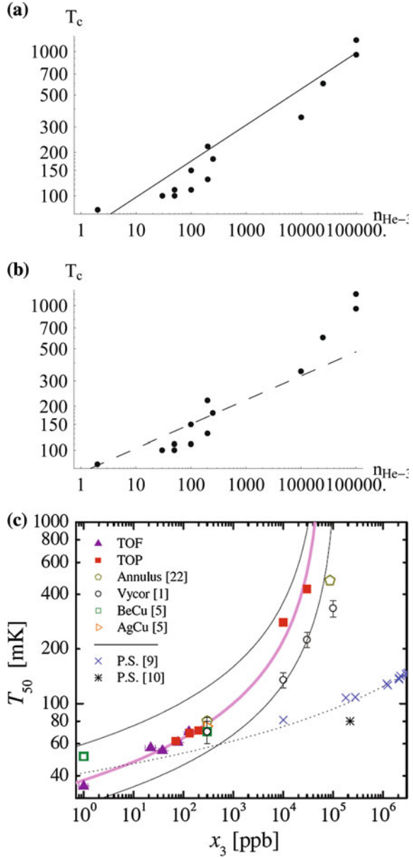
Fig. 18.2 The critical temperature (in mK) versus ^3\text{He} concentration (in parts per billion) on a log-log plot. Solid line. x = 1/4 static links prediction (see text); Dashed line x = 1/6 static links prediction. (Points are copied by hand out of Moses's proposal.) The color figure is from Kim et al. [4] and compares various experimental T_c 's with (18.8), our prediction for T_c ( solid pink line )
