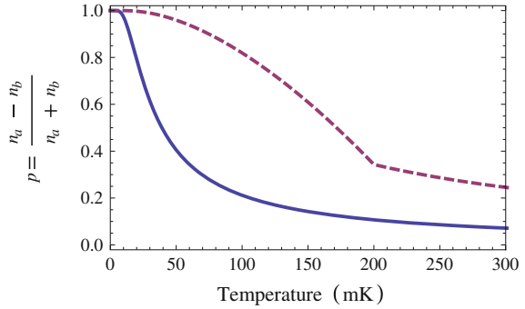
Fig. 17.2 The polarization versus temperature for the Boltzmann case ( solid line ) and the Bose-condensed case ( dashed line ), from (17.8)
