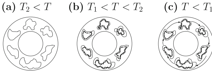
Fig. 18.1 Our model's basic idea. a The solid at T > T_2 before any superflow develops. There are two distinct types of regions: those that support superflow at low temperatures (SF) and those that will not (NSF). It is likely that T_2 is larger than the solidification temperature so that the domains are always locally superfluid in the solid. b The state of the system after cooling through one phase transition to a temperature T_1 < T < T_2 : within each of the SF regions, a superflow develops. However, no global phase coherence is present. c The state of the system after cooling to T < T_1 : global phase coherence has developed, and superflow occurs throughout the system
