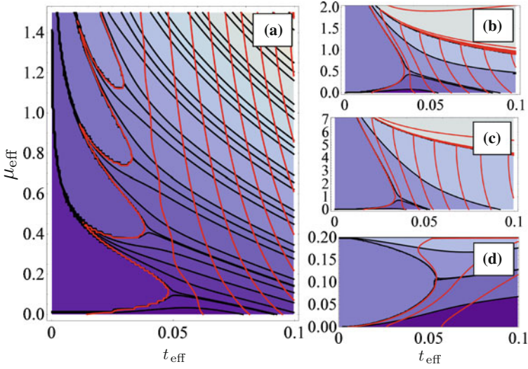
Fig. 10.3 (Color online) Representative Gutzwiller mean-field theory phase diagrams, showing constant density (black, roughly horizontal) and constant \xi \equiv \zeta_1 + \zeta_2 + \zeta_3 (red, roughly vertical) contours: \xi , similar to the condensate density, is a combination of the mean fields \zeta_m , defined after Eq. 10.2. Density contours are n = \{0.01, 0.2, 0.5, 0.8, 0.99, 1.01, 1.2, \dots\} and order parameter contours are \xi = \{0.2, 0.4, \dots\} , except (d) where we take contours \xi = \{0.02, 0.04, \dots\} . The phase diagrams are functions of \mu_{\text{eff}} \equiv \mu/E_R and t_{\text{eff}} \equiv \exp(-\sqrt{V_0/E_R}) , where the lattice depth V_0 is the natural experimental control parameter. We plot versus t_{\text{eff}} , instead of V_0 , as this is closer to the Hamiltonian matrix elements and more analogous to traditional visualizations of the Bose-Hubbard phase diagram. a Ordinary Bose-Hubbard model for a = 0.01d , b lattice bosons restricted to fillings n = 0, 1, 2 with a = 0.01d , on the next to lowest energy branch on the a > 0 side of resonance, c lattice boson model with a = d , and d FQH puddle array model taking \omega - \Omega = 0.1E_R (see text for details). Parts (b, c) use the Hamiltonian parameters from the exact two-particle harmonic well solution
