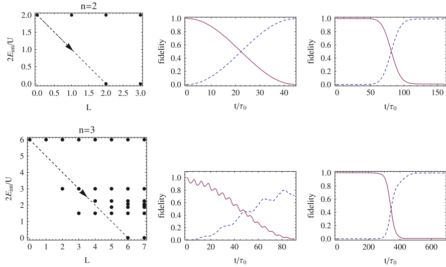
Fig. 9.1 (Color online) Transferring small clusters from non-rotating ground state to \nu = 1/2 Laughlin state using rotating quadrupolar ( m = 2 ) deformations. Left : Interaction energy (in units of U/2 ) of quantum states of harmonically trapped two dimensional clusters as a function of total angular momentum projection L in units of \hbar . Excitation paths are shown by arrows. Central : squared overlap (fidelity) of |\psi(t)\rangle with the initial ( solid ) and final ( dashed ) states as a function of the duration of a square pulse. Right : Fidelities as a function of time for an optimized Gaussian pulse of the form e^{-(t-t_0)^2/\tau^2} . Time is measured in units of \tau_0 = \hbar/U \sim 10^{-4} s. For n = 2 , the peak perturbation amplitude is V_p = 0.05(U/2) , \omega - \Omega_p = 2.0(U/2) , and a Gaussian pulse time of \tau = 24\tau_0 . For n = 3 , \tau = 102\tau_0 and \omega - \Omega_p = 2.046(U/2) and 2.055(U/2) for the Gaussian and square cases, respectively. For n = 3 , nonlinear effects (coupling with near-resonant levels) shifted the optimal frequency away from the linear response expectation, \omega - \Omega_p = 2(U/2)
