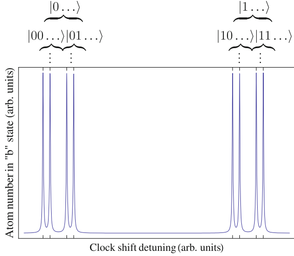
Fig. 6.4 Deep Mott RF spectra with dipolar interactions for the state given in the text. The correspondence between peak and spatial variation is indicated, where a string “ n_1 n_2 n_3 ” indicates n_1 particles in the first neighbor site, n_2 in the second neighbor, and n_3 in the third neighbor. The labels instruct how to read-off the probabilities for each state
