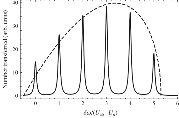
Fig. 4.3 Analytically calculated spectra for the harmonically trapped system in the deep Mott limit ( solid line ), plotted as a function of \delta\omega/(U_{ab} - U_a) . Superimposed is the spectrum of the superfluid ( dashed line ) with the same parameters, but horizontally shifted to the left by -(\delta\omega/2)(U_{ab} - U_a) . The central density is n_s(0) = [\mu_0 - \epsilon(0)]/U_a = 5.8 . This illustrates that the envelope of the spectral line in the Mott insulating state has the same shape as the superfluid spectrum, shifted horizontally
