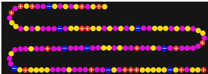
Fig. 6.4. The 130 amino acid chain of human lysozyme. Hydrophobic and polar amino acids are respectively shown in yellow and pink, whereas the sign of the charged ones is indicated.
