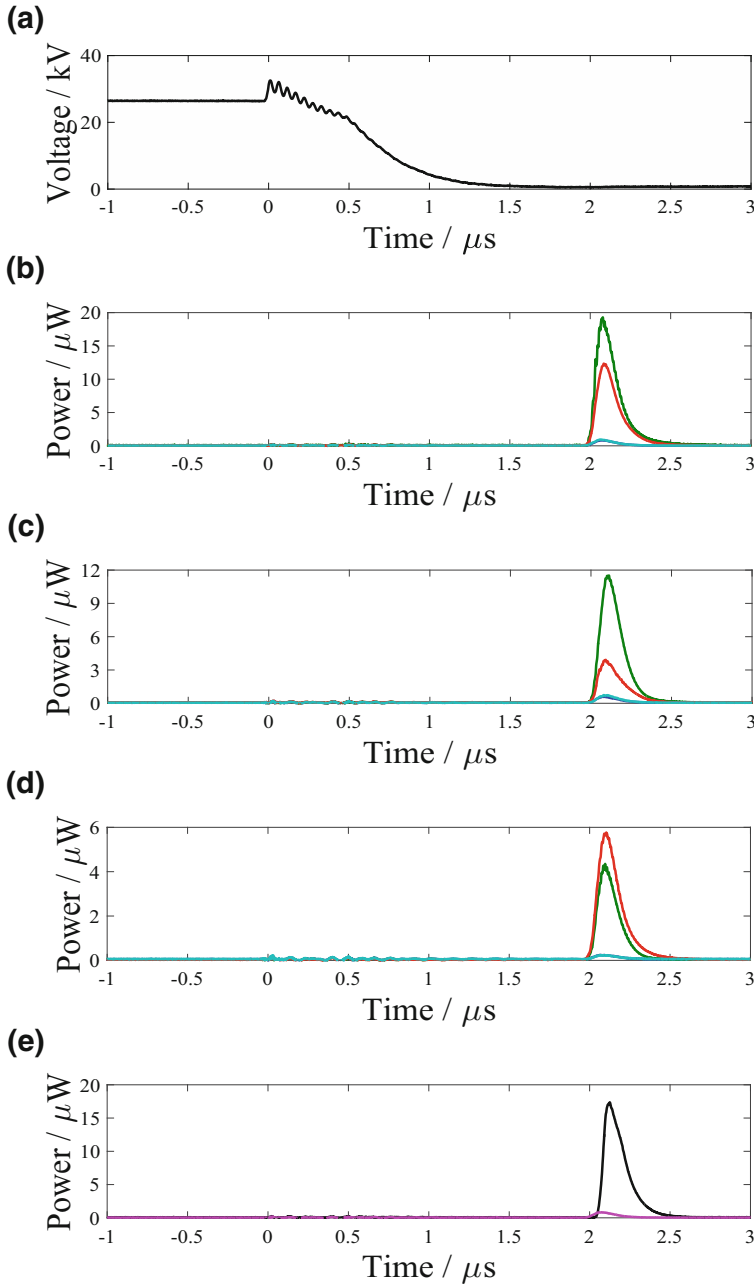
Fig. 7.8 Oscilloscope traces averaged over 128 pulses of 5:1 helium-xenon discharges at 12 mbar inside 140 cm of fibre B showing a the discharge voltage, b–d the unpolarised, S-polarised and P-polarised output powers respectively for the SP (blue line), FDP (green line), C (red line) and RDP (cyan line) cavity arrangements and e the SP powers from the anode end (black line) and cathode end (magenta line) of the fibre
