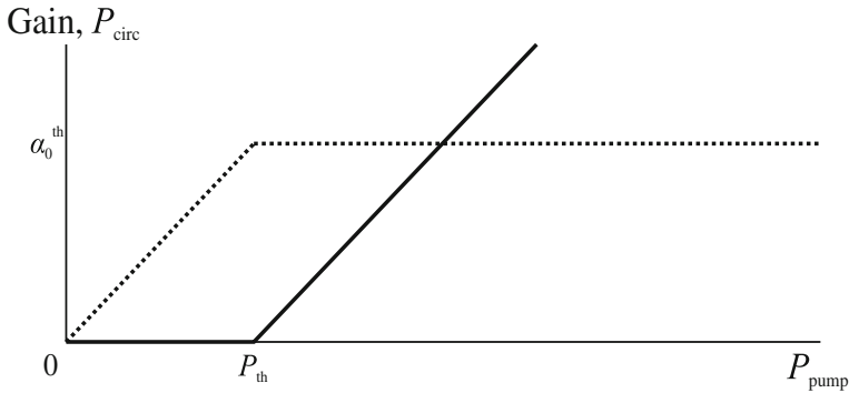
Fig. 2.6 Cavity gain (dotted) and circulating power (solid) as a function of pump power
