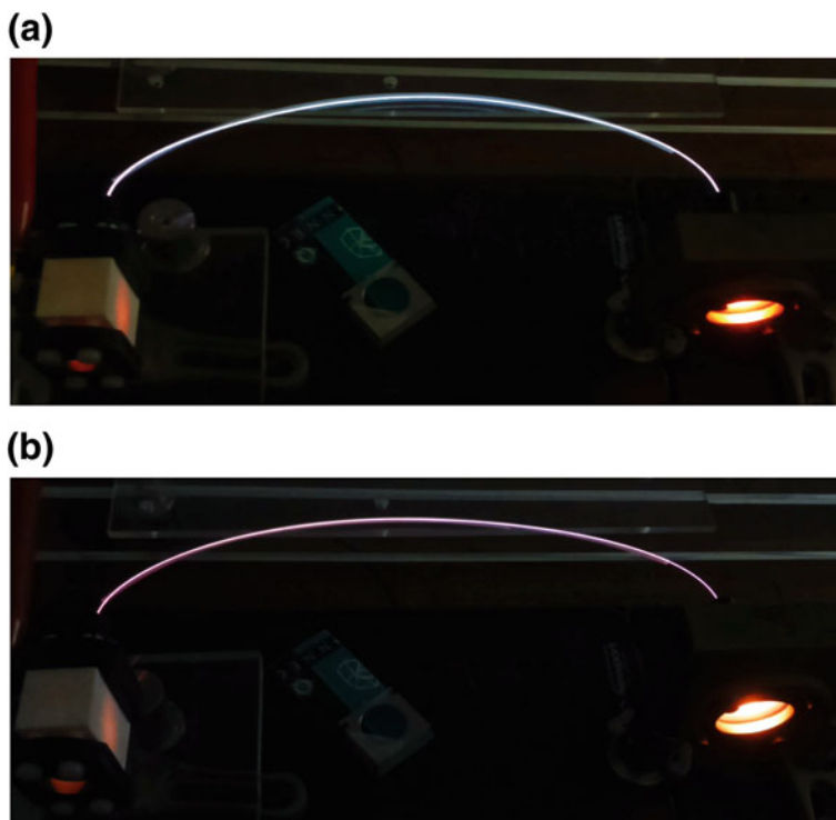
Fig. 8.2 Photographs of a 55 cm He-Ne discharge (a) with trace amounts of Xe and (b) after a number of flushes with Ne to remove any remaining Xe
