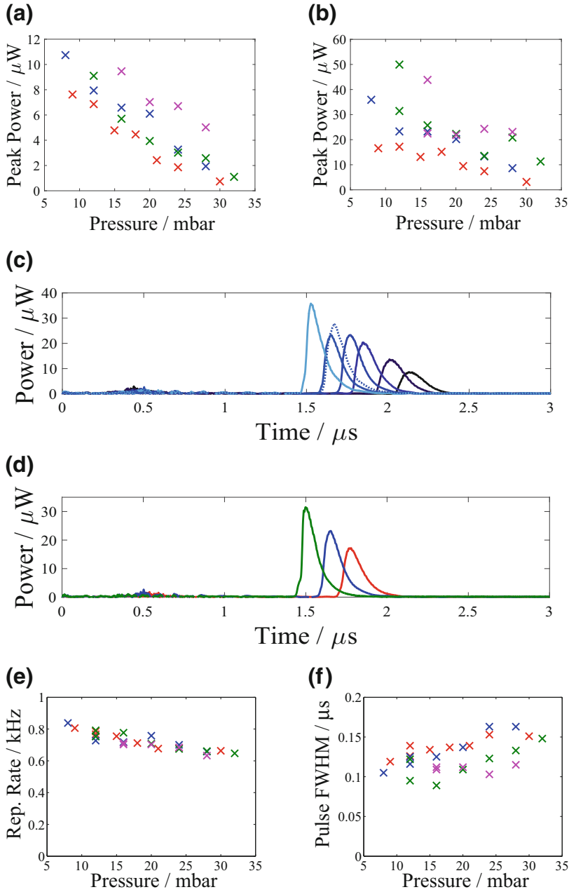
Fig. 7.13 Pressure optimisation of the He-Xe laser in 100 cm of fibre B at gas ratios of 5:1 (red), 7:1 (blue), 10:1 (green) and 20:1 (magenta). a single-pass peak power b cavity peak power c cavity output power traces for a 7:1 mixture at pressures of 8, 12, 16, 20, 24 and 28 mbar (light to dark, note the dotted 12 mbar measurement was a control taken last) (c) cavity output power traces at 12 mbar for different mixtures e pulse repetition rate f light pulse duration (FWHM)
