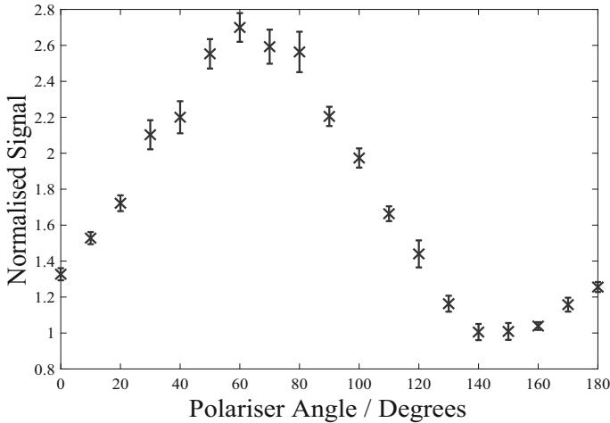
Fig. 6.19 Double-pass signal from the anode end of a 5:1 helium-xenon discharge at a pressure of 12 mbar inside 1.5 m of fibre B for various angles of an output polariser. The signal has been normalised to the single-pass signal. The \text{CaF}_2 beamsplitter placed between the cathode end and mirror creates a polarisation dependence which is rotated by the geometry of the fibre
