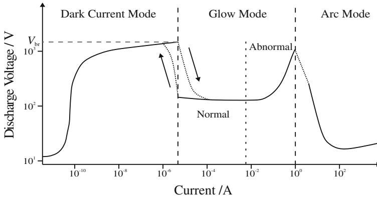
Fig. 3.2 A voltage-current plot for a typical gas discharge, showing the three main modes of operation. The fast transitions between the modes are highlighted by dotted lines. Axis scales are representative of a general case, as the real electrical parameters are dependent on many factors including the vessel dimensions and gases present
