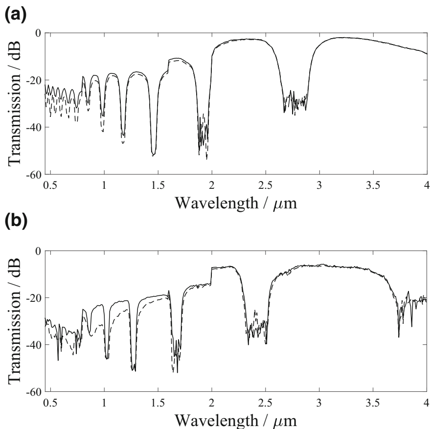
Fig. 6.2 Transmissions from a white light source through a 65 cm of fibre A and b 95 cm of fibre B for straight (solid) and bent (dashed) pieces of fibre. Measurements were taken using a Bentham DTMc300 Monochromator in combination with Si, InGaAs, PbSe and InSb detectors at a resolution of 10 nm. To remove the spectral variations in the detectors and halogen white light source the measurements were normalised to a separate spectra of the source. However there are still discontinuities at 800, 1600 and 2000 nm where the detectors change due to the differing active areas of the detectors
