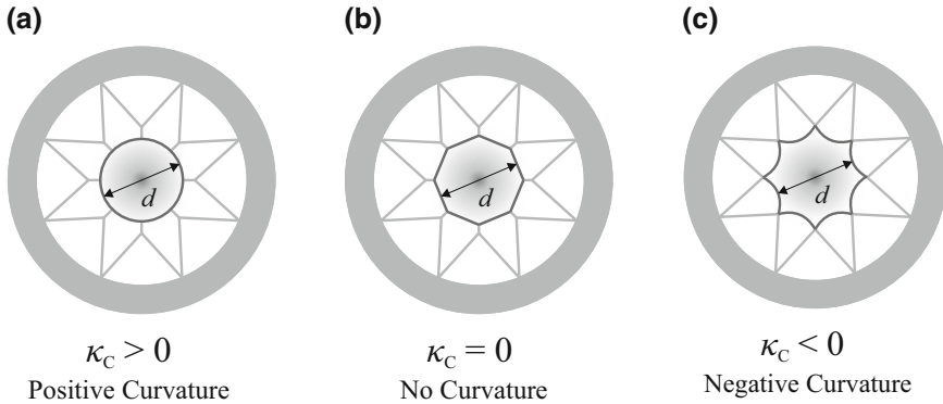
Fig. 5.7 Comparison of three anti-resonant guiding hollow core fibre structures with equal core diameters, but with a \kappa_C > 0 , b \kappa_C = 0 and c \kappa_C < 0 , where the inner wall curvature \kappa_C is defined as the derivative of the unit tangent vector normalised to the arc length. The guided mode is shown in the centre, and as \kappa_C decreases the mode overlap with the inner wall also decreases
