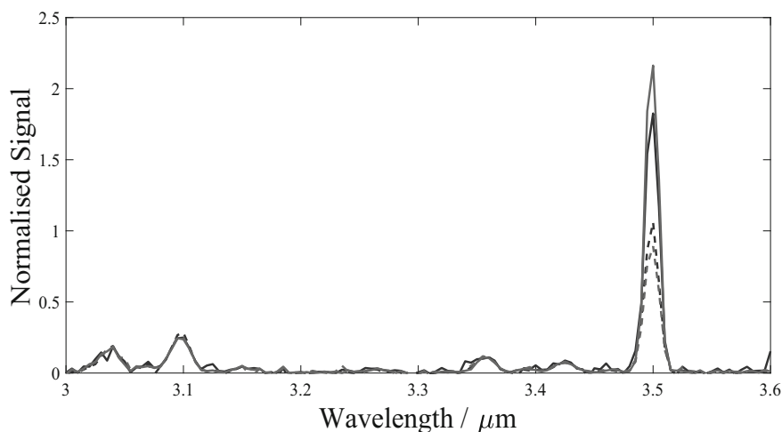
Fig. 6.16 Spectra for single-pass (dashed) and double-pass (solid) discharges in 90 cm of fibre A with a 5 : 1 ratio of helium-xenon at a pressure of 12 mbar, a discharge current of 0.25 mA, a 42 M \Omega ballast resistance and a 20 nm resolution
