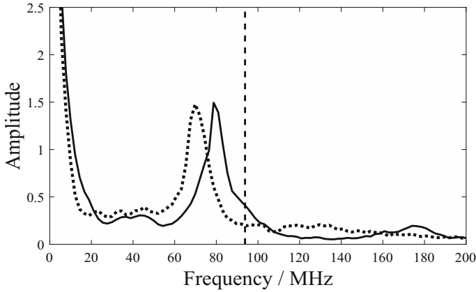
Fig. 7.11 Average of the Fourier spectra from 25 light pulses for a cavity with a focused (solid line) and a defocused (dotted line) anode mirror. The focused spectra amplitude has been reduced by a factor of 5 for an easier visual comparison. The dashed line indicates the mode separation frequency for a 160 cm long cold cavity
