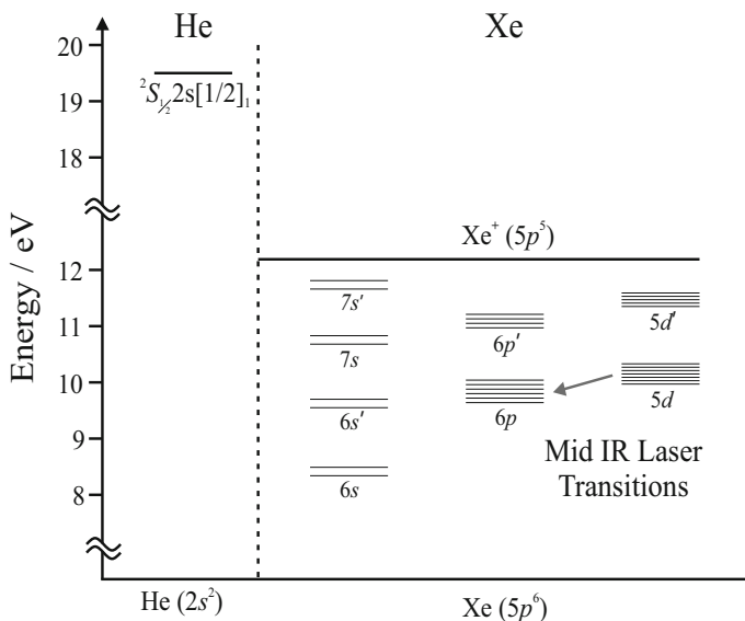
Fig. 4.5 Partial energy level diagram for helium-xenon. As the ^2S_{1/2} 2s[\frac{1}{2}]_1 helium state lies \approx 9 eV higher than the 5d xenon states, the collisional cross section for an atom-atom excitation transfer is very low. The ^2S_{1/2} 2s[\frac{1}{2}]_1 helium state is however higher than the xenon first ionisation energy of 12.1 eV, meaning collisions between the two atoms can result in a Penning ionisation collision
