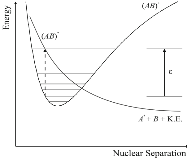
Fig. 4.3 Hypothetical potential energy curves involved in the dissociative-recombination process. (Recreated from [7])
