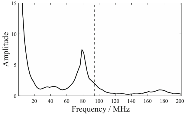
Fig. 7.10 Average of the Fourier spectra from 25 light pulses. The dashed line indicates the mode separation frequency for a 160 cm long cold cavity
