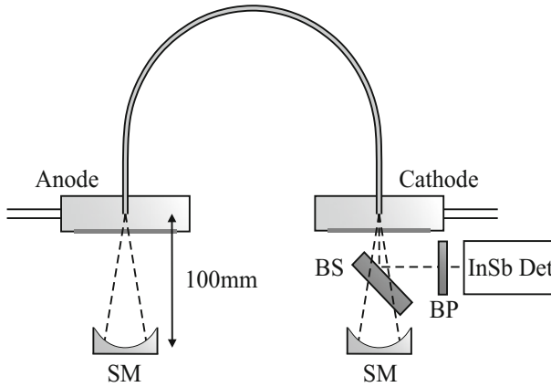
Fig. 6.9 Schematic diagram of the optical set-up; SM - silver coated spherical mirror, BS - \text{CaF}_2 beamsplitter, BP - 3.5 \mu\text{m} bandpass filter
