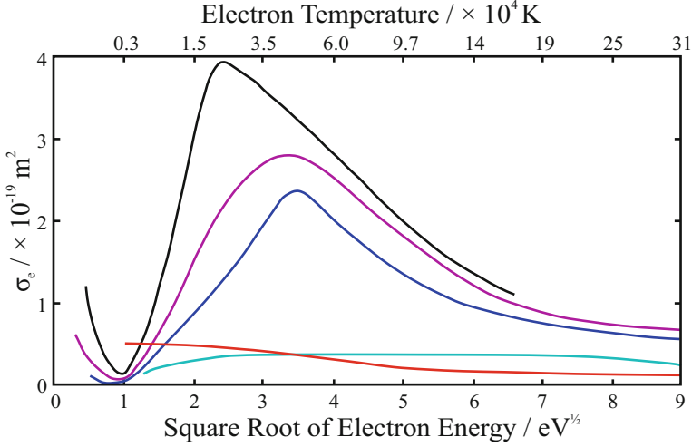
Fig. 4.1 Cross-sections for helium (red), neon (cyan), argon (blue), krypton (magenta) and xenon (black) (Recreated from [2])
