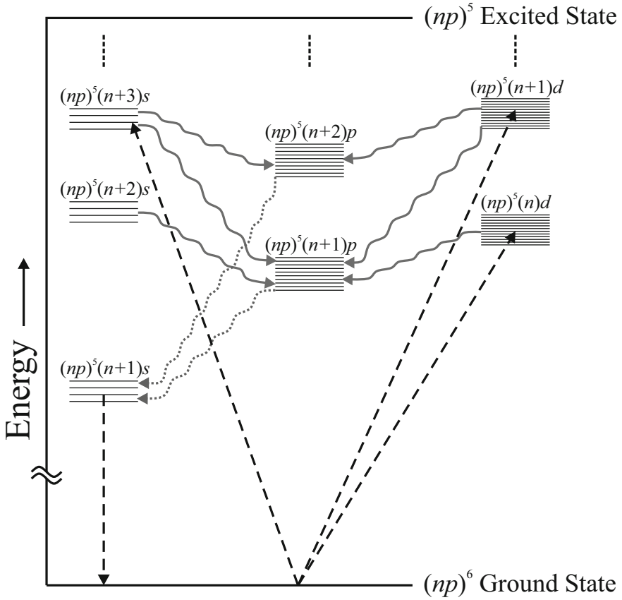
Fig. 4.2 General electronic configuration of neon, argon, krypton and xenon. The dashed lines represent collisional transitions, the dotted wavy lines are fast radiative transitions and the solid wavy lines are transitions available to lase. Note that for neon there are no (2p)^5 2d states. (Recreated from [3])
