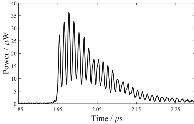
Fig. 7.9 Oscilloscope trace of a single output pulse from a 160 cm cavity
