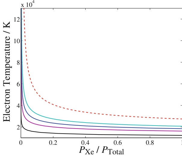
Fig. 3.7 Electron temperature T_e as a function of the partial pressure of Xe in a mixture of He-Xe for pD values of 0.9 Torr-mm (1.2 mbar-mm) (dotted red), 2 Torr-mm (2.7 mbar-mm) (cyan), 3 Torr-mm (4.0 mbar-mm) (blue), 5 Torr-mm (6.7 mbar-mm) (magenta) and 20 Torr-mm (26 mbar-mm) (black) based on Eq. 3.13 [1]
