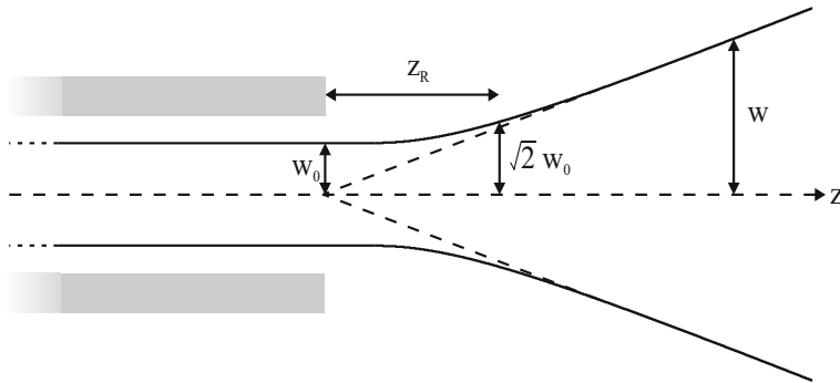
Fig. 6.10 Divergence of a Gaussian beam exiting a hollow core fibre
