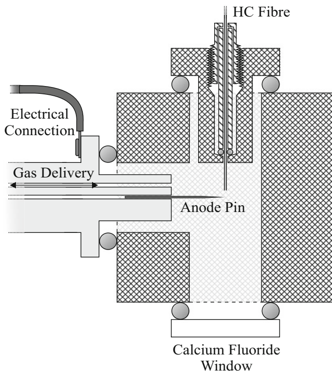
Fig. 6.7 Schematic diagram of the modified anode gas cell. The main body of the cell (hashed) is made of Macor ceramic, the gas delivery tube (shaded light grey) is brass, the rod and screw of the fibre holder (diagonal lined) are Delrin plastic and the anode pin is tungsten. The window, gas tube and fibre holder are all secured in place by Delrin plastic fittings screwed into the cell (not pictured)
