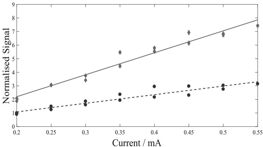
Fig. 6.15 Signal at various currents for single-pass (dashed) and double-pass (solid) discharges in 90 cm of fibre A with a 5:1 ratio of helium-xenon at a pressure of 12 mbar and a 42 M \Omega ballast resistance. The measured signals have been normalised to the initial 0.2 mA single-pass reading
