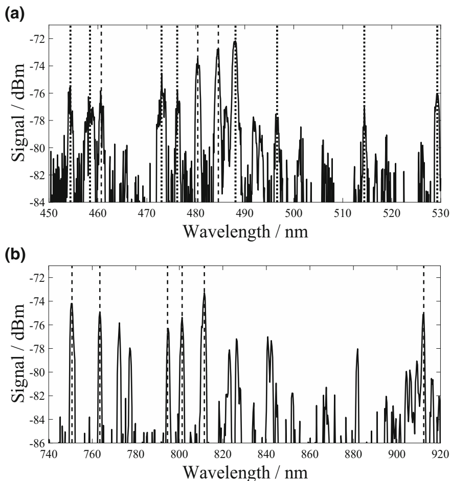
Fig. 8.11 Spectra of the light collected from the end of a 5 mbar argon discharge with a resolution of 1 nm. Emission lines that are known to lase are marked with dotted lines, notable non-lasing lines with dashed lines. Additional emission lines of neutral argon are present but unmarked as they are of little interest
