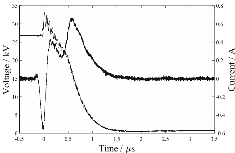
Fig. 7.3 Voltage and current across 5 : 1 helium-xenon discharges at 12 mbar inside fibre B averaged over 128 pulses. The dotted and dashed curves (left axis) represent the voltage before and after numerical low-pass filtering. The solid curve (right axis) represents an estimate of the current calculated from the dashed curve by Eq. 7.1
