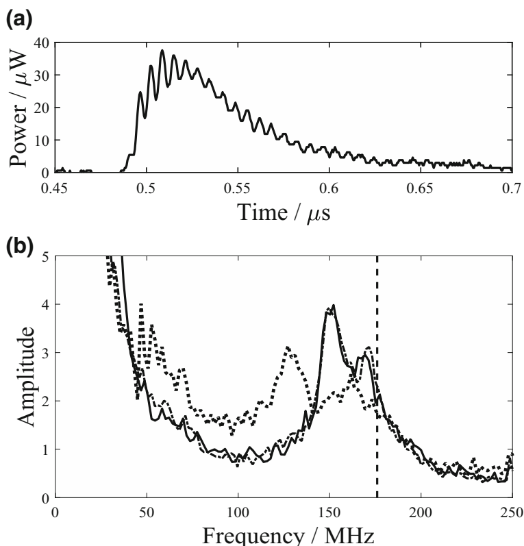
Fig. 8.6 a Oscilloscope trace of a single pulse from the cavity. b Average of the Fourier spectra from 20 light pulses for a cavity with a focused (solid line), defocused (dotted line) and refocused (dot-dashed line) anode mirror. The dashed line indicates the mode separation frequency for an 85 cm long cold cavity
