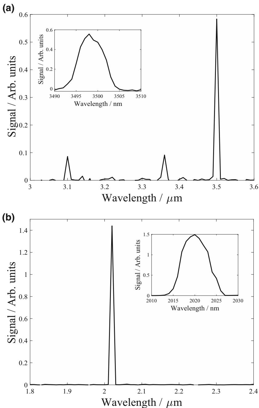
Fig. 8.7 Spectra of the cavity output signal from 200:1 neon-xenon discharges at 10 mbar inside 65 cm of fibre A (a) in the mid-IR range using an InSb detector and (b) using a PbSe detector with a resolutions of 10 nm. Insets: the (a) 3.51 \mu\text{m} and (b) 2.02 \mu\text{m} lines zoomed in with a higher number of data points. The mid-IR peak is shifted from 3.51 \mu\text{m} due to a slight miscalibration of the spectrometer
