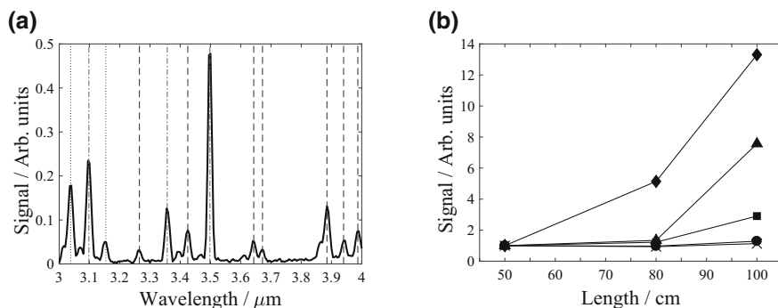
Fig. 6.6 a Spectra of a helium-xenon gas discharge inside 50 cm of fibre A at a 5 : 1 ratio of He to Xe at a pressure of 12 mbar, taken with a 5 nm resolution. The dotted, dashed and dot-dashed lines identify known xenon lines that do not lase, have demonstrated lasing and have shown evidence of gain in this system respectively. b Line analysis of the 3.04 (crosses), 3.11 (squares), 3.36 (triangles), 3.51 (diamonds) and 3.89 \mu\text{m} (circles) lines. Data taken from [1]
