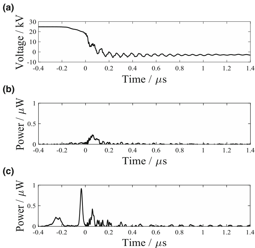
Fig. 8.10 Oscilloscope traces averaged over 128 pulses of argon discharges inside 50 cm of fibre A showing (a) the discharge voltage and the output powers from an amplified InGaAs detector sensitive to 2 \mu\text{m} at (b) 10 mbar and (c) 5 mbar. No spectral selection was used due to the very low powers detected
