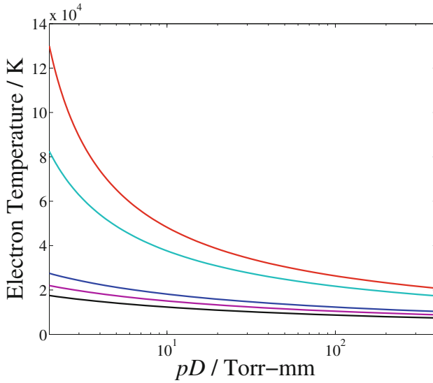
Fig. 3.6 Electron temperature T_e as a function of pD for helium (red), neon (cyan), argon (blue), krypton (magenta) and xenon (black) [1]
