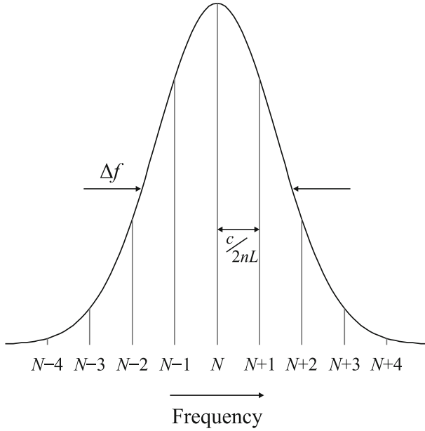
Fig. 2.5 An illustration of the gain bandwidth of an emission line (thick line) and the longitudinal modes contained within (thin lines)
