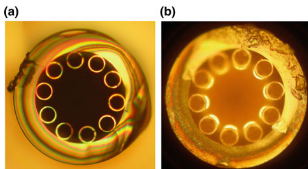
Fig. 6.14 Micrographs of the a cathode and b anode ends of a fibre after a number of discharges
