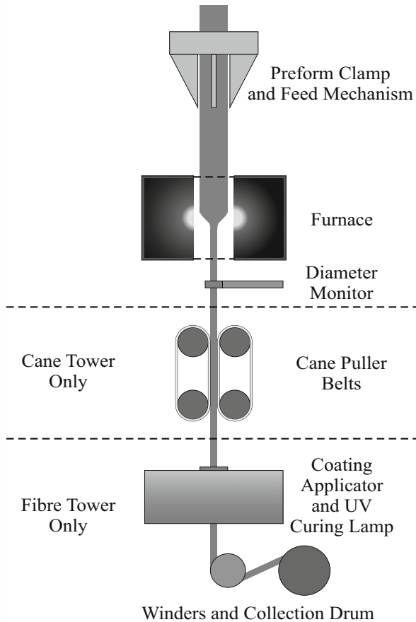
Fig. 5.8 Schematic diagram of a fibre drawing tower. The top section of a clamp, feed mechanism, furnace and diameter monitor is universal in all applications, however the pulling mechanism varies depending on the desired diameter after the draw. For larger scale draws (to \sim 1 mm) such as when drawing rods, capillaries or canes (see Sect. 5.4.2), the middle section which utilises a belt system is used. For drawing fibre the lower section is used to coat the fibres and wind them onto a drum
