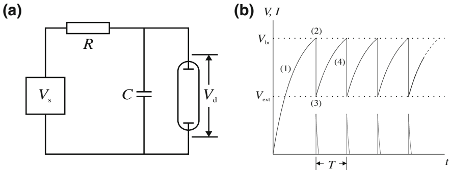
Fig. 3.9 a Circuit diagram of a Pearson-Anson Oscillator. b Voltage oscillations across the capacitor (top) and the subsequent current pulses through the discharge (bottom)
