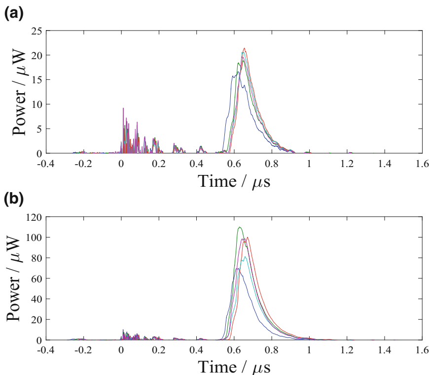
Fig. 8.3 Oscilloscope traces of the output power from He-Ne-Xe discharges inside 80 cm of fibre A showing the (a) single-pass and (b) cavity arrangements with 0.1 mbar of Xe and 12 mbar of He-Ne at ratios of 4:2 (blue), 3:3 (green), 2:4 (red), 1:5 (cyan) and 0:6 (magenta). All traces are taken with an averaging of 128
