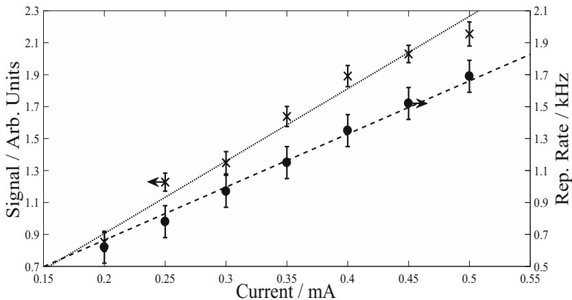
Fig. 7.2 Variation of average signal (crosses, left axis) and voltage pulse frequency (circles, right axis) with the measured current drawn from the power supply for 5:1 helium-xenon discharges at a pressure of 12 mbar inside 70 cm of fibre B. Trendlines with gradients of 4.5 \pm 0.2 \text{ AU mA}^{-1} for the signal (dotted) and 3.3 \pm 0.1 \text{ kHz mA}^{-1} for the repetition rate (dashed) have been fitted so that they pass through the origin
