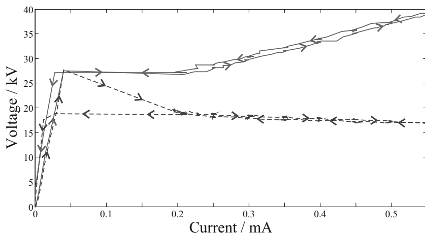
Fig. 6.13 Current-voltage plot for the supply (solid) and discharge (dashed) voltages of a 5 : 1 helium-xenon gas discharge at a pressure of 12 mbar inside 90 cm of fibre A with a ballast resistance of 42 M \Omega . One data point was recorded every second
