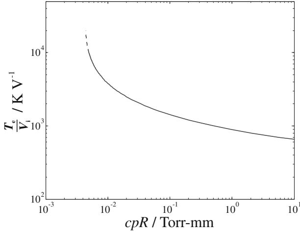
Fig. 3.5 Normalised electron temperature \frac{T_e}{V_i} as a function of c^* p R . Typical c^* values for the noble gases are; helium - 4 \times 10^{-3} , neon - 6 \times 10^{-3} , argon - 4 \times 10^{-2} (values taken from [2])
