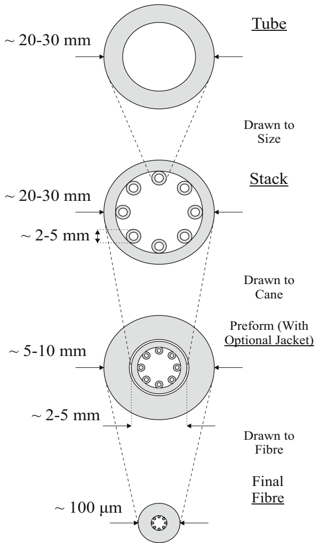
Fig. 5.9 Schematic representation of the stack and draw process
