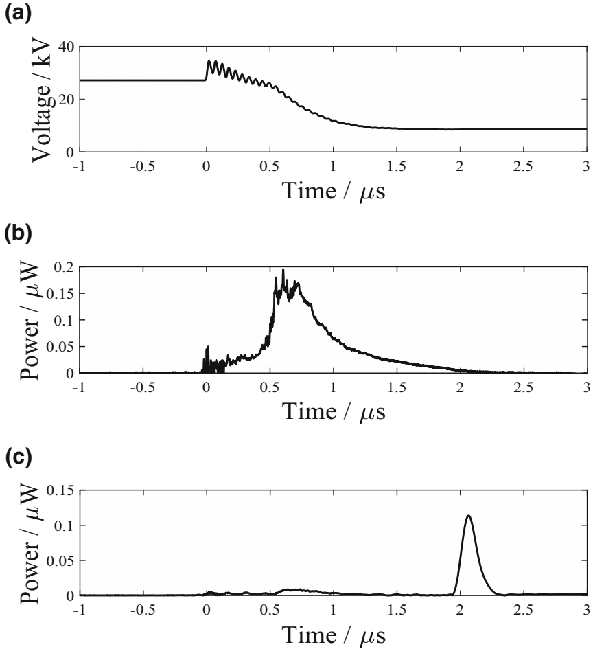
Fig. 7.6 Oscilloscope traces averaged over 128 pulses of 5:1 helium-xenon discharges at 12 mbar inside 70 cm of fibre B showing a the discharge voltage, and the single-pass output power as was measured by b an InGaAs detector after amplification and c the signal from a fast mid-IR detector
