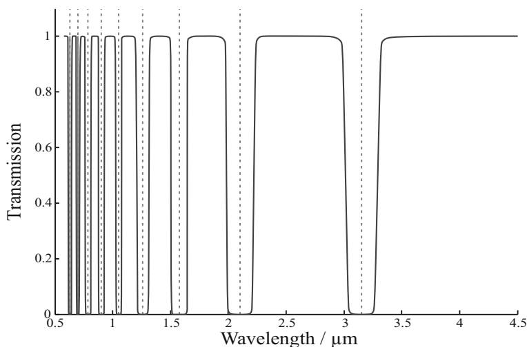
Fig. 5.6 Resonant wavelengths (dashed lines) calculated from Eq. 5.5 of the ARROW model for a hollow waveguide with 3 \mu\text{m} thick silica walls, and an schematic example of the ideal resulting waveguide transmission (solid line)
