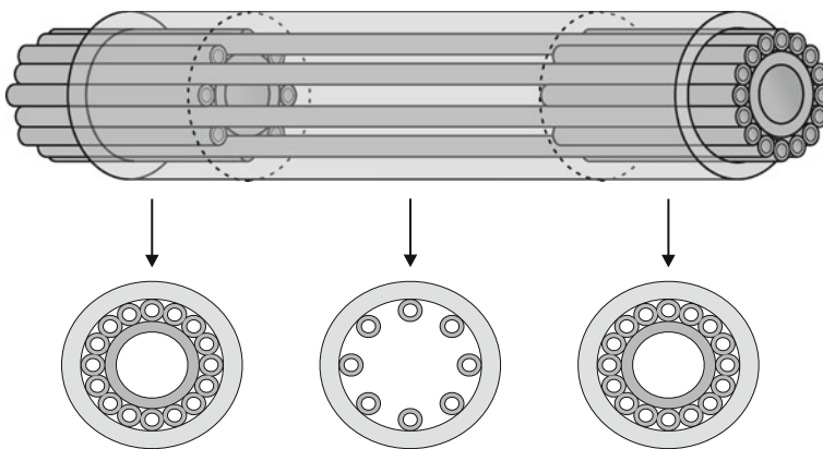
Fig. 5.10 Schematic diagram of the stack for a typical AR guiding fibre
