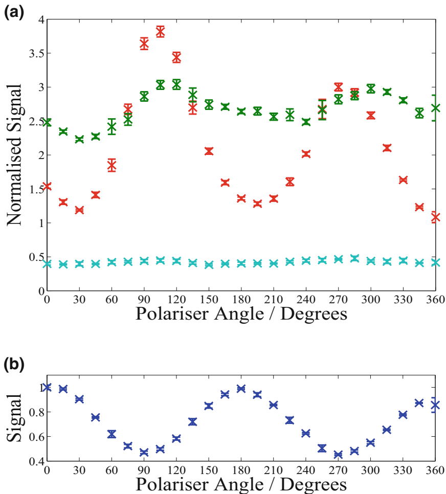
Fig. 6.20 Cathode output signals through a polariser from a 5:1 helium-xenon discharge at a pressure of 12 mbar inside 1.5 m of fibre B. a shows the forward double-pass (green), cavity (red) and reverse double-pass (cyan) cavity configuration output signals which have been normalised to the single-pass output signal shown in (b)
