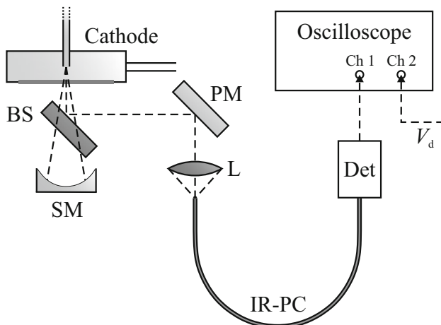
Fig. 7.5 Schematic diagram of revised cathode optical set up for the collection of light pulses. The rest of the system is left as in Fig. 6.9. PM - planar silver mirror, L - 50 mm focal length CaF 2 lens, IR-PC - InF 3 infrared fibre patch cord
