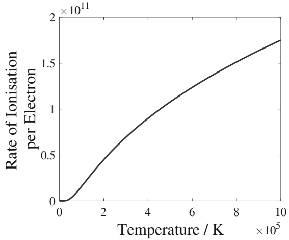
Fig. 3.4 Rate of ionisation per electron in a xenon gas at a pressure of 9 torr as a function of electron temperature
