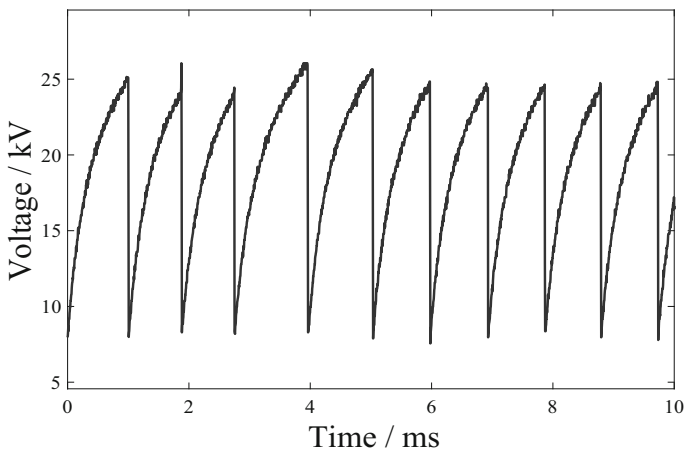
Fig. 7.1 Time trace of the voltage across a discharge
