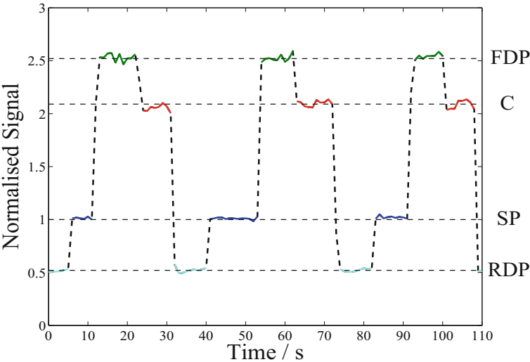
Fig. 6.18 Monitored output signal (black dotted line) from a 5:1 helium-xenon discharge at a pressure of 12 mbar inside 1.5 m of fibre B as the cavity mirrors were sequentially blocked and revealed. The signal has been normalised to the average SP reading. The signal levels in the different cavity configurations have been highlighted for clarity (SP - blue, FDP- green, C - red, RDP - cyan)
