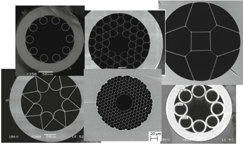
Fig. 5.3 Micrographs of a number of hollow core fibre designs. Clockwise from top left: a ten resonator free boundary fibre* [5], a kagomé cladding structure fibre* [6], a square core anti-resonant fibre [7], an early tube lattice negative curvature fibre [8], a hollow photonic bandgap fibre [9], a negative curvature anti-resonant guiding fibre* [10]. Those marked with an asterisk were fabricated at the University of Bath
