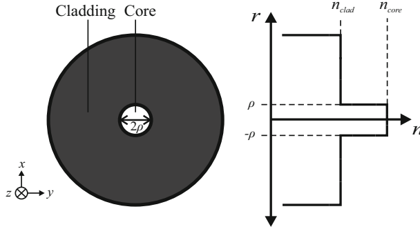
Fig. 5.1 Cross-section of a step index fibre with core radius \rho
