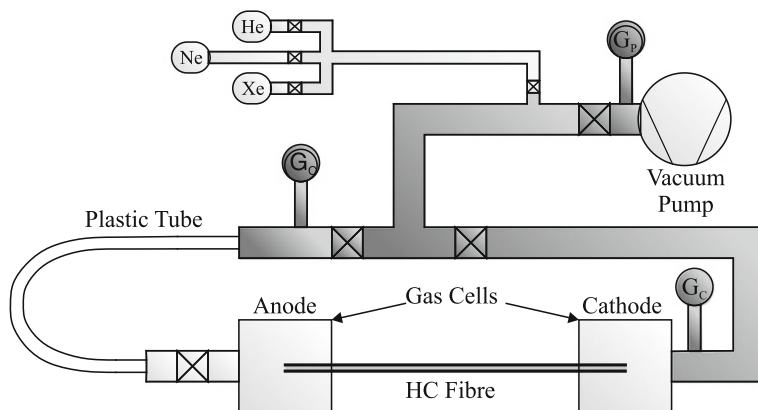
Fig. 6.3 Schematic diagram of the vacuum system. Valves are indicated by crosses, capacitance gauges by G_C and the penning gauge by G_P . KF fittings are shaded darker, with Swagelok fittings in lighter shading. The gas cells are custom made
