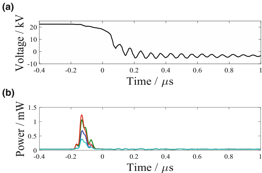
Fig. 8.8 Oscilloscope traces averaged over 128 pulses of 200:1 neon-xenon discharges at 10 mbar inside 65 cm of fibre A showing (a) the discharge voltage and (b) the unpolarised output power from an amplified InGaAs detector sensitive to 2\text{ }\mu\text{m} for the SP (blue line), FDP (green line), C (red line) and RDP (cyan line) cavity arrangements
