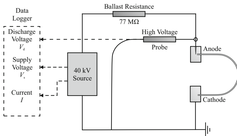
Fig. 6.5 Schematic diagram of the electrical system
