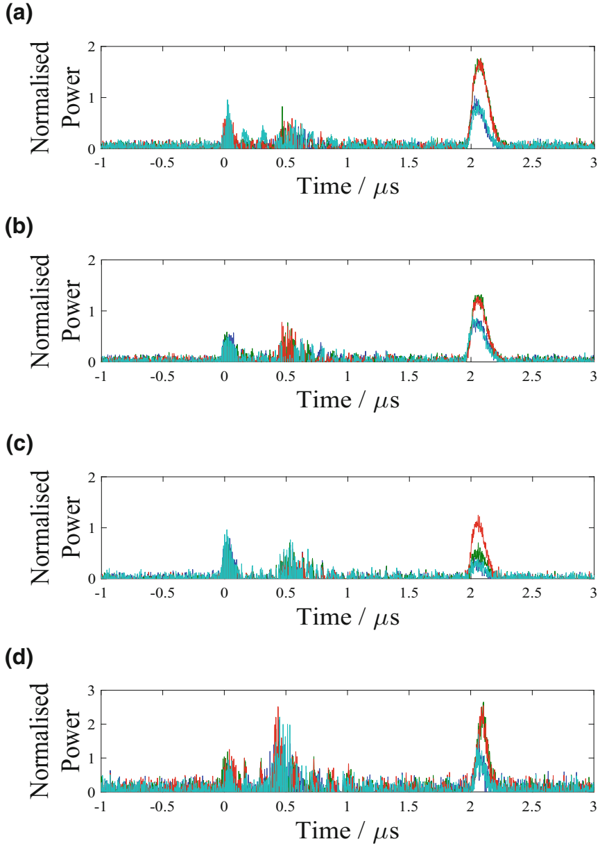
Fig. 7.12 Oscilloscope traces averaged over 64 pulses of 5 : 1 helium-xenon discharges at 12 mbar inside 140 cm of fibre B showing a–c the unpolarised, S-polarised and P-polarised output powers at 3.36 \mu\text{m} respectively normalised to the unpolarised single-pass peak and d unpolarised output power at 3.1 \mu\text{m} normalised to the single-pass peak for the single-pass (blue line), forward double-pass (green line), cavity (red line) and reverse double-pass (cyan line) cavity arrangements
