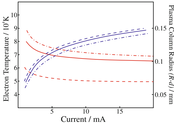
Fig. 3.8 Calculated dependence of electron temperature (blue) and plasma column radius (red) on discharge current for pure He (dashed), pure Ne (dotted) and an 8:1 mixture of He-Ne (solid) all at a pressure of 10 Torr (13.3 mbar) in a discharge tube of radius 0.2 mm. Recreated from [8]
