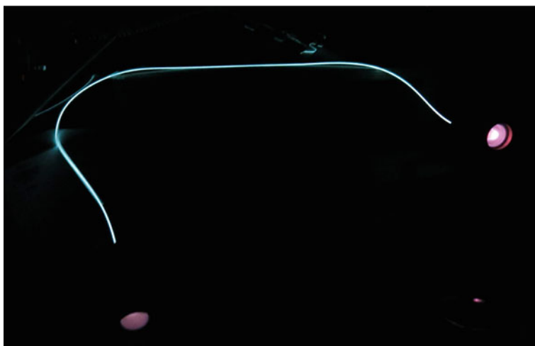
Fig. 6.11 Photograph of a helium-xenon discharge 1 m in length. The high voltage anode glow is on the left, with the cathode glow on the right
