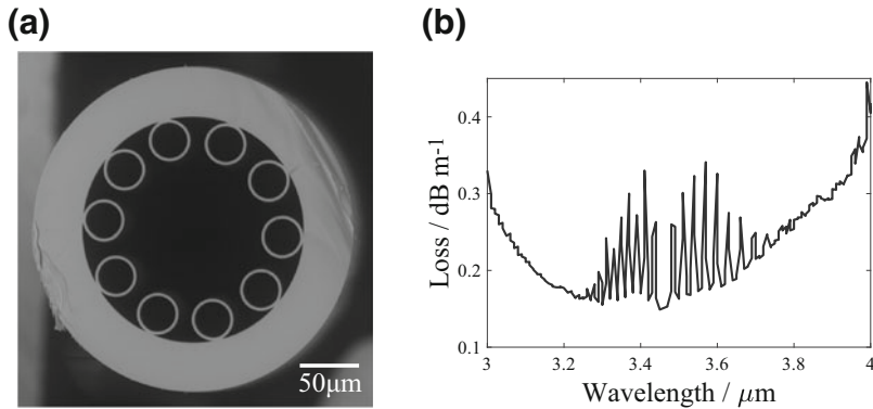
Fig. 6.1 a SEM of fibre A, with a minimum core diameter of 120 μm and resonators of diameter 35 μm and wall thickness 2.8 μm. b Measured optical attenuation of the same fibre recorded by Walter Belardi. The fine peaks between 3.2 and 3.8 μm are absorption peaks of HCl that are a remnant of the manufacturing process and can be removed by purging and evacuating the fibre [2]
