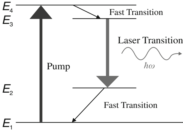
Fig. 2.4 Energy diagram of a 4-level laser system
