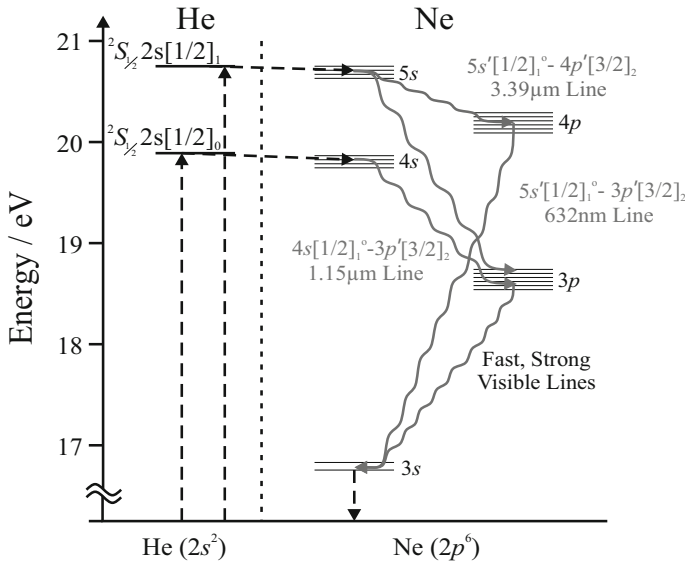
Fig. 4.6 Partial energy level diagram for helium-neon. The coincident energies of the 2S_{\frac{1}{2}} 2s[\frac{1}{2}]_1 and 2S_{\frac{1}{2}} 2s[\frac{1}{2}]_0 helium and the 5s and 4s neon levels respectively provide high collisional cross sections for atom-atom excitation transfer, allowing for fast population of these upper states and lasing on a number of lines
