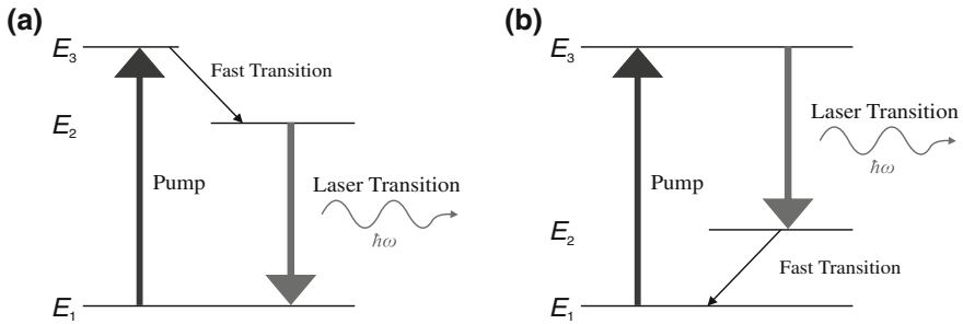
Fig. 2.3 Energy diagrams of 3-level laser systems as used in a the first ruby laser and b electrically pumped gas lasers
