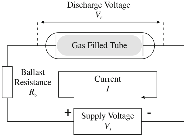
Fig. 3.1 A simple gas discharge circuit
