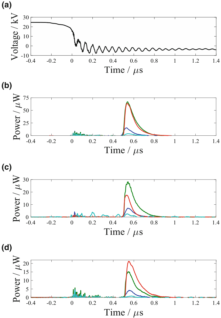
Fig. 8.5 Oscilloscope traces averaged over 128 pulses of 200:1 neon-xenon discharges 10 mbar inside 65 cm of fibre A showing (a) the discharge voltage, (b)–(d) the unpolarised, S-polarised and P-polarised output powers respectively for the SP (blue line), FDP (green line), C (red line) and RDP (cyan line) cavity arrangements. The noisy RDP trace in (c) is a result of a slight discrepancy between the ‘light’ and ‘dark’ traces, which is magnified by the subtraction of the dark trace
