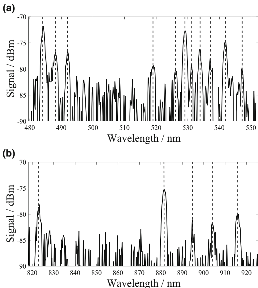
Fig. 7.4 Spectra of the light collected using a standard 600 \mu\text{m} core step-index multimode fibre patch cord ( \text{NA} \approx 0.4 ) from the side of a 5:1 helium-xenon discharge inside fibre B at a pressure of 12 mbar, measured by a Yokogawa AQ-6315A optical spectrum analyser with a resolution of 1 nm. Identified emission lines are marked with dashed lines
