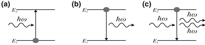
Fig. 2.1 Simple energy level diagrams for a absorption, b spontaneous emission and c stimulated emission, all involving a photon of energy E = E_2 - E_1 = \hbar\omega
