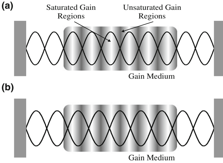
Fig. 2.7 Spatial hole-burning in a homogeneously broadened laser, demonstrated by two cavity modes of order a N = 10 and b N = 9 . The antinodes of mode (a) deplete the gain of the medium in specific regions, indicated by the white bands, leaving regions of high gain for the antinodes of mode (b) to feed off of
