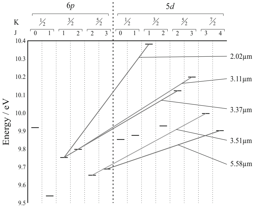
Fig. 4.4 Partial energy level diagram for xenon featuring a selection of the major mid-IR laser transition lines
