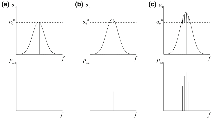
Fig. 2.8 Saturated gain coefficient \alpha_1 and output power P_{out} for different longitudinal modes in an inhomogeneously broadened laser as pumping is increased (a) to threshold (b) just above threshold and (c) further above threshold
