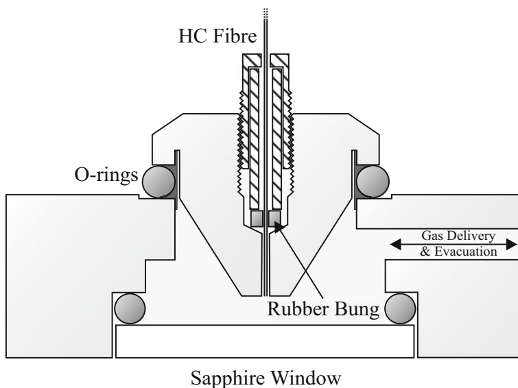
Fig. 6.4 Schematic diagram of the cathode gas cell. The majority of the cell (shaded light grey) is made of brass, while the rod and screw of the fibre holder (diagonal lined) are made of Delrin plastic. The fibre holder and window are secured in place by brass supports screwed in the cell
