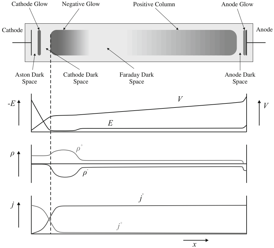
Fig. 3.3 Distribution of dark and luminous regions, electric field E , accumulated potential difference from the cathode V , positive and negative space-charge densities \rho^+ & \rho^- and current densities j^+ & j^- for the ions and electrons respectively in a glow discharge
