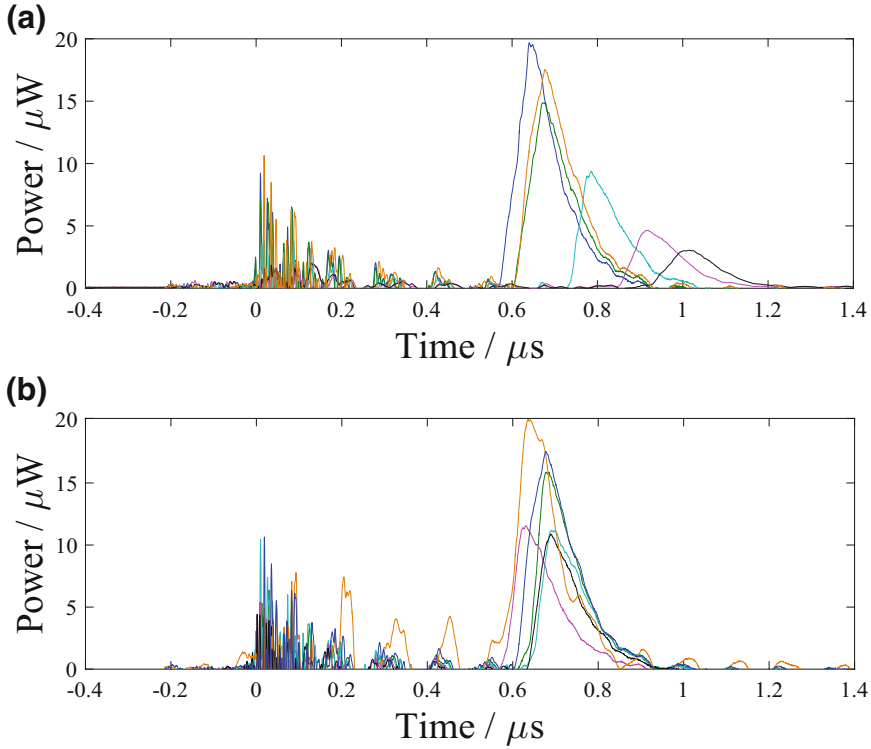
Fig. 8.4 Oscilloscope traces of the single-pass output power from Ne-Xe discharges inside 80 cm of fibre A at pressures of 12 (blue), 18 (green), 24 (cyan), 30 (magenta), 36 (black) and 12 mbar (orange) for (a) a fixed 120:1 Ne-Xe ratio and (b) a fixed 0.1 mbar of Xe. All traces are taken with an averaging of 128
