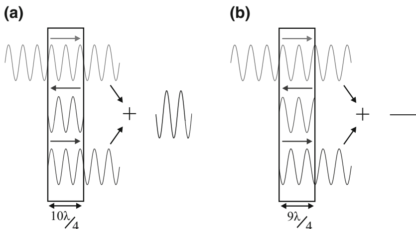
Fig. 5.5 A representation of thin film interference for a beam at normal incidence. A partial reflection (middle) from a primary beam (top) at the rear boundary is reflected back to exit the film (bottom) with a phase difference \delta_{ph} = \frac{4\pi}{\lambda}nd . In a the beams are in phase, constructive interference occurs and there is high transmission. In b the beams are exactly out of phase, destructive interference occurs and there is a strong reflection
