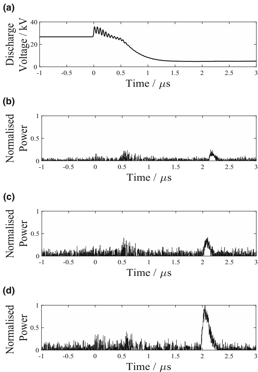
Fig. 7.7 Oscilloscope traces averaged over 64 pulses of 5:1 helium-xenon discharges at 12 mbar inside 70 cm of fibre B showing a the discharge voltage and the single-pass output powers measured through the Bentham TMc300 monochromator at b 3.11 \mu\text{m} , c 3.36 \mu\text{m} and d 3.51 \mu\text{m} . The power traces have been normalised to the 3.5 \mu\text{m} line peak power. The 3.11 and 3.36 \mu\text{m} measurements were made with a 20 nm resolution, while the 3.51 \mu\text{m} measurement was made with a 10 nm resolution
