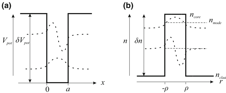
Fig. 5.2 a Solutions to the Schrödinger equation in a 1D finite potential well, where a is the width of the well and \delta V_{pot} is the potential drop, and b solutions to the Maxwell equations for a step-index fibre
