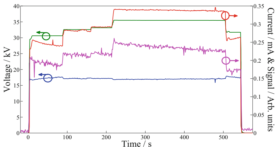
Fig. 6.12 Electrical properties of a typical 5 : 1 helium-xenon gas discharge at a pressure of 12 mbar inside 70 cm of fibre A with a ballast resistance of 54 M \Omega . Left axis; supply voltage (green) and discharge voltage (blue). Right axis; current (red) and signal (purple)
