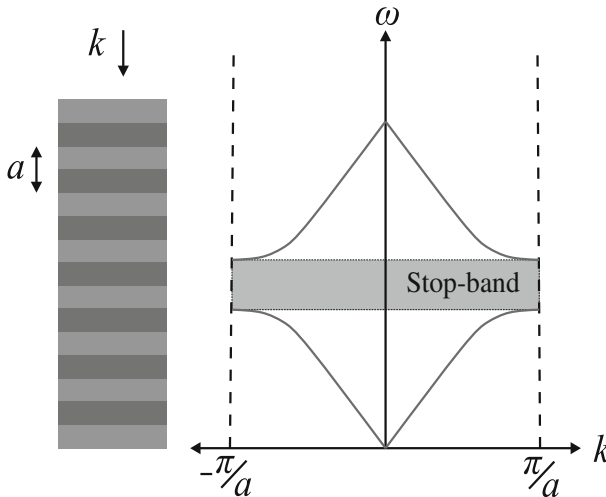
Fig. 5.4 A ‘1D photonic crystal’ and its dispersion relation. The periodic array of high index regions (dark grey) within a low index region (light grey) create a photonic stop-band (the 1D equivalent of a bandgap) in the dispersion relation, preventing light of certain frequencies from passing through the crystal
