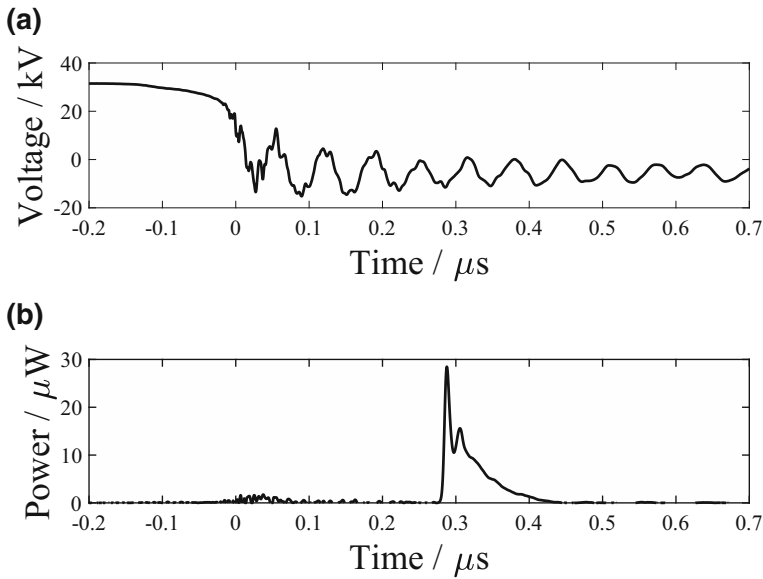
Fig. 8.1 Oscilloscope traces averaged over 128 pulses of 5:1 helium-neon discharges with trace amounts of xenon at 42 mbar inside 55 cm of fibre B showing a the discharge voltage and b the output power
