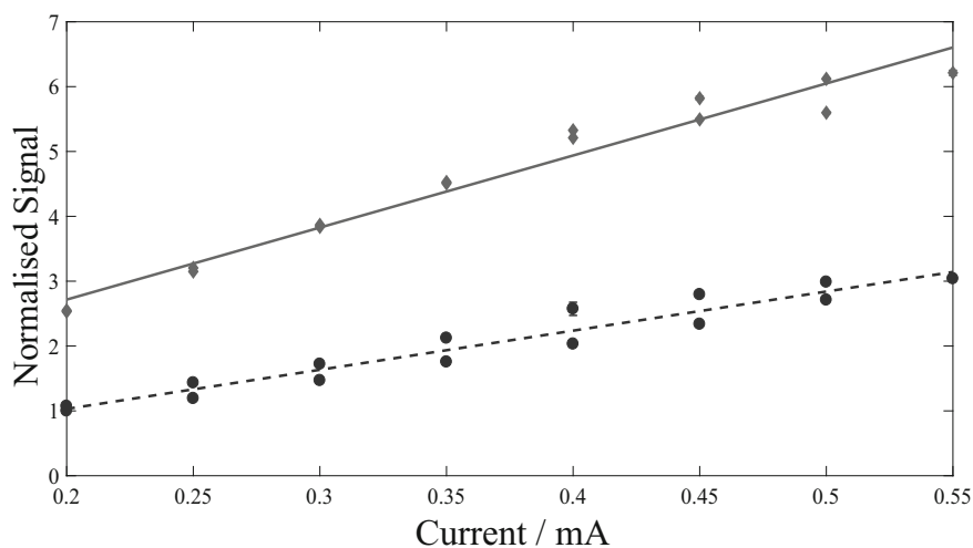
Fig. 6.17 Repeat of the double pass measurement in a fresh 1 m length of fibre A. All other parameters are the same as in Fig. 6.15
