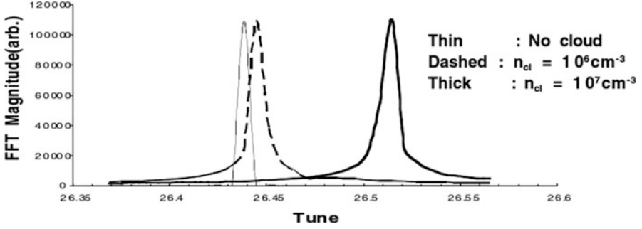
Fig. 1.12 Presence of an electron cloud shifts the betatron frequency at CERN SPS. Simulation for different cloud densities made using a QUICKPIC code [27]. The tune spread is relatively small (much less than the tune shift), suggesting that the force of the electron cloud is almost linear with displacement. The model did not include gradients of the cloud density along the ring
