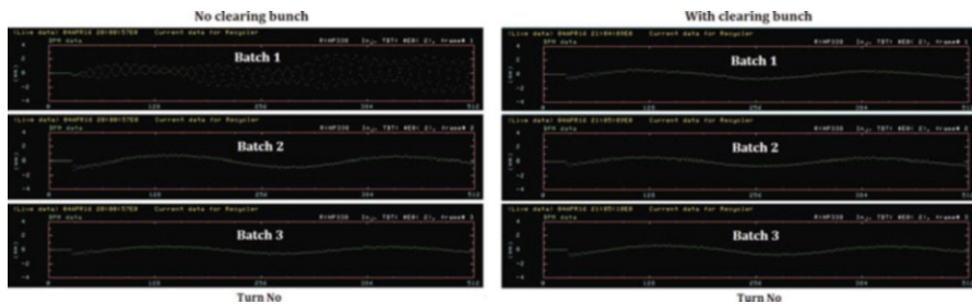
Fig. 2.16 Without the clearing bunch, the first batch is unstable, with the clearing bunch all beams are stable. Horizontal position of the beam center is plotted vs number of revolutions after its injection. Beam: 5.8 \times 10^{10} ppb
