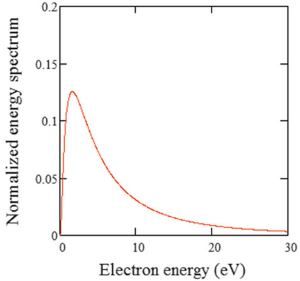
Fig. 1.3 Most of the true secondary electrons have relatively low energies, below 10 eV
