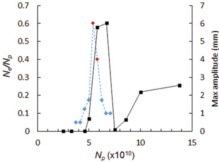
Fig. 4.14 Electron cloud density reaches its maximum density at the intensities of N_p \sim 6 - 7 \times 10^{10} ppb. The vertical axis shows the normalized electron cloud density N_e/N_p . The dashed line shows the maximum betatron amplitude measured for these intensities
