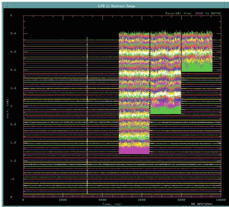
Fig. 2.15 Positions of the clearing bunch and three high-intensity batches. The horizontal axis shows bunch position in the ring in nanoseconds, the vertical – time into the machine cycle, the separation between the horizontal lines is 300 revolutions (3.3 ms)
