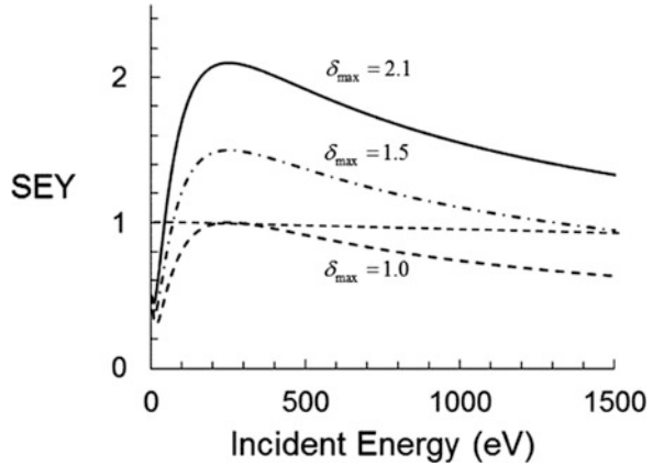
Fig. 1.4 The material behaves as an absorber when the secondary yield \delta < 1 and as an emitter when \delta > 1
