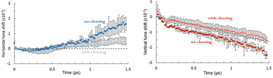
Fig. 2.13 Presence of the clearing bunch reduces the tune shift between the head and the tail of the high-intensity bunch train: 5 \times 10^{10} ppb, 80 bunches. The error bars represent the spread between different measurements. The black dotted lines represent the resistive wall tune shift
