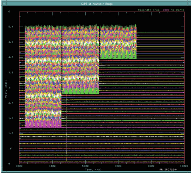
Fig. 2.17 The clearing bunch (the single spike) stabilizes the first high-intensity batch; it is then thrown away and the second and third batches are injected. No fast instability is observed in any of the batches. The horizontal axis shows bunch position in the ring in nanoseconds, the vertical – time into the machine cycle, the separation between the horizontal lines is 300 revolutions (3.3 ms)
