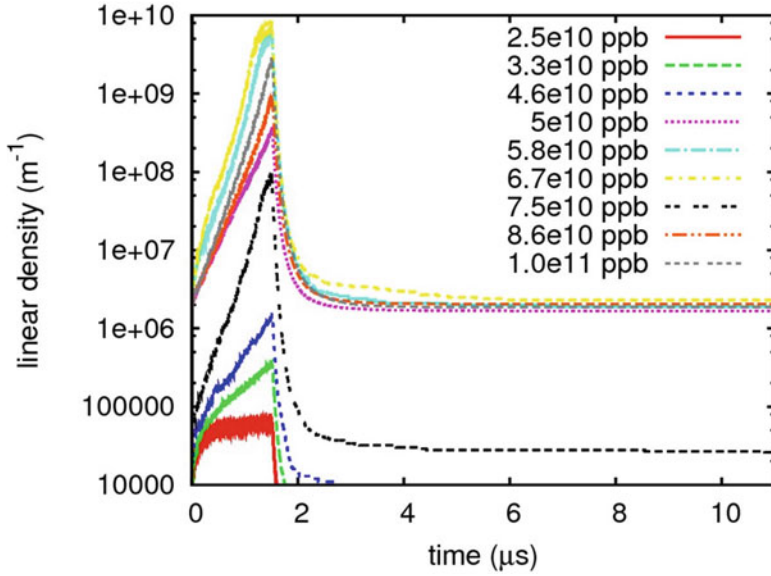
Fig. 4.13 The final distribution of the electron cloud density after 20 revolutions of multi-turn build-up. One batch of different intensities. \text{SEY} = 2.1 , \sigma_z = 40 cm, ionization density 10^4 \text{ m}^{-1}
