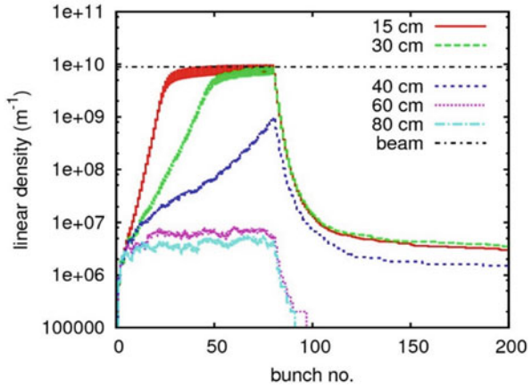
Fig. 4.7 The build-up of electron cloud is much faster for shorter bunches. SEY = 2.1; single pass, N_b = 5 \times 10^{10} , 80 bunches; ionization density 10^6 \text{ m}^{-1}
