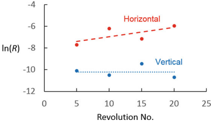
Fig. 4.20 The instability develops only in the horizontal plane. The dashed lines represent linear fits. The horizontal growth rate is 8.6 \times 10^{-2} \text{ rev.}^{-1} , the vertical growth rate is 0
