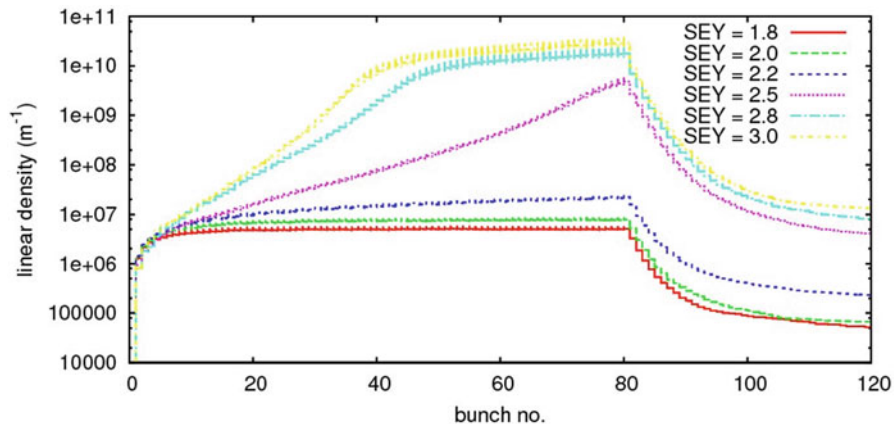
Fig. 4.6 A small change in SEY leads to a drastic increase of electron cloud density after the passage of one bunch train. N_b = 5 \times 10^{10} , \sigma_z = 60 cm. At high SEY, the cloud reaches saturation at about the linear density comparable to the density of the beam ( \sim 9 \times 10^9 \text{ m}^{-1} )
