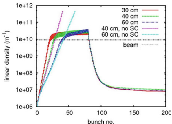
Fig. 4.8 The electron cloud saturates at a linear density comparable with the density of the beam, independent of its bunch length. Without the self space charge, the cloud intensity continues to grow exponentially with no saturation (no SC lines). The lines show different bunch lengths for the same intensity N_b = 5 \times 10^{10} and SEY = 3.0
