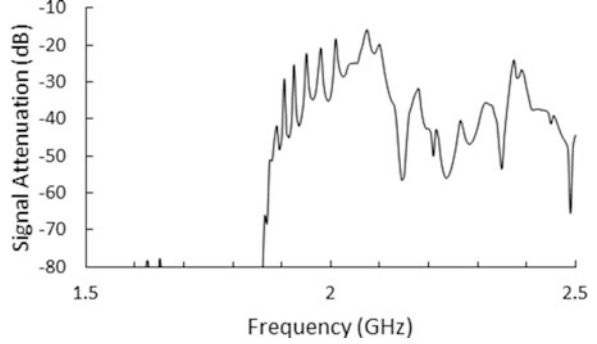
Fig. 3.3 The BPMs reflect most of the power back at 2 GHz. The total transmission loss due to reflection is 20–30 dB. Beam-pipe cutoff frequency is 1.87 GHz
