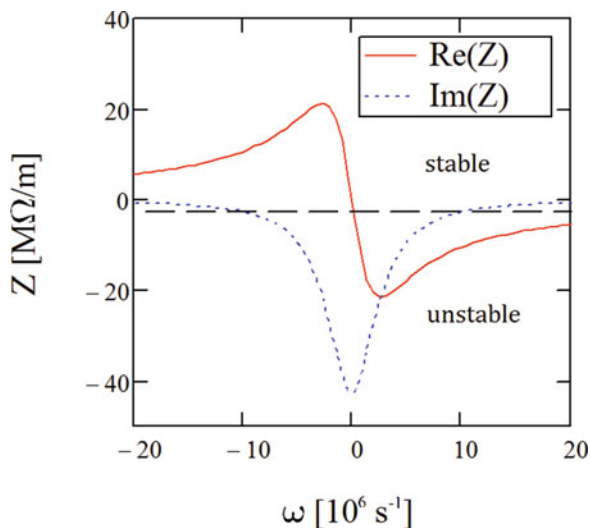
Fig. 5.3 Real and imaginary parts of impedance as a function of a mode angular frequency \omega . The dashed line represents the Landau damping term in Eq. (5.15). The modes with \text{Re}(Z(\omega)) below the dashed line are unstable
