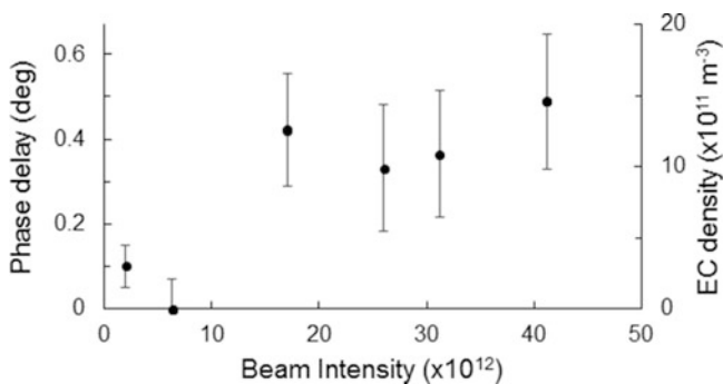
Fig. 3.6 The electron cloud density increases dramatically above 1 \times 10^{13} \text{ p} total beam intensity
