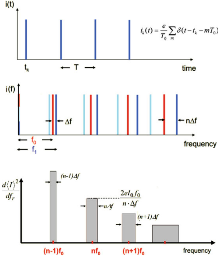
Fig. 3.4 Single particle current (top) and spectrum (middle) are series of periodic delta-functions. When all the particles in the beam are added together, the resulting spectrum gets broader with frequency (bottom) [10]
