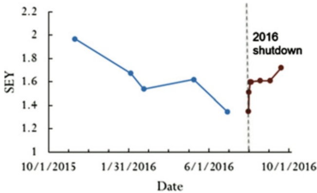
Fig. 1.15 The SEY decreases during an accelerator run and then rapidly increases after the beam has been turned off. SEY measurement at the Fermilab Main Injector test stand during the 2015–16 run and the following maintenance shutdown [31]
