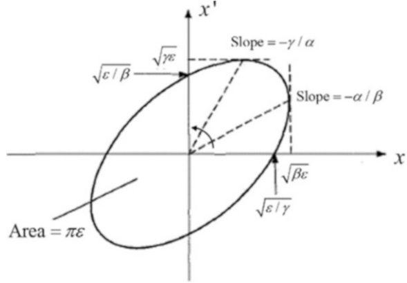
Fig. 4.19 The phase space trajectory in the physical coordinates x and x' is an ellipse. \alpha , \beta , and \gamma are the Twiss parameters, \varepsilon is the Courant-Snyder invariant \varepsilon = \gamma x^2 + 2\alpha x x' + \beta x'^2 = \text{const} [15]
