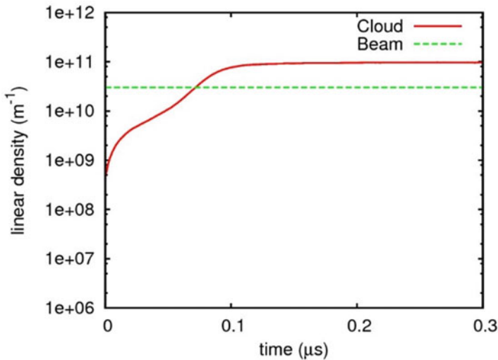
Fig. 4.11 The electron cloud reaches the saturation density within one revolution period in the DAFNE ring. The ring circumference of 0.3 \mu s is uniformly filled with 120 e^+ bunches, N_b = 2.4 \times 10^{10} . The key ring parameters are summarized in Table 4.2
