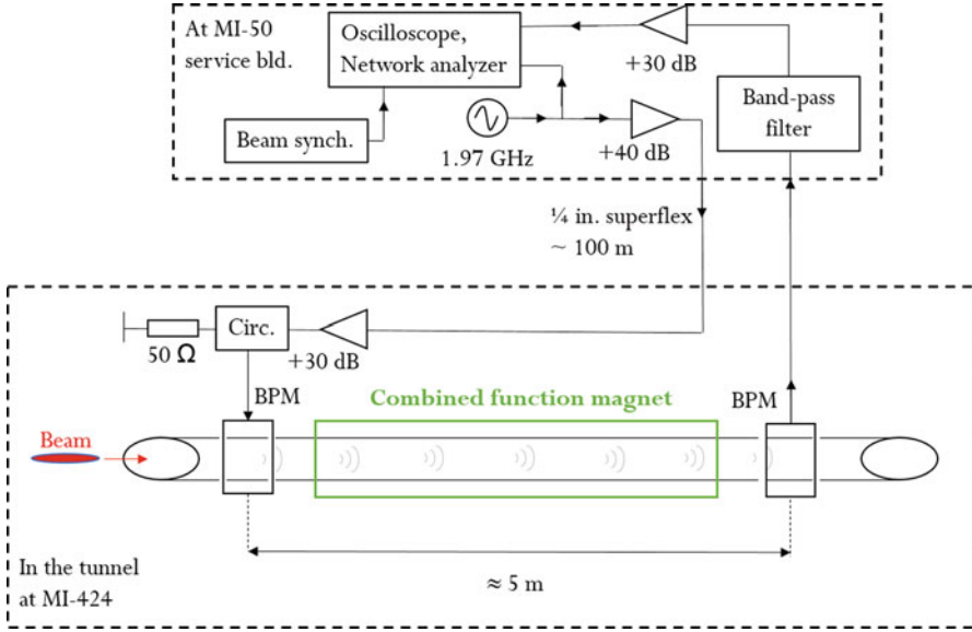
Fig. 3.2 Layout of the microwave measurement setup
