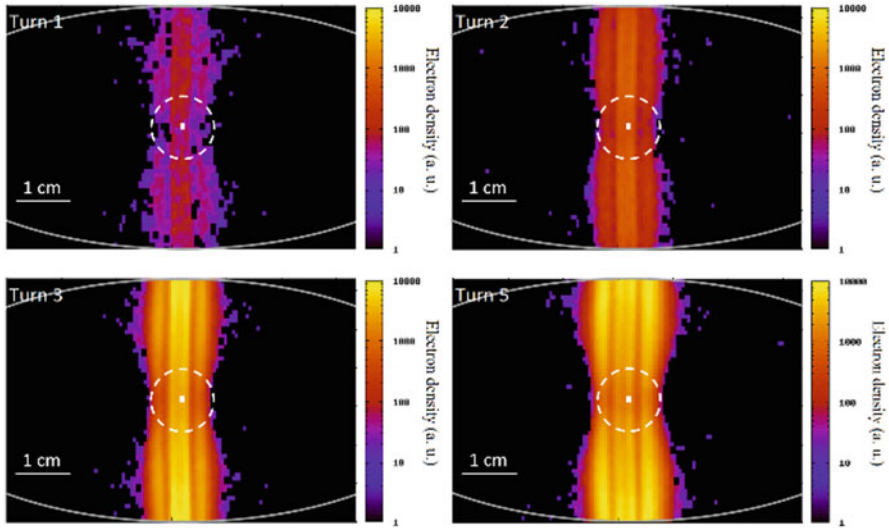
Fig. 4.10 Electron cloud forms a stripe inside the vacuum chamber and its intensity increases with the number of turns. Its horizontal position – beam center (white dot). White circles represent 2 rms beam size
