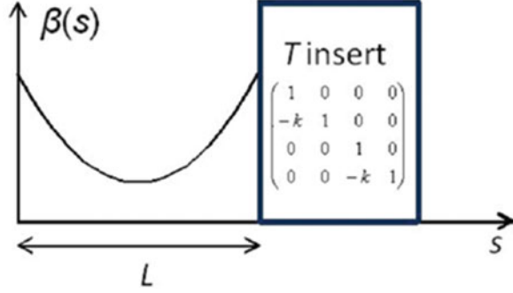
Fig. 5.8 The ring outside of the nonlinear section has a transfer matrix of a thin axially symmetric lens [13]
