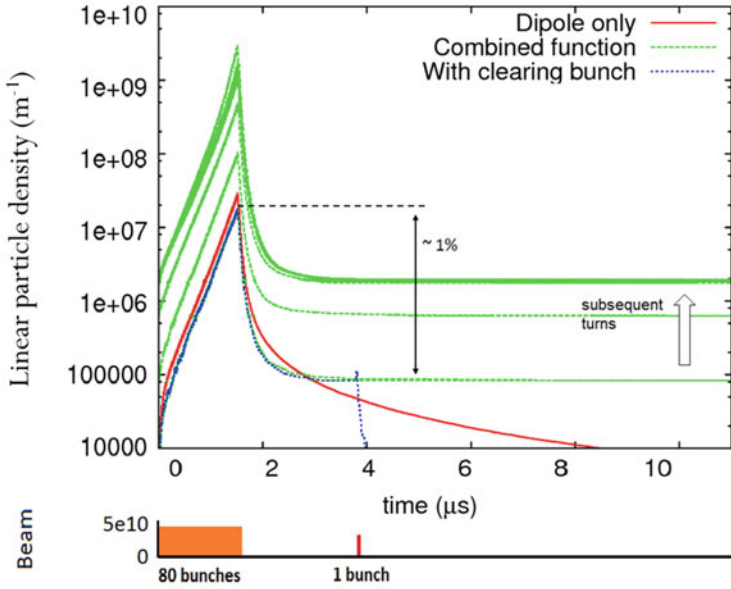
Fig. 4.12 A clearing bunch destroys the trapped cloud, preventing the multi-turn accumulation in a combined function magnet. The resulting maximum electron cloud density is the same as in a pure dipole. Beam: 5 \times 10^{10} ppb, 80 + 1 bunches
