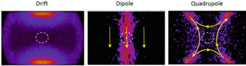
Fig. 1.8 Snapshots of electron cloud density in a drift section (left), a dipole (middle), and a quadrupole (right). Yellow lines show the direction of the external magnetic field; white circle represents 2 rms beam size. The distribution was simulated using the PEI code. The simulation procedure and parameters of the model are described in Chap. 4
