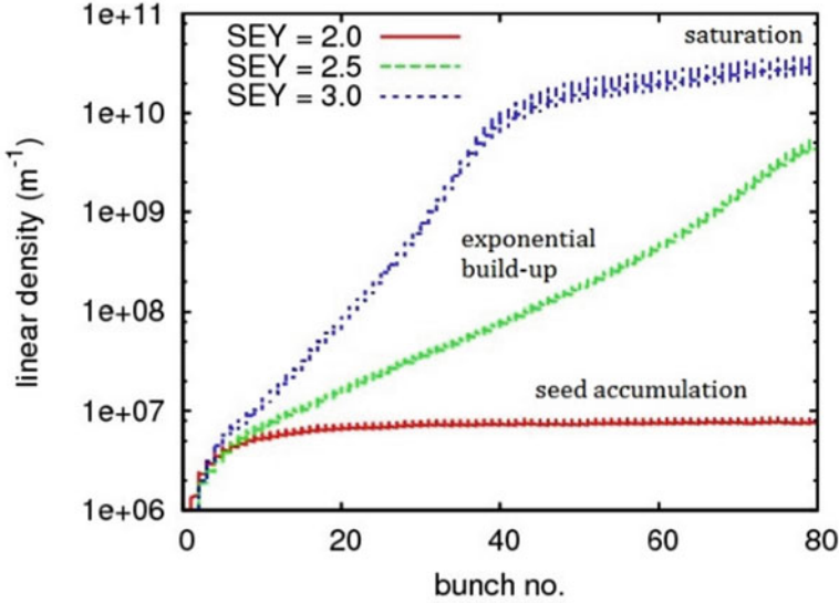
Fig. 1.5 As the secondary yield increases, the electron cloud goes from the seed accumulation regime to the exponential build-up. Linear density of the cloud in a Recycler dipole magnet is plotted as a function of time during a passage of a typical proton bunch train of 80 bunches. Each bunch produces 10^6 \text{ m}^{-1} primary ionization e^- . The SEY stands for the maximum total yield, achieved at E = 250 \text{ eV}
