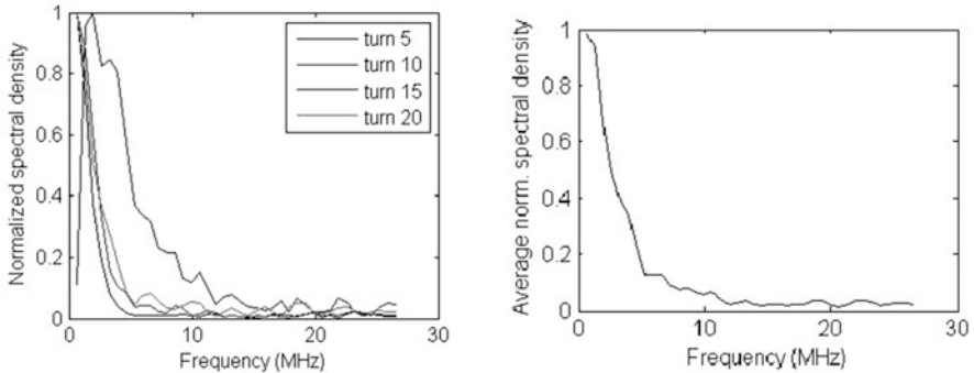
Fig. 4.21 The frequency of the most unstable mode is 0.66 MHz. Left – the evolution of the spectrum over the time scope of the instability – 20 turns. Right – the normalized spectral density, averaged over the last ten revolutions
