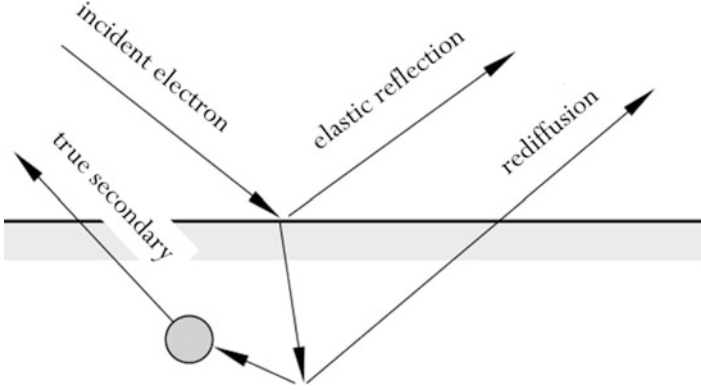
Fig. 1.2 The three types of emission processes. The blob represents a nontrivial interaction yielding true secondary electrons [18]
