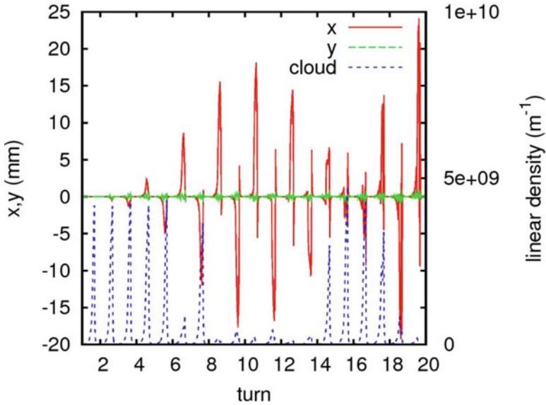
Fig. 4.18 As the electron cloud reaches its maximum density, the horizontal instability starts developing. The horizontal and vertical positions of every bunch in the batch and the electron cloud density are plotted for the first 20 revolutions after the cloud has accumulated to its maximum density (about 5 \times 10^9 \text{ m}^{-1} ). On the 21st revolution, the simulation was stopped due to loss of some of the particles
