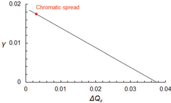
Fig. 5.7 The estimated instability growth rate decreases linearly with the spread of horizontal betatron frequencies
