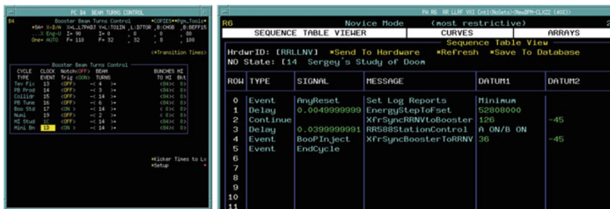
Fig. 2.2 ACNET control of injecting beam. Left – Booster intensity control that allows changing the beam intensity (in turns) and the number of bunches for each specific event. Right – Recycler injection control with two injection events into the RF buckets 126 and 36; RF frequency set at 52.8 MHz, RF phase – at -45^\circ
