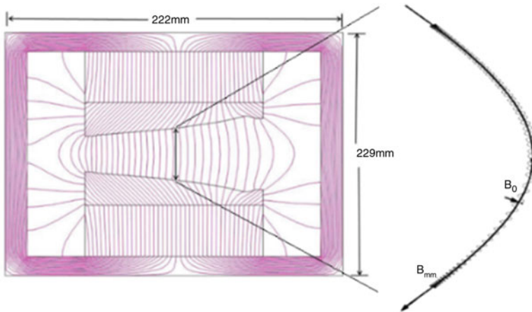
Fig. 4.1 Electron cloud can get trapped by magnetic field of a combined function magnet. Cross section of a Recycler permanent combined function dipole; the vacuum chamber is not shown
