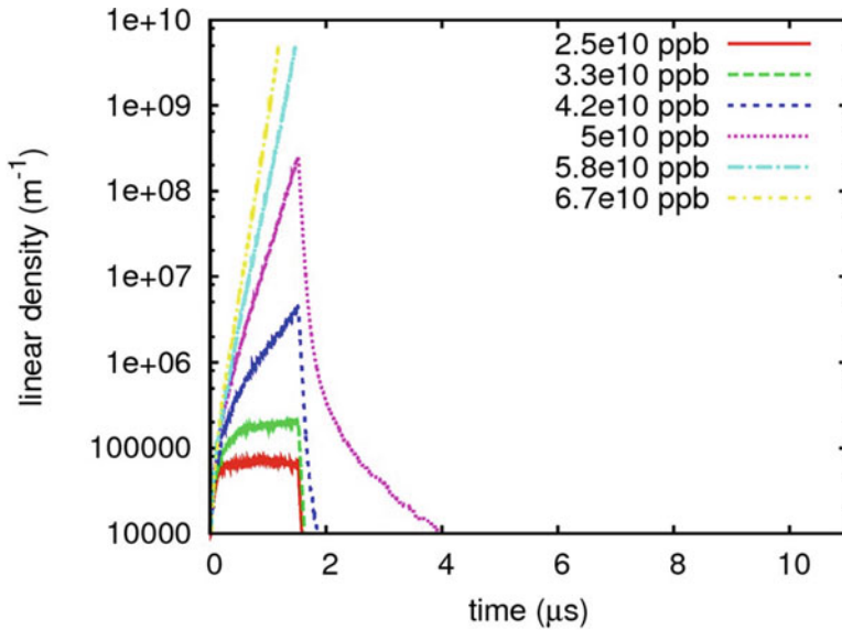
Fig. 4.16 The cloud in a drift section accumulates rapidly during the passage of a bunch train for beam intensities greater than 4 \times 10^{10} ppb, it then decays quickly after the beam has left the section. SEY = 2.1, \sigma_z = 40 cm. At the highest intensities the computation was interrupted after exhausting all available memory
