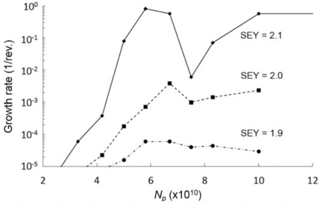
Fig. 5.6 The maximum growth rate is achieved at the intensities of 6 - 7 \times 10^{10} ppb. The growth rate decreases significantly for lower secondary emission yield
