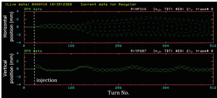
Fig. 2.4 The fast blow-up of beam centroid oscillations is observed only in the horizontal plane. Turn-by-turn measurement of beam position of 1 batch after its injection into Recycler
