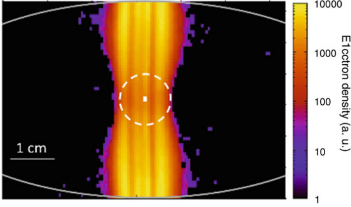
Fig. 5.1 Electron cloud forms a stripe inside the vacuum chamber; the beam center and its 2 rms size are shown in white (for more details refer to the Sect. 4.3.4)
