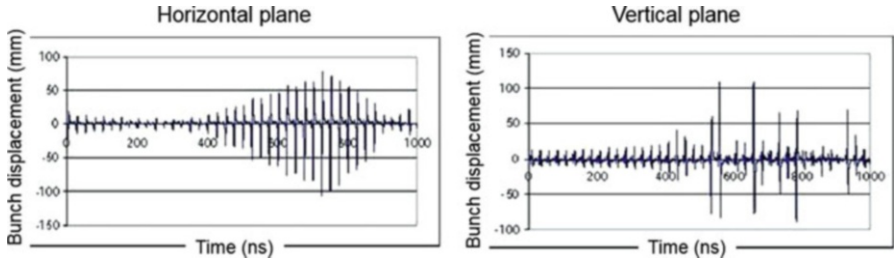
Fig. 1.11 At SPS the electron cloud instability is multibunch in the horizontal plane (left) and single-bunch in the vertical (right). Snapshots of the horizontal position of the first 48 bunches in the SPS when the instability is present [24]
