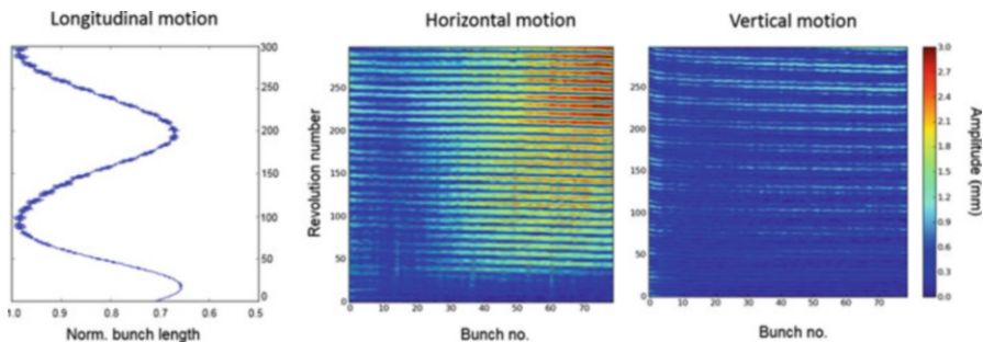
Fig. 2.7 The instability mostly affects the last bunches in the train. It starts after the beam compresses longitudinally (left) and then becomes more severe after it compresses again, half a synchrotron period later. The color depicts the amplitude of the horizontal betatron oscillations of the beam center of mass as a function revolution number and position within the batch. The horizontal stripes caused by our sampling of beam position once a revolution and appear at twice the betatron frequency: 2Q_x = 0.9 or 1/10 turns. The data was gathered over 300 revolutions with the transverse dampers off. Beam: 1 batch, 80 bunches, 5 \times 10^{10} ppb
