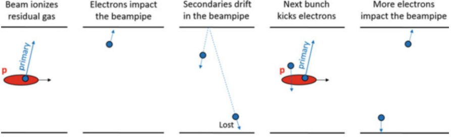
Fig. 1.1 A schematic illustration of the build-up of the electron cloud. The process starts with a proton bunch ionizing residual gas, thus creating primary electrons, and is amplified through the secondary emission
