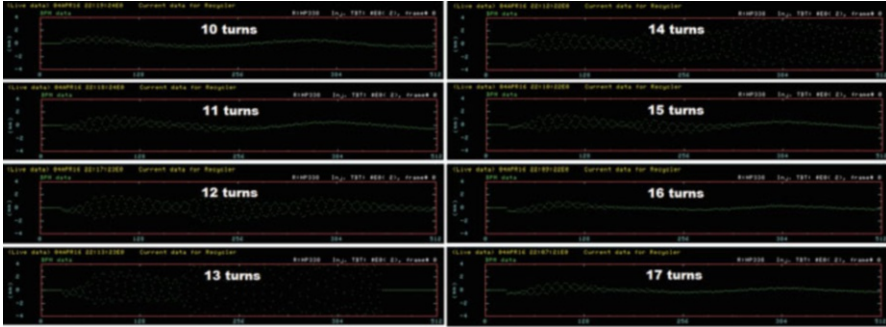
Fig. 2.9 The instability goes up and then down with intensity (in Booster injection turns). Horizontal position of the beam center vs revolution number; 1 batch of 80 bunches; \xi_{x,y} = -6, -8
