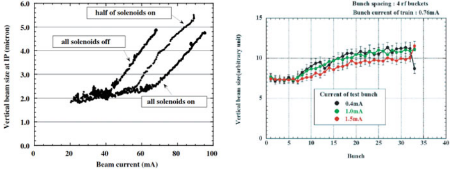
Fig. 1.10 Left – vertical beam size of the KEB increases above the threshold current. Installation of solenoids covering 800 m of ring circumference allows increasing the threshold. Two trains with 60 bunches with a bunch spacing of 4 RF buckets were injected in opposite sides of the ring. Right – when a test bunch follows the beam, its vertical size increases. The horizontal axis shows the length of the main bunch train [24]
