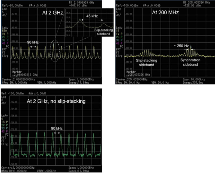
Fig. 3.5 Spectrum of the Recycler Schottky signal. When the machine operates with the slip-stacking, the two beams of different energies produce signal at the revolution harmonics of \sim 90 kHz. Because of the 2 kHz difference in the frequencies, the signals separate at high harmonic numbers. At 2 GHz (harmonic number n_h \sim 2 \times 10^4 ), the slip-stacking signal is in the middle between the main peaks (top-left). The slip-stacking signal disappears when the machine operates with a monochromatic beam (bottom left). At 200 MHz ( n_h \sim 2 \times 10^3 ) one can resolve the sidebands on the harmonics of the synchrotron frequency (top right). The distance to the slip-stacking sideband scales with the harmonic number: it is \sim 4.5 kHz at 200 MHz and \sim 45 kHz at 2 GHz
