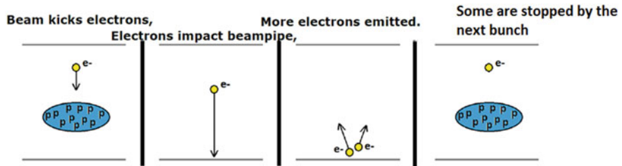
Fig. 4.2 The first bunch kicks the cloud, creating secondary electrons, the second bunch stops some of them
