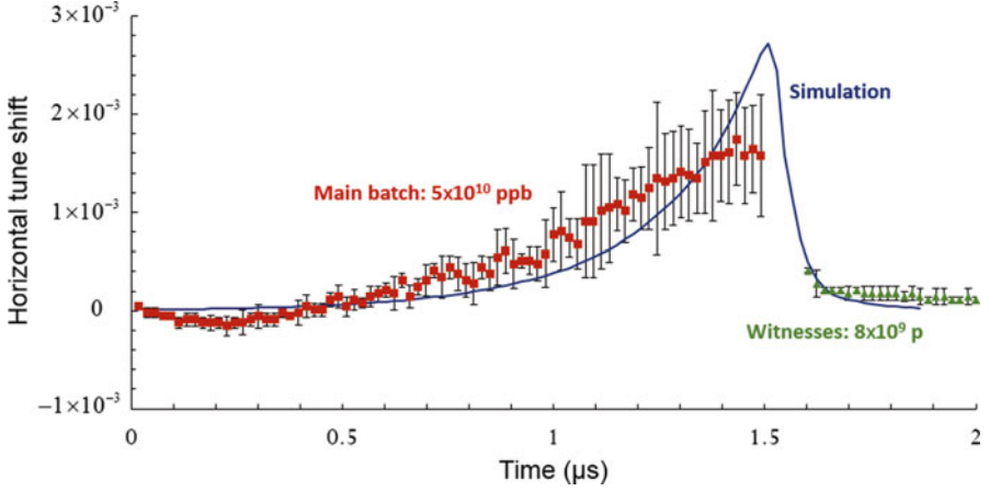
Fig. 5.2 Results of the electron cloud simulation agree with the measured horizontal tune shift. Beam: 5 \times 10^{10} ppb, 80 bunches, followed by one witness bunch of 0.8 \times 10^{10} p at various positions. The gap between the high-intensity batch and the witness is due to the rise-time of the injection kickers
