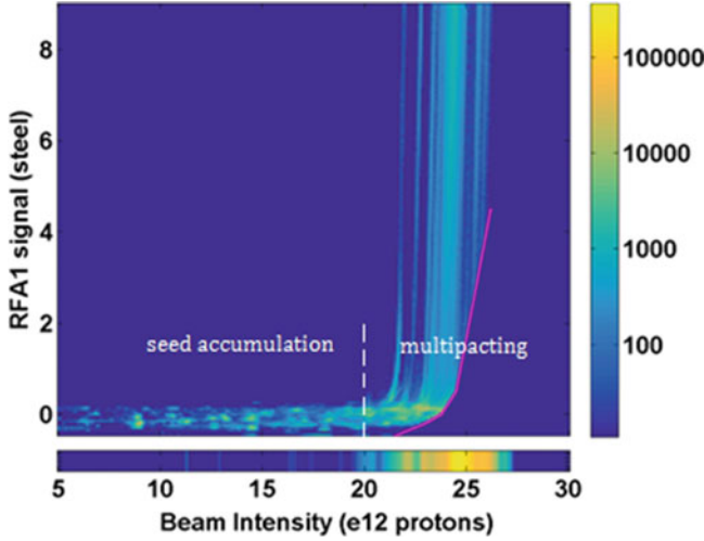
Fig. 1.6 The density of the electron cloud increases dramatically as the beam intensity crosses the threshold. The signal from an electron cloud retarded field analyzer (RFA) detector, installed in the Fermilab Main Injector, is plotted as a function of the total beam intensity. The color represents the strength of the signal in a logarithmic scale. Above the threshold intensity of \sim 20 \times 10^{12} p most of the signals exceeded the voltage limits of the preamplifier; this data is shown separately below the main plot [21]
