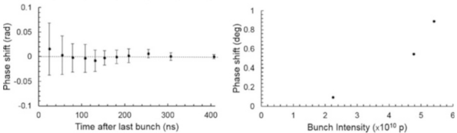
Fig. 3.7 Left – the average phase shift decreases with time after the beam has left the combined function magnet; beam: 80 bunches, 5.4 \times 10^{10} ppb. Right – the maximum phase shift, measured 25 ns after the last bunch, increases with the beam intensity; error bars not shown. RF frequency: 1.970 GHz
