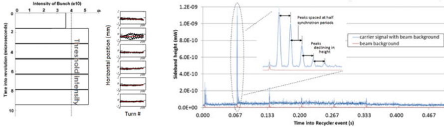
Fig. 3.1 Left – the first batch above the threshold intensity suffers the blow-up after injection into the ring. Right – a phase modulation of the 2.0 GHz carrier at the revolution frequency of 90 kHz occurs simultaneously with the instability. The fine structure of the modulation sideband implies that it is connected with the longitudinal quadrupole oscillations that have a periodicity of a half of the synchrotron period [6]
