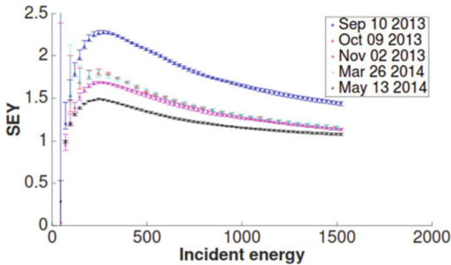
Fig. 1.14 The secondary emission yield of 316L stainless steel reduces significantly as it conditions under the exposure to the accelerator beam during the 2013–14 run [30]
