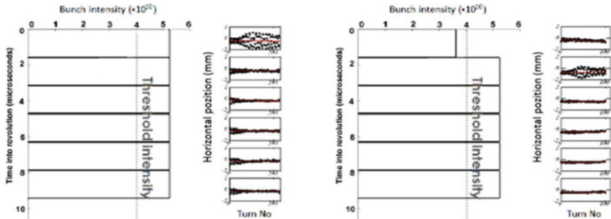
Fig. 2.8 The first batch above the threshold intensity suffers the blow-up after injection into the ring. The plots show bunch intensities of six consecutive injections into the Recycler and turn-by-turn measurement of the beam center horizontal position for each injecting batch. Left – the first batch is above the threshold intensity of 4 \times 10^{10} ppb and is affected by the instability; the other five batches of the same intensity remain stable. Right – the first batch below the threshold, the instability moves to the second batch [2]
