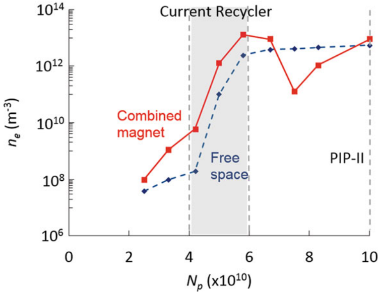
Fig. 4.17 Combined function magnets provide one to two orders of magnitude greater electron cloud density at the beam center n_e than the free space at the current Recycler intensities. For the higher PIP-II intensities, the tow effects are comparable. SEY = 2.1, \sigma_z = 40 cm, P = 10^{-8} Torr
