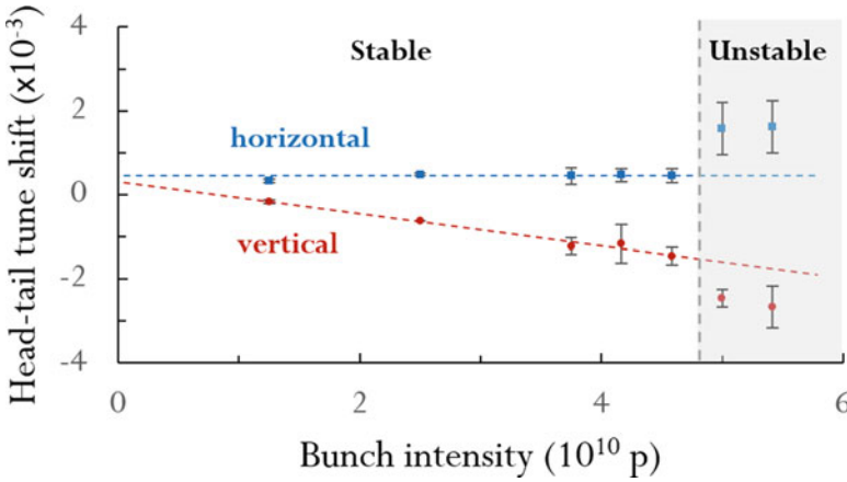
Fig. 2.14 The resistive wall contribution of the head-tail tune shift scales linearly with the beam intensity. The slope is horizontal ( <0.1/10^{10} p) in the horizontal plane and \sim 0.4/10^{10} p in the vertical. The resistive wall part of the tune shift of an unstable beam above the threshold (gray area) can be found by extrapolation. The small positive offset (non-zero shift at zero intensity) is probably caused by the injection mismatch of the leading bunches due to the finite rise time of the injection kickers
