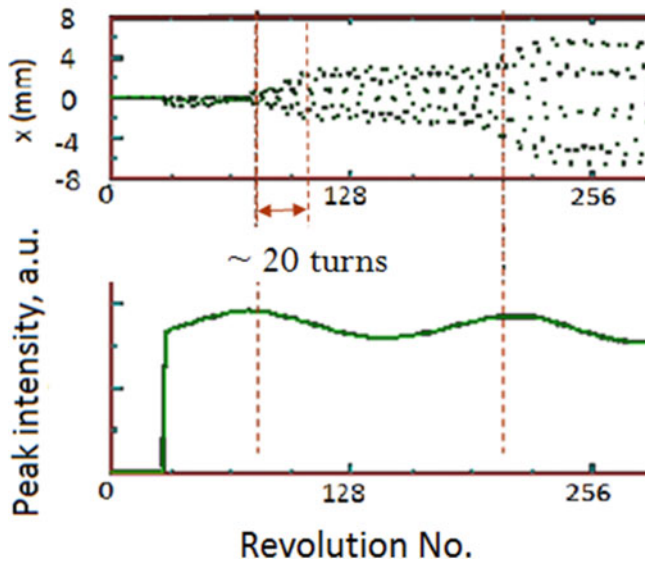
Fig. 2.6 The beam becomes unstable horizontally when its bunch length shrinks due to synchrotron oscillations and its peak intensity increases. Top – turn-by-turn BPM measurement of the beam centroid position, bottom – turn-by-turn measurement of the peak beam intensity
