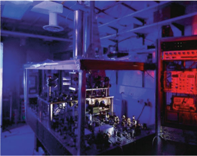
Fig. 6.9 The modern alternative to the sundial, clepsydra, or the pendulum clock – the NIST-F1 Cesium Fountain atomic clock, which provides the most accurate time standard available in the world, and keeps time to within better than one part in a thousand trillion (image courtesy of NIST)
