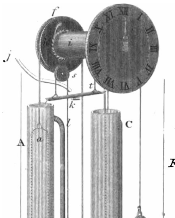
Fig. 6.7 Schematic of an early falling weight clock showing the escapement (the ratcheted wheel) which metes out equal units of time as the weight falls downward (figure from Lockyer and Seabroke 1878 )
