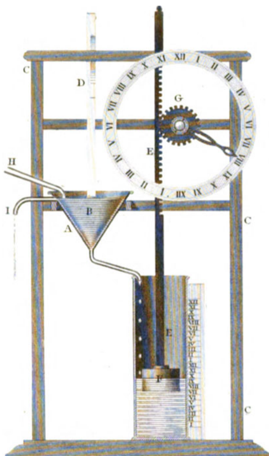
Fig. 6.5 An early European Clepsydra, showing a very simple design in which the rising water level raised a rod (E) which turned a gear attached to a timekeeping dial (Rees 1819)
