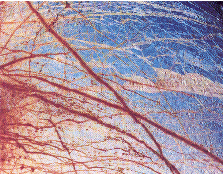
Fig. 8.2 A composite image from the Galileo spacecraft highlighting some of the prominent features on the surface of Jupiter’s moon Europa, including the Minus Linea region (cf., Table 8.2 )
