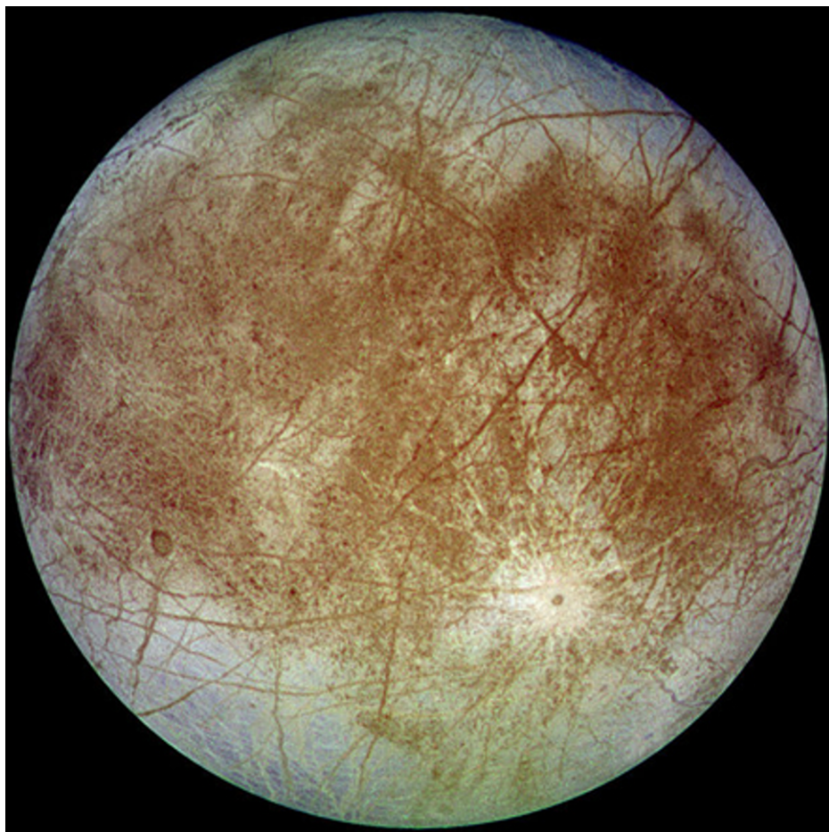
Fig. 8.3 During the Galileo orbit G2 a full hemisphere of Europe was imaged in great detail capturing most of the 'trailing hemisphere', so called since the satellite motion is in the visual direction penetrating the page. The remarkable detail includes the famous Will crater lower than the centre slightly below
