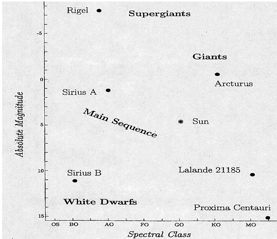
Fig. 1.7 The Hertzsprung-Russell (HR) diagram. The coordinate axes are also proportional to luminosity (visual light with respect to the Sun and surface temperature, instead of the more astronomical terms of absolute magnitude and spectral class respectively).
