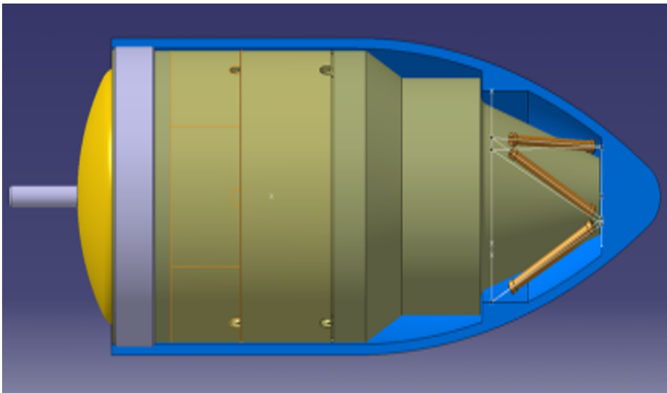
Fig12.2 Preliminary penetrator design (~11kg, length 37cm from nose to the release stud, diameter 15 cm)
