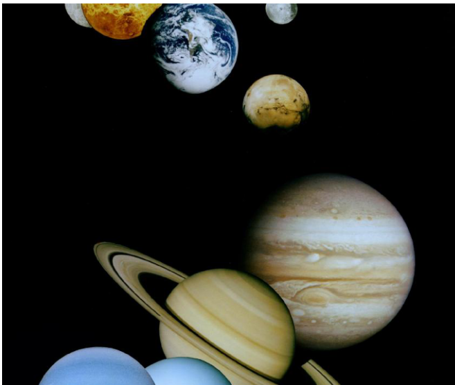
Fig. 1.9 The Earth as part of the Solar System in a combined photographic work retrieved by the Voyager missions in the period 1976-1989
