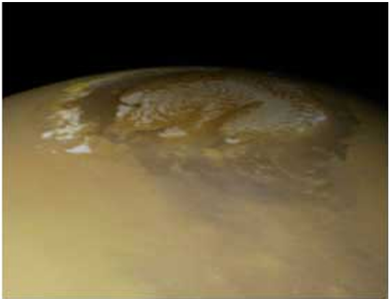
Fig. 7.5 The Martian northern polar cap
