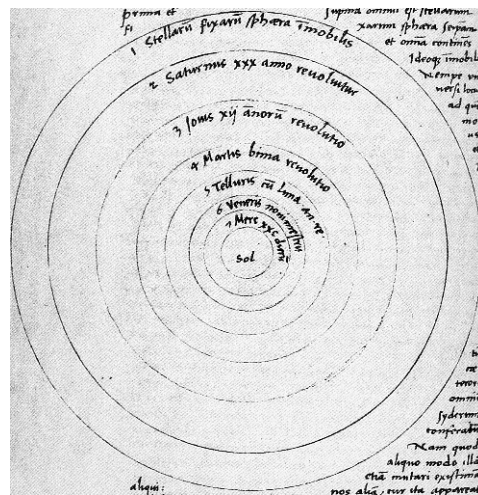
Fig. 1.1 The heliocentric view of the universe according to Copernicus, in which he included a sphere of fixed stars (Bertola, 1995). This last difficulty with the Copernican universe was discussed in the writings of Giordano Bruno.
