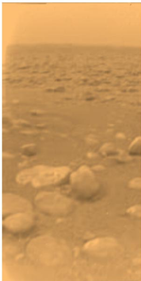
Fig. 9.6 First color view of Titan's surface
