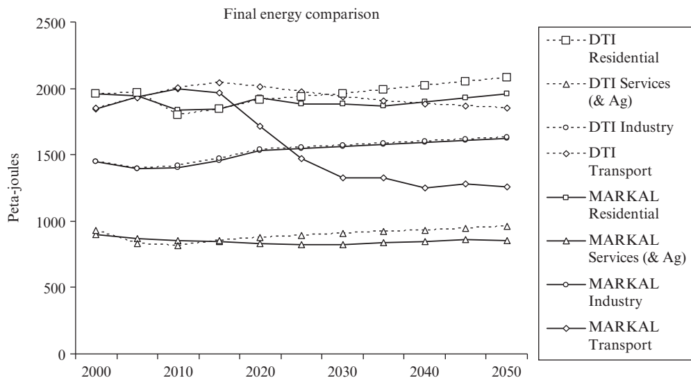
Figure 12.4 MARKAL–DTI model final energy convergence
