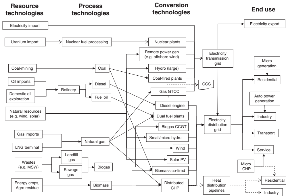
Figure 12.1 Highly aggregated example of a MARKAL reference energy system
