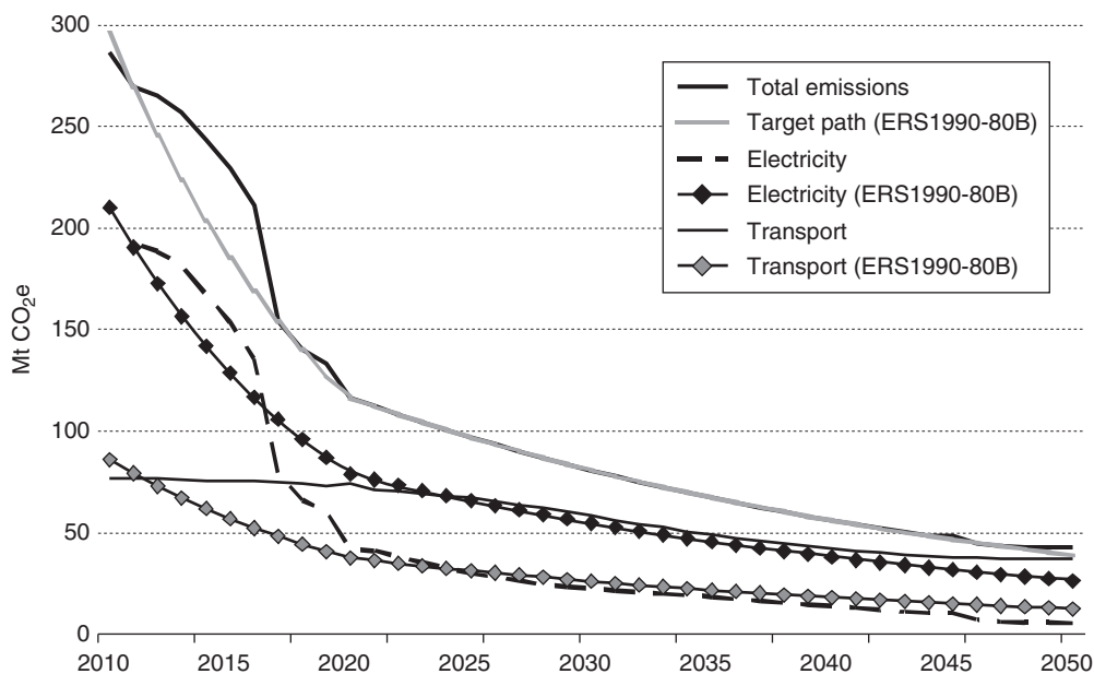
Figure 29.5 Estimated GHG emissions and target path ERS1990-80B
