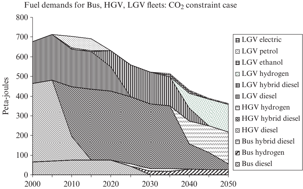
Figure 12.14 Technology transitions in bus, LGV and HGV transport modes
