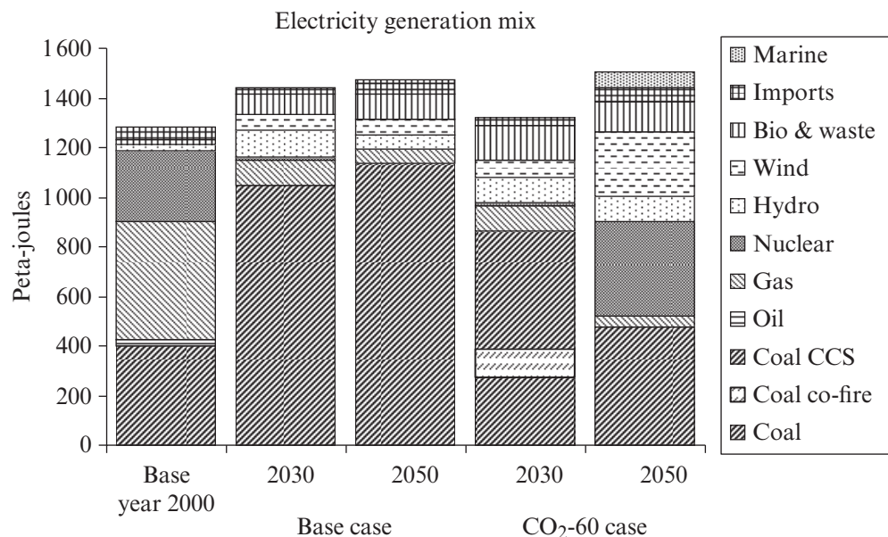
Figure 12.10 Electricity generation mix in base and CO 2 constraint cases
