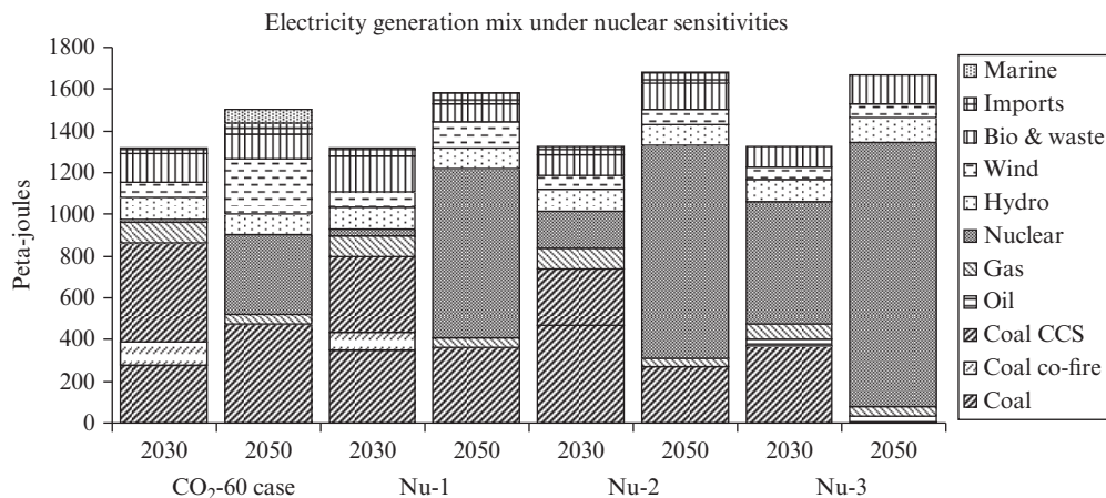
Figure 12.18 Electricity generation mix under nuclear chain improvements
