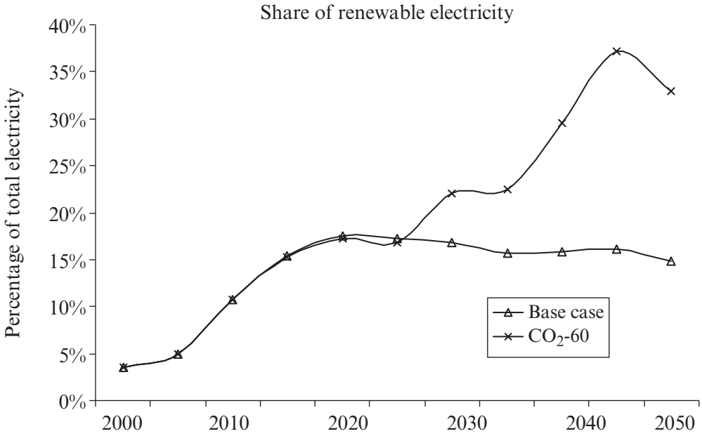
Figure 12.11 Share of renewable-based electricity generation
