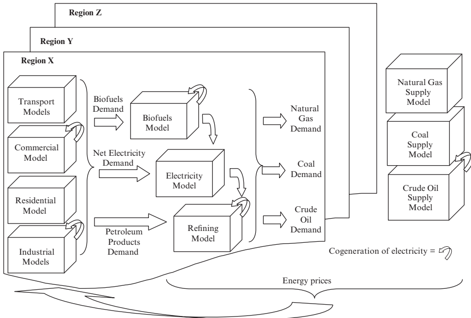
Figure 11.2 CIMS' energy supply and demand flow model
