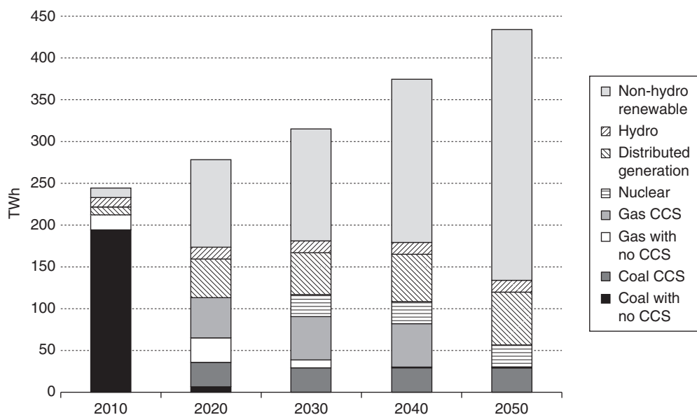
Figure 29.10 Electricity generation profile ERS1990-80B
