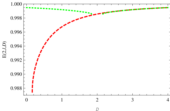
Fig. 14.5 The variation of energy E(2, 0, D) (green dotted line) on the dimension D is very similar to E(1, 0, D) . The energy E(2, 1, D) (red dashed line) increases with the increasing dimension D . Specially, it is found for D > 2 that the energy E(2, 1, D) almost overlaps E(2, 0, D)
