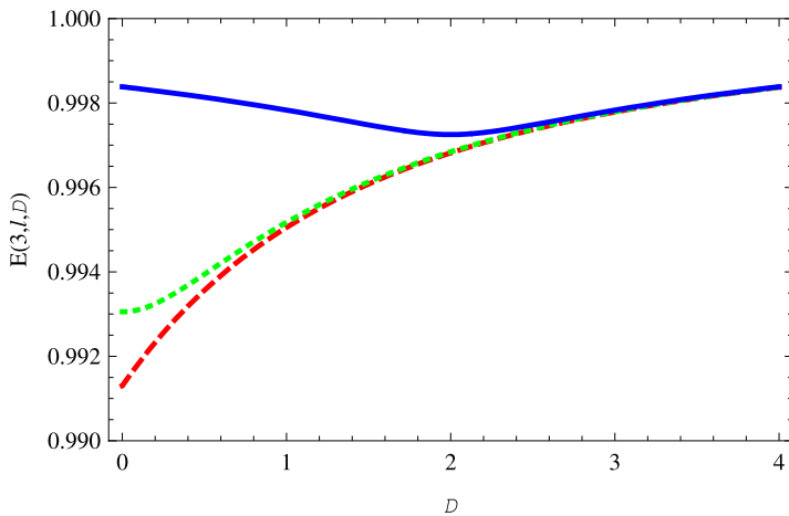
Fig. 14.15 The variations of the E(3, l, D) ( l = 2, 1, 0 ) on the dimension D are similar to E(2, l, D) ( l = 1, 0 ). The energy E(3, 2, D) (red dashed line) almost overlaps energy E(3, 1, D) (green dotted line). For D > 2.6 , the energies E(3, l, D) ( l = 2, 1, 0 ) are almost overlapped
