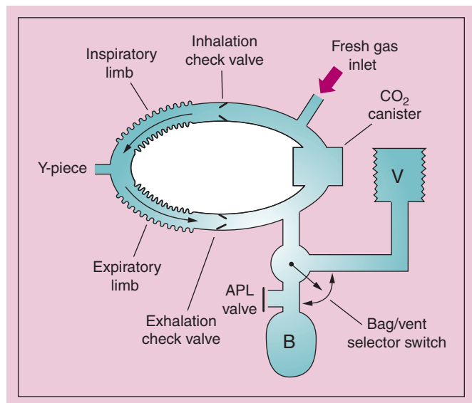
Figure 15-9 Schematic diagram of the components of a circle absorption anesthetic breathing system. Rotation of the bag/vent selector switch permits substitution of an anesthesia machine ventilator (V) for the reservoir bag (B). The volume of the reservoir bag is determined by the fresh gas inflow and adjustment of the adjustable pressure-limiting (APL) valve. (From Brockwell RC, Andrews JJ. Delivery systems for inhaled anesthetics. In Barash PG, Cullen BF, Stoelting RK [eds]. Clinical Anesthesia . Philadelphia, Lippincott Williams & Wilkins, 2006, pp 557-594, used with permission.)
