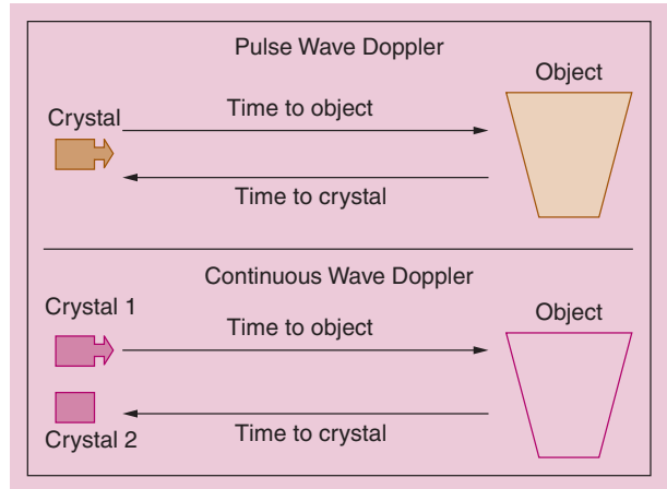
Figure 20-7 Timing differences between Doppler modalities.
