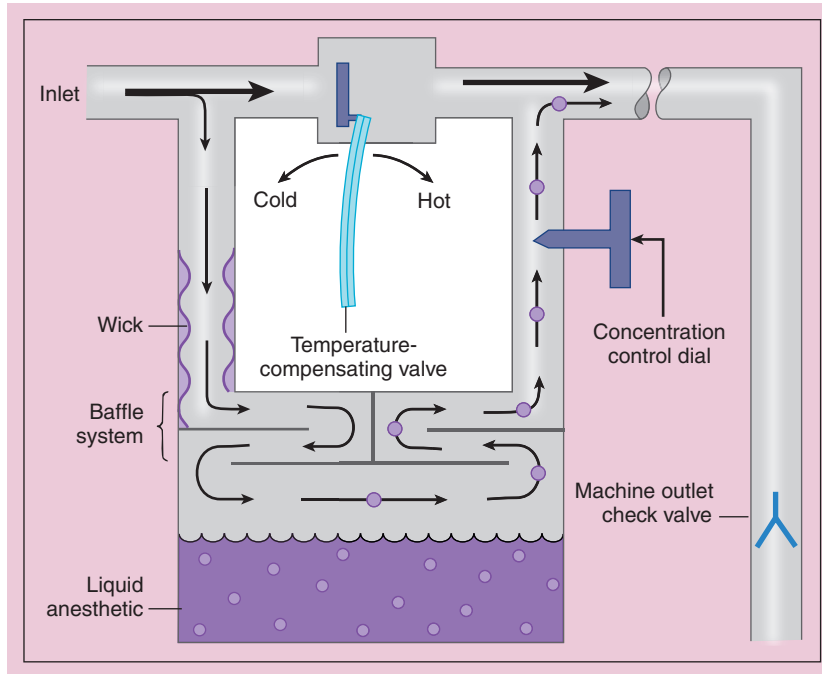
Figure 15-5 Simplified schematic of the Ohmeda Tec-type vaporizer. Rotation of the concentration control dial diverts a portion of the total fresh gas flow through the vaporizing chamber, where wicks saturated with liquid anesthetic ensure a large gas-liquid interface for efficient vaporization. A temperature-compensating valve diverts more or less fresh gas flow through the vaporizing chamber to offset the effects of changes in temperature on the vapor pressure of the liquid anesthetic (temperature-compensated vaporizer). Gases saturated with the vapor of the liquid anesthetic join gases that have passed through the bypass chamber for delivery to the machine outlet check valve. When the concentration control dial is in the off position, no fresh gas inflow enters the vaporizing chamber.
