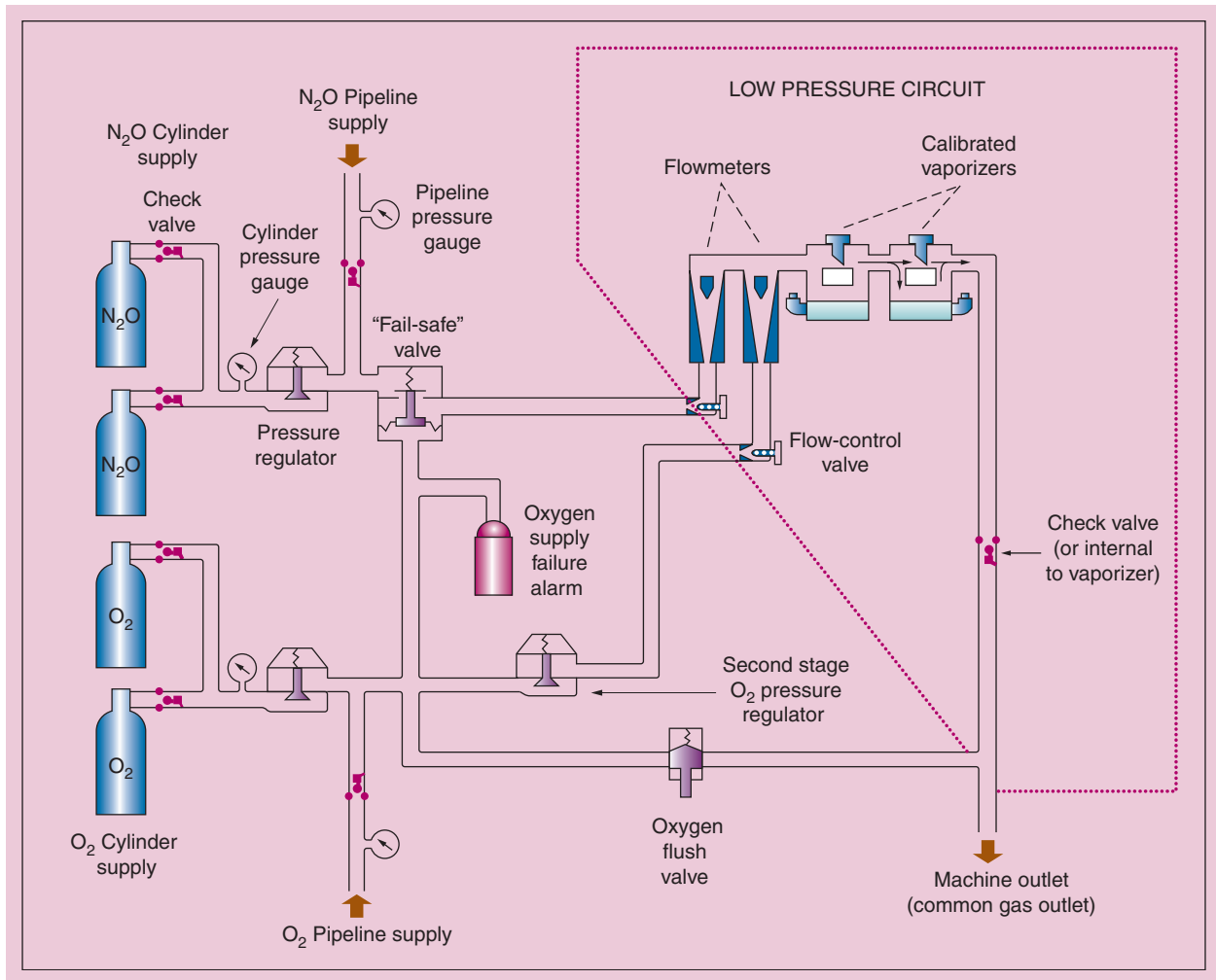
Figure 15-3 Schematic diagram of the internal circuitry of an anesthesia machine. Oxygen and nitrous oxide enter the anesthesia machine through a central supply line (most common); alternatively (infrequently), they are provided from gas cylinders attached to pin-indexed yokes on the machine. Check valves prevent transfilling of gas cylinders or flow of gas from cylinders into the central supply line. Pressure regulators decrease pressure in the tubing from the gas cylinders to about 50 psi. The fail-safe valve prevents flow of nitrous oxide if the pressure in the oxygen supply circuit decreases to less than 30 psi. Needle valves control gas flow to rotameters (flowmeters). Agent-specific vaporizers provide a reliable means to deliver preselected concentrations of a volatile anesthetic. An interlock system allows only one vaporizer to be in the “on” (delivery) setting at a time. After mixing in the manifold of the anesthesia machine, the total fresh gas flow enters the common outlet for delivery to the patient through the anesthetic breathing system (circuit). (Adapted from Check-Out. A Guide for Preoperative Inspection of an Anesthetic Machine. Park Ridge, IL, American Society of Anesthesiologists, 1987, pp 1-14, used with permission.)
