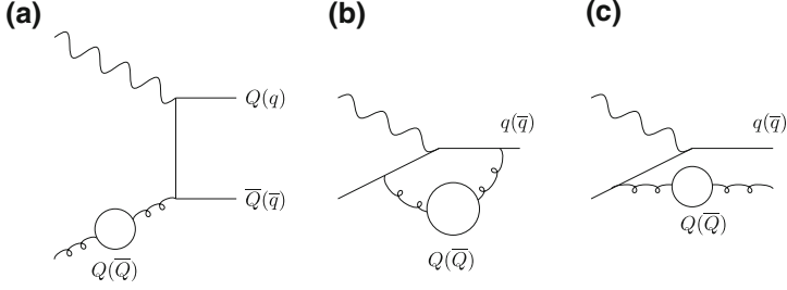
Fig. 5.1 O(a_s^2) virtual heavy quark corrections
