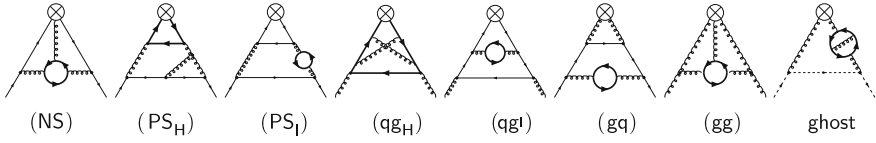
Fig. 7.1 Examples for 3-loop diagrams contributing to the massive operator matrix elements: NS non-singlet, PS H,l pure-singlet, singlet qg H,l , gq , gg and ghost contributions. Here the coupling of the gauge boson to a heavy or light fermion line is labeled by H and l , respectively. Thick lines heavy quarks, curly lines gluons, full lines quarks, dashed lines ghosts
