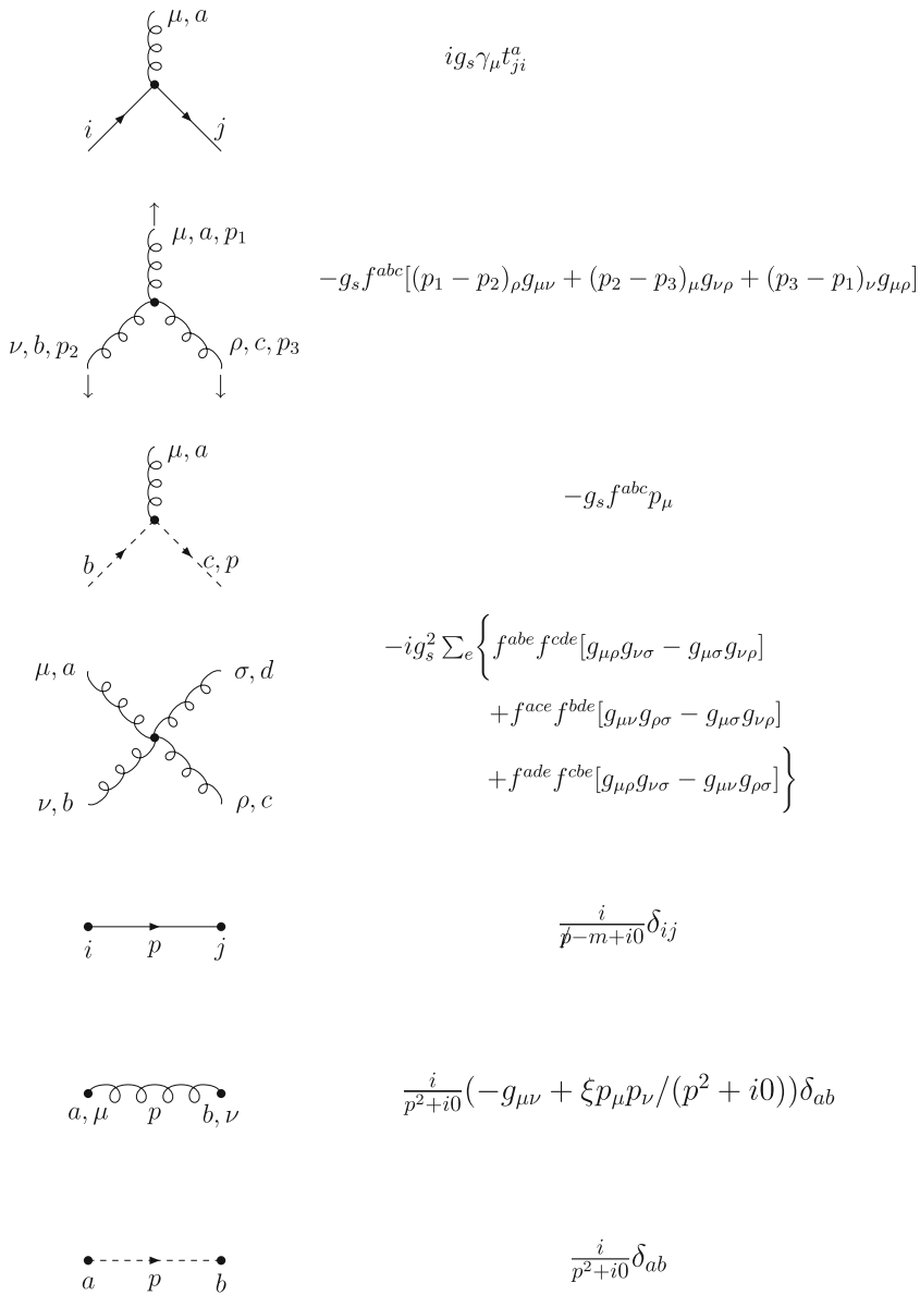
Fig. B.1 Feynman rules of QCD
