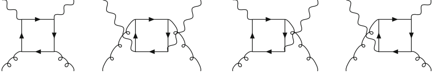
Fig. 7.2 Diagrams contributing to H_{g,(2,L)}^{(1)} via the optical theorem. Wavy lines photons; curly lines gluons; full lines quarks
