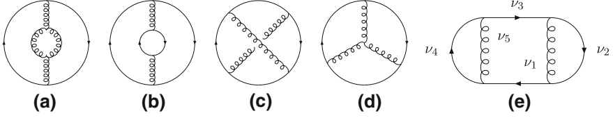
Fig. 10.1 Basic 3-loop topologies. Straight lines: quarks, curly lines: gluons. The gluon loop in a can also be replaced by a ghost loop; e 3-loop ladder graph
