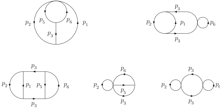
Fig. 7.7 Additional 3-loop topologies for MATAD
