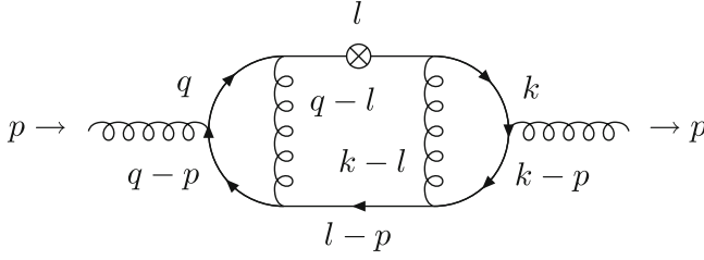
Fig. 10.2 Example 3-loop graph
