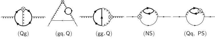
Fig. 6.1 Examples for 2-loop diagrams contributing to the massive OMEs. Thick lines heavy quarks, curly lines gluons, full lines quarks
