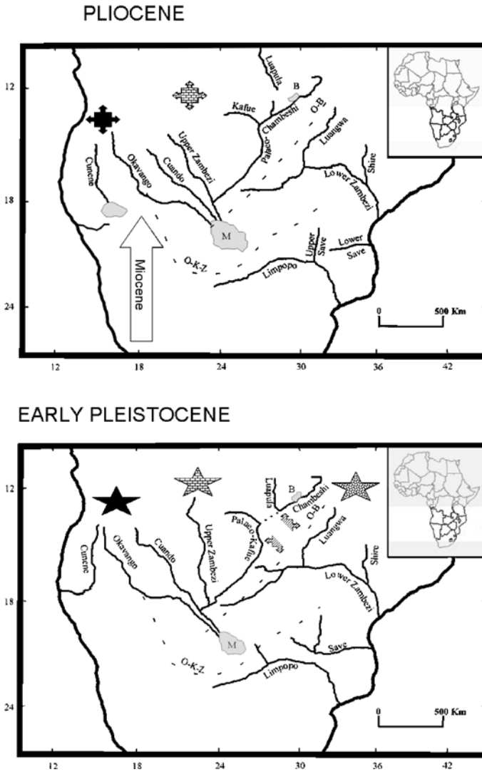
Fig. 27.5. Phylogeographic trends in Zambeesian Fukomyis estimated from Cyt b sequence differences using nonparametric rate smoothing and penalized likelihood methods as implemented in r8s (Sanderson 1997, 2002) (data adapted from Van Daele et al., accepted). The general distribution of the extant Fukomyis clades would have been determined in the Holocene, when the riversystem configuration became similar to today's situation. (Drainage system evolution in South-Central Africa. Figure modified after Du Toit (1933), Moore and Larkin (2001) and Cotterill (2003). M Paleo-lake Makgadikgadi; B Lake Bangweulu; OKZ Ovamboland – Kalahari – Zimbabwe axis of crustal flexuring and OB Okavango – Bangweulu axis of crustal flexuring)
