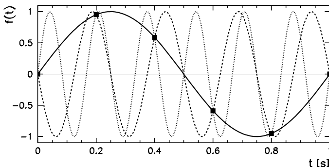
Fig. 4.4 A periodic signal \sin(2\pi\nu t) with the frequency \nu = 1\text{ s}^{-1} (full line) is sampled at \nu_s = 5\text{ s}^{-1} (squares): the critical frequency (4.6) is \nu_c = \omega_c/(2\pi) = 2.5\text{ s}^{-1} . We obtain exactly the same function values by sampling the functions \sin(2\pi(\nu - \nu_s)t) (dashed line) or \sin(2\pi(\nu + \nu_s)t) (dotted line). At this sampling rate, aliasing causes all three signals to be represented with the frequency \nu in the discrete Fourier spectrum
