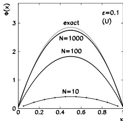
Fig. 8.8 Convergence of the scalar flux in the non-asymptotic difference scheme in upwind discretization with N = 10, 100 , and 1000 cells, to the exact solution. The values of the parameters are Q = 1 \text{ cm}^{-1}\text{s}^{-1} , \sigma_t = 10 \text{ cm}^{-1} , \sigma_a = 0.1 \text{ cm}^{-1} , and \varepsilon = 0.1 . For a precise solution we need an extremely fine mesh: for N = 1000 the cell length is equal to 1/100 of the mean free path
