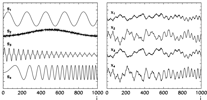
Fig. 6.21 [Left] The original signals (sources) from (6.41). [Right] The measured signals which are known mixtures of the sources (6.42)
