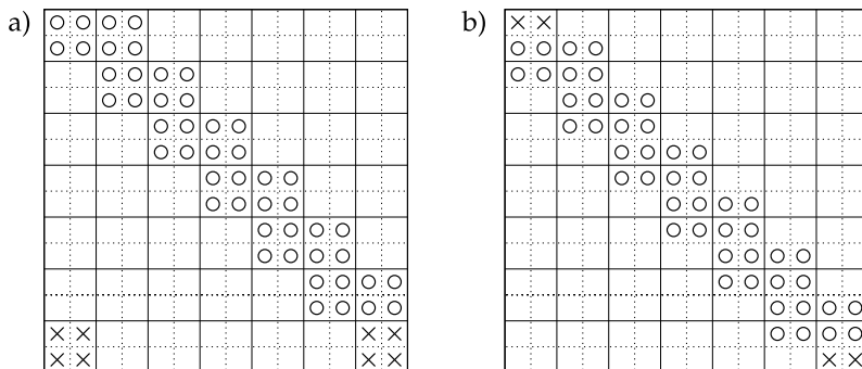
Fig. 8.2 The structure of the Jacobi matrix for systems of non-linear boundary-value problems for M = 2 , N = 6 . The symbols \circ denote the elements originating in the difference scheme, while the symbols \times denote the elements fixed by the boundary conditions. Matrices of the form (a) occur with unseparated boundary conditions \mathbf{g}(\mathbf{u}_0, \mathbf{u}_N) = \mathbf{0} . For improved numerical efficiency, one could attempt to separate the boundary conditions as \mathbf{g}_1(\mathbf{y}(a)) = \mathbf{0} and \mathbf{g}_2(\mathbf{y}(b)) = \mathbf{0} , leading to the banded structure (b)
