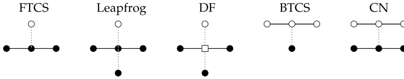
Fig. 9.6 Two-level (FTCS, BTCS, CN) and three-level (Leapfrog, DF) difference schemes for the diffusion equation v_t - Dv_{xx} = Q . (Compare to Fig. 9.2.) The properties of the depicted schemes are listed in Table 9.1. In the DF scheme the value of u at (j\Delta x, n\Delta t) does not appear ( empty square )
