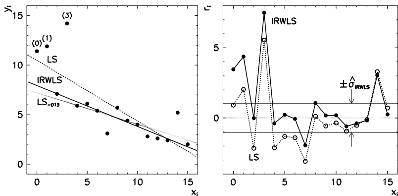
Fig. 5.13 Robust linear regression. (Example adapted from [17].) [Left] The regression straight line by the method of least squares (LS), by omitting three outliers (LS -013 ), and by the iterative reweighting method (IRWLS). [Right] The residuals r_i and the estimate of dispersion by the IRWLS method
