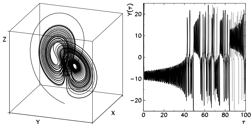
Fig. 7.21 The Lorenz problem. [Left] The solution on the time interval [0, 50] in the phase space of variables X , Y , and Z . [Right] Dependence of the solution Y(\tau) on the initial conditions. Shown are two solutions with the initial condition Y(0) = 1 (dotted curve) and with Y(0) = 1 + 10^{-12} (full curve)
