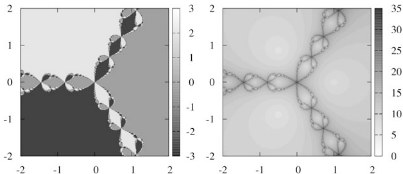
Fig. 2.3 Newton's method used to solve z^3 - 1 = 0 in the complex plane. [Left] The phase of the final value z as a function of the initial approximation given by the values \operatorname{Re} z in \operatorname{Im} z on the abscissa and the ordinate. The three shaded areas are the basins of attraction corresponding to the phases 0 , 2\pi/3 \approx 2.094395 , and -2\pi/3 \approx -2.094395 to which the individual initial approximation is “attracted” [8]. [Right] The number of iterations needed to achieve convergence, as a function of the initial approximation
