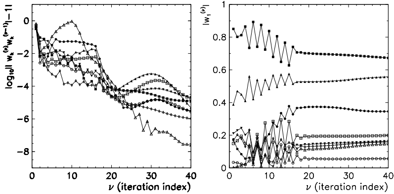
Fig. 6.17 Typical convergence in the FastICA algorithm applied to the relatively complex signals from Fig. 6.16. [Left] The difference of the scalar product |\mathbf{w}_k^{(v)\top} \mathbf{w}_k^{(v-1)}| from 1 in subsequent iterations ( \nu ) in the case of eight independent components ( k = 1, 2, \dots, 8 ). [Right] The convergence of eight components of the vector \mathbf{w}_1 in consecutive iterations ( \nu )
