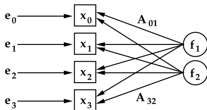
Fig. 5.27 A schematic representation of factor analysis. We construct a linear combination of a small number of factors (two in this example, f_1 and f_2 ) and remainders e_i in order to represent a larger body of data x_i . The weights are stored in the matrix A such that for each data entry we have \mathbf{x}^T = A\mathbf{f}^T + \mathbf{e}^T , where \mathbf{x} , \mathbf{f} , and \mathbf{e} are the corresponding rows of the matrices X , F , and E
