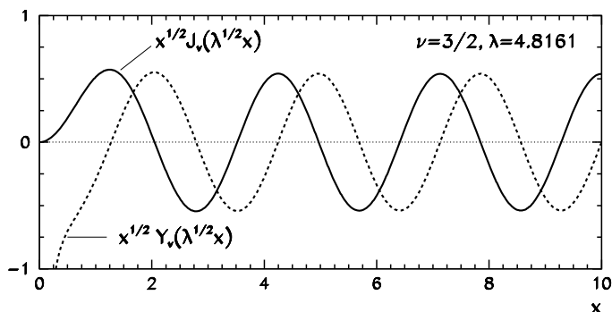
Fig. 8.12 Bessel's equation in Liouville form -y''(x) + (v^2 - 1/4)x^{-2}y(x) = \lambda y(x) for x \in (0, \infty) has two linearly independent solutions: \sqrt{x}J_\nu(\sqrt{\lambda}x) , regular everywhere, and \sqrt{x}Y_\nu(\sqrt{\lambda}x) , which has a singularity at the origin. The twofold character of the solutions is of key significance in the description of physical phenomena involving these functions. Shown are the solutions with \nu = 1.5 and the eigenvalue \lambda = 4.8161 that is determined by the boundary conditions. The zeros of one eigenfunction interlace with the zeros of the other. See also Fig. 1.13
