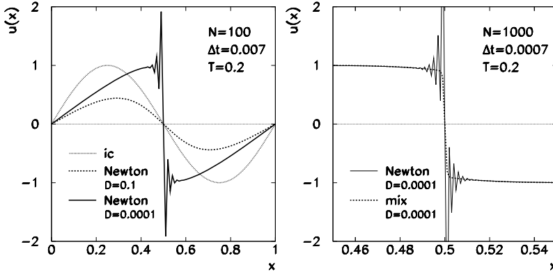
Fig. 9.12 Solutions of the Burgers equation. [Left] Initial condition (ic) and the solution by Newton's method with D=0.1 and D=0.0001 on a mesh with 100 subintervals. At small D a discontinuity forms that the scheme is unable to resolve. [Right] Solution by Newton's method and the mixed scheme (9.87) with D=0.0001 by using a 10-times finer mesh and 10-times shorter time step (zoom-in on the discontinuity)
