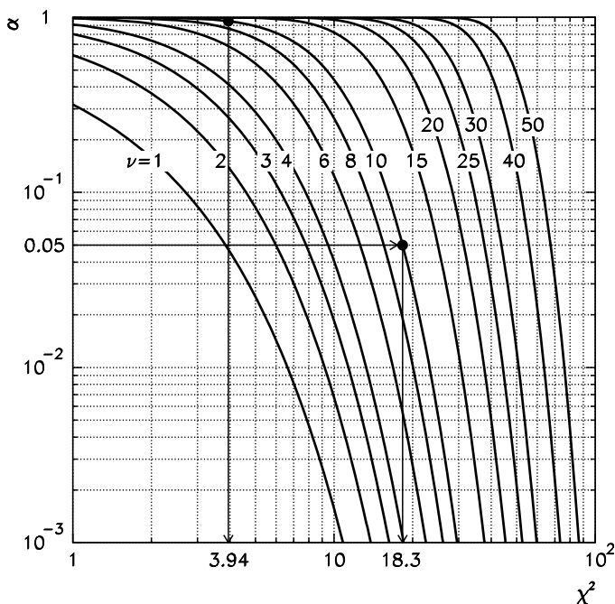
Fig. 5.6 The solution of P(\chi^2 > \chi^2_+)=\alpha and P(\chi^2 < \chi^2_-)=\alpha . The symbols \bullet denote the points (\chi^2_-, 1-\alpha) = (3.94, 0.95) and (\chi^2_+, \alpha) = (18.3, 0.05) from Example (5.28)
