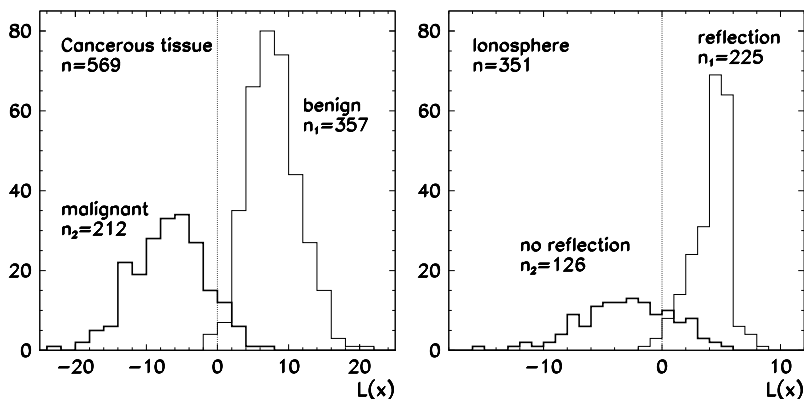
Fig. 5.26 Distribution of the measurements with respect to the linear discriminant function L(\mathbf{x}) . [Left] Cancerous tissue (misclassification rate 4.2 %). [Right] Reflections of radar signals in the ionosphere (Problem 5.12.3; misclassification rate 13.7 %)
