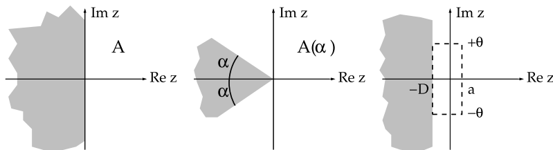
Fig. 7.8 Definitions of linear stability regions (scalar problem y' = \lambda y ) for implicit methods, where z = h\lambda . [Left] A-stability for single-step methods. [Center] A(\alpha) -stability for single-step methods. [Right] “Stiff stability” for multi-step methods
