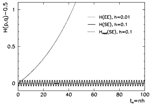
Fig. 7.14 Time evolution of the Hamiltonian for the linear harmonic oscillator with k = 1.6 . Shown is the energy (7.41) for the explicit Euler method (EE) with step h = 0.01 and the energies (7.41) and (7.55) for the symplectic Euler method (SE) with step h = 0.1 . This method exactly preserves the invariant (7.55)
