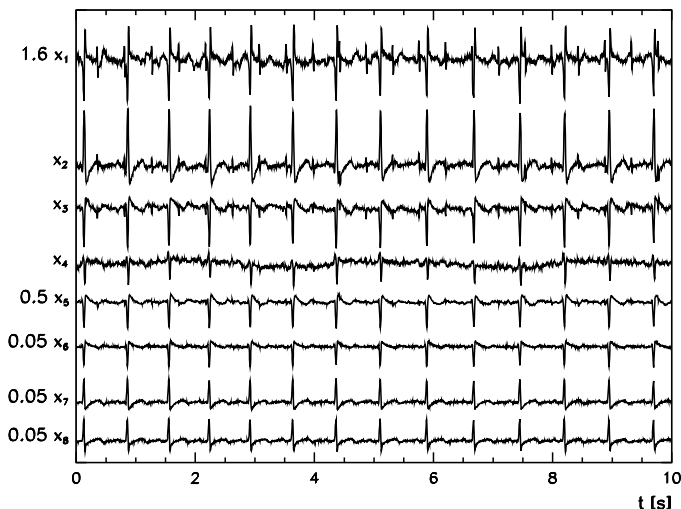
Fig. 6.16 Electro-cardiogram of a pregnant woman. The relatively weak and noisy signal of the child's heartbeat, visible in signals x_1 , x_2 , and x_3 , mixes with the signal of the mother's heartbeat (Example adapted from [56] based on data from [57])
