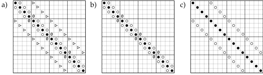
Fig. 10.2 Common structures of matrices appearing in explicit ( \mathbf{u}^{n+1} = F\mathbf{u}^n ) and implicit schemes ( F_1\mathbf{u}^{n+1} = F\mathbf{u}^n ) for the solution of two-dimensional diffusion equation. The values of the elements denoted by \bullet / \circ / \triangleright depend on the difference method (see text). Shown are matrices for the case N_x = N_y = 5
