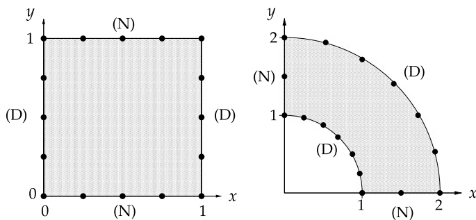
Fig. 10.18 [Left] Square geometry for the solution of the planar Laplace equation. The letters at the boundaries denote the type of the boundary condition: (D) Dirichlet, (N) Neumann. [Right] The geometry of a section of an annulus
