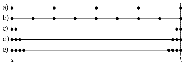
Fig. E.3 The points used to interpolate f in the Filon's method. (a) Equidistant mesh with 5 points. (b) Mesh with 9 points. (c) Inversely spaced mesh \{a, a + 1/\omega, b - 1/\omega, b\} . (d) Inverse mesh \{a, a + 1/\omega, a + 2/\omega, b - 2/\omega, b - 1/\omega, b\} . (e) Inverse mesh \{a, a + 1/\omega, a + 2/\omega, a + 3/\omega, b - 3/\omega, b - 2/\omega, b - 1/\omega, b\} . See also Fig. E.4
