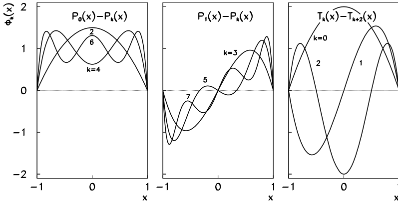
Fig. 11.4 [Left, Center] The basis functions (11.35) for the Legendre–Galerkin method with k \in \{2, 4, 6\} and k \in \{3, 5, 7\} . [Right] The basis functions (11.40) for the Chebyshev–Galerkin methods with k \in \{0, 1, 2\}
