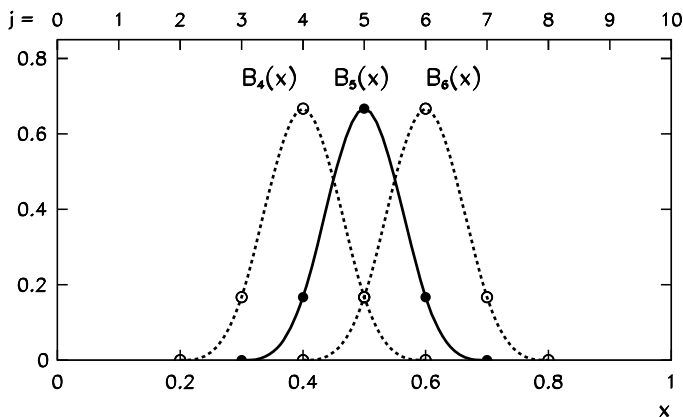
Fig. 8.9 The cubic spline B_5 and its nearest neighbors B_4 and B_6 on a uniform mesh x \in [0, 1] with (N + 1) = 11 points (including the boundaries)
