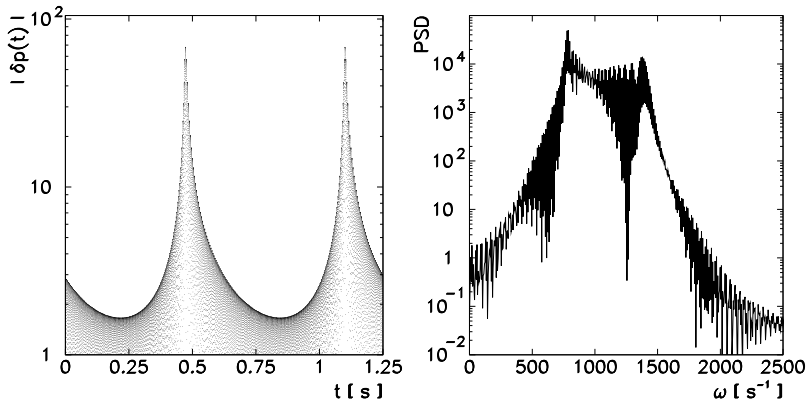
Fig. 4.21 [Left] An example of the signal at v = 100 m/s, R = 10 m, L = 10.5 m, \omega = 1000 /s, and c = 340 m/s. [Right] The Fourier power spectral density. The peaks in the spectrum occur approximately at \omega/(1 + v/c) = 773 Hz and \omega/(1 - v/c) = 1417 Hz
