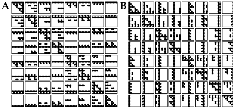
Fig. 3.1 Strassen's multiplication of 8 \times 8 matrices. The diagrams show the elements of A and B which are accessed in memory in order to form the elements of C . For example, to get the C_{18} element ( upper right corners ) we need A_{1k} ( 1 \leq k \leq 8 ) and B_{k8} ( 1 \leq k \leq 8 ) as in classical multiplication (3.1), but a different pattern for other elements
