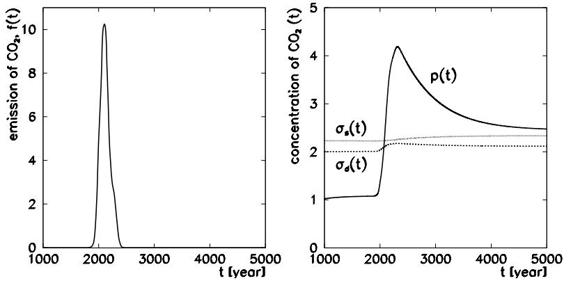
Fig. 7.17 [Left] The function f describing the emissions of CO 2 into the atmosphere from year 1000 to 5000. [Right] Concentrations of CO 2 in the atmosphere ( p ), shallow ( \sigma_s ), and deep ocean ( \sigma_d ) as functions of time (solution by the adaptive RK4 method)
