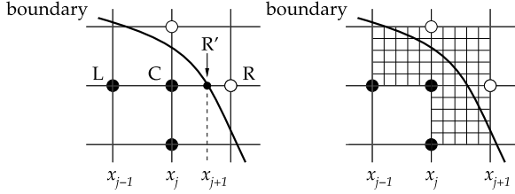
Fig. 10.6 [Left] Computing the approximations of u_x and u_{xx} in the vicinity of the domain boundary by bypassing the mesh points. In the first order of the mesh spacings we use (10.51) and (10.52). [Right] Making the discrete mesh denser
