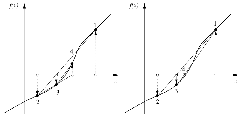
Fig. 2.4 Finding the approximations of the zeros of f by using the methods from the family defined by (2.9). [Left] Secant method. [Right] Method of false position
