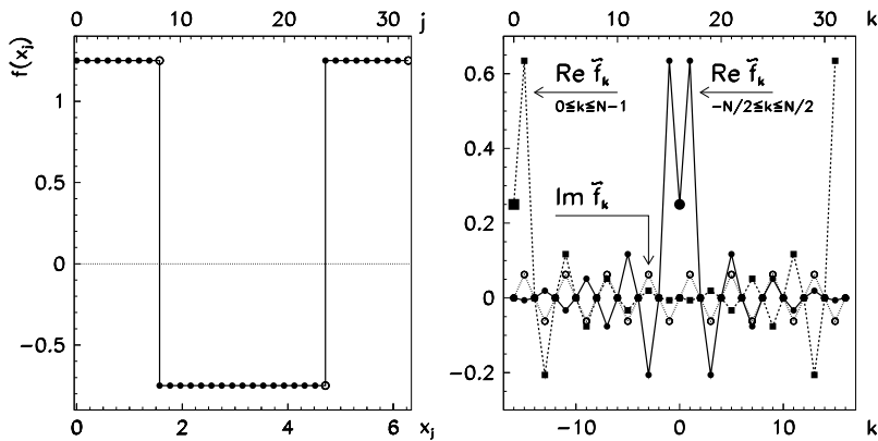
Fig. 4.1 Discrete Fourier transformation. [Left] The sum of the constant 0.25 and the square wave on [0, 2\pi] is sampled at N = 32 points x_j = 2\pi j/N , 0 \leq j \leq N - 1 (the \bullet symbols). At the points \circ the function is not sampled! [Right] The real and imaginary parts of the Fourier coefficients for two different ways of indexing ( -N/2 \leq k \leq N/2 or 0 \leq k \leq N - 1 ). The thick symbols at k = 0 denote the zero-frequency component, which is the average of the signal—precisely the 0.25 vertical shift on the left figure (If we subtract the average of the signal, the zeroth component of its transform is zero)
