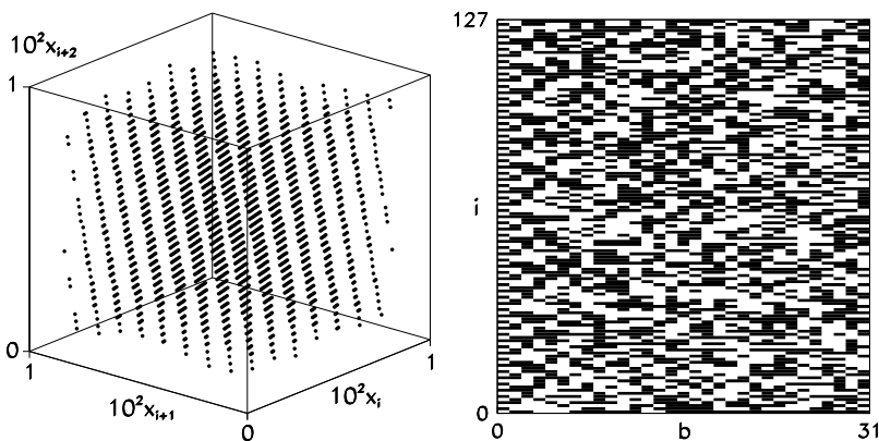
Fig. C.4 [Left] Zoom-in of the phase space [0, 1]^3 of the points 2^{-31}(x_i, x_{i+1}, x_{i+2}) picked from the sequence \{x_i\} generated by the standard 32-bit glbC generator with x_0 = 12345 . [Right] The bits b of numbers x_i (black = 1, white = 0)
