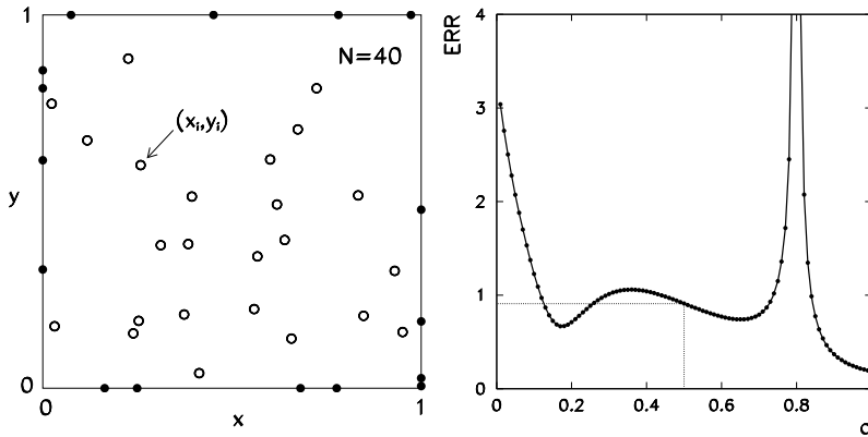
Fig. 10.15 Solving the Poisson equation on the square by using a mesh-free method based on radial basis functions. [Left] A random distribution of 16 points on the boundaries of the square (symbols \bullet ) and 24 points in its interior (symbols \circ ). [Right] The error of the solution in dependence of the parameter c
