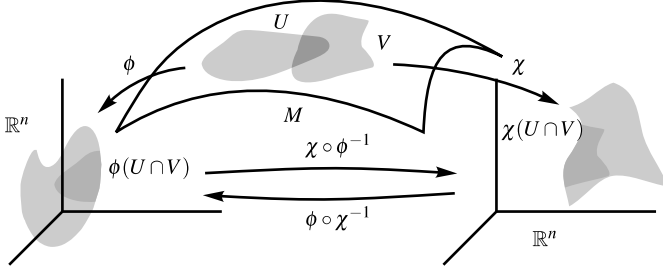
Fig. 1.2 Two coordinate systems whose domains have a nonempty intersection. A point p belonging to U \cap V corresponds to two points of \mathbb{R}^n , \phi(p) and \chi(p) ; the charts (U, \phi) and (V, \chi) are C^k -related if the maps \phi(p) \mapsto \chi(p) and \chi(p) \mapsto \phi(p) are differentiable functions of class C^k
