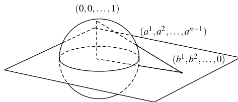
Fig. 1.3 The stereographic projection establishes a one-to-one correspondence between the points of the n -sphere, excluding the “north pole” (0, 0, \dots, 1) , and the points of the plane x^{n+1} = 0 . The point (a^1, a^2, \dots, a^{n+1}) is a point of the n -sphere different from (0, 0, \dots, 1)
