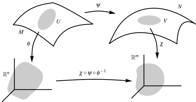
Fig. 1.5 The map \psi : M \rightarrow N is locally represented by the map \chi \circ \psi \circ \phi^{-1} . \psi is differentiable if the compositions \chi \circ \psi \circ \phi^{-1} are differentiable for any pair of charts (U, \phi) on M and (V, \chi) on N
