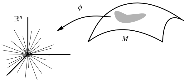
Fig. 3.1 The images in \mathbb{R}^n of the orbits of the group (3.42) under \phi are radial segments
