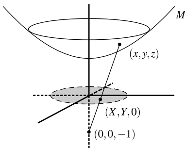
Fig. 6.1 Stereographic projection. The points (x, y, z) \in M , (X, Y, 0) and (0, 0, -1) lie on the same straight line
