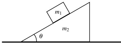
Fig. 4.1 The block remains in contact with the wedge, which lies on a horizontal table
