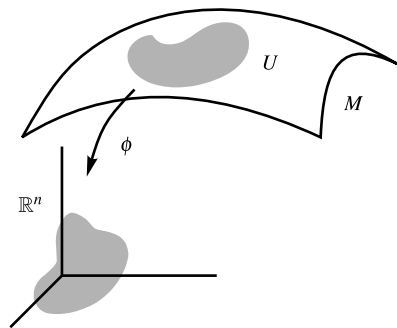
Fig. 1.1 A coordinate system in a set M ; with the aid of \phi , each point of U corresponds to some point of \mathbb{R}^n . The image of U under \phi must be an open subset of some \mathbb{R}^n
