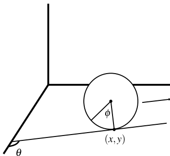
Fig. 4.2 The disk rolls without slipping on a horizontal plane. \theta is the angle between the velocity of the disk and the positive x axis
