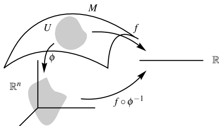
Fig. 1.4 With the aid of a coordinate system on M , a real-valued function f defined on M is represented by the function f \circ \phi^{-1} : \mathbb{R}^n \rightarrow \mathbb{R}
