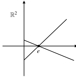
Fig. 7.2 The matrix group considered in Example 7.40 is identified with the Cartesian plane with the vertical axis removed. The point (1, 0) corresponds to the identity and the one-parameter subgroups correspond to the intersections of the straight lines passing through (1, 0) with the half-plane x^1 > 0
