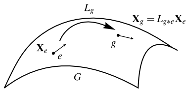
Fig. 7.1 A left-invariant vector field on G
