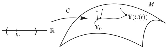
Fig. 5.1 The tangent vector \mathbf{Y}_0 is transported along the curve C
