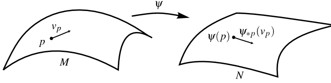
Fig. 1.8 If \psi : M \rightarrow N is a differentiable mapping from M into N , its Jacobian, or differential, maps tangent vectors to M into tangent vectors to N
