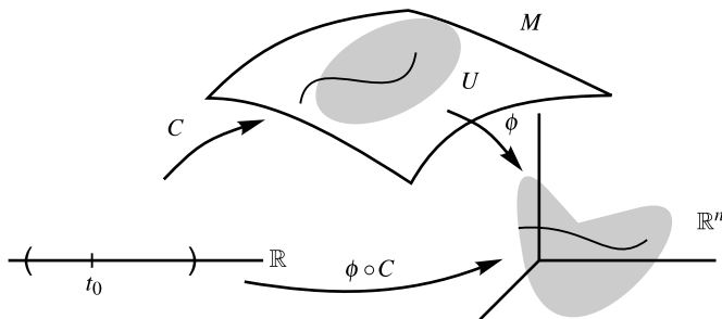
Fig. 1.6 A curve in M and its image in a coordinate system. C is differentiable if \phi \circ C is differentiable for any chart (U, \phi) on M
