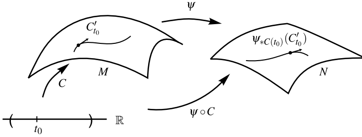
Fig. 1.9 The tangent vectors of the curve \psi \circ C are obtained applying the Jacobian of \psi to the tangent vectors of C
