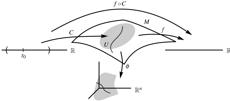
Fig. 1.7 Composition of a curve in M with a real-valued function f . The derivative of f \circ C , which is a function from \mathbb{R} into \mathbb{R} , represents the directional derivative of f along C
