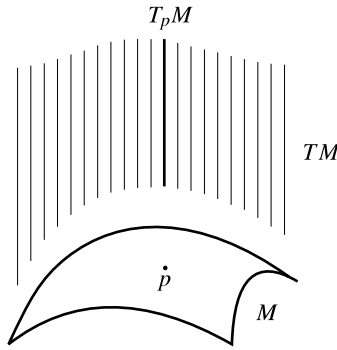
Fig. 1.10 The tangent bundle of M is formed by the union of the tangent spaces to M at all the points of M . Each tangent space to M is represented here by a vertical line
