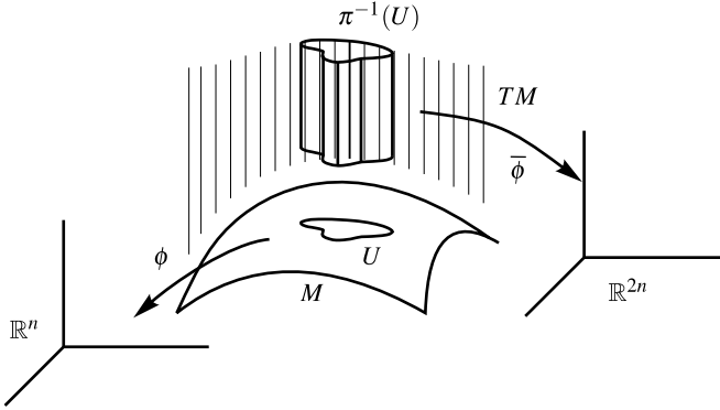
Fig. 1.11 Each coordinate system on M , (U, \phi) , induces a coordinate system on TM , (\pi^{-1}(U), \bar{\phi})
