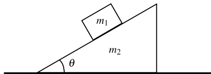
Fig. 8.1 The block can slide on the wedge-shaped block, which lies on a horizontal surface
