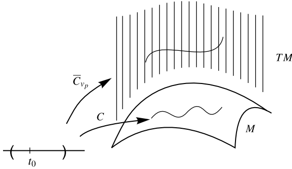
Fig. 5.2 The image of \bar{C}_{v_p} is formed by the tangent vectors obtained by parallel transport of v_p along C
