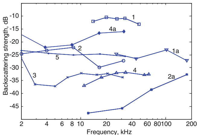
Fig. 6.2 Frequency dependence of the backscattering strength for various types of bottom sediments (1) stony bottom, \chi = 30^\circ (Urlick 1954); (1a) the same, \chi = 10^\circ (McKinney and Anderson 1964); (2) sand \chi = 70^\circ (Buntchuk and Zhitkovskii 1980), (2a) the same, \chi = 10^\circ (McKinney and Anderson 1964); (3) siltstones, \chi = 10^\circ (Volovov and Zhitkovskii 1977); (4) silt, \chi = 30^\circ (Urlick 1954); (4a) the same, \chi = 70^\circ (Buntchuk and Zhitkovskii 1980); and (5) the data averaged over regions with different bottom types, \chi = 40^\circ (Buntchuk and Zhitkovskii 1980)
