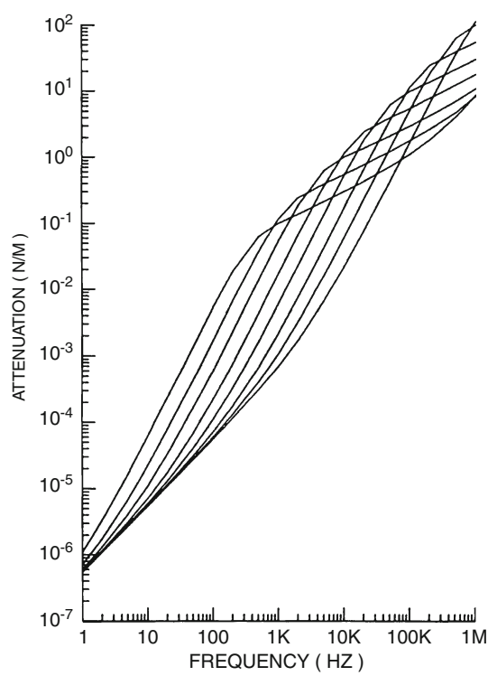
Fig. 2.27 Biot–Stoll model attenuation dispersion curve
