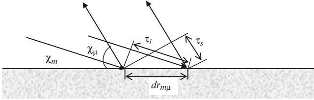
Fig. 6.5 Configuration for mode-forming beam scattering
