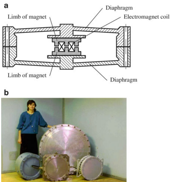
Fig. 10.1 Sound sources with an electromagnetic transducer and with a radiating diaphragm (a) schematic sketch, (b) appearance
