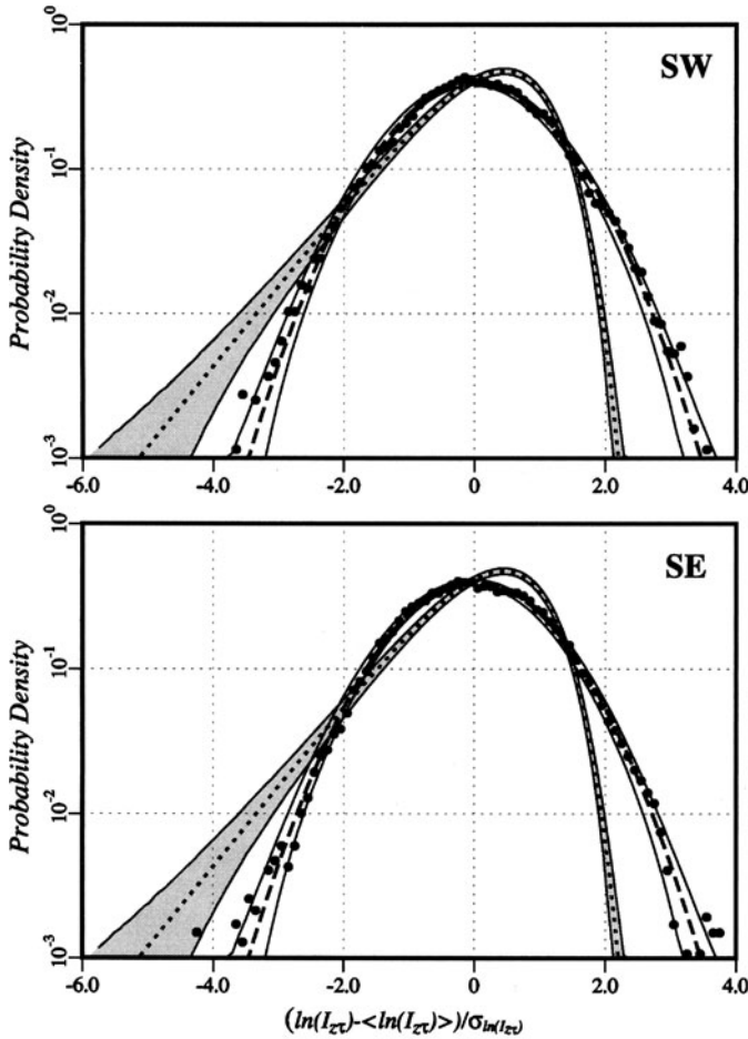
Fig. 5.14 Probability density functions of the high frequency component of the integrated intensity for the southwest and southeast transmission paths ( asterisk ) in the PRIMER experiment and the theoretical log-normal and exponential distributions ( gray in-filling ). Sampling error confidence intervals (95%) on the theoretical distributions ( dash ) are bound by solid lines
