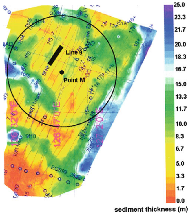
Fig. 2.23 Layer two sediment layer thickness (m) at the ASIAEX East China Sea experimental site, inferred from a survey made by L. Bartek. Miller et al. 2004 (with permission from IEEE)
