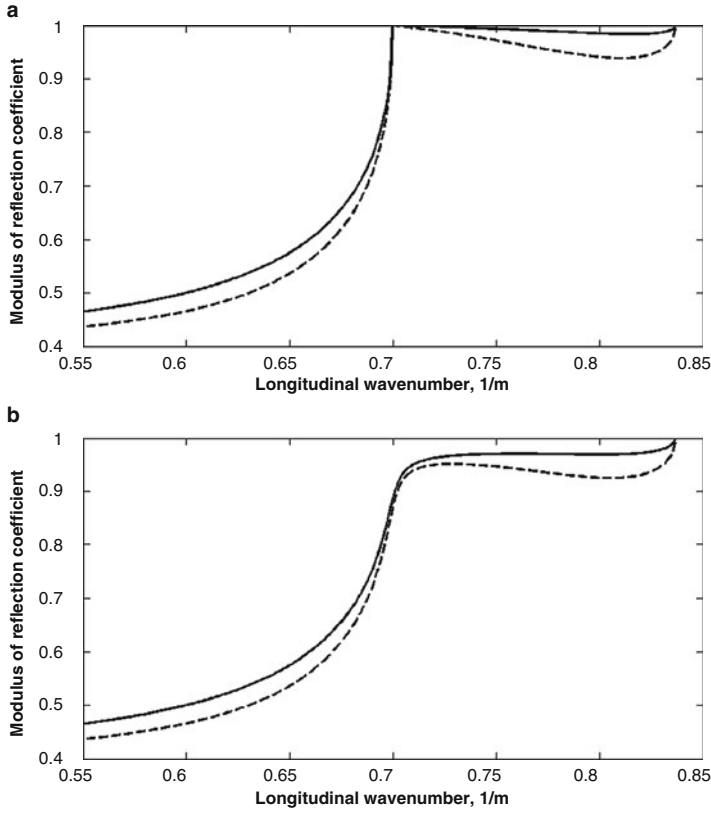
Fig. 4.7 Modulus of reflection coefficient for model with parameters m_1 = 2 , c = 1,500 m/s, c_I = 1,800 m/s, frequency 200 Hz, speed of shear waves c_s = 300 m/s ( continuous line ) and 400 m/s ( dashed line ), (a) attenuation coefficient of longitudinal waves \alpha = 0 , (b) \alpha = 0.01
