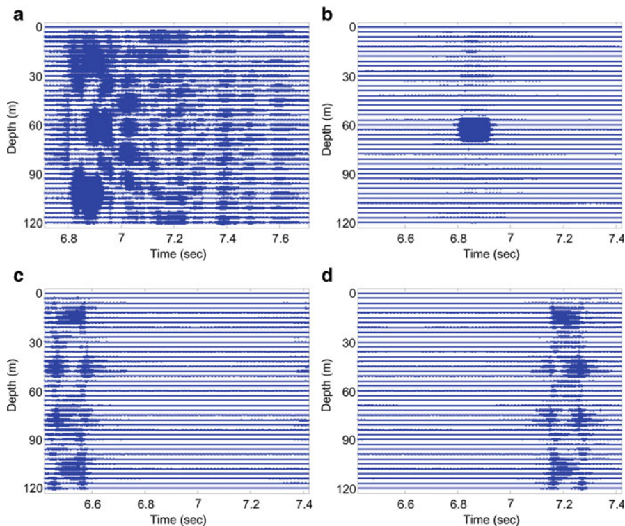
Fig. 8.23 Simulation of sound pulse focusing at the distance 10 km. (a) The pulse data received on the SRA for PS at depth 60 m. (b,c,d) The data received from the time reversed transmission of pulse shown in (a). (b) The data received at various depths in focal planes; the data received at various depth in the plane lying at distances of 1 km closer (c) and farther (d) than the focusing plane arranged at 10 km from the array. Time is measured from the point in time at which sound pulse is radiated by probe source (a) and SRA (b,c,d)
