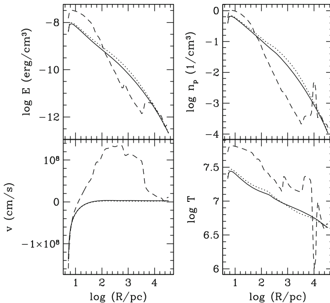
Fig. 4.7 Time evolution during the third burst of model B3 02 (see Fig. 4.5). Solid, dotted, and dashed lines refer to 6, 6.5, and 7 Gyr. The final, global degassing event is apparent, with positive velocities > 10^3 \text{ km s}^{-1} over the galaxy body. (Adapted from Ciotti and Ostriker 2007 by permission of the AAS)
