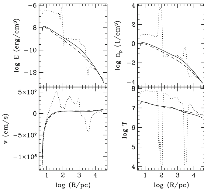
Fig. 4.6 Three snapshots of the radial distribution of internal energy per unit volume, number density, velocity, and temperature, of model B3 02 starting at (2.554 Gyr, just before the first burst), separated by 500 Myr (in order, solid , dotted and dashed lines). After ( solid ) and before ( dashed ) the central burst the profiles are almost unperturbed, while during the burst ( dotted ) we can observe two cold and high density shells, with the inner shell moving outward, while the external cold shell is falling to the center. (Adapted from Ciotti and Ostriker 2007 by permission of the AAS)
