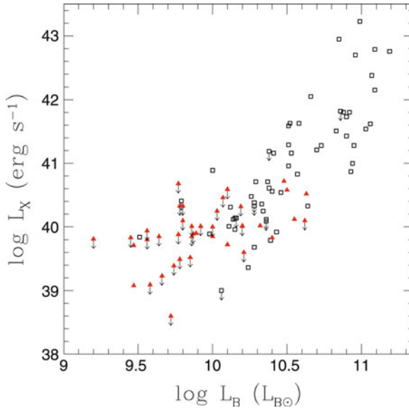
Fig. 2.17 The total X-ray emission versus the galactic luminosity L_B (from O’Sullivan et al. 2001), for ETGs with inner stellar profile classified of the cusp (red triangles) or core (squares) type by Lauer et al. (2007); downward arrows represent upper limits. Updated from Fig. 1 of Pellegrini (2005b), see the electronic version for a color version of this figure
