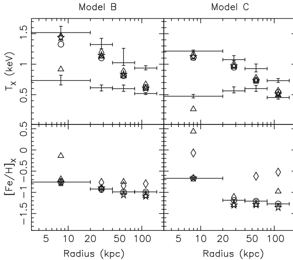
Fig. 6.16 Predicted temperature and metallicity gradients from Kawata and Gibson (2003). Different symbols correspond to the values derived by the different methods, such as spectrum fitting ( circles ), X-ray luminosity (0.5–4 keV) weighted mean values ( diamonds ), \rho^2 T^{1/2} weighted mean values for the gas with T > 12000 K ( triangles ), and \rho^2 T^{1/2} weighted mean values for the gas with T > 10^6 K ( stars )
