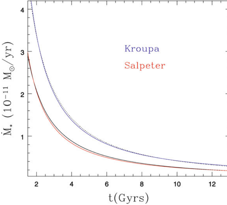
Fig. 2.1 Evolution of the stellar mass loss rate \dot{M}_*(t) according to the models in Maraston (2005) , for a Salpeter IMF ( solid line with best fit of (2.1) in red ) and for a Kroupa IMF ( dotted line with best fit of (2.1) in blue ). Solar abundance is assumed, and a total stellar mass of 1 M_{\odot} at an age of 12 Gyrs; see the electronic version for a color version of this figure
