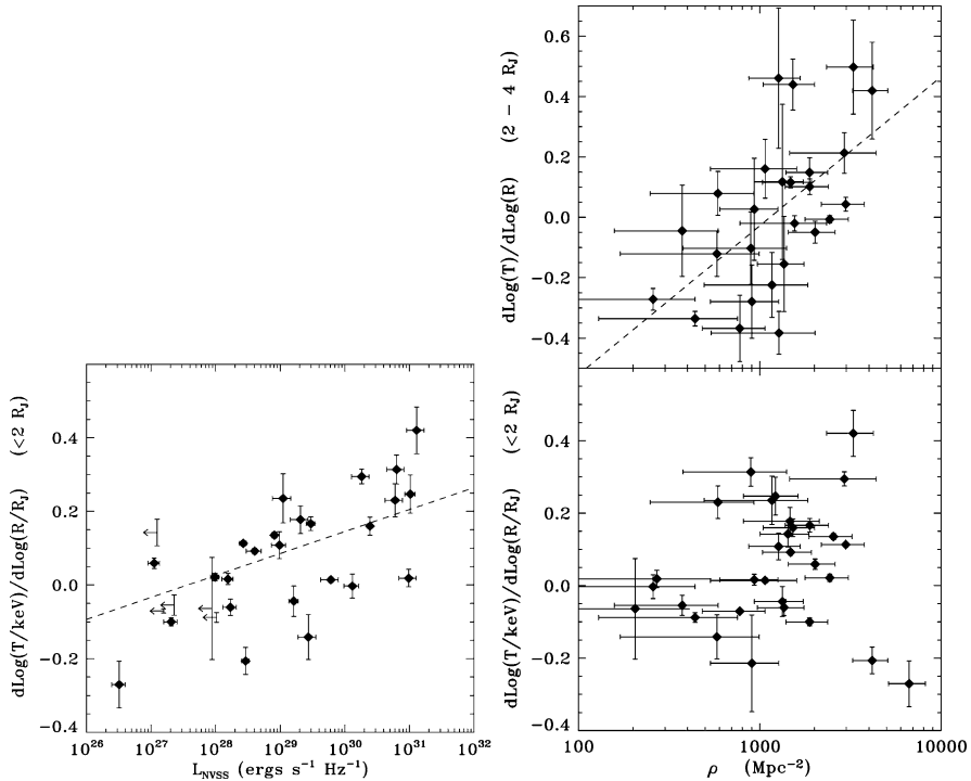
Fig. 7.6 Left: Inner gas temperature gradient \alpha_{02} plotted against 1.4 GHz radio luminosity obtained from the NVSS survey. Dashed line indicates the best-fit mean relation. (The slope may appear not to match the plotted points because upper limits are included in the fit.) Right, top: Outer temperature gradient \alpha_{24} plotted against the surface density of neighboring galaxies obtained from the 2MASS catalog. Dashed line indicates the best-fit mean trend. Right, bottom: Outer gradient plotted against 1.4 GHz luminosity; there is no significant correlation. (Figures reproduced from Diehl and Statler (2008a) )
