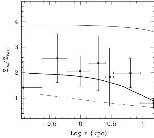
Fig. 6.15 Metallicity gradient in the stars ( dashed ) and gas ( solid ) as predicted by Brighenti et al. (2009)'s cooling flow model compared to data for NGC4649 (Humphrey et al. 2006). The lowest solid line is the fiducial model in which the Fe injected by SNe Ia is diluted by the inflow of pristine case. The upper line shows the gradient in the case in which non dilution occurs. Figure from Brighenti et al. (2009). Reproduced by permission of the AAS
