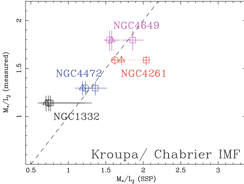
Fig. 8.12 Comparison of the stellar M/L ratios from X-ray mass modeling with those predicted from three sets of SSP models ( squares : Maraston 2005; circles : Fioc and Rocca-Volmerange 1997; triangles : Bruzual and Charlot 2003). The dotted line is “ y = x ”. The good agreement implies deviations from hydrostatic equilibrium are less than \sim 10\text{--}20\% . Adapted from Humphrey et al. (2009), see the electronic version for a color version of this figure
