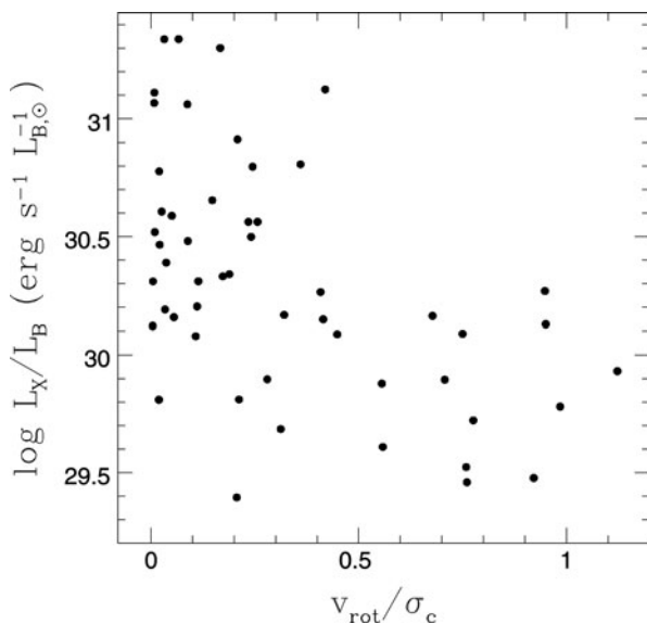
Fig. 2.15 The total X-ray emission normalized to the galactic blue luminosity L_B ( L_X and L_B determined as in Fig. 2.13), versus the indicator of rotational support v_{\text{rot}}/\sigma_c , taken from Pellegrini et al. (1997). Figure adapted and updated from Pellegrini et al. (1997)
