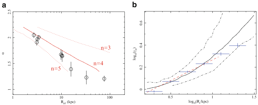
Fig. 8.9 From Humphrey and Buote (2010) : ( Left Panel ) X-ray (black circles) measurements of logarithmic mass slope plotted against optical half-light radius. The red lines are model predictions decomposing a power-law total mass profile into Sersic stellar light and NFW DM profiles (see text). ( Right Panel ) Ratio \gamma_m of total mass to stellar mass enclosed within R_e plotted vs. R_e . The solid line is the model prediction corresponding to the n = 4 curve shown in the left panel which agrees well with the data points corresponding to the K -band M/L ratios adapted from the data of La Barbera et al. (2008) , see the electronic version for a color version of this figure
