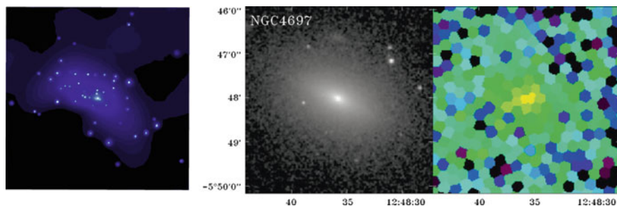
Fig. 7.2 (a) (left): Adaptively smoothed Chandra image of NGC 4697 (Sarazin et al. 2000) showing a suggestive “L-shaped” morphology in the diffuse emission at large radii. (Image credit: NASA/CXC/UVa/C. Sarazin et al.) (b) (right): Near-infrared 2MASS (left) and adaptively-binned Chandra (right) gas-only image of NGC 4697, on the same scale, reproduced from (Diehl and Statler 2007). After removal of both resolved and unresolved LMXB contributions, the L shape is no longer statistically significant
