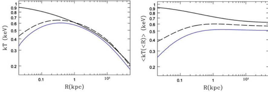
Fig. 2.9 Left : The emission-weighted and projected temperature at each radius R ( left ), and the same calculated within the radius R ( right ), for the testcase ETG (blue line) and two of the models in Fig. 2.8, with the corresponding line type, all at an age of 13 Gyr, see the electronic version for a color version of this figure
