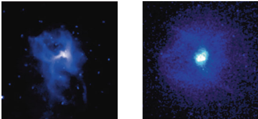
Fig. 7.1 (a) (left): Chandra image of NGC 4374 (Finoguenov and Jones 2001) showing prominent cavities in the diffuse X-ray emission that are filled by, and in pressure equilibrium with, radio lobes. (Image credit: NASA/CXC/MPE/A. Finoguenov et al.) (b) (right): Chandra image of NGC 4636 (Jones et al. 2002) showing sharp-edged structure consistent with shock models. (Image credit: NASA/SAO/CXC/C. Jones et al.), see the electronic version for a color version of this figure
