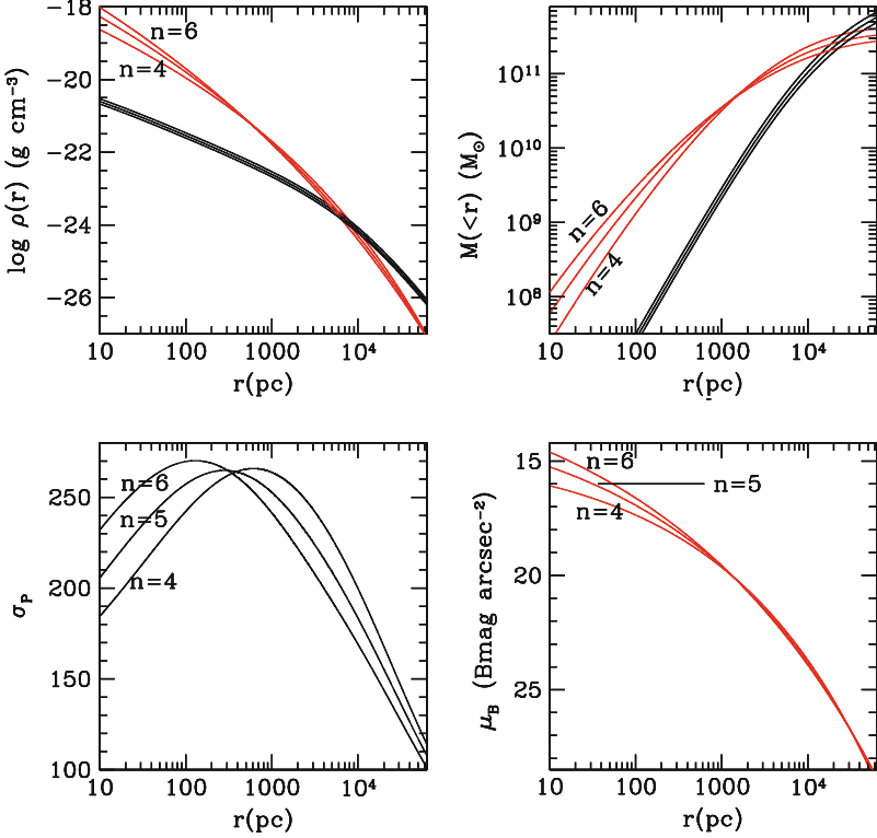
Fig. 2.4 Upper panels: density and mass profiles of a two-component galaxy model (stars+dark matter), for a representative galaxy with an aperture velocity dispersion \sigma_c = 260 km s -1 within R_e/8 , isotropic orbits, L_B = 5 \times 10^{10} L_{B,\odot} , and then R_e = 6.46 kpc, from the Fundamental Plane relation. The stellar (red) profiles follow a Sérsic law with index n = 4, 5, 6 ; the dark halo (black) has the NFW profile [ \rho_h(r) \propto M_h/4\pi r(r_h + r)^2 ] with \beta = 1.5 , \mathcal{R} = 4 and then \mathcal{R}_e = 0.48 from the Jeans equation (see Sect. 2.3.3). Lower panels: the projected velocity dispersion profile, and the B-band surface brightness profile, of the stellar component. The luminosity profile becomes more peaked with n increasing (e.g., bottom right panel), therefore the same \sigma_c is obtained with less total stellar mass (that is the dominating mass component at the center; e.g., M_*/L_B goes from 8.5 to 6.1 for n from 4 to 6); being \mathcal{R} fixed, also M_h becomes lower. The model with n = 5 (not labelled in the upper panels for clarity) is used in Sect. 2.3.3, see the electronic version for a color version of this figure
