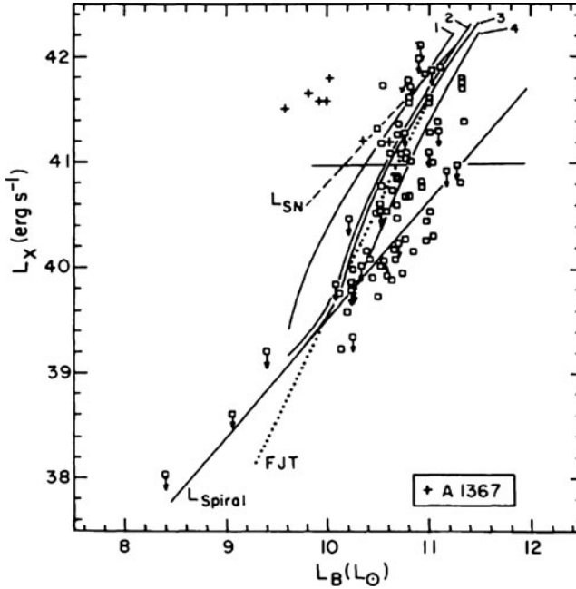
Fig. 1.3 The distribution of early-type galaxies (squares and crosses) observed in X-rays with Einstein (see CFT87). The diagonal solid line is the TF85 and CFT87 estimate of LMXB luminosity. The dotted line represents the FJT85 law of halo emission. The dashed line is the CFT87 estimate of energy input from SNe Ia, and curve represent different cooling flow models from Sarazin and White (1988; see also Sect. 3.1)
