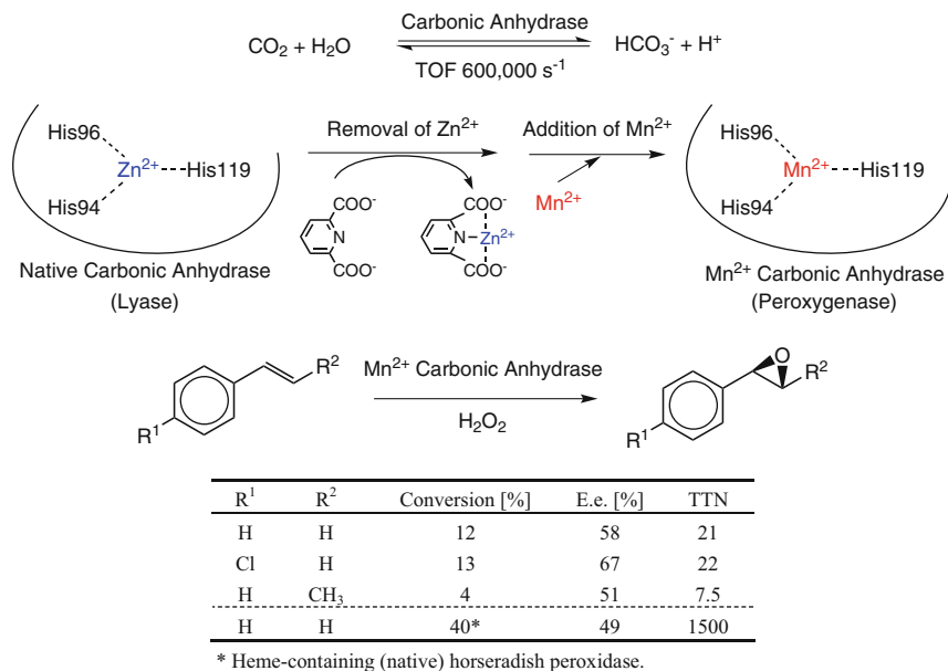
Scheme 3.54 Conversion of carbonic anhydrase (a lyase) into a peroxygenase
