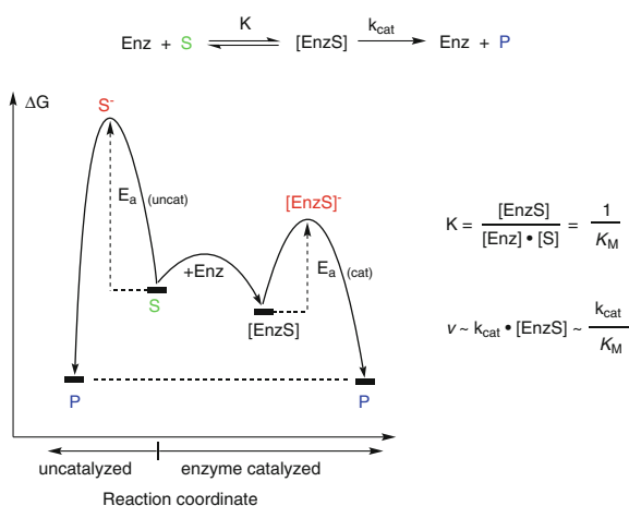
Fig. 1.7 Energy diagram of catalyzed versus uncatalyzed reaction. Enz enzyme, S substrate, P product, [EnzS] enzyme-substrate complex, K equilibrium constant for [EnzS] formation, k_{cat} reaction rate constant for [EnzS] \rightarrow Enz + P , E_a activation energy, \ddagger denotes a transition state, K_M Michaelis–Menten constant, v reaction velocity
