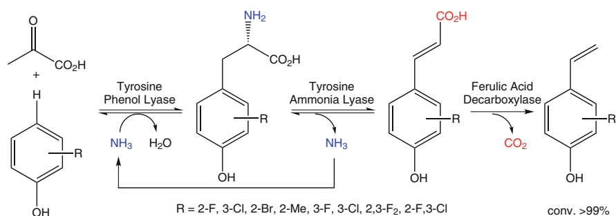
Scheme 3.43 Formal p -vinylation of phenols via a three-enzyme cascade at the expense of pyruvate producing CO 2 and H 2 O as by-products
