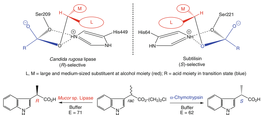
Scheme 2.46 Mirror-image orientation of the catalytic machinery of Candida rugosa lipase and the protease subtilisin and enantioselective ester hydrolysis using Mucor sp. lipase and \alpha -chymotrypsin
