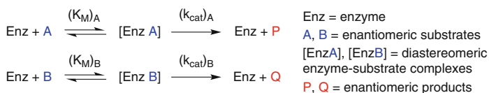
Fig. 2.3 Enzymatic kinetic resolution (irreversible reaction)
