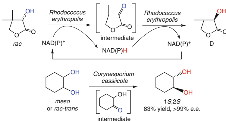
Scheme 2.128 Microbial deracemization of pantooyl lactone and 1,2-cyclohexanediol
