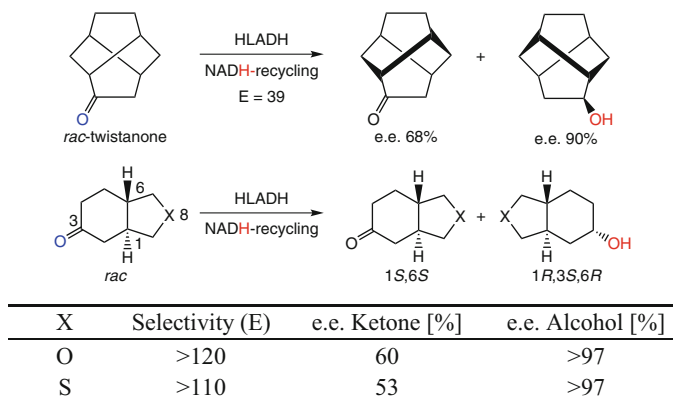
Scheme 2.113 Kinetic resolution of bi- and polycyclic ketones using horse liver alcohol dehydrogenase (HLADH)
