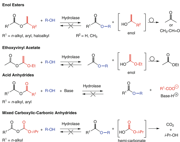
Scheme 3.4 Irreversible enzymatic acylation using enol esters and acid anhydrides
