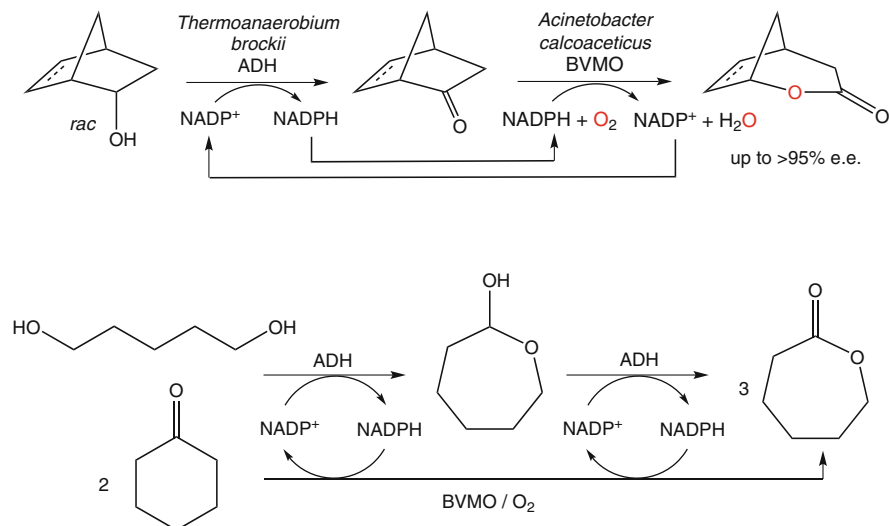
Scheme 3.42 Redox-neutral Baeyer-Villiger oxidation of ketones by starting from the corresponding alcohol ( top ) and redox-neutral formation of \epsilon -caprolactone from 1,6-hexanediol cyclohexanone ( bottom )
