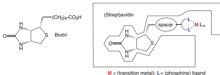
Fig. 3.11 Schematic structure of a chimeric metalloprotein based on (strept)avidin technology: A catalytically active metal ( M ) bound via ligands ( L ) onto biotin via a spacer is encaged in the biotin-binding site of the protein (strept)avidin
