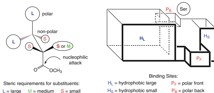
Fig. 2.11 Substrate model and active site model for porcine liver esterase
