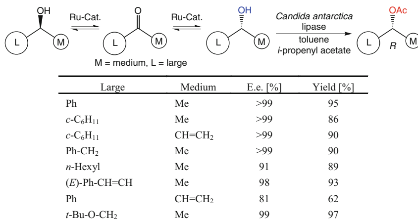
Scheme 3.17 Dynamic resolution of sec -alcohols via Ru-catalyzed in-situ racemization
