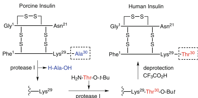
Scheme 3.30 Enzymatic conversion of porcine into human insulin
