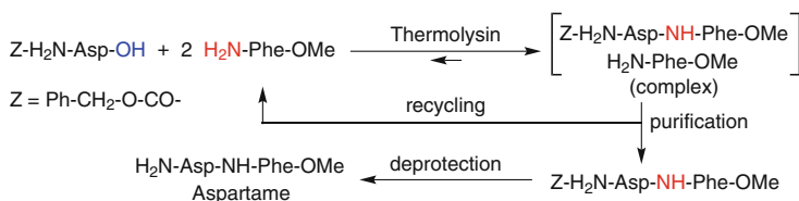
Scheme 3.28 Enzymatic synthesis of Aspartame
