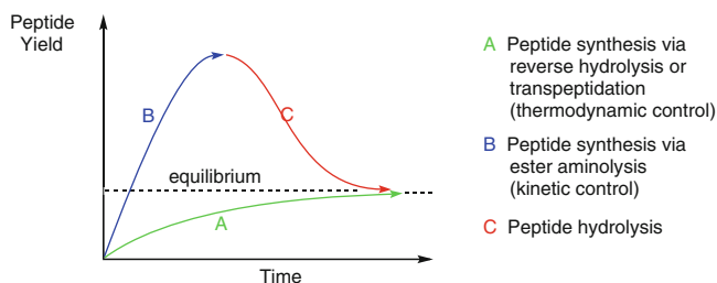
Fig. 3.2 Enzymatic peptide synthesis under thermodynamic and kinetic control
