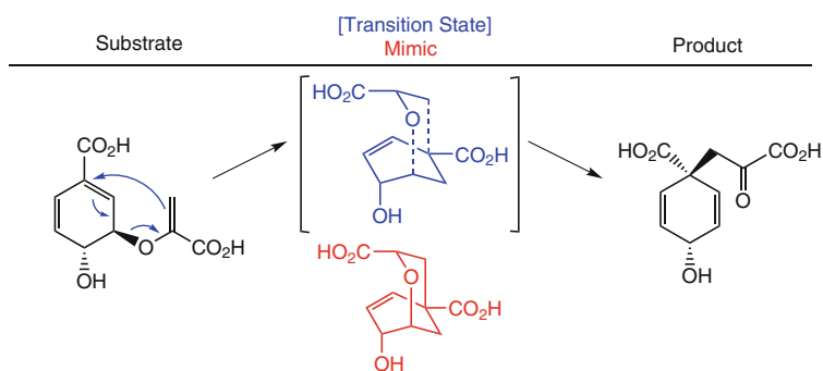
Scheme 3.56 Antibody-catalyzed Claisen-rearrangement
