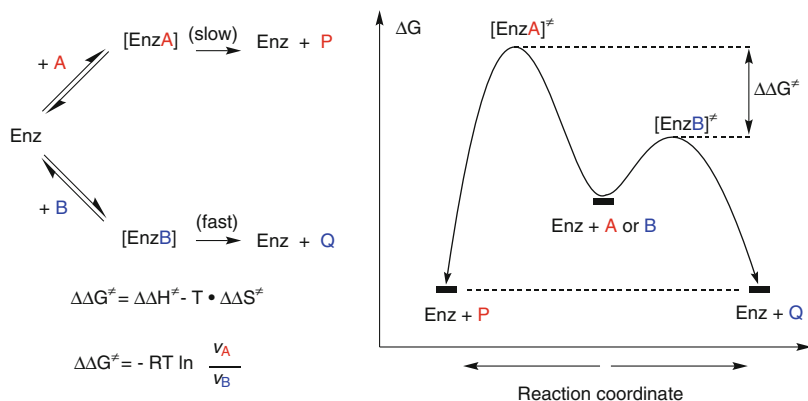
Fig. 1.8 Energy diagram for an enzyme-catalyzed enantioselective reaction. Enz enzyme, A and B enantiomeric substrates, P and Q enantiomeric products; [EnzA] and [EnzB] diastereomeric enzyme-substrate complexes; ^\ddagger denotes a transition state, \Delta\Delta G , \Delta\Delta H and \Delta\Delta S free energy, enthalpy, and entropy difference, resp., R gas constant, T temperature, v_A and v_B reaction velocities of A and B , resp.
