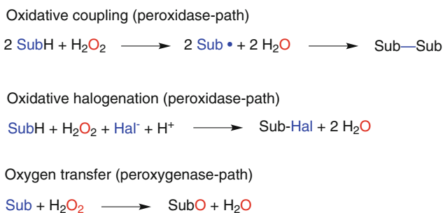
Scheme 2.172 Synthetically useful peroxidase and peroxxygenase reactions
