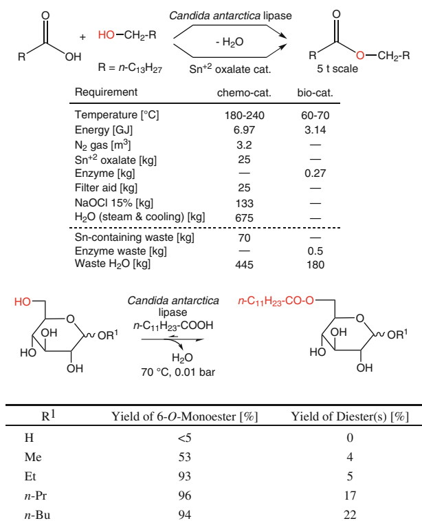
Scheme 3.1 Biocatalytic synthesis of long-chain fatty acid esters used in cosmetics
