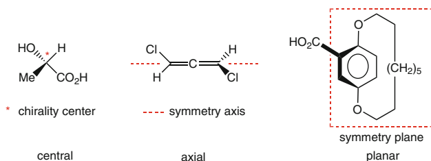
Scheme 1.3 Examples for central, axial, and planar chirality
