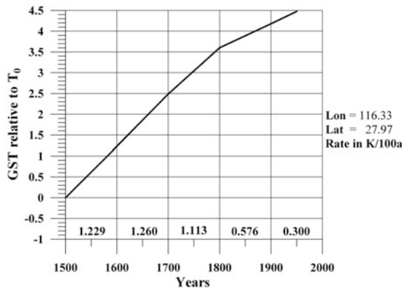
Fig. 11.10 The ground surface temperature history, borehole CN-JXzk59-38, Asia (see Table 11.1). Year of borehole logging: 1991; Mean ground surface temperature T_0 = 13.7^{\circ}\text{C}
