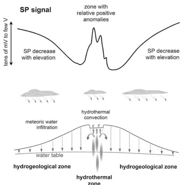
Fig. 12.11 Conceptual model of SP patterns on a volcano (after Lénat 2007)
