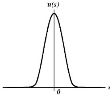
Fig. 7.14 Finite-localized solution—compacton
