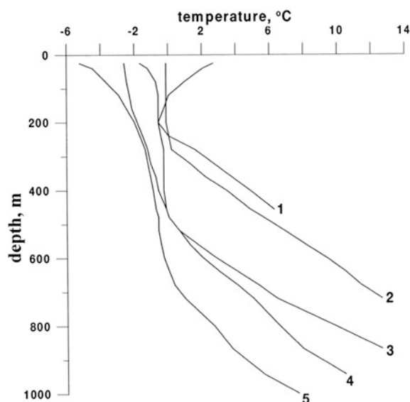
Fig. 5.2 Vertical profiles of a transient temperature field of rocks in different areas. (1) Lower Ob', (2) Kostrovskii, (3) Middle Vilyui, (4) Namtsy, (5) Bakhynai (Balobayev et al. 1973)
