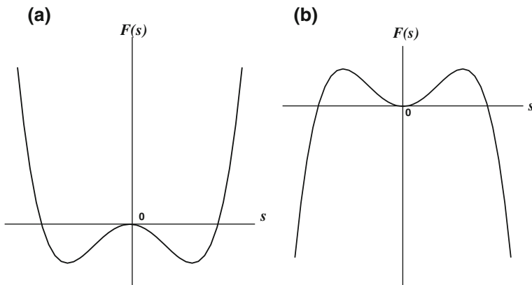
Fig. 7.12 Potential function F(u) from source f(u) = \alpha u + \epsilon u^3 : (a) \alpha < 0, \epsilon > 0 , (b) \alpha > 0, \epsilon < 0
