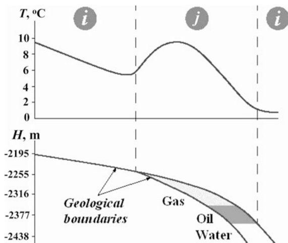
Fig. 10.17 Graph of the temperature field observed over the Black Lake deposit (Louisiana, USA) (after Lasky 1967). According to the author, intervals i and j designate background and anomalous parts of the temperature graph, respectively
