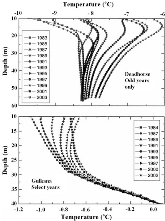
Fig. 5.17 Selected annual temperature profiles, 1983–2003, at sites near each end of the transect (Oslerkamp 2005)
