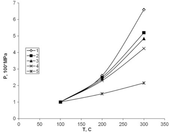
Fig. 4.5 Conditions of thermodynamic equilibrium for some rocks ( dv = 0 ): 1 bytownite gabbro, 2 dunite, 3 pink granite, 4 grey granite, 5 gabbro ( 0^\circ\text{C} = 273.15\text{ K} )
