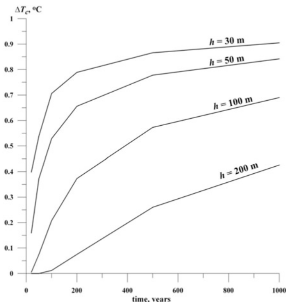
Fig. 11.19 Present perturbations versus the temperatures \Delta T_c due to instantaneous surface temperature changes of 1^\circ\text{C} at various times prior to the present. Thermal diffusivity = 0.0036\text{ m}^2/\text{h} , \Delta T in ^\circ\text{C}
