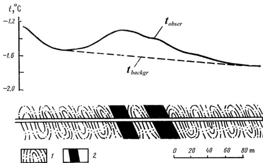
Fig. 10.11 Example of application of underground thermal prospecting in a gold-sulphide deposit in Yakutiya (Russia). (1) phyllites with siltstone, (2) gold-sulphide ore (Brodovoi et al. 1988)
