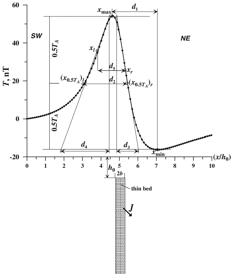
Fig. 7.10 Distribution of characteristic points and tangents on an anomaly plot for an obliquely magnetized thin bed ( J is the magnetization vector) situated in a non-magnetic medium. Open circles are points of extrema and semi-amplitude; closed circles are inflection points of the anomaly plot
