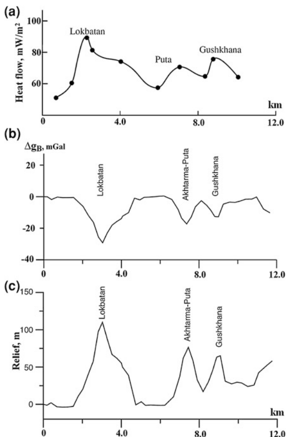
Fig. 4.4 Changes in heat flow (a), Bouguer gravity (b), and topography (c) along the profile crossing the Lokbatan–Akhtarma–Putu–Gushkhana mud volcanoes (compiled from Kadirov and Mukhtarov 2004; Kadirov et al. 2005, with modifications after Eppelbaum and Khesin 2012)
