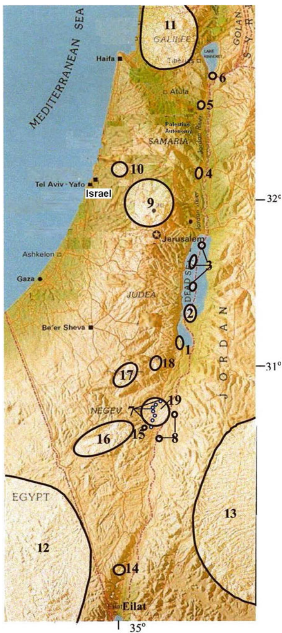
Fig. 13.6 Location of some ring structures in Israel and adjacent areas (after Eppelbaum et al. 1998).
