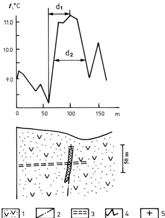
Fig. 10.5 Quantitative interpretation of temperature anomalies in the area of the Kvaisa pyrite-polymetallic deposit (southern slope of the Greater Caucasus, Georgia) (observed data and geological section after Ginzburg et al. 1974). (1) Volcanoclastic medium, (2) fault, (3) position of mine, (4) temperature graph, (5) determined position of the middle of upper edge of orebody. The massive sulfide ore body is shaded
