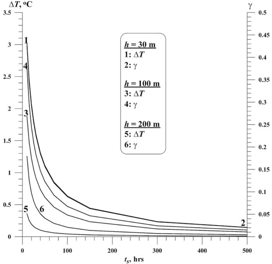
Fig. 11.18 Function \gamma and the values \Delta T = T_f - T_s
