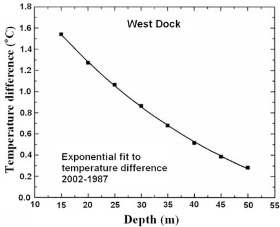
Fig. 5.18 An exponential fit to temperature differences between 1987 and 2002 for 5 m depth increments at the West Dock site (Oslerkamp 2005)
