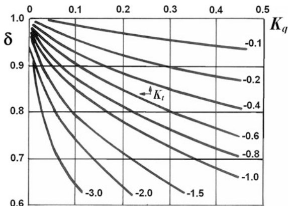
Fig. 5.7 The \delta = \delta(K_t, K_q) coefficient (Pavlov 1974)
