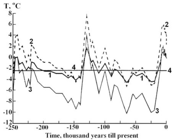
Fig. 11.2 Average global and regional paleotemperature for the last 250 T. y. (1) average global temperature for the northern semisphere (2) paleotemperature for the area of Vorotilov deep borehole (central part of the Russian platform, Russia) (3) paleotemperature for the area of Kola superdeep borehole (Kola Peninsula, Russia) (4) linearly averaged global temperature for the last 250 T. y. (after Pimenov et al. 1996, with small modifications)
