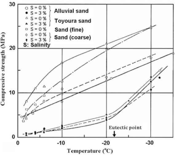
Fig. 5.3 Relation between compressive strength and temperature for sands (Ogata et al. 1982)
