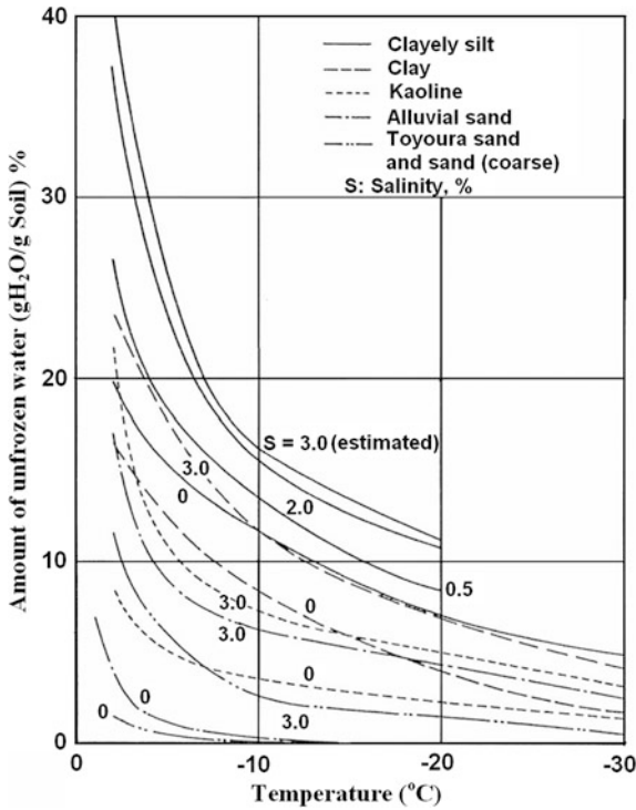
Fig. 5.5 Relation between unfrozen water content and temperature (Ogata et al. 1982)
