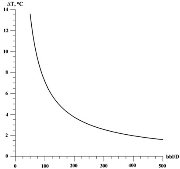
Fig. 9.3 The function \Delta T ( z = 0 , t = 200 days) versus flow rate
