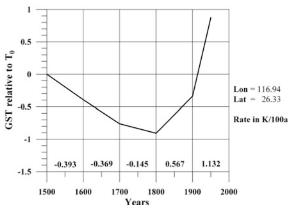
Fig. 11.11 The ground surface temperature history, borehole CN-FJ-q117, Asia (see Table 11.1). Year of borehole logging: 1987; Mean ground surface temperature T_0 = 18.5^\circ\text{C}
