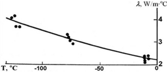
Fig. 12.1 Dependence of the thermal conductivity of ice on temperature (after Ivanov and Gavriljev 1965)
