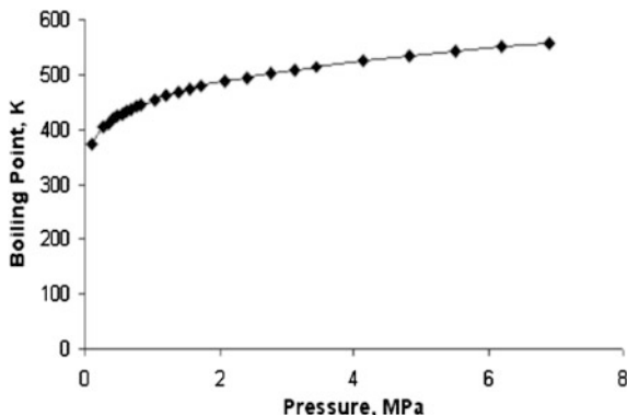
Fig. 6.1 Changes in the boiling point of water with increases in pressure in the range 0.101–6.895 MPa [compiled using data from (Speight 2005)]
