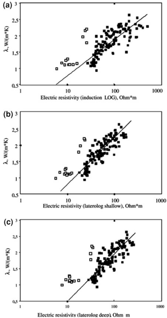
Fig. 12.6 Regressed correlations between the thermal conductivity of dry rocks and electric resistivity determined from the induction log (a) the laterlog shallow (b) and the laterolog deep (c). Empty squares —ultrabasites and high temperature suevites, solid squares —all other rocks (after Popov et al. 2003 with minor modifications)
