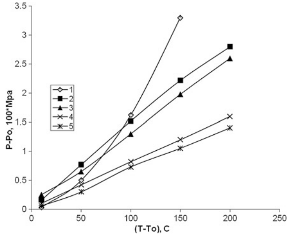
Fig. 4.6 Increase of excess pressure ( P - P_0 ) with increase of excess temperature ( T - T_0 ) for some rocks. 1 wet clay, 2 limestone, 3 granite, 4 sandstone, 5 basalt ( 0^\circ\text{C} = 273.15\text{ K} )
