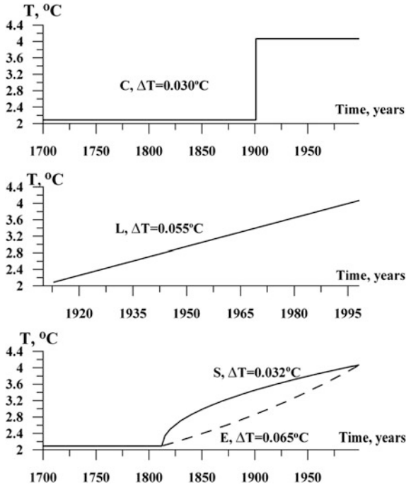
Fig. 11.9 Possible ground surface temperature history scenarios, borehole Ca-9806, North America (see Table 11.1)
