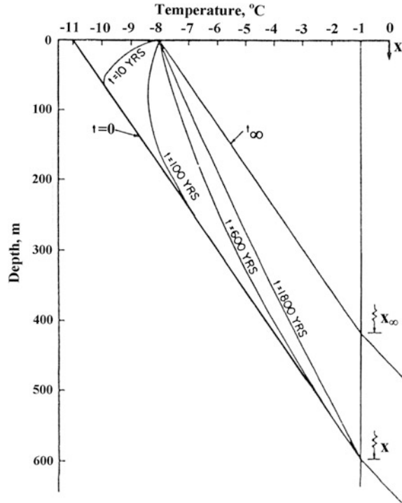
Fig. 5.10 Thermal warming model for the continuous permafrost zone (Osterkamp 1983)
