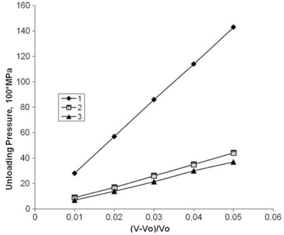
Fig. 4.9 Unloading of pressure in the case of expansion ( \Delta V > 0 ) and loading of pressure in the case of compression ( \Delta V < 0 ) for 1 sandstone, 2 basaltic melt, and 3 wet clay ( 0^\circ\text{C} = 273.15\text{ K} )
