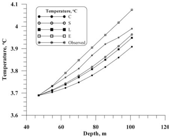
Fig. 11.7 Observed and calculated temperature profiles, borehole Ca-9807, North America (see Table 11.1)
