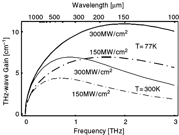
Fig. 4.54 Calculated gain coefficient for the parametric THz-wave generation using LiNbO 3 crystal pumped at 1.064 μm
