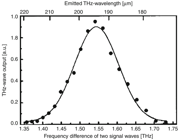
Fig. 5.45 The tunability of surface-emitted DFG without crystal
