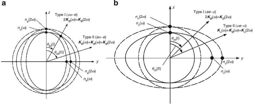
Fig. 1.8 Diagrammatic sketch of phase matching: (a) uniaxial negative crystals and (b) uniaxial positive crystals
