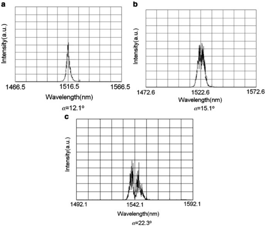
Fig. 5.50 The signal spectra for TIR-PPLN-OPG
