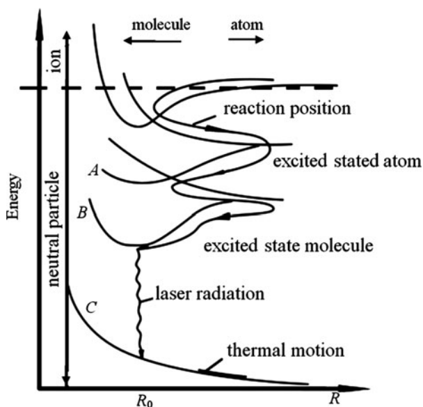
Fig. 10.31 The energy level of excimer system and interaction path
