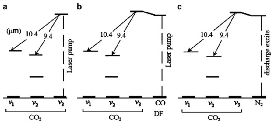
Fig. 10.24 The diagram of excitation process: (a) directly optical pumping; (b) optical pumping using transferring molecule; and (c) discharge excitation
