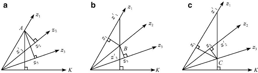
Fig. 1.37 The energy flow direction (a) \mathbf{E}_1(z_1, t) , (b) \mathbf{E}_2(z_2, t) , and (c) \mathbf{E}_3(z_3, t) in biaxial crystal
