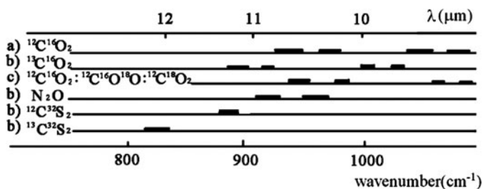
Fig. 10.25 The tuning range of \text{CO}_2 , \text{N}_2\text{O} , and \text{CS}_2 isotopes
