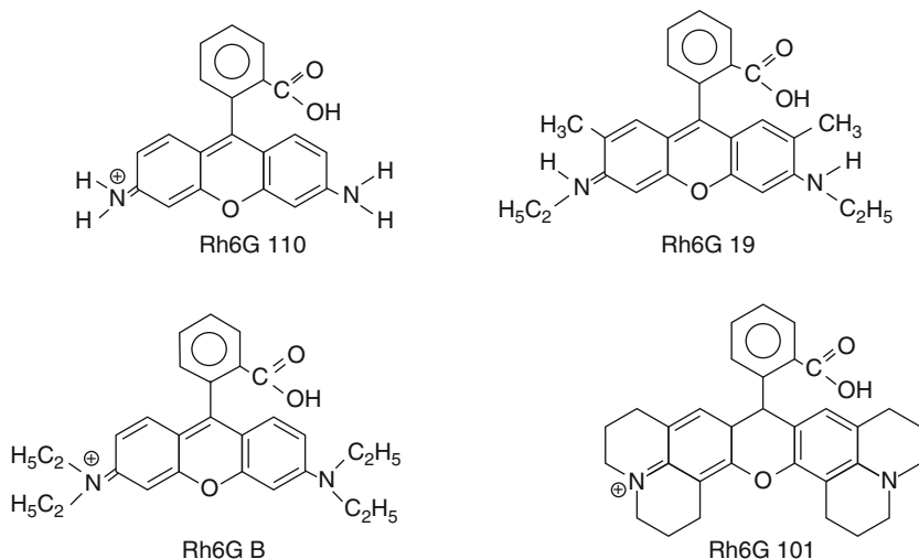
Fig. 10.1 The diagrammatic sketch of several dye molecular structures of Rh6G
