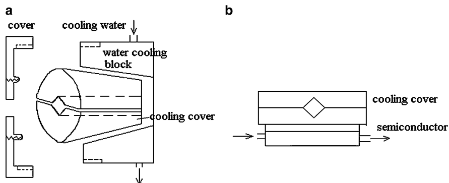
Fig. 3.6 Cooling device of KTP crystal. (a) water cooling; (b) semiconductor cooling
