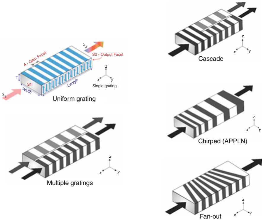
Fig. 5.1 Various QPM patterns
