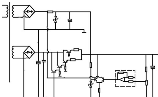
Fig. 3.12 Control circuit of Q-switch power
