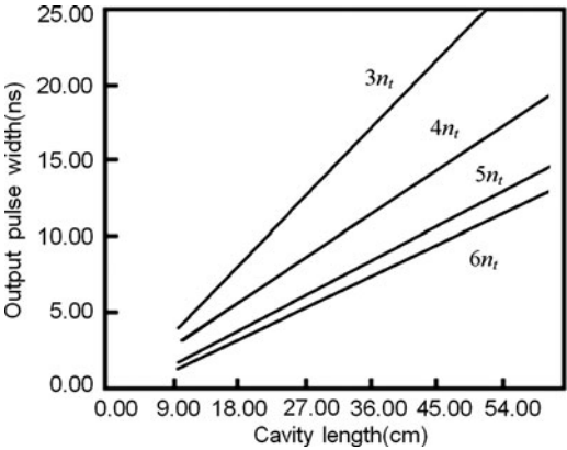
Fig. 9.70 Output pulse width vs. the cavity length at pump pulse width of 10 ns
