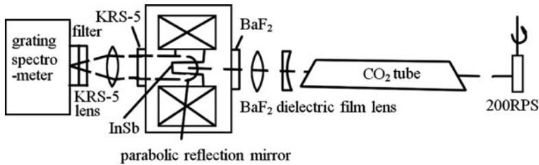
Fig. 10.13 The structure of spin-flip Raman laser
