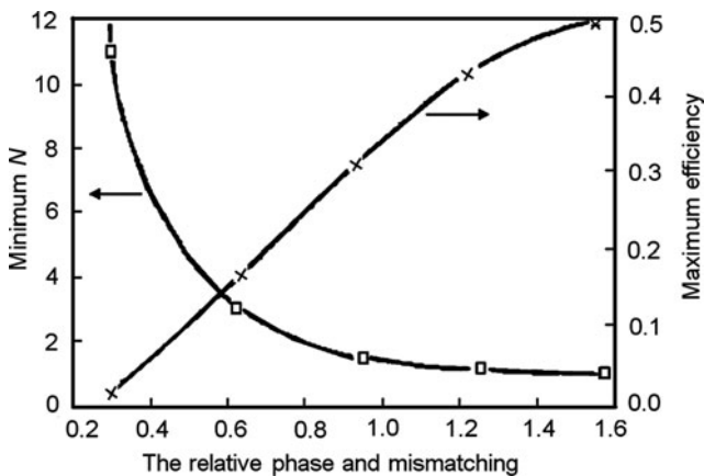
Fig. 4.17 The minimum pump multiple and maximum efficiency of DRO vs. the relative phase and phase mismatch
