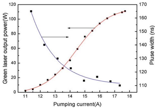
Fig. 7.13 The green output power and pulse width as a function of diode pumping current
