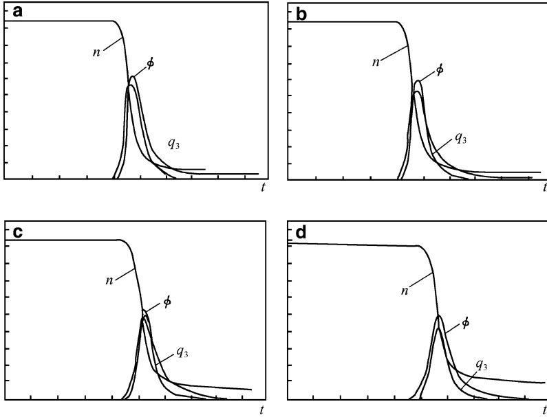
Fig. 3.4 Variation of \phi , q_3 , n with time under different intracavity losses (200 ns/lattice) (a) \alpha_0 = 5 \times 10^6 (1/s), (b) \alpha_0 = 2 \times 10^7 (1/s), (c) \alpha_0 = 5 \times 10^7 (1/s), (d) \alpha_0 = 1 \times 10^8 (1/s)
