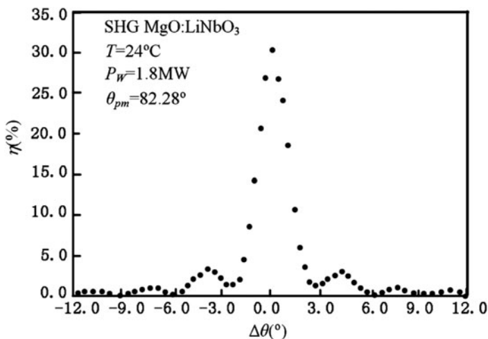
Fig. 4.36 Relationship between conversion efficiency (experimental value) \eta and phase mismatching angle \Delta\theta in MgO : LiNbO 3 SHG
