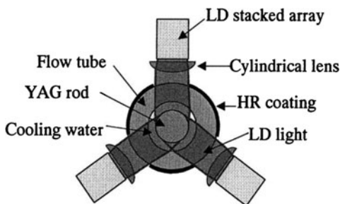
Fig. 6.17 The experiment setup of the 1.06 \mu\text{m} laser system of 407 W
