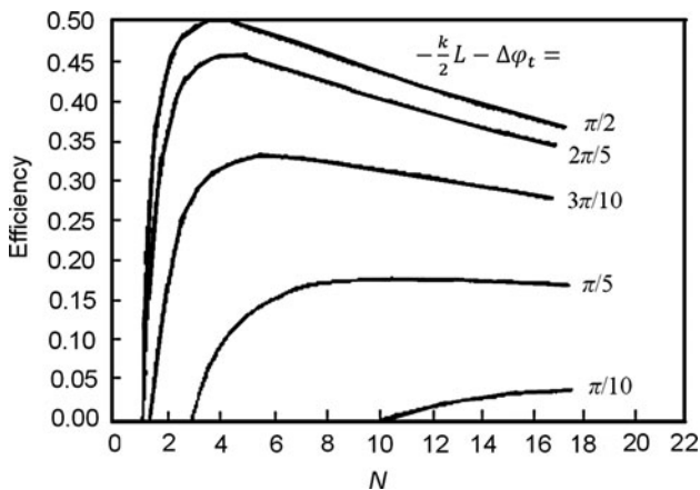
Fig. 4.16 The influence of phase mismatching and relative phase on the efficiency of DRO
