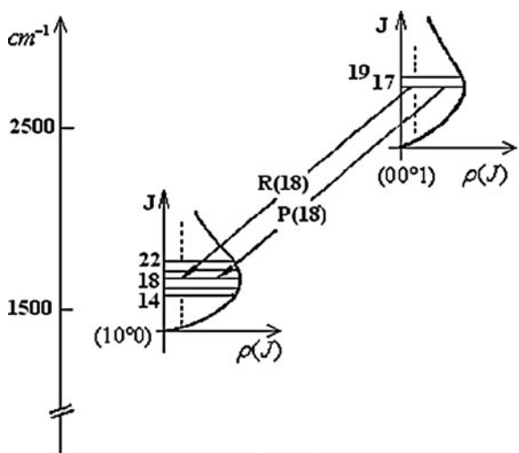
Fig. 10.22 The vibrational transition of P and R branch of \text{CO}_2
