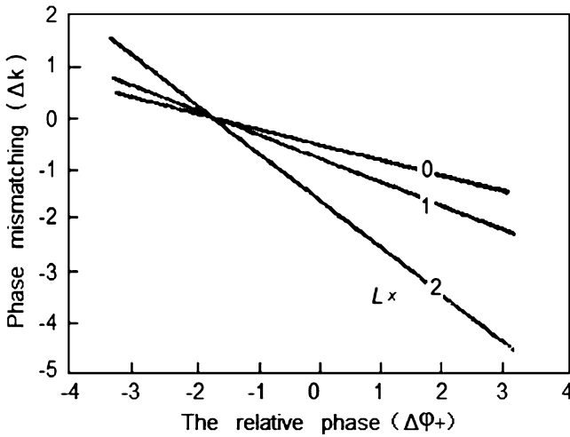
Fig. 4.15 The phase mismatching \Delta k vs. relative phase \Delta\varphi_+
