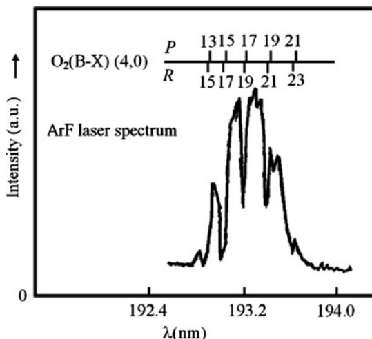
Fig. 10.38 The absorption in ArF laser spectrum
