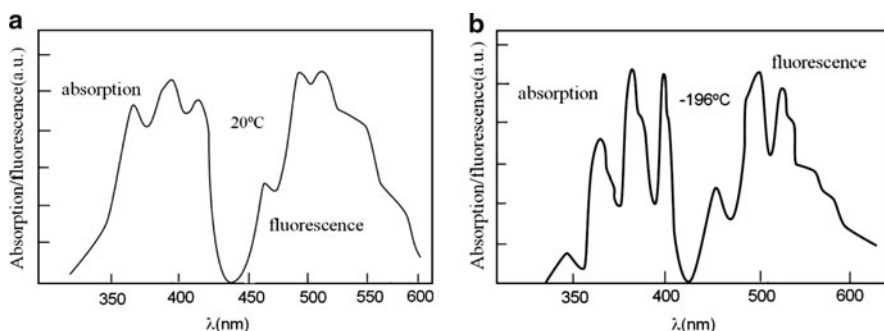
Fig. 10.4 The relationship between spectrum and temperature of dye molecule
