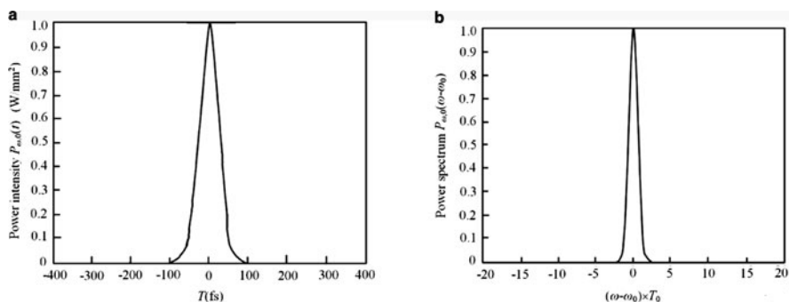
Fig. 3.39 Power of incident fundamental wave (a) P_{\omega,0}(t) and (b) P_{\omega,0}(\omega - \omega_0)
