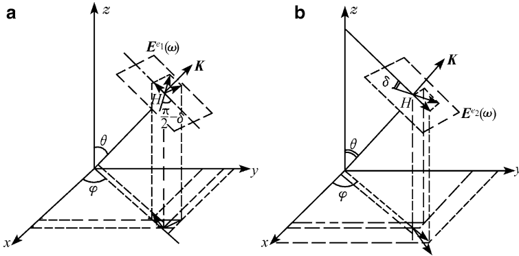
Fig. 1.12 The projection of (a) \mathbf{E}^{e_1}(\omega) and (b) \mathbf{E}^{e_2}(\omega) in the coordinate system
