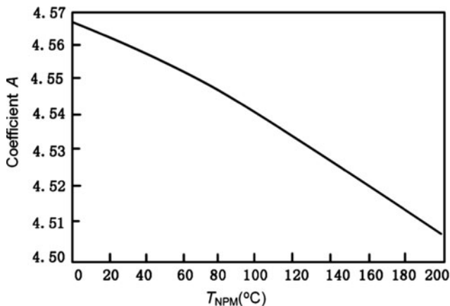
Fig. 4.34 Variation of the coefficient A with T_{\text{NPM}}
