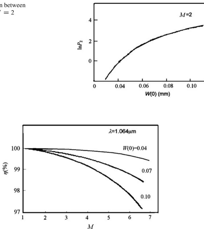
Fig. 2.15 Relation between frequency doubling efficiency and M at different W(0)
