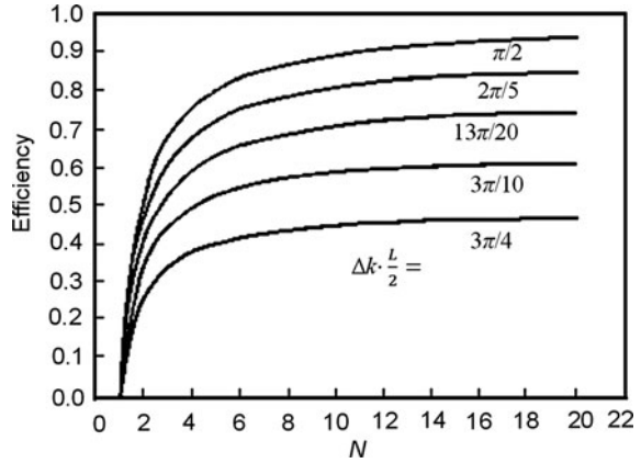
Fig. 4.18 The influence of phase mismatching on conversion efficiency in SRO
