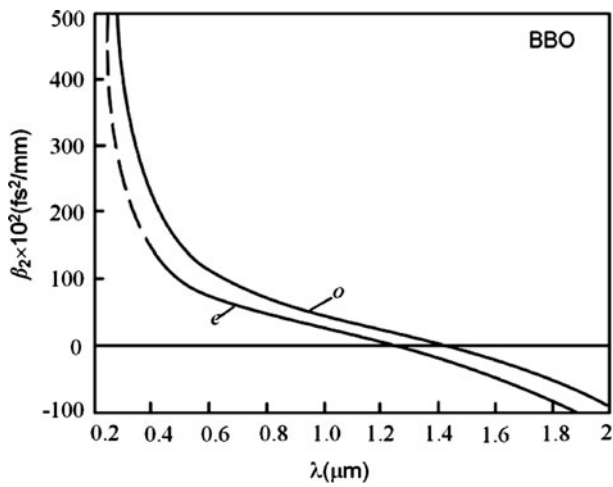
Fig. 3.32 Coefficient of group velocity dispersion of BBO crystal (low order) \beta_2(\text{fs}^2/\text{mm})
