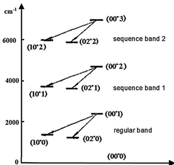
Fig. 10.21 The simplified vibrational energy level diagram of \text{CO}_2 (including sequence band and regular band)
