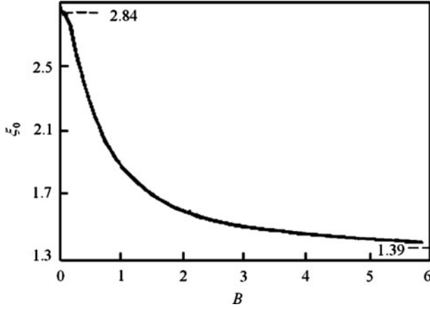
Fig. 2.7 Relation between B and \xi_0
