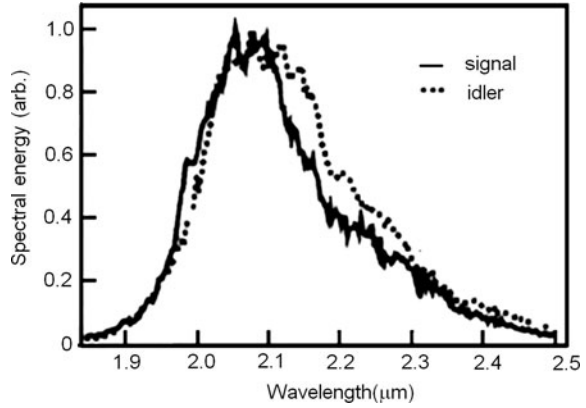
Fig. 5.36 (a) Collinear signal and (b) idler spectra
