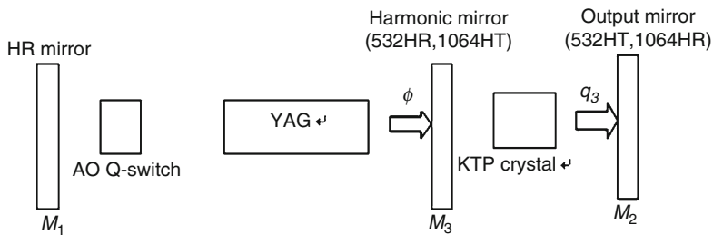
Fig. 3.1 Schematic diagram of intracavity frequency doubling YAG laser
