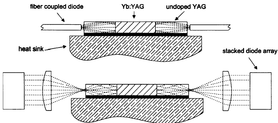
Fig. 7.38 Edge-pumping thin disk DPL
