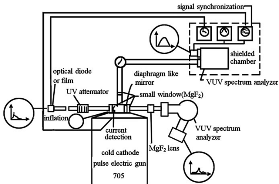
Fig. 10.37 The setup of electron beam pumped gas-phase \text{Xe}_2^* excimer laser
