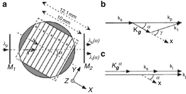
Fig. 5.24 (a) Schematic of the OPO with a PPKTP crystal with cylindrical shape. The plus and minus signs denote the polarization directions of the ferroelectric domains. The gray areas mean unpoled. x , y , and z are the crystallographic axes, and z is the polar axis; (b) The directions of QPM-OPO wave vector
