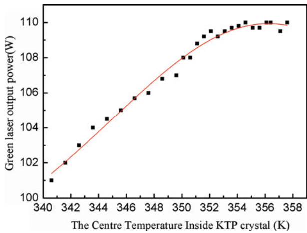
Fig. 7.12 The green output power changes with the KTP crystal center temperature
