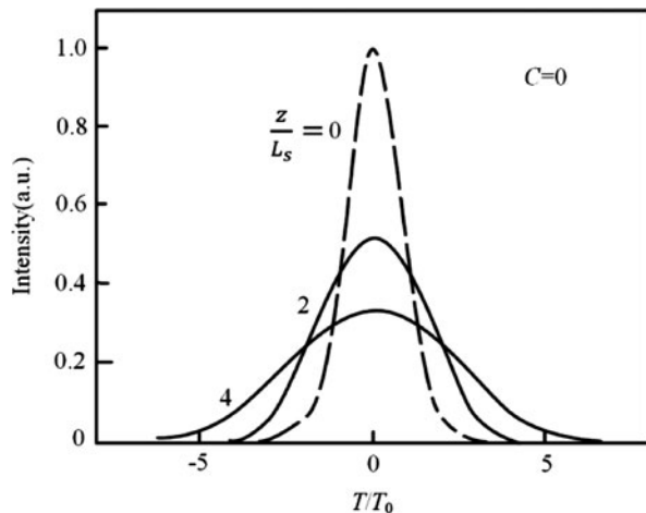
Fig. 3.35 Shapes of \text{sech}^2 x pulses at the positions of z = 2L_s and z = 4L_s
