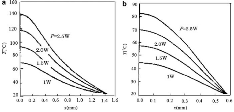
Fig. 1.47 The temperature distribution in KTP crystal with circular incident surface. (a) r = 1.5 mm; (b) r = 0.6 mm
