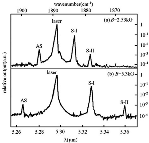
Fig. 10.14 The spectrum of spin-flip Raman laser
