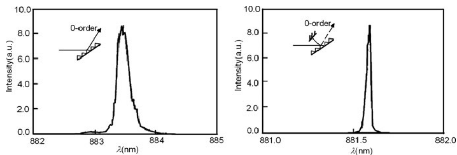
Fig. 4.22 The linewidth of single resonant ps-OPO
