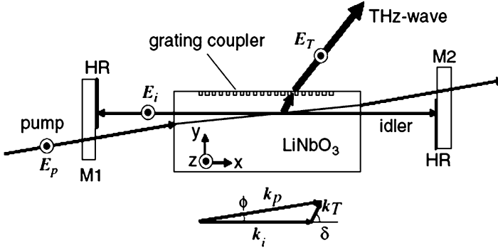
Fig. 4.56 Schematic of the grating coupler for THz-wave output
