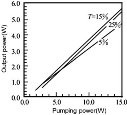
Fig. 9.38 Output power vs. input power for different transmittance of output mirror
