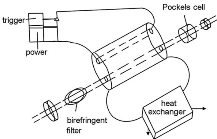
Fig. 8.11 The diagrammatic sketch of Cr:BeAl 2 O 4 laser pumped by lamp
