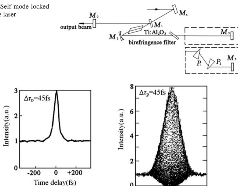
Fig. 9.89 The measurement results of pulse width with two methods
