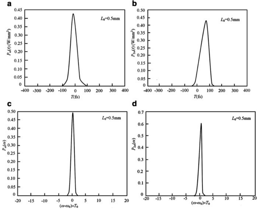
Fig. 3.42 Time and frequency spectra of the fundamental and harmonic wave power after BBO crystal ( l = 0.5 mm) (a) time spectrum of the fundamental wave; (b) time spectrum of the harmonic wave; (c) frequency spectrum of the fundamental wave; (d) frequency spectrum of the harmonic wave
