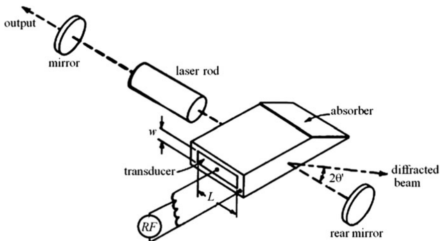
Fig. 6.20 Acousto-optic Q-switching employed in a CW-pumped Nd:YAG laser
