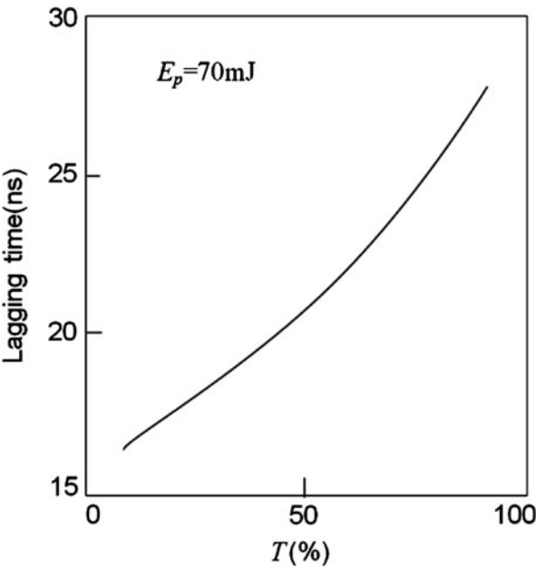
Fig. 8.32 The output lagging time with transmittance
