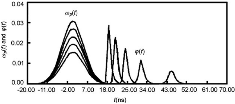
Fig. 9.60 Output pulse at pump pulse width of 10 ns and energy of 4-8n_t
