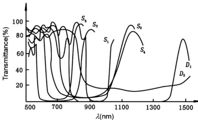
Fig. 4.44 The transmittances of cavity mirrors in the experiments
