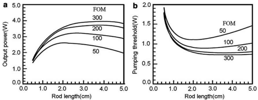
Fig. 9.11 (a) Output power and (b) pumping threshold as a function of the rod length under different FOM
