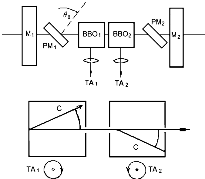
Fig. 4.26 Dual BBO-OPO with compensation of walk-off effect
