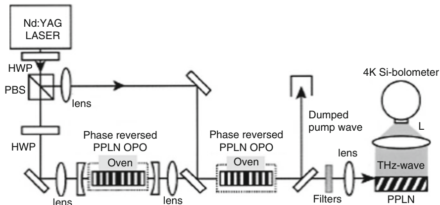
Fig. 5.44 Experimental setup for THz-wave surface-emitted difference frequency generation. HWP, half-wave plate; PBS, polarizing beam splitter; L, polyethylene lens
