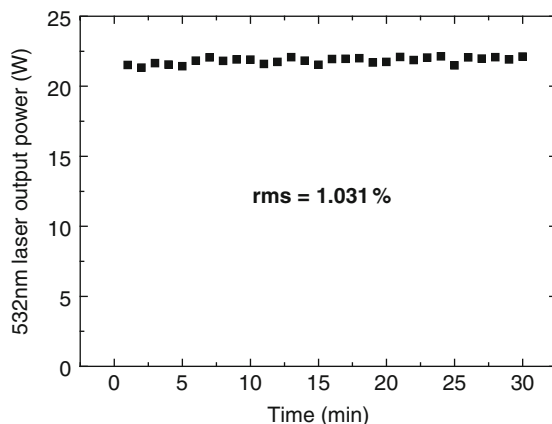
Fig. 7.17 The output power stability of the system
