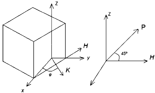
Fig. 3.7 Directions of light propagation and polarization in KTP crystal
