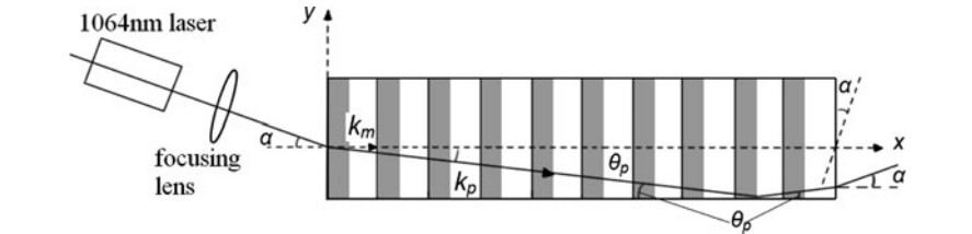
Fig. 5.49 The experimental setup for TIR-QPM PPLN OPG
