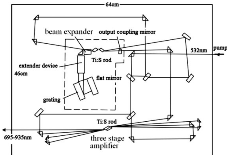
Fig. 9.56 Pulsed Ti:sapphire oscillator-amplifier system
