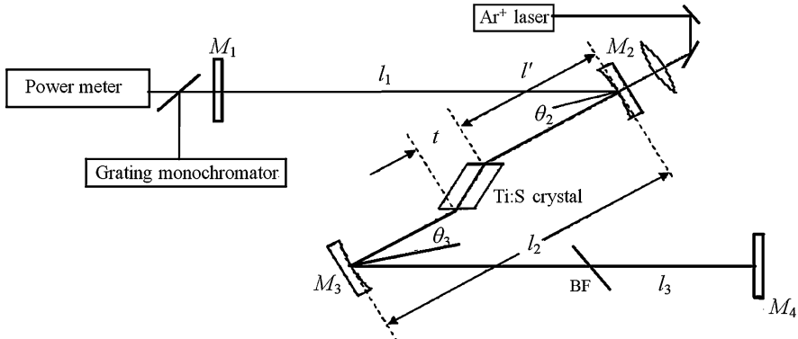
Fig. 9.19 Experimental setup of four-mirror cavity
