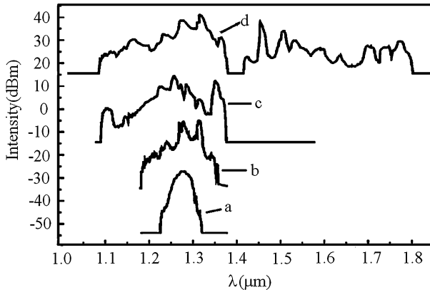
Fig. 7.59 The evolution of the spectral broadening with the average pump power of 30 mW and the energy of 120 nJ per pulse (the spectral curves were all scaled vertically for comparison)
