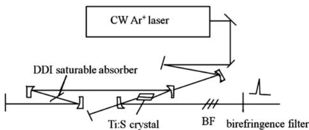
Fig. 9.79 Experimental setup of passive mode-locked Ti:sapphire laser
