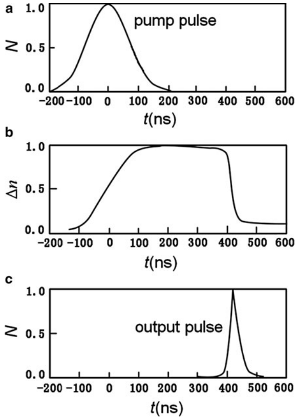
Fig. 9.27 The (a) pump pulse, (b) population inversion and (c) the density of photon in cavity at L = 30 cm and P_0 = 4 W
