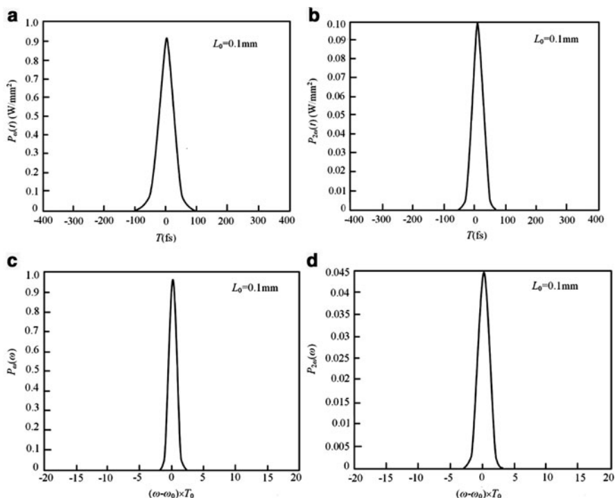
Fig. 3.41 Time and frequency spectra of the fundamental and harmonic wave power after BBO crystal ( l = 0.1 \text{ mm} ) (a) time spectrum of the fundamental wave; (b) time spectrum of the harmonic wave; (c) frequency spectrum of the fundamental wave; (d) frequency spectrum of the harmonic wave
