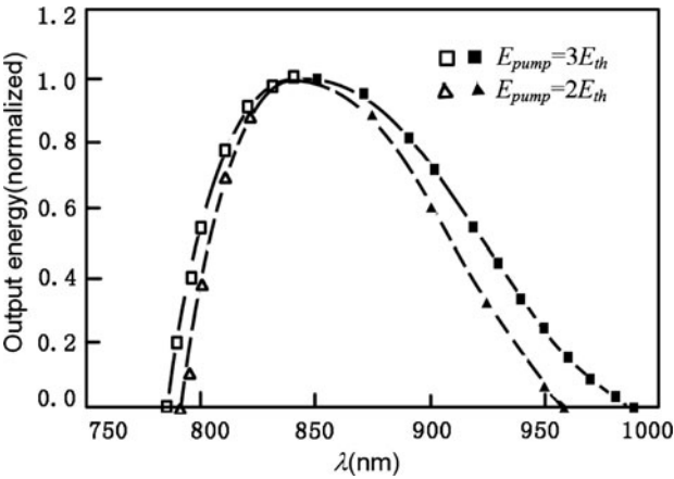
Fig. 8.41 The tuning range of Cr:LiSAF laser
