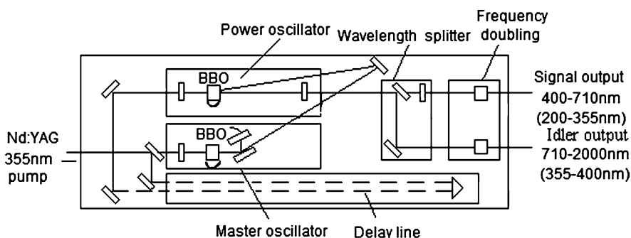
Fig. 4.23 The series of MOPO-700 BBO-OPO system
