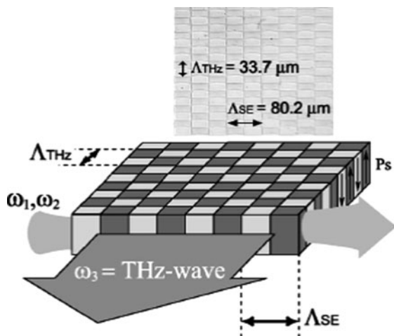
Fig. 5.46 Schematic illustration of 2D PPLN. Ps indicates the spontaneous polarization of the crystal. The top view of the 2D PPLN for 1.7 THz generation is also shown
