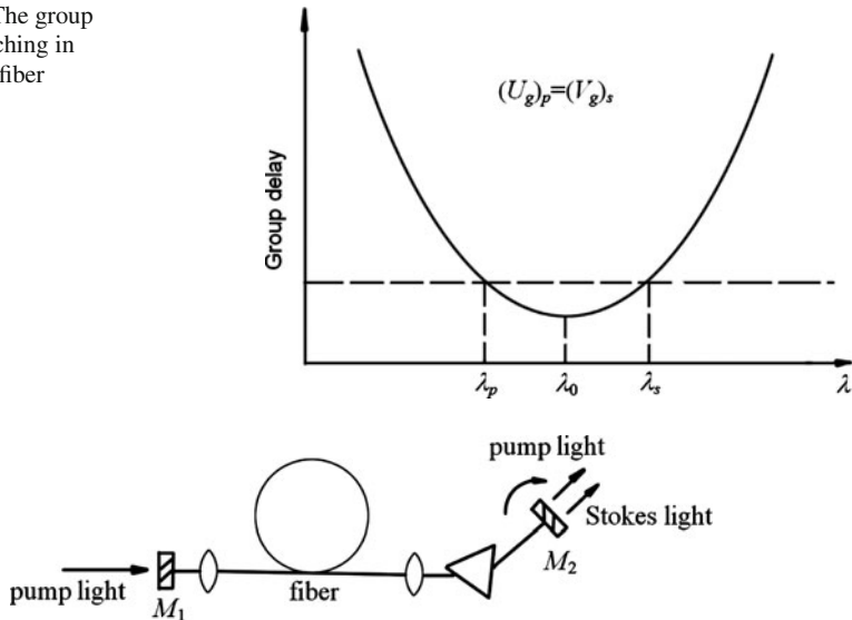
Fig. 10.19 The schematic diagram of fiber Raman laser
