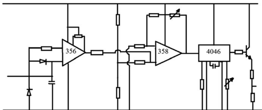
Fig. 3.11 Control circuit of Q-switch frequency
