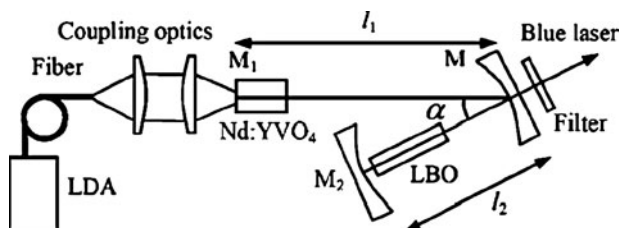
Fig. 7.20 The setup of the 4.6-W intracavity frequency-doubled 457 nm Nd : YVO 4 /LBO blue laser
