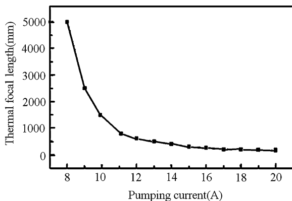
Fig. 6.12 The thermal focal length as a function of pumping current
