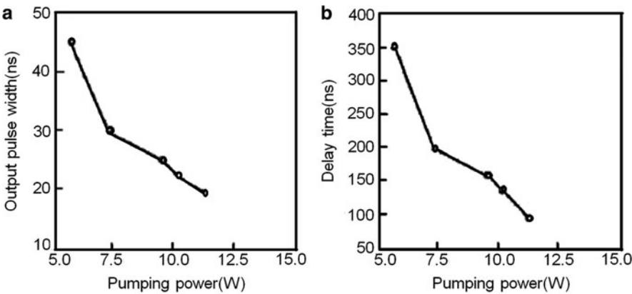
Fig. 9.48 (a) Pulse width and (b) delay time of QCW Ti:sapphire laser vs. pump power
