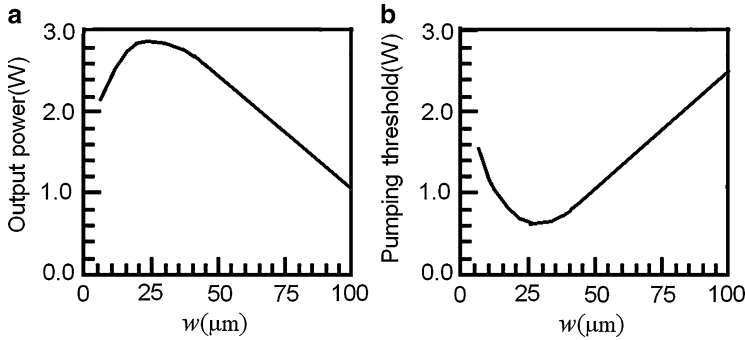
Fig. 9.15 (a) Output power and (b) pump threshold vs. the pump beam waist
