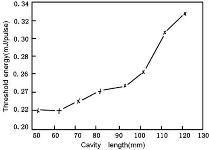
Fig. 4.48 Variation of the threshold in DRO with the cavity length
