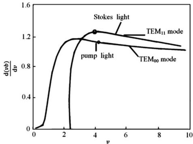
Fig. 10.17 The group velocity matching in dual-mode fiber
