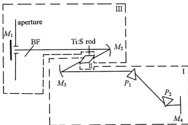
Fig. 9.97 Divided zones for different effects in self-mode-locked Ti:sapphire laser cavity
