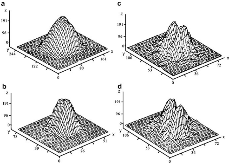
Fig. 3.24 (a, b) Measurement of typical modes; the near fundamental mode; (c) TEM 01 mode; (d) an irregular mode
