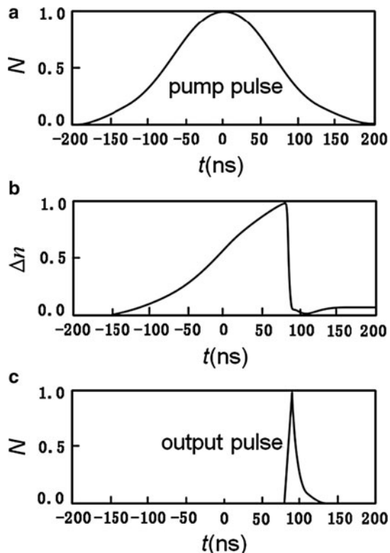
Fig. 9.28 The (a) pump pulse, (b) population inversion and (c) the density of photon in cavity at L = 20 and P_0 = 10 W
