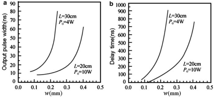
Fig. 9.31 (a) The output pulse width and (b) delay time as a function of spot size
