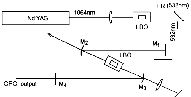
Fig. 4.21 Singly resonant ps-LBO-OPO system
