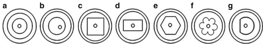
Fig. 7.41 Cross section of different inner cladding: (a) concentric, (b) eccentric, (c) foursquare, (d) rectangular, (e) polygon, (f) cinquefoil, and (g) D-shaped
