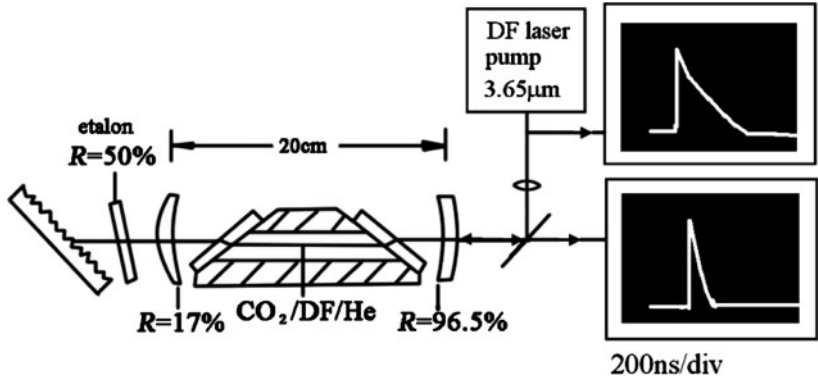
Fig. 10.26 The diagram of optical pumping tunable CO 2 laser
