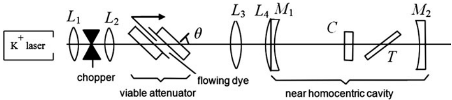
Fig. 8.42 The tunable Cr:LiSAF laser pumped by Kr^+ laser
