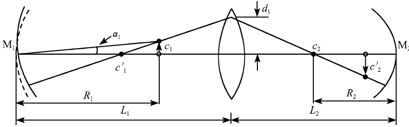
Fig. 6.4 The diagram of a misaligned resonator
