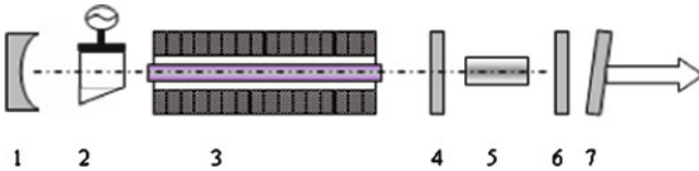
Fig. 7.1 Linear cavity Q-switched red DPL (1. 1,319-nm HR mirror, 2. Q-switch, 3. Nd:YAG rod, 4. harmonic mirror, 5. KTP, 6. output lens, and 7. filter)
