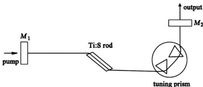
Fig. 9.53 Pulsed Ti:sapphire laser with two prisms tuning
