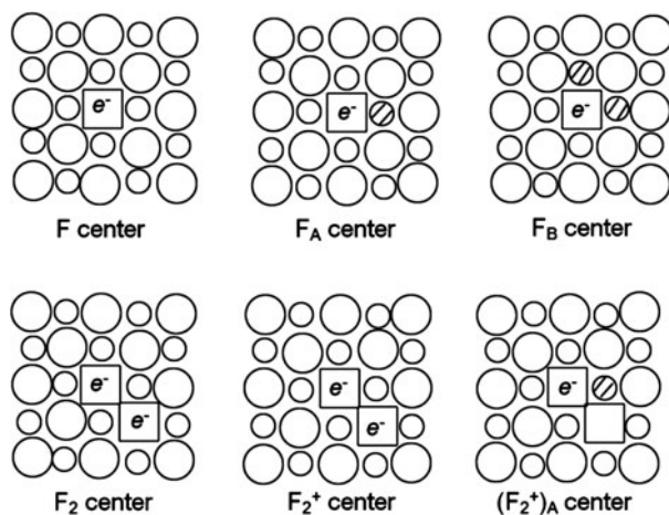
Fig. 8.43 Several typical structural pattern of F alkali halide center
