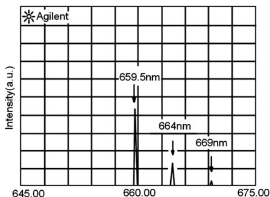
Fig. 7.3 Spectrum of the red DPL
