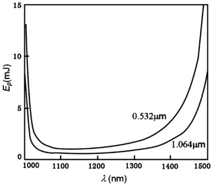
Fig. 8.24 The threshold at different pumping wavelength
