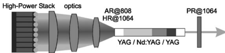
Fig. 6.17 The experiment setup of the 1.06 \mu\text{m} laser system of 407 W
