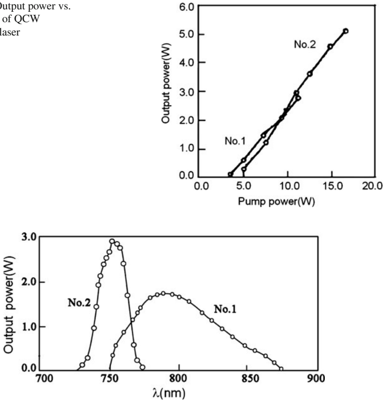
Fig. 9.44 Tuning curves of QCW Ti:sapphire laser
