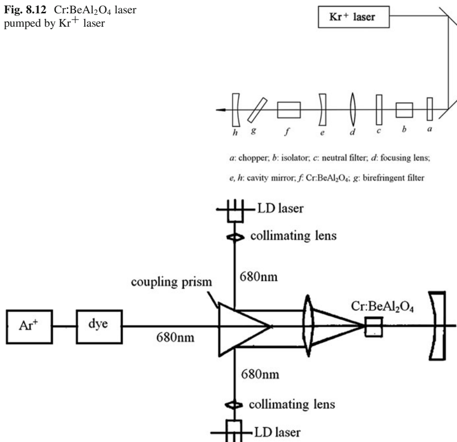
Fig. 8.13 Cr:BeAl 2 O 4 laser pumped by LD laser
