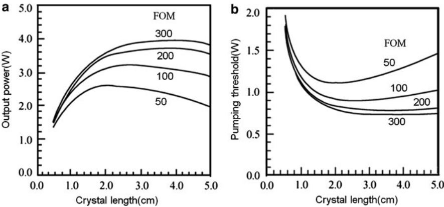
Fig. 9.36 (a) Output power and (b) pump threshold vs. crystal length at different FOM
