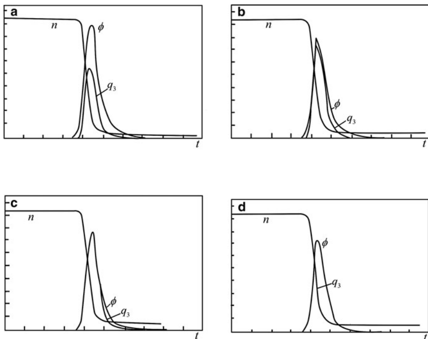
Fig. 3.3 Variation of \phi , q , n with time ( Y_0 = 2 ) (a) l = 1 mm, (b) l = 2 mm, (c) l = 3 mm, (d) l = 7 mm
