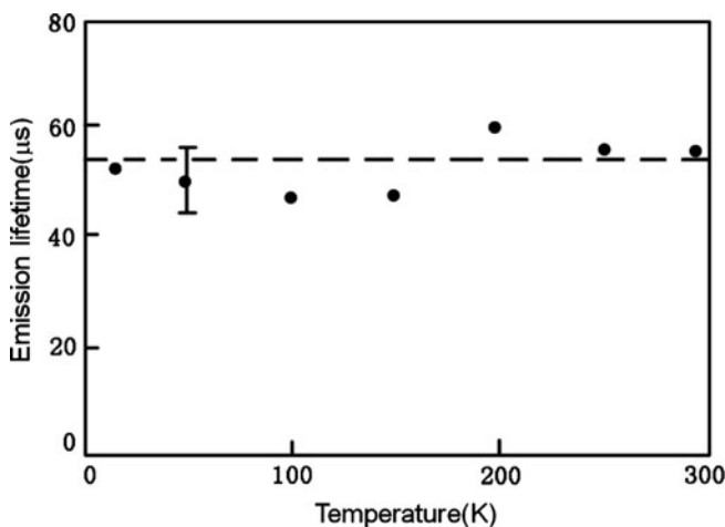
Fig. 8.40 The relationship between emission lifetime and temperature of \text{Cr:LiSAF}
