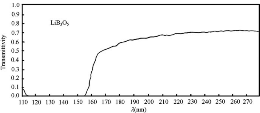
Fig. 1.56 The ultraviolet transmittivity character of LBO crystal
