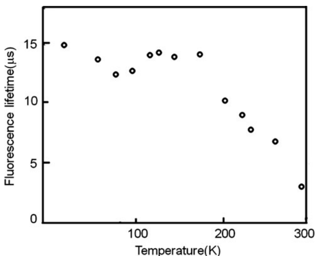
Fig. 8.20 The influence of temperature on fluorescence lifetime of Cr:Mg 2 SiO 4
