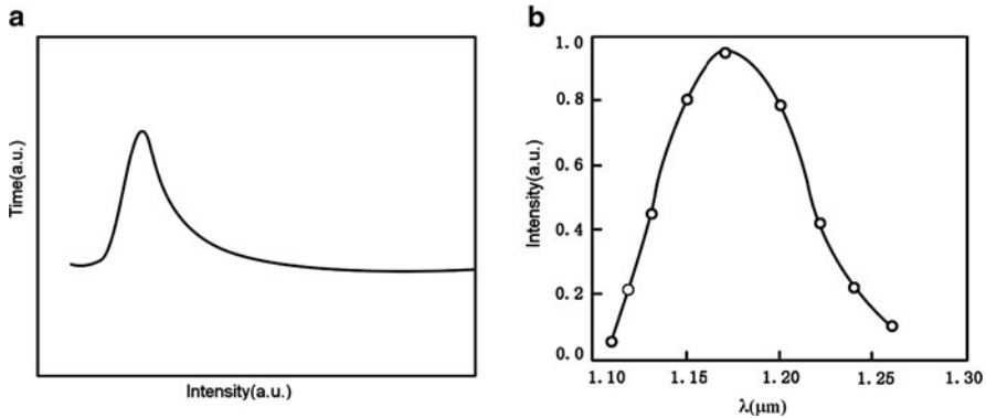
Fig. 8.55 (a) The beam profile and (b) the tuning curve of \text{LiF:F}_2^- laser
