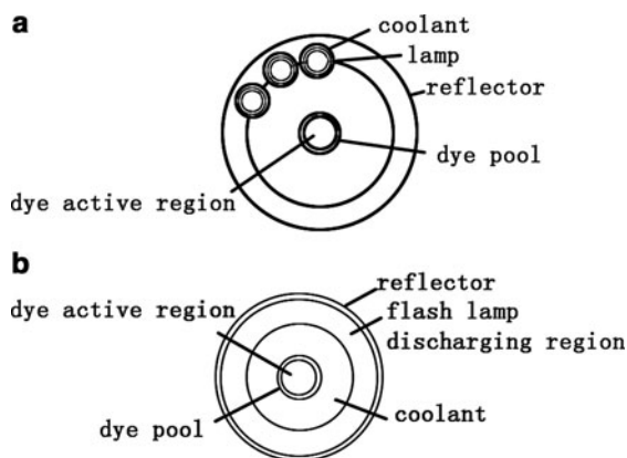
Fig. 10.11 The structure of dye laser condensing cavity pumped by flash lamp: (a) straight-tube lamp and (b) coaxial lamp
