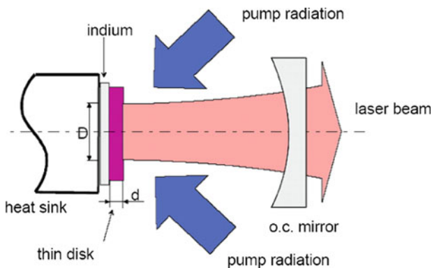
Fig. 7.33 Model of thin disk DPL
