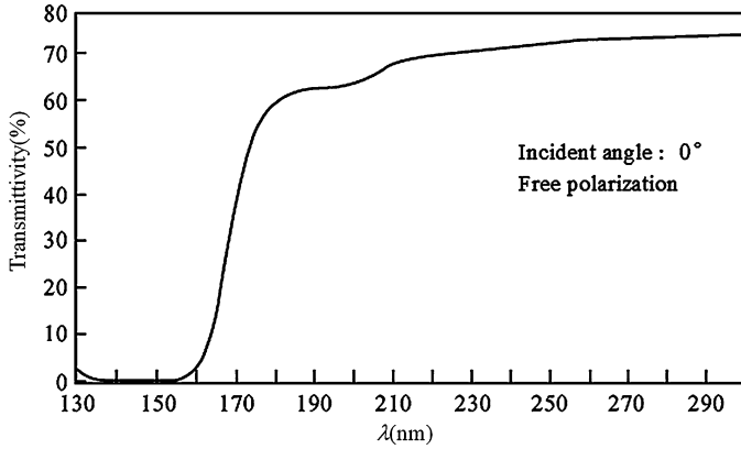
Fig. 1.74 The ultraviolet band transparent spectrum of KBBF
