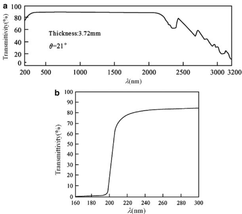
Fig. 1.52 The transmittivity curve of BBO crystal (a) 200–3200 nm; (b) 160–300 nm. (the sample thickness is 3.72 mm, type-I phase matching)
