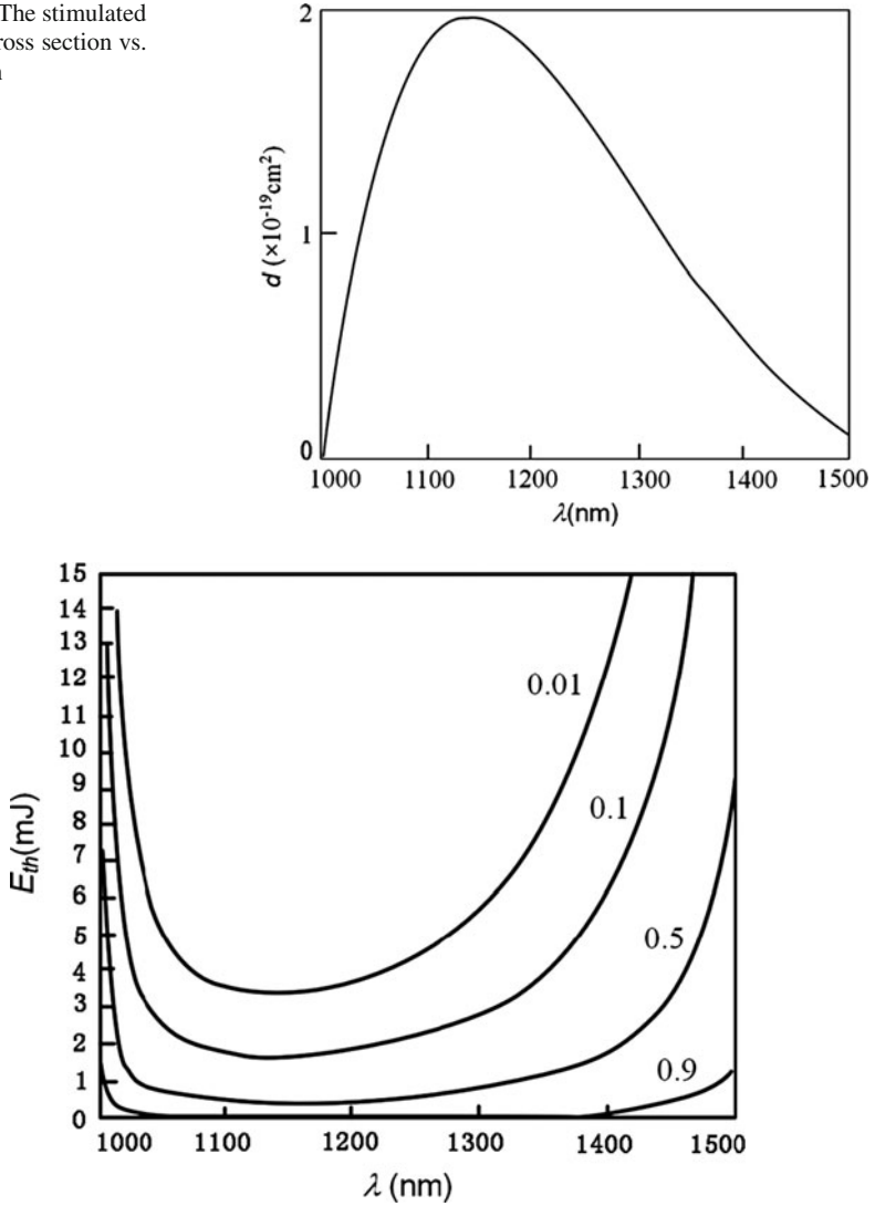
Fig. 8.22 The pumping threshold energy vs. wavelength under different R(\lambda_p = 1.064 \mu\text{m})
