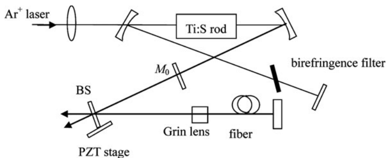
Fig. 9.83 Additive pulse mode-locking (APM) Ti:sapphire laser
