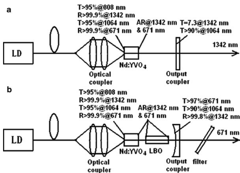
Fig. 7.6 Experimental setup of (a) high power 1,342-nm laser and (b) high power intracavity frequency-doubled red laser
