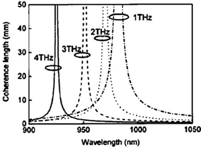
Fig. 6.26 Calculated coherence length L_c vs. the input wavelength \lambda_1
