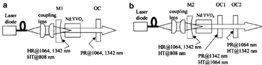
Fig. 6.19 Two experiment setups of the laser cavity for simultaneous oscillation at 1,064 and 1,342 nm
