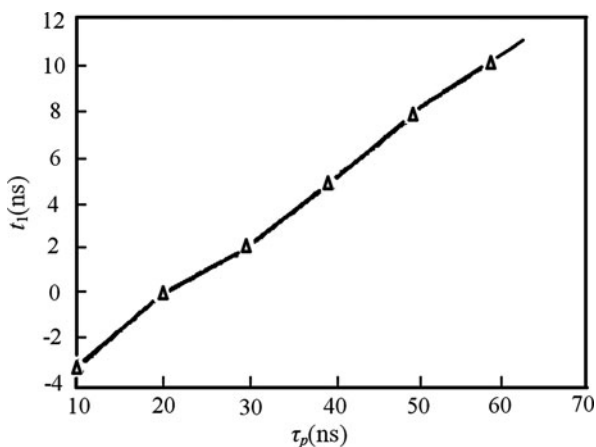
Fig. 4.10 Relationship between the pulse width and the starting time of the pulse delay
