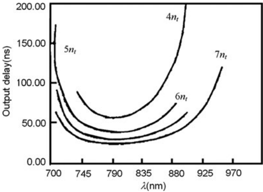
Fig. 9.74 Output delay time vs. wavelength at different pump energy
