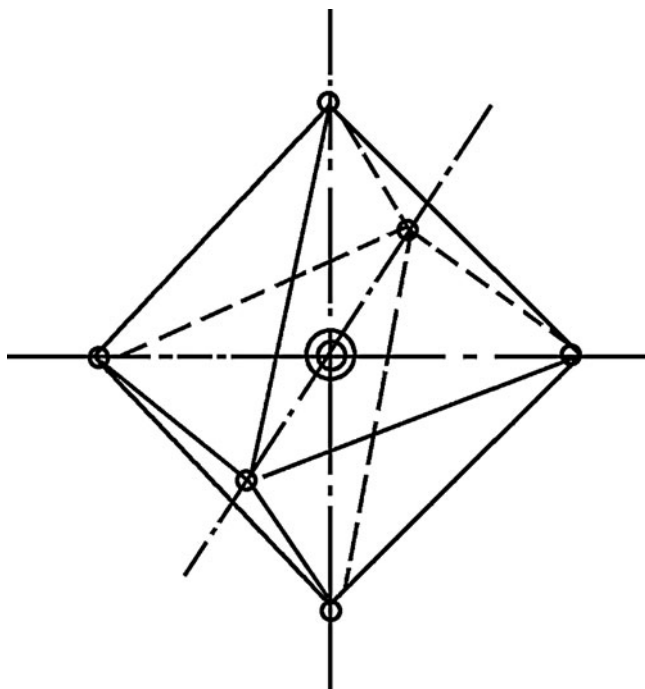
Fig. 9.1 Structure of Ti:sapphire crystal
