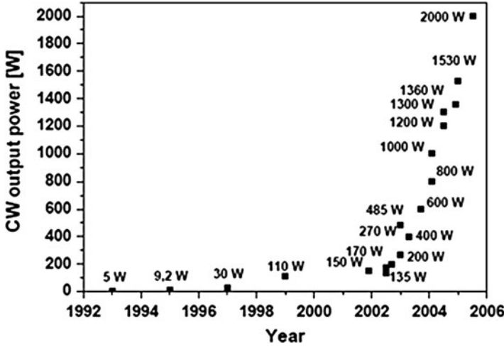
Fig. 7.40 Power evolution of CW double-clad fiber lasers with diffraction-limited beam quality over the last decade
