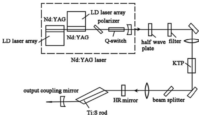
Fig. 9.103 All-solid-state Ti:sapphire laser
