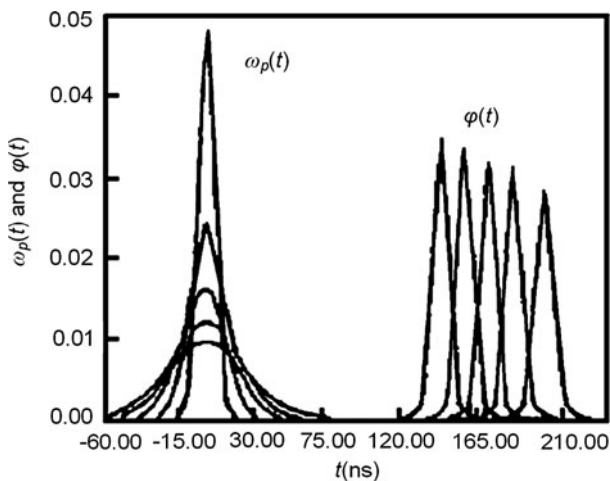
Fig. 9.64 Output pulse at pump pulse width of 10–50 ns and energy of 2.5n_l
