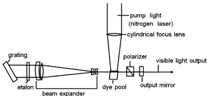
Fig. 10.9 The typical pulsed dye laser cavity
