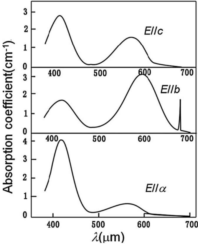
Fig. 8.8 Absorption spectrum of Cr : BeAl 2 O 2
