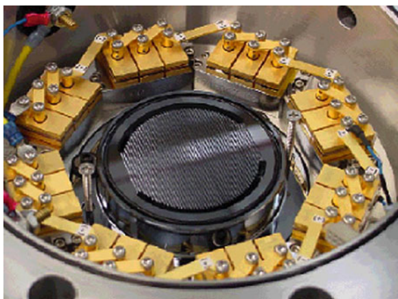
Fig. 7.39 Diodes edge-pumping thin disk DPL
