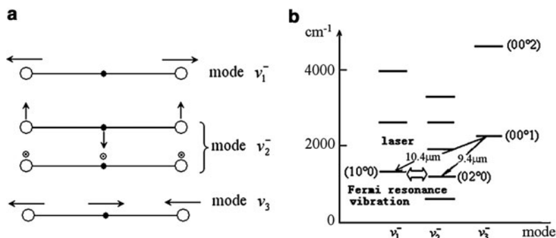
Fig. 10.20 (a) The vibration mode of CO 2 and (b) its energy level diagram
