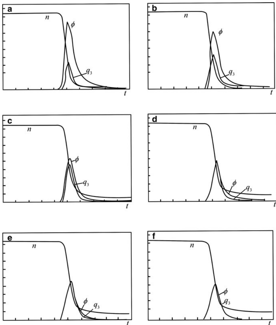
Fig. 3.2 Photon number density \phi, q_3 and population inversion density n of fundamental and harmonic waves under different crystal length (200 ns/lattice, Y_0 = 1 ). (a) l = 1 mm, (b) l = 1.5 mm, (c) l = 3 mm, (d) l = 4 mm, (e) l = 5 mm, (f) l = 10 mm
