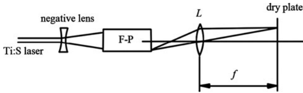
Fig. 9.22 The setup for laser linewidth measurement
