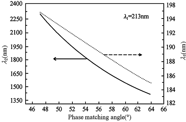
Fig. 1.72 Ultraviolet (193 nm) sum frequency phase-matching curves
