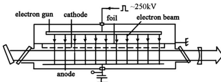
Fig. 10.28 The diagram of electron-beam-controlled TE-CO 2 laser
