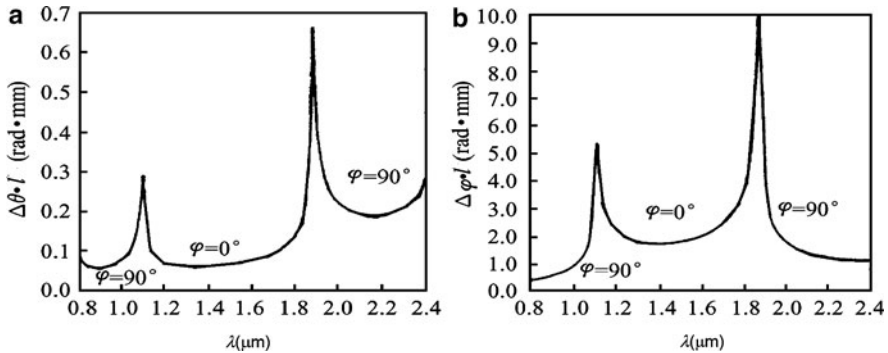
Fig. 1.24 The acceptance angles (a) \Delta\theta and (b) \Delta\varphi of frequency doubling in LBO crystal
