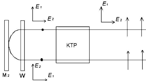
Fig. 3.8 Effect of quarter wave plate ( W ) on phase compensation
