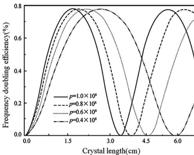
Fig. 1.68 Type-II SHG conversion efficiency vs. crystal length with different fundamental wave intensity
