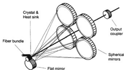
Fig. 7.34 Additional absorption passes through the disk laser medium
