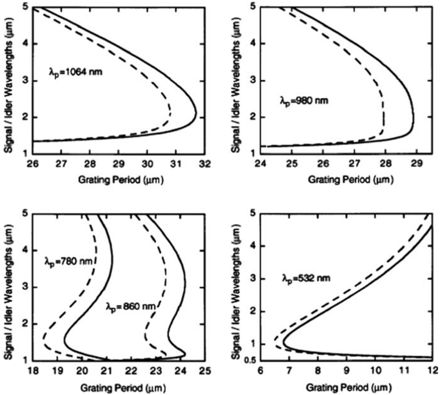
Fig. 5.26 First-order QPM periods for collinear PPLN OPO with different wavelengths. All the waves are polarized parallel to the crystal axis. The solid curves are at 25°C, and the dashed curves are at 200°C.
