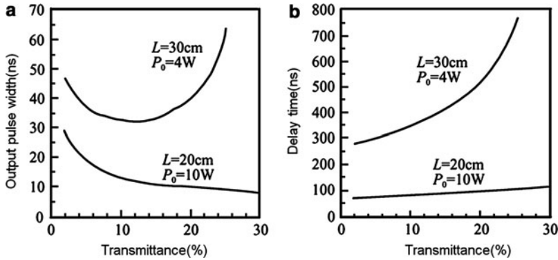
Fig. 9.34 (a) The output pulse width and (b) delay time varied with the output mirror transmittance
