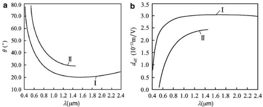
Fig. 1.55 OPO angle tunable curves in BBO crystal: (a) Type-I phase match and (b) Type-II phase match
