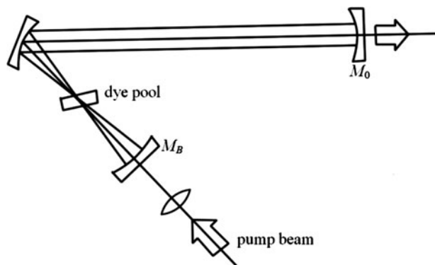
Fig. 10.7 The three-mirror folded cavity structure
