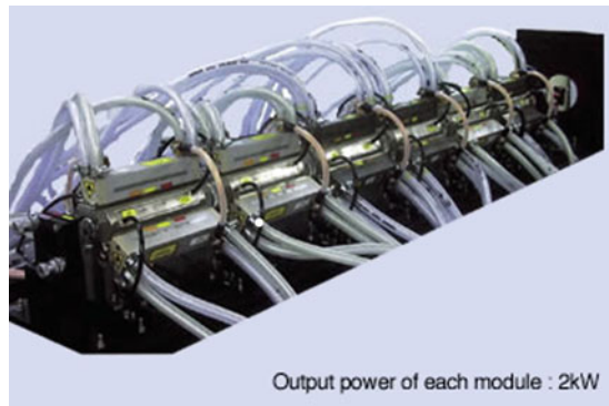
Fig. 7.27 The multirod DPL (10 kW)
