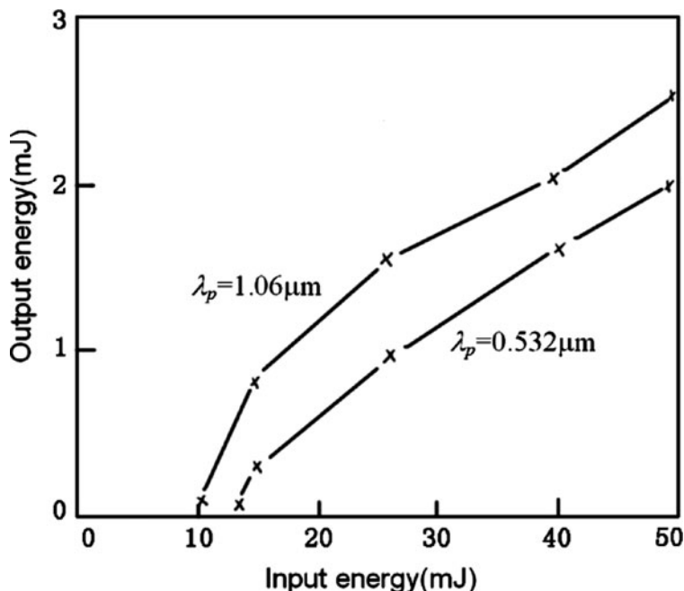
Fig. 8.36 The output characteristic curve of Cr:Mg 2 SiO 4 laser
