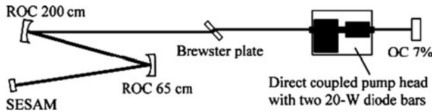
Fig. 6.23 Experimental setup of the 10.7 W ps Nd:YAG laser
