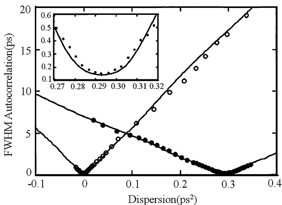
Fig. 5.47 Input ( open circles ) and output ( filled circles ) autocorrelation widths with the chirp of the input pulse (expressed in terms of delay line GVD) for SHG in a chirped QPM grating. The inset shows the output-pulse autocorrelations near maximum compression point.
