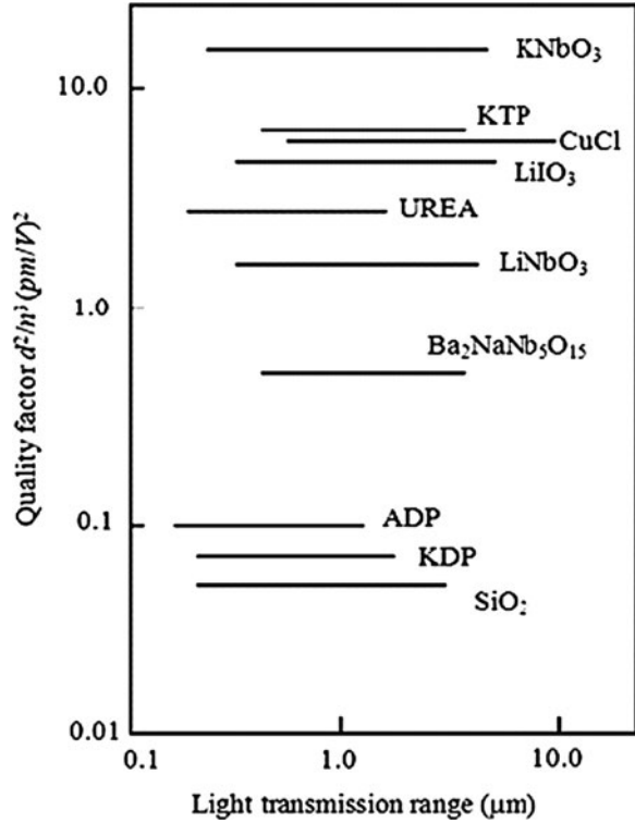
Fig. 1.61 The quality factor (FOM) of several crystal in common use
