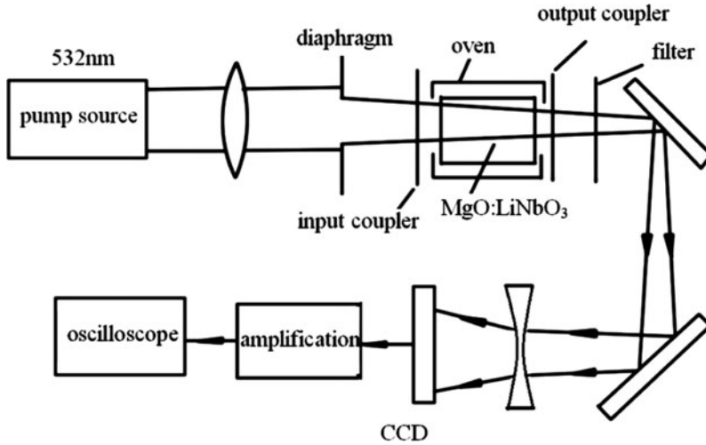
Fig. 4.51 The measurement setup of transverse parametric energy
