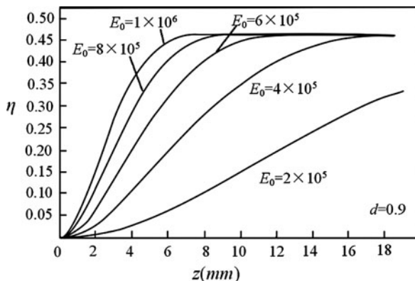
Fig. 2.1 Relation of frequency doubling efficiency, fundamental wave field intensity and crystal length
