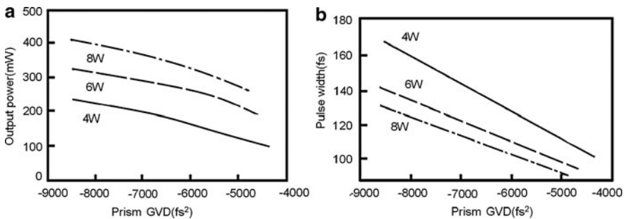
Fig. 9.95 (a) Output power and (b) pulse width as a function of GVD in prism at different pump power
