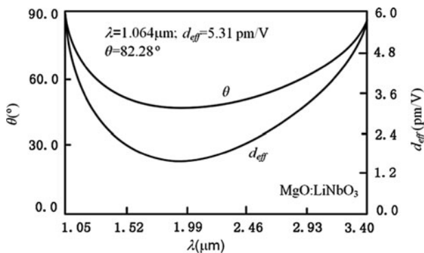
Fig. 4.35 Variation of the phase matching angle \theta and d_{\text{eff}} with the wavelength in MgO : LiNbO 3 SHG
