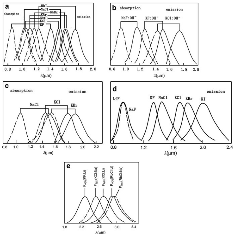
Fig. 8.45 The absorption and fluorescent spectra of several kinds of main color center: (a) The absorption and emission bands of F_A(Tl) center (77 K). (b) The absorption and emission bands of (F_2^+)^{**} center. (c) The absorption and emission bands of (F_2^+)_H center (77 K). (d) The absorption and emission bands of F_2^+ center. (e) Several II color center emission bands.
