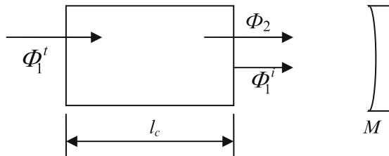
Fig. 3.17 Schematic diagram of fundamental and harmonic waves going into and out of crystal
