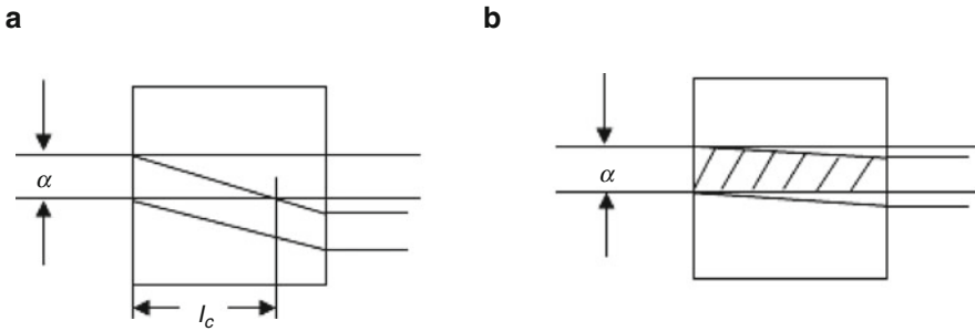
Fig. 1.36 The walk-off effect in nonlinear crystal (a) l > l_c ; (b) l \ll l_c
