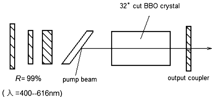
Fig. 4.20 Narrow linewidth BBO-OPO system with intracavity etalon
