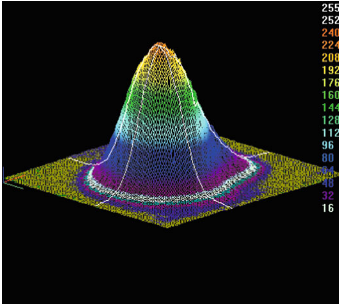
Fig. 7.14 The distribution of green beam at 110-W green output power
