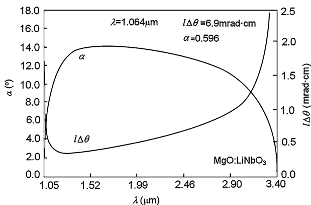
Fig. 4.37 Relationship between walk-off angle \alpha , acceptance angle \Delta\theta \cdot l and the wavelength
