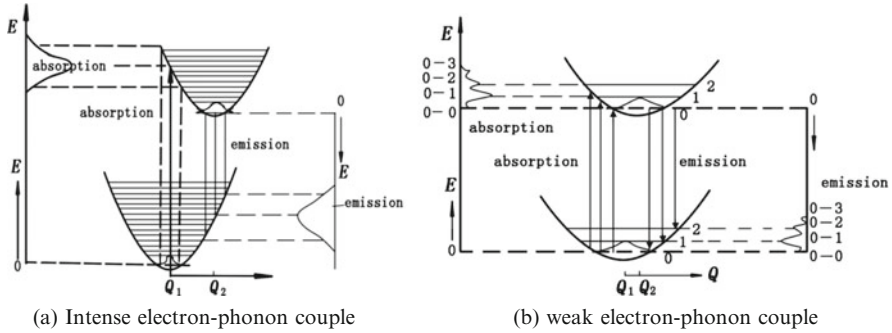
Fig. 8.44 The Frank–Condon coordinate chart of color center: (a) intense electron–phonon couple and (b) weak electron–phonon couple
