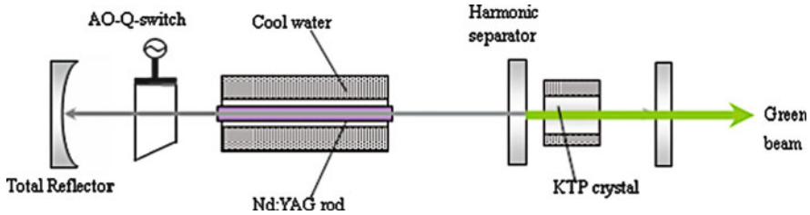
Fig. 7.11 The high power green laser.
