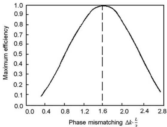
Fig. 4.19 The maximum conversion efficiency in SRO vs. phase mismatching (under low-gain condition)
