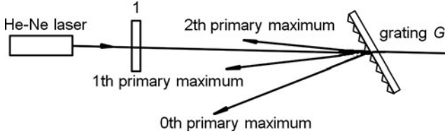
Fig. 8.53 The diagrammatic sketch of grating tuning
