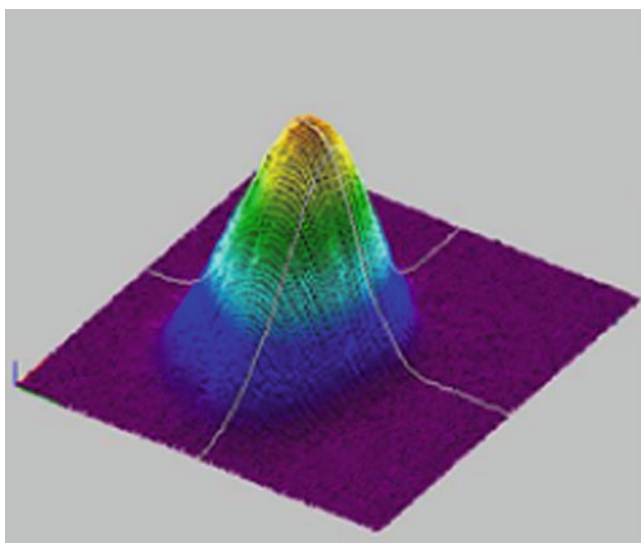
Fig. 7.4 Beam profile of the 8.5-W red DPL
