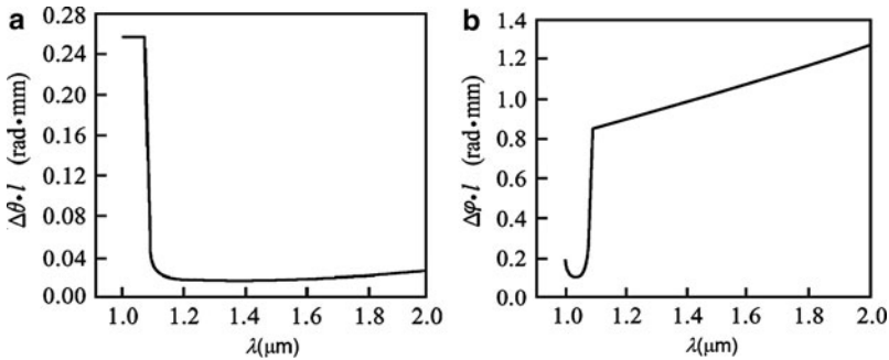
Fig. 1.23 The acceptance angles (a) \Delta \theta and (b) \Delta \varphi of frequency doubling in KTP crystal (type-II phase matching)
