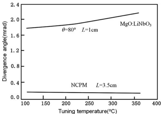
Fig. 4.43 The acceptance divergence angle in MgO : LiNbO 3 -SRO
