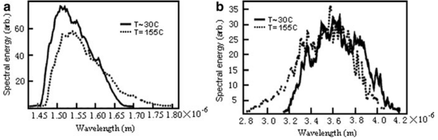
Fig. 5.36 (a) Collinear signal and (b) idler spectra
