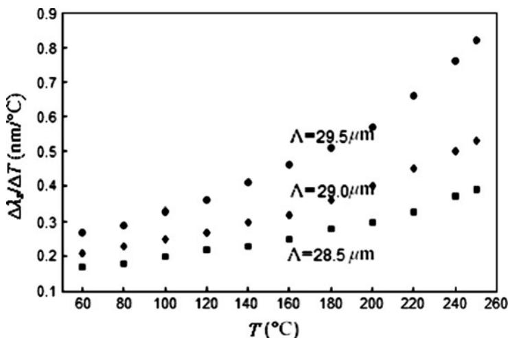
Fig. 5.7 Calculated signal wavelength change rate vs. the crystal temperature for 1,064-nm pumped PPLN–OPO
