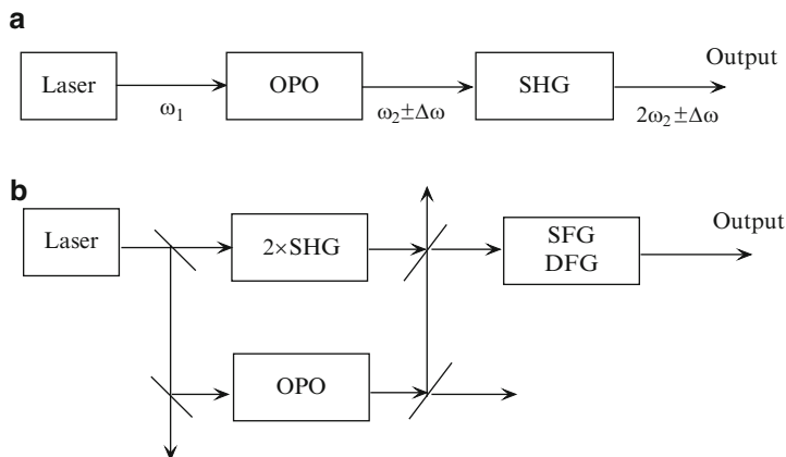
Fig. 4.59 The combination of tuning methods
