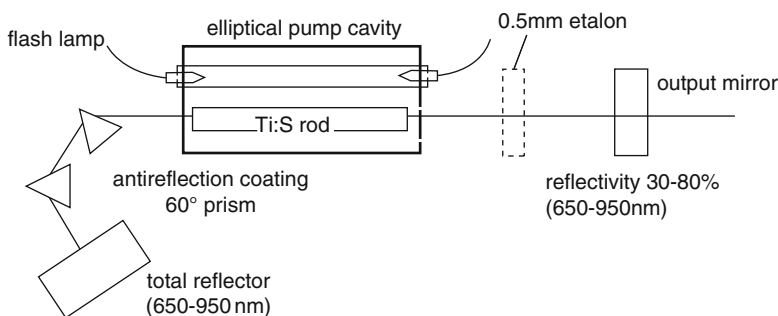
Fig. 9.51 Experimental setup of flash lamp-pumped Ti:sapphire laser
