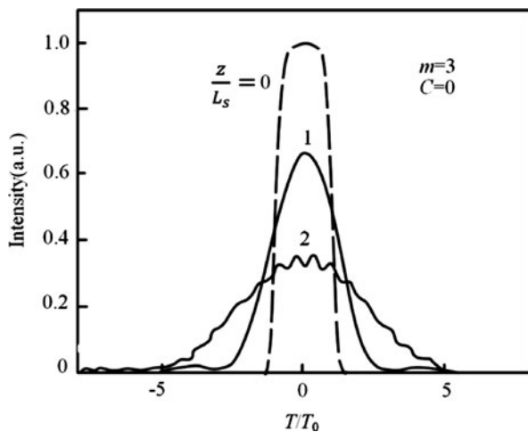
Fig. 3.36 Super-Gaussian pulse shapes at the positions of z = L_s and z = 2L_s
