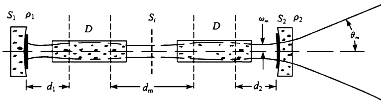
Fig. 6.6 The two-rod resonator
