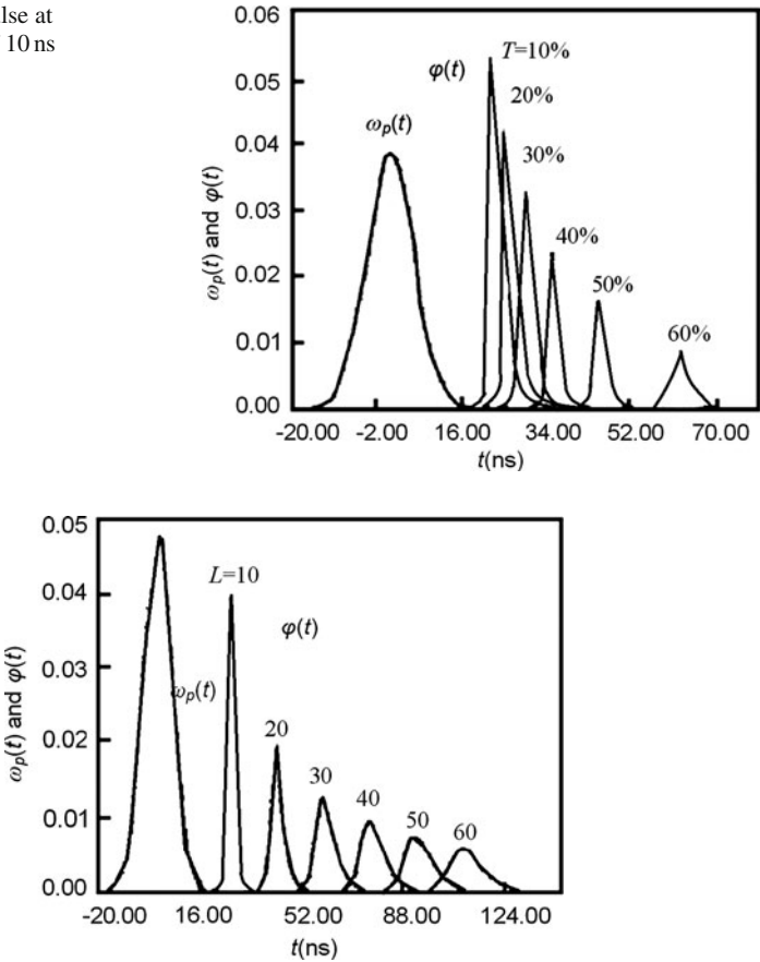
Fig. 9.69 Output pulse at pump pulse width of 10 ns, energy of 5n_t , and L = 10\text{--}60 cm
