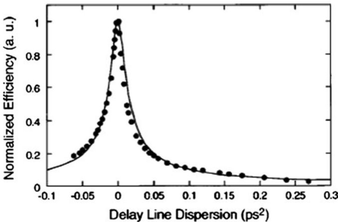
Fig. 5.48 Normalized efficiency with delay line dispersion
