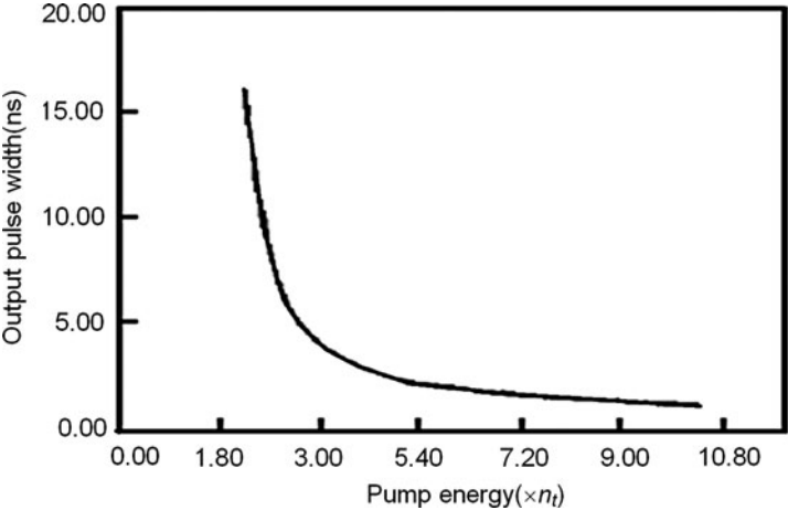
Fig. 9.62 The output pulse width vs. pump energy at pump pulse width of 10 ns
