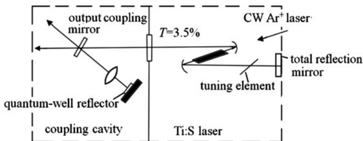
Fig. 9.85 Coupled-cavity resonant passively mode-locking laser with a quantum well reflector
