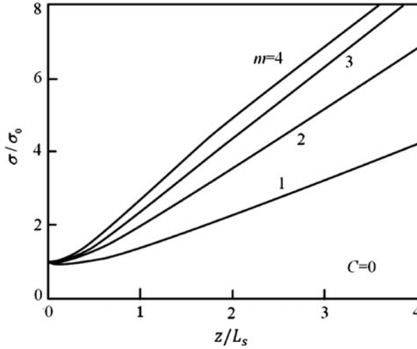
Fig. 3.37 Broadening factor of super-Gaussian pulse at different values of m
