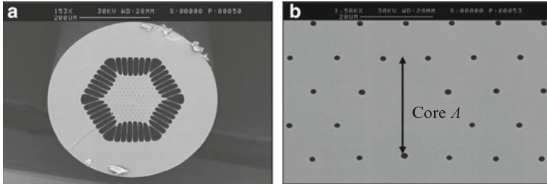
Fig. 7.53 Scanning electron microscope images of (a) the air-clad ytterbium-doped large-mode-area fiber and (b) close-up of core region
