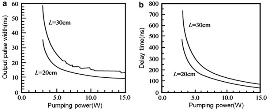
Fig. 9.29 (a) The output pulse width and (b) the delay time as a function of average pump power
