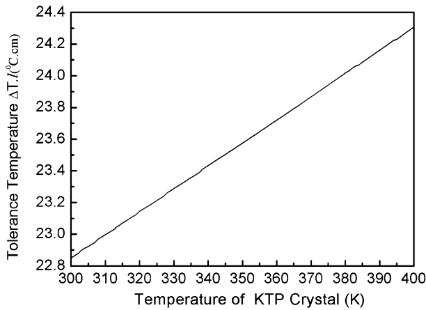
Fig. 7.9 The temperature bandwidth \Delta T \cdot l of type-II KTP as a function of temperature
