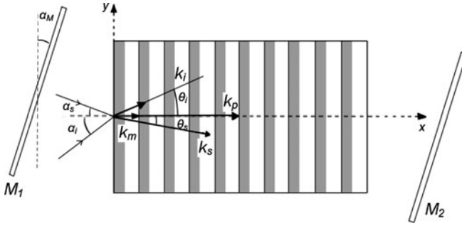
Fig. 5.15 The definitions of various wave vectors and angles in signal resonance OPO
