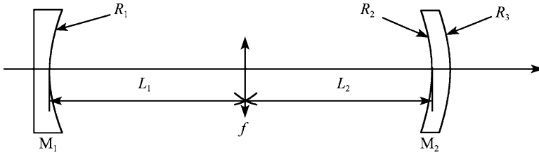
Fig. 6.2 The diagram of the equivalent resonator
