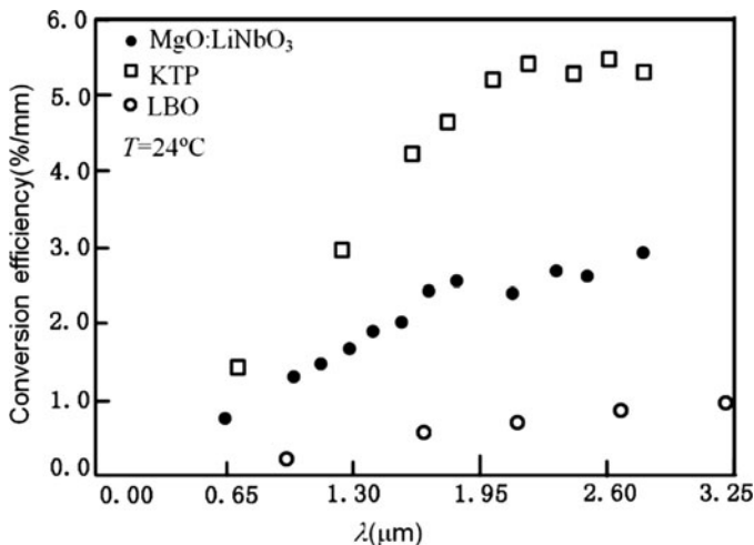
Fig. 4.38 The efficiency curves of MgO : LiNbO 3 , KTP, and LBO (experimental results)
