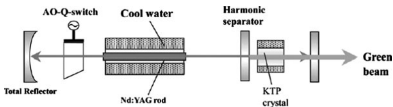
Fig. 6.21 Schematic diagram of the high power acousto-optic Q-switched green laser
