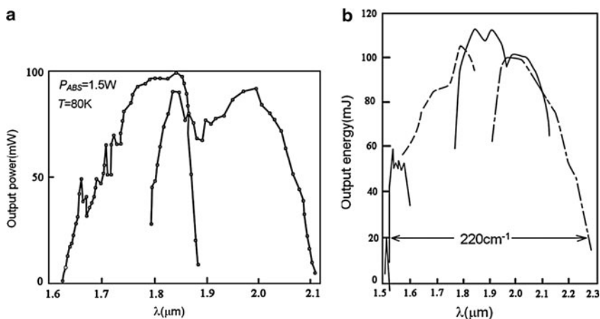
Fig. 8.5 The output characteristics of \text{Co}^{2+}:\text{MgF}_2 laser under: (a) CW operation and (b) pulse operation
