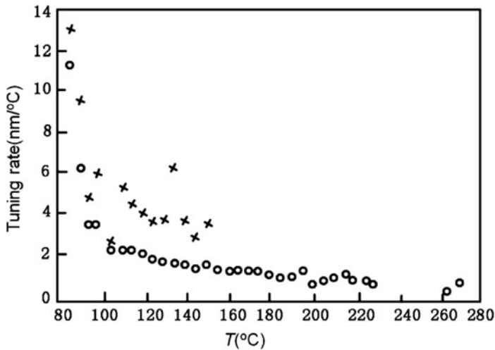
Fig. 4.47 Tuning rate (×-idler wave, o-signal wave)
