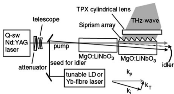
Fig. 4.58 Schematic of setup used for injection-seeded TPG
