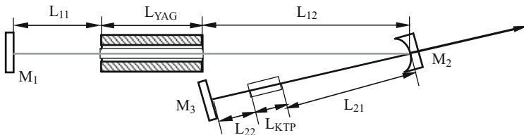
Fig. 7.15 The side-pumped CW green SHG DPL with a plane-concave-plane cavity
