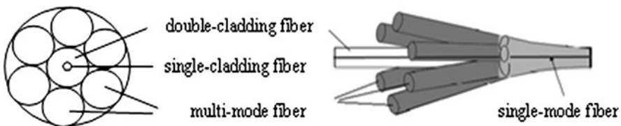
Fig. 7.42 Fused taper side-pumping
