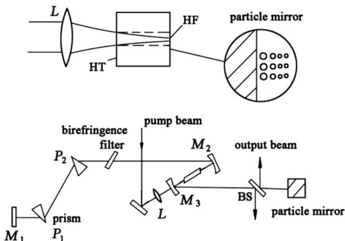
Fig. 9.87 The structure of microdot mirror modulator
