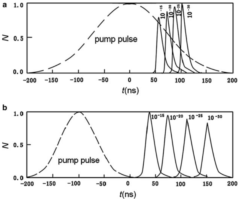
Fig. 9.25 The pump and output pulse shape at different \beta . (a) L = 20 cm, P_0 = 10 W; (b) L = 30 cm, P_0 = 4 W
