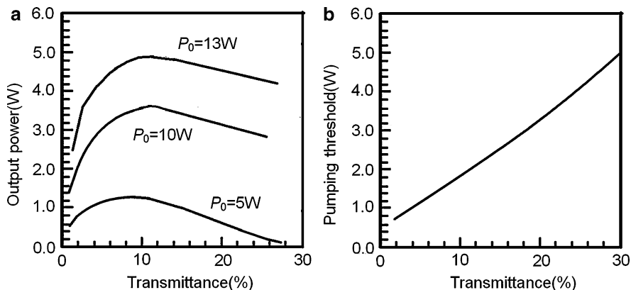
Fig. 9.14 (a) Output power and (b) pump threshold vs. the output transmittance under different pumping power
