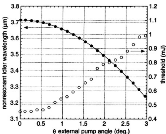
Fig. 5.21 PPLN OPO idler wavelength and threshold vs. external pump angle
