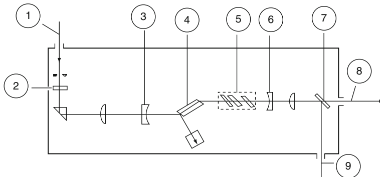
Fig. 9.52 Experimental setup of Ti:sapphire laser employing birefringence filter. (1) pump light (532 nm), (2) \lambda/2 filter, (3) total reflection mirror, (4) Ti:sapphire rod, (5) birefringence filter, (6) output mirror, (7) beam splitter, (8) output laser, (9) wavelength monitor
