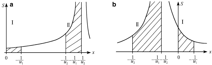
Fig. 6.5 Misalignment sensitivity S vs. 1/f of the lens. (a) |u_1| \gg |u_2| and (b) |u_1| \approx |u_2|
