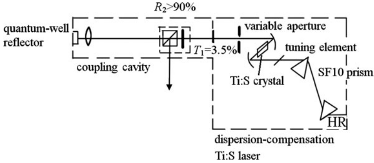
Fig. 9.91 The self-mode-locked Ti:sapphire laser with coupled cavity starting using quantum-well reflector
