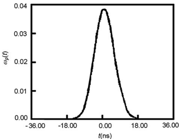
Fig. 9.57 Pump pulse shape at t = 10 ns, b = 5
