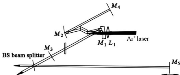
Fig. 9.86 Linear external cavity auxiliary mode-locking laser
