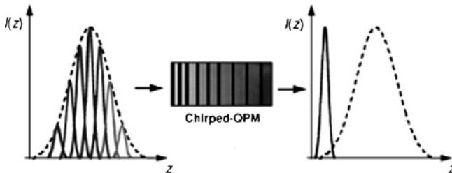
Fig. 5.4 Time-domain representation of pulse compression during SHG in aperiodic QPM gratings. Different shadings correspond to the optical frequency of each temporal slice of the fundamental pulse ( dashed curve ) and to the optical frequency for which SHG is quasi-phase matched in each spatial region of the aperiodic QPM grating
