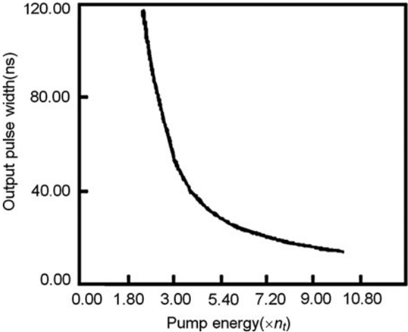
Fig. 9.62 The output pulse width vs. pump energy at pump pulse width of 10 ns
