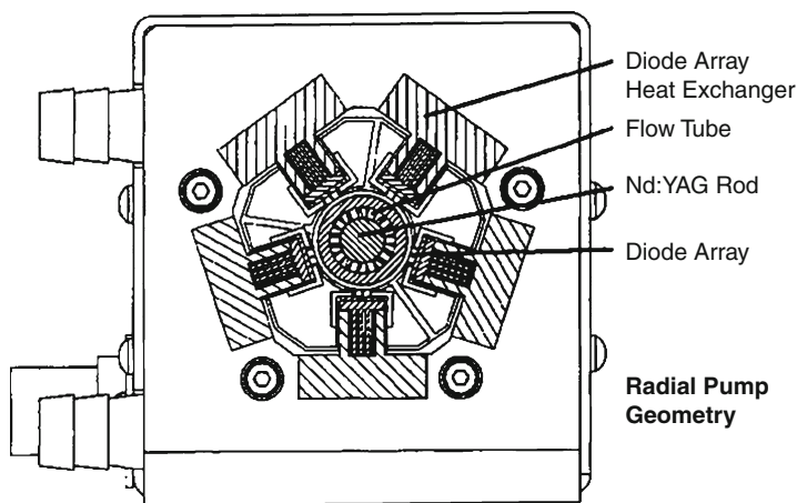
Fig. 7.24 The cross section of pumping module
