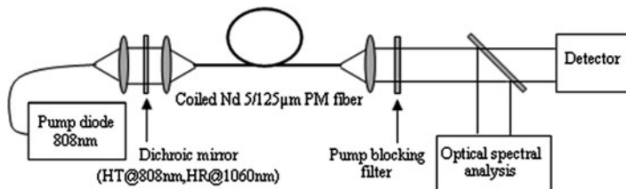
Fig. 7.45 The experimental setup of double-cladding PMF laser
