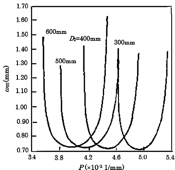
Fig. 3.15 Schematic of stable zone when changing D_2 and fixing D_1 = 500
