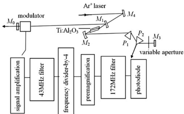
Fig. 9.90 The schematic of the regenerative self-mode-locked Ti:sapphire laser based on acousto-optic modulation
