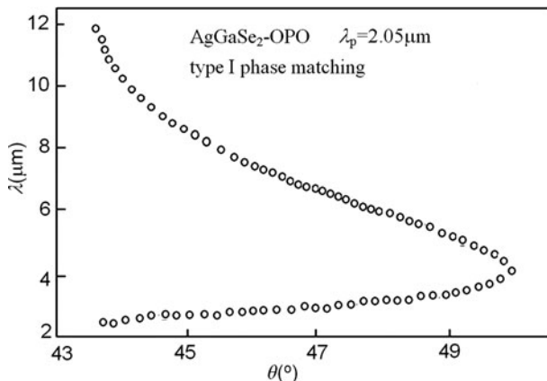
Fig. 4.28 AgGaSe 2 -OPO tuning curve ( \lambda_p = 2.05\mu\text{m} , type-I phase matching)
