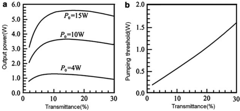
Fig. 9.39 (a) Output power and (b) pump threshold vs. transmittance of output mirror for different pump power
