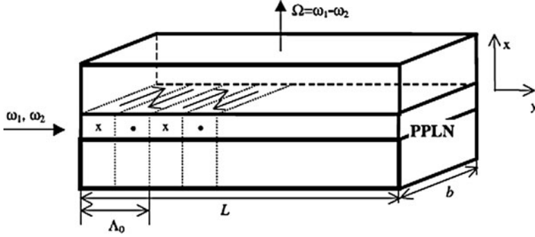
Fig. 6.29 The scheme of surface-emitted DFG in planar PPLN waveguide
