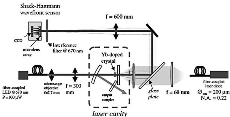
Fig. 6.13 Experimental setup used for thermal lens measurement
