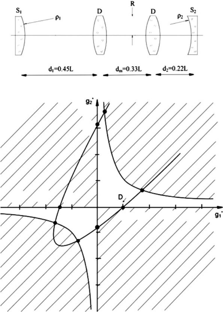
Fig. 6.7 For two rods resonator, the resonator moves with increasing refractive power on a parabola with eight points of instability
