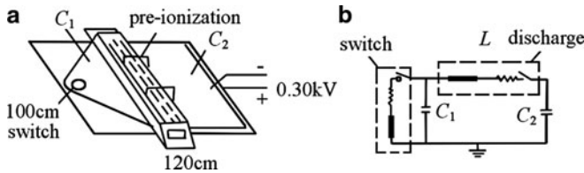
Fig. 10.35 (a) The diagram of quick discharge and (b) its equivalent circuit
