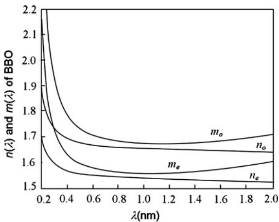
Fig. 3.30 n(\lambda) and m(\lambda) of BBO crystal
