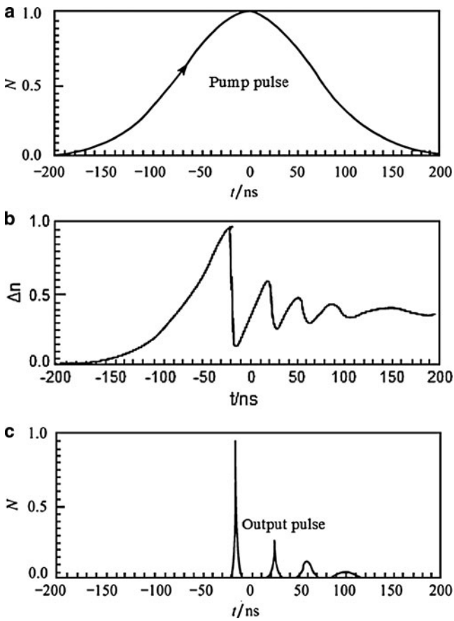
Fig. 9.33 (a) Pump pulse, (b) population inversion and (c) photon density in cavity as a function of time
