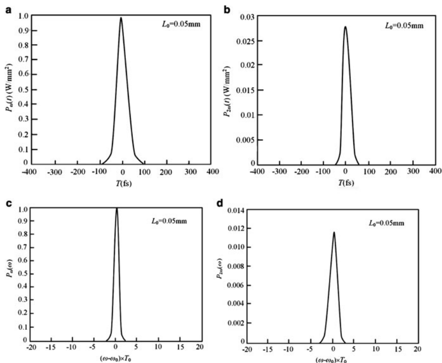
Fig. 3.40 Time and frequency spectra of the fundamental and harmonic wave power after BBO crystal ( l = 0.05 mm) (a) time spectrum of the fundamental wave; (b) time spectrum of the harmonic wave; (c) frequency spectrum of the fundamental wave; (d) frequency spectrum of the harmonic wave
