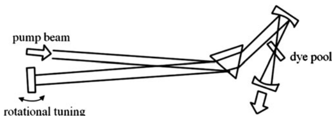
Fig. 10.8 The three-mirror folded cavity with prism tuning
