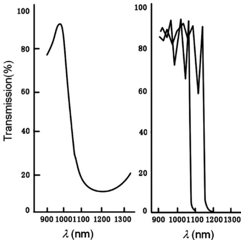
Fig. 8.35 The transmission curves of two cavity mirrors: (a) half-reflection and (b) total reflection
