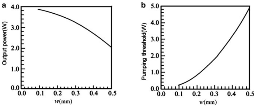
Fig. 9.40 (a) Output power and (b) pump threshold as a function of beam radius
