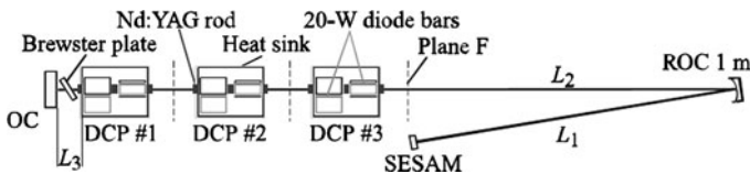
Fig. 6.24 Experimental setup for 27 W ps Nd:YAG laser
