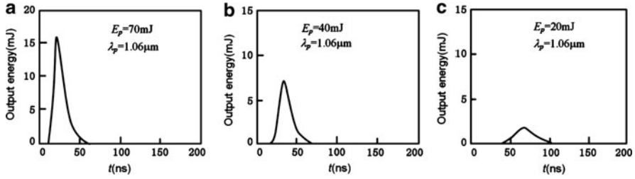
Fig. 8.28 The output characteristic with different pumping energy when pumped by 1.064 \mu\text{m} . (a) E_p = 70 \text{ mJ} ; (b) E_p = 40 \text{ mJ} ; and (c) E_p = 20 \text{ mJ}
