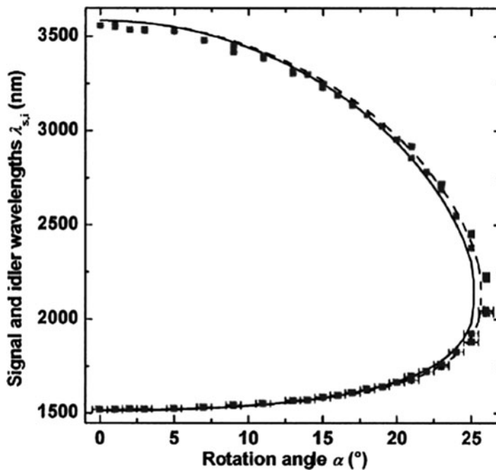
Fig. 5.25 Spectral tuning curve as a function of the revolution angle, \alpha . The filled squares are the experimental points, the solid curve and the dashed curve are accurate and approximate theoretical predictions, respectively.
