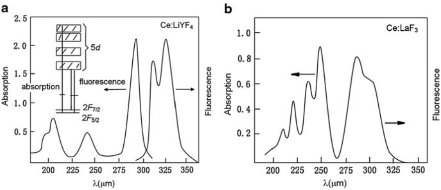
Fig. 8.6 Absorption spectra (a) and fluorescent spectra (b) of Ce 3+ :LiYF 4 and Ce 3+ :LaF 3
