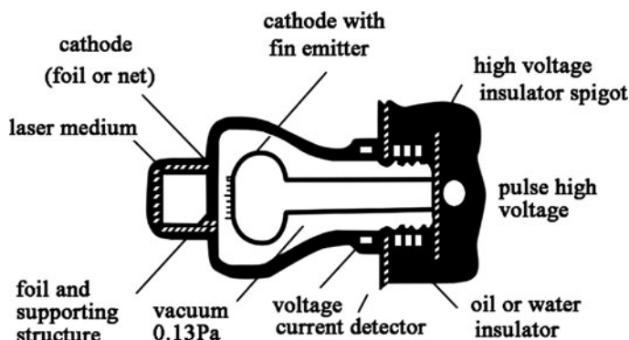
Fig. 10.33 The diagram of electron beam pumped excimer laser
