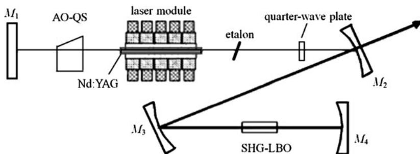
Fig. 7.5 The 28-W side-pumped red DPL
