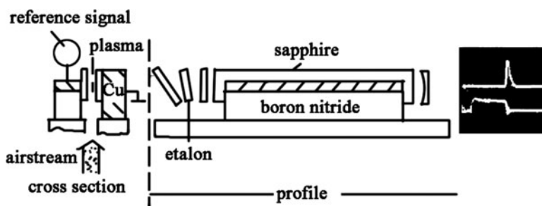
Fig. 10.29 The diagram of radio-frequency-excited waveguide CO 2 laser and the output pulse of gain switch
