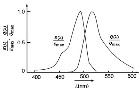
Fig. 10.3 The absorption and fluorescence spectra of fluorescein sodium solution
