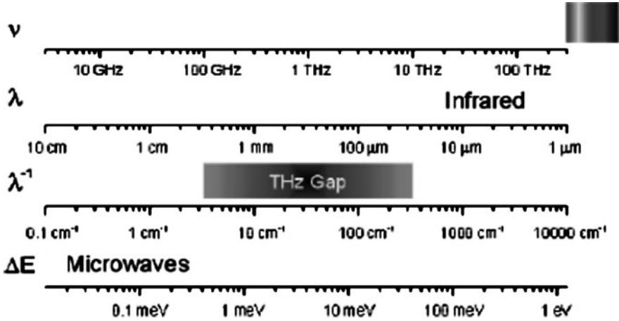
Fig. 4.52 Spectral range of THz electromagnetic wave.
