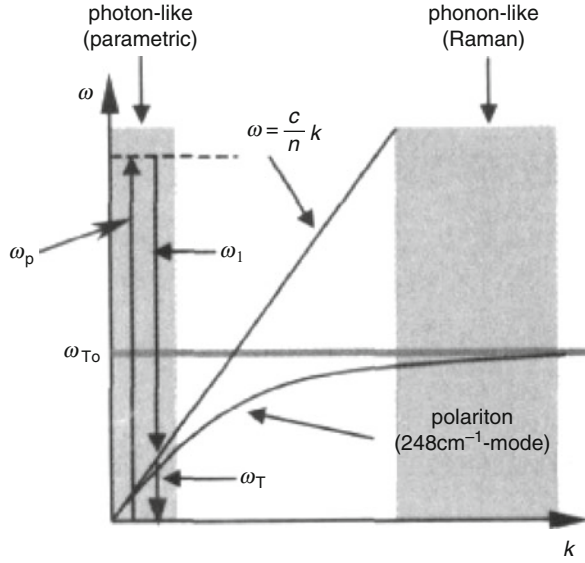
Fig. 4.53 Dispersion characteristic of polariton
