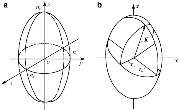
Fig. 1.2 Biaxial crystal refractive index ellipsoid (a) refractive index ellipsoid and (b) the case of giving vector \mathbf{K}
