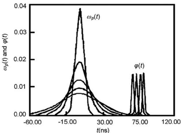
Fig. 9.65 Output pulse at pump pulse width of 10–50 ns and energy of 5n_l
