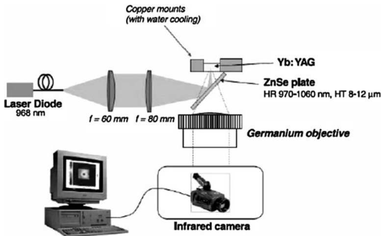
Fig. 6.14 Experimental setup of temperature measurement of focal length of the thermal lens
