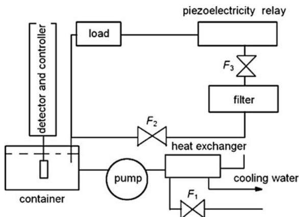
Fig. 3.20 Schematic diagram of water cooling system
