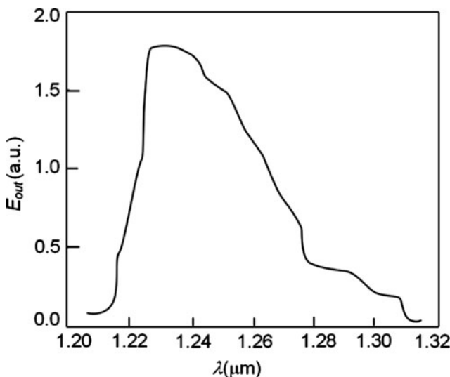
Fig. 8.37 The tuning curve of Cr:Mg 2 SiO 4 laser
