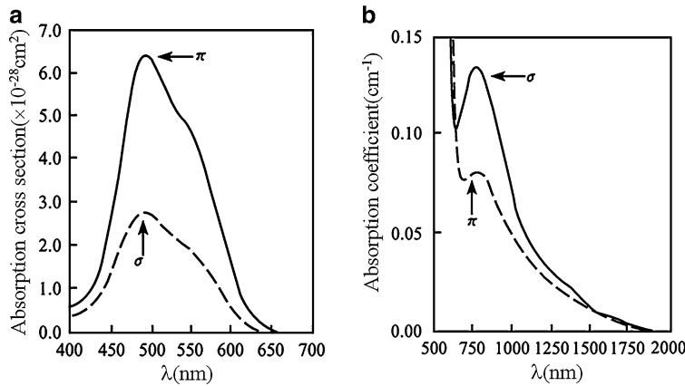
Fig. 9.5 (a) The blue-green absorption spectrum and (b) infrared absorption spectrum of the Ti:sapphire crystal
