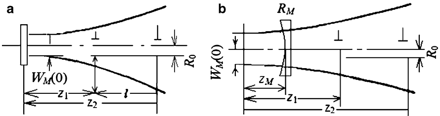
Fig. 2.12 Schematic diagram of M coefficient measurement, output mirror is a plane (a) or concave (b) mirror
