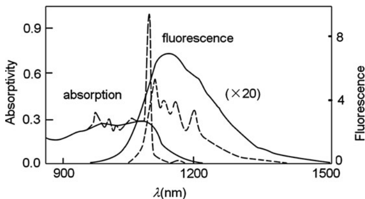
Fig. 8.19 The absorption spectrum and fluorescence spectrum of Cr:Mg 2 SiO 4 at different temperature
