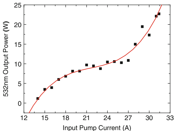
Fig. 7.15 The side-pumped CW green SHG DPL with a plane-concave-plane cavity
