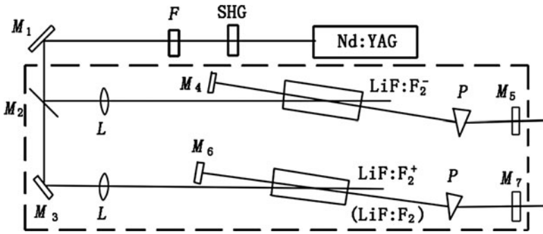
Fig. 8.57 The experiment setup for wide tuning
