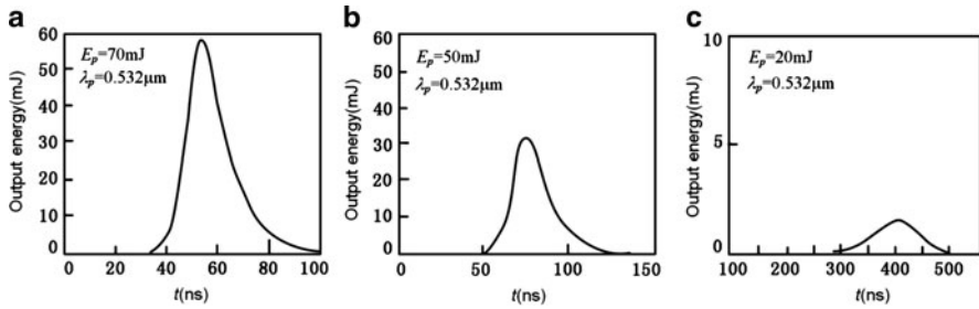
Fig. 8.29 The output characteristic with different pumping energy when pumped by 0.532 \mu\text{m} . (a) E_p = 70 \text{ mJ} ; (b) E_p = 50 \text{ mJ} ; and (c) E_p = 20 \text{ mJ}
