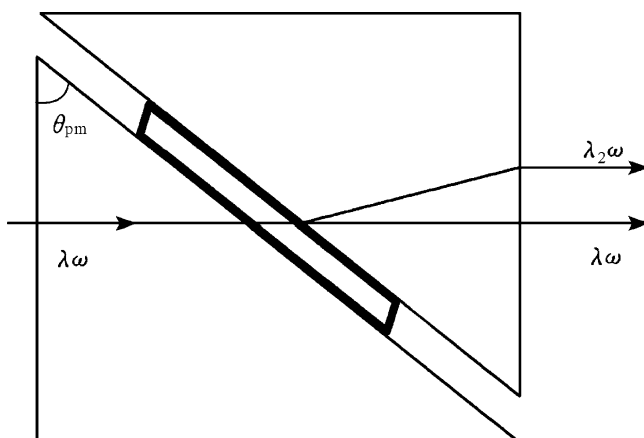
Fig. 1.77 The sketch map of prism coupling of KBBF
