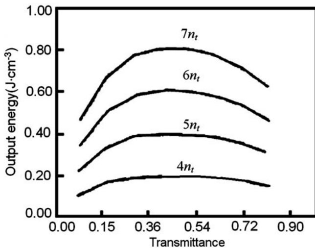
Fig. 9.75 Output energy vs. the transmittance at different pump energy
