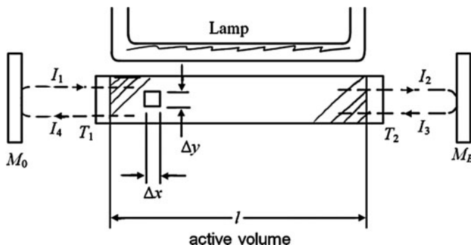
Fig. 10.12 The resonant cavity of flashlamp-pumped dye laser
