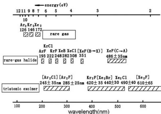
Fig. 10.30 The frequency range and central wavelength of excimer laser
