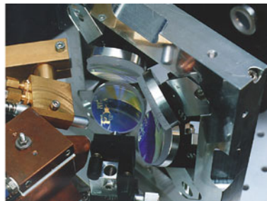
Fig. 7.34 Additional absorption passes through the disk laser medium
