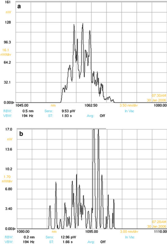
Fig. 7.47 Spectrum of PMF laser (a) fine structure of spectrum at 1,060 nm and (b) fine structure of spectrum at 1,092 nm
