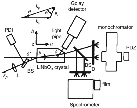
Fig. 4.55 The angle surface coupler for THz-wave output
