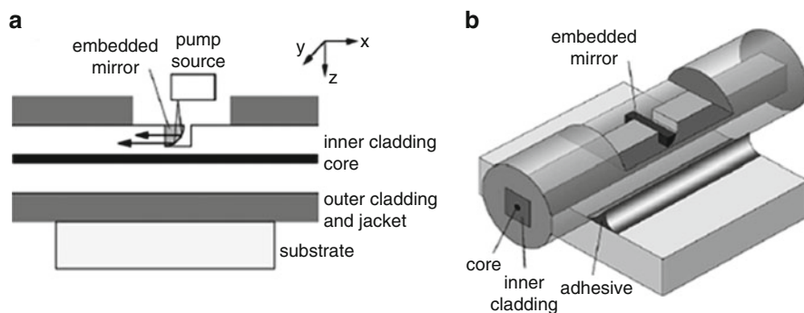
Fig. 7.43 The embedded-mirror side pumping: (a) cross-sectional side view and (b) three-dimensional view
