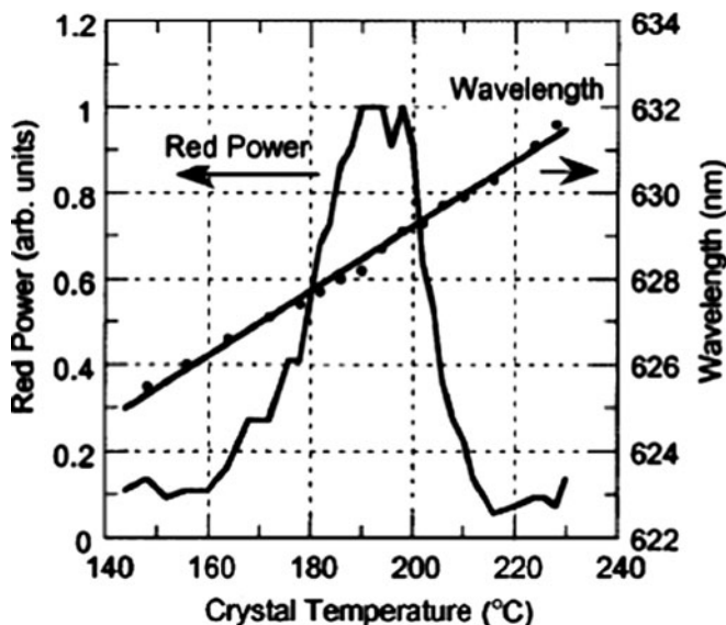
Fig. 5.29 Red power and output wavelength for the SFG–OPO device. The two gratings operate optimally at 195°C with a relatively broad temperature span of 10°C. Broader tuning is available if the grating periods are varied.
