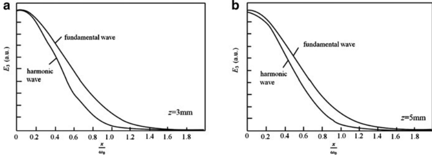
Fig. 2.4 Compression phenomenon of frequency doubling beam transverse distribution, E_0 = 1 \times 10^6 V/m, d = 0.9 (a) z = 3 mm; (b) z = 5 mm
