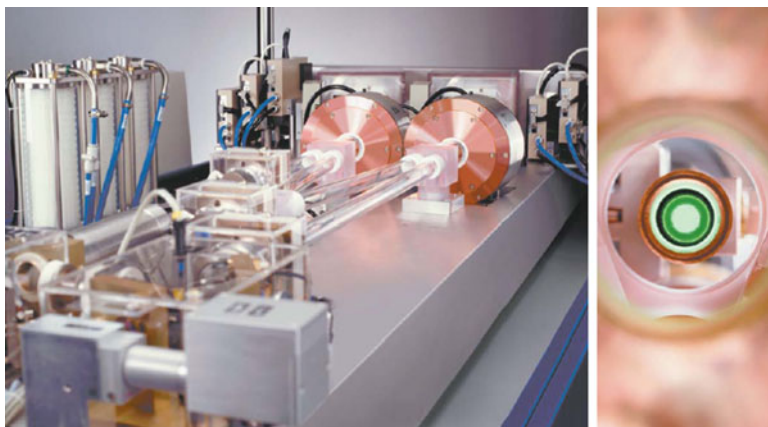
Fig. 7.37 Trumpf's thin disk laser for laser machining
