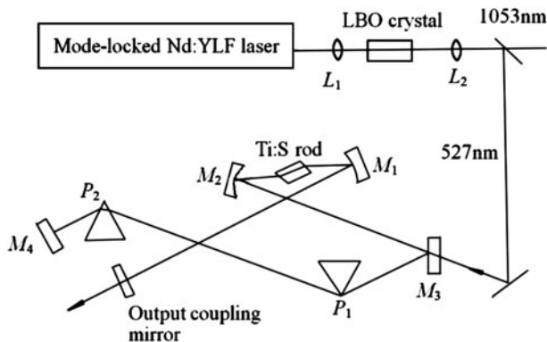
Fig. 9.82 The synchronous pump system
