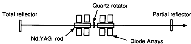
Fig. 6.11 Schematic diagram of the resonator for birefringence compensation
