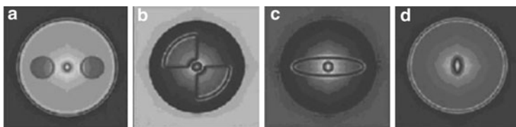
Fig. 7.44 The cross section of PMF: (a) panda-type, (b) bow tie-type, (c) ellipse clad-type, and (d) ellipse core type
