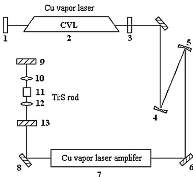
Fig. 9.49 Ti:sapphire laser pumped by copper vapor laser
