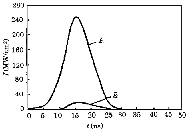
Fig. 4.11 Formation of the parametric wave in pulsed SRO
