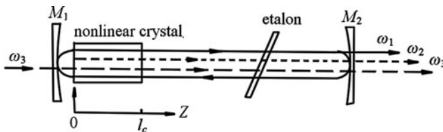
Fig. 4.12 The schematic of synchronously pumped SRO
