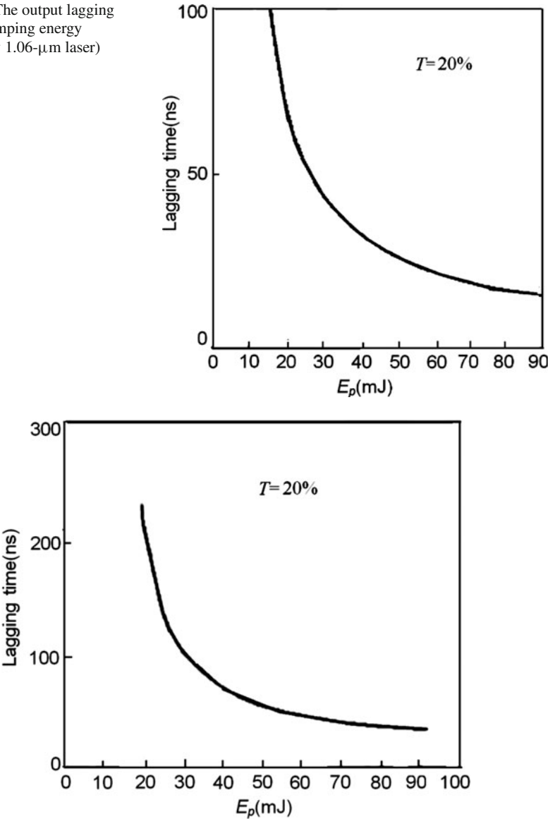
Fig. 8.31 The output lagging time vs. pumping energy (pumped by 0.532- \mu\text{m} laser)
