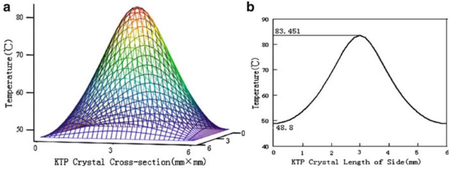
Fig. 7.7 The distribution of temperature inside the KTP crystal (a) 3D distribution and (b) 2D distribution
