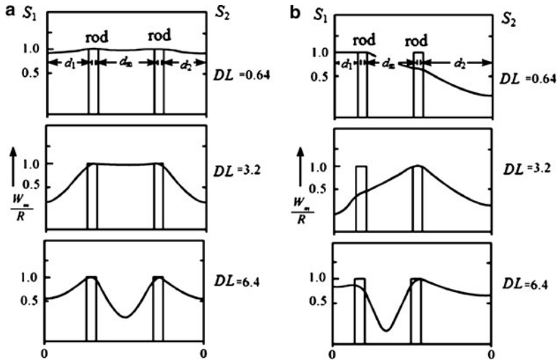
Fig. 6.8 The mode radius inside the resonator with increasing normalized refractive power. The horizontal scale represents the resonator axis. (a) Symmetric resonator with d_1 = d_2 = d_m . (b) Asymmetric resonator with d_1 = 0.17L , d_2 = 0.34L , d_m = 0.45L . L is the distance of two mirrors
