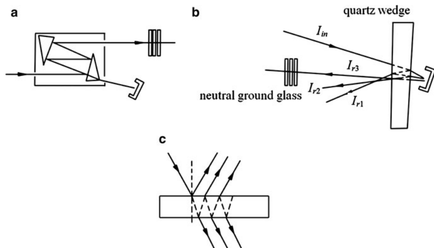
Fig. 3.23 Schematic diagram of some kinds of multiple reflections attenuation methods to measure laser mode. (a) prism multi-reflection; (b) wedge multi-reflection; (c) plate multi-reflection
