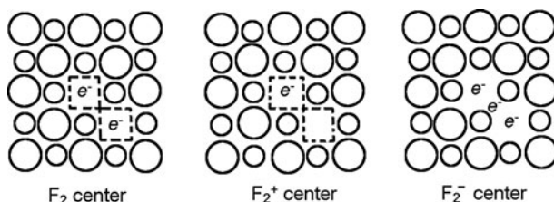
Fig. 8.47 The structures of \text{LiF:F}_2 , \text{LiF:F}_2^+ , and \text{LiF:F}_2^- color center
