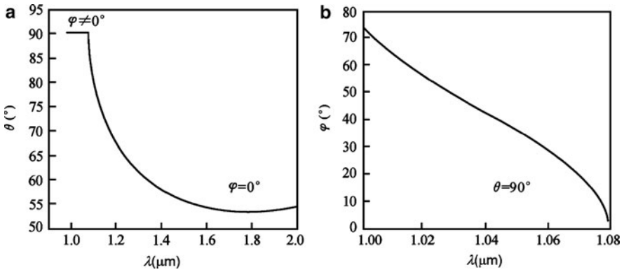
Fig. 1.17 The optimum phase matched angles of frequency doubling in KTP crystal. (a) \varphi = 0^\circ ; (b) \theta = 90^\circ
