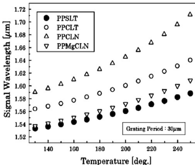
Fig. 5.10 Experimental comparison of the signal wavelengths of PPSLT, PPLT, PPLN, and PPMgLN pumped by 1,064-nm laser with a grating period of 30 \mu\text{m}
