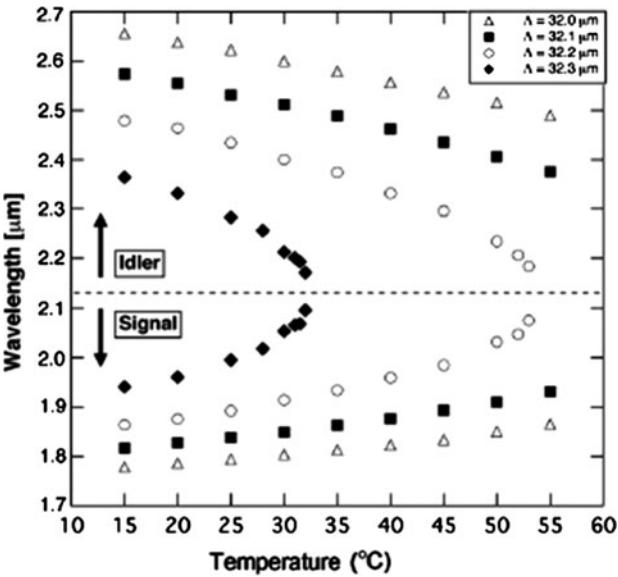
Fig. 5.35 Dependence of the OPO output wavelength on device temperature and QPM period
