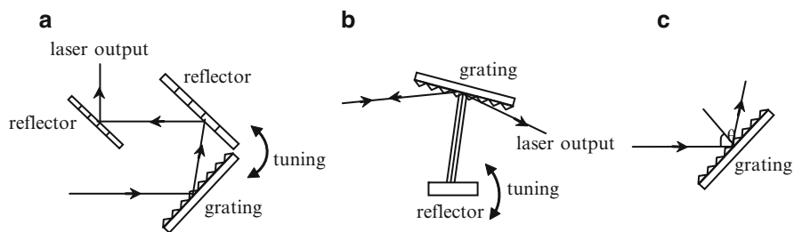
Fig. 8.52 The tuning structure of grating. (a) Littrow grating; (b) grazing-incidence grating; and (c) simplified Littrow grating
