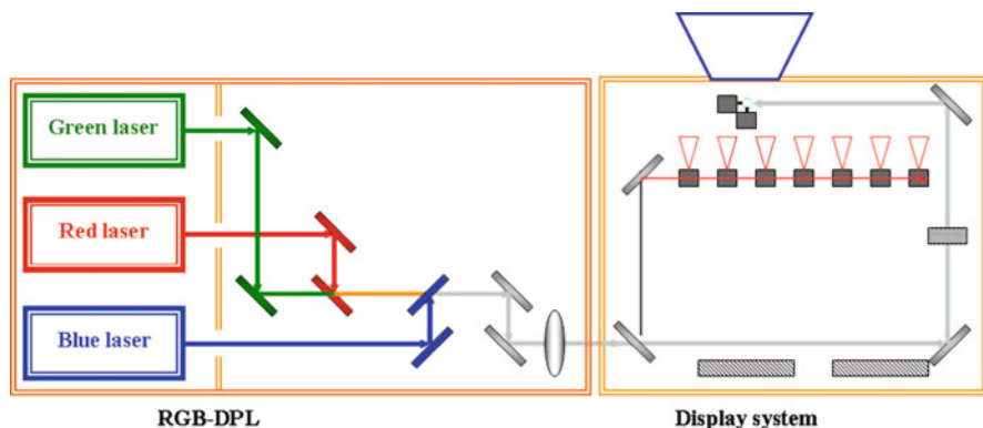
Fig. 7.22 The configuration of the whole laser display system based on RGB-DPL
