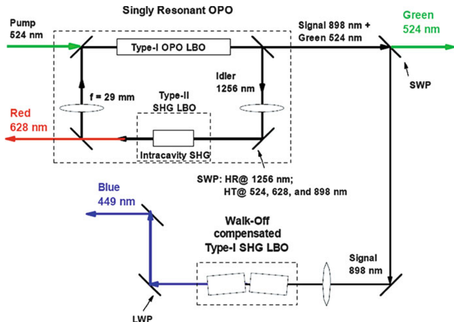
Fig. 7.21 RGB OPO configuration based on DPL
