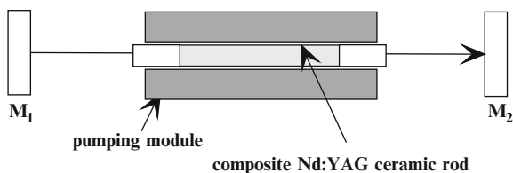
Fig. 7.23 The schematic of diode pumped composite Nd:YAG laser
