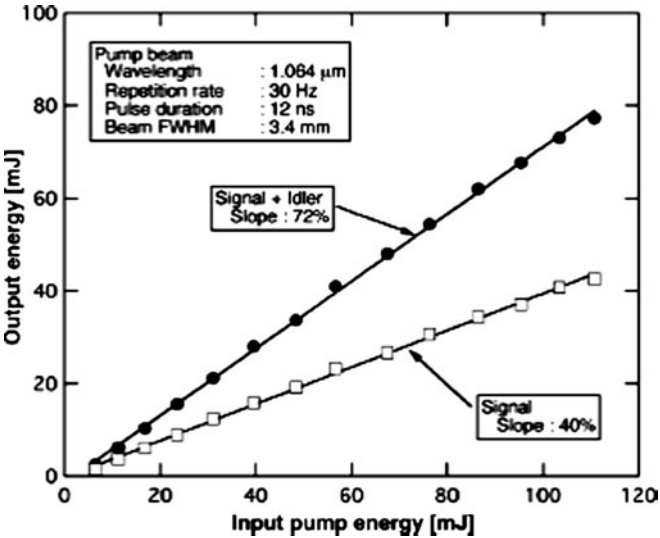
Fig. 5.34 OPO output energy dependence on input pump energy
