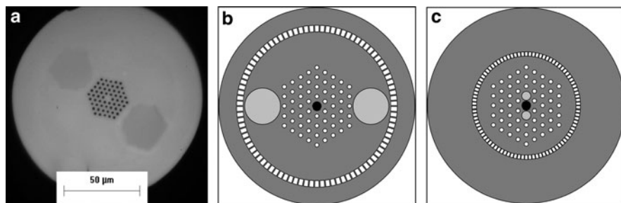
Fig. 7.54 Examples of cross sections of (a) a polarization-maintaining large mode area fiber, (b) polarization-maintaining air-clad fiber, and (c) alternative design of a polarization-maintaining air-clad fiber
