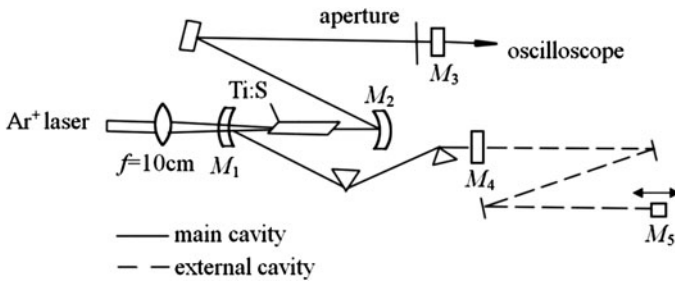
Fig. 9.92 The self-mode-locked Ti:sapphire laser with vibration mirror
