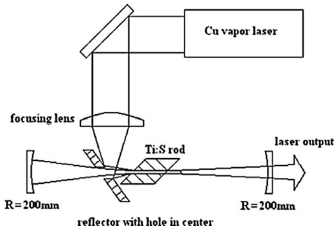
Fig. 9.50 Improved Ti:sapphire laser pumped by copper vapor laser
