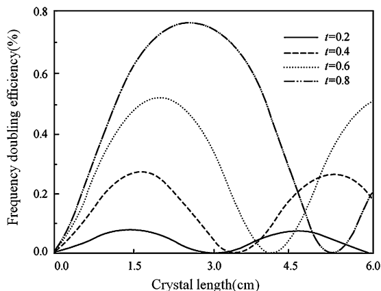
Fig. 1.69 The frequency doubling efficiency vs. crystal length with different polarization ratio
