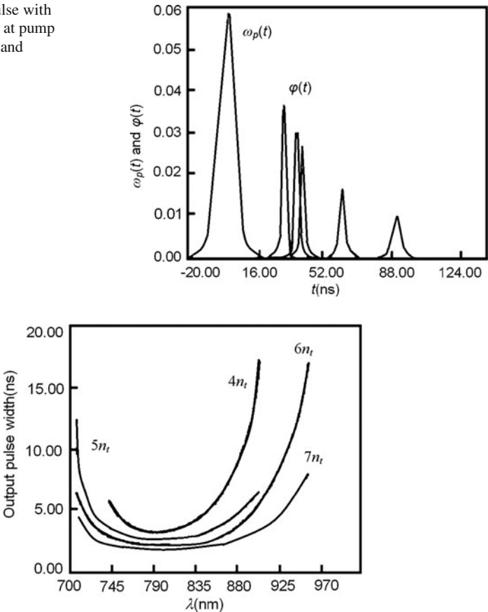
Fig. 9.73 Output pulse width vs. wavelength at different pump energy
