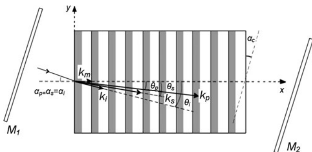
Fig. 5.18 The geometric sketch for the crystal tuning
