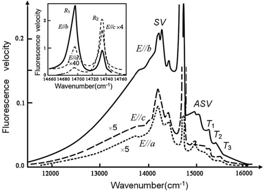
Fig. 8.9 Fluorescence spectrum of Cr:BeAl 2 O 4
