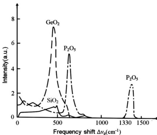
Fig. 10.15 The Raman spectrum of oxide glasses
