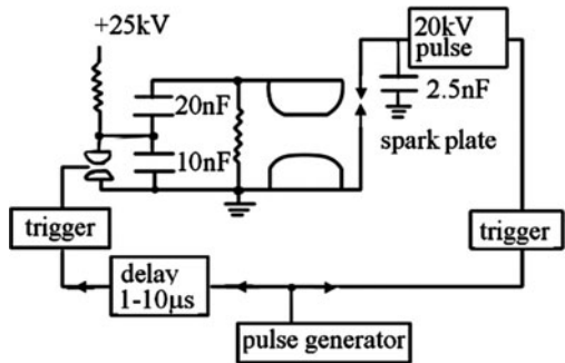
Fig. 10.35 (a) The diagram of quick discharge and (b) its equivalent circuit
