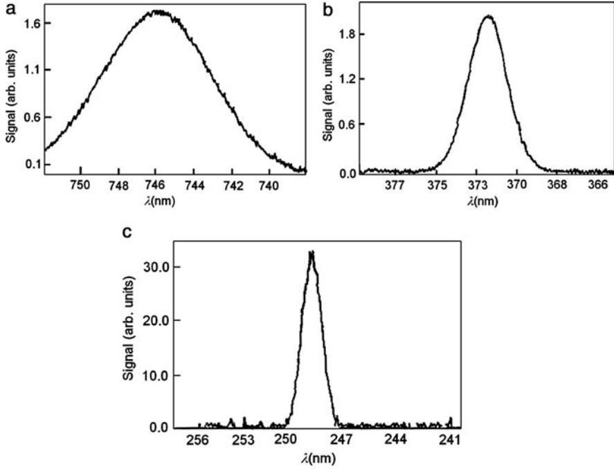
Fig. 3.44 Spectra of (a) fundamental, (b) second-harmonic and (c) third-harmonic waves using KDP
