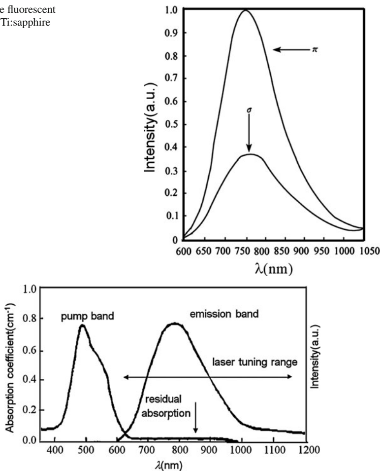
Fig. 9.7 The fluorescent and absorption spectrums of Ti:sapphire
