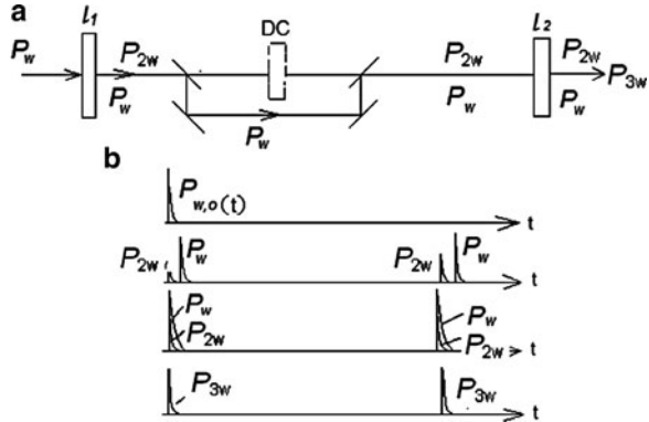
Fig. 3.43 (a) Schematic diagram of frequency mixing compensation and (b) time relation of ultrashort pulses
