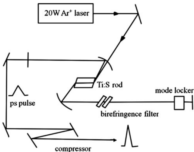
Fig. 9.78 Schematic diagram of an active mode-locked laser
