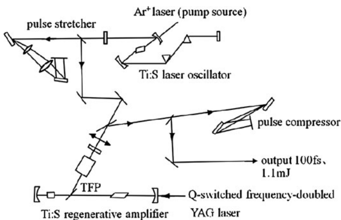
Fig. 9.100 Femtosecond Ti:sapphire laser amplification system
