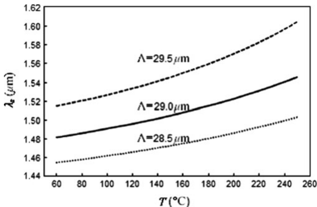
Fig. 5.6 Calculated signal wavelength vs. the crystal temperature for 1,064-nm pumped PPLN–OPO
