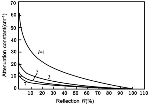
Fig. 4.2 The relationship between the attenuation constant \Gamma_i and reflectivity R ( l = 1, 3, 5, 7 cm, \alpha_i = 0.015 cm ^{-1} , n_i = 2.2467 )
