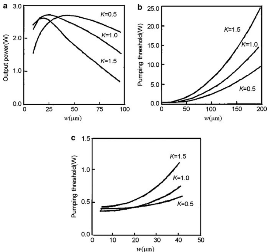
Fig. 9.16 Curves of output power (a) and pumping threshold (b) (c) vs. the beam waist of oscillating light
