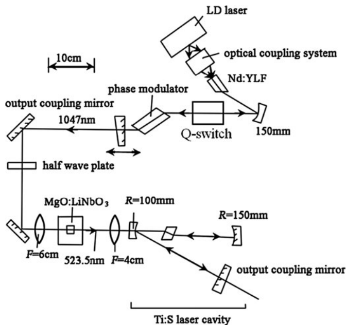
Fig. 9.102 All-solid-state Ti:sapphire laser
