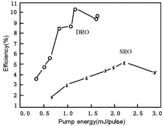
Fig. 4.49 Relationship between conversion efficiency and pump energy
