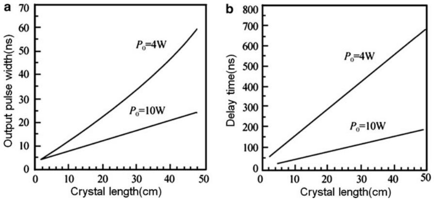
Fig. 9.32 (a) The output pulse width and (b) the delay time as a function of cavity length
