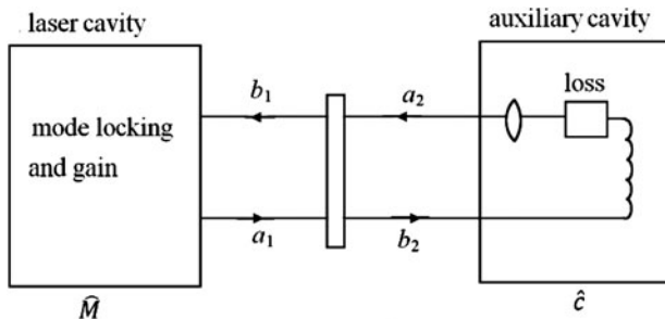
Fig. 9.84 Equivalent network of auxiliary cavity mode locking
