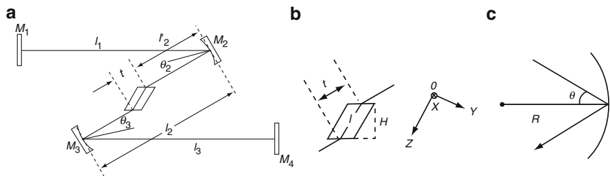
Fig. 9.17 Four-mirror cavity
