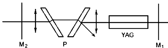
Fig. 3.19 A polarizer inserted into YAG laser cavity
