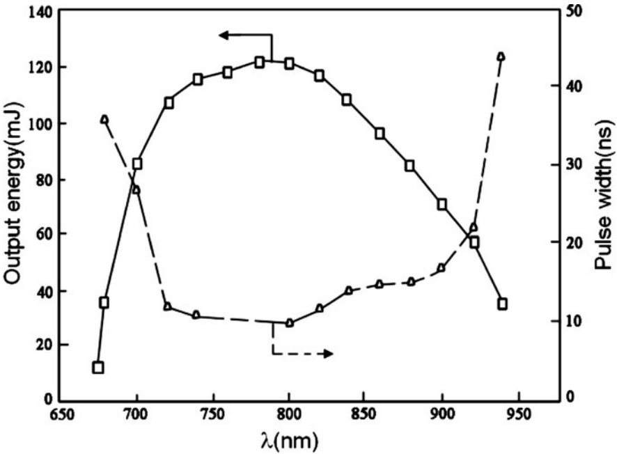
Fig. 9.55 The output energy and pulse width vs. wavelength
