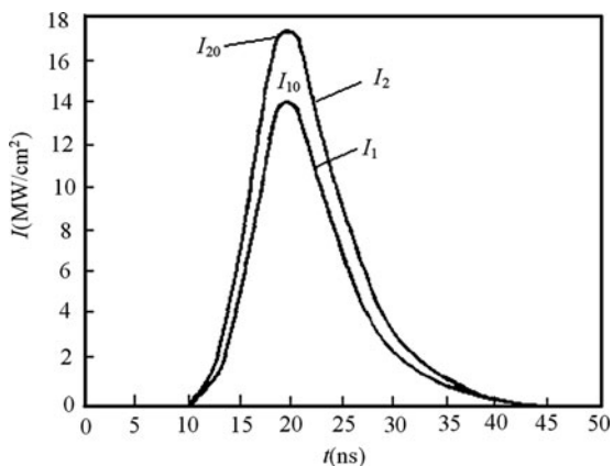
Fig. 4.4 Comparison between the pulse peaks for DRO under same attenuation constants ( \lambda_1 = 1.3 \mu\text{m} , \lambda_2 = 0.9 \mu\text{m} )
