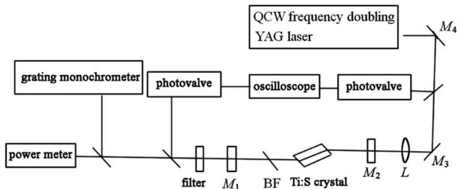
Fig. 9.41 Diagrammatic sketch of QCW Ti:sapphire laser with linear cavity
