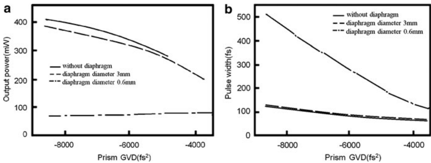
Fig. 9.94 (a) Output power and (b) pulse width as a function of GVD in prism
