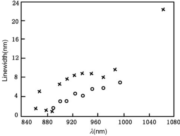
Fig. 4.50 The linewidth of DRO (○ — 0.495 mJ/pulse, × — 0.825 mJ/pulse)
