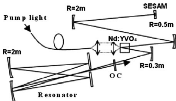
Fig. 6.25 1.2 MHz low repetition rate mode-locked laser
