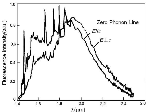
Fig. 8.4 Polarized fluorescence spectrum zero phonon line of \text{Co}^{2+}:\text{MgF}_2
