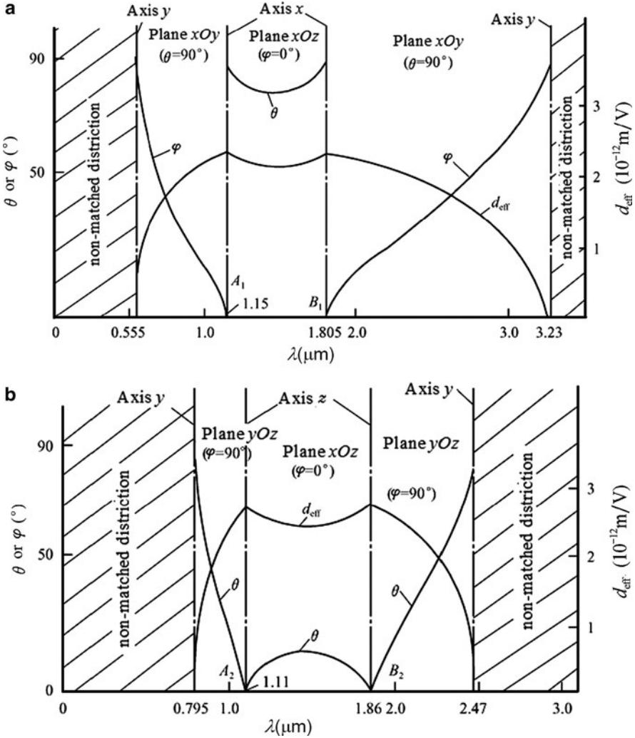
Fig. 1.57 The optimum phase matched angle \theta (or \varphi ) of type I (a) and type II (b) SHG phase match in LBO crystal
