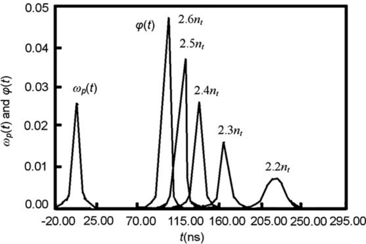
Fig. 9.61 Output pulse at pump pulse width of 10 ns and energy of 2.2-2.6n_t
