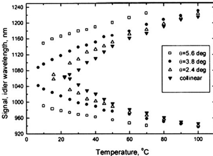
Fig. 5.22 Tuning characteristics of the noncollinear OPO
