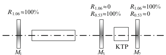
Fig. 3.16 Double-pass intracavity frequency doubling laser: linear cavity
