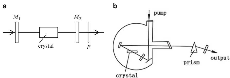
Fig. 8.46 The schematic drawing of two different color center lasers (a) linear cavity; (b) laser cavity under lower temperature operation
