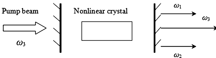
Fig. 4.1 A model of optical parametric oscillator
