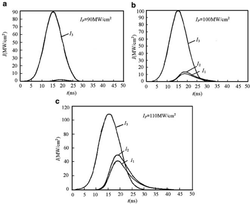
Fig. 4.3 Generation of OPO pumped by a Gaussian-shape pulse
