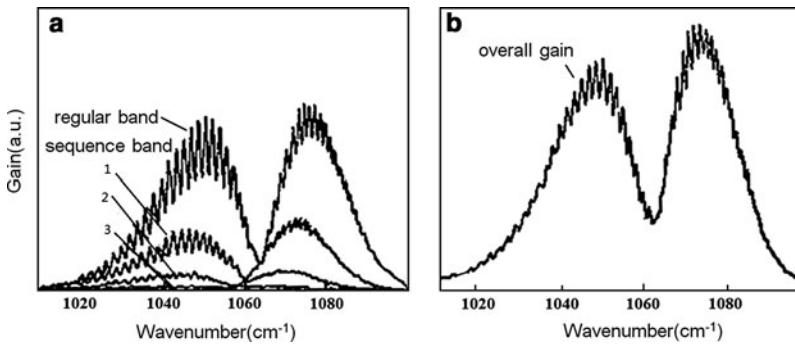
Fig. 10.23 (a) Sequence and regular band gain of gas mixture CO_2:N_2:He = 2:2:96 ( T_3 = 2,000 K, 10 atm.) and (b) overall gain
