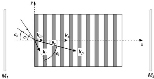
Fig. 5.12 The definitions of various wave vectors and angles in signal resonance OPO
