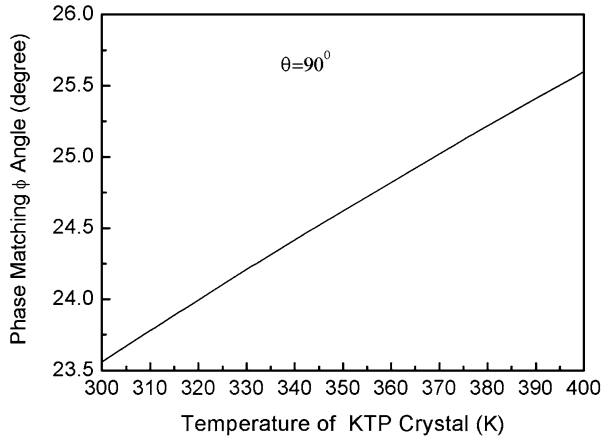
Fig. 7.8 The phase matching angles at different temperatures
