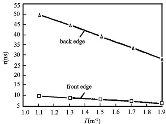
Fig. 4.8 The change of front edge and back edge of I_2(t) with I
