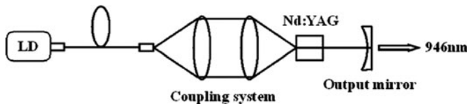
Fig. 6.16 Schematic diagram of the high power diode-end-pumped 946 nm laser
