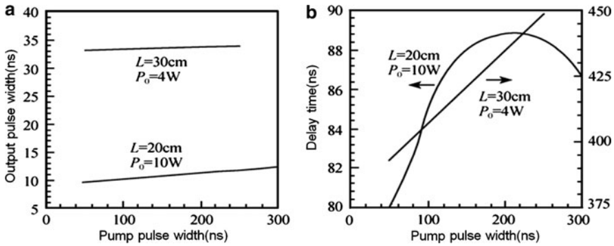
Fig. 9.30 (a) The output pulse width and (b) delay time as a function of pump pulse width
