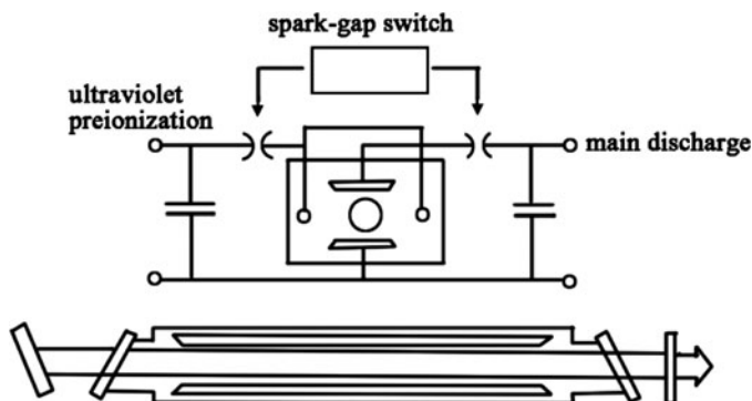
Fig. 10.27 The diagram of ultraviolet preionization TE-CO 2 laser
