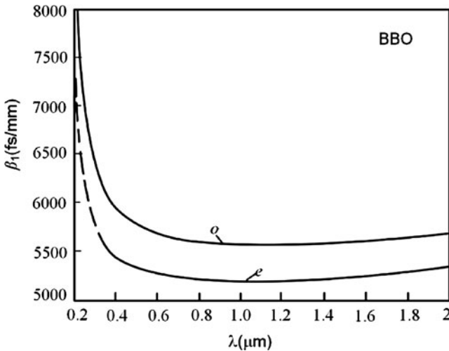
Fig. 3.31 Coefficient of group velocity delay of BBO crystal \beta_1 (fs/mm)
