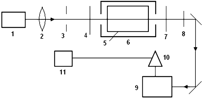
Fig. 4.45 The experimental setup of MgO : LiNbO 3 OPO 1-pump source, 2-lens, 3-diaphragm, 4, 7-cavity mirrors, 5 – MgO : LiNbO 3 , 6-temperature controller, 8-filter, 9-monochrometer, 10-detector, 11-oscilloscope
