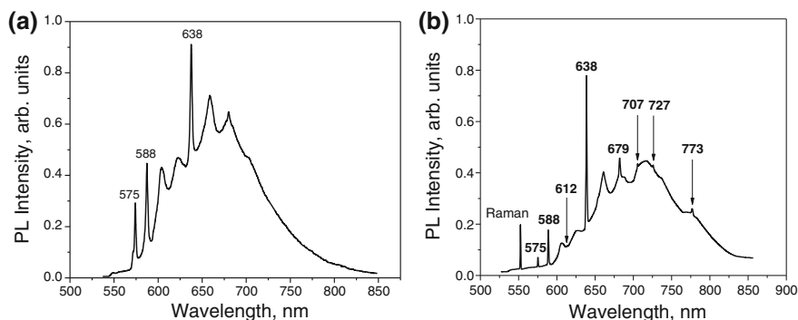
Fig. 6.33 a PL spectrum of a natural diamond of intense greenish-yellow color treated with irradiation and annealing. The spectrum exhibits three major centers 575 nm ( \text{NV}^0 ), 588 nm and 638 nm ( \text{NV}^- ). This diamond does not show obvious evidence of HPHT treatment save for the high intensity ratio I_{638}/I_{575} , which is about 4. b PL spectrum of a greenish-yellow HPHT-treated diamond [re-plotted from (Zhonghua Song et al. 2009)]. High ratio of intensities of the 638 and 575 nm centers I_{638}/I_{575} suggests HPHT treatment. However the presence of the 588 nm center and traces of the centers 612, 679, 707, 727 and 773 nm can be considered as an indication that the treatment was performed at low temperatures not exceeding 1,800 °C
