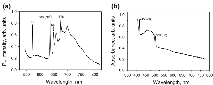
Fig. 6.45 a PL spectrum (taken at LNT) of an irradiated and subsequently annealed natural diamond (no HPHT treatment). The spectrum is dominated by the 638, 649 and 676.5 nm centers. b Absorption spectrum of the same diamond. Although the H3 center is strong in absorption, it does not reveal the “green transmission” effect. Strong absorption without “green transmission” is a characteristic behavior of the H3 center in diamonds treated by irradiation followed by annealing at temperatures below 1,400 °C
