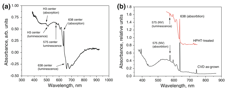
Fig. 6.28 a FSI absorption spectrum of an Imperial Red diamond of fancy deep purple color. Very strong 638 nm center ( \text{NV}^- center) is seen in regimes of absorption and luminescence (“ red transmission” effect)—a typical feature of HPHT-treated diamonds of red color. A weak H3 center also shows “ green transmission” effect. The 575 nm center is seen in the regime of emission, not absorption—a typical feature of FSI absorption spectra of Imperial Red diamonds. b Comparison of absorption spectra of a natural HPHT-treated diamond of red color and an as-grown CVD diamond of pink color. Both diamonds exhibit dominating 638 nm ( \text{NV}^- ) center and minor 575 nm ( \text{NV}^0 ) center. In the HPHT-treated diamond, the 575 nm center is observed in the regime of luminescence, whereas it shows absorption in as-grown CVD diamond [based on data from (Wang 2009b; Johnson and Breeding 2009)]
