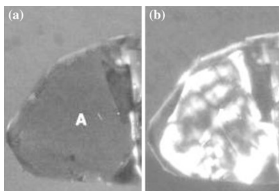
Fig. 5.8 Images of a synthetic type IIa diamond taken in polarized light before (a) , and after (b) HPHT treatment performed at a temperature of 1,600 °C and a pressure of 6 GPa for 2 h. The image taken after HPHT processing reveals strong birefringence pattern due to internal strain produced by plastic deformation (Kanda et al. 2005) (with permission of Diamond and Related Materials magazine)
