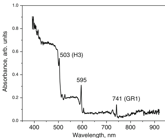
Fig. 6.34 Absorption spectrum of a fancy deep brownish yellow diamond, which exhibits an intense 595 nm center. This diamond has been reported as treated by multi-process treatment. Based on the intensity and phonon structure of the GR1 center, one can conclude that the final annealing used for the treatment was performed at a temperature below 700 °C
