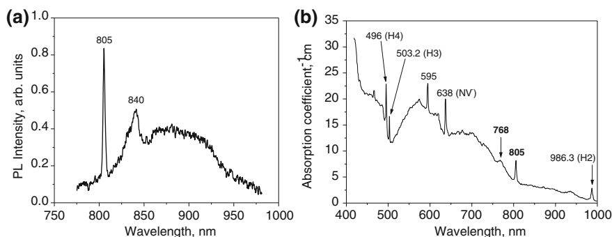
Fig. 6.59 a PL spectrum of the 805 nm center in a HPHT-treated fancy intense greenish yellow diamond. ZPL of the 805 nm center is accompanied by the vibrational sideband spreading from 800 to 950 nm, a characteristic feature of which is a peak at 840 nm due to interaction with acoustic phonons of energy 70 meV. b Absorption spectrum of a type Ia diamond after multi-process treatment. The treatment has converted the diamond into ABC diamond. Absorption of many optical centers characteristic of multi-process treatment can be seen. The 805 nm center is presented by its ZPL at 805.2 nm and phonon replica at wavelength of 768 nm (interaction with optical phonons of energy 116 meV) [re-plotted from (Vins et al., 2011b)]
