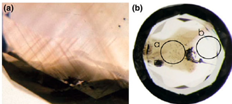
Fig. 2.8 a Brown graining in a natural regular brown diamond (Kitawaki 2007). b A natural diamond exhibiting brown coloration due to high content of CO 2 molecules (Hainschwang et al. 2008) (with permission of the Diamond and Related Materials journal)
