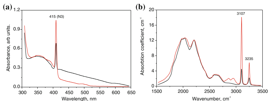
Fig. 4.20 Exemplary Vis (a), and IR (b) absorption spectra of initially gray type IaA diamonds before (black curves) and after (red curves) HPHT treatment at temperatures in the range 1,800–2100 °C under pressure 6–7 GPa. Treatment removes the absorption continuum in the visible spectral range and stimulates the C Defect absorption continuum, the N3 center and the hydrogen-related centers, the most intense being the 3,107 \text{cm}^{-1} line. Gray color of these diamonds is converted into straw-yellow [re-plotted from Vins and Kononov (2003)]
