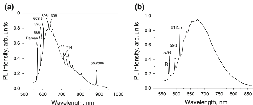
Fig. 6.35 a PL spectrum of a low-nitrogen, fancy orange yellow diamond measured at LNT. Many Ni-related centers characteristic of HPHT treatment are seen. This stone showed yellow color “fluorescence cage”, which is frequently observed in type Ia Ni-containing HPHT-treated natural diamonds. b PL spectrum of an untreated fancy dark yellow brown natural diamond showing the 596 nm center. The presence of the 576 and 711 nm centers and the narrow Platelets Peak (FWHM of 8.8\text{ cm}^{-1} ) confirm that the diamond is untreated. In this diamond, the 711 nm center is very strong when excited at a wavelength of 658 nm
