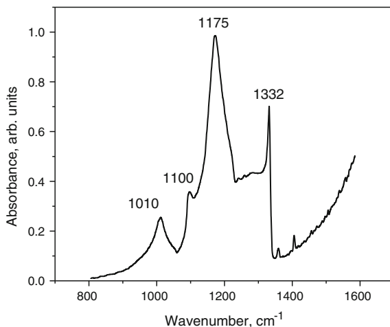
Fig. 6.80 FTIR absorption spectrum of natural diamond of a pure type IaB showing sole absorption of the B-center. The features of the B-center are at 1,010, 1,100, 1,332 and 1,175 \text{cm}^{-1} , the latter being the most intense
