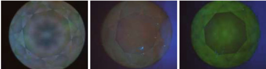
Fig. 7.7 Typical fluorecence images of natural untreated diamonds. There is no sign of enhanced fluorescence on the facet edges
