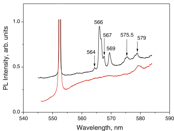
Fig. 6.31 PL spectra of originally brown type IIa natural diamond ( black curve ) converted by HPHT treatment into colorless ( red curve ). A complex spectral structure with major lines at 566 and 569 nm is completely removed by the treatment. The 579 nm center is the only feature in the spectral range from 560 to 585 nm (Simic and Zaitsev 2012)
