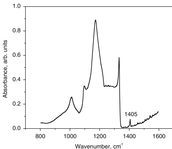
Fig. 6.71 FTIR absorption spectrum of an untreated type IaB diamond (F color) showing the 1,405\text{ cm}^{-1} center. This diamond reveals traces of natural irradiation: a weak GR1 center in Vis absorption and PL spectra and rather weak 575 and 638 nm centers in PL spectra. Intensity ratio of the NV centers I_{638}/I_{575} is about 0.1 supporting the conclusion that the diamond is in pristine untreated state
