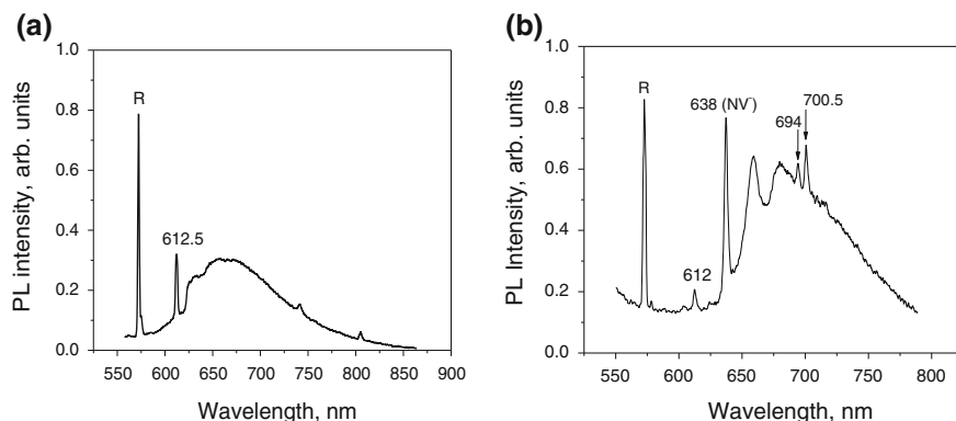
Fig. 6.37 PL spectra taken from an untreated type IaB natural diamond (a) and untreated high-nitrogen type IaB diamond (b). A well-developed 638 nm center ( \text{NV}^- ) in spectrum (b) has natural origin and it is not an indicator of HPHT treatment. The presence of sole \text{NV}^- center without any trace of the 575 nm ( \text{NV}^0 ) center is a feature of a diamond with an appreciable content of C defects
