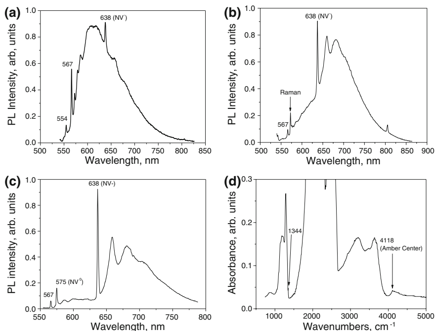
Fig. 6.26 a, b PL spectra of two ABC natural diamonds exhibiting the 567 nm Ni-related center. Although the 638 nm ( \text{NV}^- ) center is strong ( b ), it is not an indicator of HPHT treatment in this case. Along with the 567 nm center, the untreated nature of this stone has been confirmed by the presence of the Amber Center and deep brown coloration. The absence of the 575 nm ( \text{NV}^0 ) center in both spectra indicates an appreciable concentration of C defects. ( c, d ) PL and IR absorption spectra of a fancy deep brownish yellow HPHT-treated diamond. The treatment of this stone has been confirmed by simultaneous presence of the 638 nm ( \text{NV}^- ) and 575 nm ( \text{NV}^0 ) centers in PL spectrum ( \text{NV}^- \gg \text{NV}^0 ), by the presence of the \text{NV}^- center in absorption spectrum, by the presence of the 1,344\text{ cm}^{-1} line (C defects) in IR absorption spectrum and by two small “frosted” facets. This diamond shows the 567 nm center. One can assume that this stone was HPHT treated at a low temperature
