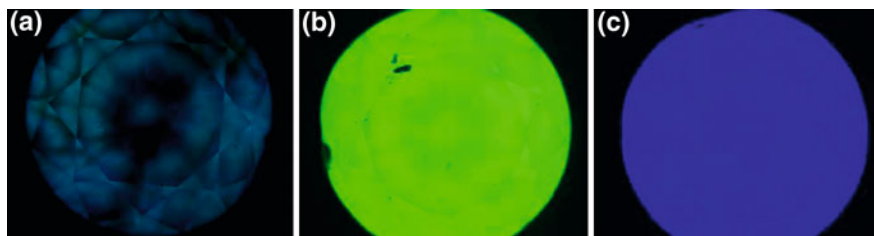
Fig. 6.17 Fluorescence images of a natural type Ia initially brown diamond before treatment (a), after first HPHT treatment at a temperature of 1,900 °C (b) and after second treatment at a temperature of 2,400 °C (c). After the first low temperature treatment, the diamond exhibits very strong green fluorescence of the H3 center, which disappears after the heating at 2,400 °C
