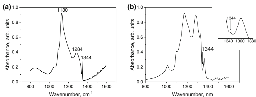
Fig. 6.78 a FTIR absorption spectrum of a fancy deep yellow orange synthetic diamond of a pure type Ib. The main features of C-center are sharp peak at 1,344\text{ cm}^{-1} and relatively narrow band at 1,130\text{ cm}^{-1} . A minor broad band at 1,284\text{ cm}^{-1} is also a feature of the C-center. b FTIR absorption spectrum of a diamond of red color after multi-process treatment. A tiny feature at a wavenumber 1,344\text{ cm}^{-1} manifests the presence of the C defects at a concentration of 2 ppm. The insert shows the 1,344\text{ cm}^{-1} line is greater detail. The Platelets peak is characteristically broad. This type of spectrum is very common for HPHT-treated type IaAB diamonds. Although the intensity of C-center in IR absorption is negligibly weak, Vis absorption and PL spectra of this diamond show very strong 638 nm center, which is a direct derivative of the C defects
