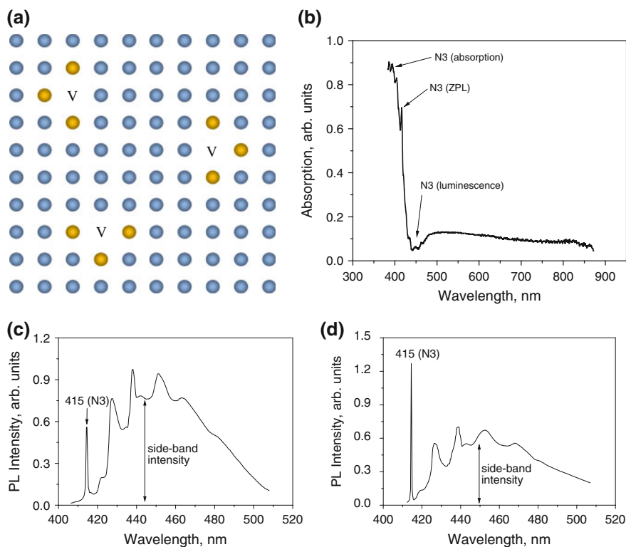
Fig. 6.6 a Atomic model of the N3 center: three adjacent substitutional nitrogen atoms bound to a common vacancy. Blue and yellow circles denote carbon and nitrogen atoms respectively. b Absorption spectrum of a natural diamond showing strong N3 center in regime of absorption and luminescence (“blue transmission” effect). High color (F) of this diamond is partially due to blue luminescence of the N3 center. c PL spectrum of the N3 center in natural untreated type IaB diamond. ZPL intensity in its maximum is lower than that of the side-band because of considerable non-homogeneous internal stress in this diamond. d PL spectrum of the same diamond as in (c), but after HPHT treatment performed at a temperature of 2,000 °C [re-plotted from (Nadolinny et al. 2009)]. Now ZPL intensity in its maximum is stronger than that of the side-band. This seeming increase in the intensity of ZPL occurs because of its spectral narrowing after treatment
