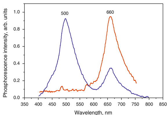
Fig. 6.44 Phosphorescence spectra of natural type IIb diamonds: a fancy intense blue diamond exhibiting dominating “Red Band” ( red curve ) and a very light blue diamond exhibiting “Blue Band” and “Red Band” ( blue curve ). Lifetime of the emission of the “Blue Band” is shorter than that of the “Red Band”. Therefore, if the two bands are present with comparable intensities, the “Red Band” dominates in visual phosphorescence [based on the data from (Eaton-Magana and Lu 2011)]
