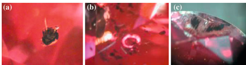
Fig. 5.2 Typical macroscopic defects observed in HPHT-treated diamonds. a This black inclusion is observed in an Imperial Red diamond. It is associated with the graphitized diamond-inclusion interface, which was formed during HPHT annealing. Several transparent micro-cracks were formed around the inclusion—a very characteristic feature of HPHT treatment. In most treated diamonds of dark colors, these inclusions are barely visible. Sometimes, the graphitized inclusions emerge on the diamond surface after repolishing and, when their interior crumbles out, leave characteristic caverns. b Disk-shaped fractures frequently surround black crystalline inclusions in HPHT-treated diamonds. c Sometimes the surface of fractures is stained by graphite, which forms during HPHT annealing (courtesy of S. Z. Smirnov)
