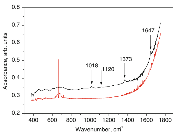
Fig. 6.72 FTIR absorption spectra of a type IIa initially brown diamond converted into colorless by HPHT treatment: black curve —before treatment, red curve —after treatment. The spectral lines, which change their intensity after HPHT treatment are indicated
