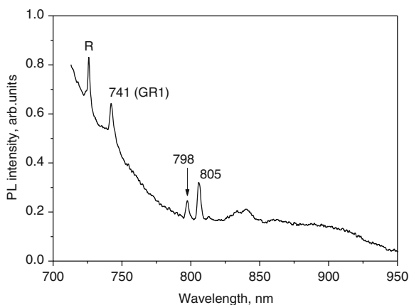
Fig. 6.58 PL spectrum of a low-nitrogen fancy intense orangey pink diamond after multi-process treatment. The dominating centers are GR1, 798 and 805 nm. Presence of the GR1 center either indicates that the final annealing step of the treatment was performed at a temperature below 800 °C, or that, after the multi-process treatment, the diamond was additionally irradiated with low dose of energetic electrons
