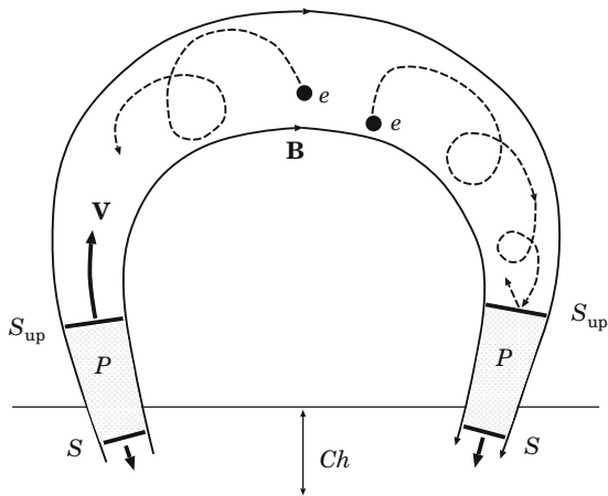
Fig. 6.4 The flare-heated chromospheric plasma P rapidly expands into the corona. Particle acceleration of the first order Fermi type may occur in a magnetic loop between two converging shock waves S_{up}
