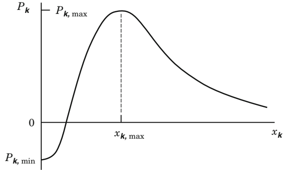
Fig. 8.6 The Coulomb losses (with the sign minus in formula (8.58)) of energy of a test particle as a function of its velocity measured in the most probable velocity of the field thermal particles of the kind k
