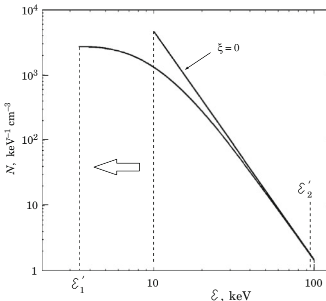
Fig. 4.4 The energy spectrum of fast electrons in a high-temperature plasma on the column depth \xi = 0 (the right straight line ) and on the column depth \xi = 1.5 \times 10^{19} \text{ cm}^{-2} ( left curve ). Here \xi'_1 = 3.41 \text{ keV} and \xi'_2 = 99.56 \text{ keV} according to (4.42)
