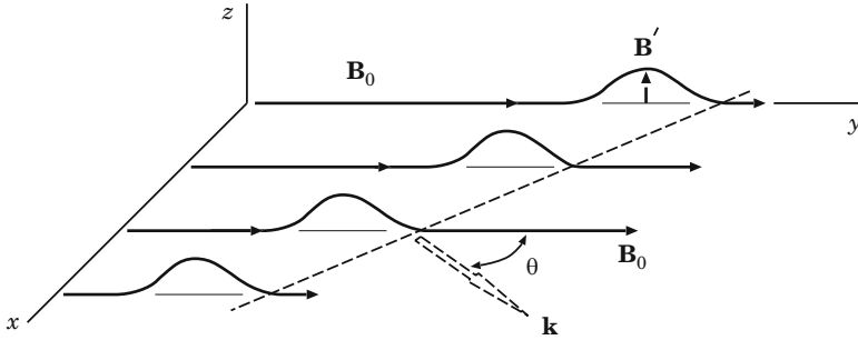
Fig. 15.1 The transversal displacements of plasma and magnetic field in the Alfvén wave
