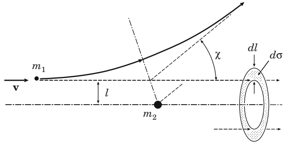
Fig. 8.1 The trajectory of a light particle with mass m_1 near a heavy particle with mass m_2
