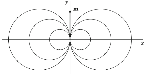
Fig. 14.6 The field lines of a plane magnetic dipole
