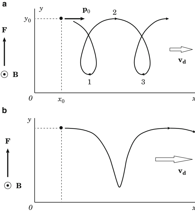
Fig. 5.2 The trajectory of motion a positively charged particle in a homogeneous magnetic field under action of a non-magnetic force. Slow (a) and fast (b) drifts
