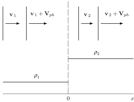
Fig. 17.2 Six small-amplitude waves leaving an immovable discontinuity surface ( x = 0 ) being perturbed
