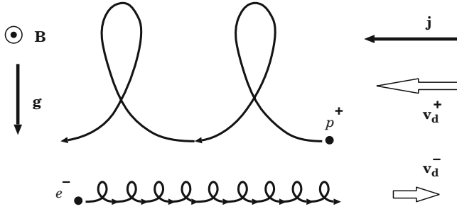
Fig. 5.4 Gravitational drift. Initiation of an electric current by the action of the gravity force in a collisionless plasma with magnetic field
