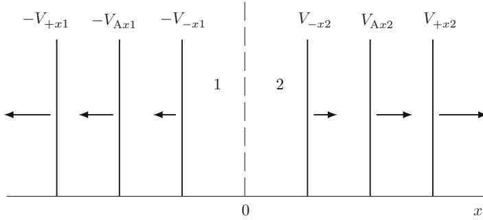
Fig. 17.2 Six small-amplitude waves leaving an immovable discontinuity surface ( x = 0 ) being perturbed
