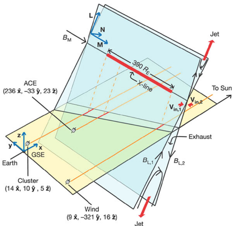
Fig. 12.4 Reconnection in the solar wind. Diagram encounters the three spacecraft: Wind , ACE and Cluster on 2 February 2002. The spacecraft positions are shown in units of Earth radius ( R_E ) and in geocentric solar ecliptic (GSE) coordinates with the x -axis pointing from Earth to Sun, the y -axis pointing towards dusk and the z -axis is perpendicular to the ecliptic plane (in yellow). (Reproduced with permission © NATURE Publishing Group)
