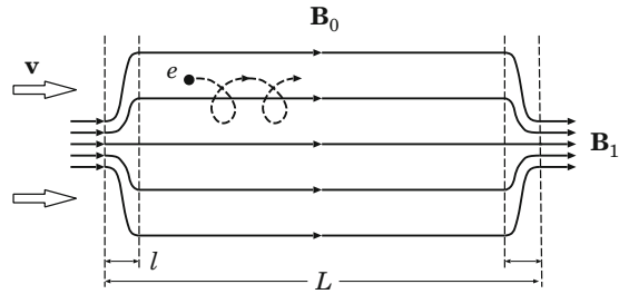
Fig. 6.3 An idealized model of a long trap with a short moving cork. Unless a charged particle has its velocity vector very close to the axis of the trap, it is reflected back and forth between the mirrors, thereby remaining trapped
