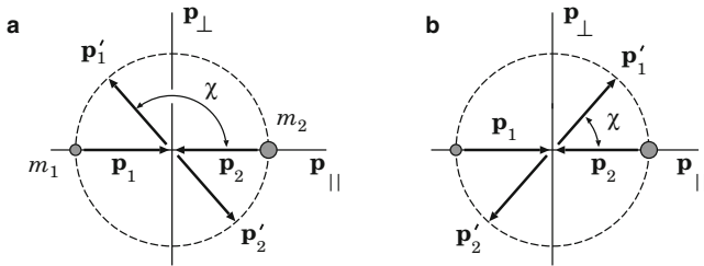
Fig. 8.2 Close (a) and distant (b) collisions of particles in the momentum space in the centre-of-mass system
