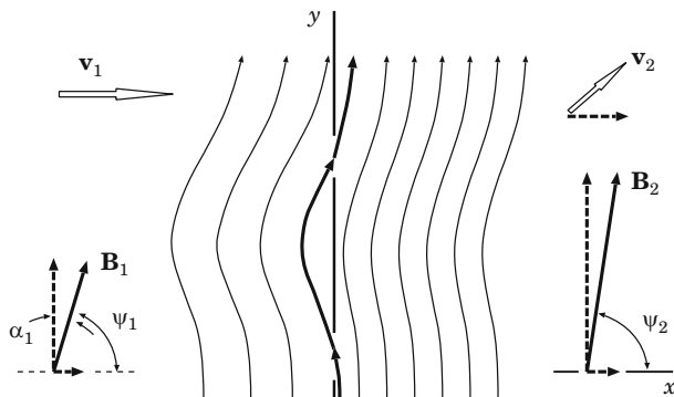
Fig. 18.5 A collapsing magnetic trap on the upstream side of a quasi-perpendicular shock wave
