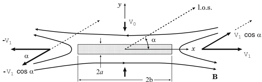
Fig. 8.5 Magnetic reconnection changes the topology of magnetic field lines and creates the fast plasma outflows. v_1 and -v_1 are the high-temperature plasma velocities near a reconnecting current layer
