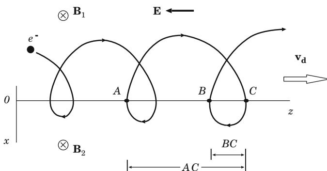
Fig. 18.3 The trajectory of a negatively charged particle (an electron) multiply crossing the perpendicular shock front
