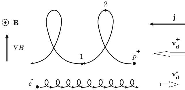
Fig. 5.9 The simplest interpretation of the gradient drift. A gradient in the field strength, \nabla B , in the direction perpendicular to \mathbf{B} will produce a drift motion of ions and electrons
