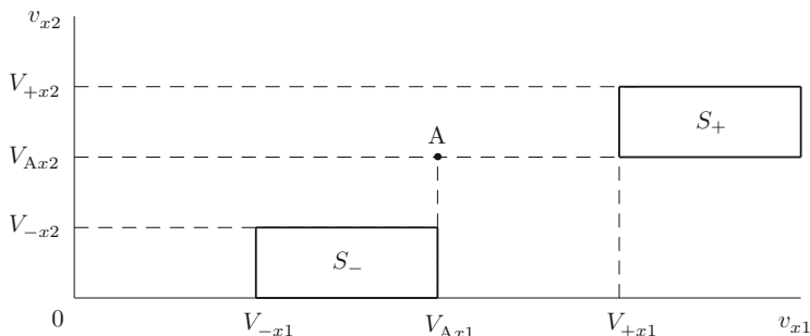
Fig. 17.5 The evolutionarity domains for the fast ( S_+ ) and slow ( S_- ) shocks and the Alfvén discontinuity (the point A)
