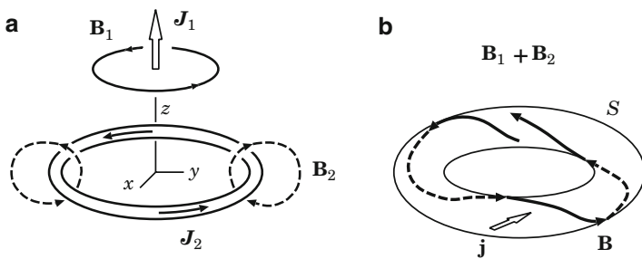
Fig. 19.2 (a) A line current J_1 and a ring current J_2 . (b) The field lines of the total field B_1 + B_2 form a toroidal surface S
