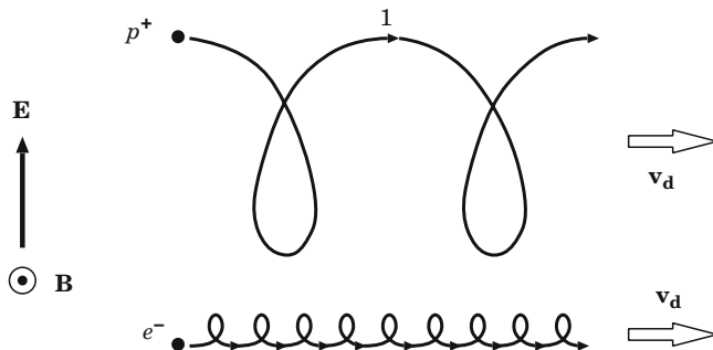
Fig. 5.3 Electric drift. The kinetic energy \mathcal{E} of a positively charged particle p^+ is a maximum at the upper point 1, hence the curvature radius r_L of the trajectory is a maximum at this point
