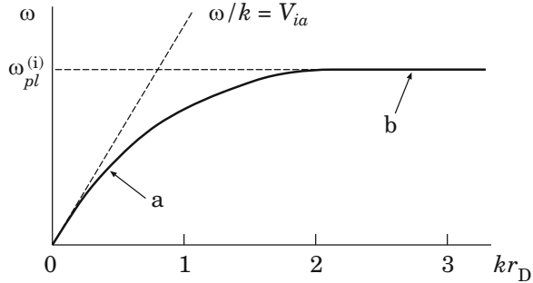
Fig. 10.2 A dispersion diagram for ion-acoustic waves (part a ) and for ion plasma waves (part b ) in a warm plasma without magnetic field
