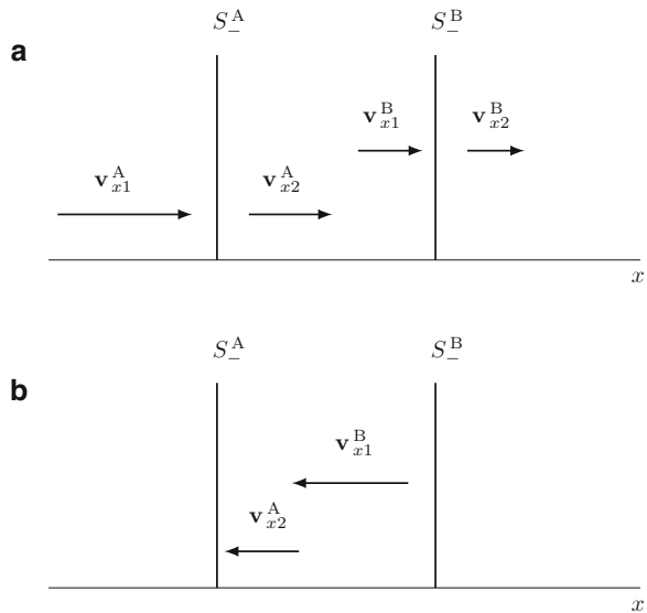
Fig. 17.6 Plasma flow velocities relative to: (a) shock wave fronts, (b) the plasma between the shock waves
