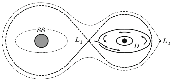
Fig. 13.1 The standard model of a binary stellar system with an accretion disk. The tidally and rotationally distorted secondary star SS loses plasma from the unstable L_1 point. The resulting plasma stream feeds an accretion disk D , centered on the primary star
