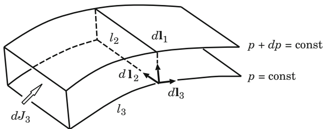
Fig. 19.3 The calculation of the electric current between two magnetic surfaces
