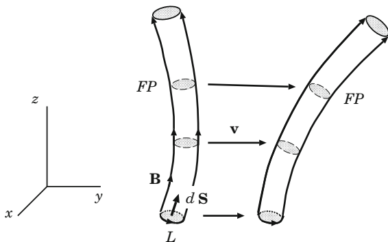
Fig. 12.3 The magnetic-field flux tube through the surface d\mathbf{S} moves with a plasma with velocity \mathbf{v} . L is the “liquid contour” bounding the surface d\mathbf{S} . The “fluid particles” ( FP ) that are initially in this flux tube remain in the same tube
