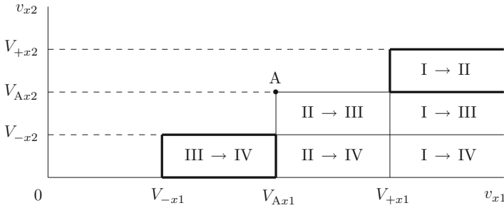
Fig. 17.10 Transitions with increasing entropy. Evolutionarity domains ( bold rectangles ) for the fast ( I \rightarrow II ) and slow ( III \rightarrow IV ) shock waves
