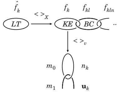
Fig. 9.1 From the microscopic to the macroscopic view of a plasma. LT is the Liouville theorem and the Liouville equation (1.26) for an exact distribution function \hat{f}_k . KE and BC are the kinetic equation (2.39) and the equation for the binary correlation function. m_0 is the equation for the zeroth moment of the distribution function f_k , the number density n_k of the particles of kind k . This equation is unclosed
