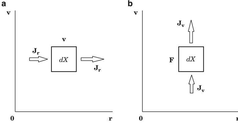
Fig. 1.3 Action of the two different terms of the Liouville operator in the 6D phase space X . (a) A simple kinematic effect. (b) Particle acceleration
