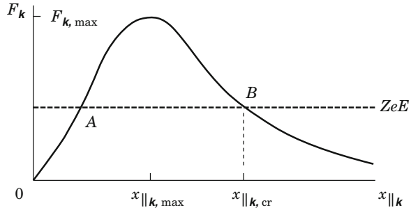
Fig. 8.7 The collisional drag force F_k (with the sign minus in formula (8.70)) on a test particle as a function of its velocity v_{\parallel} measured in the most probable velocity v_k of the field particles of the kind k
