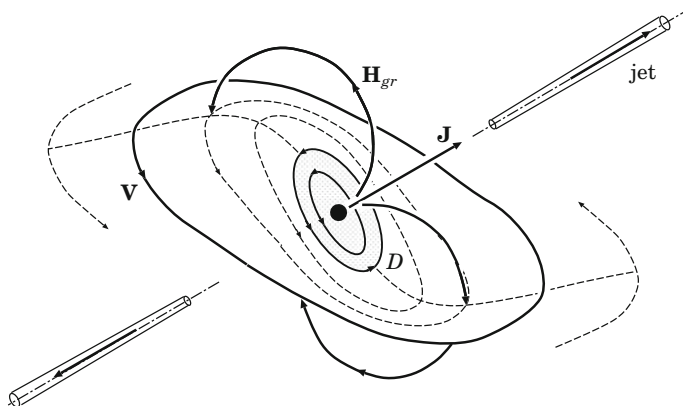
Fig. 13.2 An accretion disk D around a rotating black hole is driven into the hole's equatorial plane at small radii by a combination of gravitomagnetic forces (action of the gravitomagnetic field \mathbf{H}_{gr} on orbiting plasma) and viscous forces
