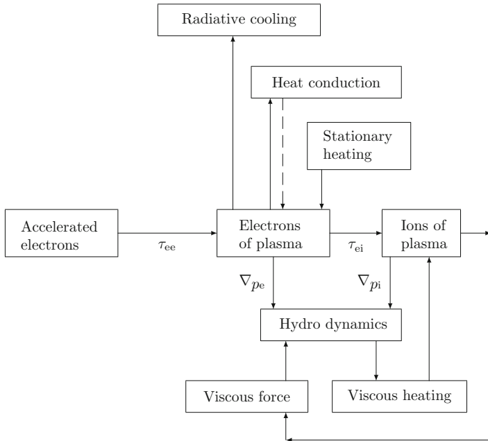
Fig. 8.3 A scheme of the energy exchange in the two-temperature model of a single-fluid hydrodynamic response of the solar atmosphere to impulsive heating by an electron beam
