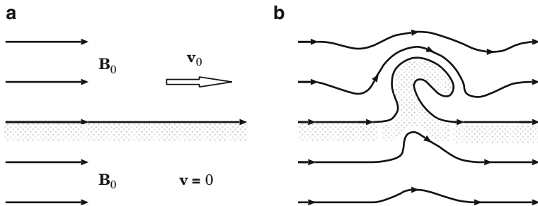
Fig. 16.4 (a) The simplest type of the MHD tangential discontinuities. (b) Formation of a turbulent vortex gives rise to the magnetic field growth
