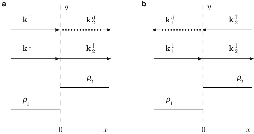
Fig. 17.7 The direction of the wave propagation in the case of a switch-on shock (a) and a switch-off shock (b)
