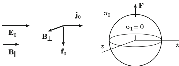
Fig. 20.11 The expulsion force \mathbf{F} acting on the non-conducting ball submerged in a conducting fluid with electric and magnetic fields
