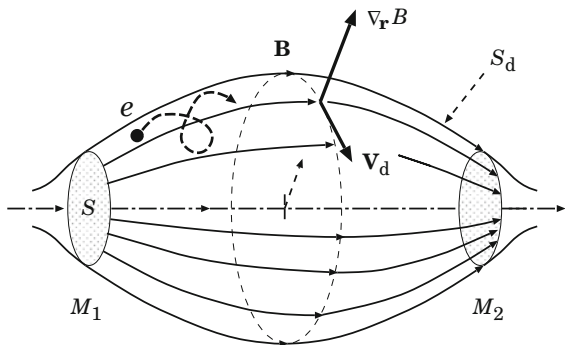
Fig. 6.5 Particle drift in a trap, due to the radial gradient of field
