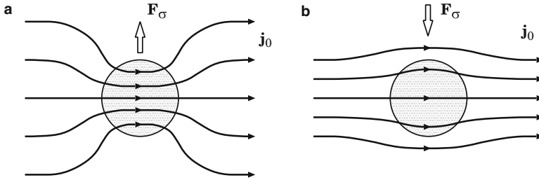
Fig. 19.6 Opposite orientation of the \sigma -dependent force in two opposite cases: (a) \sigma_1 > \sigma_0 and (b) \sigma_1 < \sigma_0 . Appearance of a non-uniform distribution of electric current is shown
