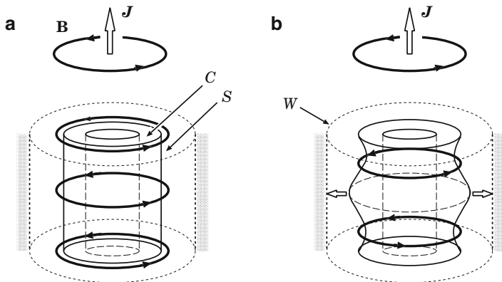
Fig. 19.4 (a) An equilibrium plasma configuration. (b) Unstable perturbations of the outer boundary
