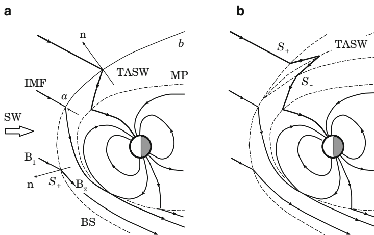
Fig. 17.11 (a) 2D schematic of the bow shock (BS) with the primary trans-Alfvénic shock wave (TASW) segment ( ab ); vector \mathbf{n} is a normal to the shock front. The magnetopause (MP) is shown for reference. (b) Disintegration of the bow shock: TASW is a secondary trans-Alfvénic shock; S_+ and S_- are fast and slow shocks, respectively
