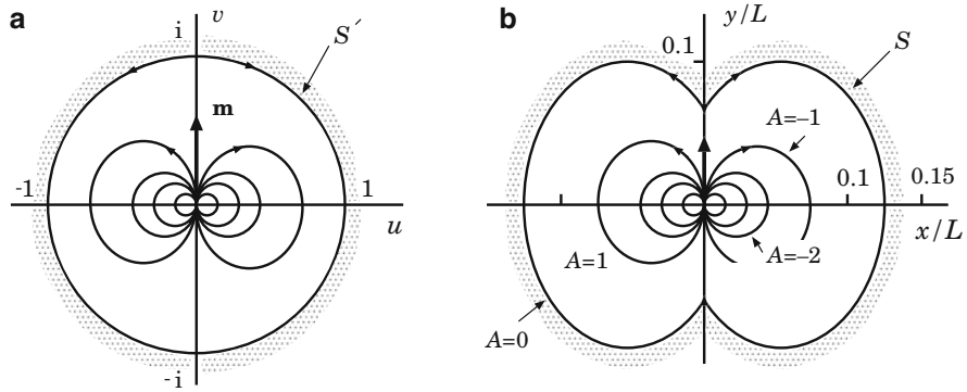
Fig. 14.8 The field lines of a plane dipole \mathbf{m} inside: (a) the unit circle in the plane w , (b) the cavity in a plasma of constant pressure
