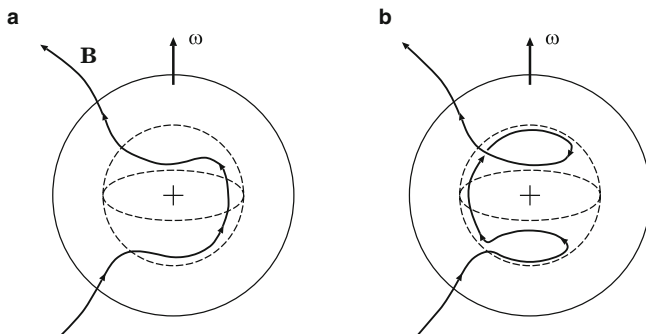
Fig. 20.3 Differential rotation creates the toroidal ( B_\phi ) component of a magnetic field inside a star
