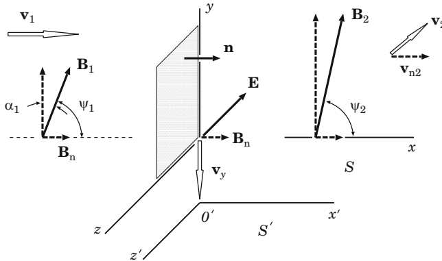
Fig. 18.4 A quasi-perpendicular shock wave in the frame of reference S where \mathbf{v}_1 \parallel \mathbf{n}
