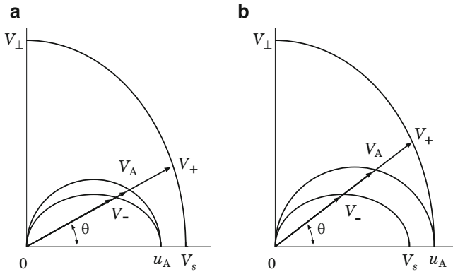
Fig. 15.2 The phase velocities of MHD waves versus the angle \theta for the two cases: (a) u_A < V_s and (b) u_A > V_s
