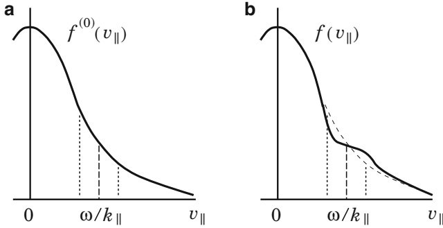
Fig. 7.1 The Landau damping. (a) The initial distribution function of thermal electrons with some narrow region centered at the resonance with the wave. (b) The distribution function after an evolution due to interaction of the electrons with the wave
