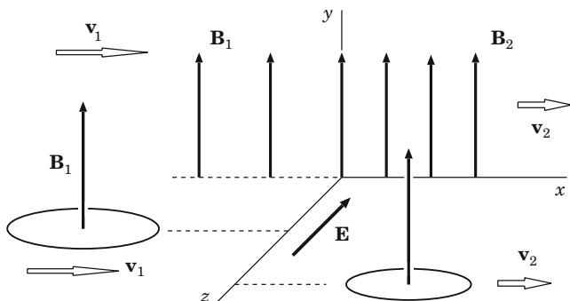
Fig. 18.2 The Larmor ring moves together with the plasma and the magnetic field across the perpendicular shock front
