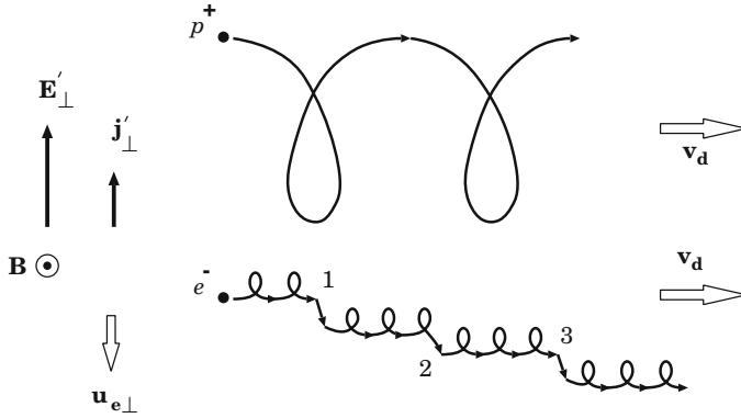
Fig. 11.2 Initiation of the current in the direction of the perpendicular field \mathbf{E}'_{\perp} as the result of rare collisions (1, 2, 3, ...) against a background of the electric drift. Only collisions of electrons are shown
