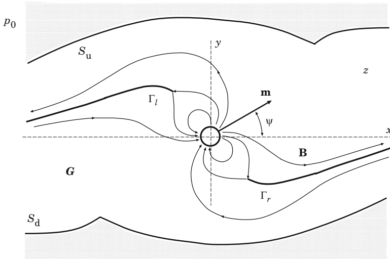
Fig. 14.9 A model of the star magnetosphere with an accretion disk; \Gamma_l and \Gamma_r are the cross sections of the disk. The plane z corresponds to the complex variable z = x + iy . S_u and S_d together with \Gamma_l and \Gamma_r constitute the boundary of the singly connected domain G in the plane z
