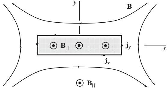
Fig. 14.3 A model of a reconnecting current layer with a longitudinal component \mathbf{B}_{\parallel} of a magnetic field
