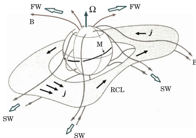
Fig. 12.5 A model of a wavy reconnecting current layer (RCL). Traditional view of the solar wind origins suggests that the fast wind (FW) blows along the open magnetic field lines, whereas the slow wind (SW) emanates from the coronal streamers
