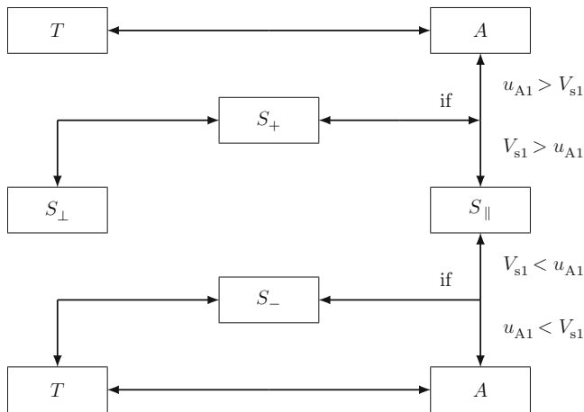
Fig. 16.11 A scheme of the continuous transitions between discontinuous solutions in MHD, following from comparison of the properties of the discontinuities and small-amplitude waves on the phase velocity diagram
