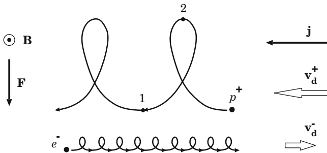
Fig. 5.10 The physical nature of the drift under the action of a non-magnetic force \mathbf{F} which is perpendicular to the uniform magnetic field \mathbf{B}
