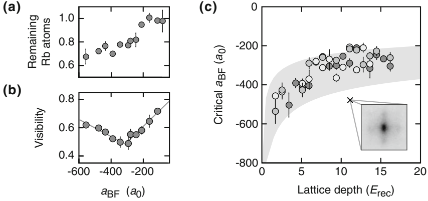
Fig. 8.5 Critical interspecies scattering lengths for the loss dominated regime at attractive interactions. The experimentally observed loss feature of ^{87}\text{Rb} atoms (a) is accompanied by a simultaneous minimum in the visibility versus interspecies interaction (b), shown here for V_{\text{lat}} = 9 E_{\text{rec}} and N_F = 2 \times 10^5 fermions. (c) The critical interspecies interactions obtained from bilinear fits to the visibility data are shown as a function of lattice depth. Darker colors indicate higher fermion numbers N_F . The gray shaded area shows a theoretical estimate of the scattering length, at which bosonic three-body losses become relevant on the scale of the experimental hold time (see main text). The inset shows a typical time-of-flight image in the loss-dominated regime with increased visibility ( V_{\text{lat}} = 11 E_{\text{rec}} and a_{BF} = -480 a_0 )
