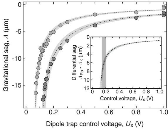
Fig. 5.6 Measurement of the gravitational sag \Delta for ^{87}\text{Rb} (dark gray dots) and ^{40}\text{K} (light gray dots). The conversion of dipole trap control voltage to beam power is P_x = U_x \cdot 0.95 \text{ W/V} . Dashed lines show the results of the numerical trap model, the gray shaded areas correspond to a 10 % error in the voltage-to-power conversion. The agreement between measurement and numerical model is excellent. The inset shows the calculated differential sag between ^{87}\text{Rb} and ^{40}\text{K} corresponding to the distance of the cloud centers in a noninteracting Bose-Fermi mixture. The gray bar indicates the operating range of the dipole trap in the experiments with Bose-Fermi mixtures. The typical differential sag is about 6 \mu\text{m}
