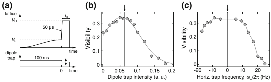
Fig. 7.10 Minimization of underlying confinement for quantum phase revival dynamics. a Picking a revival at a hold time t_0 of about 2.5 ms, we vary the intensity of the dipole trap laser and b monitor the change of the visibility at the revival, identifying a clear maximum. c Converting the dipole trap intensity to trap frequency using the model outlined in Sect. 5.3, we find that maximal coherence time is observed at the expected point of vanishing harmonic confinement \omega_{\perp} = 0 (arrow)
