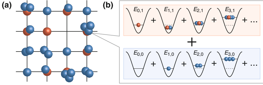
Fig. 9.1 Few-body on-site states of a delocalized Bose-Fermi mixture. a In a shallow optical lattice both the bosonic and the fermionic species are delocalized and show atom number fluctuations. The cartoon picture displays a possible result of a projection measurement assuming an average fermionic filling of \bar{m} = 0.5 . Blue (red) balls indicate bosons (fermions). b The local quantum state at a lattice site corresponds to coherent superpositions of bosonic atom number states with and without a fermion with eigenenergies E_{n,m} (see main text)
