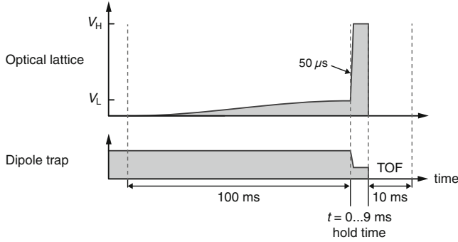
Fig. 7.7 Experimental sequence as described in the text
