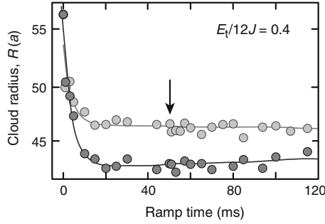
Fig. 6.8 Experimental determination of the optimal ramp time for lattice loading. The in-situ cloud size is measured at intermediate compression ( E_t/12J = 0.4 ) as a function of the ramp time, both for a noninteracting (black) and an interacting ( U/12J = 1.0 , gray) spin mixture. The rapid initial decrease of the cloud size can be attributed to improved spatial redistribution of atoms during the ramp and corresponds to better adiabaticity. The slowly increasing radii for longer ramp times mainly originate from heating effects in the optical lattice. The arrow indicates the ramp time of 50 ms used in the experiment, which is a compromise between adiabaticity and heating
