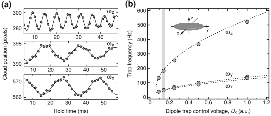
Fig. 5.7 Comprehensive measurement of trap frequencies using spin-polarized ^{40}\text{K} . a Oscillations along the individual axes at U_x = 0.14 V (corresponding to P_x \approx 135 mW). The momentum of the oscillating cloud is monitored after time-of-flight expansion. The corresponding oscillation frequencies are obtained from a fit (solid lines) yielding \omega_z = 2\pi \times 185 Hz (top), \omega_y = 2\pi \times 51 Hz (middle) and \omega_x = 2\pi \times 47 Hz (bottom). b Measurements of the trap frequencies at several power levels yield a full characterization of the trapping potential as a function of the beam power ( P_x \propto U_x , see above). The dashed lines are the result of our numerical ab-initio model. The gray-shaded area highlights the data of panel a
