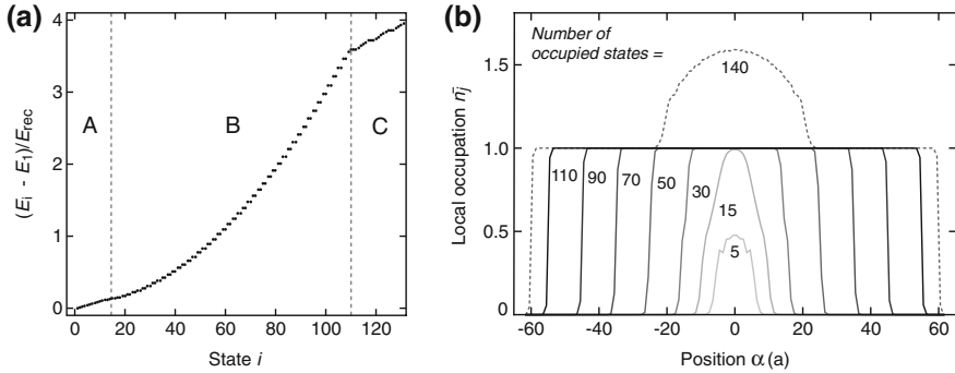
Fig. 3.8 (a) Single-particle spectrum as a function of the quantum number i for a one-dimensional 8 E_{\text{rec}} lattice with a harmonic confinement of \omega_\alpha = 2\pi \times 200 \text{ Hz} (same parameters as in Fig. 3.7). (b) Formation of a band insulator. Noninteracting fermions at T = 0 fill the eigenstates from bottom up. The local occupation \bar{n}_j is shown for an increasing number of fermions N (solid lines with increasing darkness). The band insulating state is reached at about N \approx 110 . When more single-particle states are occupied, population enters the second band shown as gray dashed line
