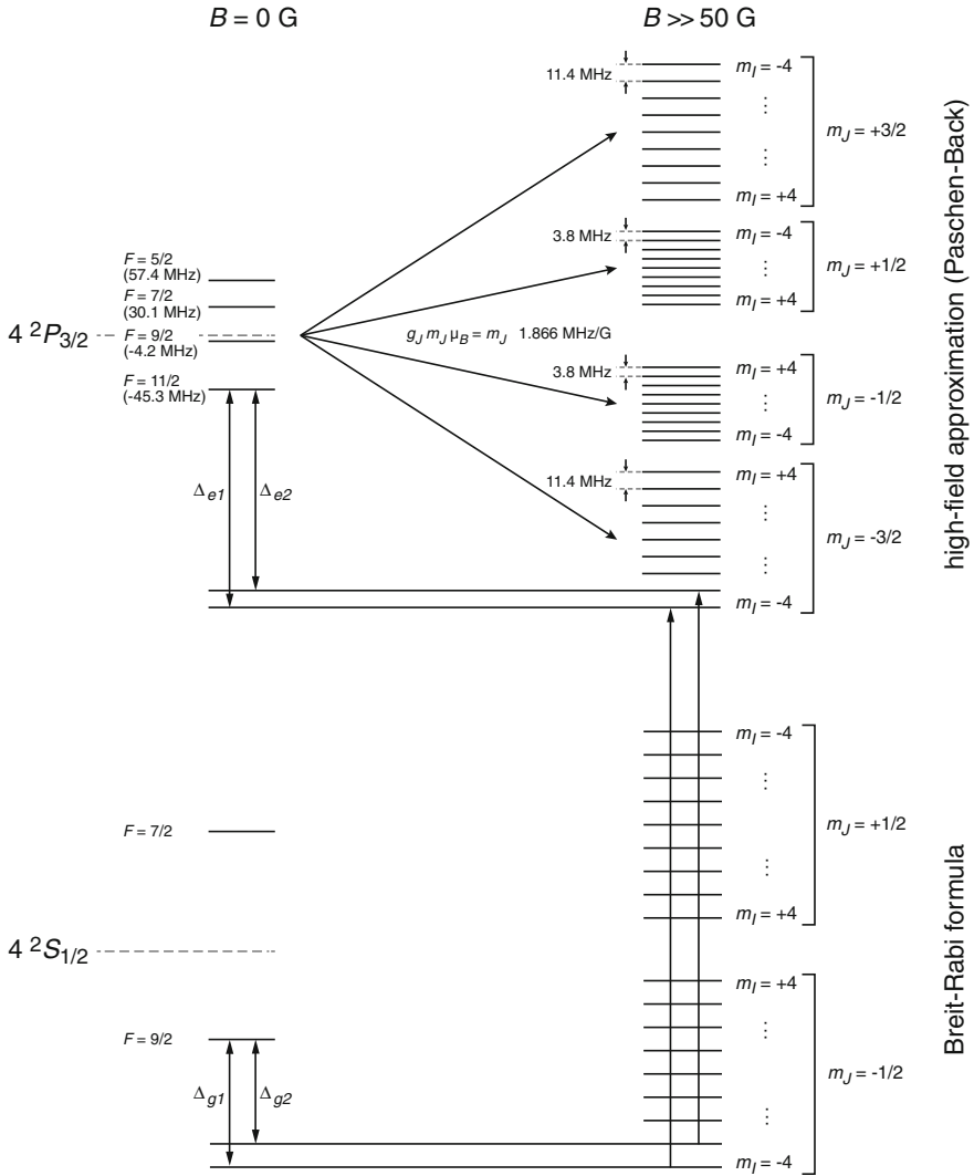
Fig. B.3 Shifts in the potassium 4^2S_{1/2} and 4^2P_{3/2} manifolds at high magnetic fields that are relevant to high-field phase contrast imaging. The ground state \Delta_{g1} and \Delta_{g2} are obtained using the Breit-Rabi formula, while the excited state allows to use the Paschen-Back formula (B.3) to calculate \Delta_{e1} and \Delta_{e2}
