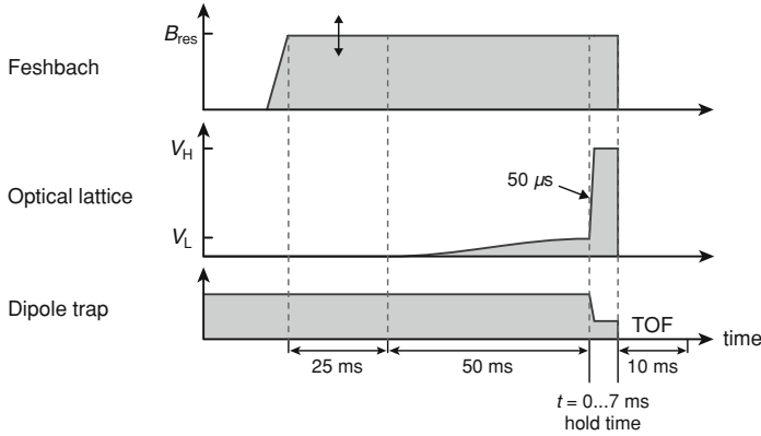
Fig. 9.3 Visualization of the experimental sequence. The steps of the sequence are timed to ensure adiabatic preparation, on the one hand, and minimal total duration to avoid heating or atom loss, on the other hand
