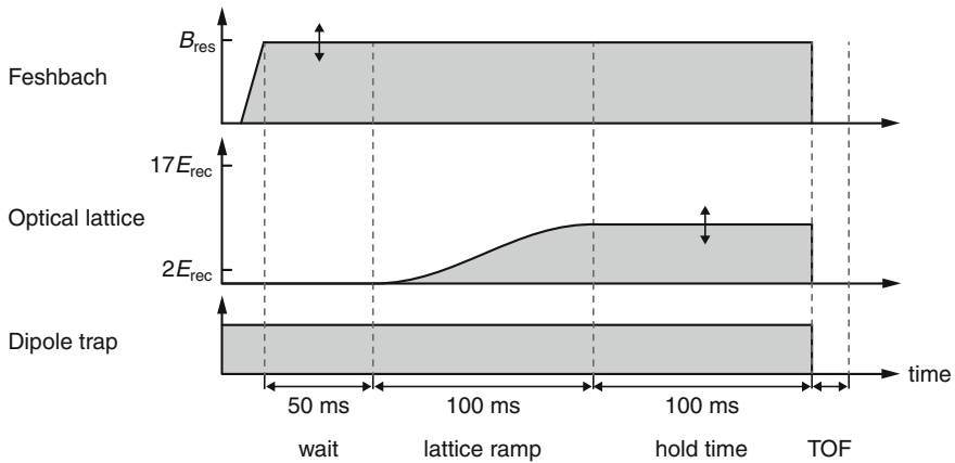
Fig. 8.2 Experimental sequence to adiabatically load a Bose-Fermi mixture into a 3D optical lattice. Measurements are performed at various magnetic fields, corresponding to various interspecies scattering length a_{BF} , and lattice depths ranging from 2 to 17 E_{\text{rec}}
