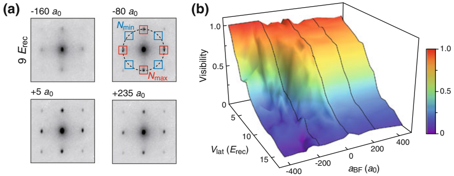
Fig. 8.3 a Time-of-flight images of the bosonic component of an interacting Bose-Fermi mixture in a V_{\text{lat}} = 9 E_{\text{rec}} deep lattice. The influence of interspecies interactions on the bosonic interference pattern is shown in four exemplary images ranging from strong attraction to strong repulsion. The visibility (see Eq. 8.3) is used to quantitatively measure the contrast of the patterns. b The visibility of the bosonic component in mixtures with about N_B = 4 \times 10^5 ^{87}\text{Rb} and N_F = 3 \times 10^5 ^{40}\text{K} atoms is shown as a function of the lattice depth V_{\text{lat}} and the interspecies scattering length a_{\text{BF}} . The lattice depth in units of the respective recoil energy is identical for the bosonic and the fermionic component ( \lambda_{\text{lat}} = 755 \text{ nm} )
