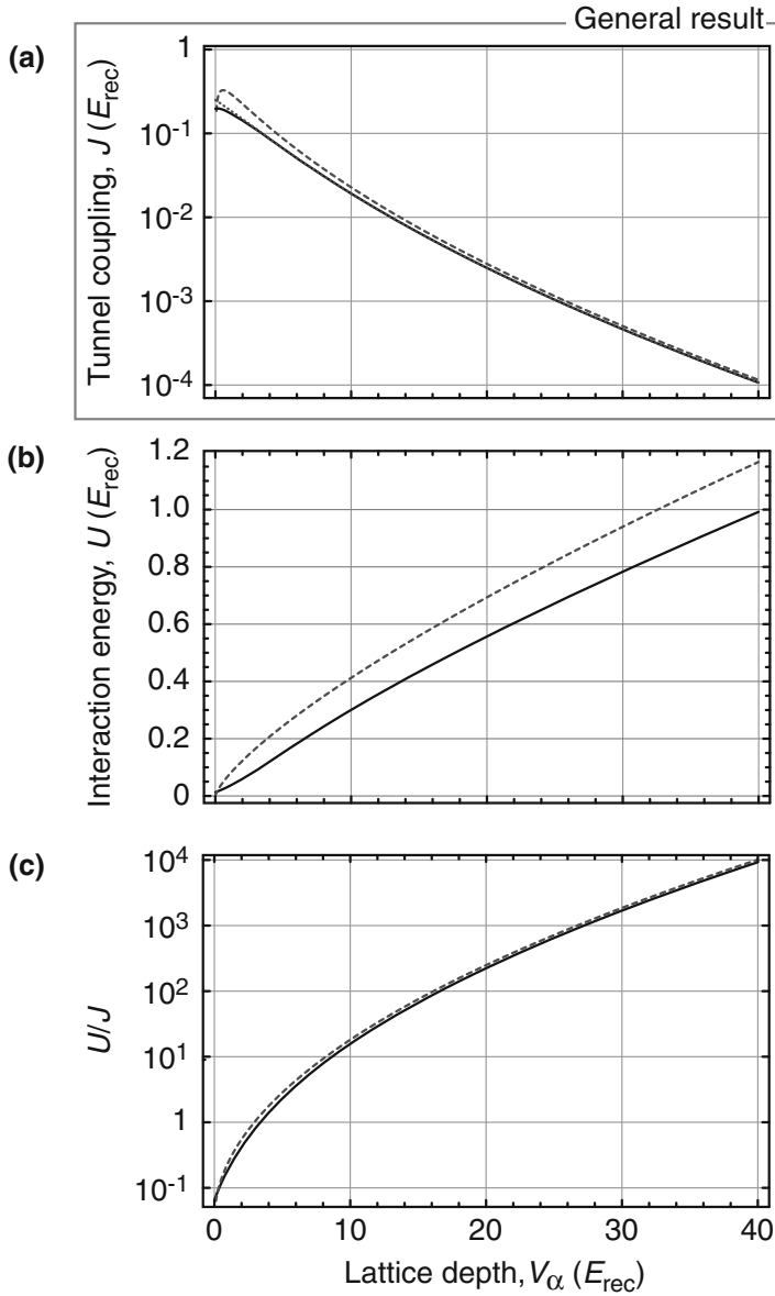
Fig. 3.2 Tunneling and interaction matrix elements. a The tunneling matrix element is calculated numerically ( solid ) and using the approximate formulas 3.14 ( dashed ) and 3.15 ( dotted ). The results are independent of the atomic species or lattice constant ( a = \lambda/2 ), because V_{\alpha} ( \alpha = x, y, z ) and J are given in units of E_{\text{rec}} . b On-site interaction energy U for ^{87}\text{Rb} in the |F, m_F\rangle = |1, +1\rangle state ( a_s = 102 a_0 ) as a function of the depth of a three-dimensional 738 nm-lattice. The exact numerical result and the harmonic approximation 3.17 are shown as solid and dashed lines, respectively. c The relative strength of the interaction U/J can be tuned over several orders of magnitude. The solid curve shows the exact numerical result, the dashed curve uses the approximations in 3.15 and 3.17
