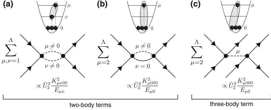
Fig. 7.6 Second-order diagrams relevant to the generation of effective two- and three-body interactions. a, b Diagrams of this type give rise to two-body interactions within the second order shift. Their contributions are canceled by introducing the counter term proportional to an adjustable constant A (see Eq. 7.38) for proper renormalization. c This diagram exemplarily shows a process generating three-body interactions. Two atoms in the lowest vibrational state \mu = 0 collide promoting one atom to a higher-lying state \mu \neq 0 that subsequently collides with a distinct third atom in state \mu = 0 . An effective three-body interaction between the three distinct incoming atoms is created, mediated by a virtual transition to the \mu \neq 0 intermediate state. The diagrams are adapted from Johnson et al. [12]
