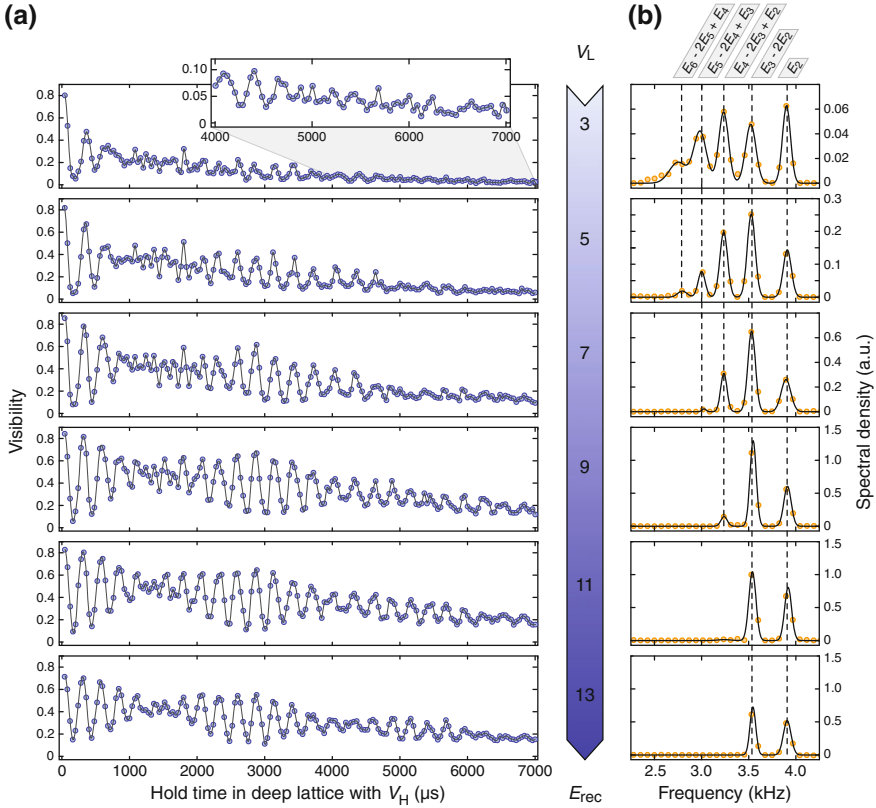
Fig. 7.13 Influence of the global atom number statistics on quantum revival spectra when the Mott insulator transition is approached. a Multi-orbital quantum revivals in a deep lattice ( V_H = 40 E_{\text{rec}} ) after adiabatic loading of 3.3(3) \times 10^5 ^{87}\text{Rb} atoms into lattices with depths ranging from V_L = 3 E_{\text{rec}} to 13 E_{\text{rec}} . The mean atom number of the individual traces differed by as little as \pm 1\% . The coherence time for shallow lattices seems significantly reduced, however, the visibility reliably shows dynamics down to the per cent level (inset). b The corresponding Fourier spectra reveal frequency contributions from Fock states containing up to six atoms. The peak positions agree with the theoretical predictions obtained from exact diagonalization (dashed vertical lines) and are independent of V_L . Number squeezing manifests itself both in reduced peak amplitudes and in a narrowing of the spectra for increasing V_L . The solid lines show Gaussian fits to the peaks
