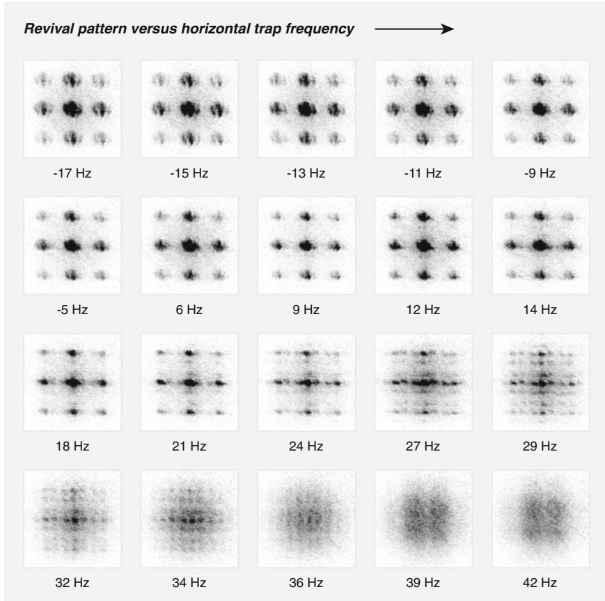
Fig. 7.15 Time evolution originating from underlying harmonic confinement; the displayed images are the raw data that entered the evaluation in Fig. 7.10. A fixed evolution time t_0 of about 2.5 ms was chosen coinciding with a strong quantum phase revival in a V_H = 40 E_{\text{rec}} deep lattice. The horizontal trap frequency \omega_{\perp}/(2\pi) was increased starting from slightly negative values, corresponding to an anticonfining potential. At vanishing confinement, the regular momentum pattern of a superfluid state appears, while more complex structures of the momentum distribution arise for increasing confinement, indicating fractional rephasing, that is higher-order Talbot fringes
