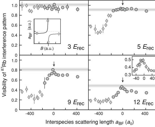
Fig. 8.4 Visibility versus interspecies scattering length at four lattice depths ranging from 3 E_{\text{rec}} to 12 E_{\text{rec}} for high fermion number ( N_F = 3 \times 10^5 ). The cuts are taken from the full data set shown in Fig. 8.3b. At lattice depths larger than 3 E_{\text{rec}} the visibility shows a maximum at a position, which is consistent with a_{\text{BF}} \approx 0 (indicated by the arrow) given the experimental uncertainties. The diamonds (circles) indicate points measured above (below) resonance, as shown in the upper inset. The gray shaded horizontal lines represent the visibility in a purely bosonic ^{87}\text{Rb} cloud measured for the same experimental parameters
