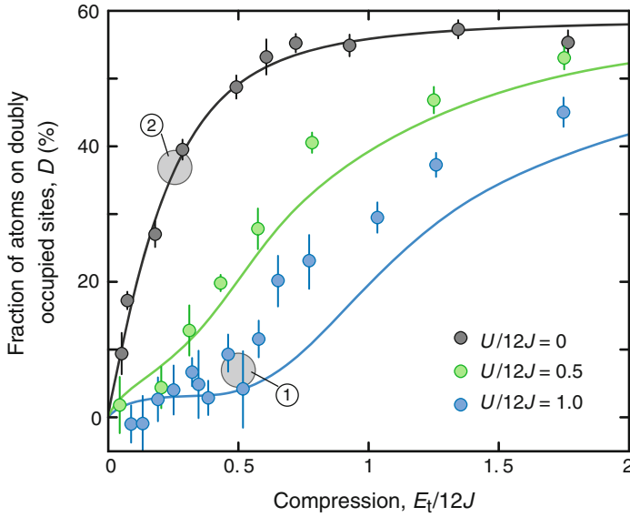
Fig. 6.9 Double occupancy D as a function of compression for the interaction strengths U/12J = 0, 0.5 and 1 . The shaded circles ① and ② indicate the fraction of atoms on doubly occupied sites for a constant cloud size R_{sc} \approx 0.5 (see Fig. 6.6), which illustrates the strong suppression of double occupancy in the interacting case. Error bars denote the standard deviation of at least four measurements
