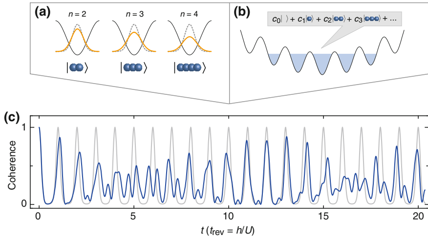
Fig. 7.3 Signature of multi-body interactions in quantum phase revivals. a For repulsive interactions, virtual transitions to higher lattice orbitals broaden the ground-state wavefunction at a lattice site depending on the atom number ( orange solid lines ). This gives rise to characteristic Fock state energies, which can be described by effective multi-body interactions. b A BEC loaded into a weak optical lattice forms a superfluid in which each atom is delocalized over several lattice sites. The quantum states at each site can be expressed as a superposition of Fock states, |n\rangle , with amplitudes c_n . c Quantum phase revivals of a coherent state of interacting atoms in the multi-orbital system of a deep lattice well ( blue solid line ). The beat signal indicates coherent multi-body interactions. The dynamics are markedly different from the monochromatic evolution expected in a single-orbital model with a single two-body interaction energy, U ( gray solid line )
