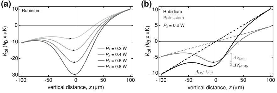
Fig. 5.5 Numerically calculated potential profiles V_{\text{tot}}(0, 0, z) of the crossed dipole trap along the vertical axis taking into account gravity and the experimental beam parameters. a Potential for rubidium at various laser powers. Gravitational sag strongly pulls the trap minimum ( black dots ) downwards for lower laser powers. b Additionally, the effective trap depth for rubidium \Delta V_{\text{eff,Rb}} is effectively lower than \Delta V_{\text{eff,K}} when the laser power stays below a certain critical level. Therefore, dominantly rubidium is lost when the laser power is reduced during final evaporation. The differential sag is \Delta_{\text{Rb}} - \Delta_{\text{K}} \approx 5 \mu\text{m} . Dashed lines indicate the pure gravitational potential for rubidium and potassium
