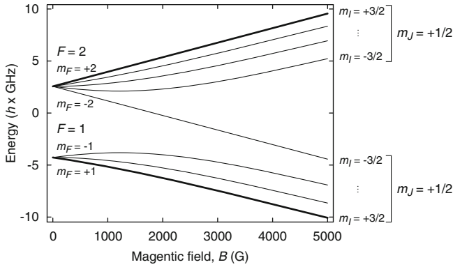
Fig. B.1 Zeeman shifts for ^{87}\text{Rb} in the 5^2S_{1/2} manifold. In the experiments of this thesis, only the magnetically trappable state |2, +2\rangle and the absolute ground state |1, +1\rangle are used ( bold lines ). The Paschen-Back regime is only reached well above 1000 G, beyond the experimentally relevant range
