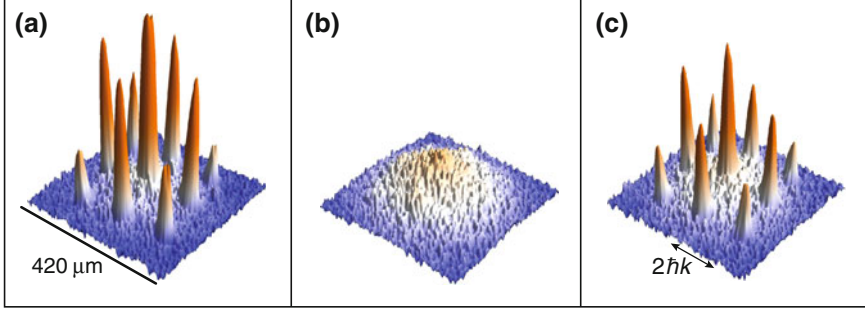
Fig. 4.2 Momentum distribution of ^{87}\text{Rb} atoms during collapse and revival dynamics in a 41 E_{\text{rec}} deep lattice. The data show three points of the evolution at hold times of a 40 \mu\text{s} (start), b 120 \mu\text{s} (collapse) and c 320 \mu\text{s} (partial revival). The data are taken from the set in Fig. 7.8. While the overall atom number is almost constant, the off-diagonal correlations vary in time and result in the emergence or suppression of interference
