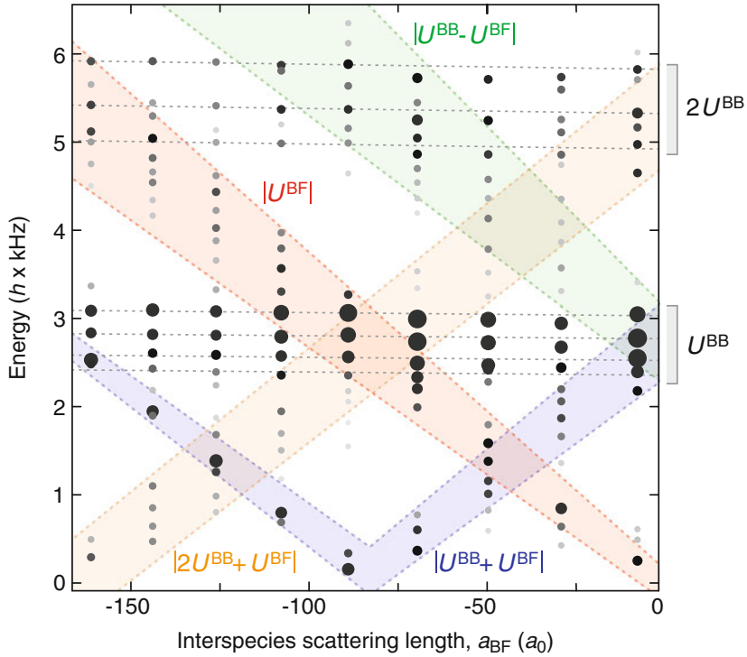
Fig. 9.7 Summary of the spectral features in a broad range of interspecies interactions. The peaks of nine Fourier spectra (including those of Fig. 9.6) are fitted by Gaussians. The resulting positions are shown as bubbles , whose size as well as gray shading indicate the peak height (the larger and darker , the higher ). Spectral components arising from direct Bose-Fermi interactions are highlighted by shaded areas corresponding to energies of order |U_{\text{BF}}| (red), |U_{\text{BB}} - U_{\text{BF}}| (green), |U_{\text{BB}} + U_{\text{BF}}| (blue) and |2U_{\text{BB}} + U_{\text{BF}}| (orange). Additionally, black dashed lines serve as guides to the eye for the energies of orders U_{\text{BB}} and 2U_{\text{BB}} . Note that the three data sets between a_{\text{BF}} = -75 a_0 and -25 a_0 are measured at a slightly lower lattice depth V_{\text{H}} = 26.7(3) E_{\text{rec}}^{\text{B}} . This explains the slight shift with respect to the other data
