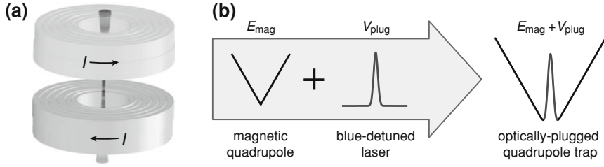
Fig. 5.3 Optically-plugged magnetic quadrupole trap. a A coil pair with counterpropagating currents I creates a magnetic quadrupole field that vanishes at the trap center and increases linearly in all directions. A blue-detuned laser is focussed along the symmetry axis. b Schematic of the combined magnetic and optical potentials
