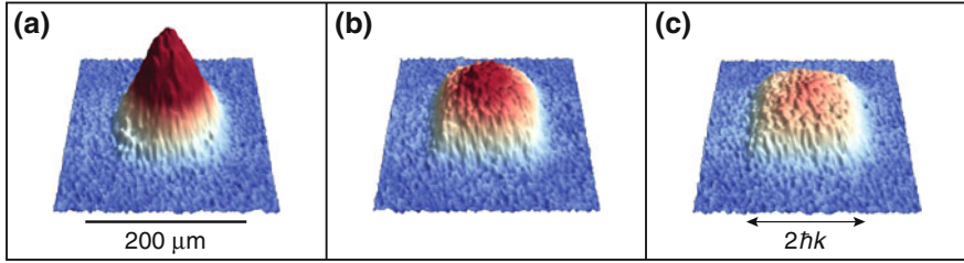
Fig. 4.5 Brillouin zone mapping reveals the quasi-momentum distribution for a noninteracting spin mixture of ^{40}\text{K} in a 8 E_{\text{rec}} lattice. While the overall atom number is approximately constant, the filling of the Brillouin zone varies as a function of the external harmonic confinement corresponding to a \omega_{\perp} = 2\pi \times 46 Hz, b 2\pi \times 90 Hz and c and 2\pi \times 157 Hz. For the strongest harmonic confinement the first Brillouin zone is homogeneously filled and population in higher Brillouin zones is negligible. This observation is compatible with the formation of a band insulator in the center of the trap, which is independently confirmed by a cloud size measurement. (Images are selected from the black data in Fig. 6.6)
