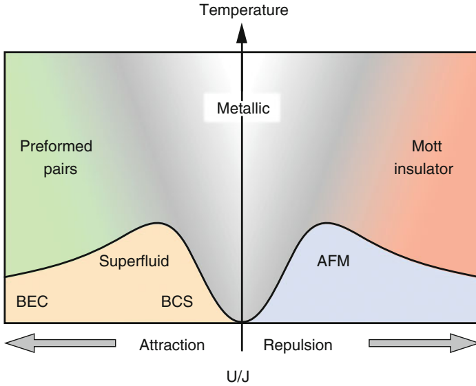
Fig. 3.5 Sketch of the phase diagram for the Fermi-Hubbard model at half-filling in a three-dimensional optical lattice (adapted from reference [20]). The following abbreviations have been used: molecular Bose-Einstein condensate (BEC), Bardeen-Cooper-Schrieffer (BCS) and anti-ferromagnetic phase (AFM)
