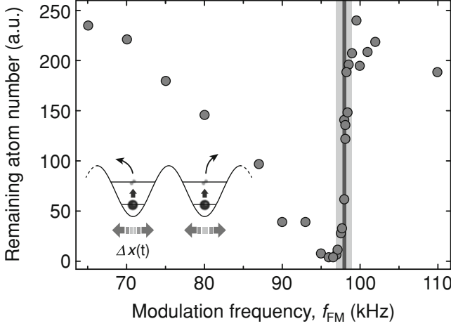
Fig. 5.9 Lattice calibration via frequency-modulation spectroscopy. The data shows a resonance between the first and second band at 98.2 \pm 1.0 kHz, which corresponds to a lattice depths of 34.9 \pm 0.6 E_{\text{rec}}^{\text{F}} . The light-gray shaded area indicates the experimental uncertainty of the resonance position. The dark-gray shaded bar represents the width of the resonance as expected from a band structure calculation. The inset illustrates frequency modulation spectroscopy (see main text)
