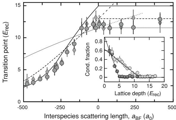
Fig. 8.6 Shift of the Mott insulator transition as a function of interspecies interaction. The diamonds ( circles ) represent the experimental runs at N_F = 2 \times 10^5 = N_B/2 ( N_F = 3 \times 10^5 = 3N_B/4 ). The error bars include the fit uncertainty and the average over typically two experimental runs. The lines show theoretical results for the transition point as obtained by the variational model for n = 1 ( dotted line ) as well as exact diagonalization for Mott shells with n = 1 ( dashed line ) and n = 2 ( solid line ) bosons. For a_{BF} > 0 the solid lines correspond to a phase separation scenario, while the dashed lines would correspond to a scenario, in which bosons and fermions occupy the same sites. The inset shows the behavior of the condensate fraction at a_{BF} = -295 a_0 ( black circles ) and a_{BF} = +235 a_0 ( gray circles ) at N_F = 2 \times 10^5 . The black solid lines show bilinear fits to the data. The kink determines the respective critical lattice depth V_{\text{lat}}^{\text{crit}} corresponding to the transition point
