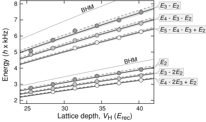
Fig. 7.11 Quantum phase revival energies in a multi-orbital system. Long collapse and revival traces have been recorded under identical loading conditions ( V_L = 8 E_{\text{rec}} ), but variable lattice depth V_H during phase evolution. The contributing frequencies f_{mn} of orders U/h and 2U/h have been derived using numerical Fourier transform and are plotted as energies h \times f_{mn} . The typical experimental uncertainty is \pm 50 h \times \text{Hz} . The shading of the data points reflects the relative spectral weight (the darker the higher). The solid lines with grey shading indicate the theoretically expected energies. They have been calculated using exact diagonalization (see Sect. 7.2.4) with an on-site basis set of 4^3 orbitals at an s -wave scattering length of a_s = 102(2) a_0 , where a_0 is the Bohr radius. A calculation using a smaller basis set with 3^3 orbitals yields slightly higher energies ( dashed lines ). The dotted lines show the single-orbital interaction energies U and 2U that have been calculated using Wannier orbitals, which are commonly used in the Bose-Hubbard model (BHM). At low lattice depth we can only resolve the strongest peaks owing to smaller peak spacings
