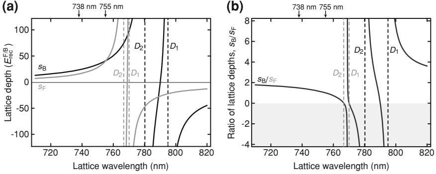
Fig. 5.8 Species-dependence of the optical lattice. a Lattice depth for ^{87}\text{Rb} (black, index B) and ^{40}\text{K} (gray, index F) as a function of wavelength. The depths are displayed in units of the respective recoil energy. A Gaussian standing wave with a total power of P = 100\text{ mW} and a beam waist of w_0 = 170\text{ }\mu\text{m} are assumed, corresponding to typical experimental parameters. b Ratio s_B/s_F of lattice depths for ^{87}\text{Rb} and ^{40}\text{K} as a function of the wavelength. Negative values indicate that the lattice has opposite detunings for the two species (gray shading). Dashed lines indicate the position of the respective D_1 and D_2 lines
