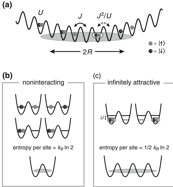
Fig. 6.11 Attractively interacting fermionic spin mixture and finite entropy. a The cloud size R is determined by the interplay between entropy and several energy scales: The interaction energy U , the tunneling matrix element J and the characteristic trap energy E_t . Additionally, the tunnel coupling J^2/U of bound atom pairs becomes relevant at strongly attractive interactions. b, c Configurations of two fermions (spin up and down) in a zero-tunneling double well potential. For vanishing interactions there are four possibilities to arrange the atoms. In the limit of infinitely attractive interactions the atoms are tightly bound, merely allowing for two configurations. Therefore, the entropy per lattice site is reduced by a factor of two. The atom cloud is forced to expand in order to accommodate the total entropy present in the finite-temperature system
