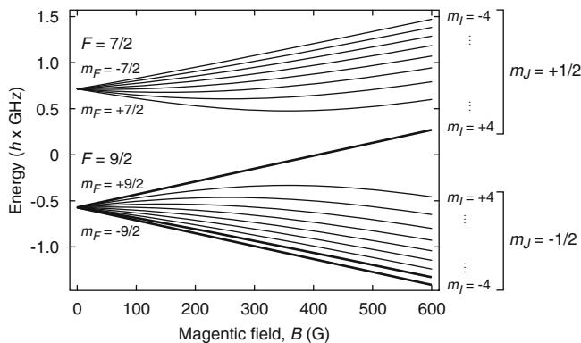
Fig. B.2 Zeeman shifts for ^{40}\text{K} in the 4^2S_{1/2} manifold. Mainly the magnetically trappable |9/2, +9/2\rangle state and the two lowest lying states |9/2, -7/2\rangle and |9/2, -9/2\rangle are used in this work ( bold lines ). The Paschen-Back approximation is not applicable for the experimentally relevant magnetic fields below 600 G
