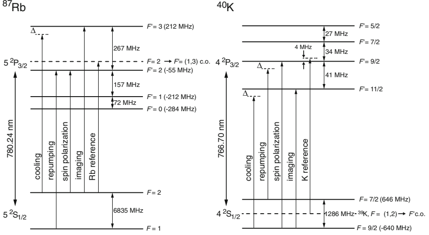
Fig. 5.1 Level scheme for the D_2 lines of ^{87}\text{Rb} and ^{40}\text{K} and corresponding optical transitions used in the experimental sequence. Cooling and repumping denote the transitions used for laser cooling. Spin polarization is used to transfer the atoms to hyperfine sublevels that are magnetically trappable. Absorption and phase-contrast images are recorded on the imaging -transition. The \Delta indicates that the potassium cooling and repumping transitions are detuned, but the exact detunings are different. Strong reference transitions are stabilized and used to lock the other laser frequencies by means of offset-locks. The label c.o. indicates crossover resonances
