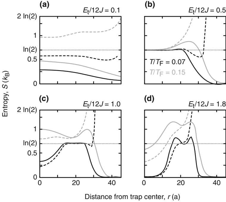
Fig. 6.12 a–d Calculated spatial entropy distribution of a balanced spin mixture for various compressions and fixed global atom number N ( N_\uparrow = N_\downarrow = N/2 ). The interaction parameter is strongly repulsive U/12J = 1.5 . The solid (dashed) lines show the entropy per lattice site (per particle) for initial temperatures of T/T_F = 0.07 ( black ) and T/T_F = 0.15 ( gray ). Identical entropy per particle and lattice site of \ln(2) indicates a Mott insulating phase with unity filling, but without magnetic ordering. A Mott insulating core is clearly visible in b for both temperatures. The calculations have been performed by Theo Costi, Achim Rosch and collaborators published in the supplementary online material of [4]
