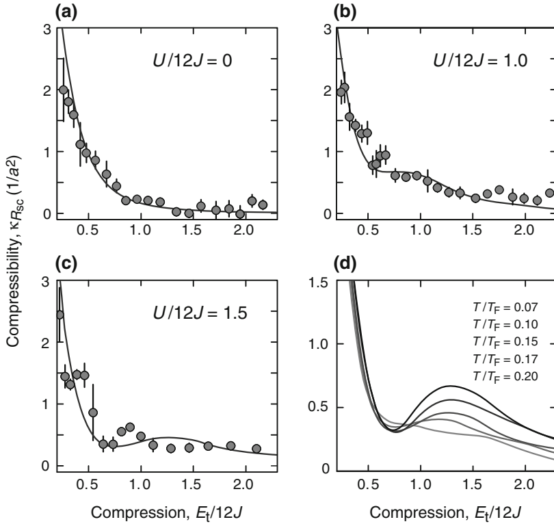
Fig. 6.7 a–c Global compressibility \kappa_{R_{sc}} as a function of the compression for several interactions. Each data point corresponds to the linear slope of four consecutive points in the cloud size data (see Fig. 6.6). Error bars represent the uncertainty of the fit. Solid lines show the theoretically expected results for an initial temperature T/T_F = 0.15 . Panel d illustrates the influence of the initial temperature on the calculated compressibility at strong repulsion U/12J = 1.5
