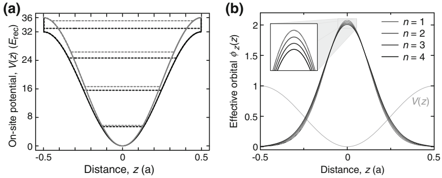
Fig. 7.4 a On-site potential at lattice depth V_{\text{lat}} = 32 E_{\text{rec}} and V_{\text{lat}} = 36 E_{\text{rec}} with hard boundary conditions. The dashed lines show the lowest lying single-particle energies with three and four classically bound states, respectively. b The effective one-dimensional ground state wavefunction in a V_{\text{lat}} = 40 E_{\text{rec}} lattice is modified as a function of the filling n = 1 to 4 for interacting ^{87}\text{Rb} atoms. The black solid line shows the single-particle on-site wavefunction \phi_1(z) calculated on an individual lattice site with hard boundary conditions (see a ). \phi_1(z) is essentially identical to the Wannier function w(z) of the lowest lattice band ( dashed line ). The figure is displayed with kind permission of Dirk-Sören Lühmann [46]
