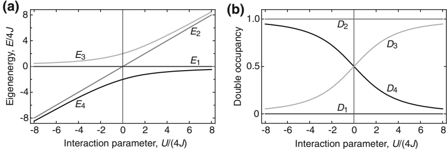
Fig. 3.4 Properties of the double-well Fermi-Hubbard model with a spin up and a spin down particle. The eigenenergies (a) and the double occupancy (b) of the four eigenstates are shown as a function of the normalized interaction U/(4J)
