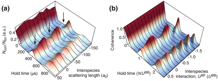
Fig. 9.4 Interference of Bose-Bose and Bose-Fermi phase dynamics. a The measured initial quantum phase revivals are modulated as a function of the interspecies scattering length a_{\text{BF}} . The intraspecies scattering length a_{\text{BB}} is fixed at +102(2) a_0 . The first revival is suppressed at a_{\text{BF}} = -126(2) a_0 , -40(3) a_0 and +41(3) a_0 , as marked by the arrows. Black lines indicate the traces recorded in the experiment. b The general structure of the experimental data is well captured by the simple model of Eq. 9.7. In the simulation the bosonic filling is kept fixed at \bar{n} = 0.85 and the fermionic filling is varied according to the results extracted from a (see also inset of Fig. 9.9). Additionally, a temporal exponential decay comparable to the experimental data ( \tau = 1.1 ms) is applied
