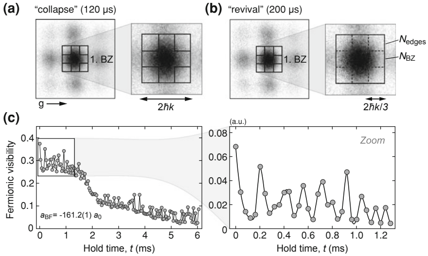
Fig. 9.11 Quantum phase revival dynamics of the fermionic component in a Bose-Fermi mixture. Exemplary momentum distributions recorded after 10 ms time-of-flight expansion show a collapse a and a revival b , which are hardly discernible with the bare eye. The interspecies attraction is a_{\text{BF}} = -161.2(1) a_0 and the lattice depth V_{\text{H}}^{\text{F}} = 18.8(2) E_{\text{rec}}^{\text{F}} . c Evaluation of the fermionic visibility \tilde{V} (see Eq. 9.26) clearly reveals collapse and revival dynamics arising from the interspecies interactions U^{\text{BF}} . The kink at about t = 2 ms arises due to dephasing induced by superimposed Bloch oscillations [26] along the direction of gravity. Therefore, the analysis is restricted to the first 1.2 ms. The baseline \tilde{V} = 0 corresponds to a homogeneously filled first Brillouin zone
