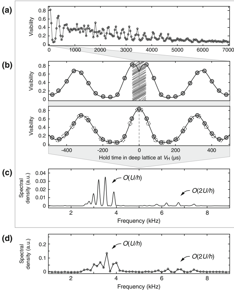
Fig. D.1 Processing of quantum phase revival traces and numerical Fourier analysis. a The measured data points, which are typically spaced by 40 \mu\text{s} , are interpolated using cubic splines (solid line). b Typically, the first 30 \mu\text{s} of the interpolated curve are removed to compensate for the 50 \mu\text{s} ramp from V_L to V_H (crossed-out area). Furthermore, a simple exponential decay is appended to the data for times longer than the original observation times (see text). The resulting long interpolation curve is concatenated to its mirror image and the resulting composite curve is again sampled in steps of 40 \mu\text{s} (solid circles). The positions of the original data points are shown as dashed circles. c Numerical Fourier transform is applied to these data, revealing frequencies of orders U/h and 2U/h . d Direct Fourier transform of the data in a without further processing
