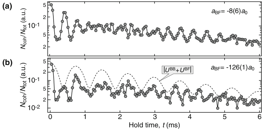
Fig. 9.5 High-resolution quantum revival traces of the Bose-Fermi system are shown for vanishing, a , and strong interspecies attraction, b . For the later case, one observes that every second revival is suppressed by an envelope ( gray dashed line ) that corresponds to the spectral components of order |U^{BB} + U^{BF}| . Each data point represents a single run of the experiment. Special care has been taken to ensure identical conditions for each run, particularly stable atom numbers. The solid lines interpolate the data and serve as a guide to the eye
