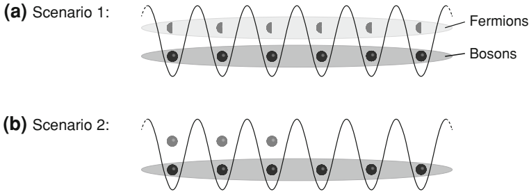
Fig. E.1 Schematic illustrations of the scenarios for the distribution of the fermions discussed in the main text. The shaded ovals indicate delocalization
