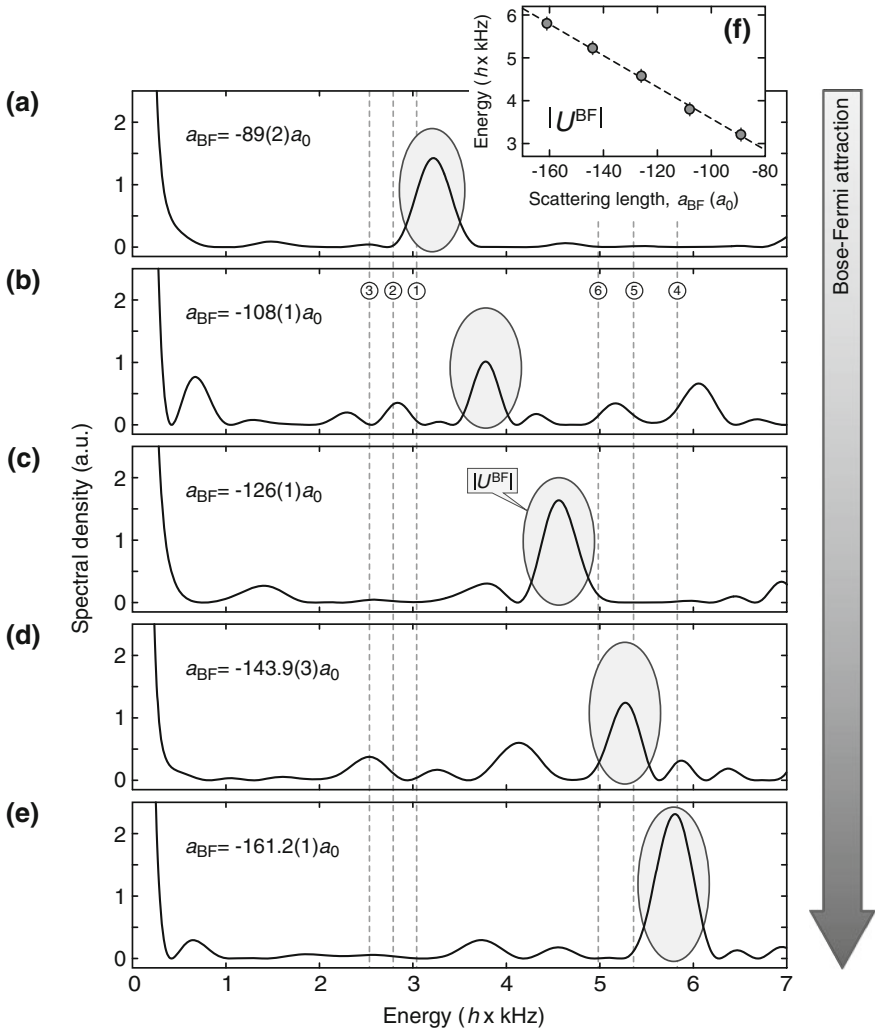
Fig. 9.12 a–e Fourier spectra of fermionic quantum revival traces for linearly increasing inter-species attraction. The spectral contribution corresponding to the Bose-Fermi interaction energy |U^{BF}| is highlighted by shaded ovals. Dashed lines (① to ⑥) indicate the locations of the contributions of orders U^{BB} and 2U^{BB} that are suppressed in the fermionic dynamics (compare Fig. 9.6). f The experimentally measured Bose-Fermi interaction energy |U^{BF}| shows a linear trend as a function of a_{BF} in analogy to our findings in Sect. 9.2
