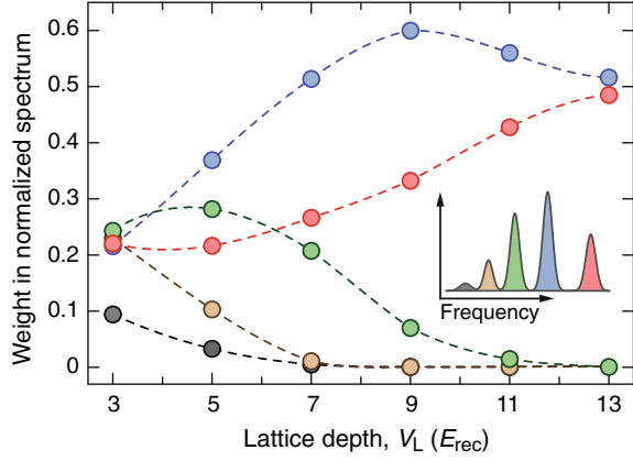
Fig. 7.14 Relative weight of frequencies in the spectra for different lattice depths V_L (see Fig. 7.13). For each spectrum the area under the individual peaks has been determined (see inset) and normalized to the area under all peaks of order U/h . The evaluation shows that the spectrum narrows down to the frequencies E_2/h and (E_3 - 2E_2)/h with the theoretical weights c_0c_1^2c_2 and c_1c_2^2c_3 , respectively
