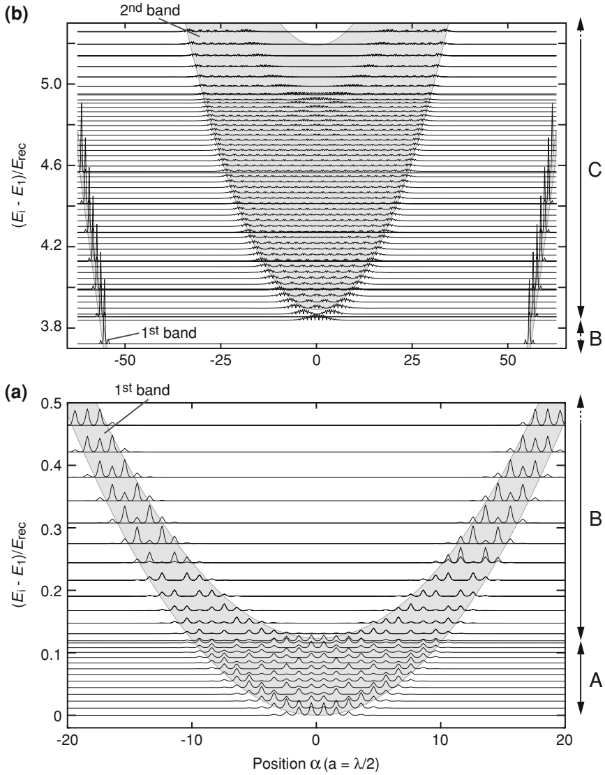
Fig. 3.7 Numerically calculated single-particle wavefunctions \phi_i(\alpha) and eigenenergies E_i in an one-dimensional optical lattice ( \lambda = 738\text{nm} ) at 8 E_{\text{rec}} with an underlying harmonic potential ( \omega_\alpha = 2\pi \times 200\text{Hz} for ^{40}\text{K} ). Solid lines indicate the probability density |\phi_i(x)|^2 that is vertically positioned at the respective eigenenergy E_i . Panel (a) shows the lowest energy states of the first band, while panel (b) displays the onset of the second band. Mind the different scaling of the position axis and the gap on the energy axis. Gray areas show the widths of the first and second band derived from a band structure calculation (see Sect. 2.2.3). The band widths are locally offset by the underlying harmonic potential
