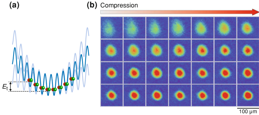
Fig. 6.1 Compression of a fermionic spin mixture. a The characteristic trap energy E_t defines the compression of the atom cloud. b In-situ phase-contrast images for strong repulsive interactions U/12J = 1.5 (see Fig. 6.6, red data). The compression of the dipole trap is continuously increased from left to right and top to bottom covering a range of horizontal trap frequencies from \omega_{\perp} = 2\pi \times 20 to 2\pi \times 120 Hz. The rescaled cloud size R_{sc} = R/(\gamma N_{\sigma})^{1/3} is derived by measuring the cloud radius R in phase-contrast images (see main text). The atom number N_{\sigma} per spin state \sigma is extracted from a subsequent time-of-flight image in the same experimental run (see Fig. 6.5)
