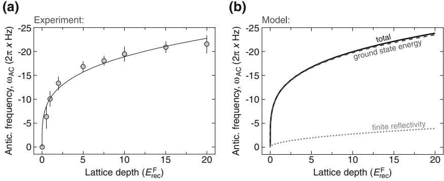
Fig. 5.11 Anticonfinement of the blue-detuned optical lattice in practice. a Measured anticonfining trap frequencies for the lattice axis along z -direction. A power law fit ( \omega_{AC} = as^b ) yields the parameters a = -10.2(7) Hz and b = 0.27(3) (black line). The exponent b is in good agreement with the dominant s^{1/4} scaling originating from the varying on-site ground state energy (see Eq. 2.67). b Anticonfining frequencies extracted from our numerical ab-initio model. The only free parameter is the reflection coefficient \rho of the retroreflection beam path (see Sect. 2.2.2). Here, \rho = 0.8 is chosen to illustrate the effect, while the actual experimental value is rather \rho \approx 0.9 . The contributions from varying ground state energy (dashed line) and finite reflectivity (dotted line) are added in quadrature to yield the total anticonfinement (black line)
