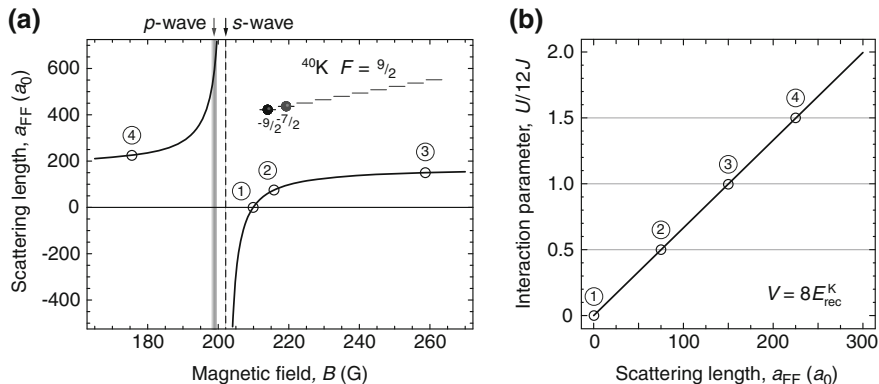
Fig. 2.15 Tunable fermionic ^{40}\text{K} spin mixture. a An s -wave Feshbach resonance between the hyperfine levels |9/2, -9/2\rangle and |9/2, -7/2\rangle is located at B_0 = 202.1 G. Slightly below at 198.8(5) G, there is a p -wave resonance (gray shaded) of atoms in the |9/2, -7/2\rangle state [55, 56]. b In Chap. 6 we investigate repulsively interacting Fermi-Fermi mixtures in an optical lattice ( \lambda = 738 nm) at discrete values of the interaction parameter U/12J = 0, 0.5, 1.0 and 1.5 . For the fixed lattice depth of V = 8 E_{\text{rec}} , these working points correspond to the magnetic fields ① 209.9 G, ② 215.8 G, ③ 258.7 G and ④ 175.5 G
