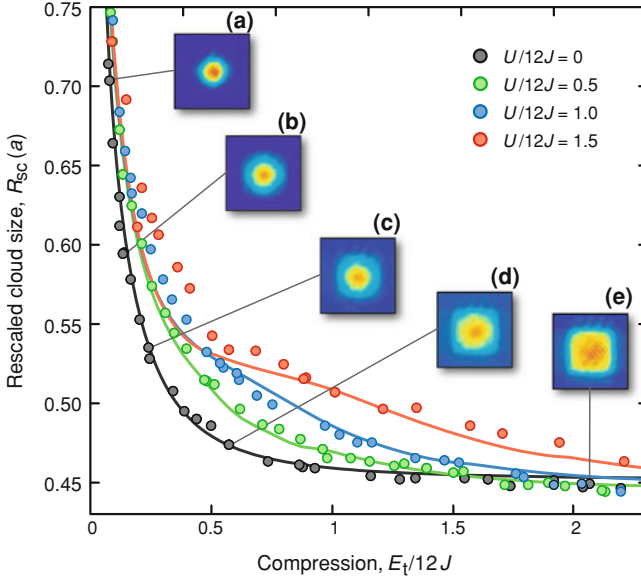
Fig. 6.6 Response of the interacting spin mixture to compression of the underlying harmonic confinement. The rescaled cloud sizes R_{sc} in a V_{lat} = 8 E_{rec} lattice are shown as a function of the external trapping potential for interactions U/12J ranging between 0 and 1.5. Circles denote individual experimental shots, while lines show the theoretical expectations obtained by DMFT for an initial temperature T/T_F = 0.15 prior to lattice loading. The insets a-e show the quasi-momentum distributions for the noninteracting case obtained via Brillouin zone mapping (averaged over several experimental shots)
