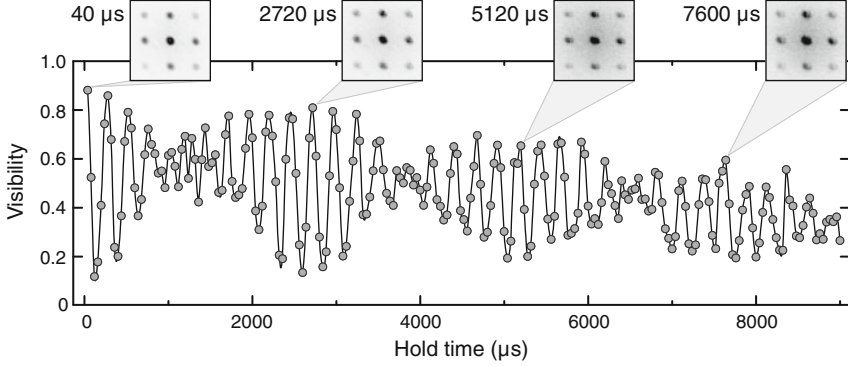
Fig. 7.8 Multi-orbital quantum revivals of a number-squeezed state. Collapse and revival dynamics of number-squeezed superposition states in a deep optical lattice. A Bose-Einstein condensate of about 1.9(3) \times 10^5 ^{87}\text{Rb} atoms was adiabatically loaded into a V_L = 8 E_{\text{rec}} lattice within 100 ms. Quantum phase evolution was induced by a nonadiabatic jump to a V_H = 41(1) E_{\text{rec}} deep lattice, while the superposition states with finite number fluctuations are preserved. The sample has an ensemble-averaged mean atom number of \langle \bar{n} \rangle \approx 1.0 and a central mean atom number of \bar{n}_c \approx 2.5 . Simultaneously with the lattice jump, the underlying harmonic confinement is instantaneously minimized to maximize the coherence time. The quantum phase dynamics show a beat signal resulting from coherent multi-body interactions. Each data point corresponds to a single run of the experiment. The solid line interpolates the data and serves as a guide to the eye
