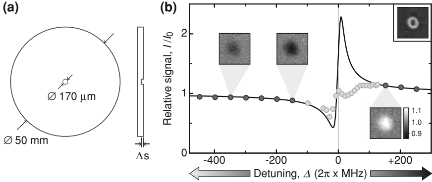
Fig. 5.13 Phase-contrast imaging with a retarding phase plate. a The retarding phase plate has a central dimple with a diameter of 170\ \mu\text{m} and a depth of \Delta s = 430\ \text{nm} . It induces a phase shift of approximately \alpha \approx -\pi/2 for both ^{40}\text{K} and ^{87}\text{Rb} . b Phase-contrast signal versus detuning for ^{40}\text{K} atoms. The data shows the relative signal I/I_0 at the center of the cloud. Dark points are fitted by the model I/I_0 = t(n, \Delta)^2 + 2 - 2\cos(\alpha) - 2t(n_{\text{col}}, \Delta)\sqrt{2 - 2\cos(\alpha)}\cos[\phi(n_{\text{col}}, \Delta) + \alpha/2] (compare Eq. 4.7) using the column density n_{\text{col}} and the phase shift \alpha as fit parameters. Gray points are excluded due to proximity to the atomic resonance. The fit yields n_{\text{col}} = 1.125 \times 10^{13}\ \text{m}^{-2} and \alpha = -1.568(3) \approx -\pi/2 (black solid line). A low atom number is chosen in order to stay in the linear regime \phi \propto n_{\text{col}} . Otherwise phase wrapping can occur for small detunings (upper right inset, ^{87}\text{Rb} Bose-Einstein condensate imaged at \Delta = +2\pi \times 60\ \text{MHz} )
