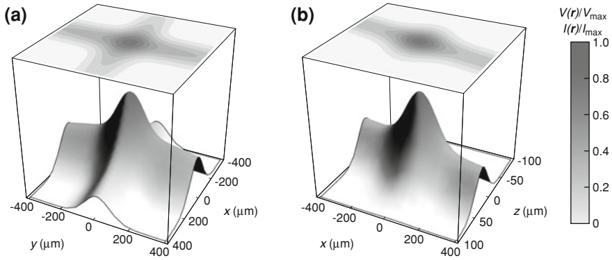
Fig. 5.4 Potential landscape of the crossed dipole trap in the horizontal xy -plane (a) and the vertical xz -plane (b) . The potential is calculated with a numerical model that takes all experimental beam parameters and tilts into account (see main text). Gravity is neglected in the plots for clarity. The difference in the waists of the two beams is clearly visible in panel a . A symmetric trapping potential [top view of a ] is achieved by choosing a power ratio of P_y/P_x \approx 2 . Note that the scaling of the z -axis in panel b is stretched by a factor of four
