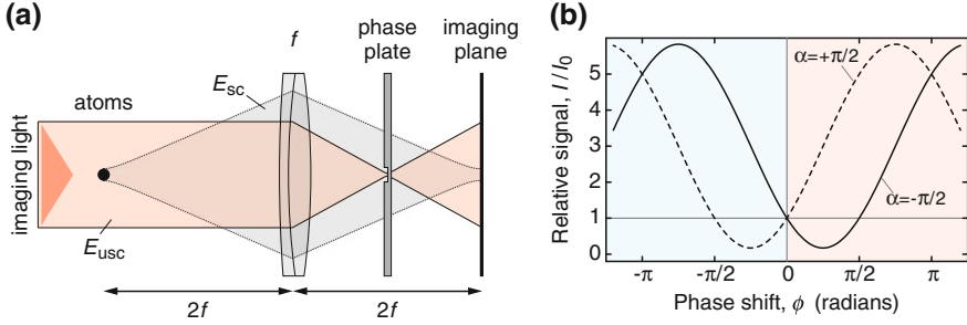
Fig. 4.1 Theory of phase-contrast imaging. a Elementary phase-contrast setup. Far-detuned imaging light is coherently scattered by the atoms (gray shaded area). A phase plate in the Fourier plane shifts the relative phase between scattered ( E_{sc} ) and unscattered ( E_{usc} ) light. In the imaging plane, the phase modulation \phi(x, y) , which the atoms imprint on the imaging beam, can be converted into an intensity modulation I(x, y) , if the phase shift \alpha of the phase plate is chosen appropriately (see main text). b Relative signal I/I_0 as a function of the phase shift \phi for advancing ( \alpha = +\pi/2 , dashed) and retarding ( \alpha = -\pi/2 , solid) phase plates. For simplicity a transparent atom cloud is assumed ( t = 1 ) corresponding to the limit of far detuning. The shading indicates that the phase shift \phi is positive (negative) for red (blue) detuned imaging light (see Eq. 4.3). The method is usually used in the linear regime I/I_0 \propto \phi . Only here the phase-contrast signal is proportional to the column density of the atom cloud, because \phi \propto n_{col}(\mathbf{r})
