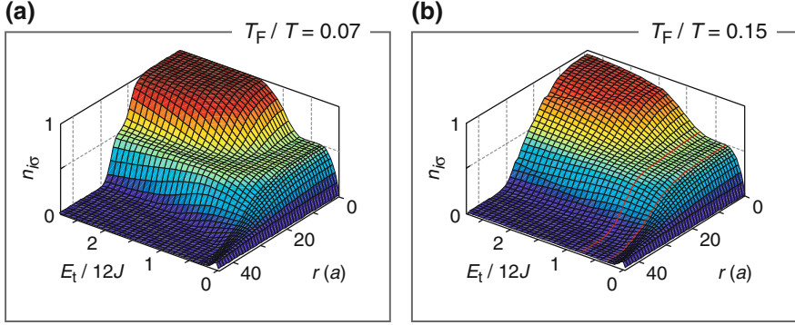
Fig. 6.3 Theoretical in-trap density distributions at strongly repulsive interactions ( U/12J = 1.5 ). The radial distance from the trap center is denoted by r given in units of the lattice constant a = \lambda/2 . While for lower temperature the different phases can be clearly distinguished in the radial profile (a), higher temperature washes out the boundaries (b). The red solid lines enclose the region, where a Mott insulating core has formed. In this regime the global compressibility is reduced as shown in Fig. 6.7d. Please note that the dimensionless temperatures T/T_F given here, refer to the Fermi gas in the harmonic trap prior to lattice loading. The DMFT calculations have been performed by Theo Costi, Achim Rosch and collaborators [4]
