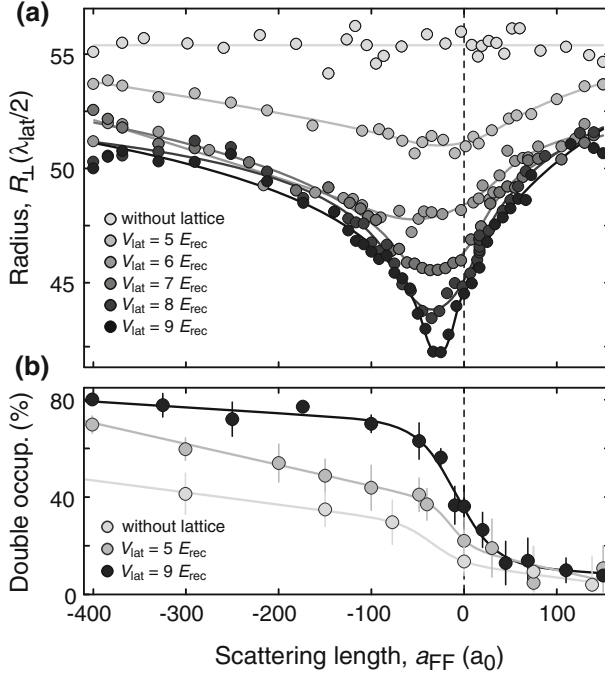
Fig. 6.10 Measured cloud size and double occupancy. a The cloud radius in the horizontal plane R_{\perp} and b the fraction of atoms on doubly occupied lattice sites as a function of scattering length are shown for several lattice depths. The data points in a correspond to a moving average over three consecutive points to smoothen the noise. Each point in b shows the average of at least five measurements at identical parameters; the error bars denote the standard deviation. The data is recorded at a fixed horizontal (vertical) trap frequency \omega_{\perp} = 2\pi \times 25 Hz ( \omega_z \approx 2\pi \times 100 Hz)
