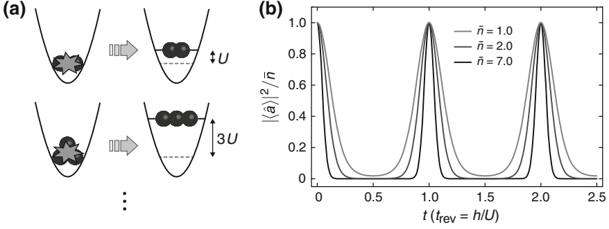
Fig. 7.1 Interactions in a single-orbital system and quantum phase revival dynamics. a Interacting atoms in the ground state of a confining potential undergo coherent collisions. If only the single ground state orbital is taken into account, the interaction energy per atom pair U is independent of the filling n as given by Eq. 7.7. b Under such conditions a coherent matter wave field undergoes perfectly periodic collapses and revivals. The revival time t_{\text{rev}} = \hbar/U is inversely proportional to the interaction energy U , while the collapse time t_{\text{coll}} = \hbar/(\sqrt{\bar{n}}U) is additionally inversely proportional to \sqrt{\bar{n}} , which is the standard deviation of the Poisson distribution
