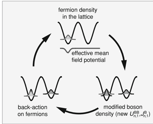
Fig. 8.7 Self-consistent calculation of the deformation of on-site orbitals induced by attractive interactions. Starting with a single fermion at a lattice site, an added boson feels an attractive mean-field potential. This narrows the bosonic on-site wavefunction compared to the noninteracting case. In turn, also the fermionic wavefunction becomes narrower. The wavefunction deformation eventually gives rise to renormalized interaction strengths U_{n,1}^{BB} and tunneling parameters J_{n,1}^B . The procedure is repeated until convergence, see also Ref. [28]
