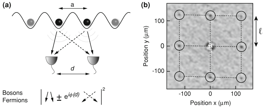
Fig. 4.4 Quantum noise correlations for bosonic and fermionic atoms. a When two identical atoms are released from neighboring lattice sites, they can reach the independent detectors via two, fundamentally indistinguishable paths. The respective probability amplitudes interfere constructively (destructively) for bosons (fermions) corresponding to the upper (lower) sign. The correlation between the detectors is sinusoidally modulated as a function of the distance d . For more than two atoms the correlations evolve from a sinusoidal modulation to narrow peaks, in analogy to optical diffraction from a grating with an increasing number of slits. b Experimental noise correlations of a ^{87}\text{Rb} Mott insulator released from a three-dimensional optical lattice ( V_{\text{lat}} = 32 E_{\text{rec}} ). About 30 images have been averaged. The position of the correlation peaks with a periodicity \ell = \hbar t / (ma) resembles the in-situ order with a lattice constant a
