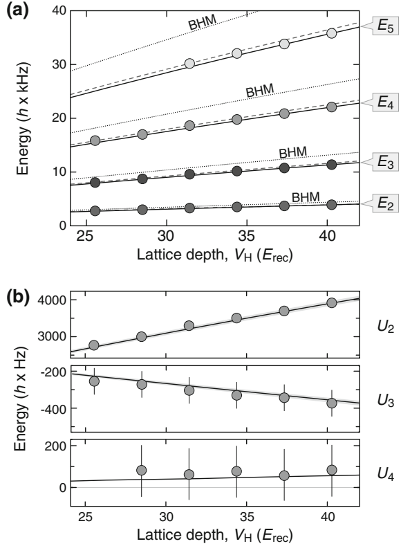
Fig. 7.12 Fock state energies and effective multi-body interactions in experiment (points) and theory (lines). a Multi-orbital Fock state energies as derived from both experimental and theoretical data in Fig. 7.11. The solid (dashed) lines show the multi-orbital Fock state energies E_n^{\text{MO}} as calculated by exact diagonalization on a Hilbert space with 4^3 ( 3^3 ) single-particle orbitals. The corresponding energies of the Bose-Hubbard model (BHM, dotted lines) lie considerably higher. b Effective two-body (top), three-body (middle) and four-body (bottom) interaction strengths as derived from experiment and theory, assuming a_s = 102(2) a_0 and 4^3 contributing single-particle orbitals. The error bars correspond to one standard deviation
