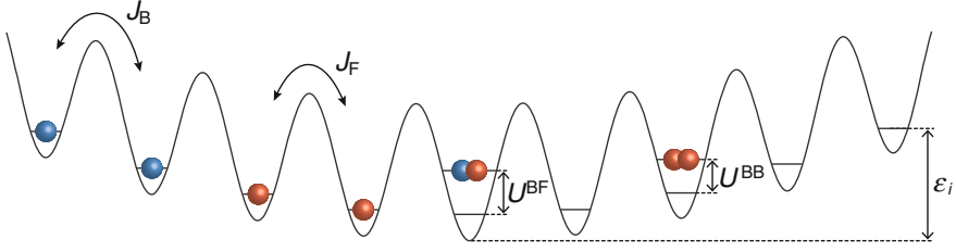
Fig. 8.1 Illustration of the matrix elements of the Bose-Fermi Hubbard model (see text)
