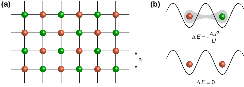
Fig. 3.6 Antiferromagnetic ordering and exchange interactions. (a) The Mott insulating ground state of the Fermi-Hubbard model, which is characterized by localized spins, shows antiferromagnetic ordering when the temperature of the system is low enough. (b) When opposite spins occupy neighboring lattice sites ( upper panel ), they reduce their energy by -4J^2/U through a virtual exchange process. This process has two possible exchange paths, during which either the left or the right well are virtually doubly occupied. The intermediate state is detuned by the interaction energy U . For identical spins ( lower panel ) the exchange process is not possible, because Pauli's principle forbids the intermediate doubly occupied state [1]
