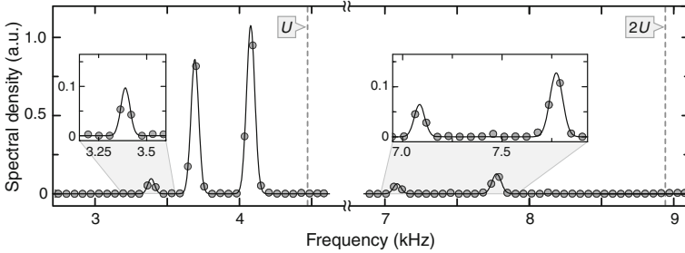
Fig. 7.9 Spectral analysis of the time trace in Fig. 7.8 reveals the contributing frequencies. The solid line shows Gaussian fits to the peaks. Grey dashed lines display the frequencies corresponding to the single-orbital interaction energies U and 2U at a lattice depth of 41 E_{\text{rec}}
