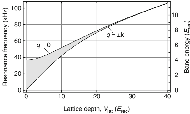
Fig. 5.10 Energy gap between the first and second lattice band E_q^{(2)} - E_q^{(1)} as a function of lattice depth. The scale on the left side shows the resonance frequencies for ^{40}\text{K} in a 738 nm lattice, while the scale on the right side is valid in general. Boundaries of the resonance frequencies are set by the band gaps for q = 0 and q = \pm k (see Sect. 2.2.3 and Fig. 2.8)
