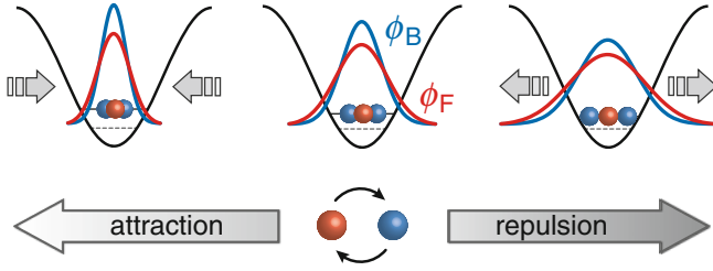
Fig. 9.8 The schematic shows that repulsive (attractive) interspecies interactions broaden (shrink) the on-site orbitals \phi_B(\mathbf{r}) and \phi_F(\mathbf{r}) and thereby affect the Bose-Bose interaction strengths U_{n,1}^{\text{BB}} \propto a_{\text{BB}} \int d^3r |\phi_B(\mathbf{r})|^4
