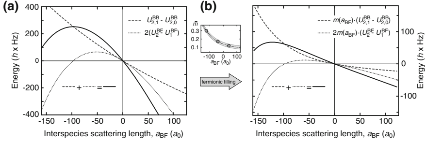
Fig. 9.10 Variational model for atom number dependent on-site interaction strengths U_{n,m}^{BB} and U_n^{BF} . a The contributions to the shift with respect to U_{2,0}^{BB} [see Eq. (9.13)] are displayed as a function of the interspecies scattering length a_{BF} : U_{2,1}^{BB} - U_{2,0}^{BB} (dashed) and 2(U_2^{BF} - U_1^{BF}) (dotted) and their sum (solid line). b Weighing the shift with the interaction dependent fermionic filling \bar{m}(a_{BF}) (as measured in the experiment) yields an almost linear trend (solid line) for a_{BF} \gtrsim -125 a_0
