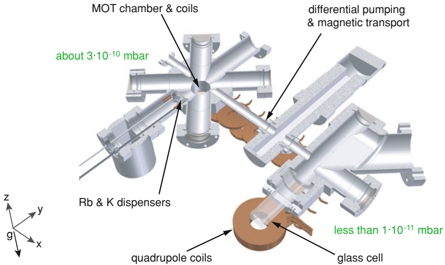
Fig. 5.2 Cross-sectional view of the experimental apparatus showing the vacuum chamber and the most important magnetic field coils. Green annotations show the pressure in the corresponding part of the vacuum chamber
