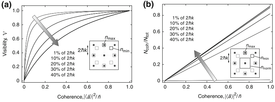
Fig. 4.3 Comparison of visibility and fraction of coherent atoms as measures for bosonic coherence. Based on simulated momentum distributions of a two-dimensional lattice system ( 11 \times 11 sites) with a known value of |\langle \hat{a} \rangle|^2 / \bar{n} ( \bar{n} is the mean on-site filling) the experimental observables are extracted: a The visibility is defined by \mathcal{V} = (n_{\max} - n_{\min}) / (n_{\max} + n_{\min}) and b the fraction of coherent atoms follows from (N_{\max} - N_{\min}) / N_{\text{norm}} . Both quantities are evaluated for several sizes of the n_{\max} - and n_{\min} -counting boxes given in units of the Brillouin zone width 2\hbar k
