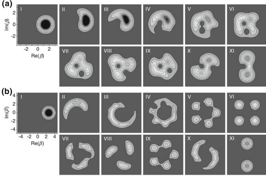
Fig. 7.2 Matter wave dynamics of a coherent state in a single-orbital system visualized by the Q -function. The coherent states |\beta\rangle are characterized by points in the complex plane. The contour plots show their overlap with |\psi_\alpha(t)\rangle at discrete times t ranging from 0 (I) to t_{\text{rev}}/2 (XI) scanned in steps of t_{\text{rev}}/20 . |\psi_\alpha(t)\rangle evolves away from a coherent state until it forms a Schrödinger cat-type superposition of two quasi-coherent states with a phase difference of \pi at the time of maximal collapse ( t_{\text{rev}}/2 ). Panel a shows the evolution for \bar{n} = 2.0 and b for \bar{n} = 7.0 , where the latter reveals even more complex superpositions of quasi-coherent states at intermediate times. Contour lines are spaced by 0.02 and the maximal value of the Q -function is 1/\pi \approx 0.32 by definition
