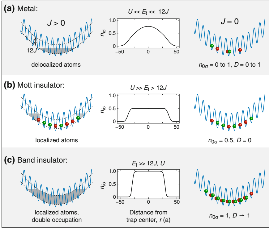
Fig. 6.2 a–c Zero-temperature quantum phases of the Hubbard model for a balanced spin mixture in a harmonic confining potential. The left column schematically illustrates the equilibrium atom distribution, dashed lines indicate the extent of the first band (compare Fig. 3.7). The center column displays the corresponding in-trap density profiles. The right column shows the distribution of singly and doubly occupied lattice sites after projection into the zero-tunneling limit. Experimentally the projection is achieved by a rapid increase of the lattice depth. n_{0\sigma} denotes the central filling and D the fraction of atoms on doubly occupied lattice sites. Strictly speaking, the Mott insulator (b) shows antiferromagnetic ordering at zero temperature (see Sect. 3.3.2). Here, a paramagnetic Mott insulator is displayed, because experimental temperatures are larger than the Néel temperature for magnetic ordering
