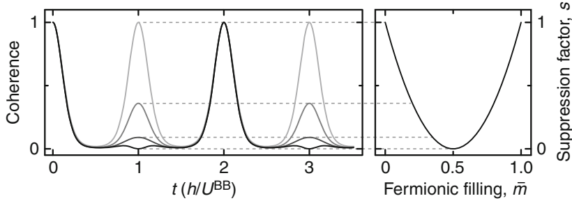
Fig. 9.2 Quantum phase revivals in a few-body Bose-Fermi system. Suppression of odd quantum phase revivals in a Bose-Fermi mixture at |U^{\text{BF}}/U^{\text{BB}}| = 0.5 for variable fermionic fillings: \bar{m} = 0, 0.2, 0.35 and 0.5 (solid lines, darker color for larger \bar{m} ). The right panel displays the suppression factor s as a function of the filling \bar{m}
