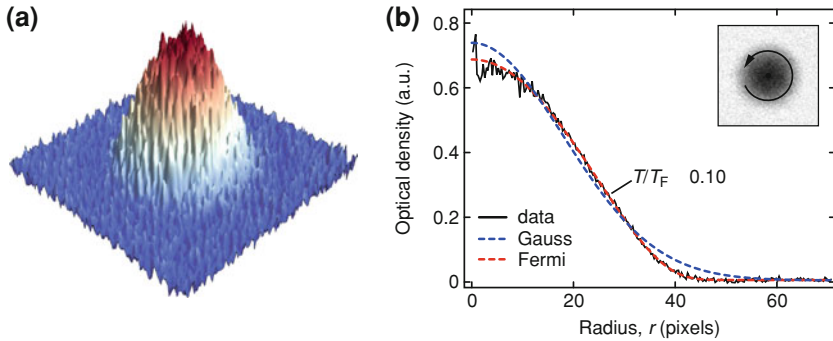
Fig. 6.4 Ultracold fermionic spin mixture. a Column density of a noninteracting ^{40}\text{K} spin mixture after 10 ms time-of-flight expansion. The vertical axis corresponds to the optical density (a.u.). b The azimuthally averaged raw data (solid line, see inset) is fitted by a Gaussian (blue dashed line) and a Fermi-Dirac model (red dashed line) omitting the noisy data of the central pixels. The Fermi fit yields a temperature of T/T_F \approx 0.10 , which is close to the reliability limit of this thermometry method for the given cloud sizes [12]
