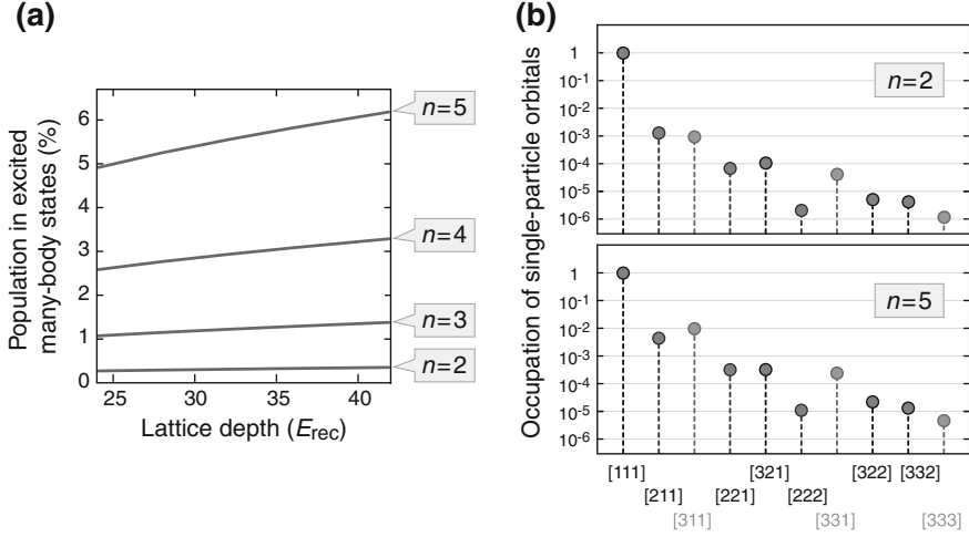
Fig. 7.5 Occupation of many-body states on a lattice site. a Population that is not found in the many-body ground state of the noninteracting n -atom system |1\rangle = |n, 0, \dots, 0\rangle as a function of lattice depth and atom number assuming a_s = 102 a_0 and 4^3 single-particle orbitals. b Occupation of single-particle orbitals for Fock states with n = 2 and n = 5 atoms ( 3^3 orbitals, V_{\text{lat}} = 40 E_{\text{rec}} , a_s = 102 a_0 ). The notation [\alpha\beta\gamma] comprises all permutations of \alpha , \beta , and \gamma . All orbitals corresponding to a set [\alpha\beta\gamma] are energetically degenerate and their occupations have been added up. The energy of the orbitals increases from left to right . Occupation of the second band, while energetically favorable compared to the third band, is suppressed due to conservation of parity
