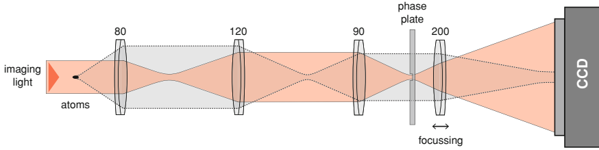
Fig. 5.12 Schematic of the main imaging system for absorption and phase-contrast imaging. The numbers at the lenses denote the respective focal length f . The overall magnification is m = 3.3 . In phase-contrast imaging the unscattered light passes through the center of the phase plate imprinting a phase shift relative to the coherently scattered light. For absorption imaging the phase plate is laterally moved out of the beam path
