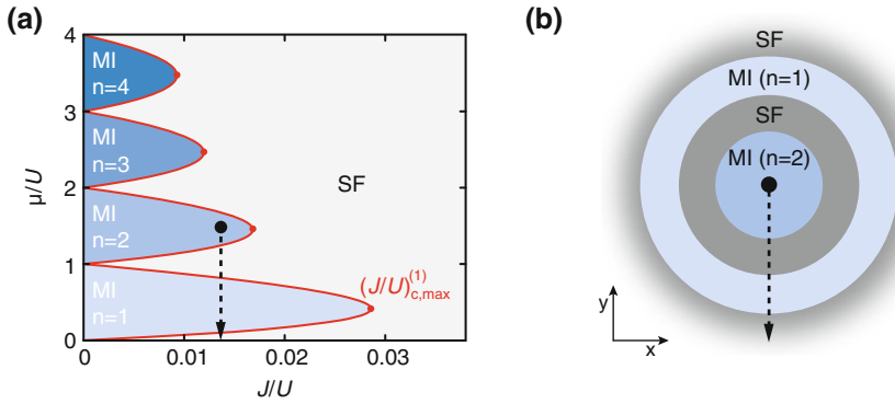
Fig. 3.3 Phase diagram of the Bose-Hubbard model at T = 0 . a As the ratio J/U decreases the system undergoes a phase transition from a superfluid (SF) to a Mott insulator (MI). The phase boundaries (Eq. 3.25) are shown as red lines. The Mott lobes (shaded in blue) contain the incompressible Mott phases at integer filling n . b In a trapped geometry, the phase diagram ( a ) gives rise to a shell structure: moving from the trap center outwards corresponds to sampling a continuously decreasing chemical potential. The Mott insulator shells are separated by superfluid layers, which become thinner for decreasing J/U
