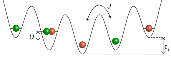
Fig. 3.1 Illustration of the matrix elements of the Hubbard model (see text)
