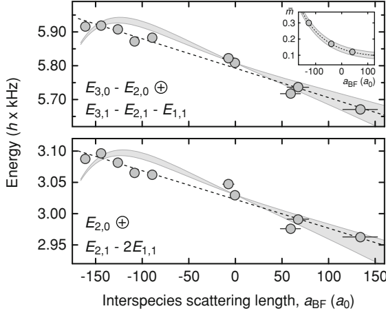
Fig. 9.9 Modification of the Bose-Bose interaction strength induced by an interacting fermion. The highest spectral contributions of order U^{\text{BB}} ( 2U^{\text{BB}} ) are shown as a function of a_{\text{BF}} in the lower ( upper ) panel [Corresponding to the spectral features close to the dashed line ① (④) in Fig. 9.6]. The underlying energies E_{2,0} and E_{2,1} - 2E_{1,1} ( E_{3,0} - E_{2,0} and E_{3,1} - E_{2,1} - E_{1,1} ) cannot be resolved individually appearing as a single superposition peak in the spectra. The dashed line shows a linear fit with a slope of s_{2,1} = -0.46(4) \text{ Hz}/a_0 ( s_{3,1} = -0.87(5) \text{ Hz}/a_0 ). Shaded areas show the shift calculated within a variational model (see main text). It explicitly accounts for the measured values for the fermionic filling fitted by an exponential function, \bar{m}(a_{\text{BF}}) (inset). The measurement has been performed at a lattice depth V_{\text{H}} = 28.2(3) E_{\text{rec}}^{\text{B}} . The data at a_{\text{BF}} = 0 a_0 have been obtained in a sample without fermions
