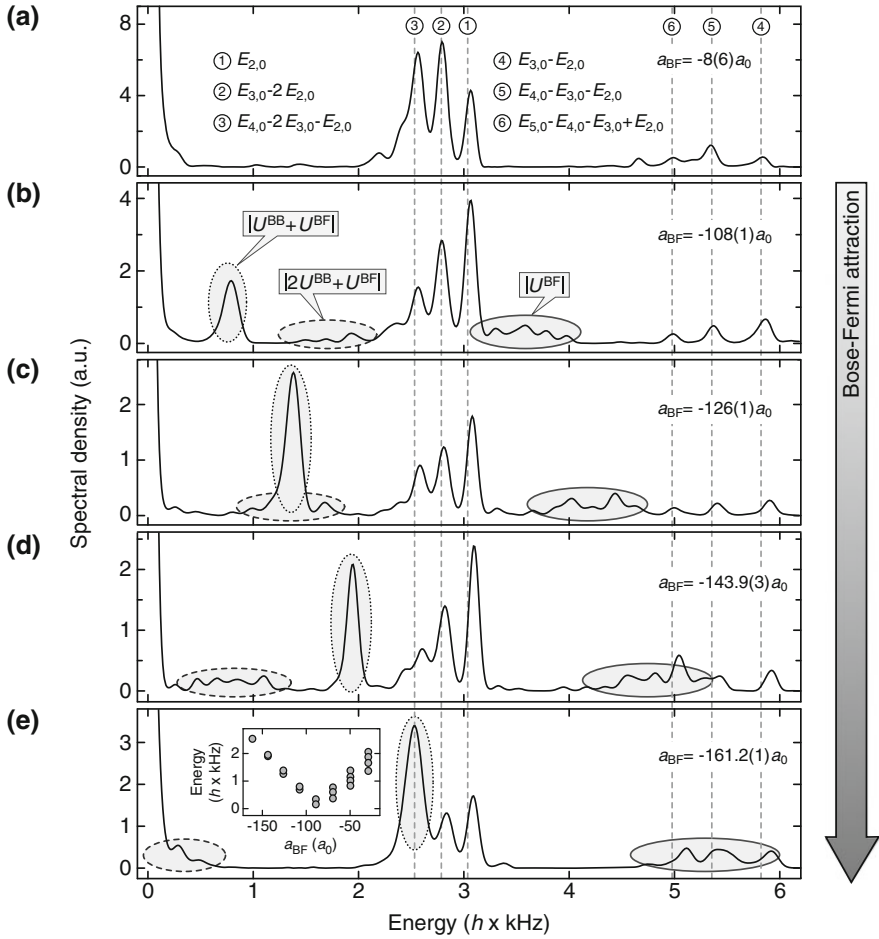
Fig. 9.6 Fourier spectra of time traces for vanishing, a , and linearly increasing Bose-Fermi attraction, b–e . The contributions involving direct Bose-Fermi interactions ( |U^{BF}| , |U^{BB} + U^{BF}| and |2U^{BB} + U^{BF}| ) are highlighted by shaded ovals (solid, dotted and dashed lines, respectively). The |U^{BB} + U^{BF}| components are shown in the inset of panel e as a function of a_{BF} . Dashed vertical lines indicate the spectral contributions of orders U^{BB} (① to ③) and 2U^{BB} (④ to ⑥) for a purely bosonic system or vanishing interspecies interactions [23]
