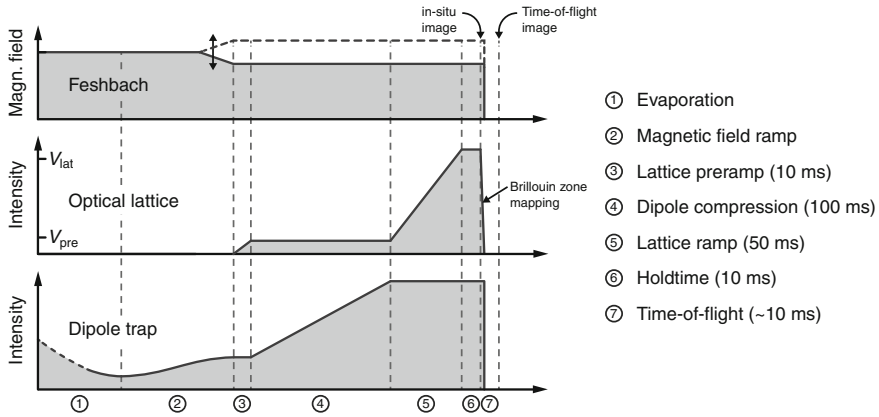
Fig. 6.5 Overview of the experimental sequence as described in the main text. Remarkable features are the preramp of the optical lattice ③, the nondestructive in-situ phase-contrast image after ⑥ and the subsequent time-of-flight absorption image after ⑦ mapping out the Brillouin zone
