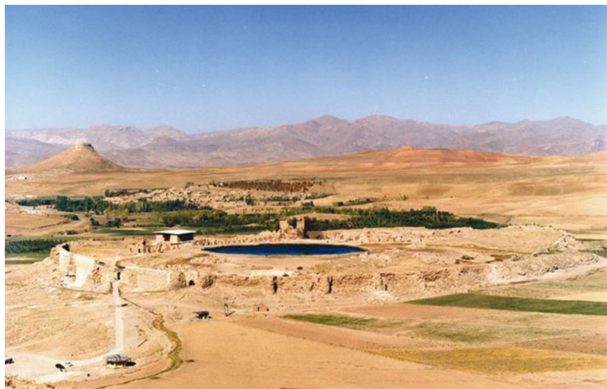
Fig. 1.5 A view of Takht-e Soleyman Spring and dried spring of Zendan-e Soleyman and ancient city of Ganjeh near Takab (used to be called Shiz in Arabic, but it is known today as Takht-e Soleyman) (Photographed by Alireza Amrikazemi)
