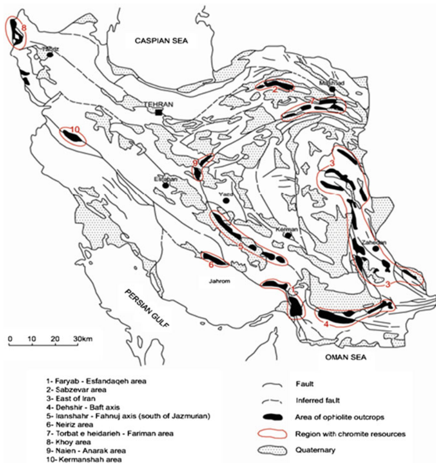
Fig. 5.3 Prioritized chromite-bearing areas of Iran
