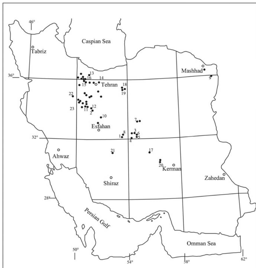
Fig. 5.14 Distribution map of barite deposits of Iran (Khoshjou 1999) (1 Haft-har, 2 Darreh Kashan, 3 Ardekan, 4 Dorbid, 5 Niyook, 6 Dasht-e Deh, 7 Haji Abad, 8 Hooodeh, 9 Ghara Gheythan, 10 Kamshacheh, 11 Tappeh-sorkh Bichegan, 12 Vavan, 13 Elite, 14 Lar, 15 Ahoorak Taleghen, 16 Seplark, 17 Chari-Abtorsh, 18 Garmab, 19 Chah Shirin, 20 Baghin, 21 Khaneh Hozeh-abad, 22 Tang-abad, 23 Jasb)
