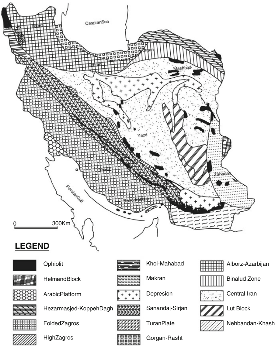
Fig. 2.4 Structural zones of Iran (Nabavi 1976)
