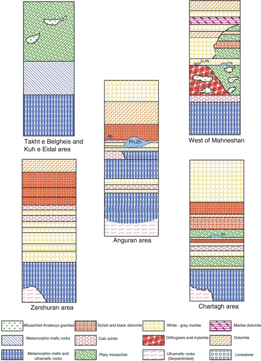
Fig. 6.9 Precambrian-Early Cambrian rocks and mineralization in Takab area
