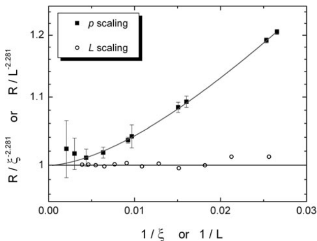
Fig. 5.12 Scaling corrections to the resistance near the percolation threshold in a simple cubic lattice. The resistance divided by the expected power law is represented as a function of the inverse of the side of the cube 1/L (open circles), in this case up to 500, for the case of site percolation (in the case of bond percolation the corrections are not measurable in this range of sizes) and as a function of the inverse of the coherence length 1/\xi(p) (filled squares), for the case of bond percolation for a cube of 500 \times 500 \times 500 (after [13])
