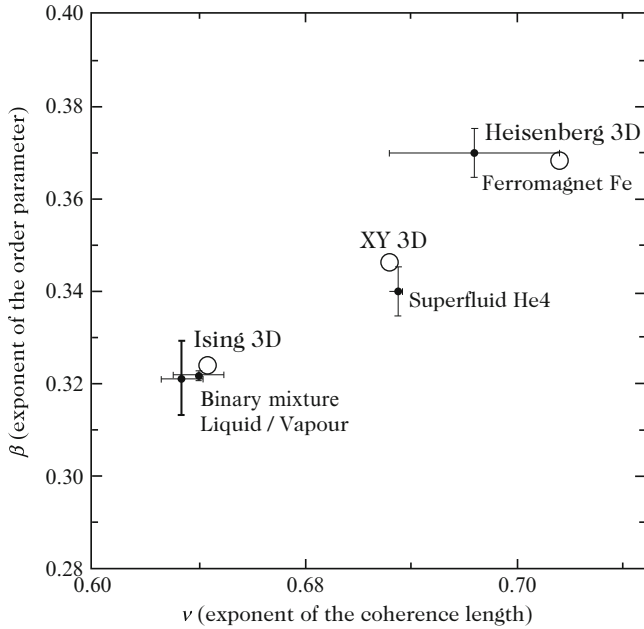
Fig. 1.23 Critical exponents measured for four families of transitions, compared to values predicted by the three corresponding models that take into account the scale invariance of the critical state
