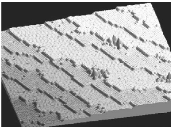
Fig. 8.2 Growth along the edge of, initially straight, atomic steps on a monocrystal of silicon shown by Scanning Tunnelling Microscopy (IEMN, Laboratoire de Physique, Lille)
