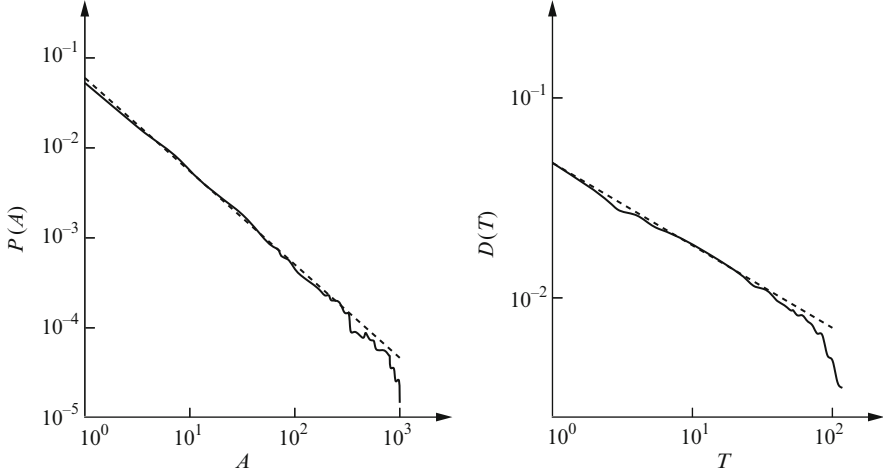
Fig. 10.2 Log-log plots showing the behaviour of a simulated sandpile (after [3]). Left: distribution of avalanches as a function of their size: P(A) \sim A^{-\mu} with \mu \approx 1.03 . Right: distribution of avalanches as a function of their lifetime weighted by the average response \langle A(T) \rangle / T (see text): it scales as D(T) \sim T^{-\mu'} with \mu' \approx 0.43 , corresponding to a spectral density S(f) \sim f^{-1.57}
