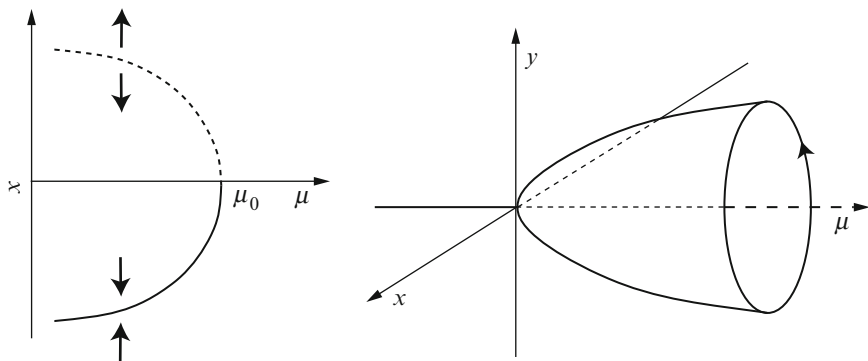
Fig. 9.3 Left: Saddle-node bifurcation observable in the evolution \dot{x} = \mu - \mu_0 + x^2 . For \mu < \mu_0 , we have two fixed points, \sqrt{\mu_0 - \mu} (unstable) and -\sqrt{\mu_0 - \mu} (stable). They collide at \mu_0 and disappear for \mu > \mu_0 . Arrows indicate the instability of the upper branch and stability of the lower branch. Right: Hopf bifurcation observable in the evolution \dot{r} = r(\mu - r^2) , \dot{\theta} = \omega . The branch r \equiv 0 is stable for \mu < 0 and destabilises at \mu_0 = 0 being replaced by a limit cycle r(\mu) = \sqrt{\mu} (as attractor)
