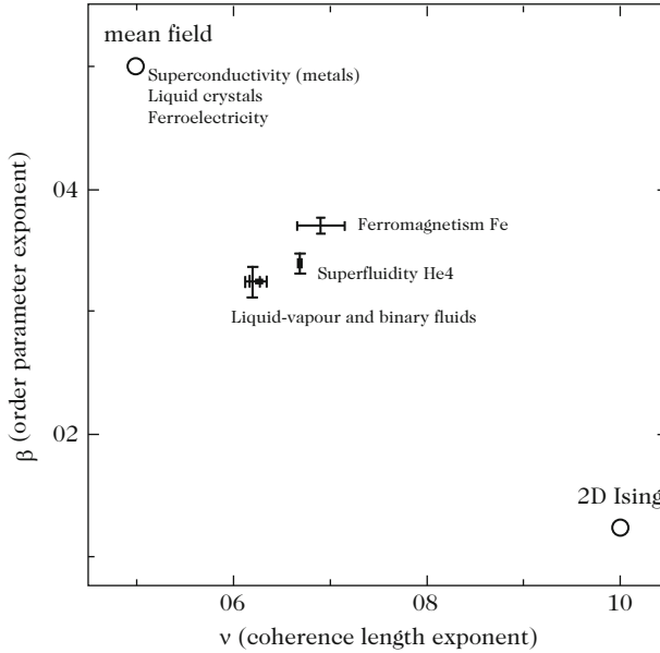
Fig. 1.22 Critical exponents \beta and \nu : experimental results obtained for seven difference families of transitions, compared to values predicted by the mean field and 2D Ising models
