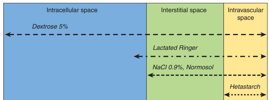
FIGURE 34–18. Volume of distribution of crystalloid solutions.
