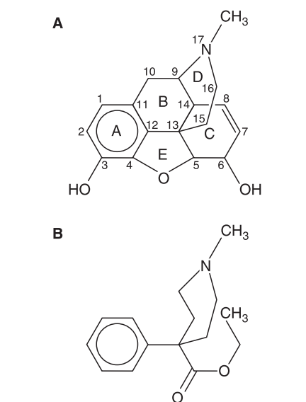
FIGURE 41-2. Structural formulas of morphine ( A ) and meperidine ( B ).
