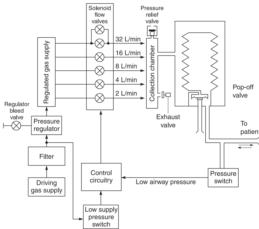
FIGURE 38-34. Ohmeda 7000 electronic anesthesia ventilator. Schematic of driving gas circuit. (Courtesy of Ohmeda, BOC Health Care, Madison, WI.)
