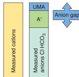
FIGURE 34–11. The anion gap. A - , phosphate and albumin; UMA, unmeasured anions.
