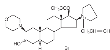
FIGURE 33–10. Chemical structure of steroidal class neuromuscular blocking drugs.
