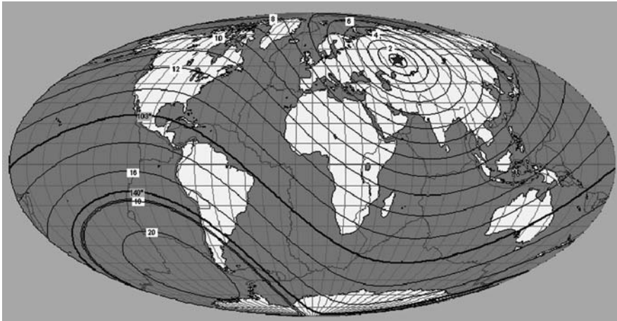
Fig. 5.24 Station BRVK is marked by a star. The great circles indicate P-travel time in minutes from the station. Note, the back azimuth from BRKV can only be measured off approximately on the figure
