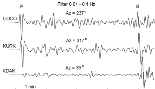
Fig. 7.23 Broadband seismograms of the vertical component showing P and S for a deep earthquake near Japan. The three stations have similar distances ( 54\text{--}58^\circ ) but different azimuths ( Az ) as indicated on the figure. The origin time is 2007 0928 13:38, hypocentral depth is 260 km and m_b(\text{PDE}) = 6.7
