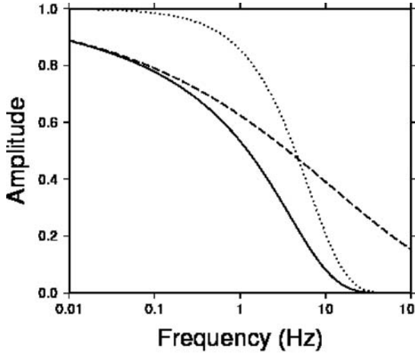
Fig. 8.3 Illustration of equation (8.7) showing the functions e^{-\pi f t^k} (dotted) and e^{\frac{\pi f t}{Q(f)}} (dashed) and the product of the two (solid). In this example we use Q(f) = 200 * f^{0.7} , k = 0.05 and t = 30 s
