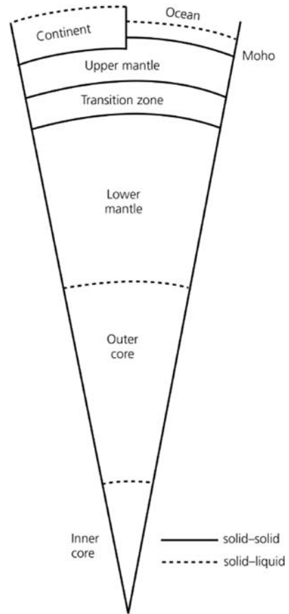
Fig. 2.1 Earth structure showing the main interfaces within the earth (not to scale). Figure from Stein and Wysession (2003) and copied from http://epscx.wustl.edu/seismology/book/book_no_captions/figures/
