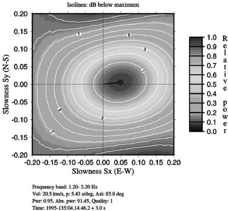
Fig. 9.6 Result from beam forming in the time domain (also called beam packing) of the NORES data in Fig. 9.5 in an equi-spaced slowness grid. The data were pre-filtered in the band 1.2–3.2 Hz. The isolines represent power of each beam within the 3-s window analyzed. Copyright granted by IASPEI. (Figure from NMSOP, Fig. 9.24)
