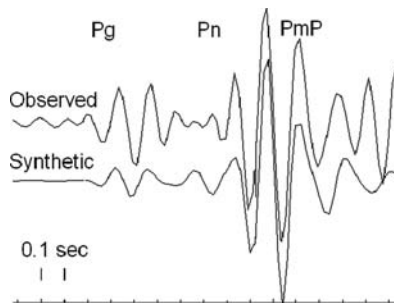
Fig. 7.42 An observed short period vertical seismogram of P compared to the synthetic seismogram modeled with WKBJ as implemented in SEISAN. Only the phases Pg, Pn and PmP are modeled in this case. The trace is from SNART, origin time 2004 0705 18:09, depth 17 km, M_L = 2.2 , epicentral distance 94 km and strike, dip and rake 147, 17 and 76, respectively. A filter of 5–10 Hz is used
