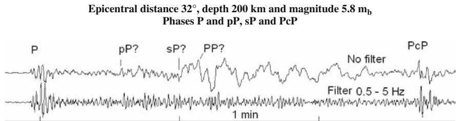
Fig. 2.26 Seismogram of the global network broadband station WRAB, vertical component. The origin time is 1996 0610 01:04. The bottom trace is filtered 0.5–5 Hz
