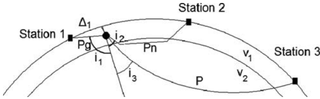
Fig. 7.9 Angle of incidence for different rays. v_1 and v_2 are the P velocities in respective layers and \Delta_1 is the epicentral distance to station 1
