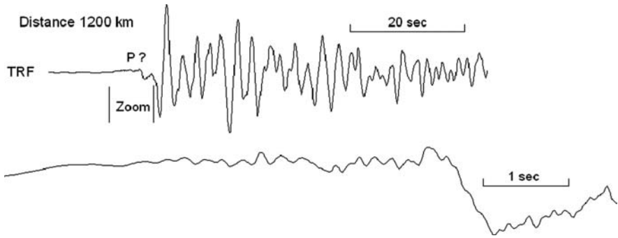
Fig. 7.18 Example of unclear polarity or station TRF, vertical channel broadband. It is the same event as in Fig. 7.17
