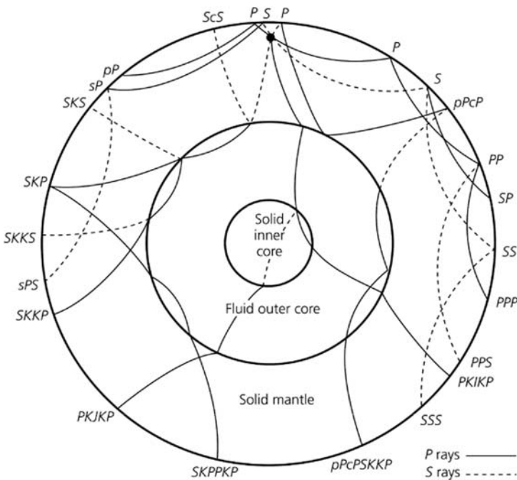
Fig. 2.9 Examples of body wave phases on a global scale. The large figure is from Stein and Wysession (2003) and copied from http://epscx.wustl.edu/seismology/book/book_no_captions/figures/
