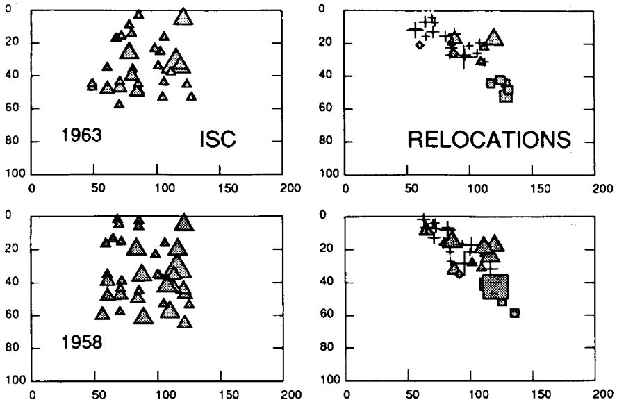
Fig. 5.9 Comparison of earthquake locations using the normal procedure at ISC ( left ) and JHD relocations ( right ). The events are located in the Kurile subduction zone along the rupture zones of large thrust events in 1963 and 1958. The vertical cross sections shown traverse the thrust zone from left to right . Note that the JHD solutions reduce the scatter and make it possible to define a dipping plane. Figure reproduced by permission from the American Geophysical Union. From Schwartz et al. (1989)
