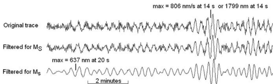
Fig. 6.19 Example of determining M_S . The top trace shows the original velocity long period record, the middle trace the record filtered for M_S , the bottom the traces filtered for M_S . The station is KONO, vertical channel. The location of the reading is indicated by max and the amplitudes are measured peak to peak divided by 2. The origin time is 1996 0623 01:17, m_b(\text{ISC}) is 5.4 and M_S is 5.4 (ISC). Epicentral distance is 66^\circ and depth is 33 km
