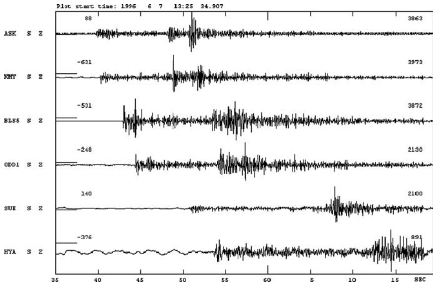
Fig. 5.21 A seismogram of a local earthquake in Western Norway. The numbers above the traces to the right is the maximum count and the numbers to the left are the DC values (count)
