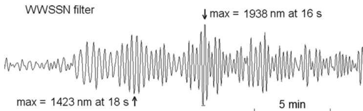
Fig. 6.16 Reading maximum amplitude (peak to peak divided by 2) on a WWSSN LP simulated trace. The seismogram is from station KBS, vertical channel. The origin time is 1996 0603 19:55, M_s = 5.5(\text{ISC}) and the epicentral distance is 52^\circ . The amplitude is not corrected for filter gain. The true ground displacement at 18 s is 1454 nm and at 1939 nm at 16 s. Thus the filter gain is small for WWSSN LP
