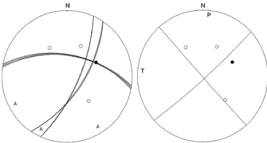
Fig. 7.29 Fault plane solutions of the California event above. The figure to the left shows the solutions using amplitudes from 4 stations and polarities from 4 stations and the figure to the right shows the CMT solution. The open circles are dilatations and the closed circles compression. Amplitude ratios are marked with A
