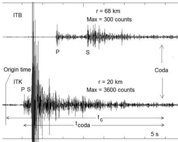
Fig. 6.6 Signals from two stations at different hypocentral distances r shown on plot. The amplitude scale on both seismograms is the same. The signals are filtered 5–10 Hz. The data is from a Tanzanian network. Origin time is 1992 1012 04:49 and M_L = 1.5 . Notice the equal coda wave amplitude for the 2 stations at the same absolute time, which is what we would expect in an ideal case
