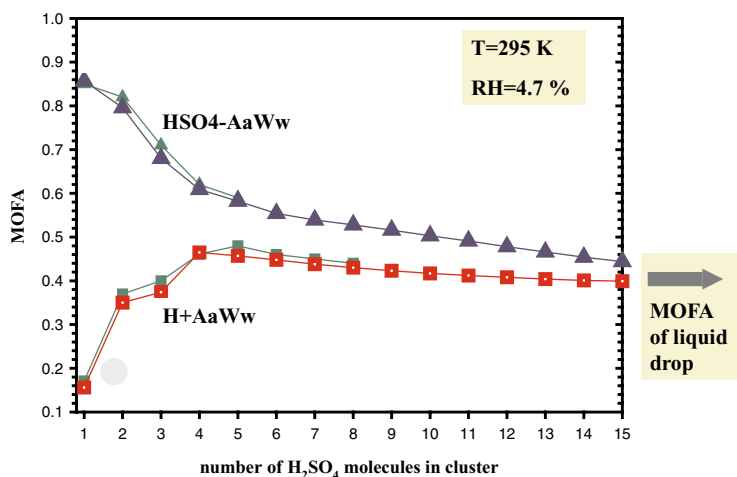
Figure 4. Sulphuric acid mole fraction MOFA of \text{HSO}_4^- (\text{H}_2\text{SO}_4)_a (\text{H}_2\text{O})_w and \text{H}^+ (\text{H}_2\text{SO}_4)_a (\text{H}_2\text{O})_w cluster ions measured in the laboratory flow reactor experiment of MPIK (Sorokin et al. , 2006). Also given are model calculations for cluster ions, electrically neutral \text{H}_2\text{SO}_4/\text{H}_2\text{O} droplets, and droplets carrying a single elementary electrical charge. See text for details. From Sorokin et al. (2006).
