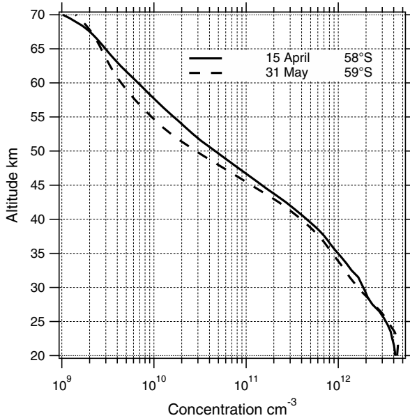
Figure 8. Evolution of \text{O}_3 profile at southern high latitude from 15 April to 31 May.
