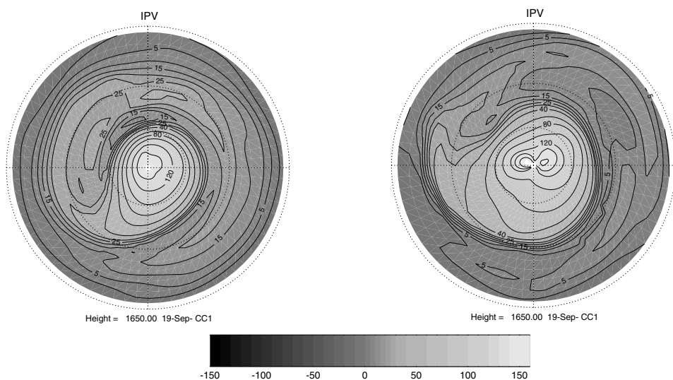
Figure 7. Typical distribution of the Northern Hemisphere Ertel potential vorticity on the 1650 K isentropic surface ( 10^{-4} \text{ Km}^{-1} \text{ s}^{-1} ) at day 50 from (left) the mechanistic model experiment (see Figure 5) in which an easterly forcing was applied in the subtropics 0\text{--}30^{\circ}\text{N} , 40\text{--}50 \text{ km} , and (right) the equivalent control run distribution. Figure adapted from Gray et al. (2004).
