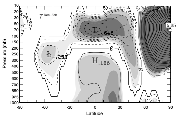
Figure 4. Anomalous wintertime (DJF) temperature (contoured) that varies coherently with that at 90^{\circ}\text{N} and 70 mb (open circle), which is a proxy for anomalous downwelling over the Arctic. Analogous to regression, values represent the anomalous temperature (K) associated with a 1-std deviation increase of downwelling. Shading marks regions where the two are coherent at the 95%, 99%, and 99.9% significance levels. Derived from the record of NCEP reanalyses over 1955 – 2000. After Salby and Callaghan (2005).
