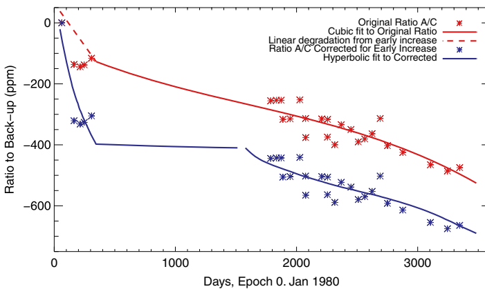
Figure 3. The original ratios of sensor A to sensor C (red symbols) of the ACRIM-I experiment on SMM are from Willson and Hudson (1991). The cubic fit corresponds to the correction originally applied and the dashed line includes the linear fit found by fitting the early increase. The blue symbols are corrected for the early increase and then fitted with a hyperbolic function.
