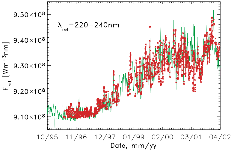
Figure 3. Comparison of solar spectral irradiance in the 220–240 nm band measured by the SUSIM instrument on UARS (solid line) with the SATIRE reconstruction (stars).
