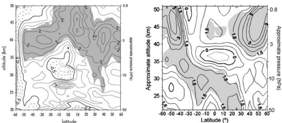
Figure 4. Annual mean ozone response to solar activity in units of percentage change per 100 F10.7 cm units (recent solar cycle amplitude \sim 130 F10.7 cm units). Left Panel : Zonal mean response from SAGE II data for the period October 1984–June 2002. From Haigh et al. (2004). Right Panel : zonal mean response from SBUV data for the period 1978–2004. From Zerefos et al. (2005). Contour intervals 0.5%. Shading indicates regions of 95% statistical significance.
