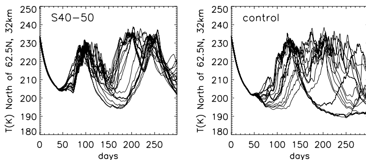
Figure 5. As Figure 4 but from (left) the experiment in which an easterly anomaly was imposed in the subtropics at 0-30^{\circ}\text{N} and 40-50\text{ km} , and (right) the control experiment with no easterly forcing. Figure adapted from Gray et al. (2004).
