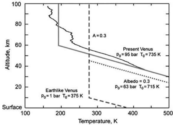
Figure 3. Simple climate models for Venus, corresponding to (a) the present day (solid gray line), (b) a decrease in albedo to 0.3 (dotted line), and (c) atmospheric loss of CO 2 such that the surface pressure fell to 1 bar (dashed line). A measured profile, obtained by the radio-occultation experiment on the Magellan orbiter on 5 October 1991 at latitude 67°N, is shown for comparison (solid black curve). While individual profiles do not necessarily coincide with the global mean represented by the model, the main difference seems to be due to heating by the absorption of solar radiation in the cloud layer in the 40–70 km height range.
