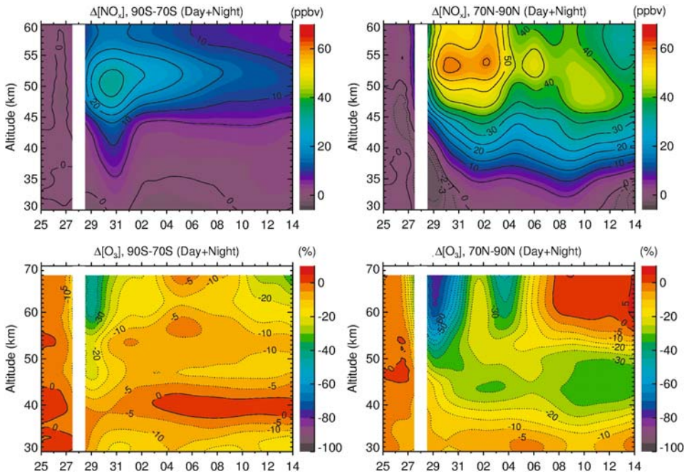
Figure 1. \text{NO}_x (upper panels) and \text{O}_3 (lower panels) anomalies in the upper stratosphere and lower mesosphere following the SPE event of 28 October–7 November 2003, derived from Envisat-MIPAS data. Left panels show Antarctic data (70–90°S), right panels Arctic data (70–90°N). Horizontal axis: day of month October, November. Reproduced from López-Puertas et al. (2005) with permission of American Geophysical Union.
