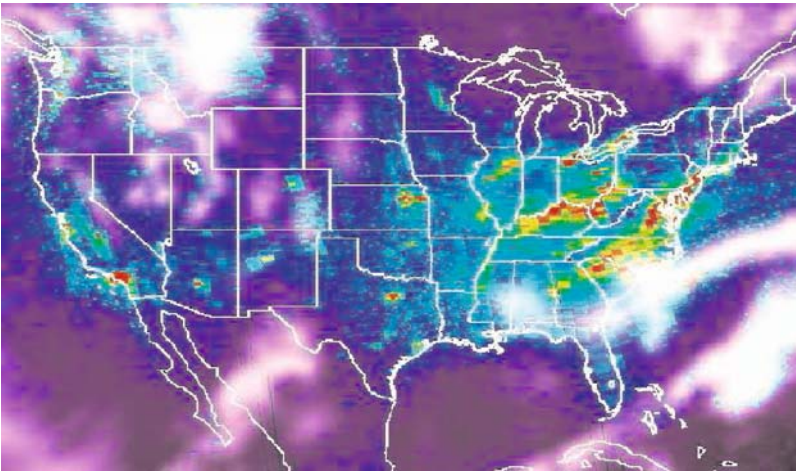
Figure 6. \text{NO}_2 measured by OMI over the United States on April 14, 2005. Red is high and blue are low values. White areas are clouds.
