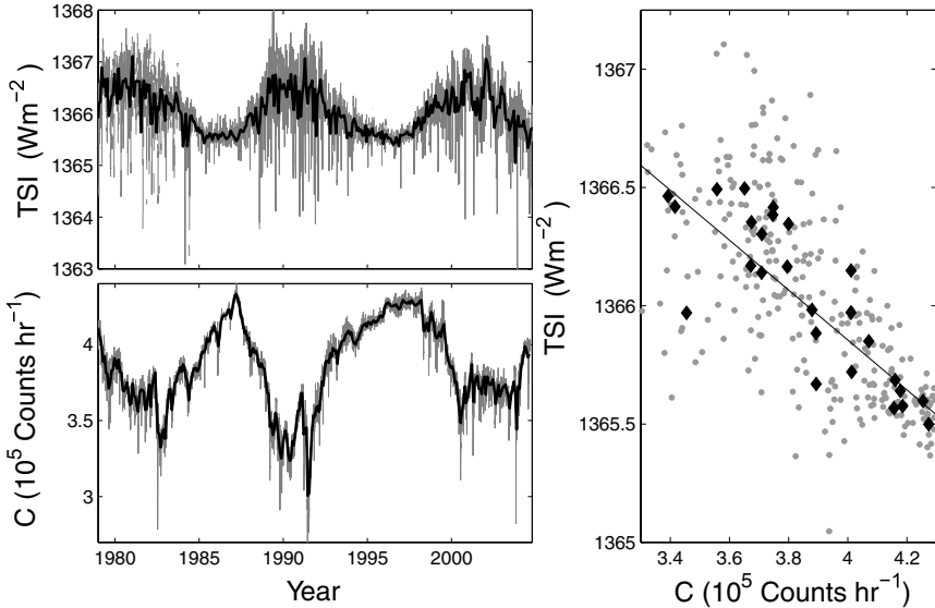
Figure 1. The anticorrelation of GCR fluxes with the total solar irradiance (TSI) since 1978. Left-hand panels: the variations of (top) the PMOD TSI composite (Fröhlich, 2006) and (bottom) the GCR counts, C , detected by the neutron monitor at Climax. In both cases, the grey line gives the daily values, and the black line the monthly means. It can be seen that the agreement is poor on a daily basis because of the effect of individual sunspot groups on TSI. Right-hand panel: Scatter plot of TSI as a function of C . The grey points show monthly means, the black diamonds the annual means. The best-fit linear regression to the annual data is also plotted. The correlation coefficients (and significance levels) are -0.68 (99.99%) and -0.85 (91.5%) for, respectively, monthly and annual data.
