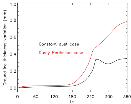
Figure 5. Results obtained by the model in a situation of reversed perihelion. The two curves show the thickness variation of water ice at the surface of the south pole during a martian year. In both cases, water ice accumulates at rates slightly less than 1 mm/yr. The red curve shows what would happen if the reversed perihelion climate had the same dust cycle and thus the same seasonal contrast as today. The black curve shows what would happen if the dust loading was low and had no seasonal variation, as might be expected from dust lifting predictions in a reversed perihelion climate.
