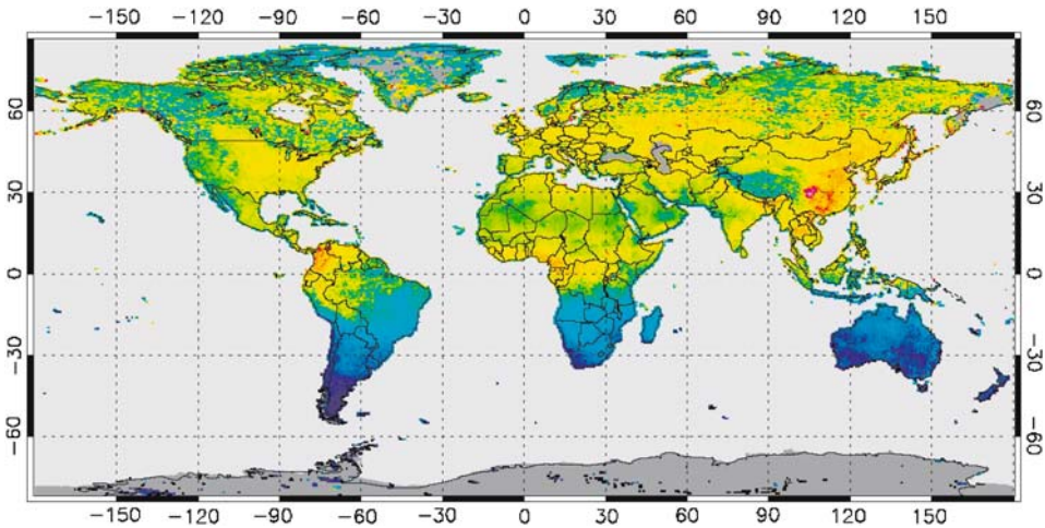
Figure 5. SCIAMACHY annual mean CH 4 dry air mixing ratio (ppb).
