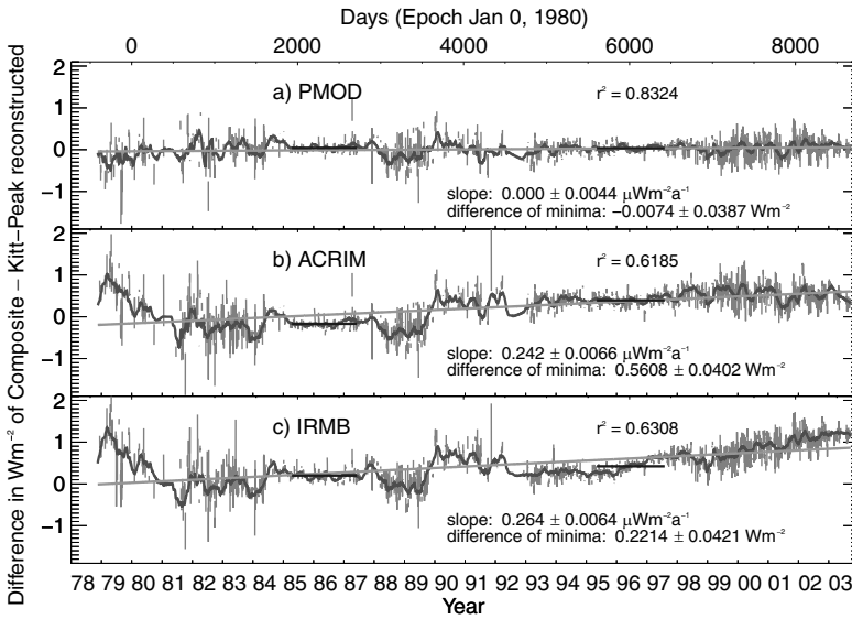
Figure 10. The comparison of the three composites with a reconstruction of TSI from Kitt-Peak magnetograms by Wenzler (2005).
