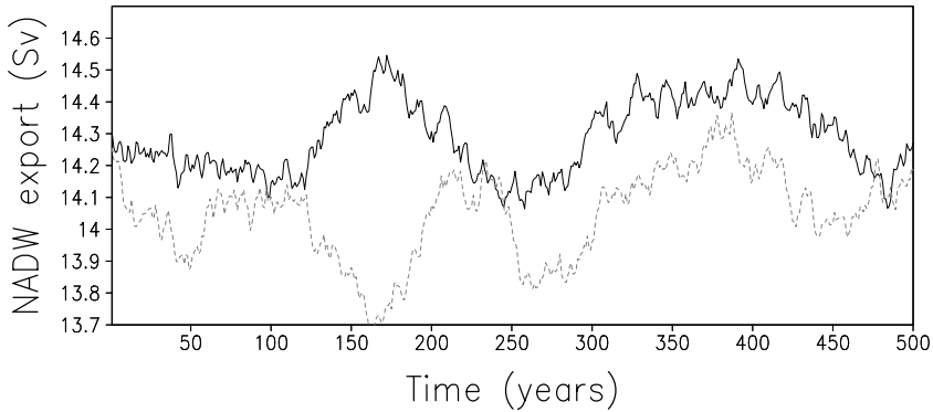
Figure 3. Maximum of the meridional overturning streamfunction in the Atlantic at 20^{\circ}\text{S} in Sv ( 10^6 \text{ m}^3 \text{ s}^{-1} ) (which is a measure of the export of North Atlantic Deep Water out of the Atlantic and thus of the intensity of the MOC) in a numerical experiment in which the total solar irradiance has been abruptly increased by 5 \text{ W/m}^2 at year 0 (grey dashed curve) and in the control experiment (black plain curve). A 25-year running mean has been applied to the time series to filter high frequency changes. Nevertheless, internal variability could mask the forced changes during some periods (e.g., around year 200–250).
