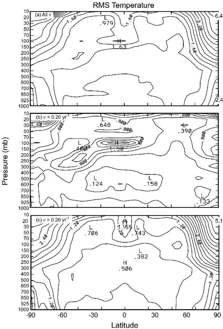
Figure 8. Root mean square variation of temperature in the entire monthly record: (a) inclusive of all periods, (b) for periods longer than 5 years, (c) for periods shorter than 5 years. Derived from the NCEP record. After Salby and Callaghan (2006).
