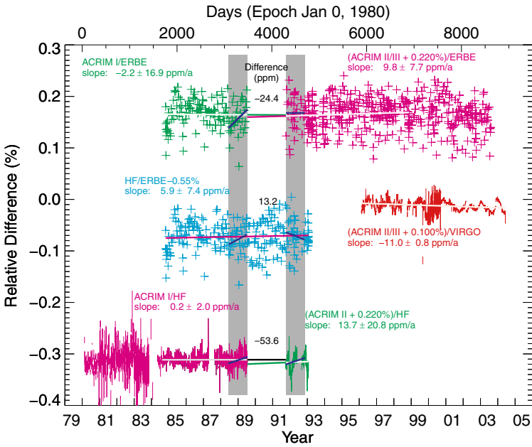
Figure 8. This plot illustrates the tracing of ACRIM-II to ACRIM-I. The change of the ACRIM-II level is determined by a weighted average of the comparison of ACRIM-I and II with HF and ERBS during the periods indicated by shading.
