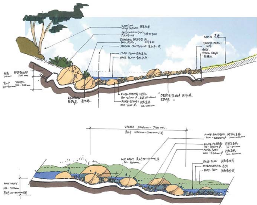
Fig. 2.39 Cross-sections of possible measures to slow down runoff water (Source: Bing et al., 2008b)
