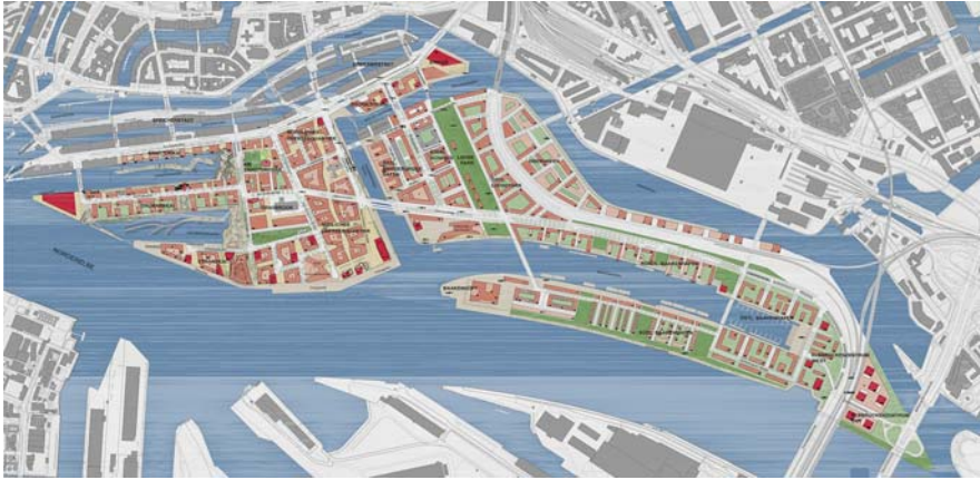
Fig. 3.35 Urban design for Hafencity (Source: GHS, 2002)
