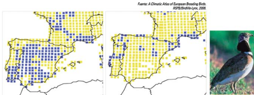
Fig. 1.35 Current and modelled dispersion in 2100 of the Little bustard ( tetrax tetrax ) (Source: Huntley, et al., (2007))
