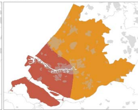
Fig. 2.5 Decrease in number of ice days (Source: Alterra et al., 2007)
