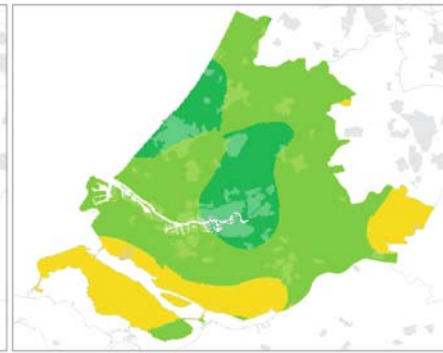
Fig. 2.10 Number of days with intense showers (Source: Alterra et al., 2007)
