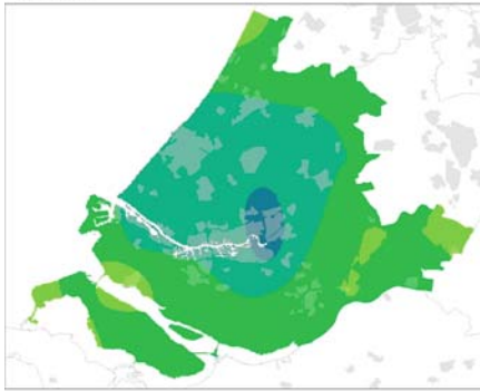
Fig. 2.9 Average summer precipitation (Source: Alterra et al., 2007)
