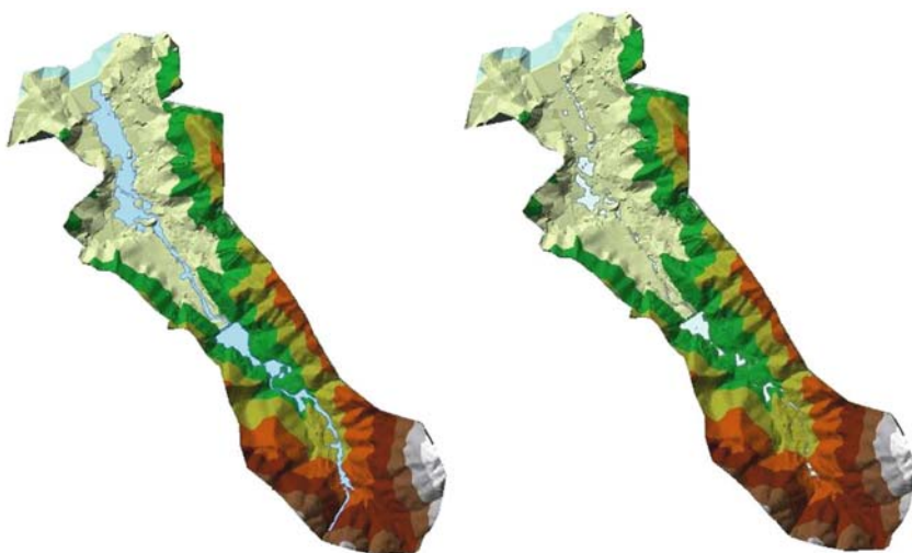
Fig. 2.37 Amount of water in summer (left) and winter (right) (Source: Bing et al., 2008b)
