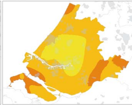
Fig. 2.9 Average summer precipitation (Source: Alterra et al., 2007)
