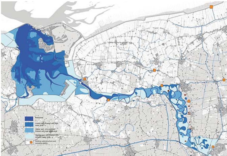
Fig. 8.13 Proposal for fresh water storage in Lauwers Lake (Meliefste et al., 2008)
