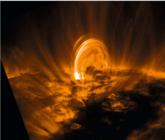
Fig. 6.8 Post-flare loops. This image was taken from the Transition Region And Coronal Explorer , abbreviated TRACE , telescope in the 17.1-nm passband sensitive to gas temperatures of about 1 \times 10^6 . It shows some post-flare loops, cooling after an M2 flare that started 2 h prior to this image. (Courtesy of Dawn Myers, the TRACE consortium and NASA; TRACE is a mission of the Stanford-Lockheed Institute for Space Research, and part of the NASA Small Explorer program.)
