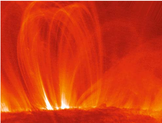
Fig. 4.4 Loops heated from below. Tall, thin coronal loops observed from the Transition Region And Coronal Explorer , abbreviated TRACE , satellite, taken on 9 August 1999, in the 17.1-nm passband sensitive to a temperature of about 1 million degrees. High arching loops stand out, to a height of approximately 120,000 km. The loops are visible along their entire length, and comparisons with the 19.5-nm observations indicate the temperature varies little along them. The fact that the temperature is so nearly constant along the length requires that most of the heating is concentrated low down, in the bottom 15,000 km or so. (Courtesy of the TRACE consortium and NASA. TRACE is a mission of the Stanford-Lockheed Institute for Space Research, and part of the NASA Small Explorer program.)
