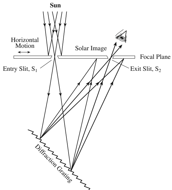
Fig. 2.2 Spectroheliograph.
