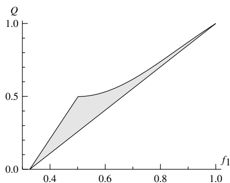
Figure 4.5. The optical ambiguity field for OD-micas. Depending on the relationship between fractions f_2 and f_3 one and the same value of Q corresponds to the certain range of the fraction f_1 contained within the shaded region
