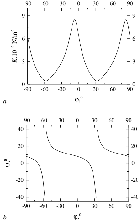
Figure 2.1. (a) The value of multiplier K in equation (2.38) and (b) the orientation of the principal axes of the stress tensor \psi as a function of orientation of the optic axial plane \varphi
