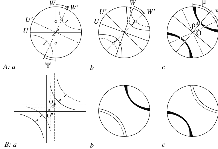
Figure 4.17. Appearance of isogyres during stage rotation. (A) Simultaneous appearance of the branches of the isogyre: (b, c) Successive positions of the stage rotating in the direction of the double unidirectional arrow from the extinction position of first component (a). Solid and dashed lines are the optical elements of the components misoriented by the angle \psi . Bold arrows denote directions of isogyres motion. B – alternate appearance of two isogyre branches. (a) direction of the isogyre branch motion (solid and dashed crosses – asymptotes of corresponding to isogyres, dot-dashed lines – cross hair position) (b, c) conoscopic figures for different orientations of the stage
