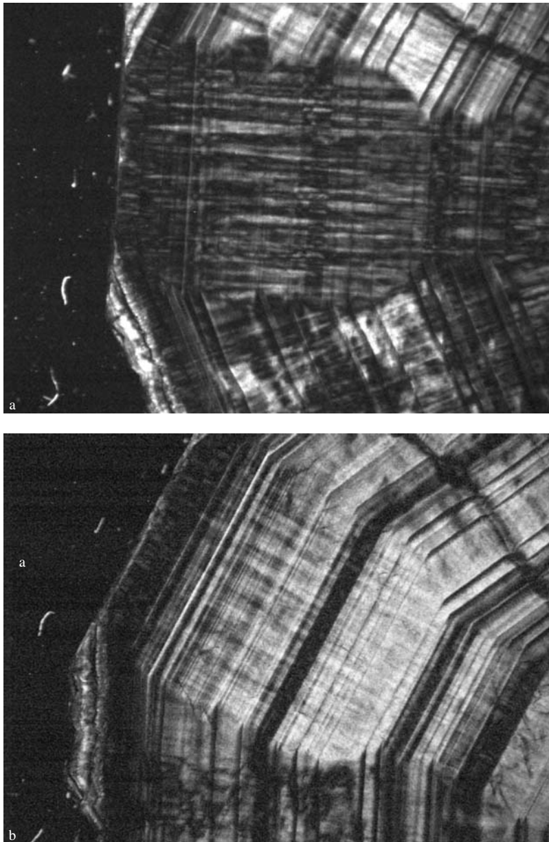
Figure 2.7. Birefringence bands in garnet \text{Ca}_3(\text{Al,Fe})_2(\text{SiO}_4)_3 from the Dalnegorsk mine, Far East, Russia. These bands originate from elastic stress on dislocation bundles and are directed normal to the growth front. (a) and (b) correspond to different crystal orientations relative to the crossed polarizers directed vertically and horizontally, respectively. The growth front positions are marked by numerous concentric zoning boundaries. Birefringence more or less homogeneously distributed over concentric zones is caused by growth desymmetrization (see Chapter 3). The sample was kindly provided by P.B. Sokolov (see Color Section following page 254)
