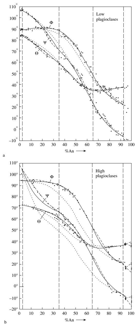
Figure 4.12. Euler angles \Phi , \Theta and \Psi describing the orientation of the optical indicatrix in relation to the crystal coordinates in plagioclase. Measured points interpolated (dashed line) are compared with the calculated curves assuming a solid solutions of An 2.5 and An 92.5 (dotted line) and ex-solutions with An 2.5 , An 35 , An 65 and An 92.5 (solid line). (a) low-plagioclase series, (b) high-plagioclase series (after Hauser and Wenk, 1976)
