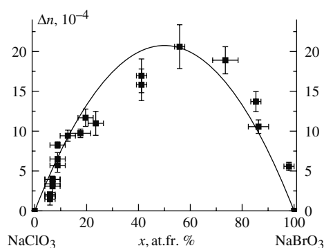
Figure 3.40. Anomalous birefringence in {100} growth sectors of sodium halate Na(Br_xCl_{1-x})O_3 solid solutions as a function of the average composition. Solid line is a parabola
