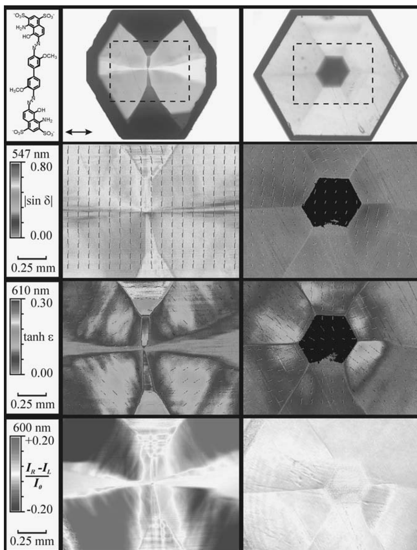
Figure 3.24. Chicago sky blue dyed LiKSO 4 crystals. Images in the left column are made along the [100] direction of 0.68 mm thick section, [001] is vertical. Images in the right column are made along the [001] of 0.38 mm thick section. (a, b) Photographs in light polarized along the arrow. Dotted, rectangular enclosures are imaged below. (c, d) Linear birefringence micrographs, \delta = 2\pi L\Delta n/\lambda . (e, f) Linear dichroism micrographs, \tanh \varepsilon = 2(T' - T'')/(T' + T'') . (g, h) circular extinction micrographs, (I_R - I_L)/I_0 . Source: Reprinted with permission from Claborn, K., Chu, A.S., Jang, S.H., Su, F., Kaminsky, W. and Kahr, B. "Circular Extinction Imaging: Determination of the Absolute Orientation of Embedded Chromophores in Enantiomorphously Twinned LiKSO 4 crystals" Cryst. Growth Des. 2005 , 5, p.2117–2123. Copyright 2005 American Chemical Society (see Color Section following page 254)
