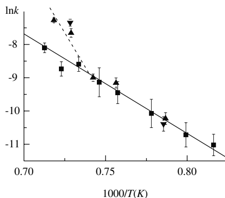
Figure 3.30. Arrhenius plot for the transformation from birefringent to isotropic {110} growth sectors of two grandite garnet crystals (squares and triangles, respectively)
