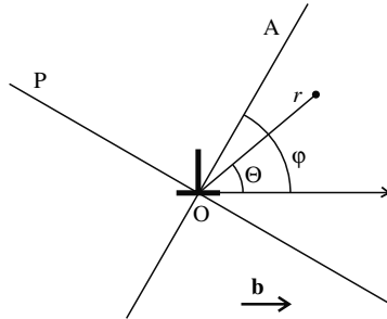
Figure 2.4. The edge dislocation in the cylindrical coordinate frame. b is the Burgers vector, P and A are the polarizer and analyzer, respectively
