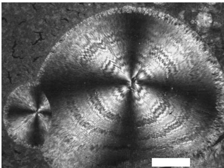
Figure 1.10. Hippuric acid ( \text{C}_6\text{H}_5\text{CONHCH}_2\text{COOH} ) spherulites between crossed polarizers. An extinction cross, typical for spherulites, arises when the refracting components are parallel with either the crossed polarizer or analyzer. The concentric banding is best accounted for by assuming fibrous crystallites twisting about the radius. Scale bar = 0.44 mm (see Color Section following page 254)
