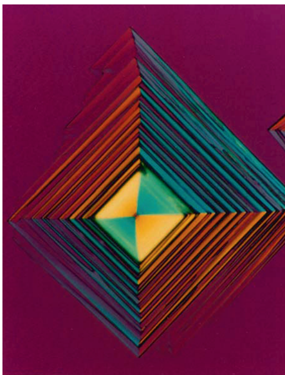
Figure 3.18. Photomicrograph of 1,5-dichloro-2,3-dinitrobenzene grown from chloroform. Crystal between crossed polarizers with a first order red retarder in the diagonal position. Diagonal width = 0.24 mm. Thickness = 0.024 mm at perimeter of central bright square
