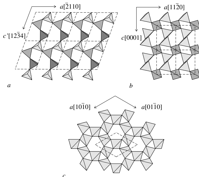
Figure 3.32. \alpha -Quartz planes: (a) (01\bar{1}) , (b) (\bar{1}120) and (c) (0001) (Tsinober and Samoilovich, 1975). \text{SiO}_4 tetrahedra which are marked by different levels of the gray scale have different orientations with respect to growth face and different vacancy levels
