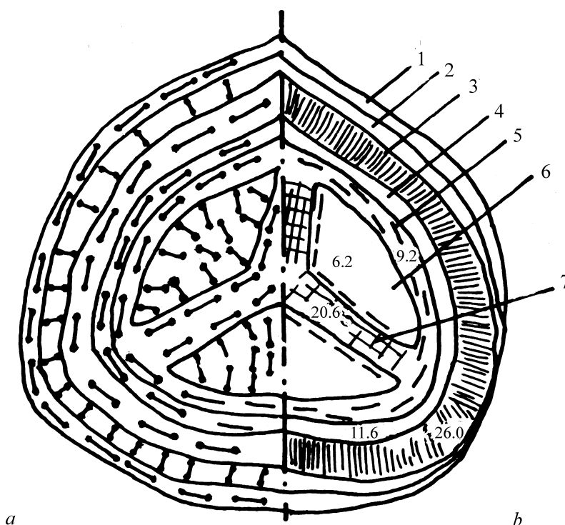
Figure 2.29. (a) Orientation of the optic axial plane and (b) preferable crack orientations in a zoned (0001) polychrome tourmaline section (after Gorskaya et al. , 1992). The cracking coefficient (cracks per unit volume) is shown for the inner zones. Zones are numbered at right
