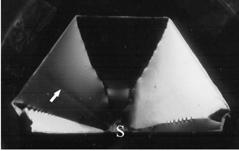
Figure 2.6. Birefringence bands (shown by arrow) related to a dislocation bundle in alum (K_{0.5}(NH_4)_{0.5})Al(SO_4)_2 \cdot 12H_2O . This bundle, formed at the seed (S), lies perpendicular to the growth front (111) and to the growth zones. The variation of indicatrix orientations in growth sectors is a consequence of growth dissymmetrization (see Chapter 3)
