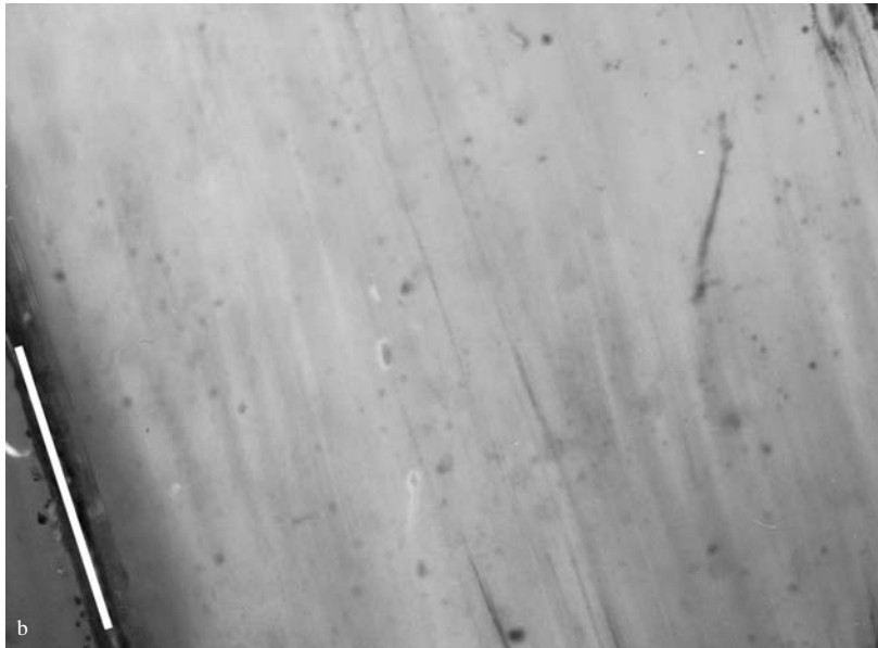
Figure 3.8. (a) Subsector zoning in alum (K_{0.77}Rb_{0.23})Al(SO_4)_2 \cdot 12H_2O {111}, section parallel to (111) growth face. Sub-sector boundaries shown by bold lines are the boundaries between different vicinal faces on the crystal surface. Sub-sector boundaries shown by thin lines are observed between crossed polarizers. Numbers denote birefringence \times 10^{-7} . (b) The same crystal with section through the center of (111) face parallel to the growth direction [111] between crossed polarizers and with a first order red retarder. White line marks position of (111) face (see Color Section following page 254)
