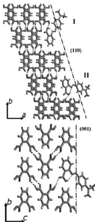
Figure 3.36. Simulations of methyl red ((\text{CH}_3)_2\text{N}-\text{C}_6\text{H}_4-\text{N}=\text{N}-\text{C}_6\text{H}_5\text{CO}_2\text{H}) docking to two distinct sites (I) and (II) on the asymmetric (110) surface above and the one unique site on the (001) with local symmetry m . Black dashed lines denote lowest energy stable surfaces for the indicated facets Source: Reprinted with permission from Benedict, J.B., Cohen, D.E., Lovell, S., Rohl, A.L. and Kahr, B. "What is syncrystallization? States of pH indicator methyl red in single phthalic acid crystals" J. Am. Chem. Soc. , 2006, 128, p.5548–5559 Copyright 2003 American Chemical Society (see Color Section following page 254)
