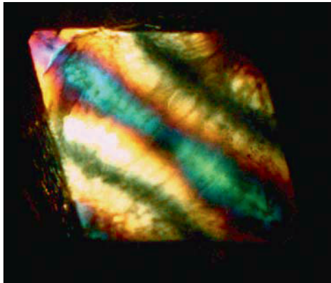
Figure 4.2. Anomalous birefringence in \text{NH}_4\text{Cl} related to syntactic intergrowth with \text{MnCl}_2 \cdot (\text{NH}_4\text{Cl})_2 \cdot 2\text{H}_2\text{O} . Crystal size \sim 0.8\text{ mm}
