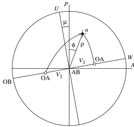
Figure 4.16. The view field of conosccope. P , A - orientations of vibration directions in polarizers, OA - outcrops of the optic axes, AB and OB denote acute and obtuse bisectrices, respectively. Direction W lies in the optical axial plane, U is normal to the optic axial plane
