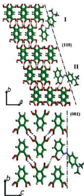
Figure 3.36. Simulations of methyl red ( ((\text{CH}_3)_2\text{N}-\text{C}_6\text{H}_4-\text{N}=\text{N}-\text{C}_6\text{H}_5\text{CO}_2\text{H}) ) docking to two distinct sites (I) and (II) on the asymmetric (110) surface above and the one unique site on the (001) with local symmetry m . Black dashed lines denote lowest energy stable surfaces for the indicated facets Source: Reprinted with permission from Benedict, J.B., Cohen, D.E., Lovell, S., Rohl, A.L. and Kahr, B. "What is syncrystallization? States of pH indicator methyl red in single phthalic acid crystals" J. Am. Chem. Soc. , 2006, 128, p.5548–5559 Copyright 2003 American Chemical Society
