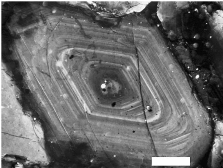
Figure 1.5. Concentric, compositional zoning of plagioclase (\text{Na}, \text{Ca})(\text{Al}, \text{Si})_4\text{O}_8 from crystal-lapilli (volcano B. Tolbachek, Kamchatka, Russia). Variation in albite ( \text{NaAlSi}_3\text{O}_8 ) to anorthite ( \text{CaAl}_2\text{Si}_2\text{O}_8 ) ratio manifests itself in variations of birefringence and extinction position. Scale bar = 0.22 mm (see Color Section following page 254)
