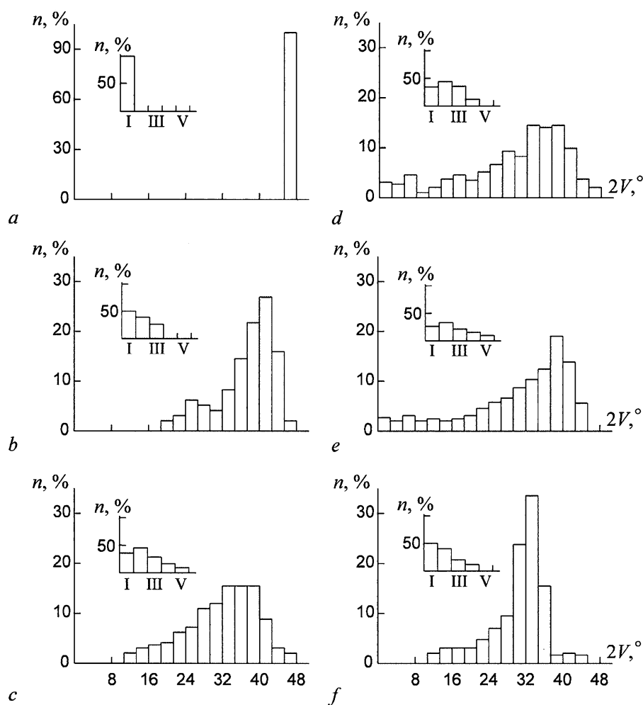
Figure 4.30. Effect of the chemical composition on the axial angle 2V and on the distortions of the conoscopic figures (I–V) for the lithium-aluminum micas. Content of \text{Li}_2\text{O} (%): (a) less 0.7, (b) 0.7–1.2, (c–e) 1.2–4.0, (f) 4.0–5.8
