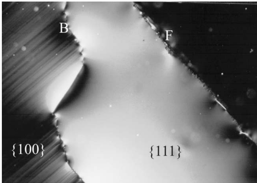
Figure 2.41. Anomalous birefringence in alum (K, NH_4)Al(SO_4)_2 \cdot 12H_2O . B is the sector boundary, F is a crack. Horizontal = 6.5 mm
