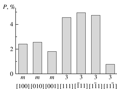
Figure 3.17. Percent of cubic equivalent reflections that violate I_{\max} - I_{\min} > 2(I_{hkl} - I_{\bar{h}\bar{k}\bar{l}})_{\max} . The trigonal symmetry is supported by the slight violation of one three-fold axis compared with the other three-fold axes and also with all mirror planes
