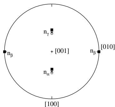
Figure 3.22. Orientation of the optical indicatrix in two solid solutions of \text{Na}(\text{Cl}, \text{Br})\text{O}_3 . Stars correspond to the observed optical indicatrix, circles and squares represent calculations
