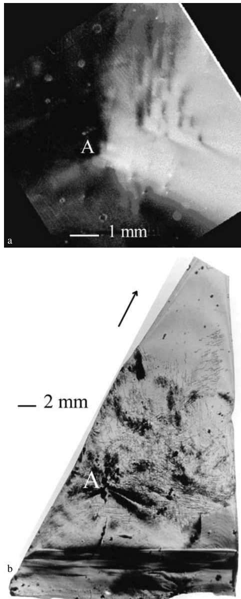
Figure 3.9. Sub-sector zoning in alum ( \text{K}_{0.5}(\text{NH}_4)_{0.5}\text{Al}(\text{SO}_4)_2 \cdot 12\text{H}_2\text{O} ) section parallel to the (111) growth face. (a) Anomalous birefringence around the apex of vicinal hillock (A). (b) X-ray diffraction topograph. The arrow indicates diffraction vector \mathbf{g} for reflection 220
