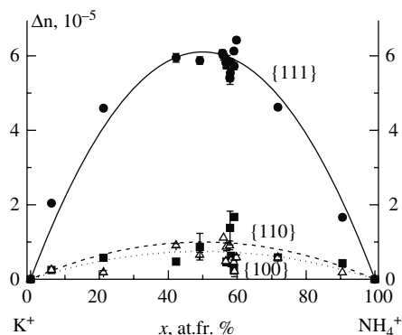
Figure 3.39. Anomalous birefringence in alums (K_{1-x}(NH_4)_x)Al(SO_4)_2 \cdot 12H_2O as a function of the average crystal composition. Growth sectors: \{111\} = circles, \{110\} = squares, \{100\} = triangles. Lines represent parabolic fits
