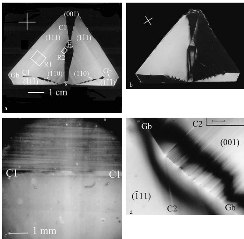
Figure 3.6. Optical inhomogeneity of alum, (K_{0.5}(NH_4)_{0.5}Al(SO_4)_2 \cdot 12H_2O) . The \{110\} section was cut through the center of the crystal. (a) and (b) have different orientations with respect to the crossed polarizers. Optical orientations are indicated by crossed white lines. The birefringence is strong in \{111\} growth sectors and weak in \{110\} and \{100\} . In \{111\} growth sectors, the X vibration direction is always normal to the growth front direction. Some growth sector boundaries are marked by Gb, S = seed crystal, H = solution inclusion. Regions R1 and R2 are magnified in (c) and (d), respectively. They display fine zoning related to unstable growth and changes of step sources. Horizontal stripes in (c) are associated with dislocation stresses. The boundaries C1-C1 and C2-C2 mark a supersaturation jump and the cessation of crystal rotation for one hour, respectively. Scale bar in (c) = 0.38 mm
