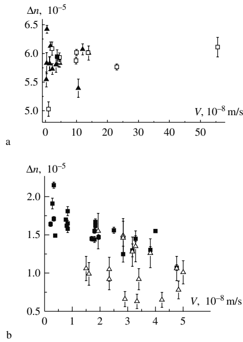
Figure 3.46. Anomalous birefringence in alum crystals as a function of growth rate. (a) Series (K_{1-x}(NH_4)_x)Al(SO_4)_2 \cdot 12H_2O , triangles correspond to x = 0.55-0.60 ( T = 28-30^\circ C ); squares correspond to x = 0.36-0.42 ( T = 29.5-32^\circ C ). (b) Series K(Al_{1-x}Cr_x)(SO_4)_2 \cdot 12H_2O , triangles correspond to x = 0.03-0.05 ( T = 24-37^\circ C ); squares correspond to x = 0.04-0.05 ( T = 34-36^\circ C ). Open symbols correspond to growth under free convection. Solid symbols correspond to growth under strong solution stirring (Reynolds number Re = 1400-3200 )
