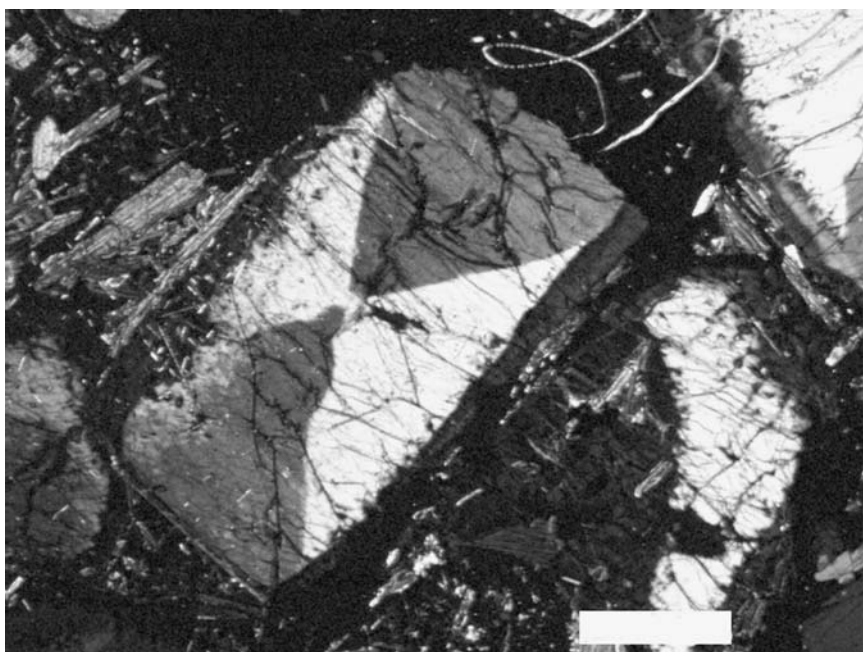
Figure 1.7. Growth sector zoning in birefringence in eudialyte (\text{Na}_4(\text{Ca}, \text{Ce}, \text{Fe}, \text{Mn})_2\text{ZrSi}_6\text{O}_{17}(\text{OH}, \text{Cl})_2) related to variations of chemical composition. Scale bar = 0.88 mm (see Color Section following page 254)
