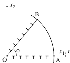
Figure 2.38. Representaion of sector boundaries by plane dislocation ensembles
