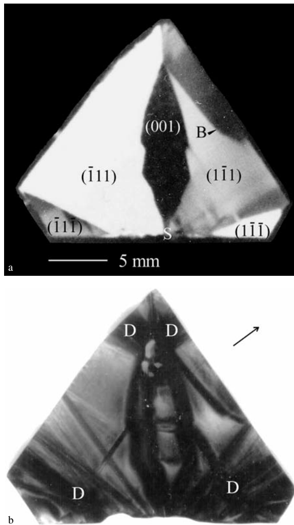
Figure 3.12. Sub-sector zoning in alum (K(Al_{0.5}Cr_{0.5})(SO_4)_2 \cdot 12H_2O) . S = seed, B = sub-sector boundary that separates two regions formed by steps from different vicinal hillocks. (a) Anomalous birefringence. (b) X-ray diffraction topograph. The arrow indicates the diffraction vector \mathbf{g} for reflection 333. D - bundles of dislocations originating from the seed and solution inclusions
