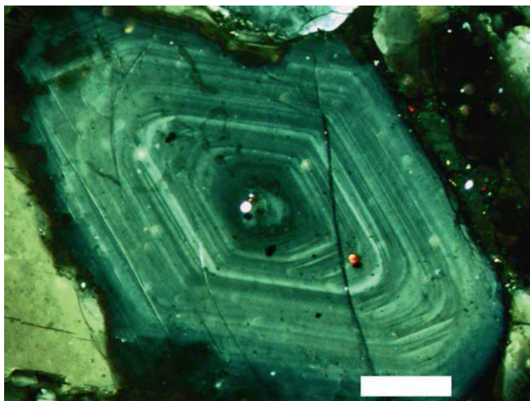
Figure 1.5. Concentric, compositional zoning of plagioclase ((\text{Na}, \text{Ca})(\text{Al}, \text{Si})_4\text{O}_8) from crystal-lapilli (volcano B. Tolbachek, Kamchatka, Russia). Variation in albite ( \text{NaAlSi}_3\text{O}_8 ) to anorthite ( \text{CaAl}_2\text{Si}_2\text{O}_8 ) ratio manifests itself in variations of birefringence and extinction position. Scale bar = 0.22 mm
