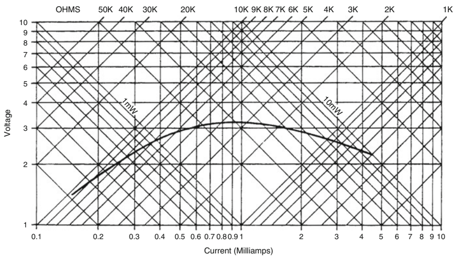
Fig. 16.14 Voltage–current characteristic of an NTC thermistor in still air at 25°C (curvature of the characteristic is due to a self-heating effect)
