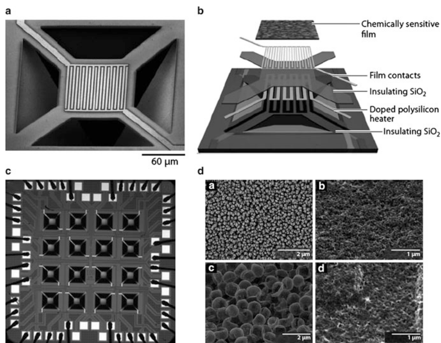
Fig. 17.25 Top view of a single chemical-sensor element (a); expanded schematic of the critical components of the microsensor device (b); a 16-element microsensor array (c); and scanning electron microscope images of a variety of chemically sensitive films deposited on microhot-plate-sensor platforms; and (d) images are shown at different scales to highlight each film’s nanostructure and morphology: (a) Polycrystalline metal-oxide films deposited via chemical vapor deposition. Shown here is tin oxide ( \text{SnO}_2 ); titanium oxide ( \text{TiO}_2 ), \text{TiO}_2 layered on \text{SnO}_2 , and ruthenium (Ru) deposited on \text{TiO}_2 have also been used. (b) Mesoporous \text{TiO}_2 film applied by drop coating. (c) Drop-coated shells of \text{Sb}:\text{SnO}_2 . (d) Electrophoretically deposited nanostructured conductive polymer (here, colloidal polyaniline). Courtesy of Dr. Steve Semancik, NIST (stephen.semancik@nist.gov)
