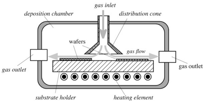
Fig. 18.7 Simplified structure of a CVD reactor chamber
