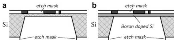
Fig. 18.13 Micromachining of a diaphragm or membrane
