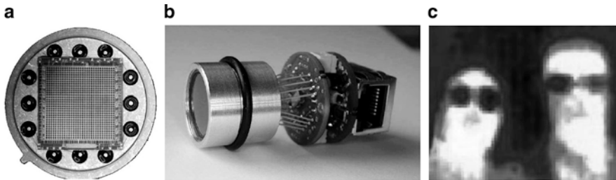
Fig. 14.21 Thermopile thermal-imaging sensor: sensing surface (a); imaging module (b); and example of a thermal image (c) (courtesy of Heimann Sensors, www.heimansensor.com )
