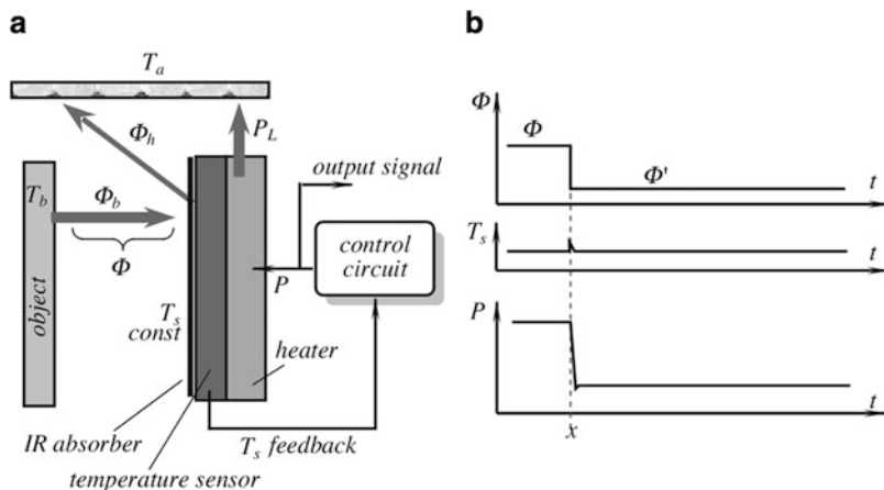
Fig. 14.29 AFIR element radiates thermal flux \Phi_n toward its housing and absorbs flux \Phi_b from the object (a); timing diagrams for radiative flux, surface temperature, and supplied power (b)
