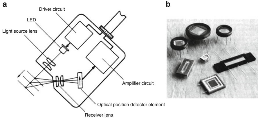
Fig. 7.40 Optical position displacement sensor (a) (From Keyence Corp. of America, Fair Lawn, NJ); one- and two-dimensional PSD sensing elements (b)
