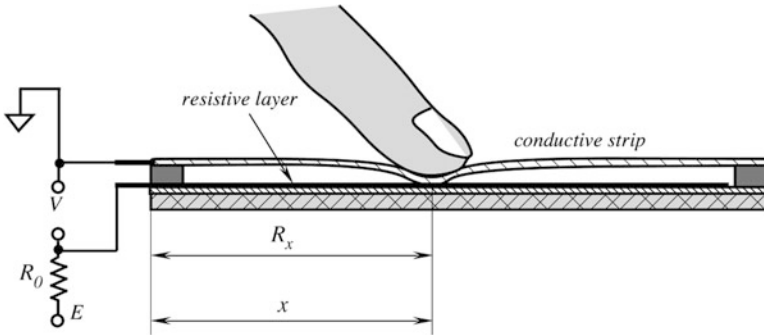
Fig. 7.3 Principle of a pressure-sensitive potentiometric position sensor
